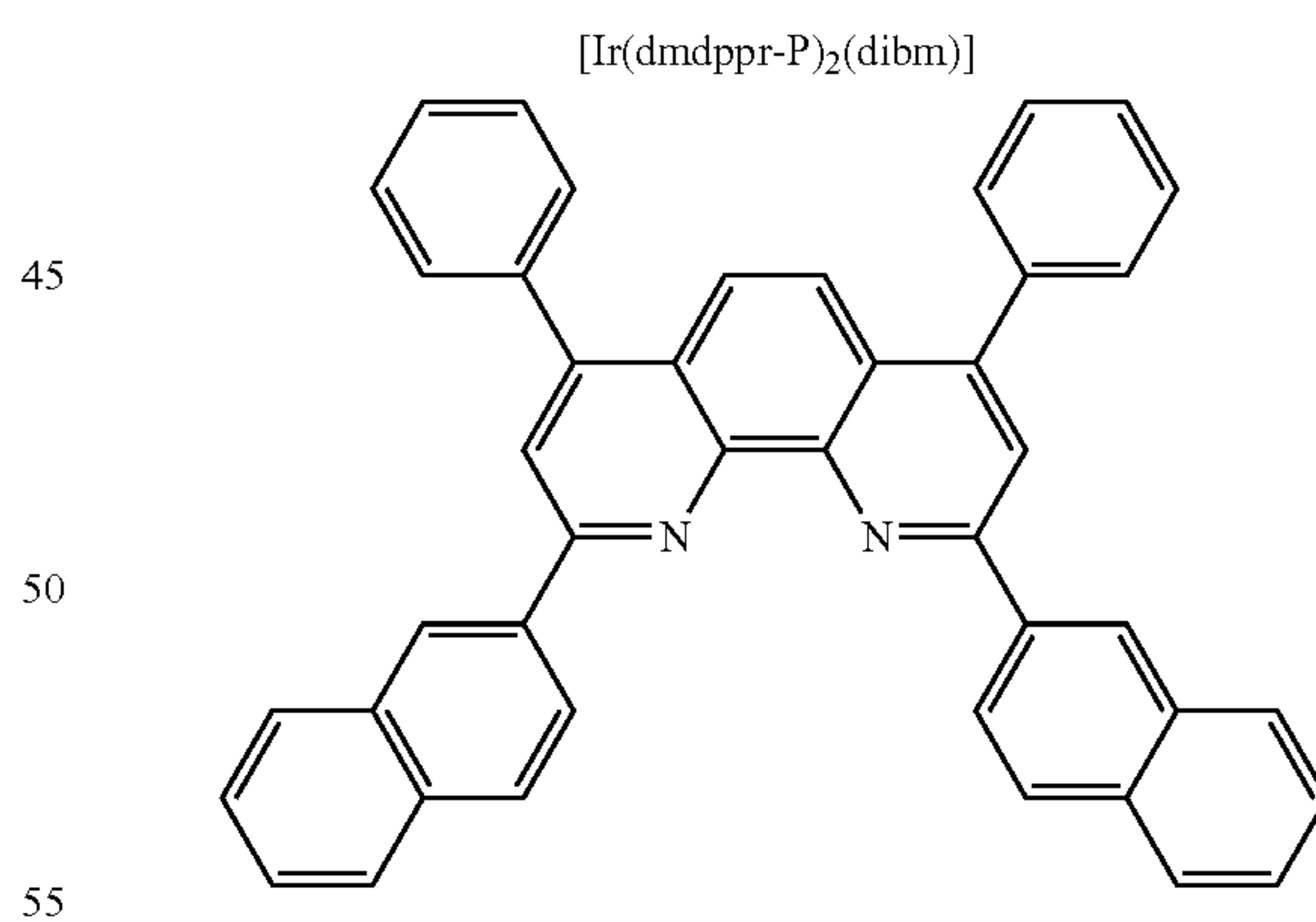
NBphen
