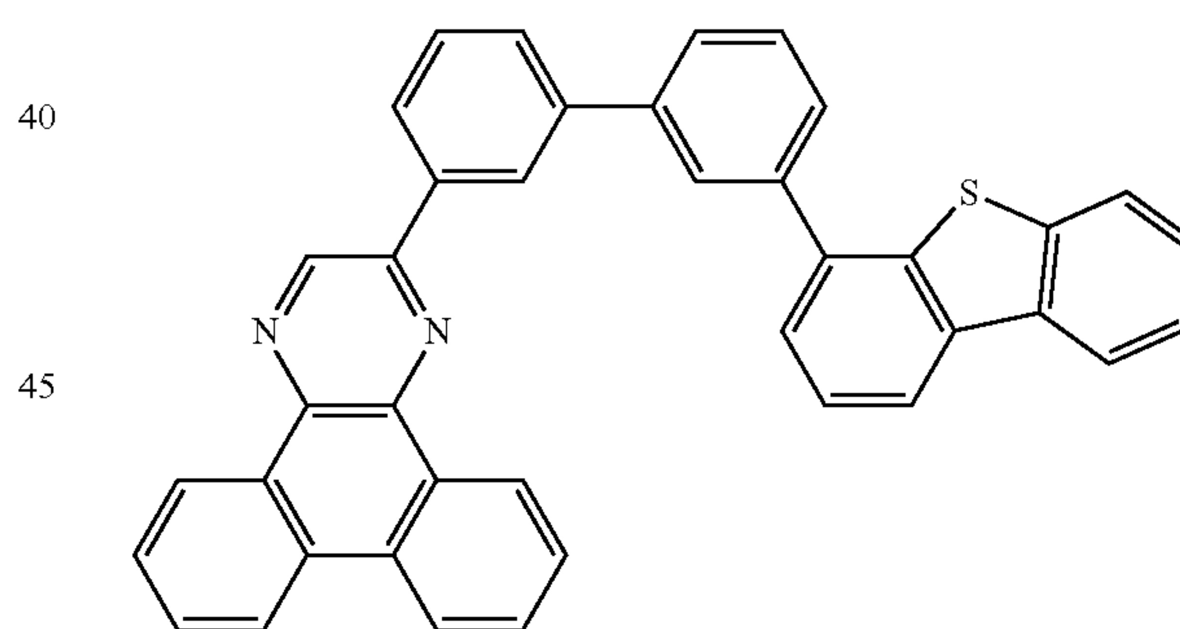
2mDBTBPDq-II
