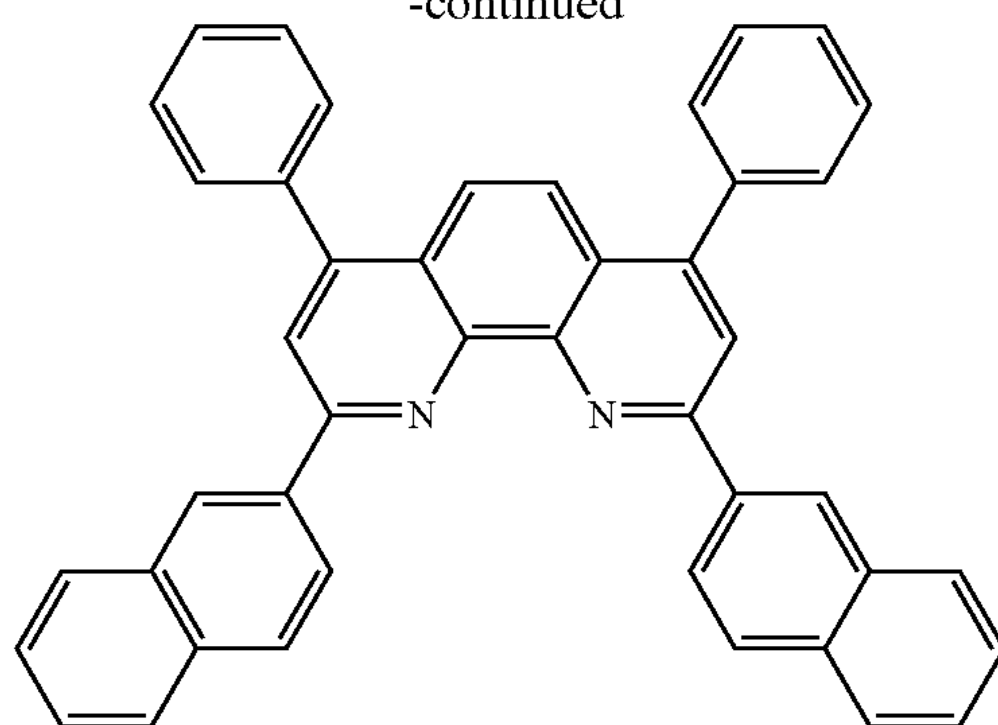
NBphen
