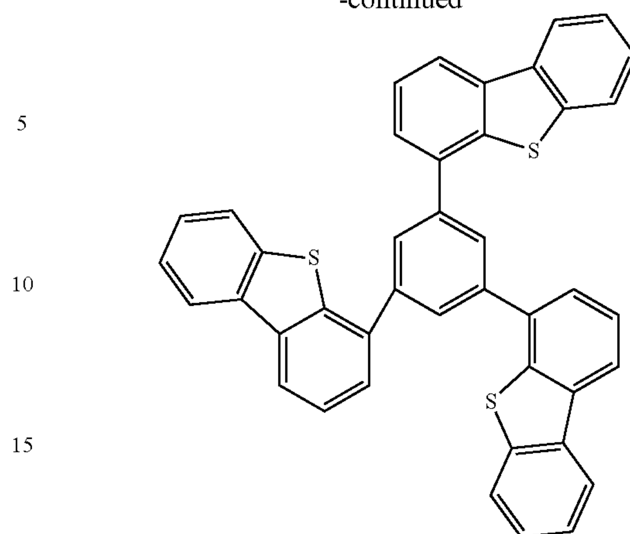
DBT3P-II
