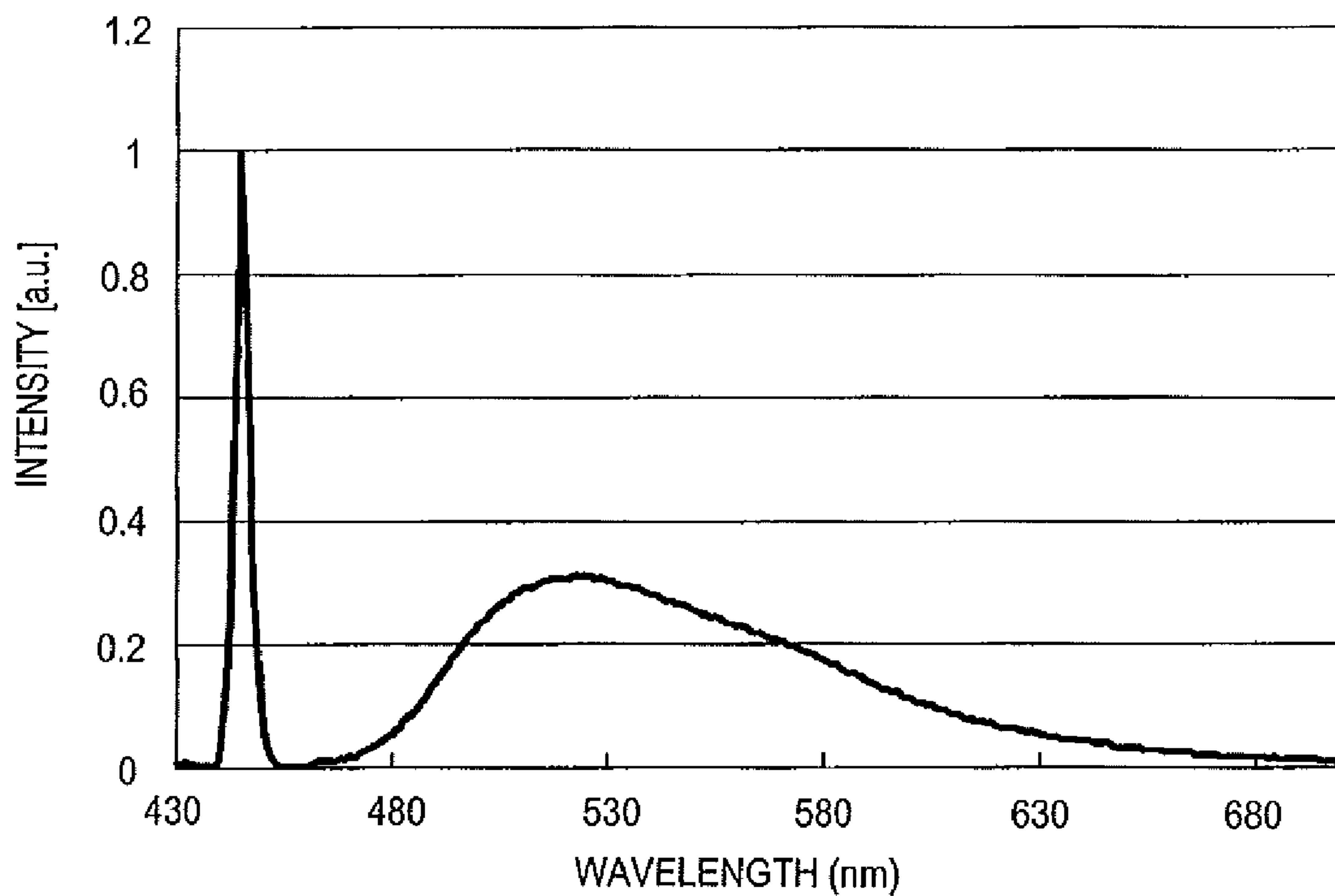
SPECTRAL CHARACTERISTIC OF EMITTED LIGHT
