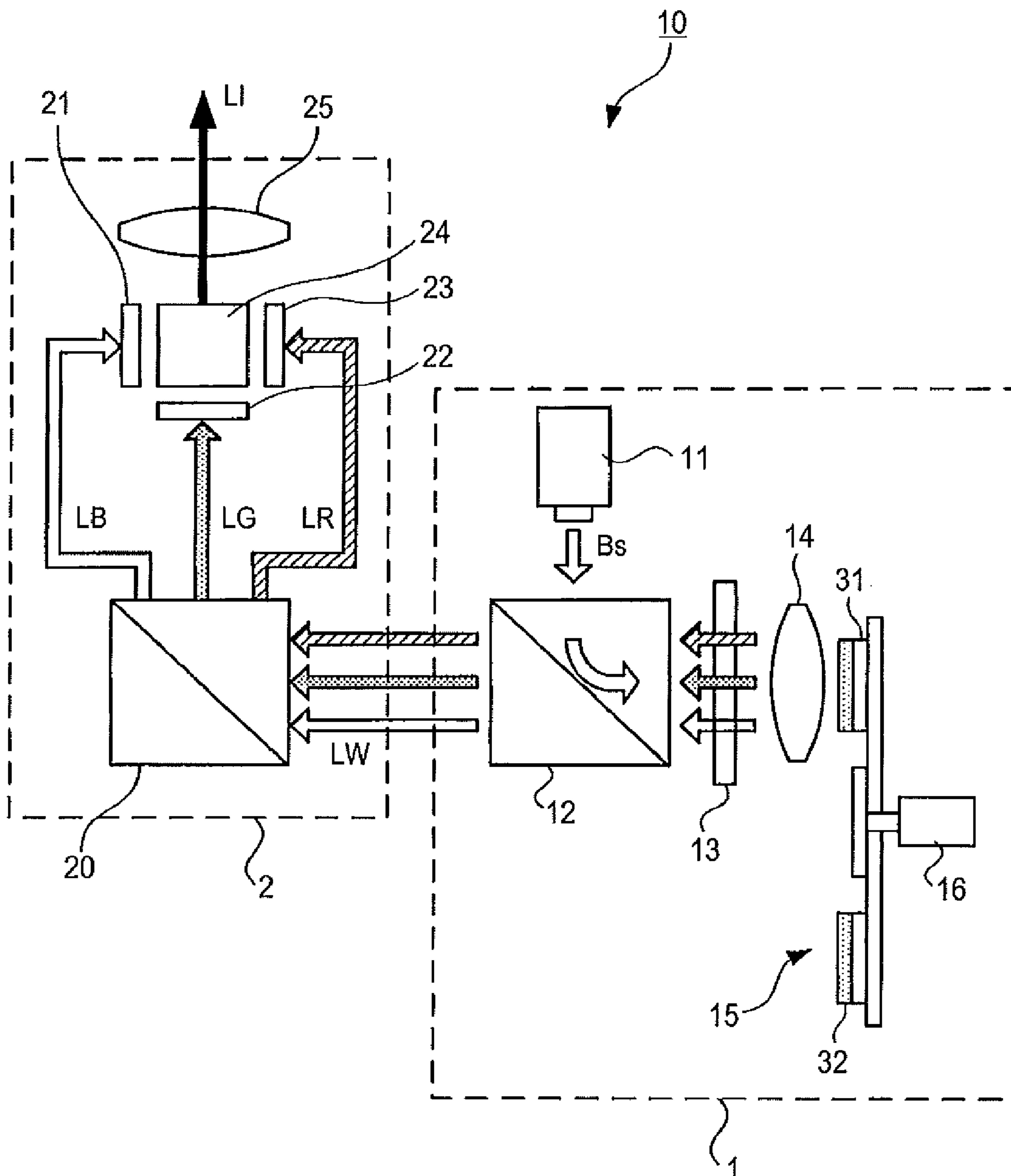
CONFIGURATION EXAMPLE OF IMAGE DISPLAY APPARATUS
