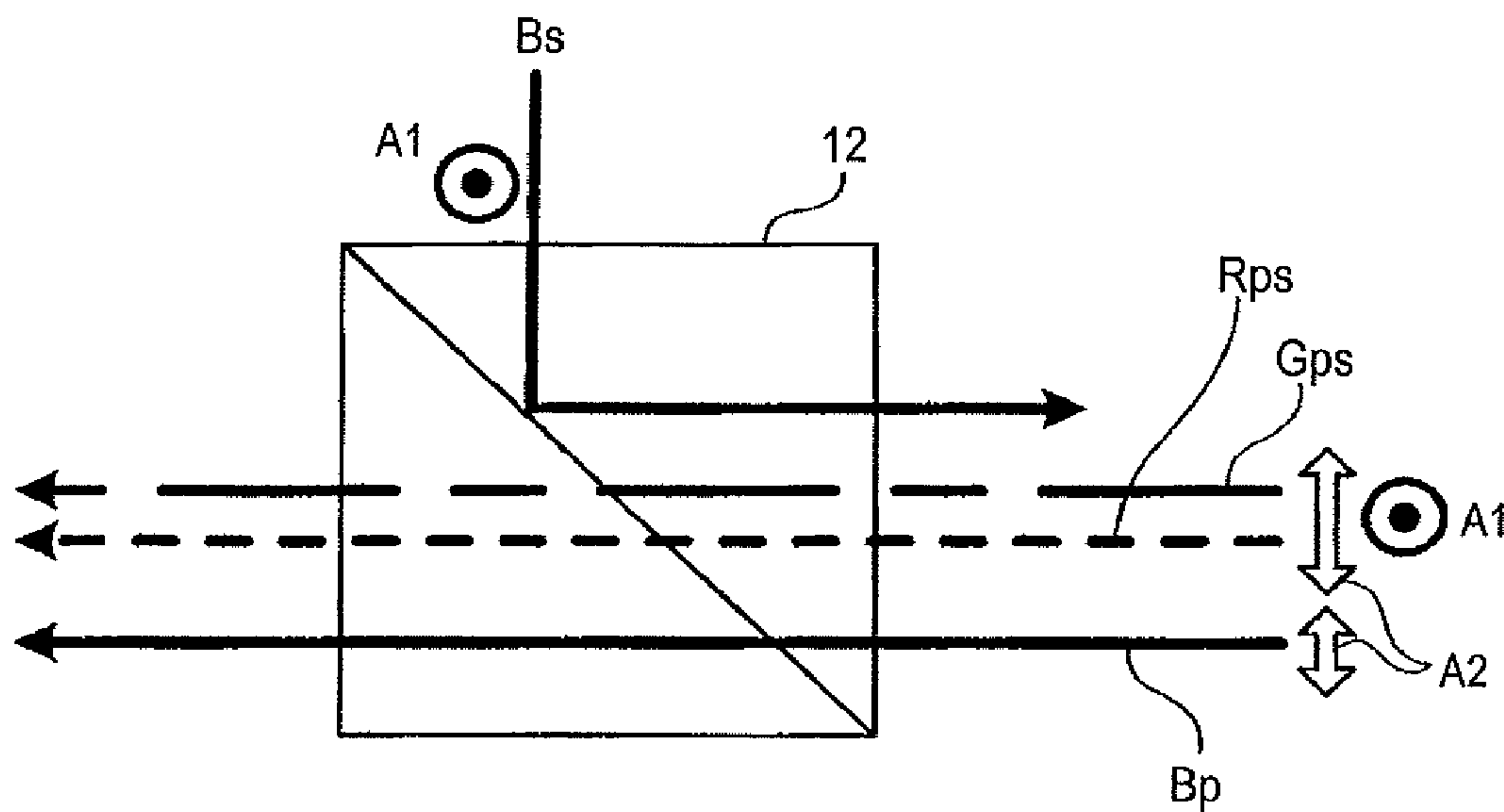
OPERATION OF POLARIZATION SPLITTER
