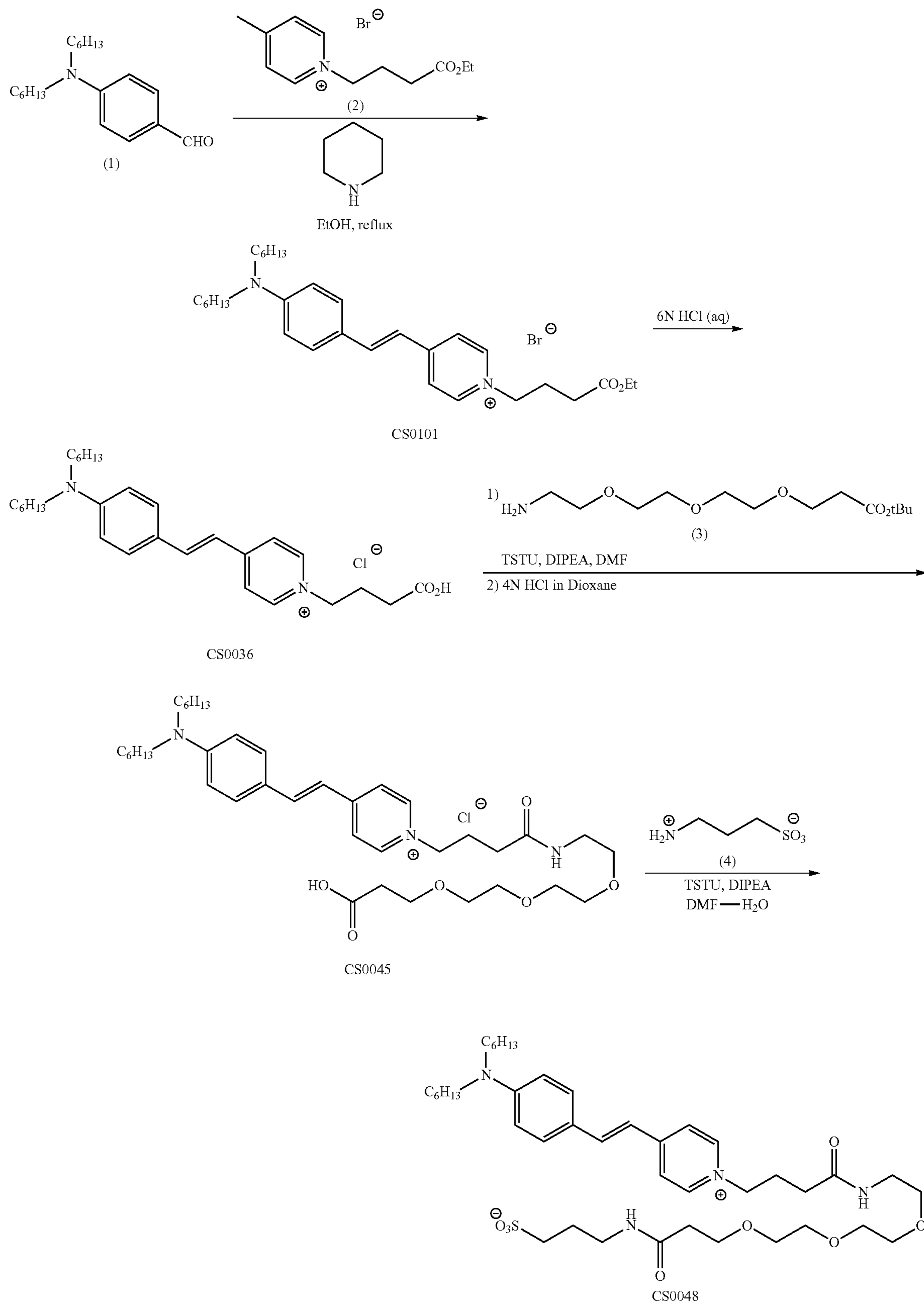
Scheme 1
