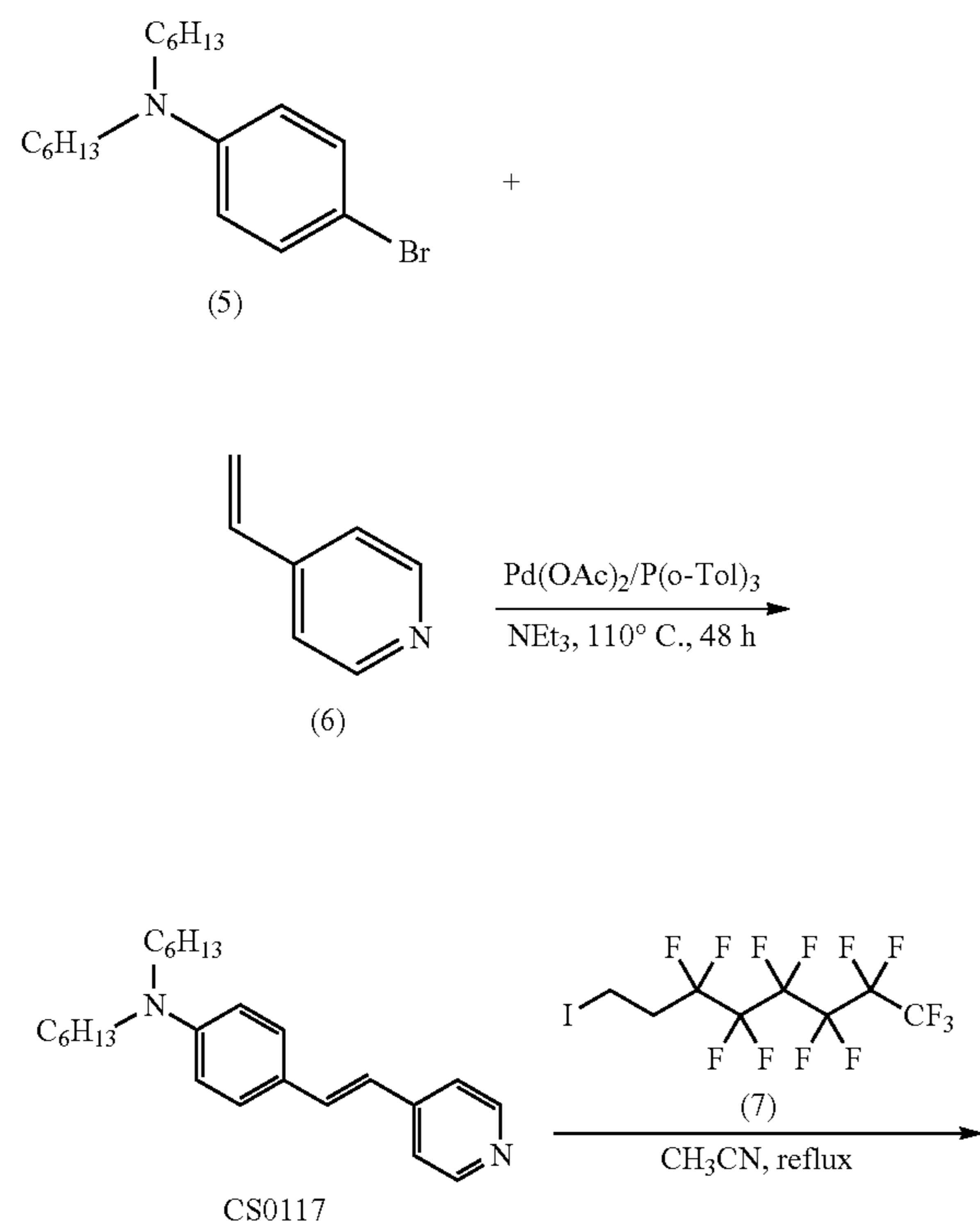
Scheme 3
