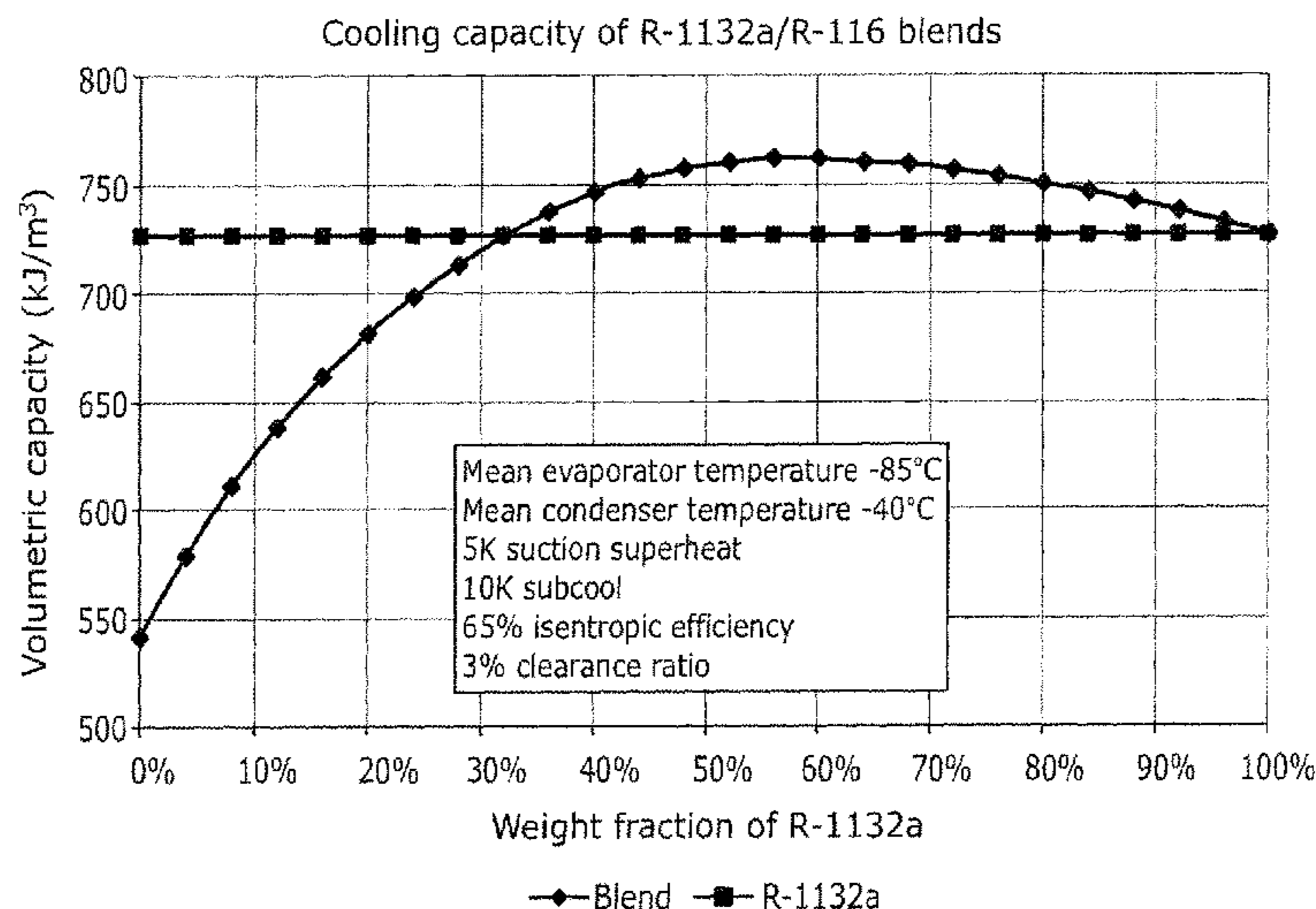
Calculated refrigeration cycle performance for R-1132a/R-116 mixtures
