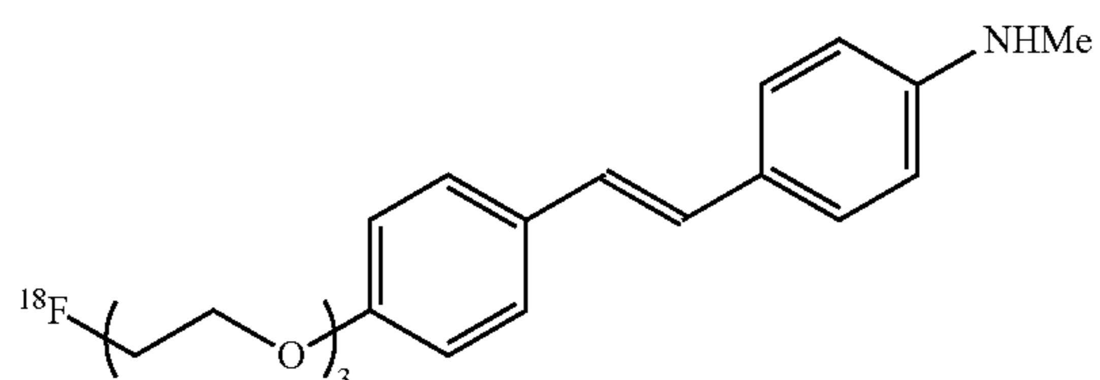
[ 18 F]florbetaben (clogP = 4.12)
