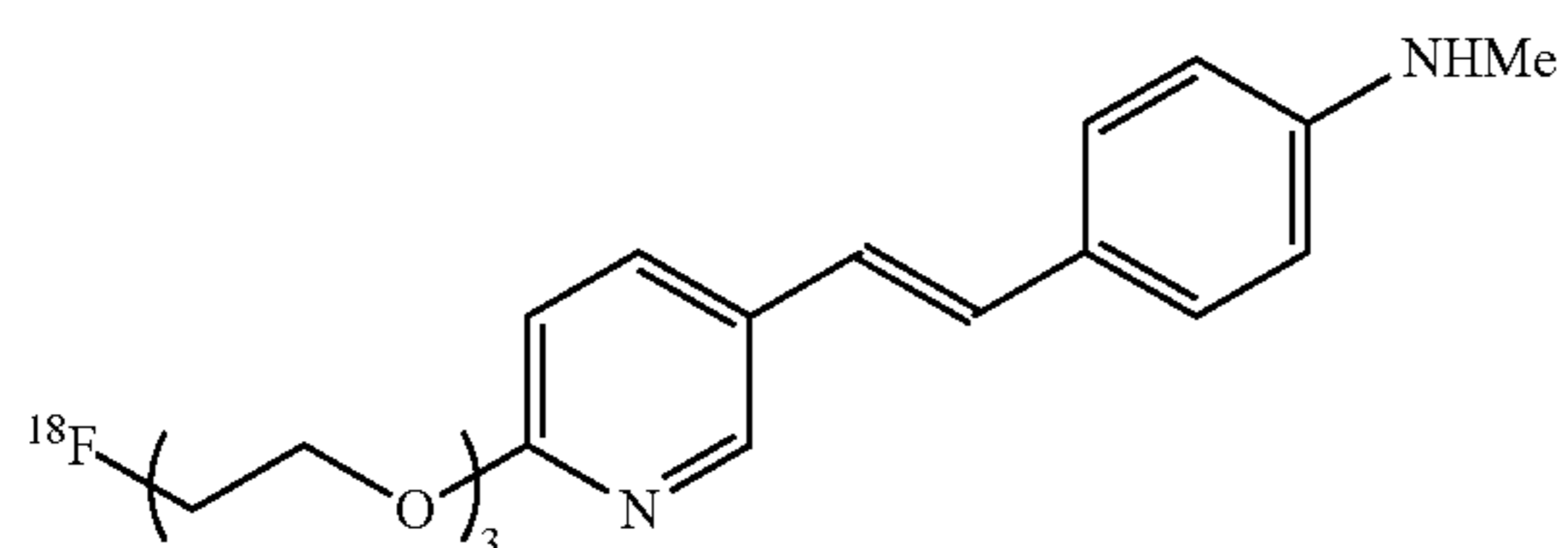
[ 18 F]florbetapir (clogP = 3.52)
