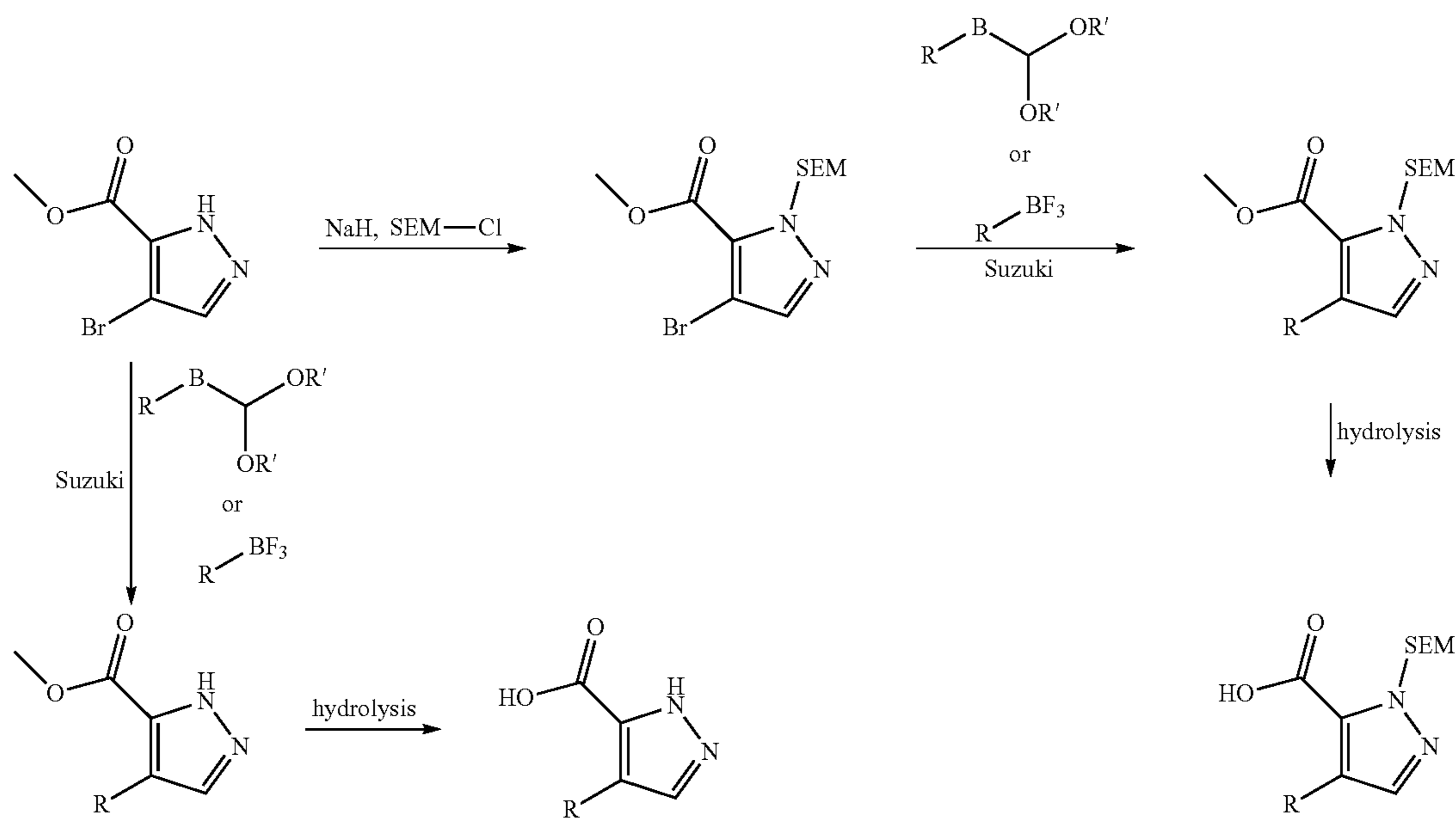
Scheme 2: synthesis of 4-substituted pyrazole derivatives
