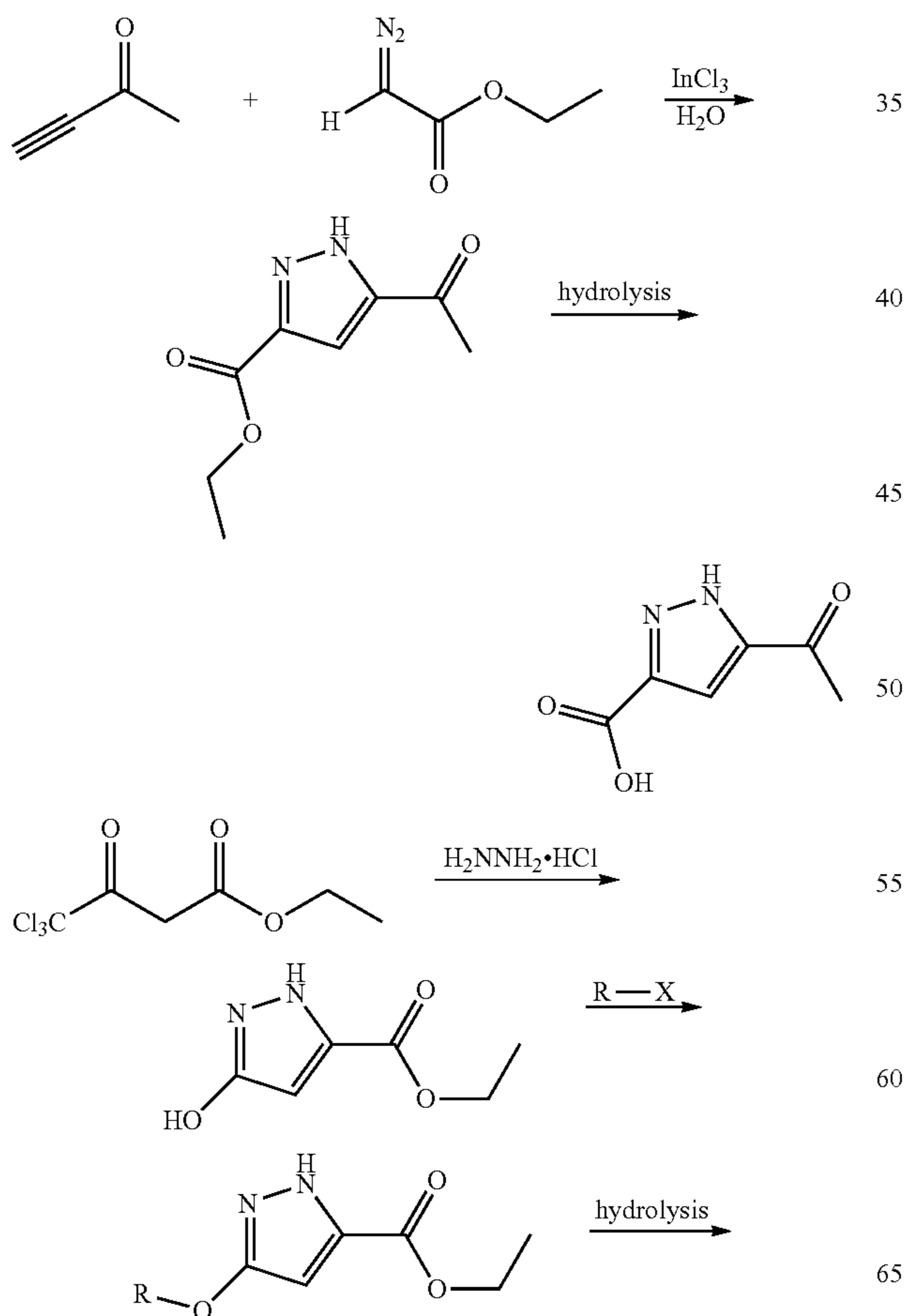
Scheme 3: synthesis of 3-substituted pyrazole derivatives
