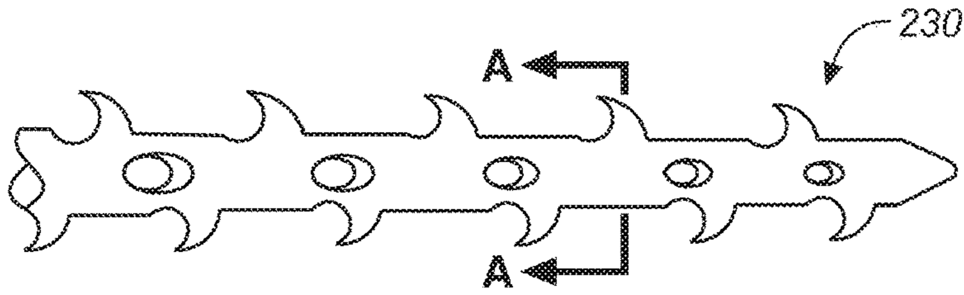
FIG. 2C (PRIOR ART)
