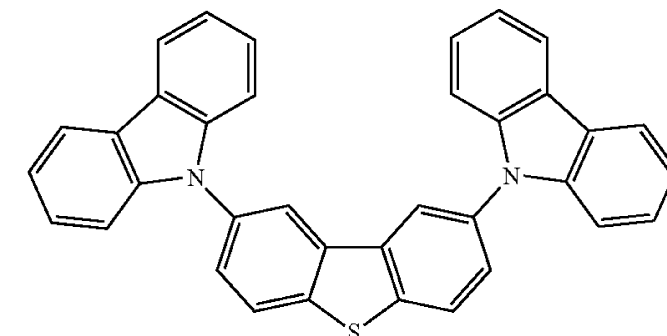
Compound C
