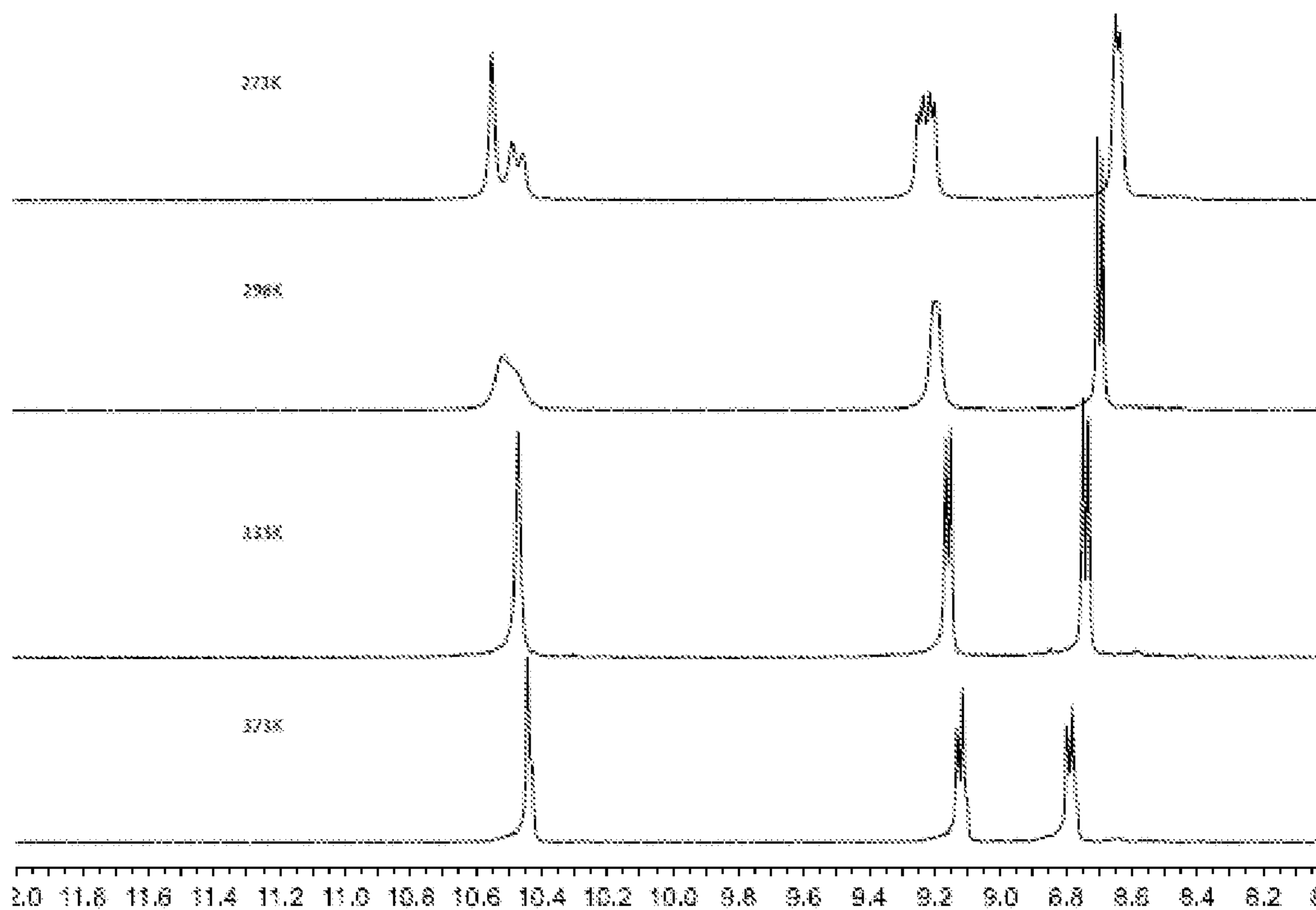
(A) Dimer (Compound 1)
