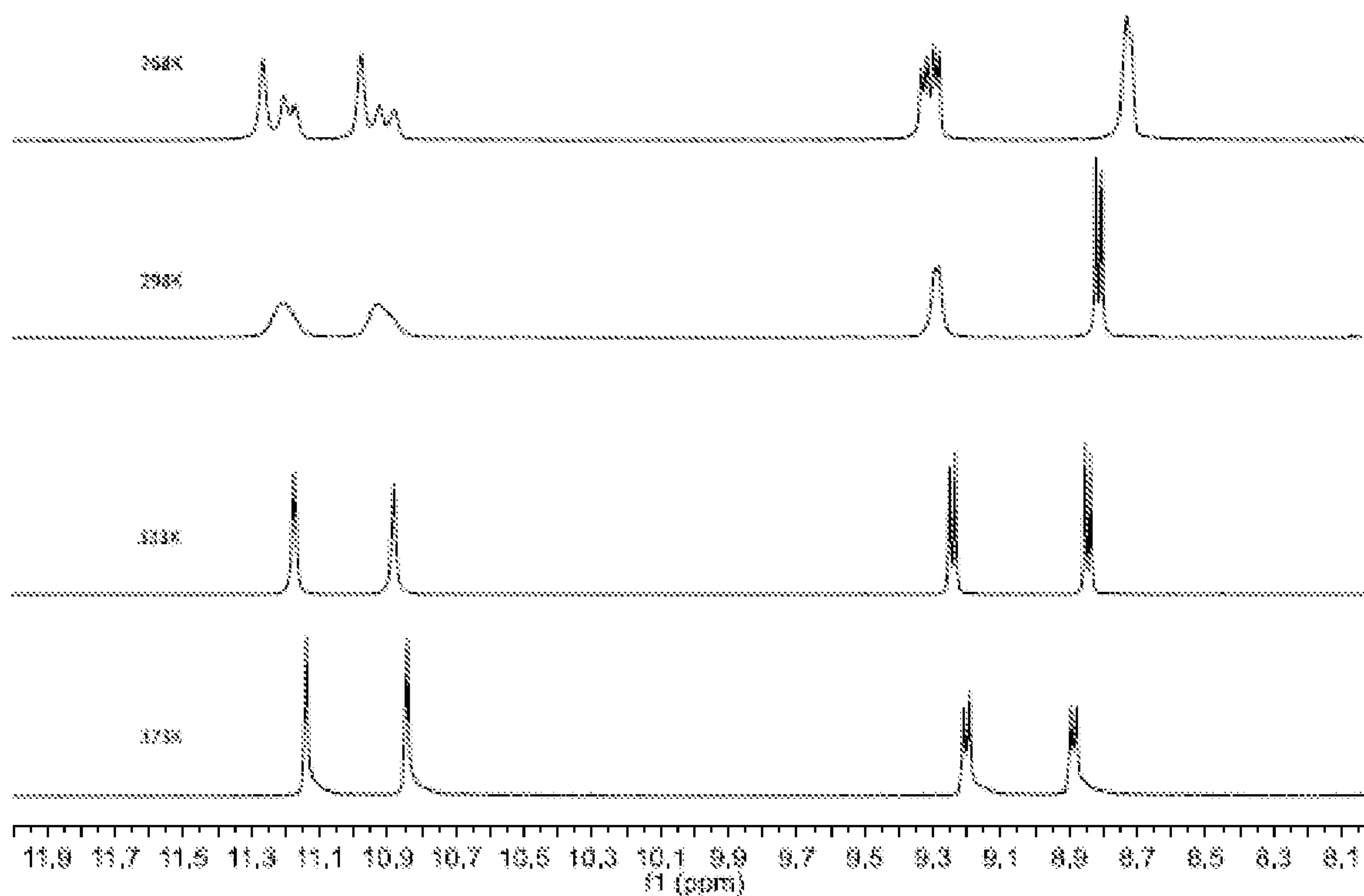
(B) Trimer (Compound 2)
