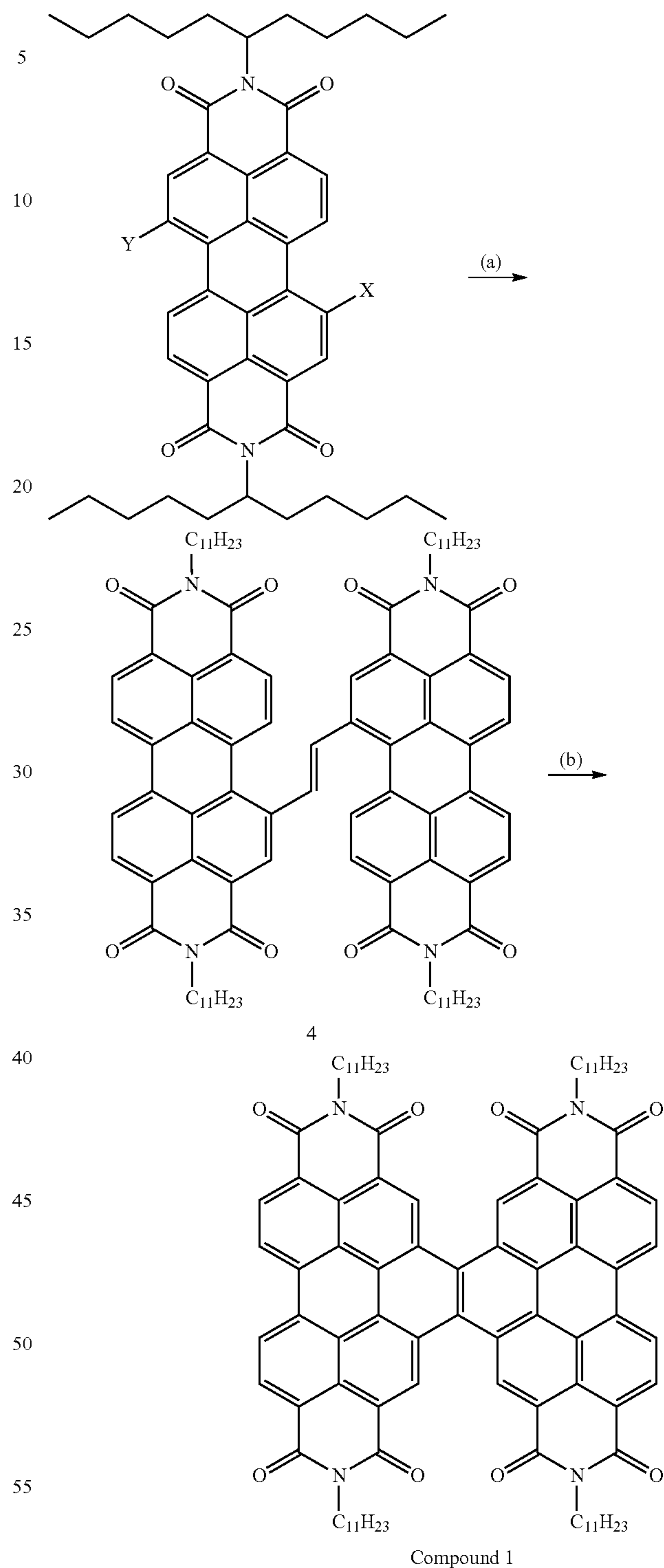
Scheme 1. Synthesis of Dimer (Compound 1):
