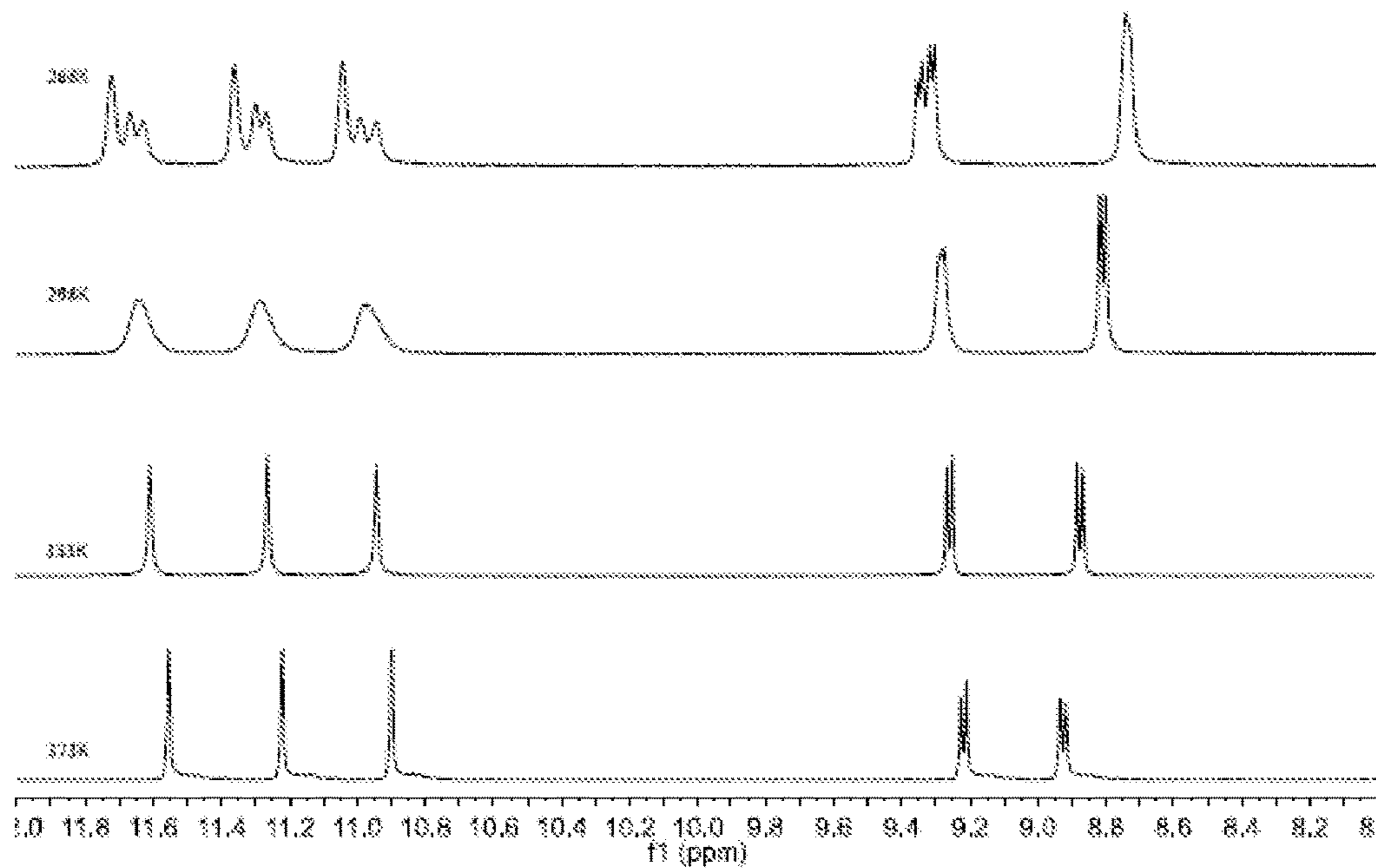
(C) Tetramer (Compound 3)
