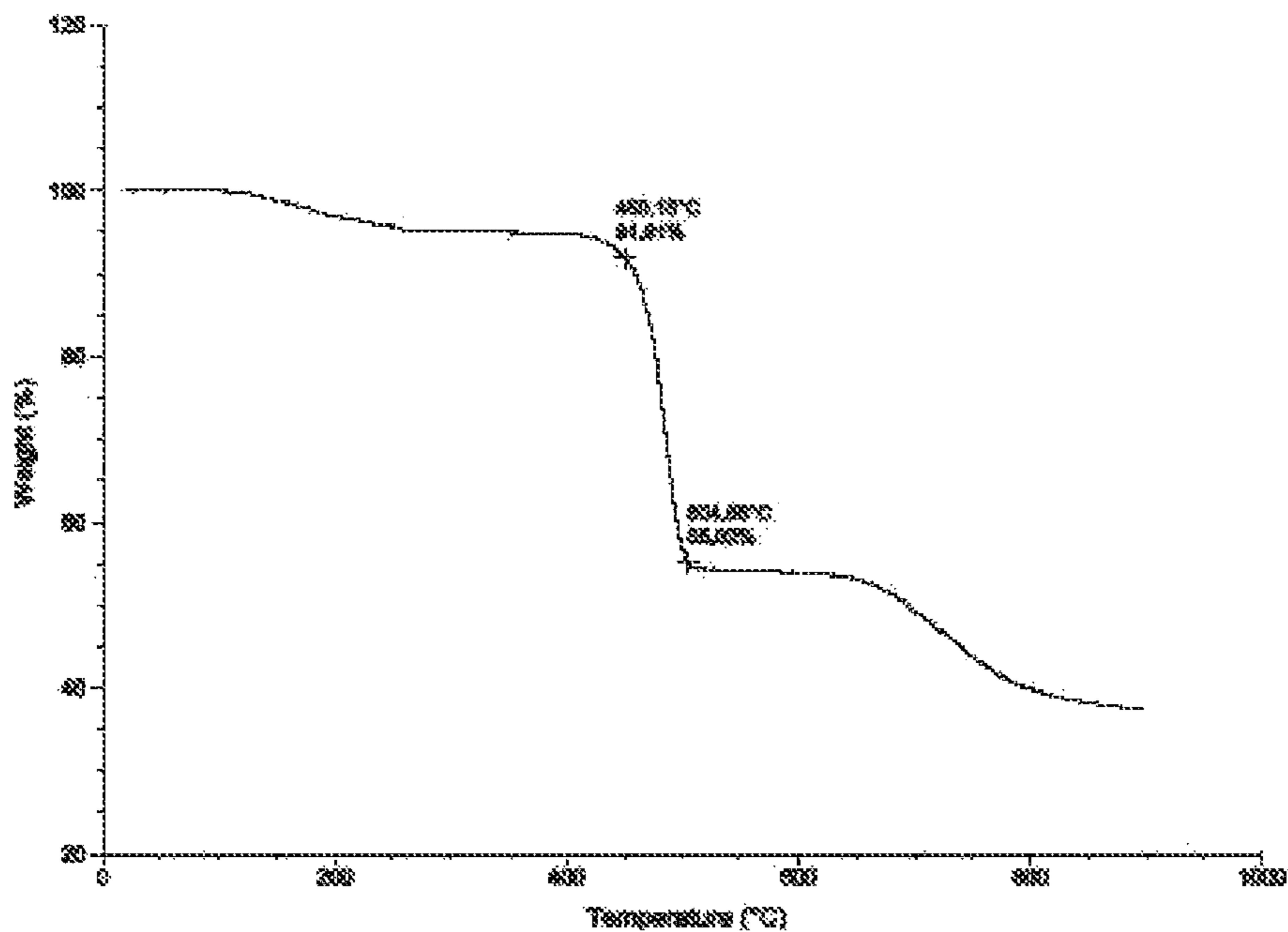
(B) Cyclized Trimer of Compound 2
