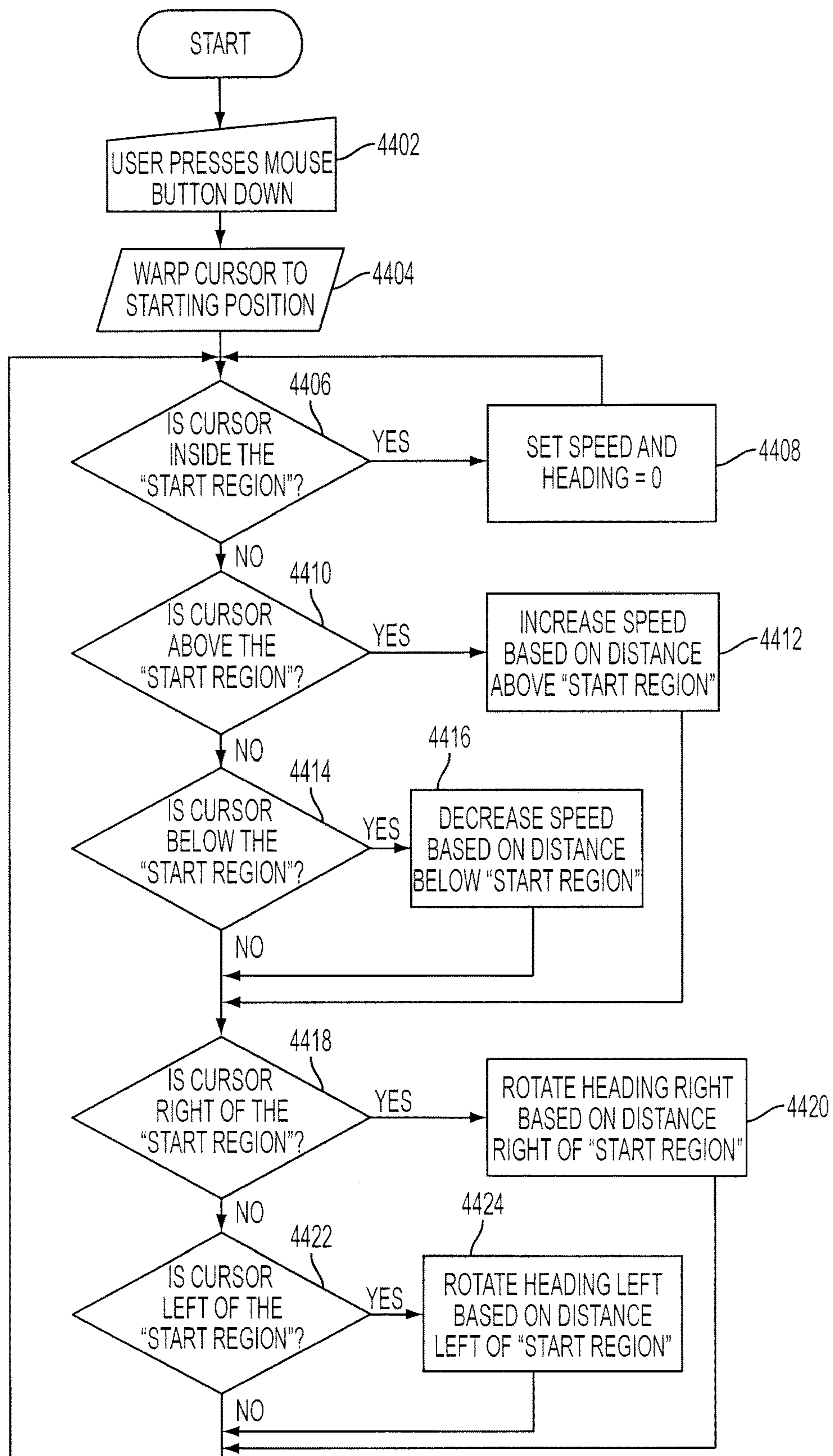
FLOWCHART OF WALK TOOL
