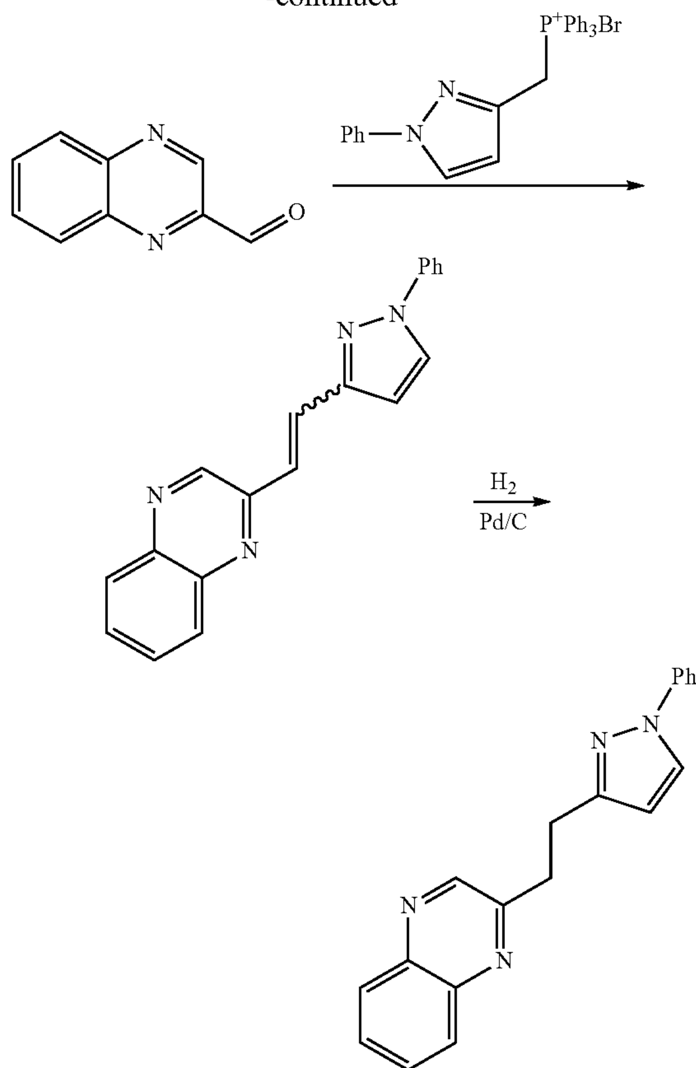
(a) Quinoxaline-2-carbaldehyde
