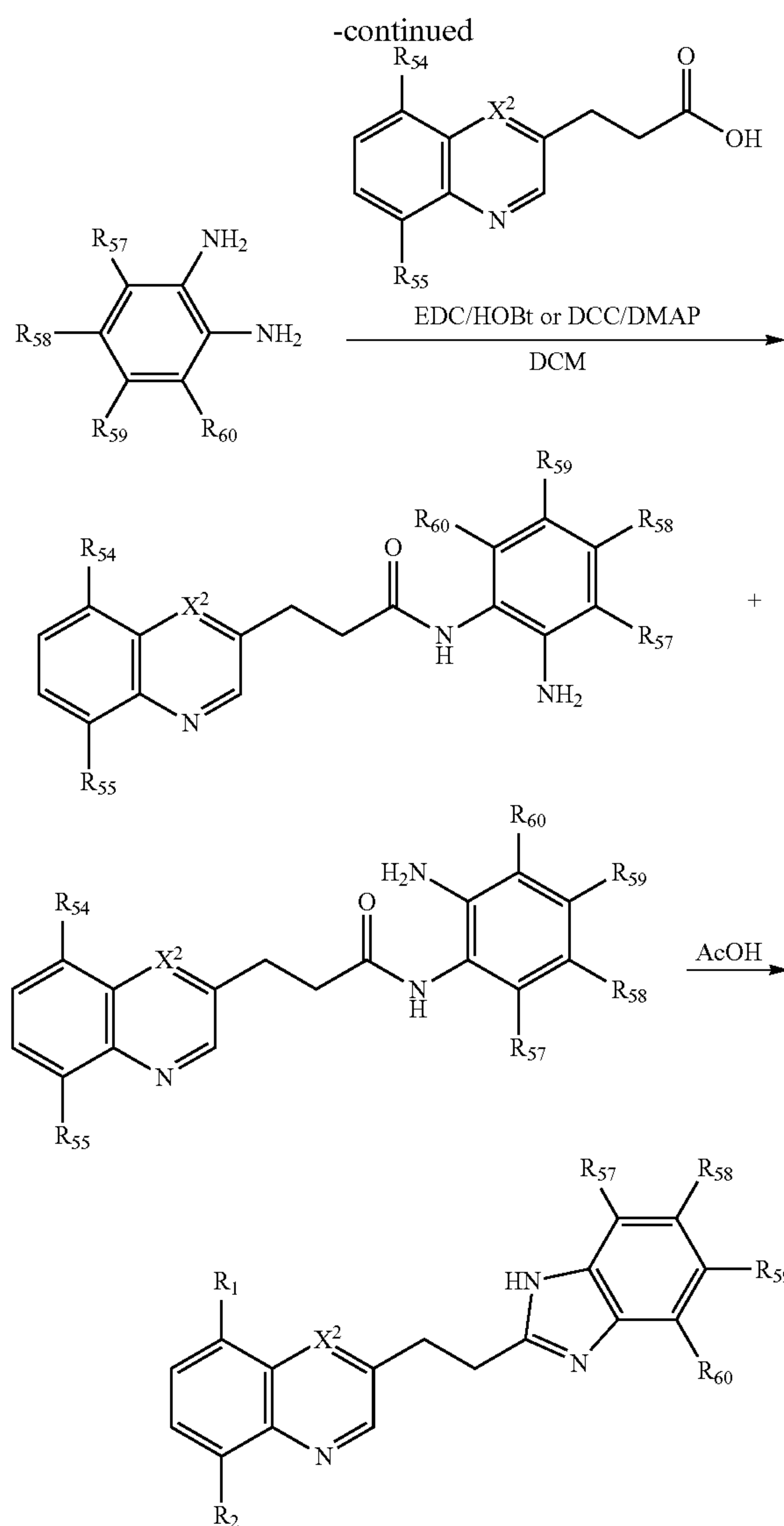
(a) Quinoline-5,6-diamine
