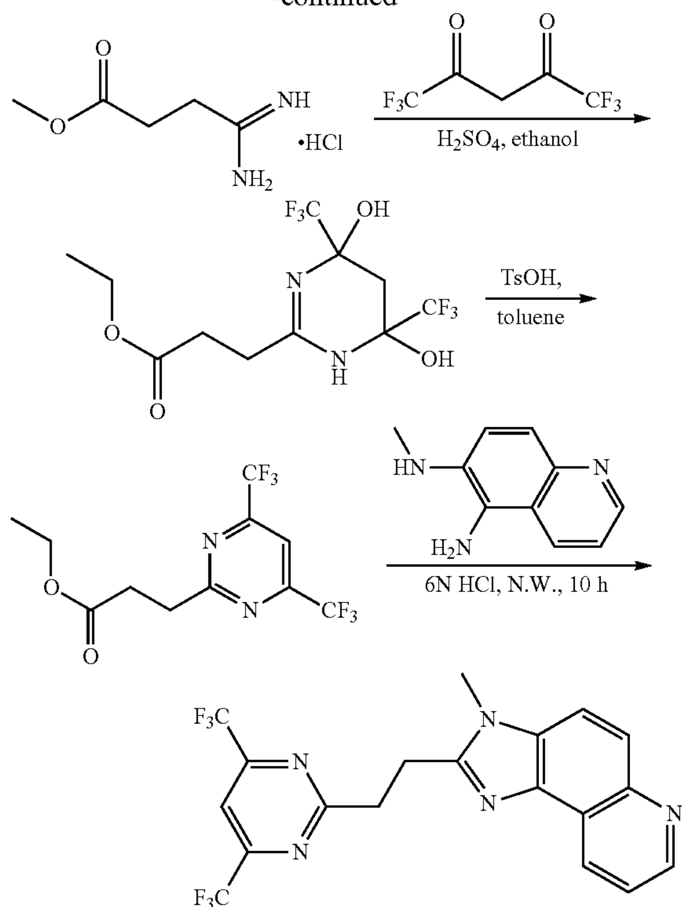
(a) Methyl 4-ethoxy-4-aminobutanoate
