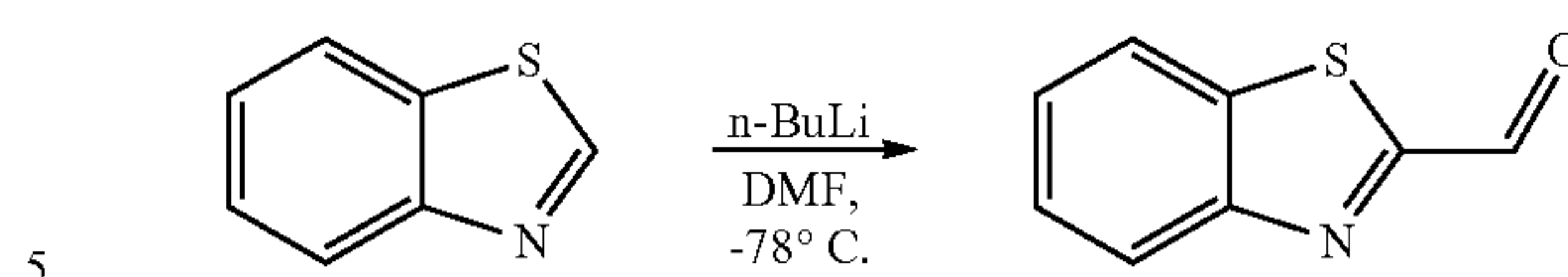
(j) Benzo[d]thiazole-2-carbaldehyde
