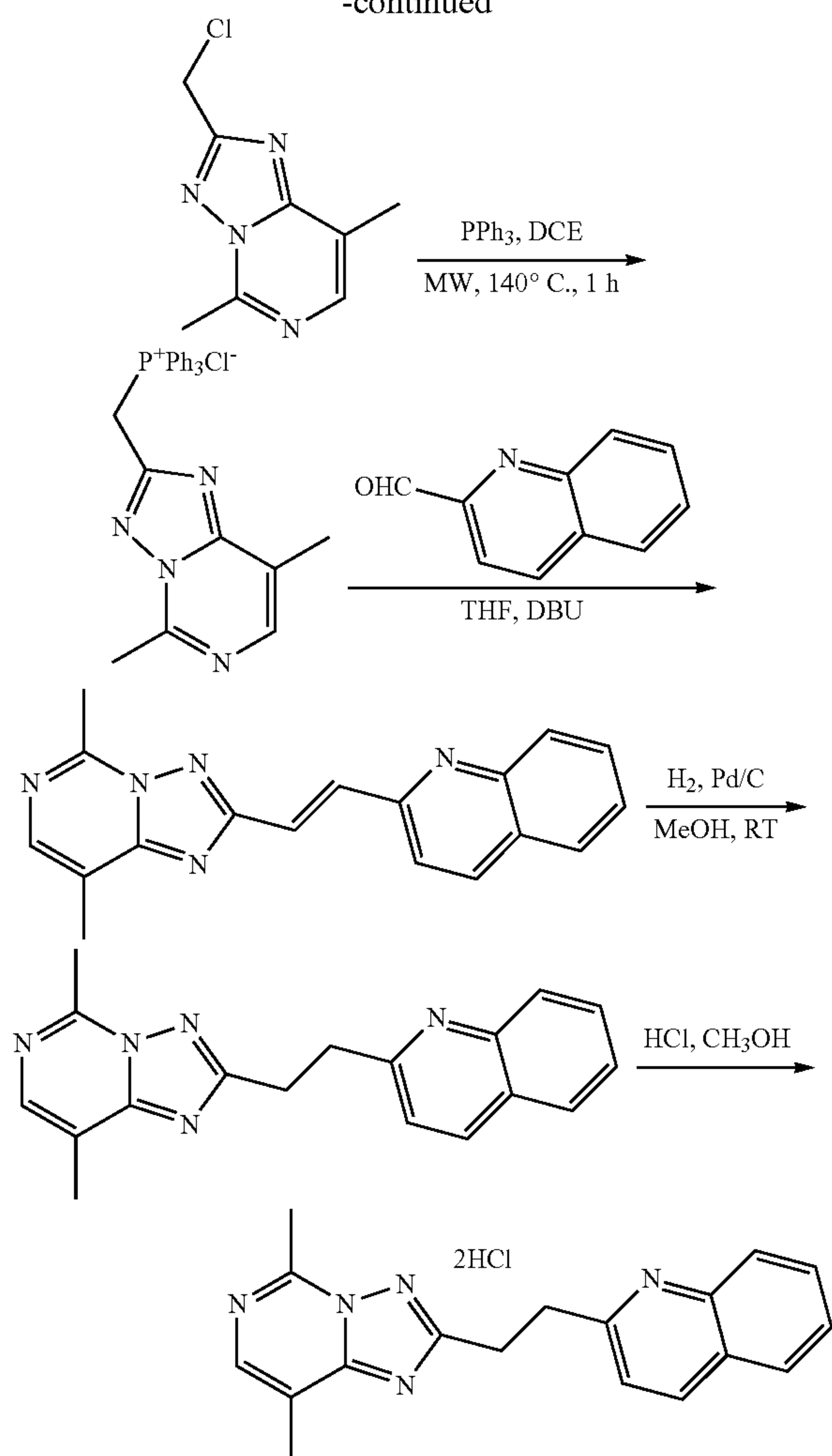
(a) 2,5-Dimethylpyrimidine-4,6-diol
