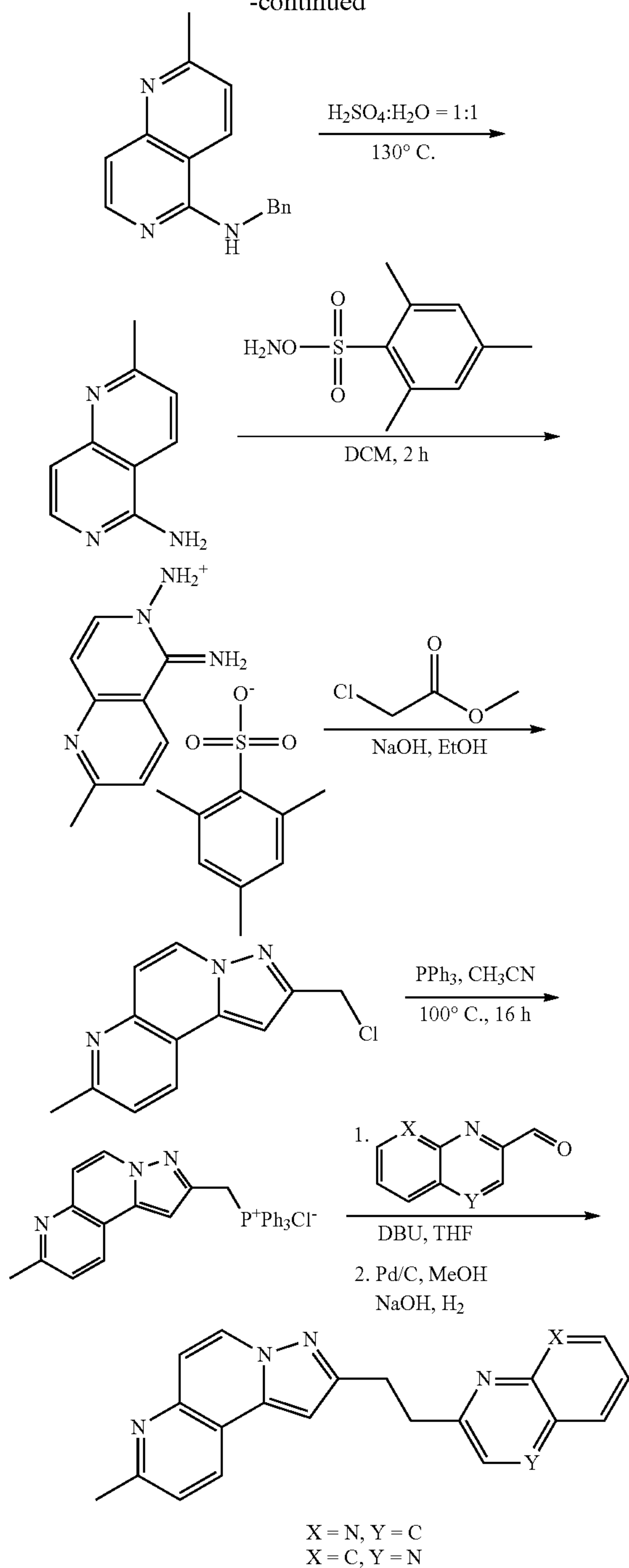
(a) N-Oxide-2-bromopyridine
