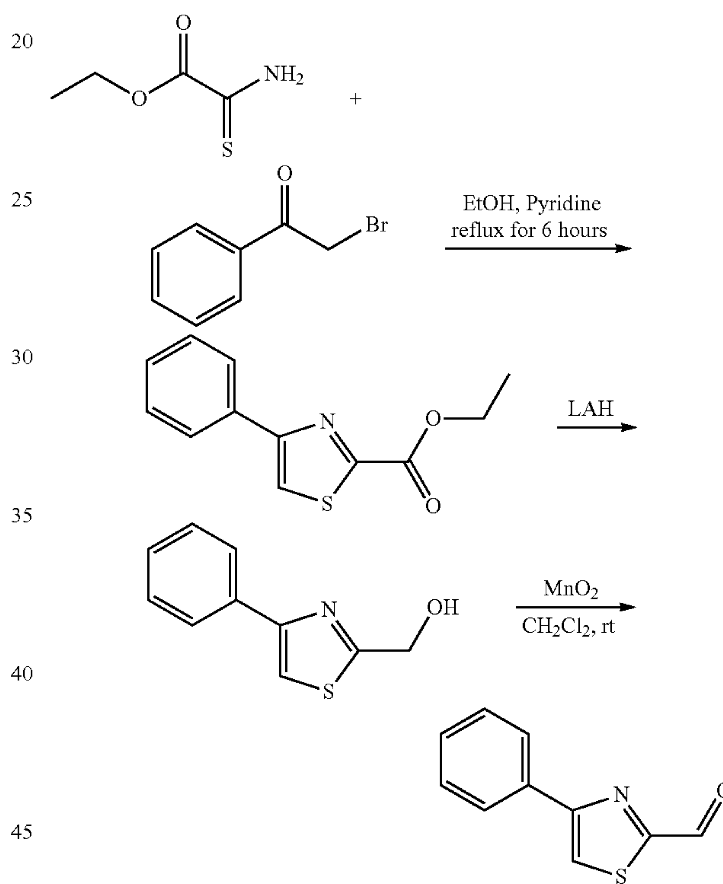
(k) Ethyl 4-phenylthiazole-2-carboxylate
