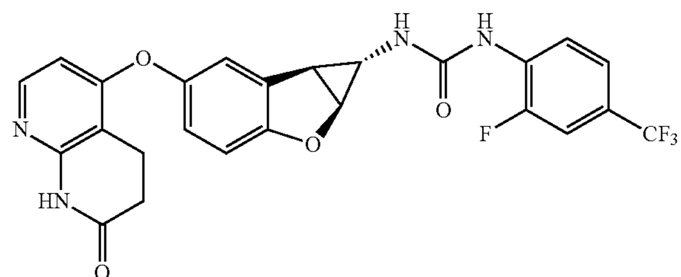
Compound 1.20
