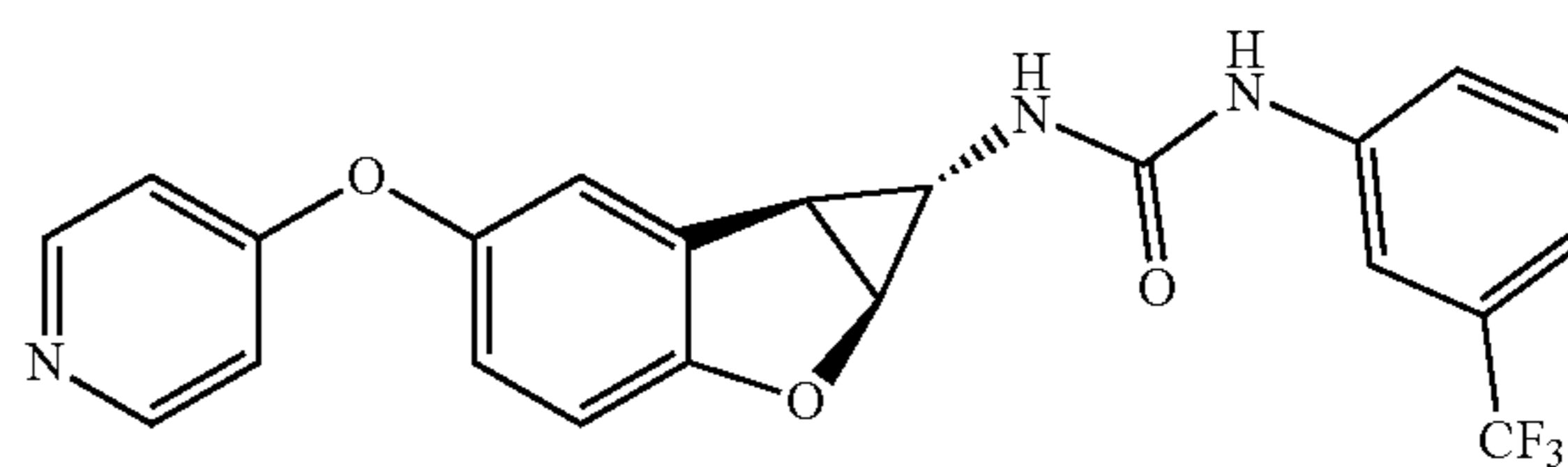
Compound 2.11
