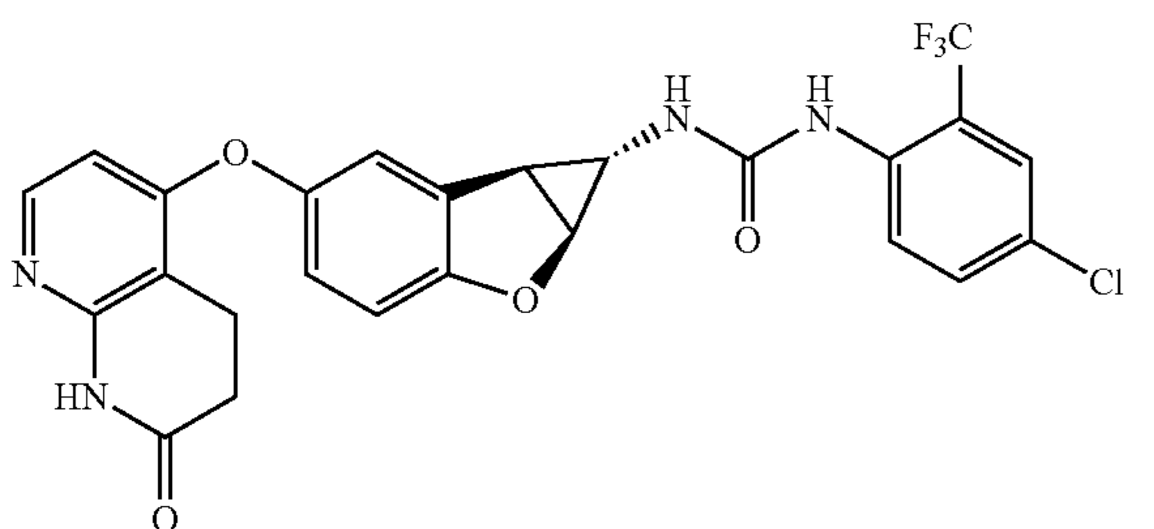
Compound 1.9
