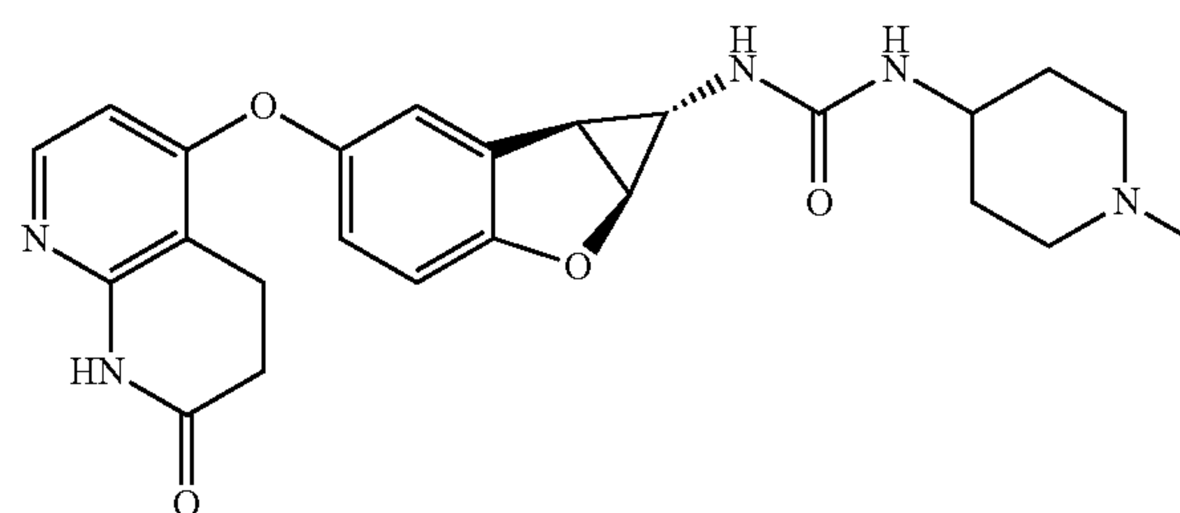
Compound 1.70
