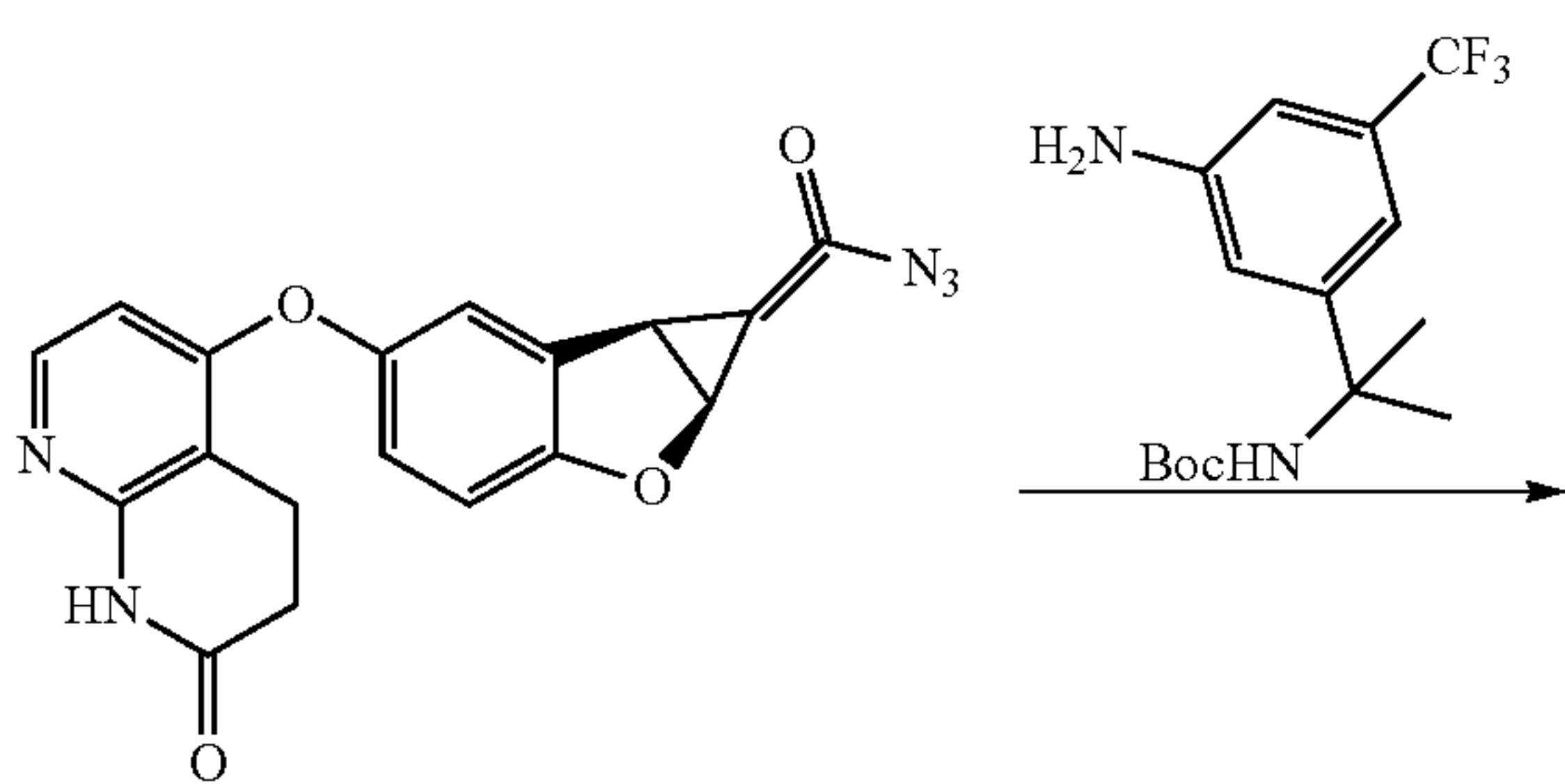
Intermediate I
