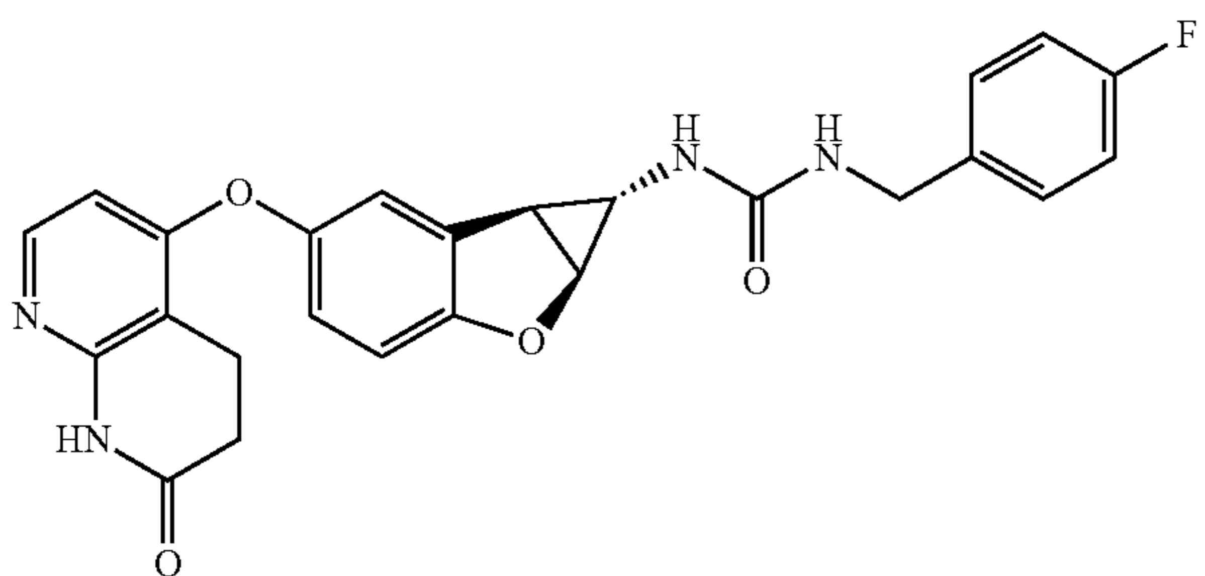
Compound 1.59
