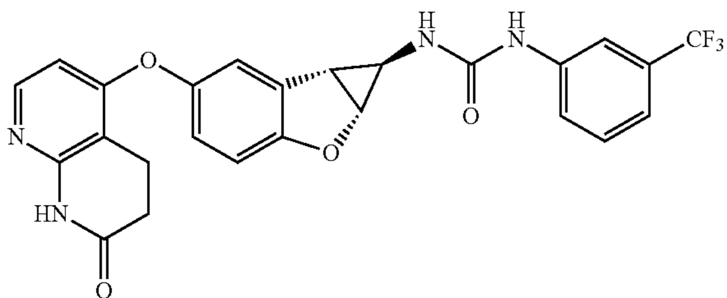
Compound 1.71
