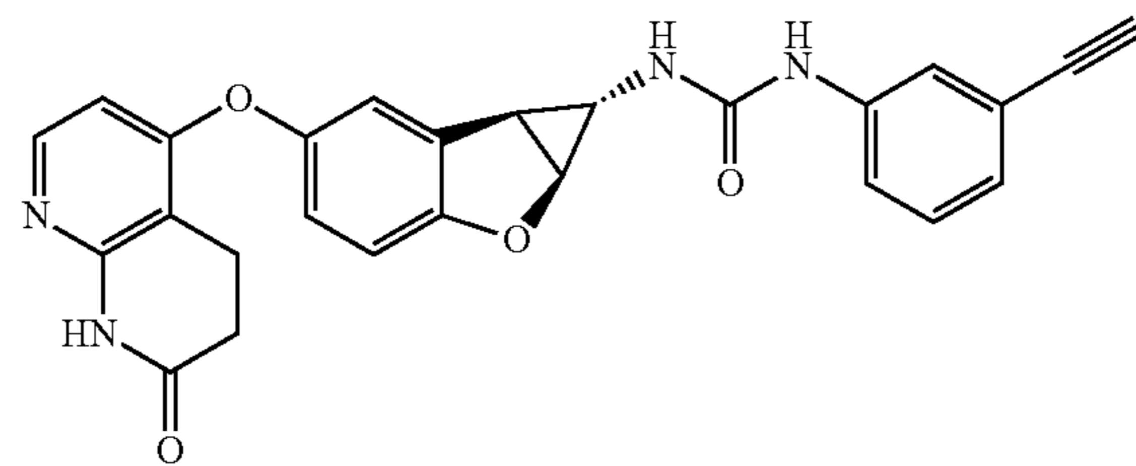
Compound 1.14
