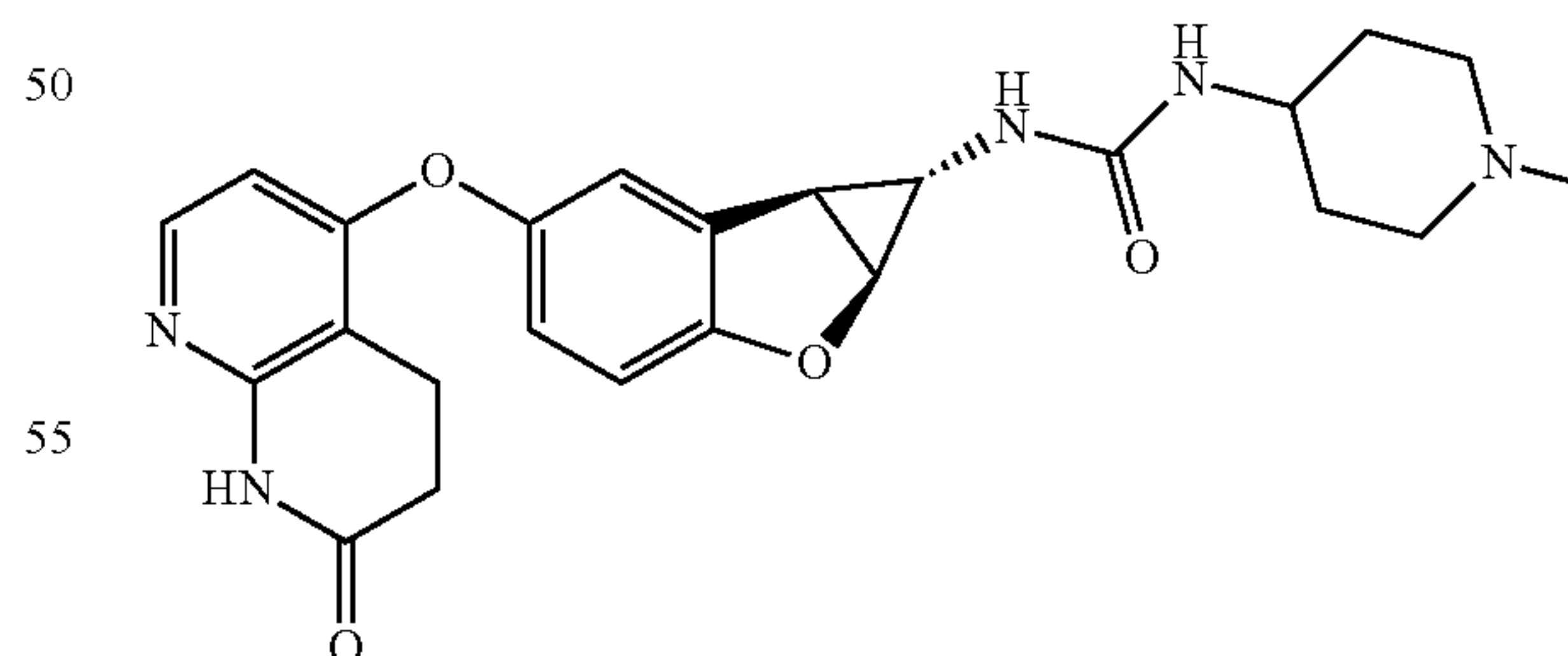
Compound 1.68
