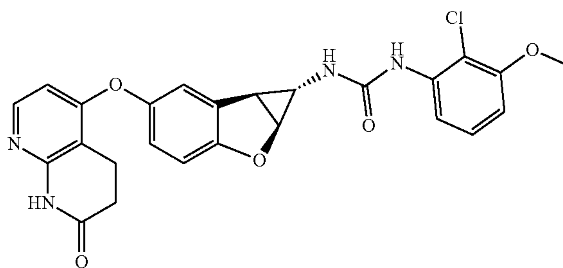
Compound 1.6
