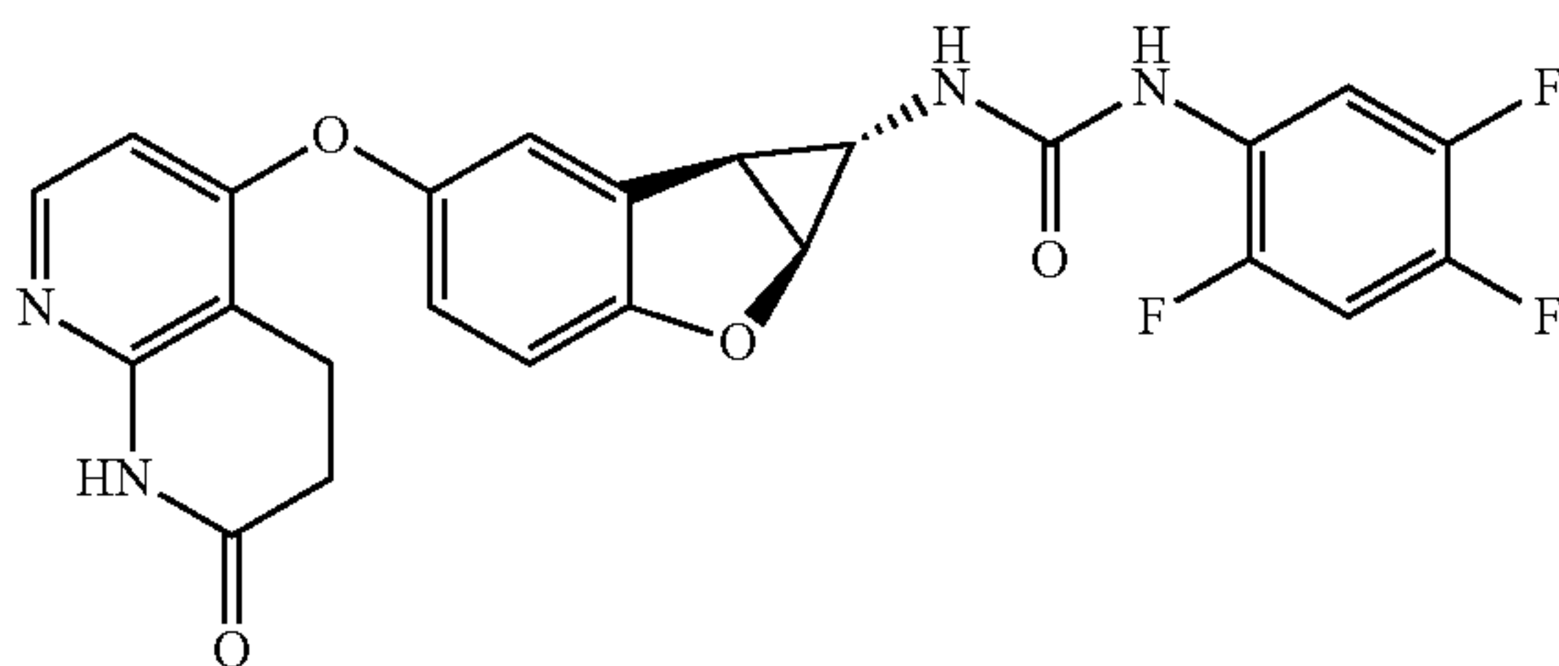
Compound 1.49
