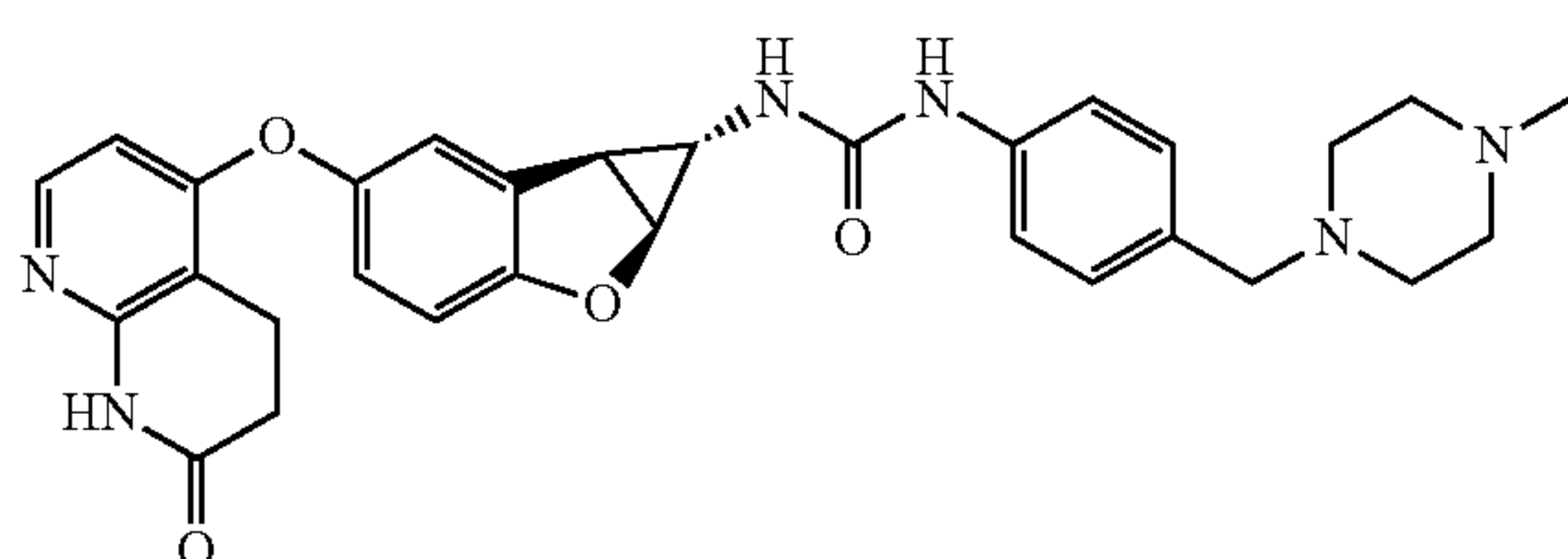
Compound 1.63
