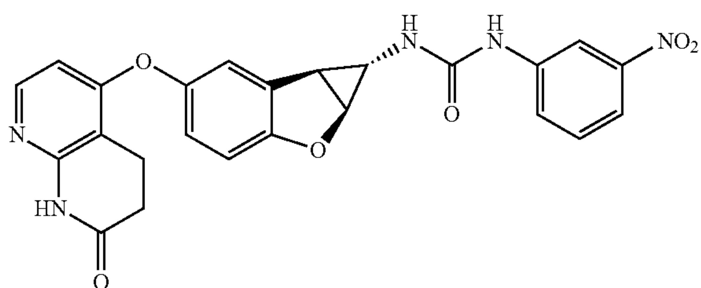
Compound 1.13
