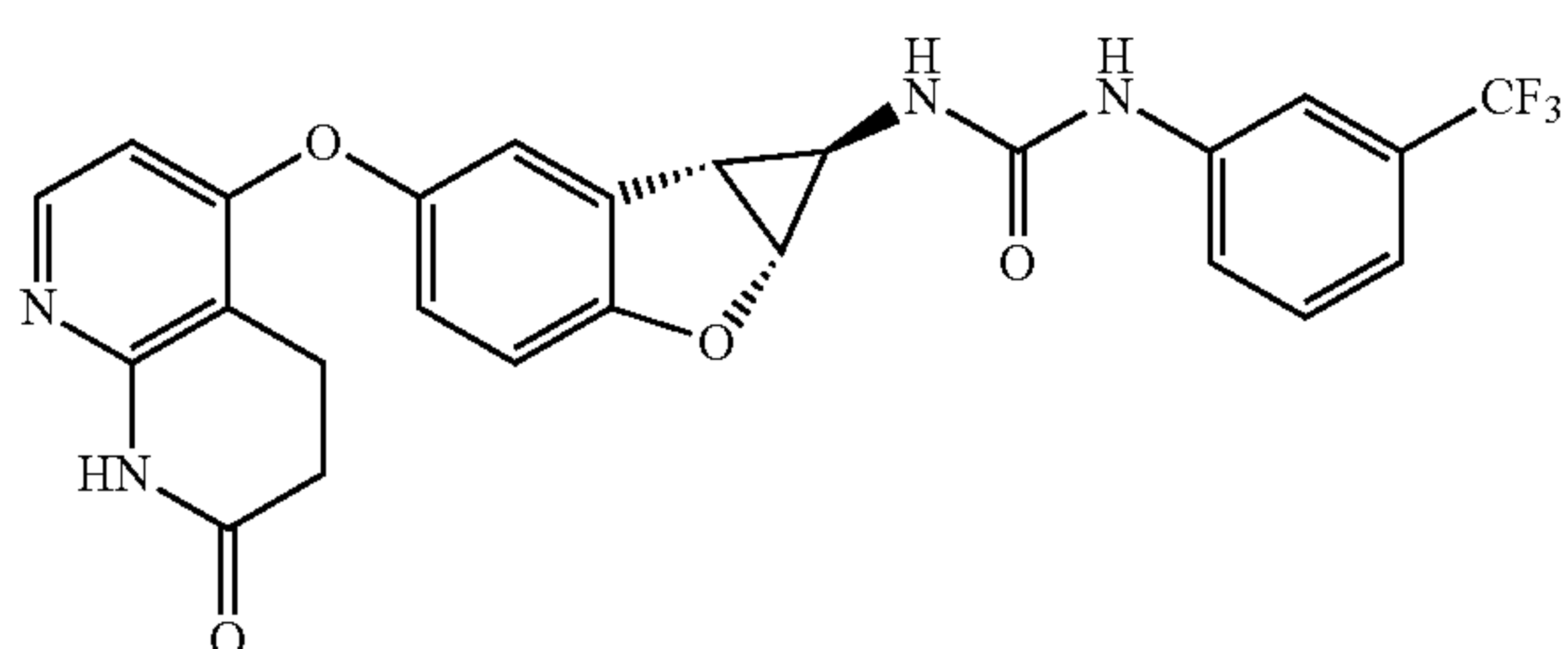
Compound 1.71
