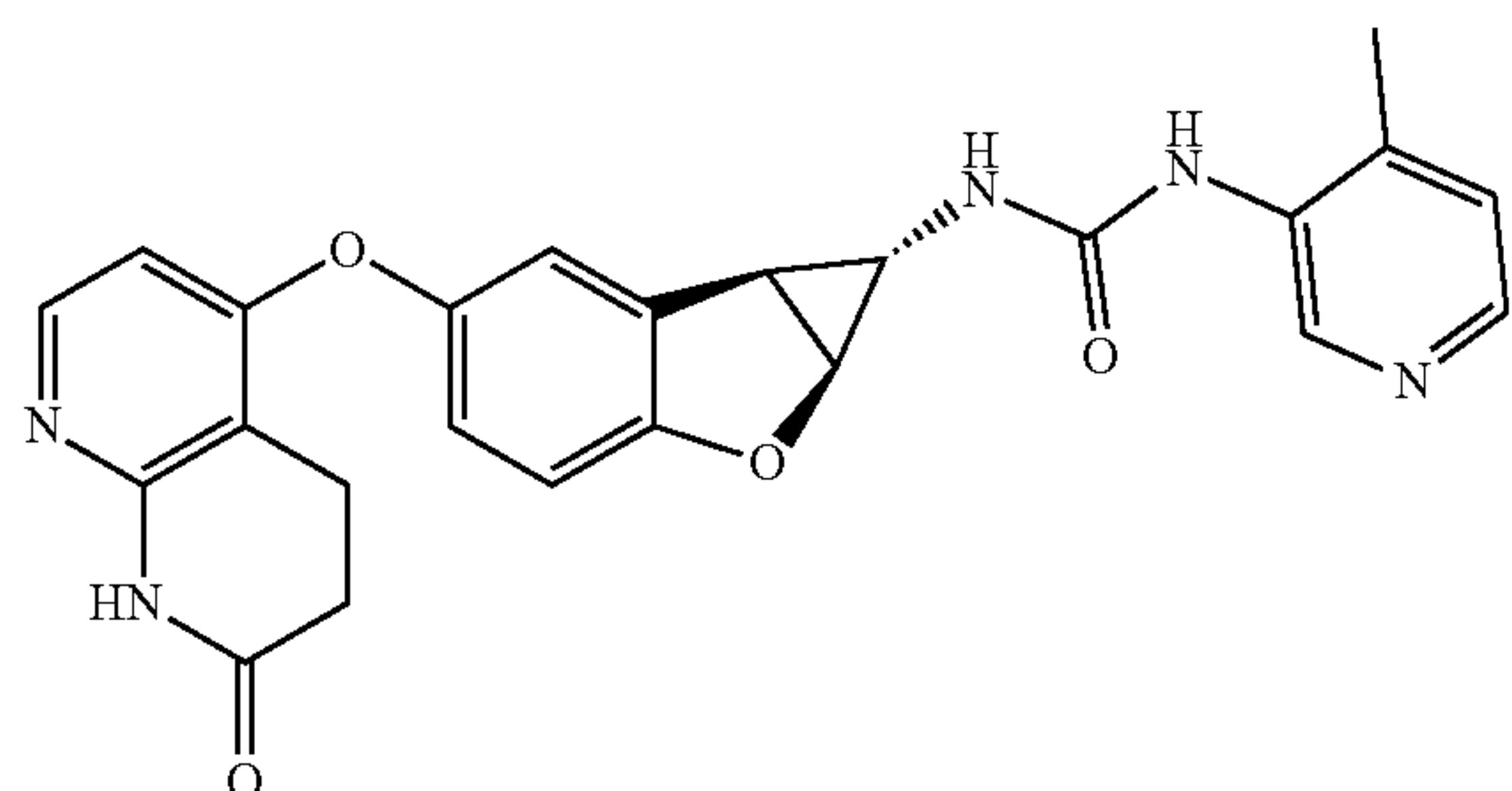
Compound 1.39
