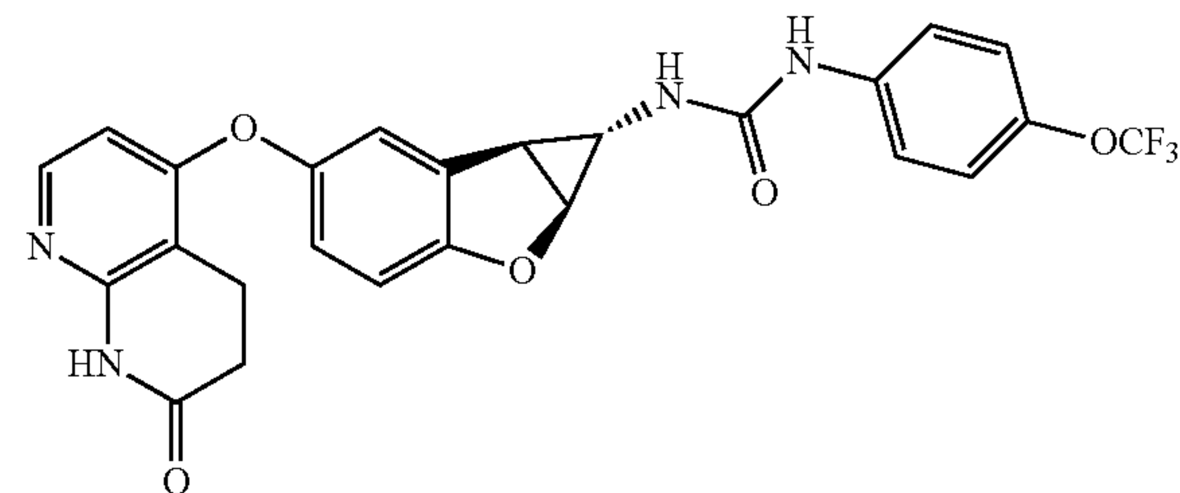
Compound 1.61
