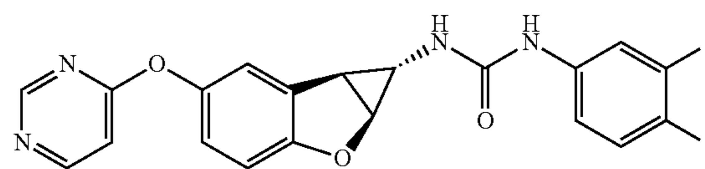
Compound 2.2
