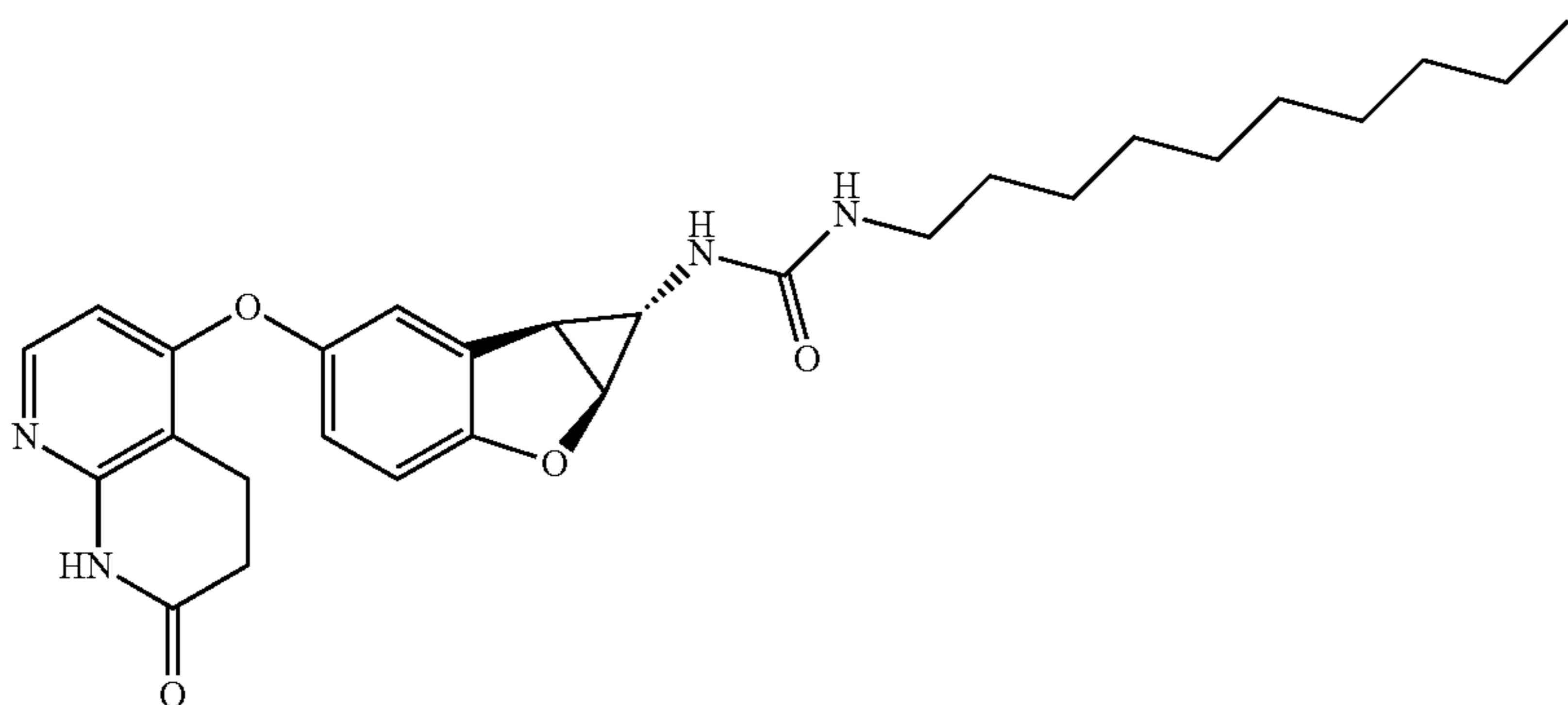
Compound 1.86
