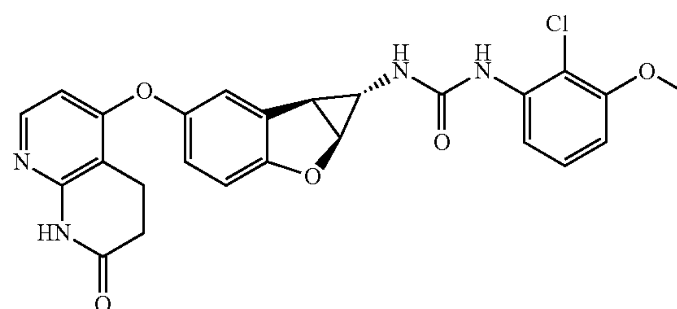
Compound 1.6
