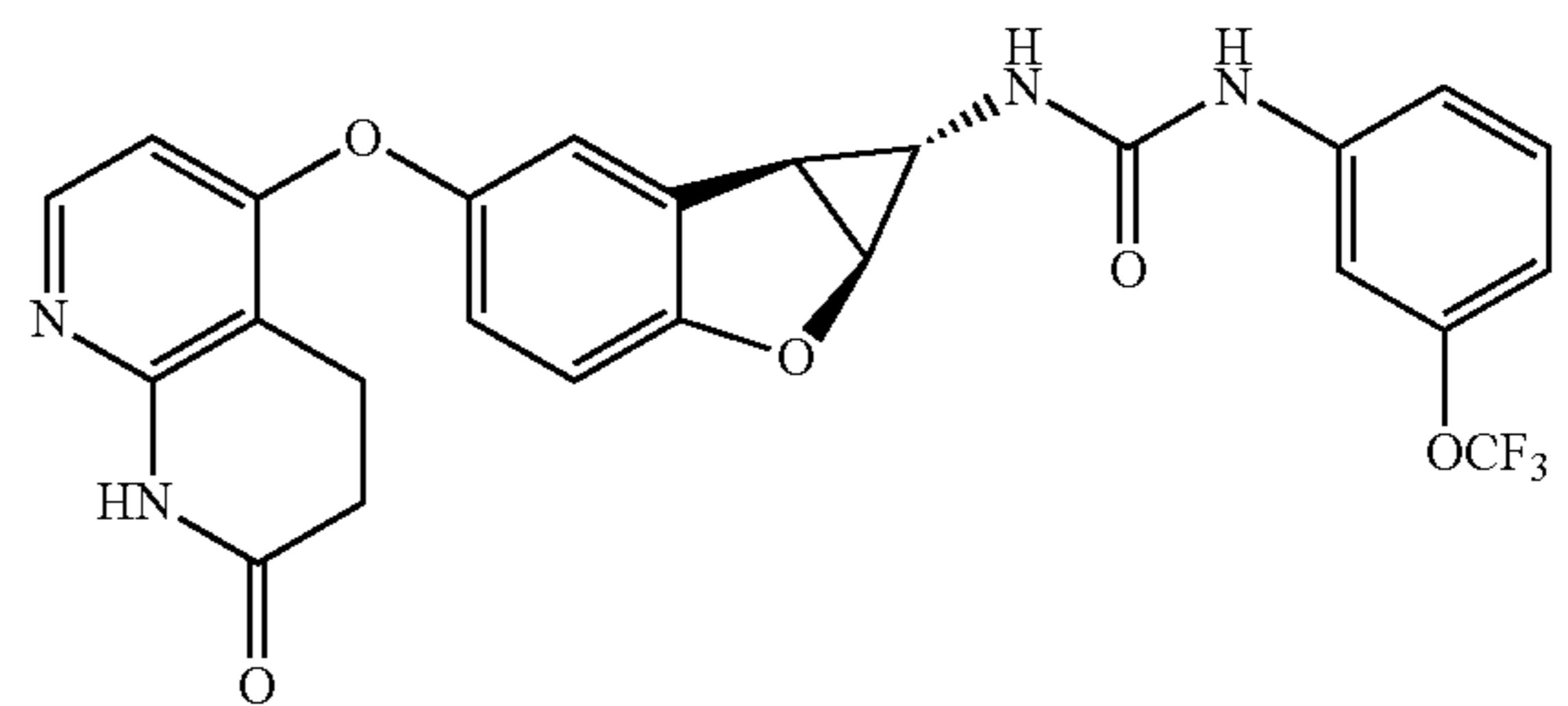
Compound 1.60
