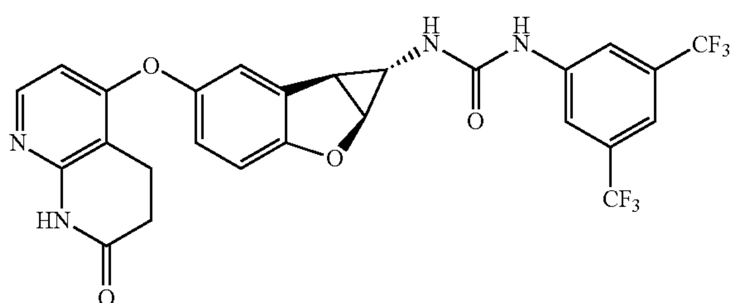
Compound 1.67
