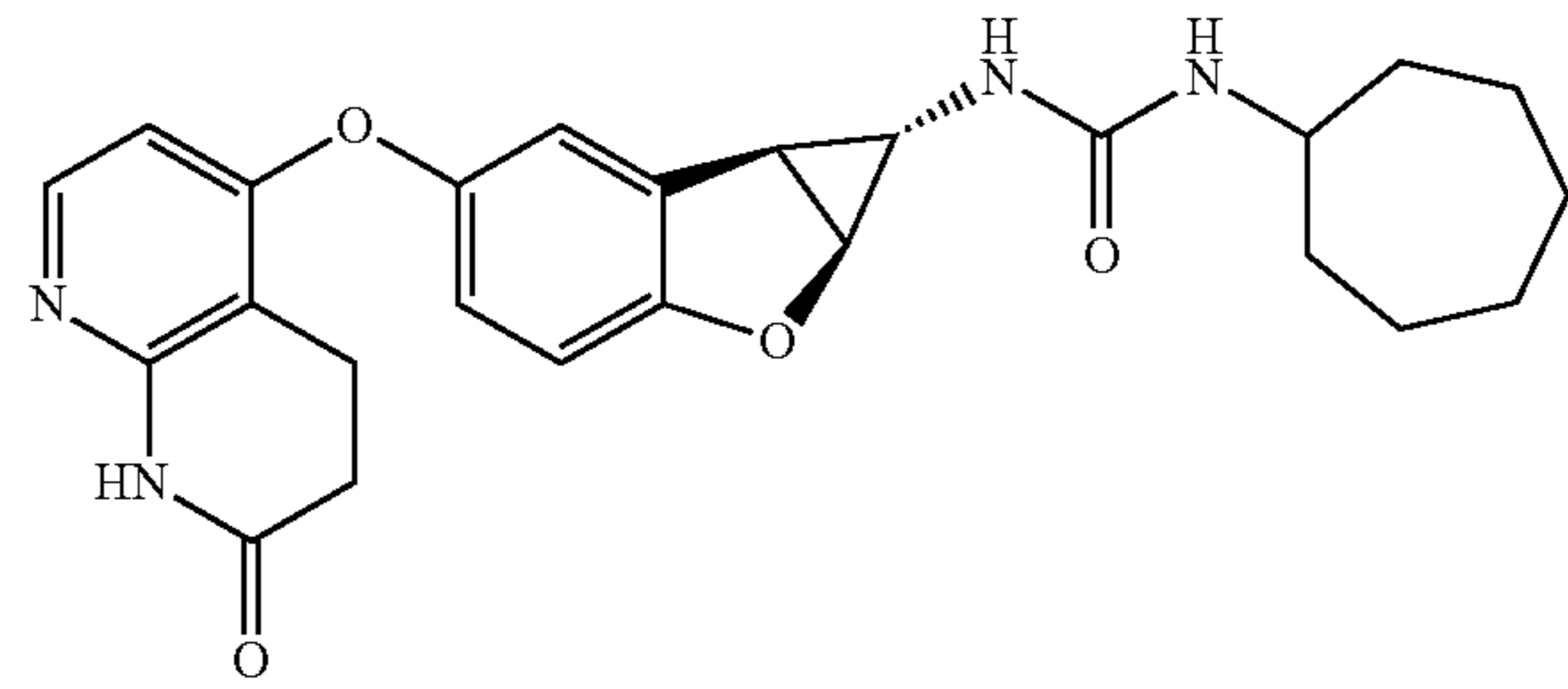
Compound 1.52
