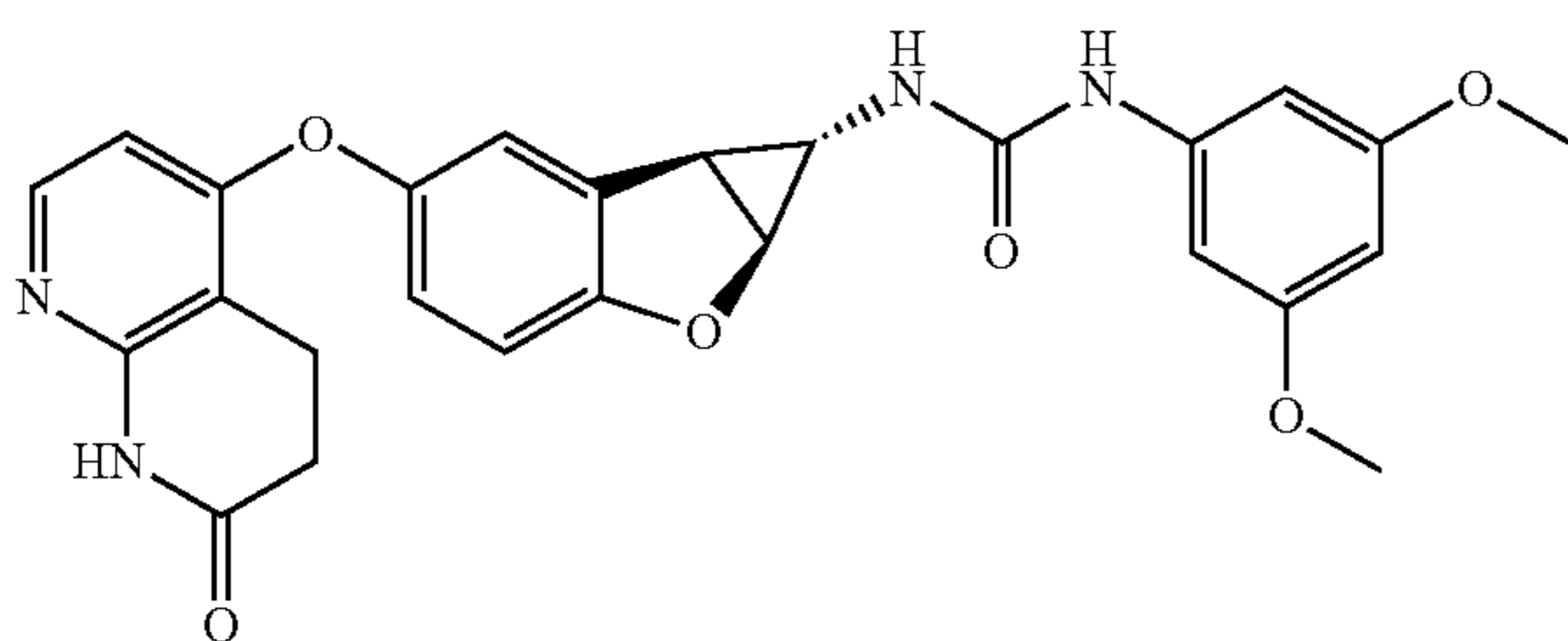
Compound 1.17
