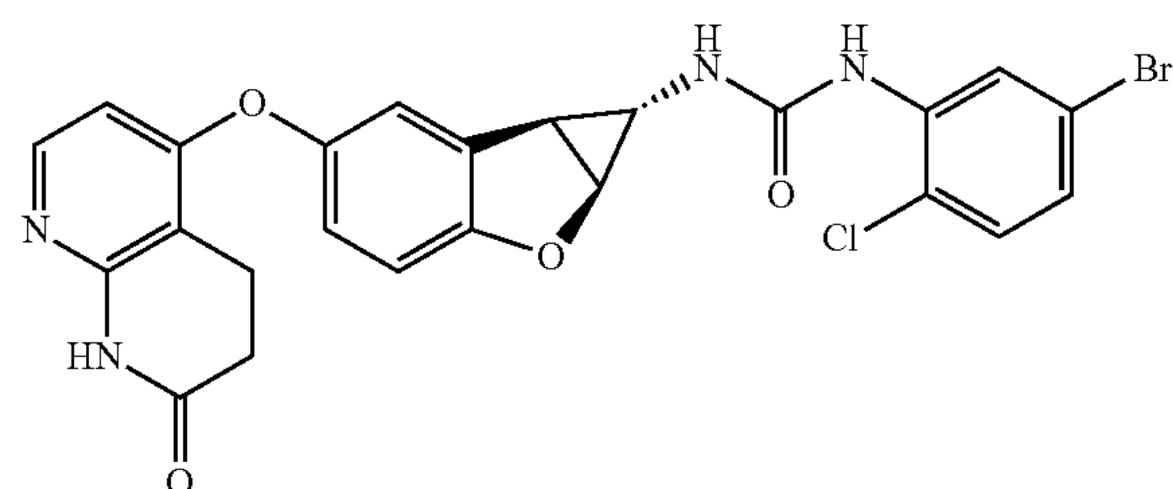
Compound 1.8
