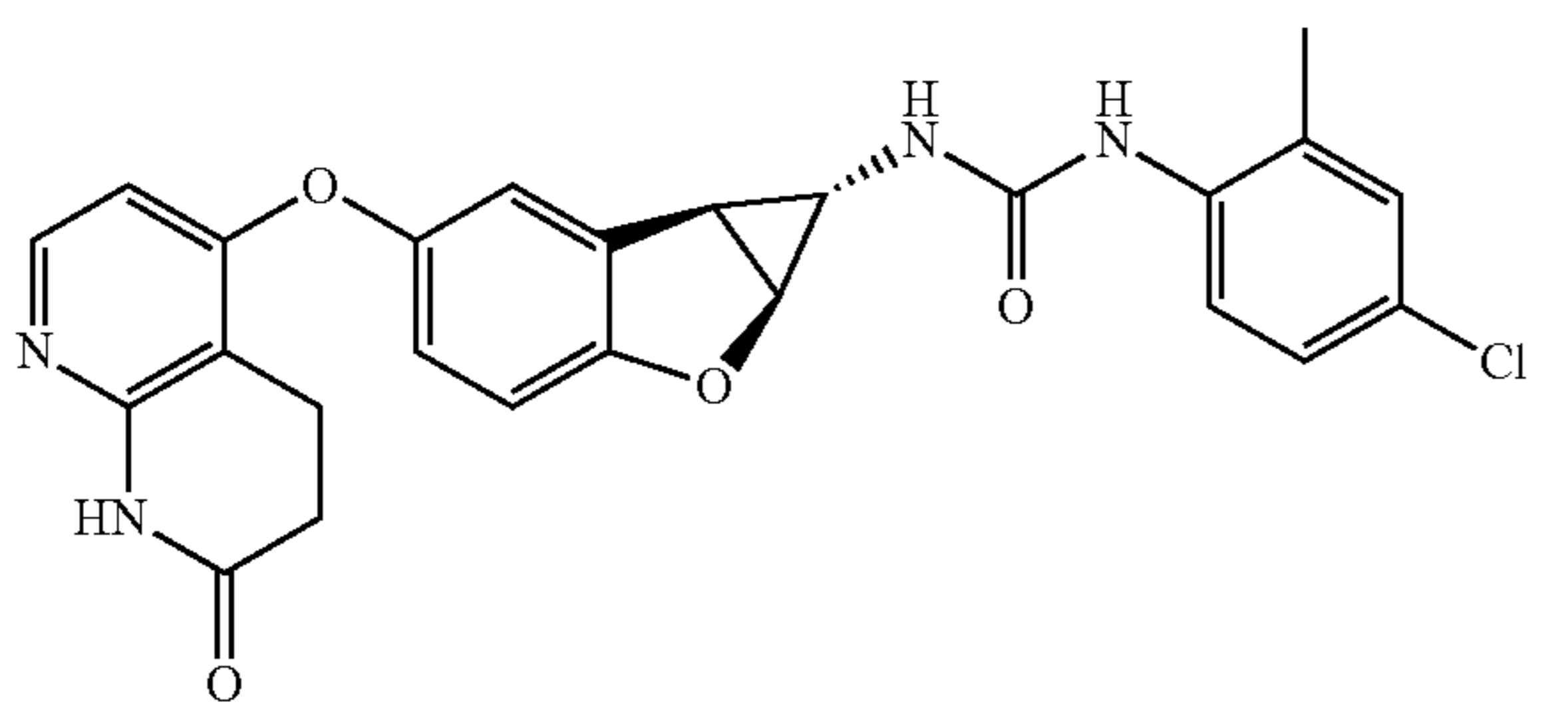
Compound 1.7
