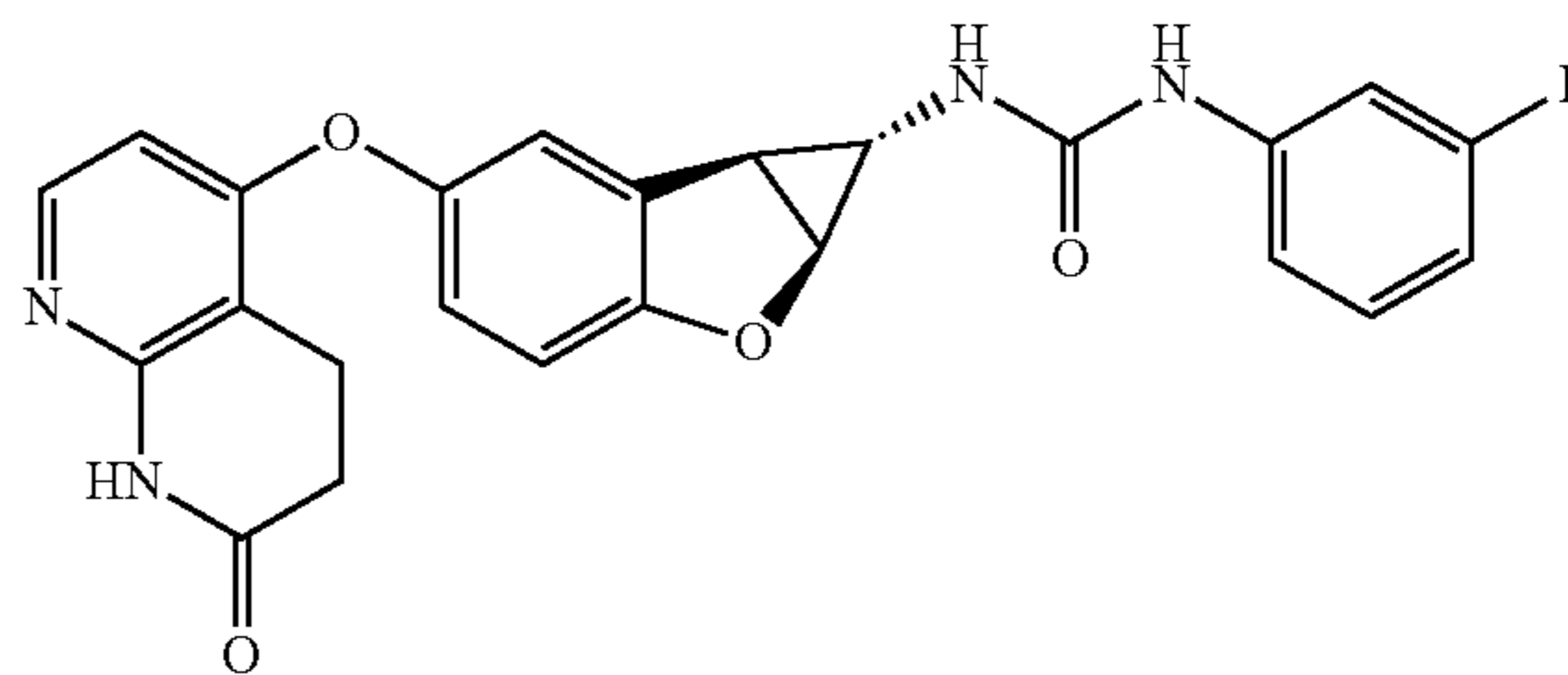
Compound 1.22
