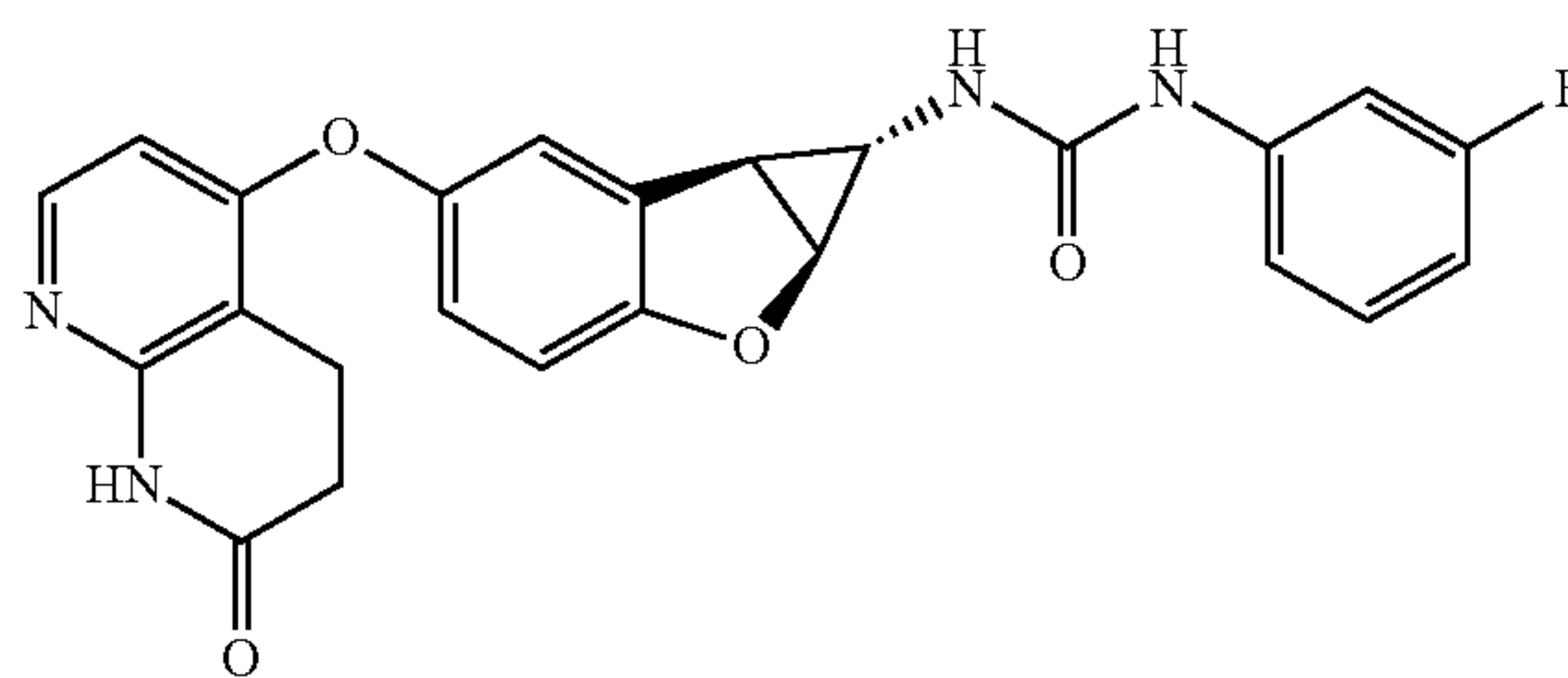
Compound 1.22
