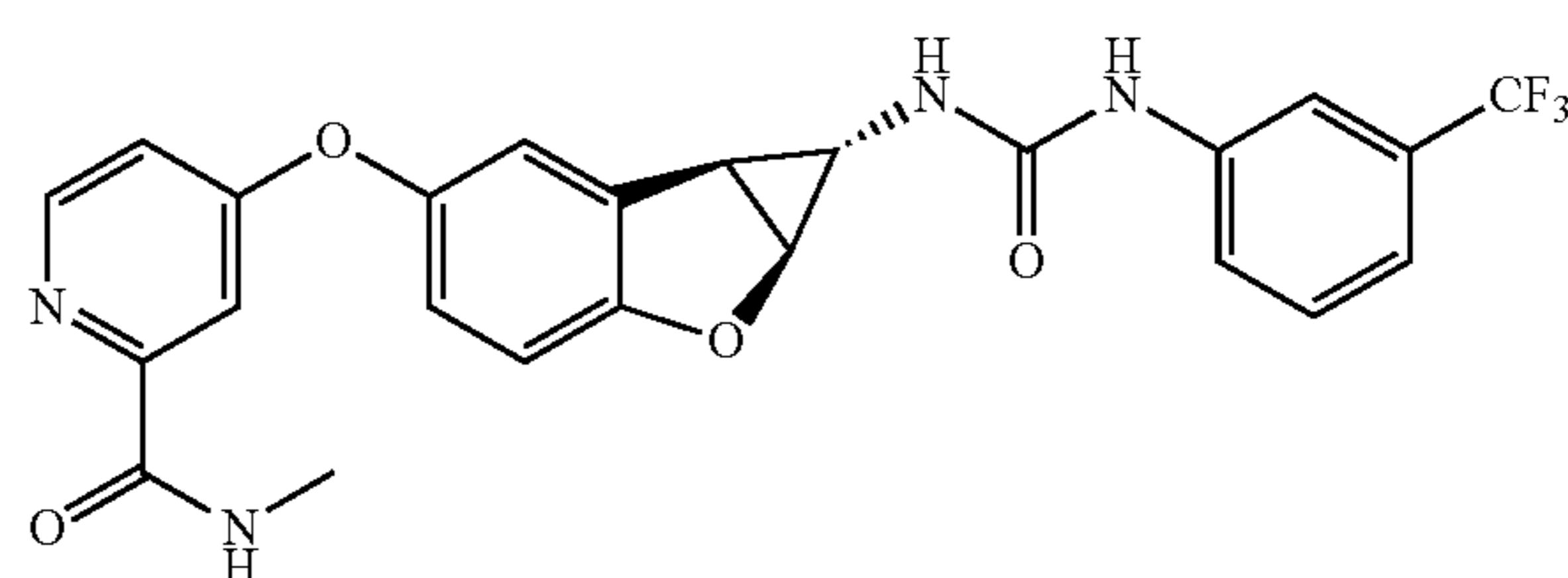
Compound 2.6
