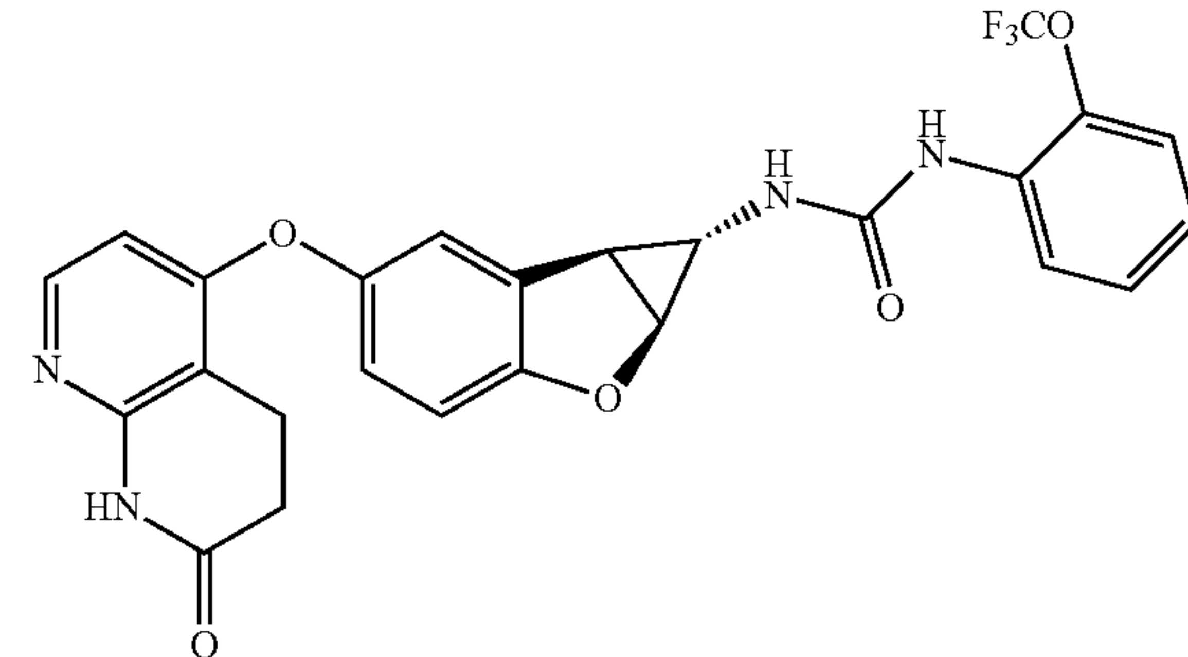
Compound 1.62
