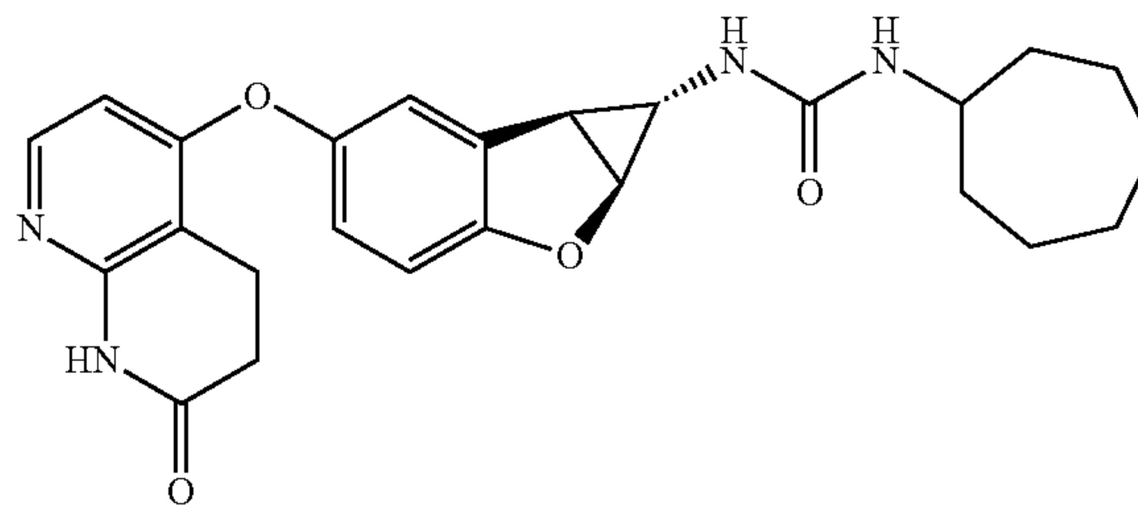
Compound 1.52
