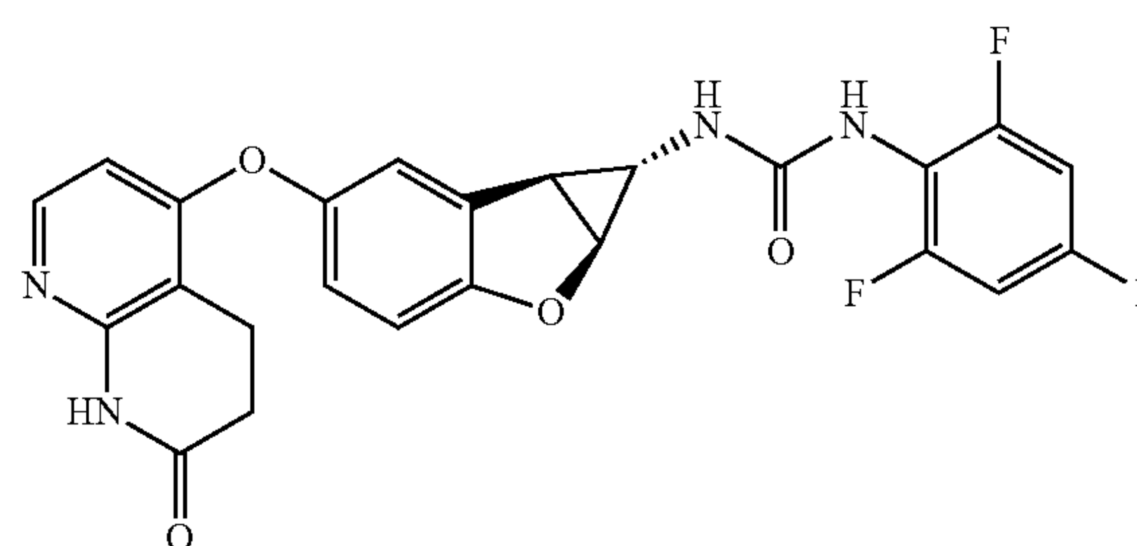
Compound 1.40
