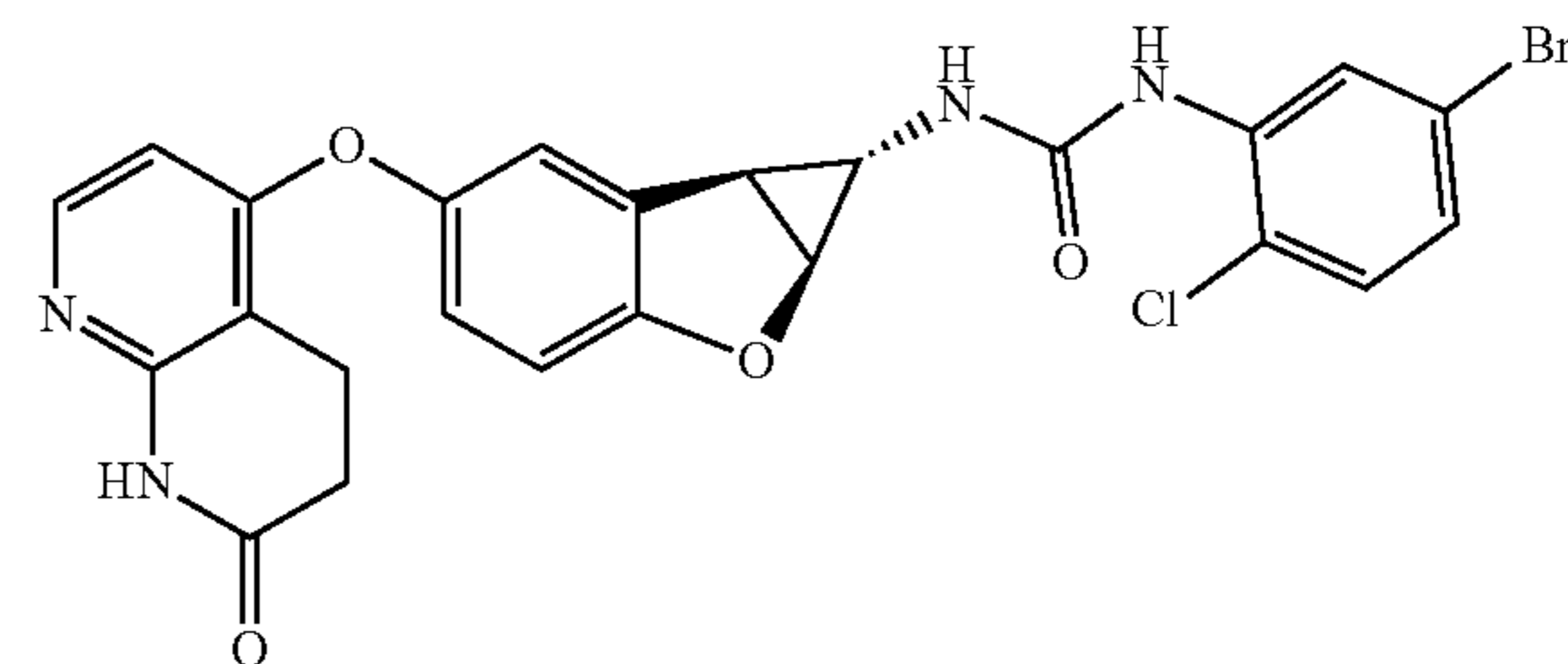
Compound 1.8
