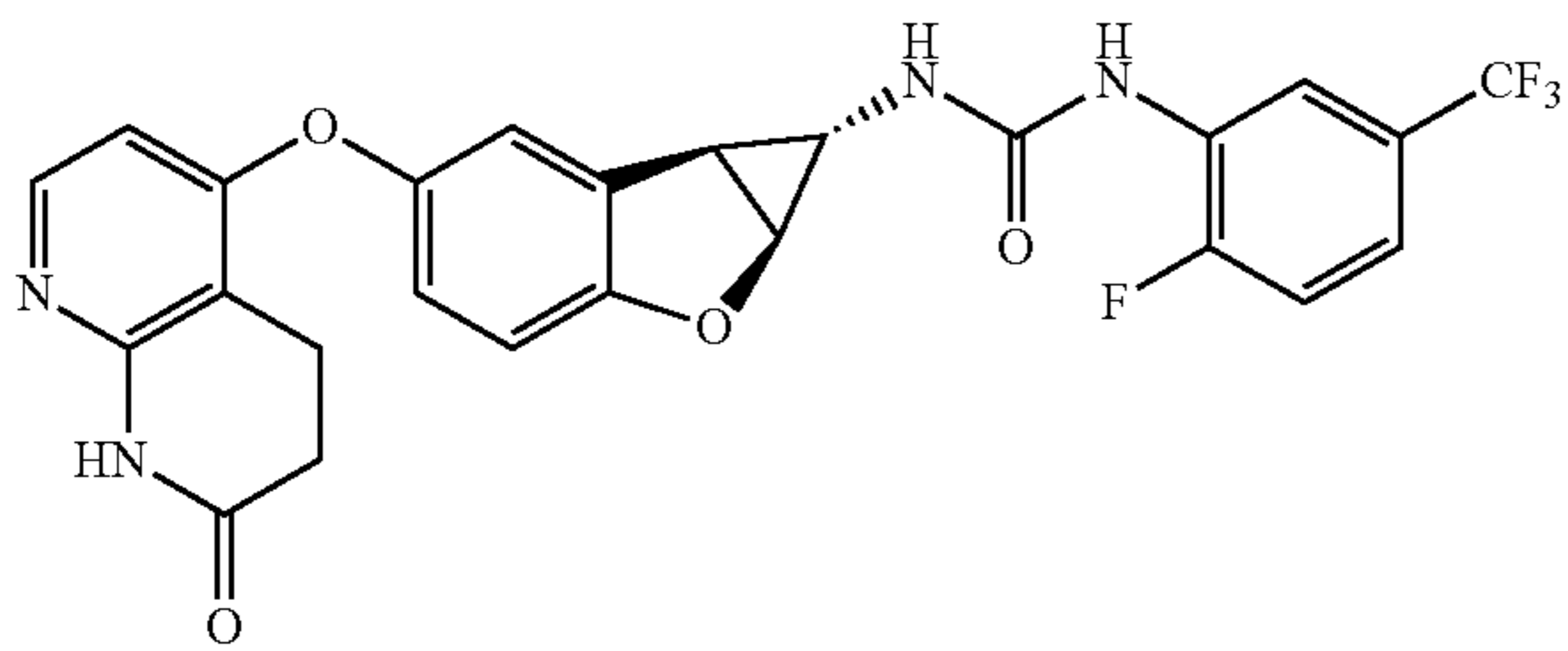
Compound 1.33
