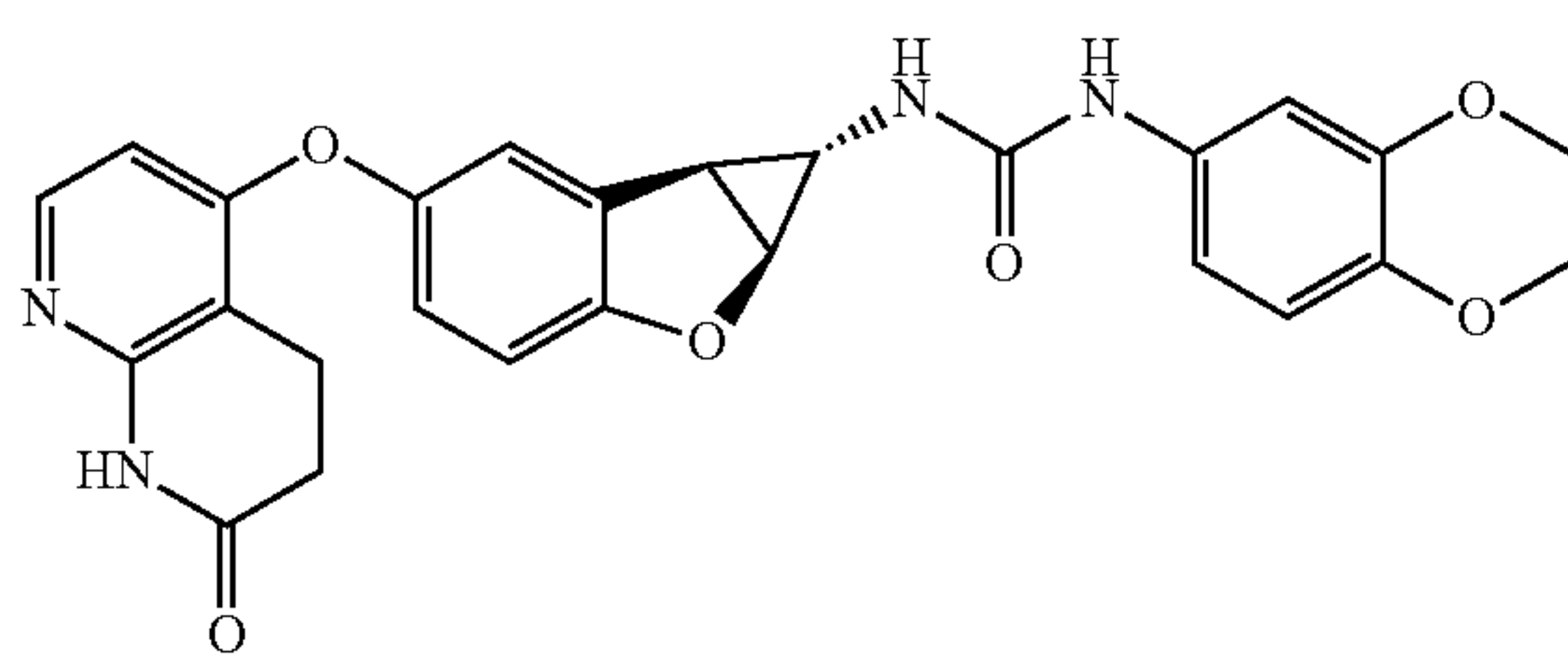
Compound 1.15
