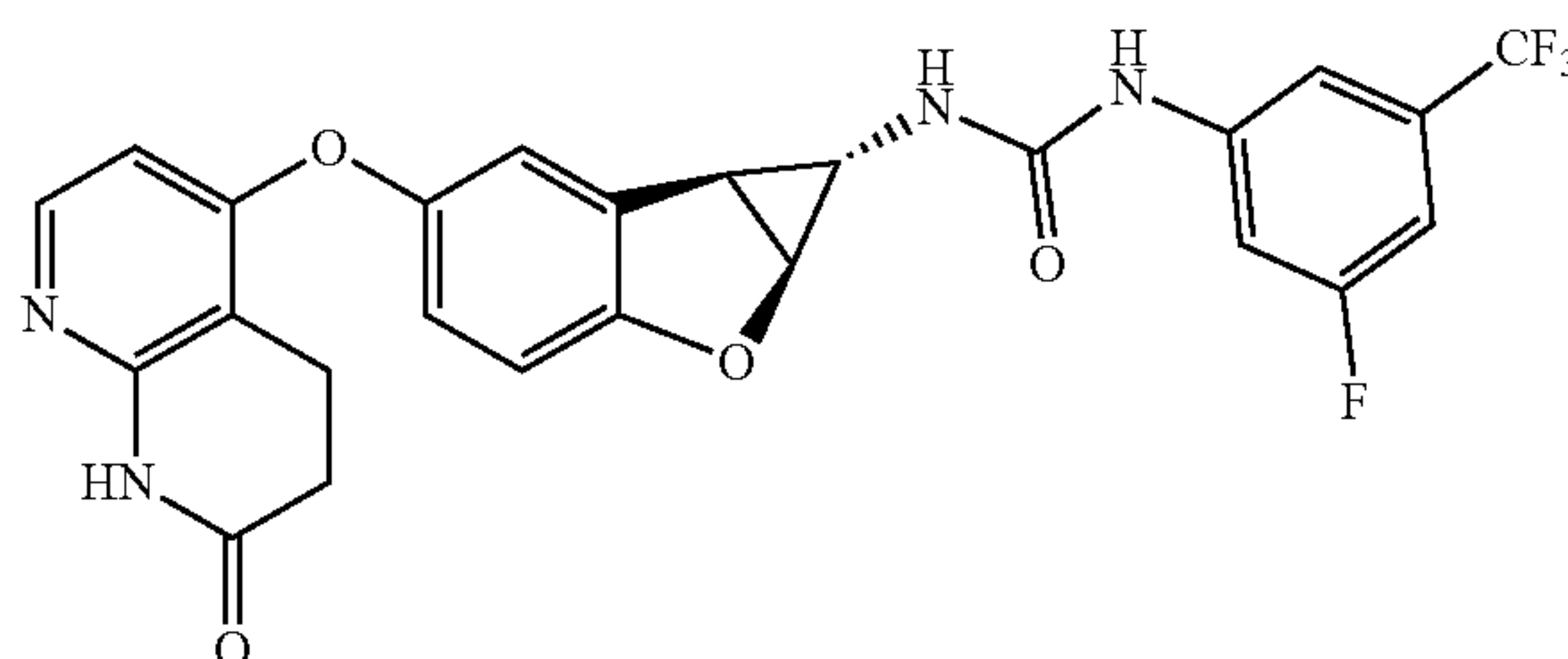
Compound 1.11
