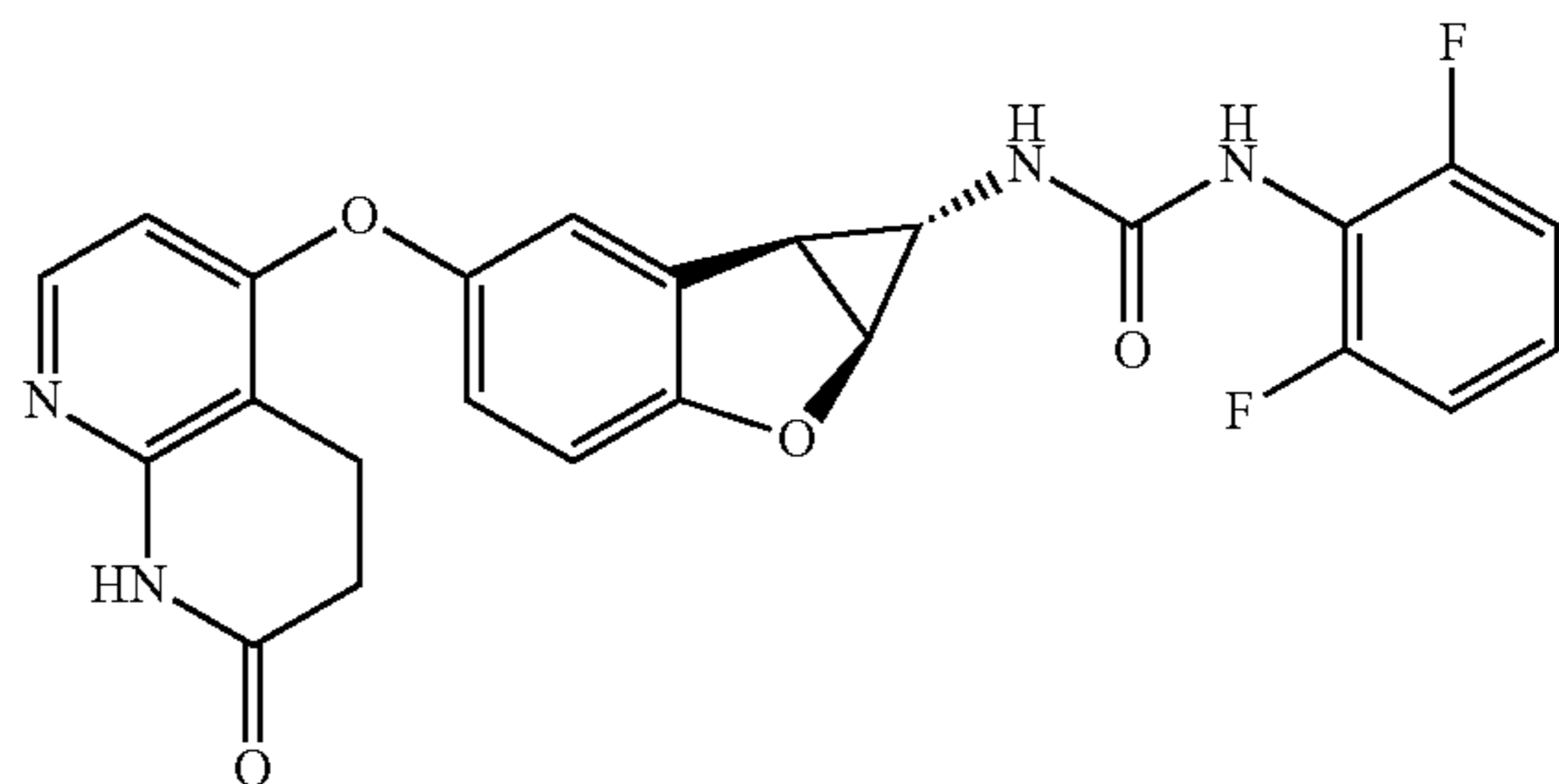
Compound 1.44
