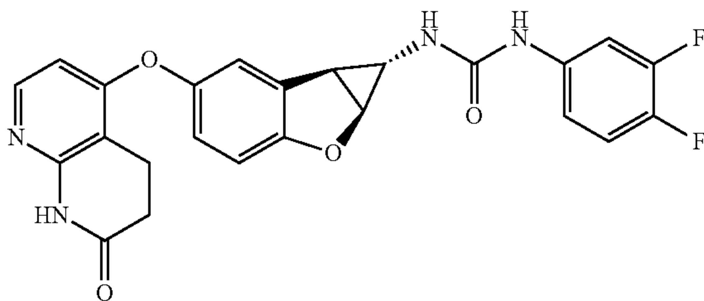
Compound 1.45
