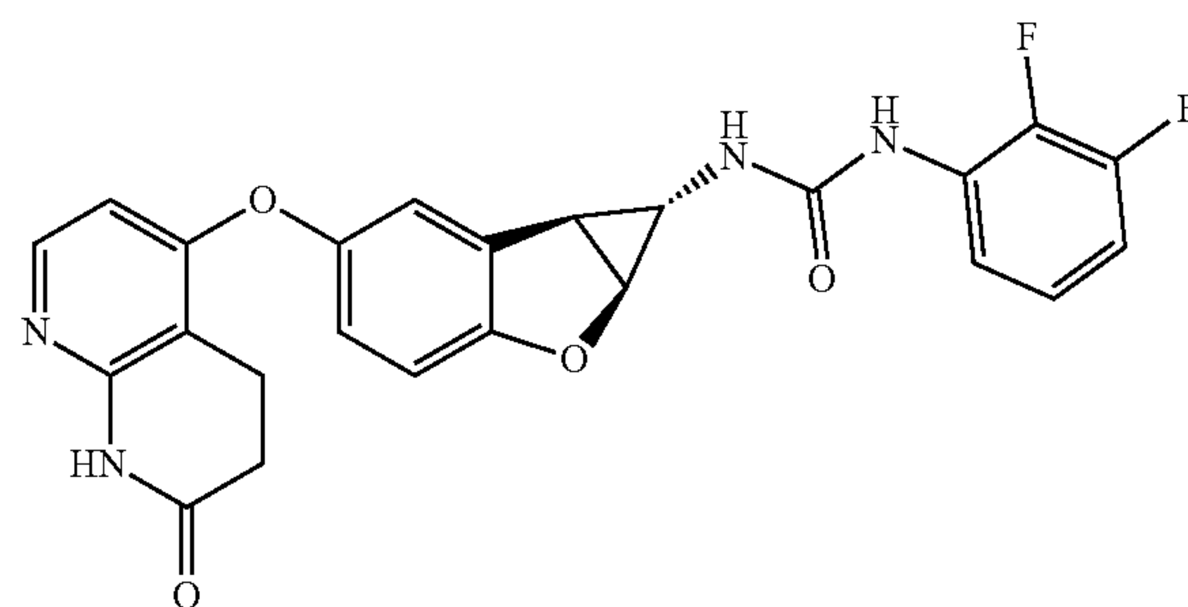
Compound 1.42
