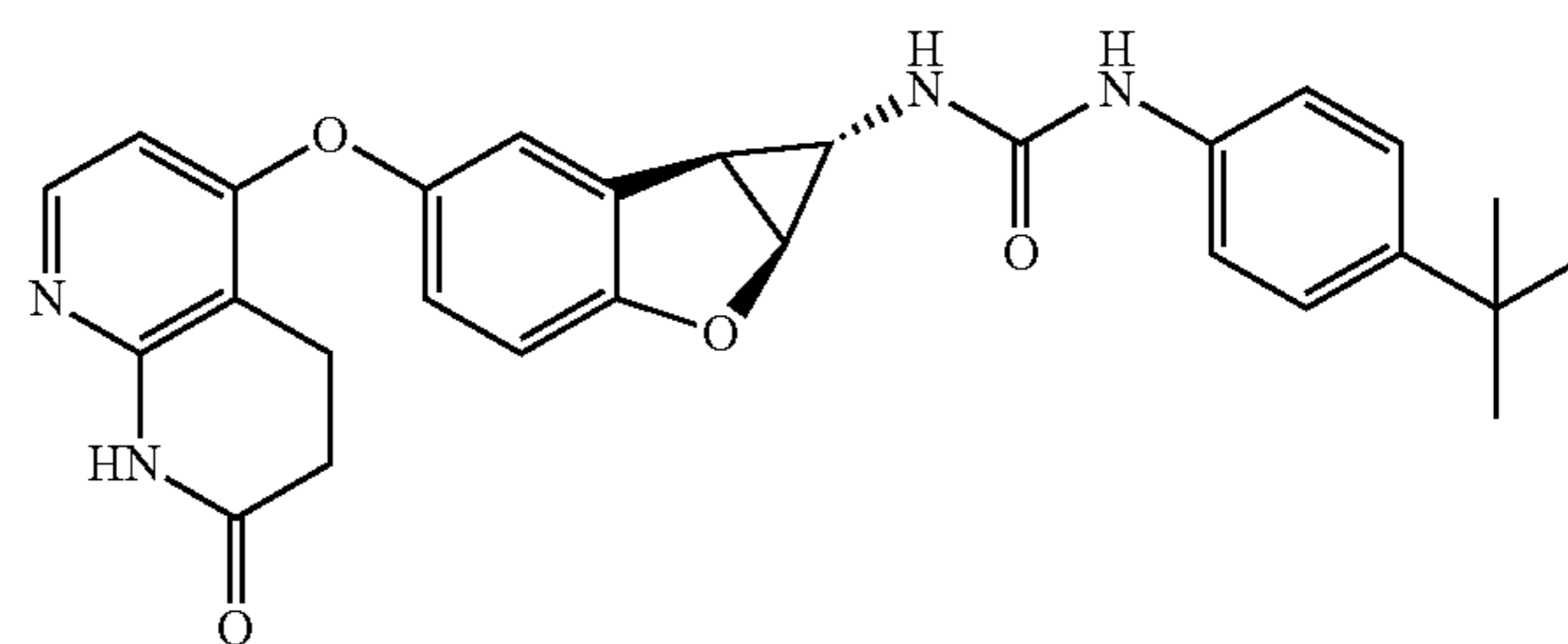
Compound 1.18
