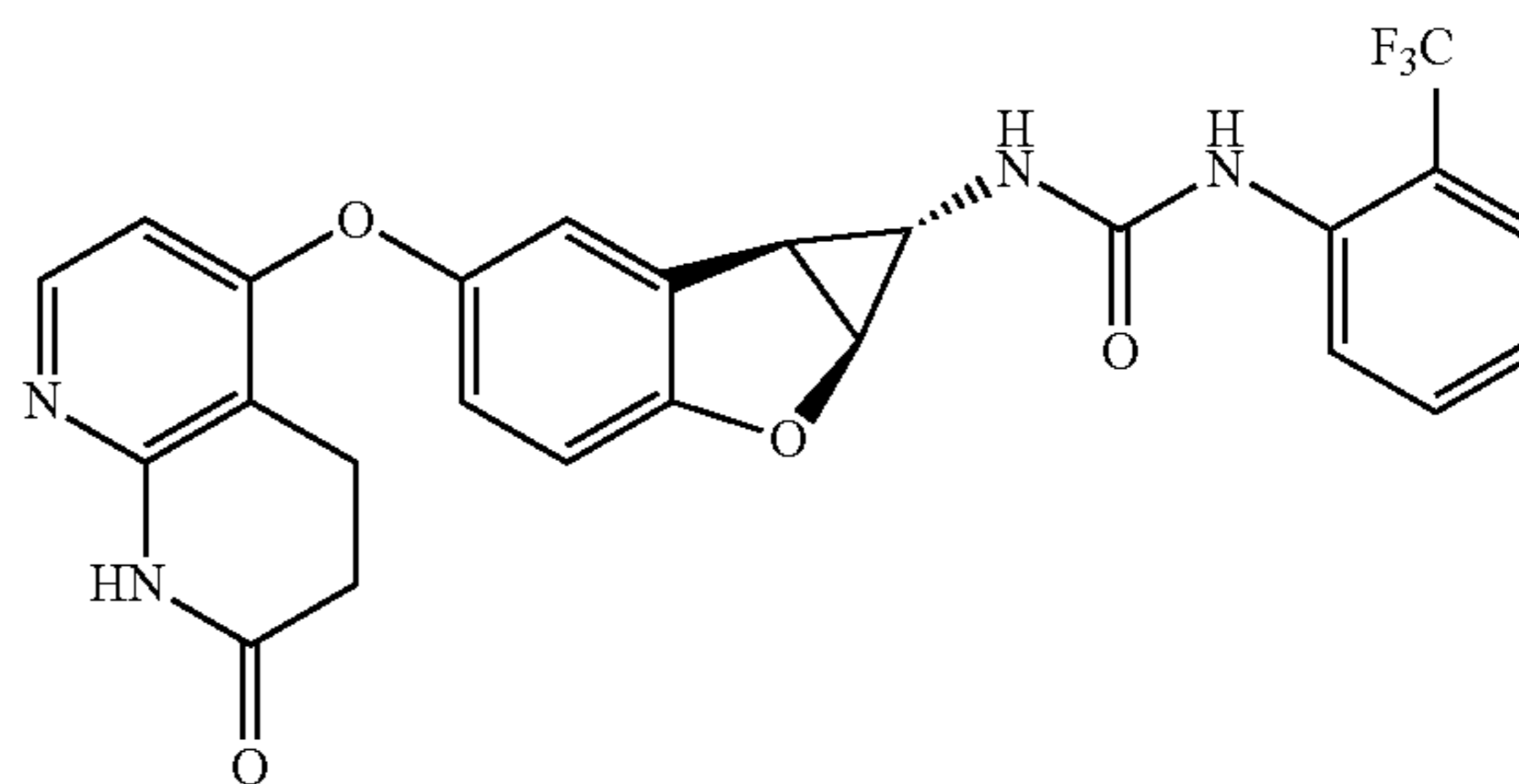
Compound 1.30
