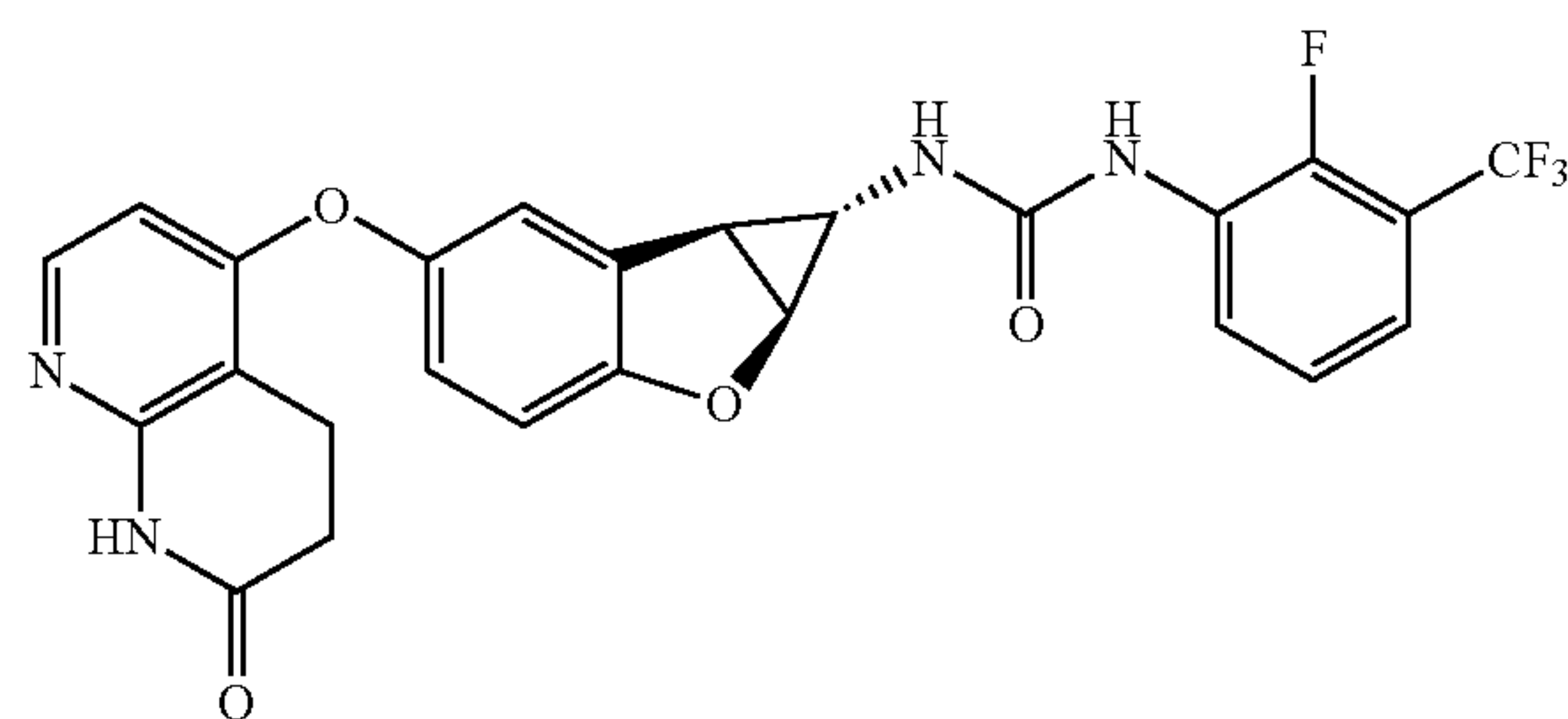
Compound 1.12
