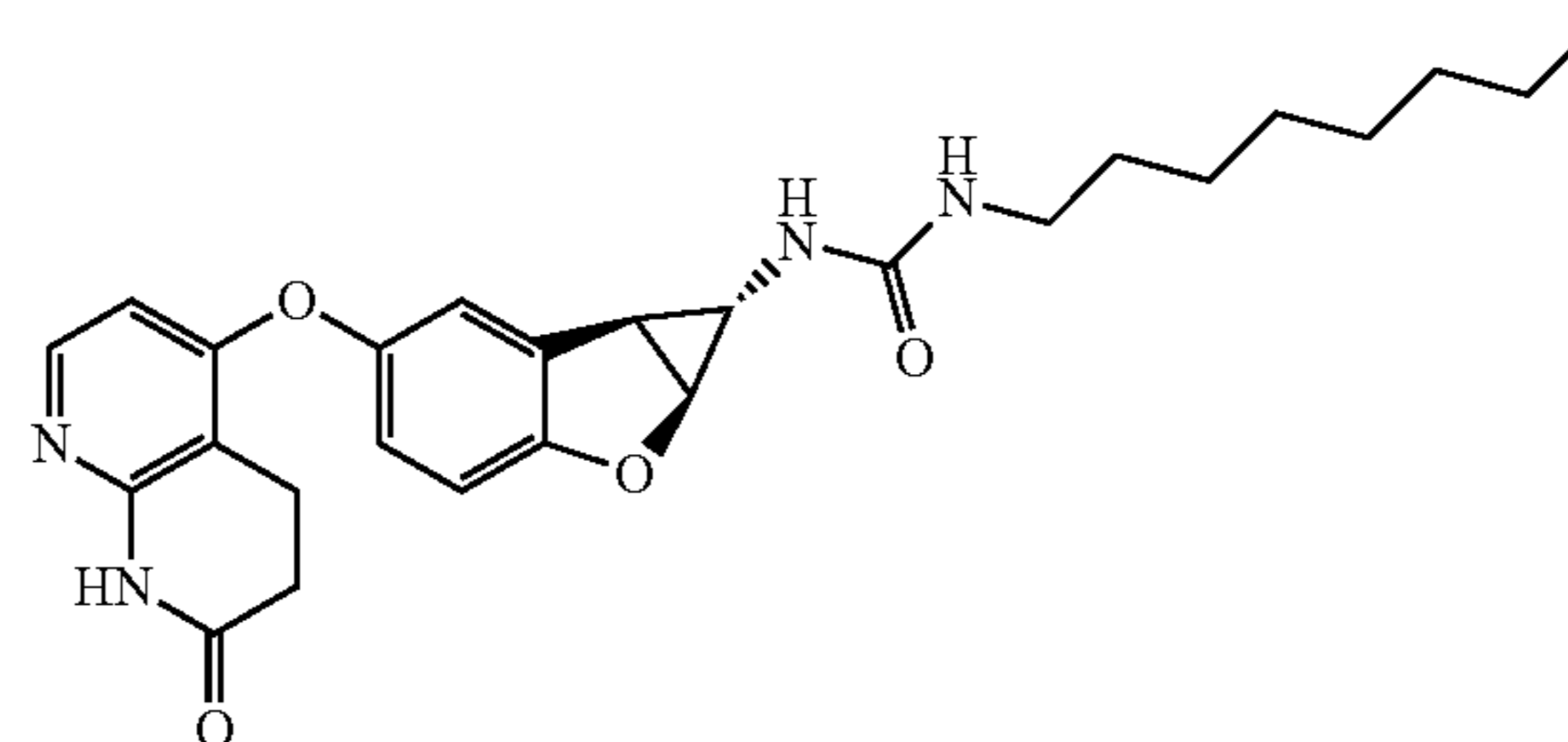
Compound 1.84
