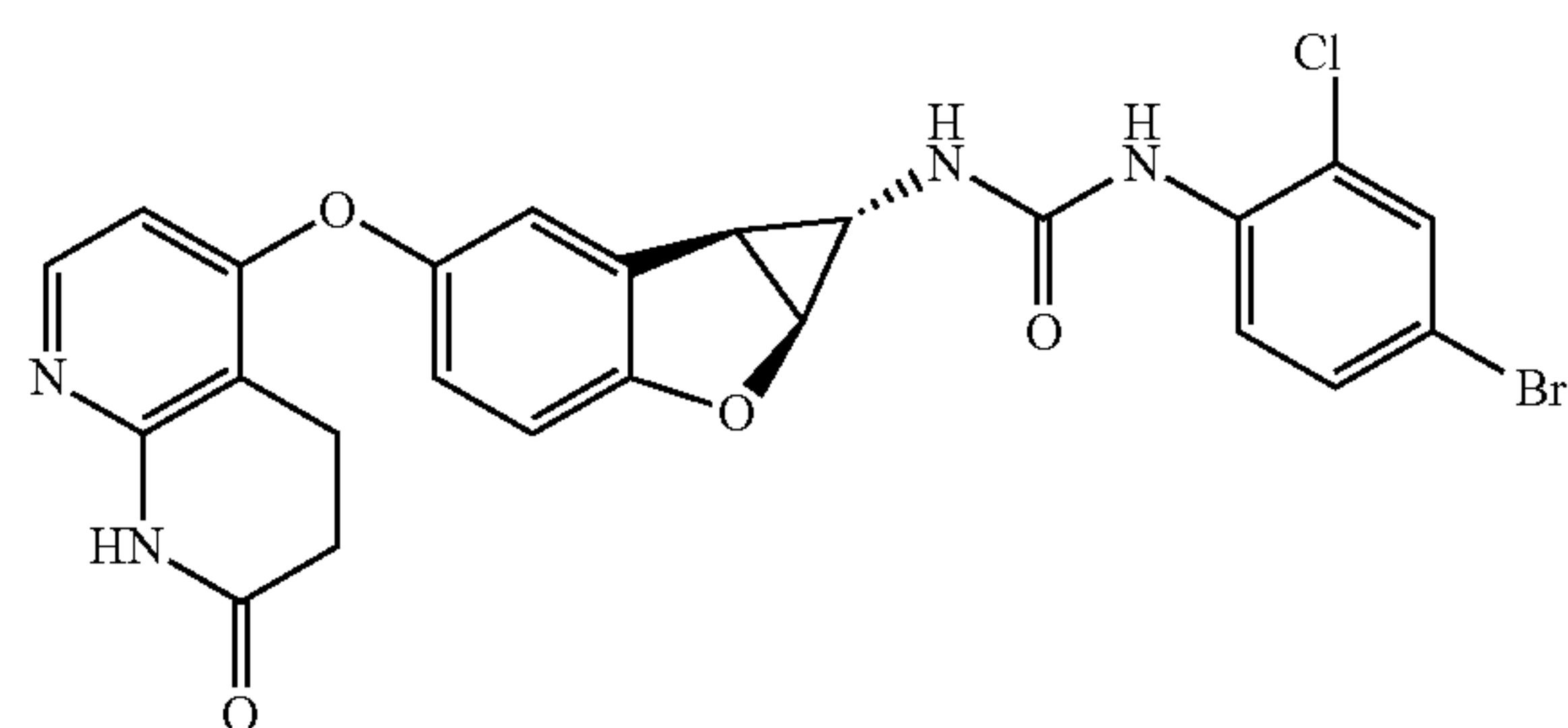
Compound 1.10
