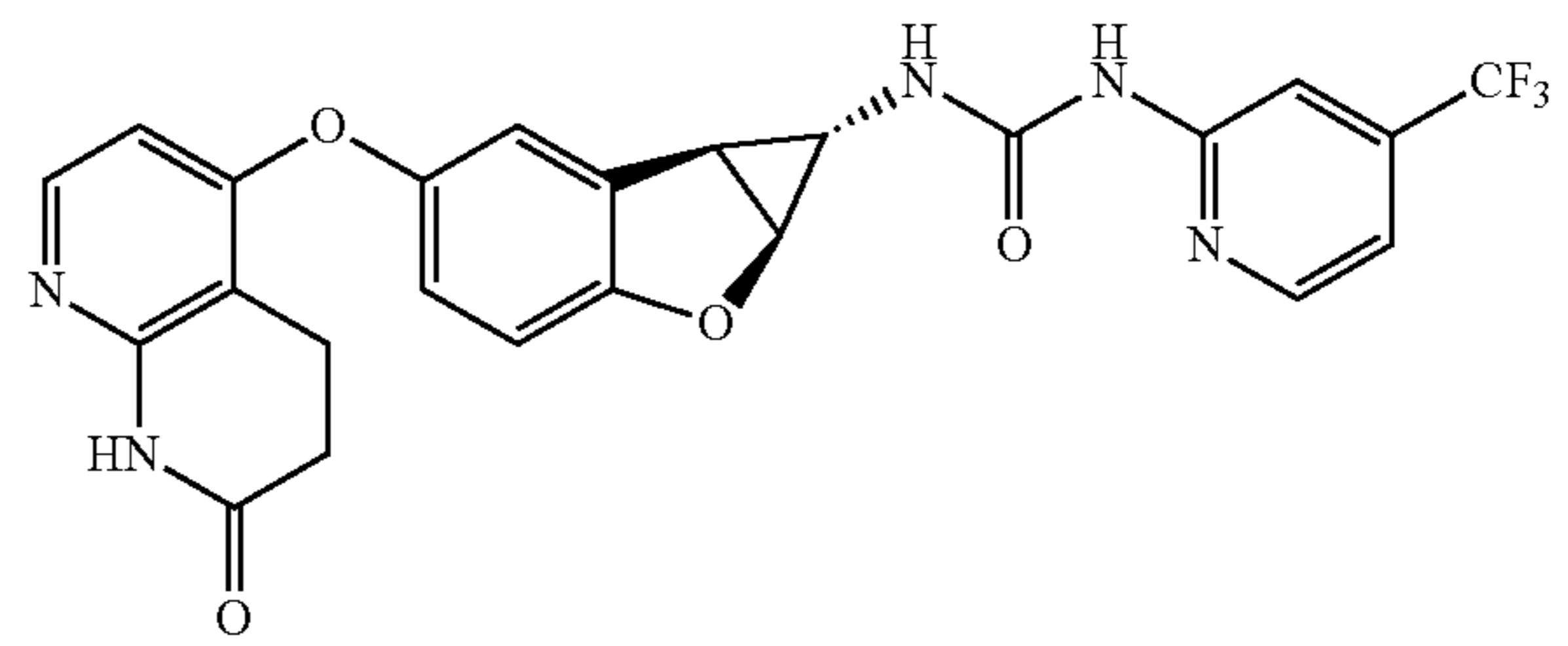
Compound 1.2
