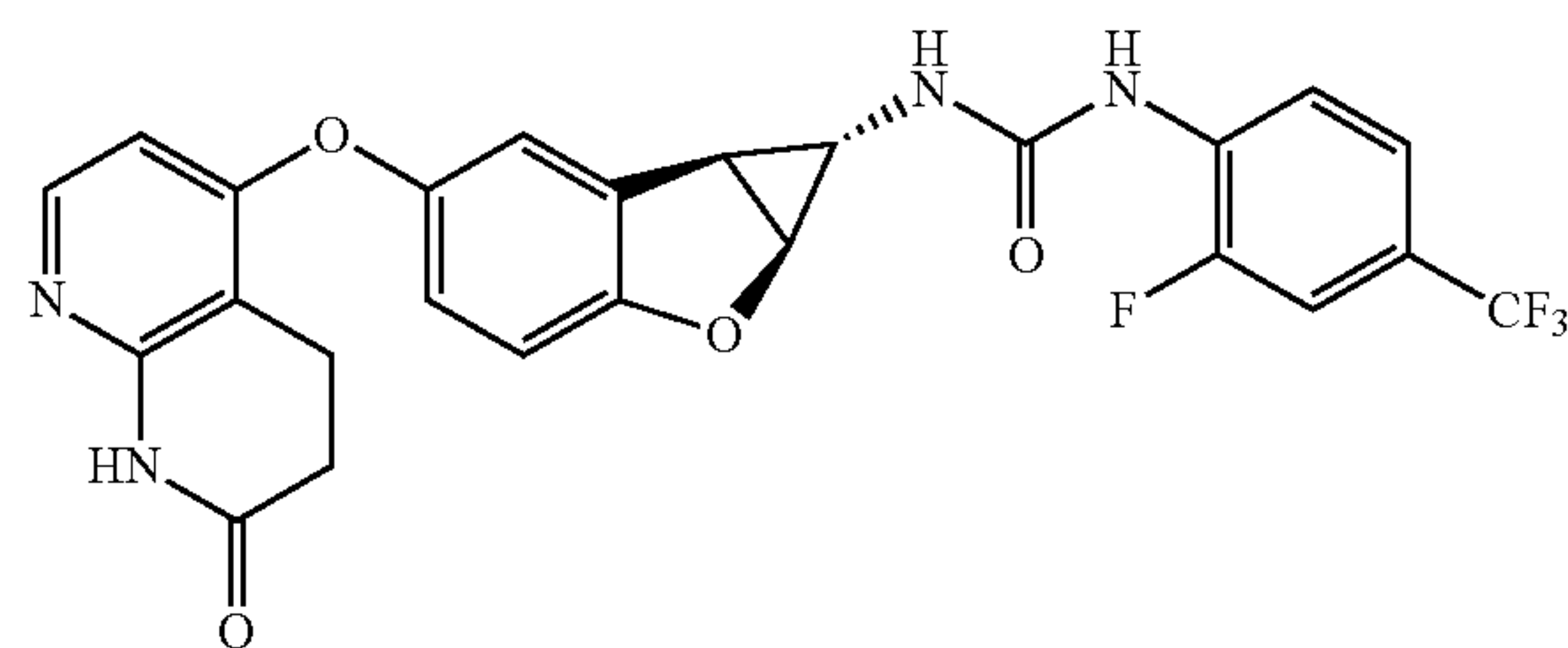
Compound 1.20
