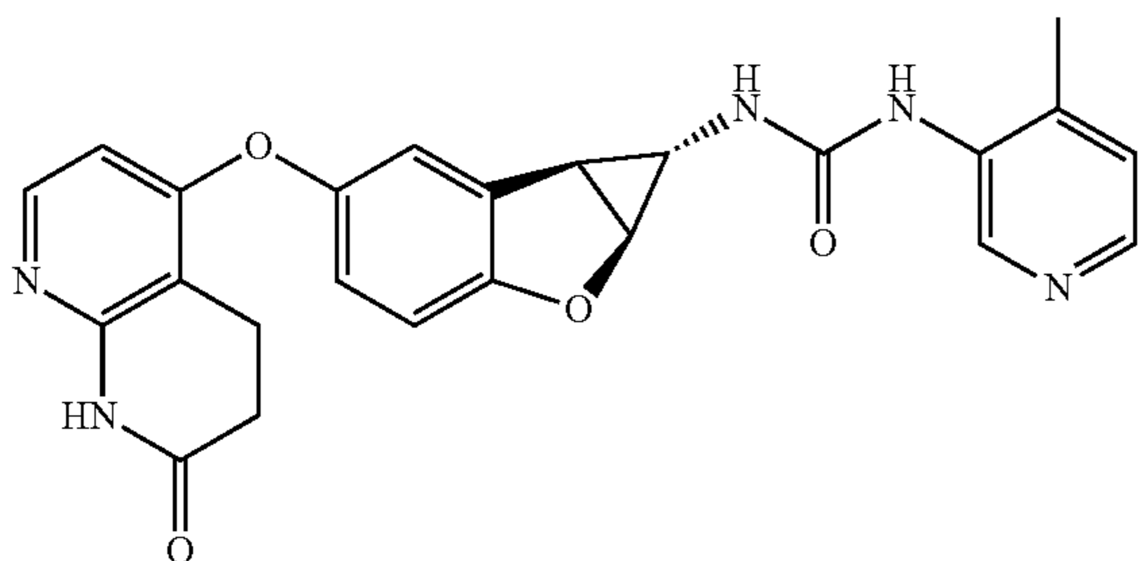
Compound 1.39
