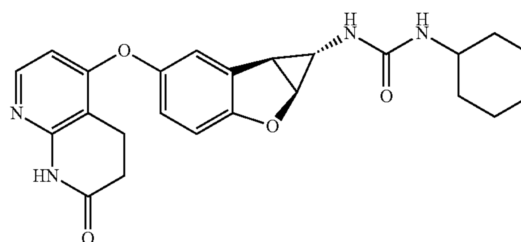
Compound 1.68
