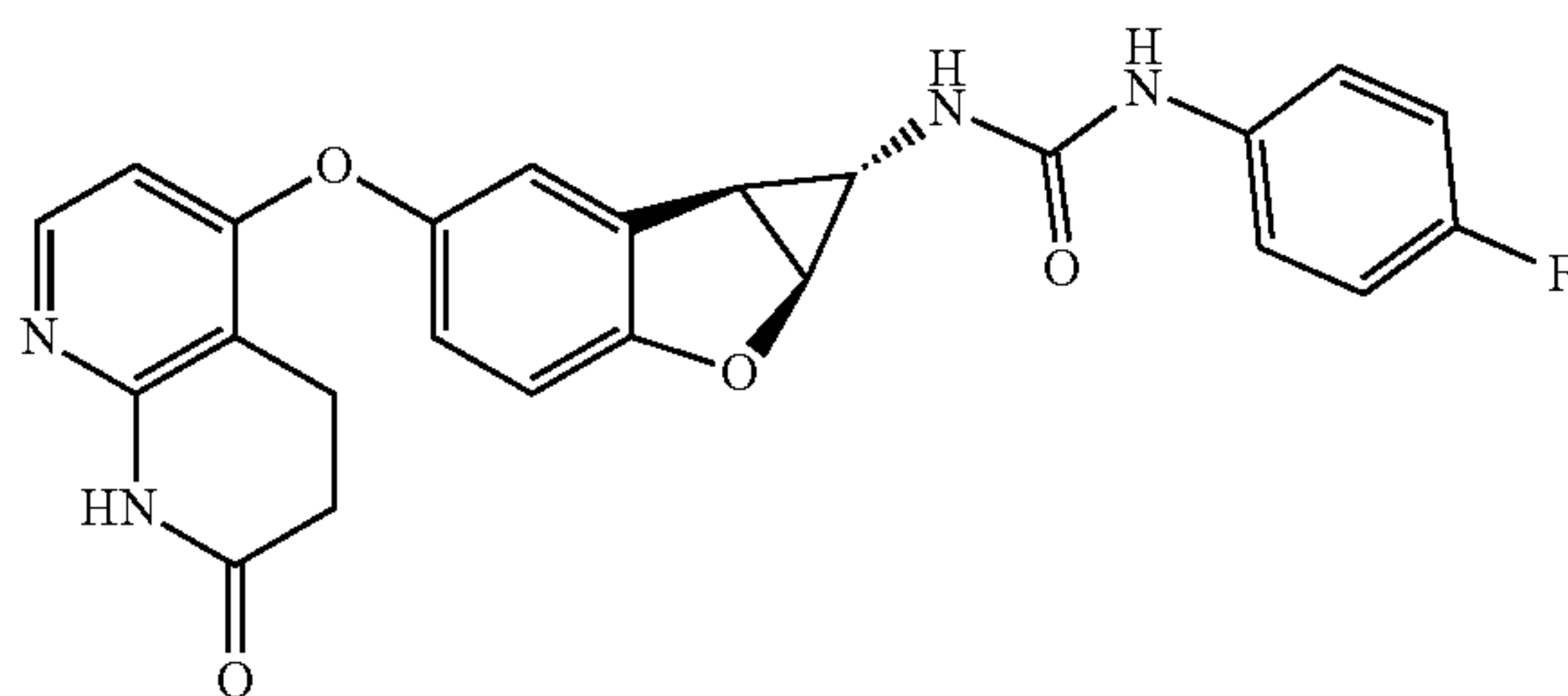
Compound 1.41
