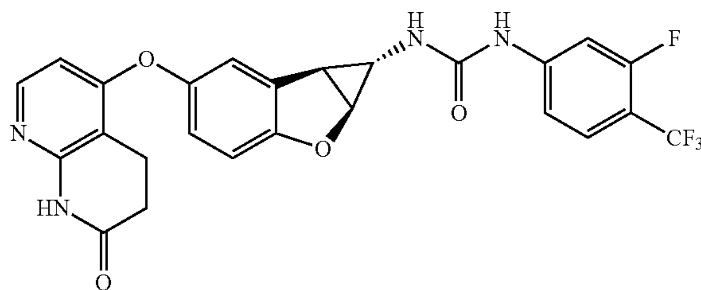
Compound 1.66
