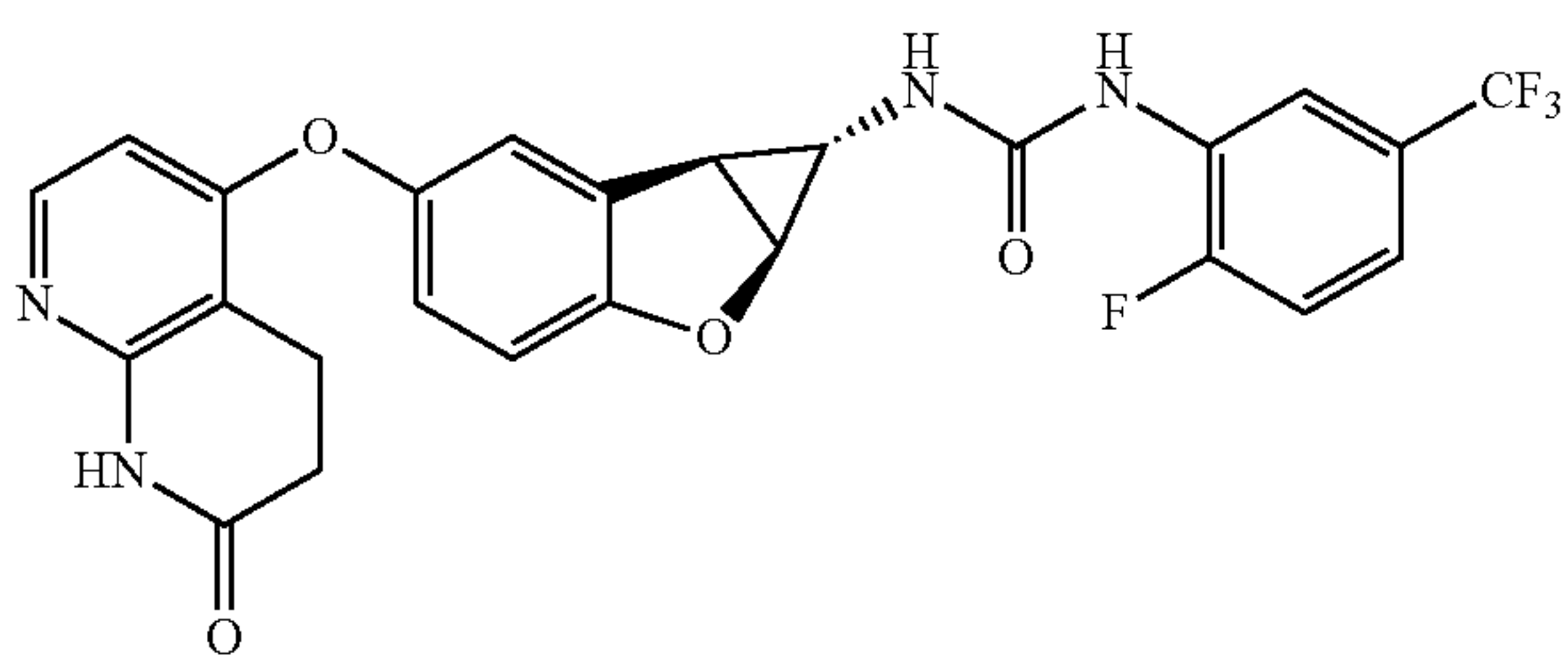
Compound 1.33
