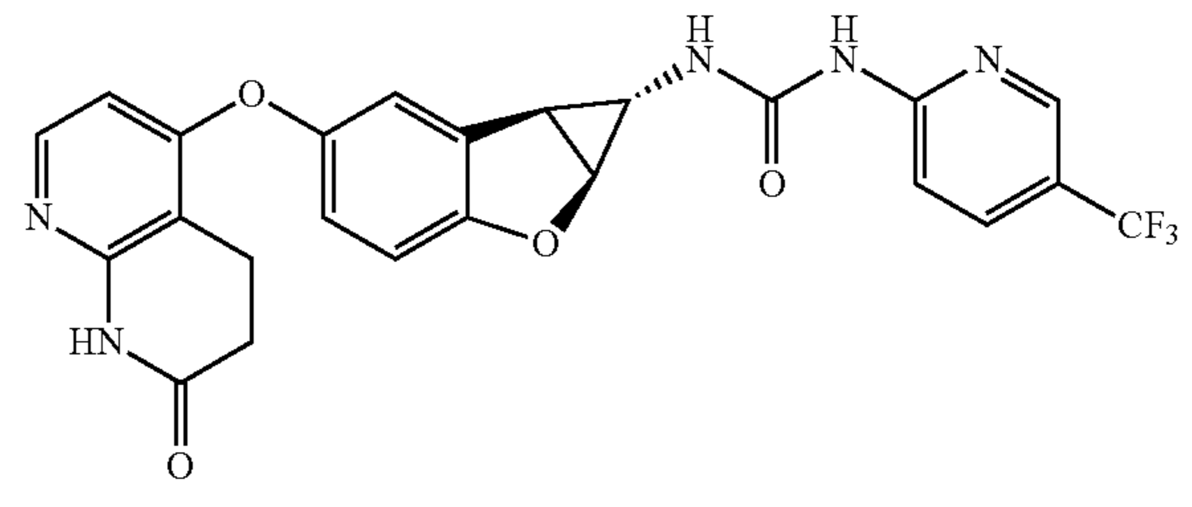
Compound 1.38
