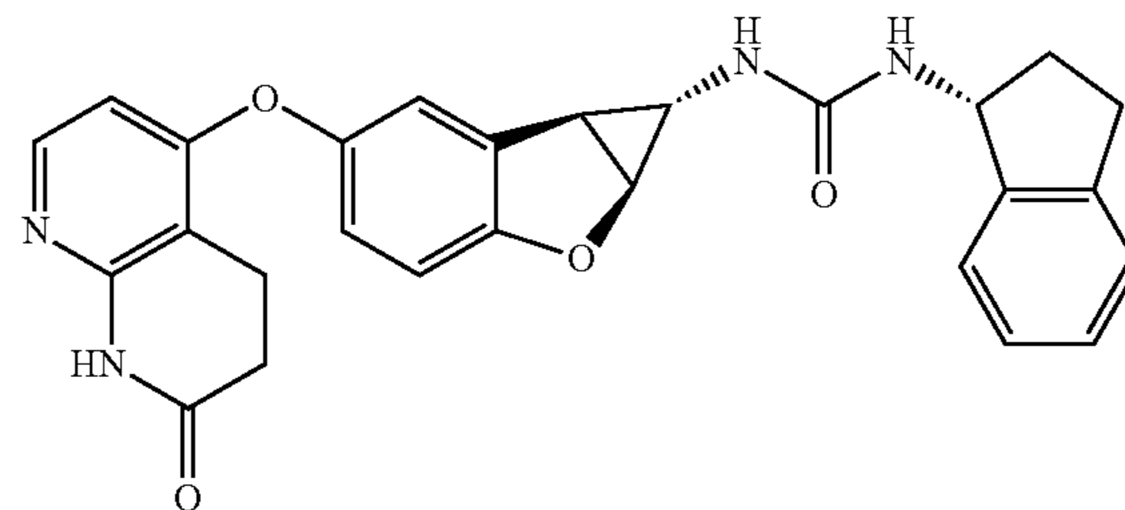
Compound 1.84
