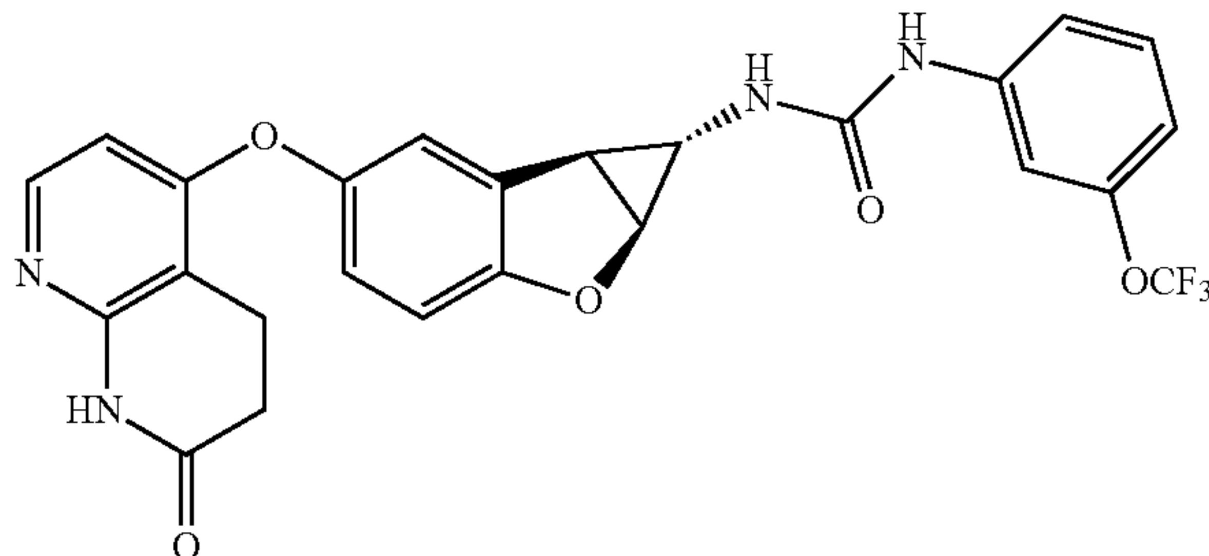
Compound 1.60
