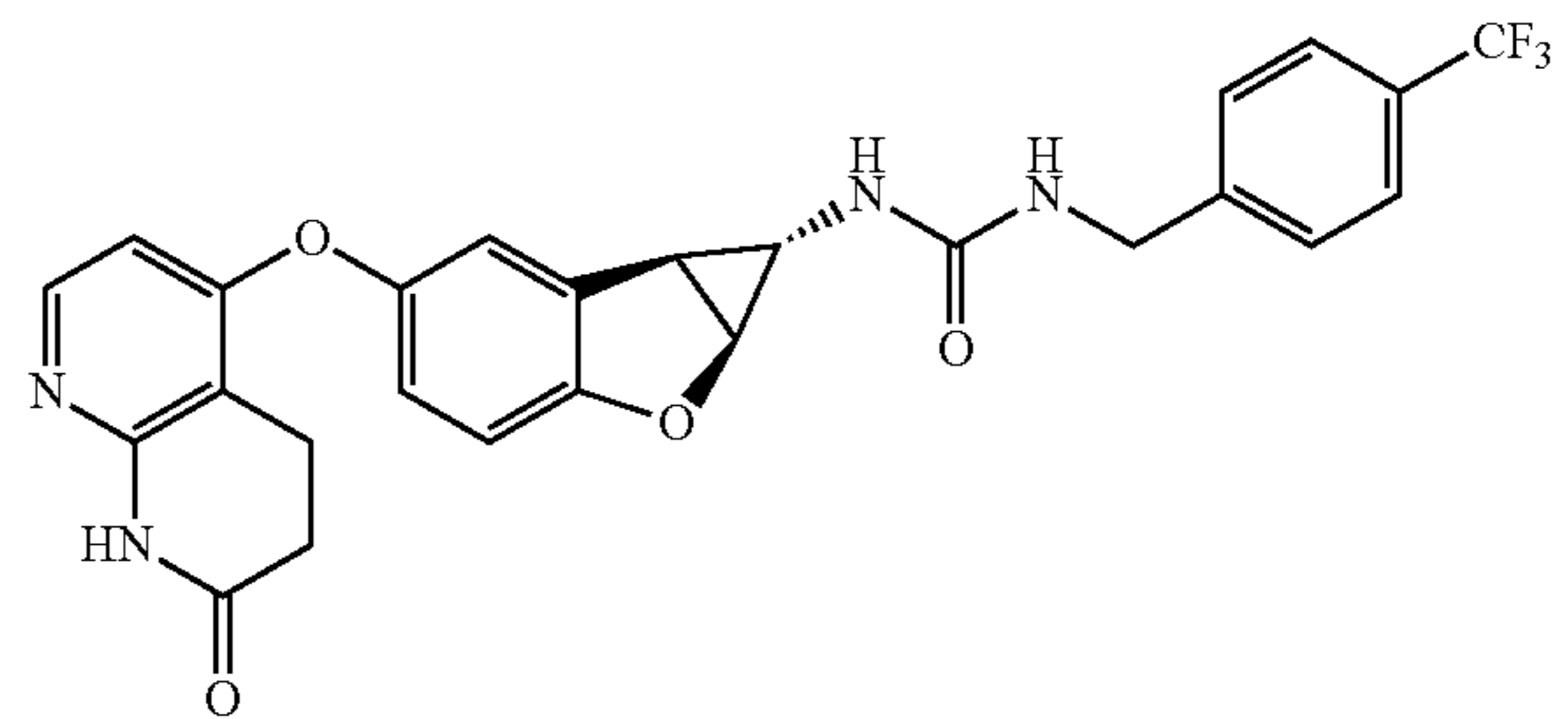
Compound 1.56
