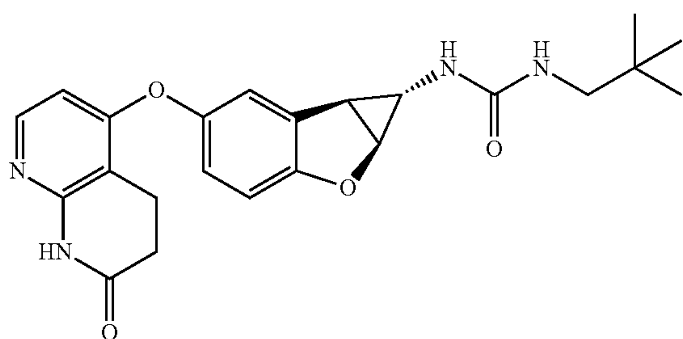
Compound 1.83
