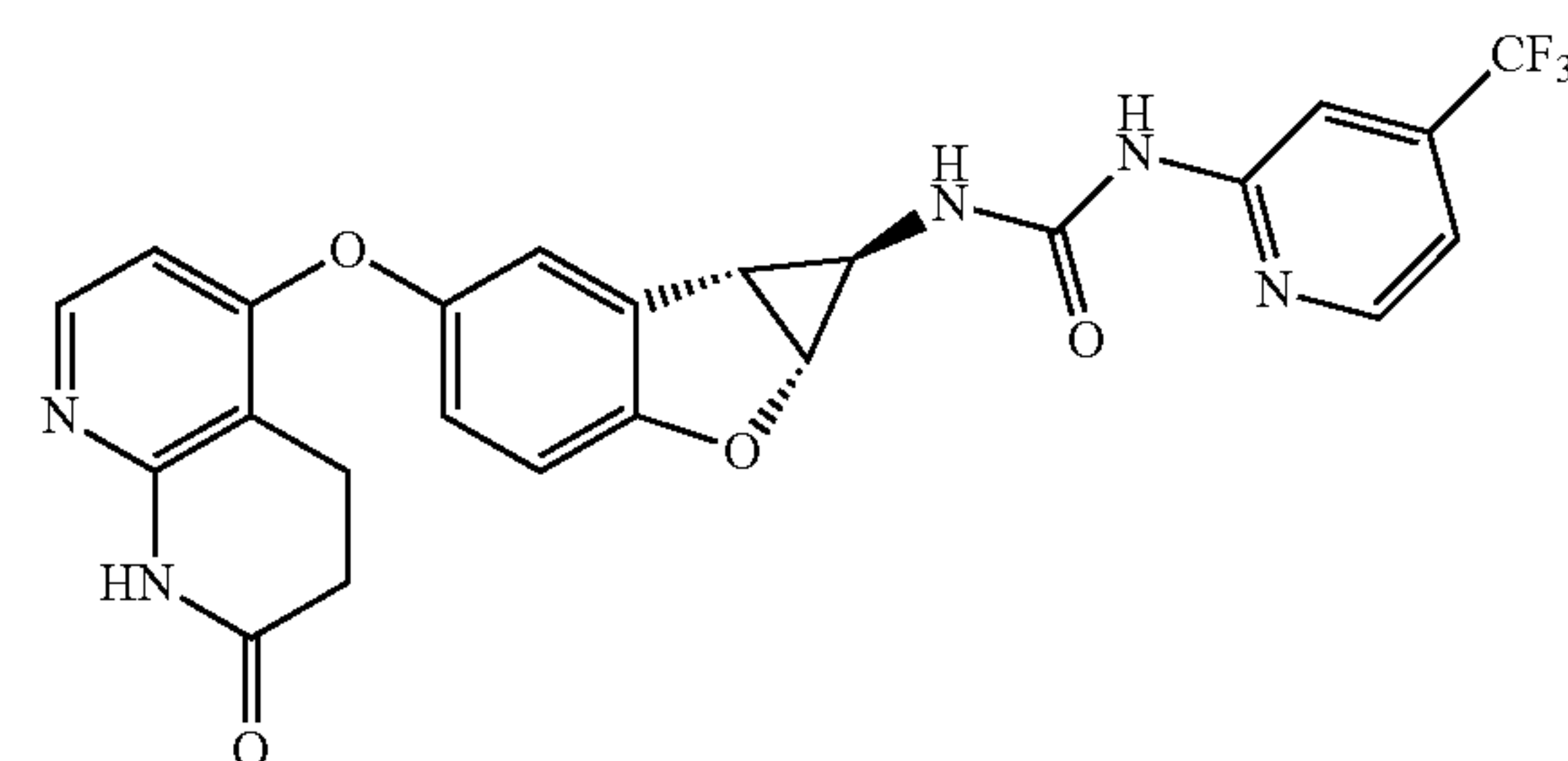
Compound 1.72
