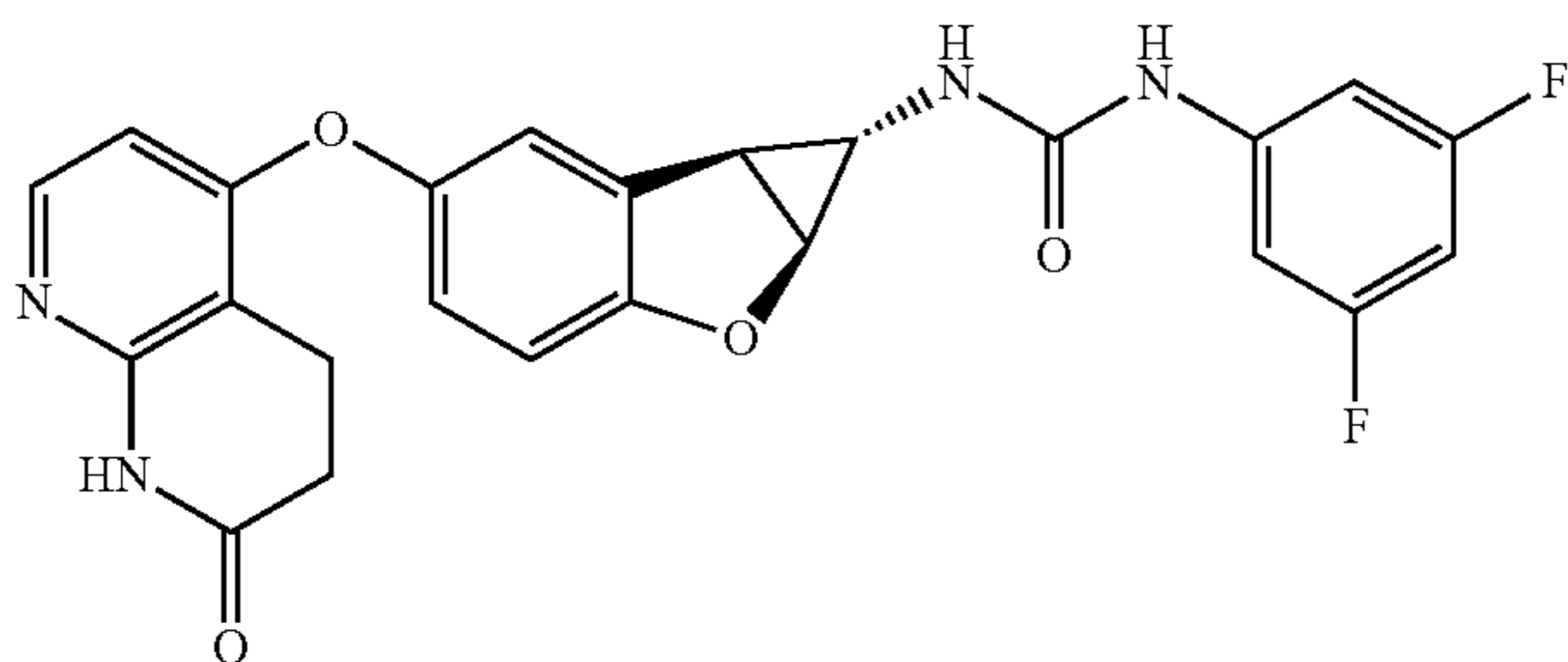
Compound 1.23
