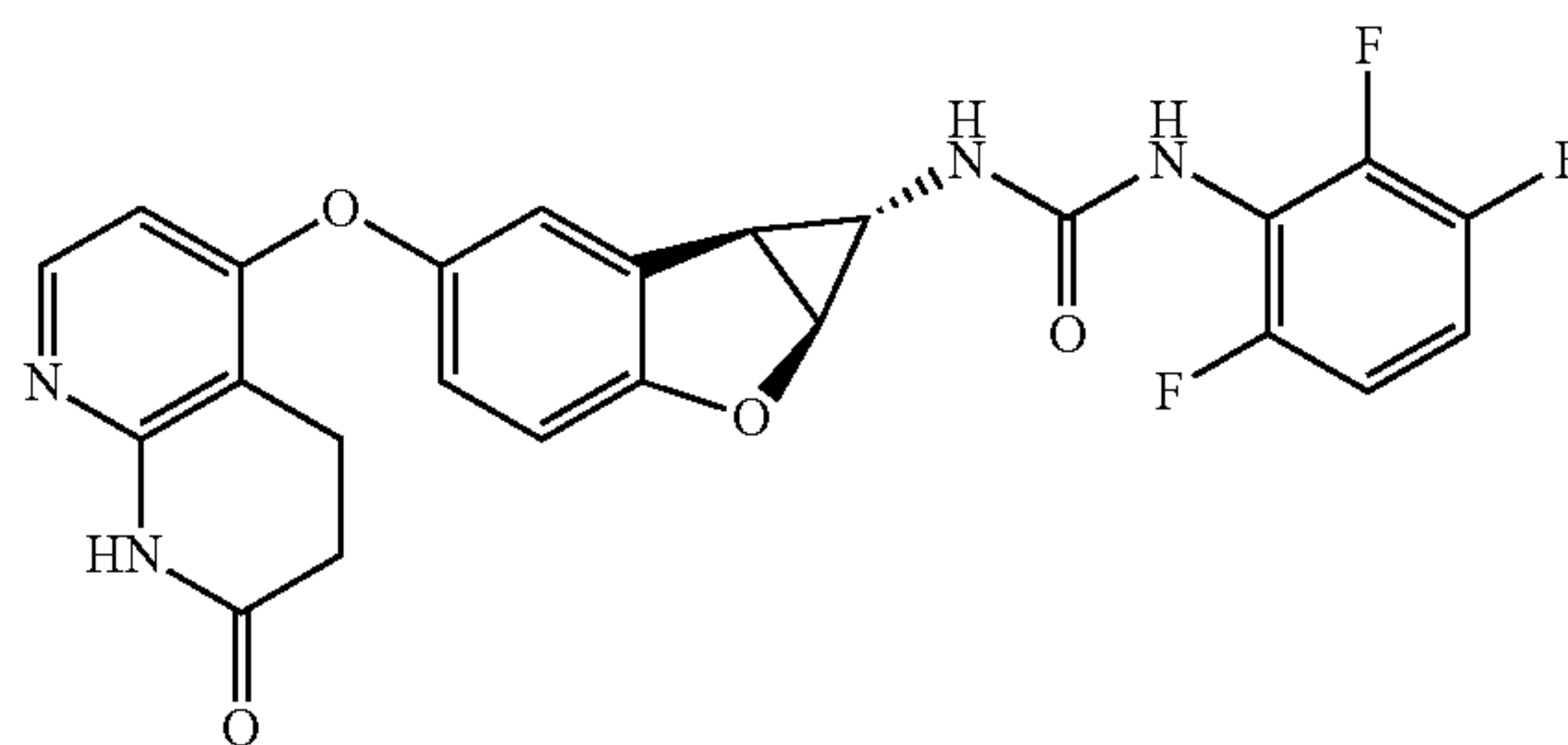
Compound 1.48
