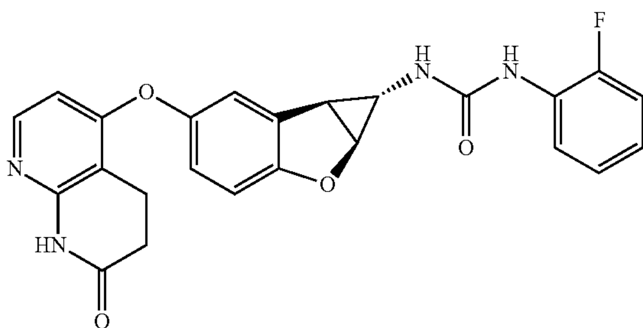
Compound 1.21
