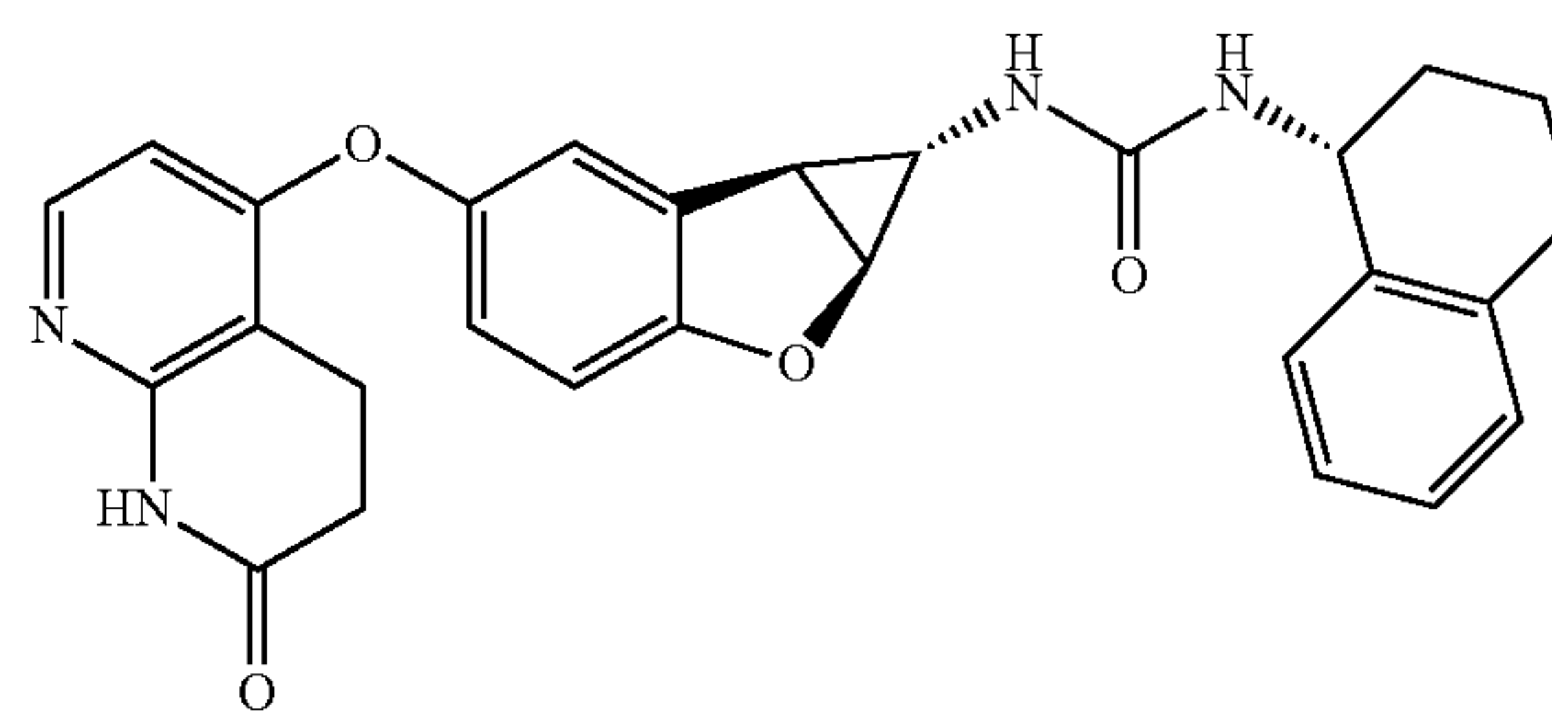
Compound 1.82
