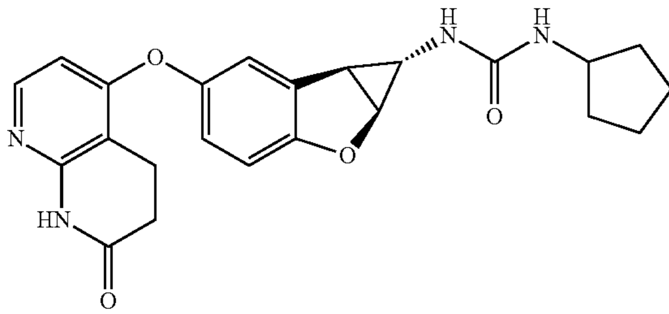
Compound 1.51
