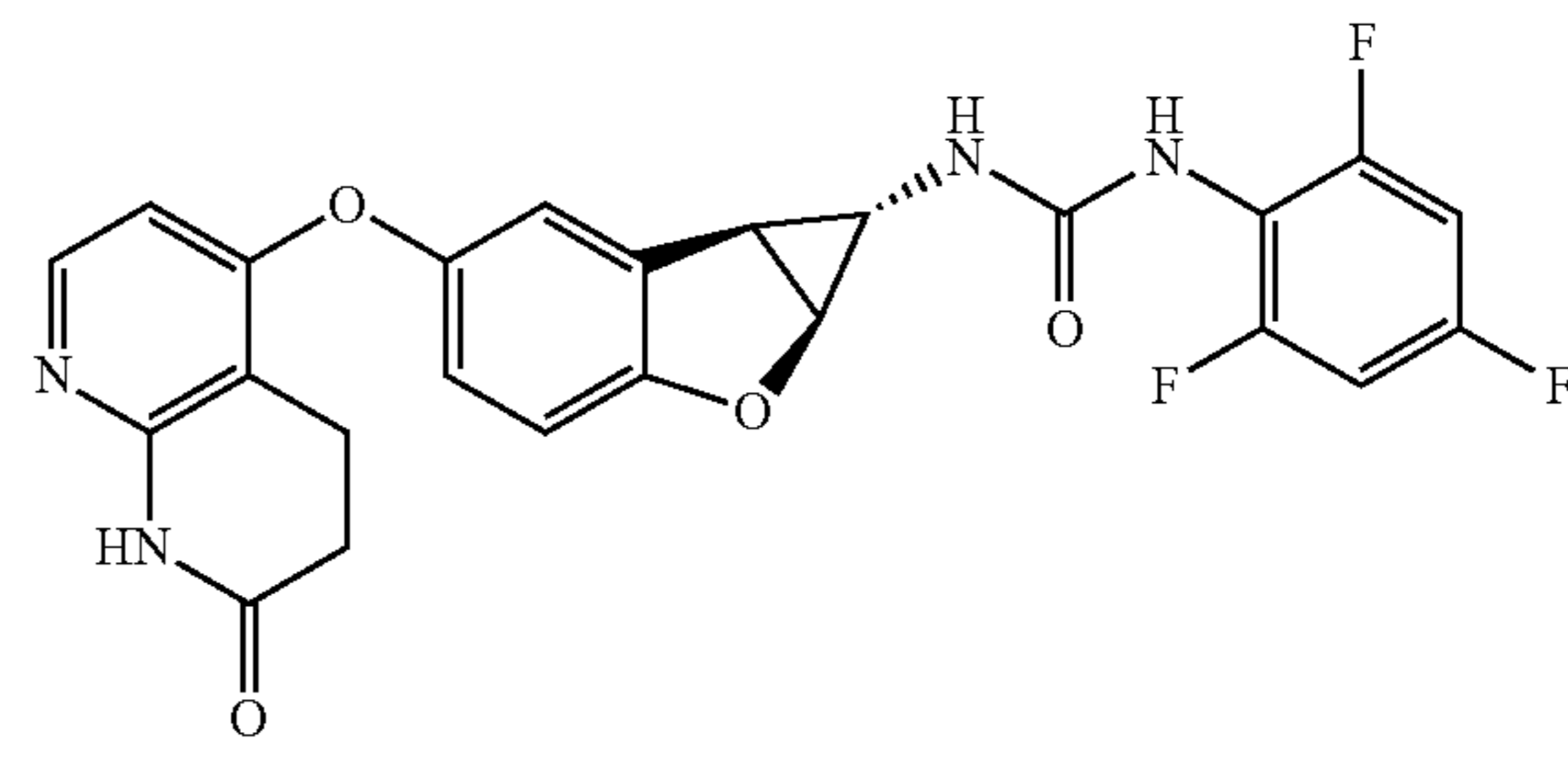
Compound 1.40
