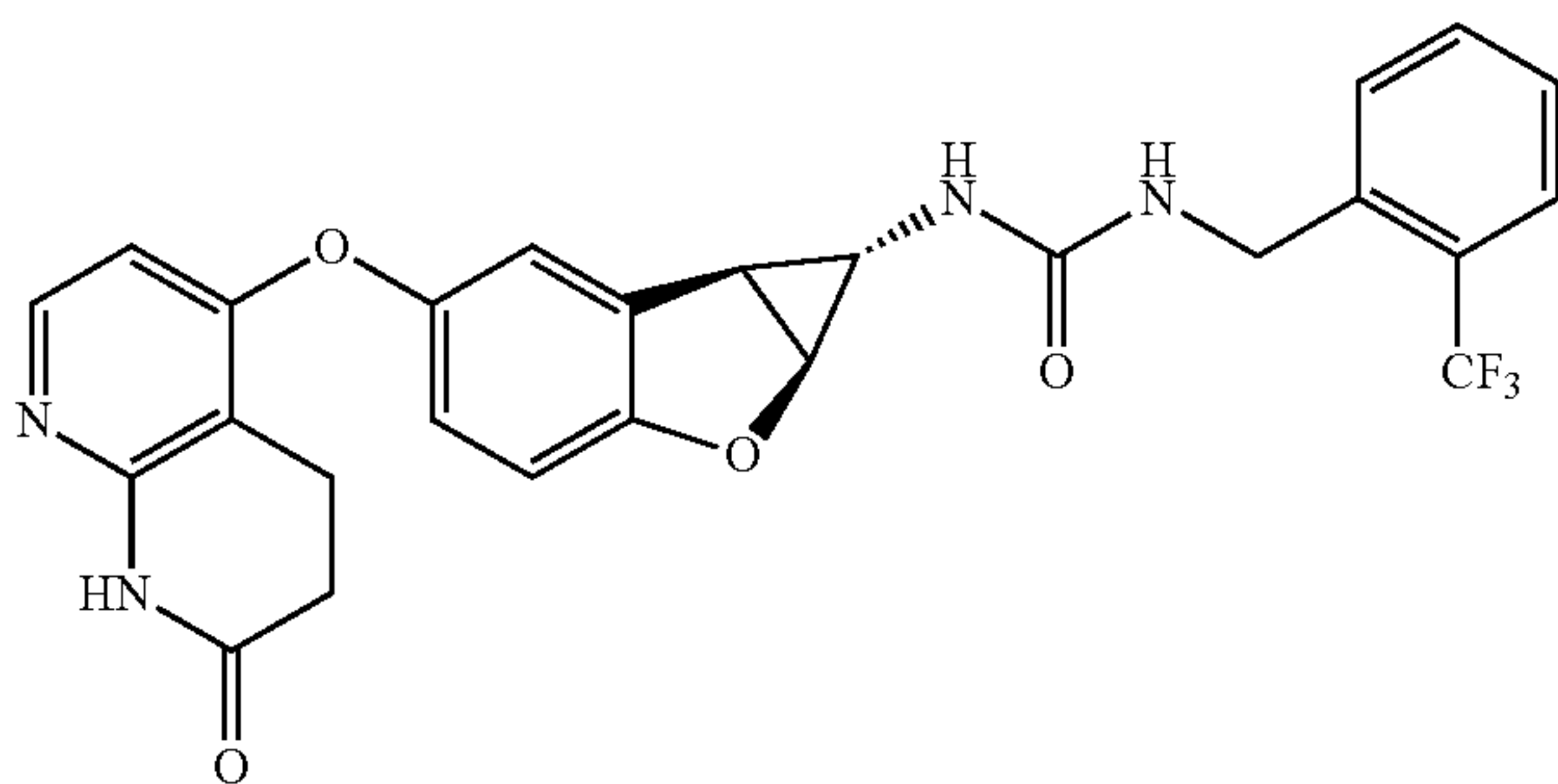
Compound 1.55
