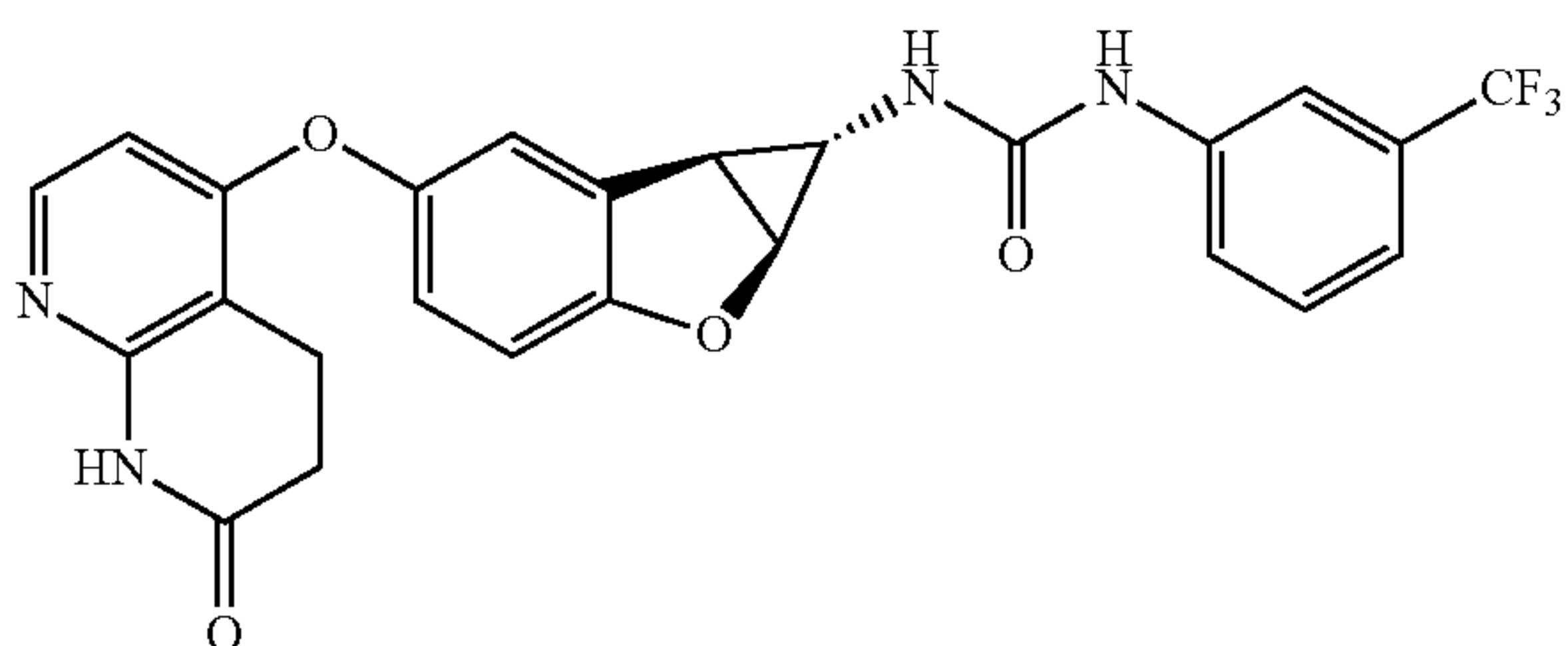
Compound 1.1
