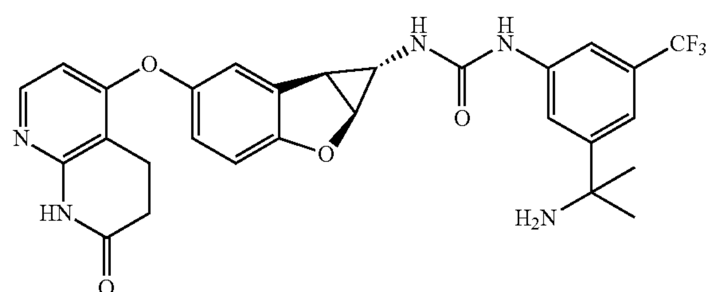
Compound 1.72
