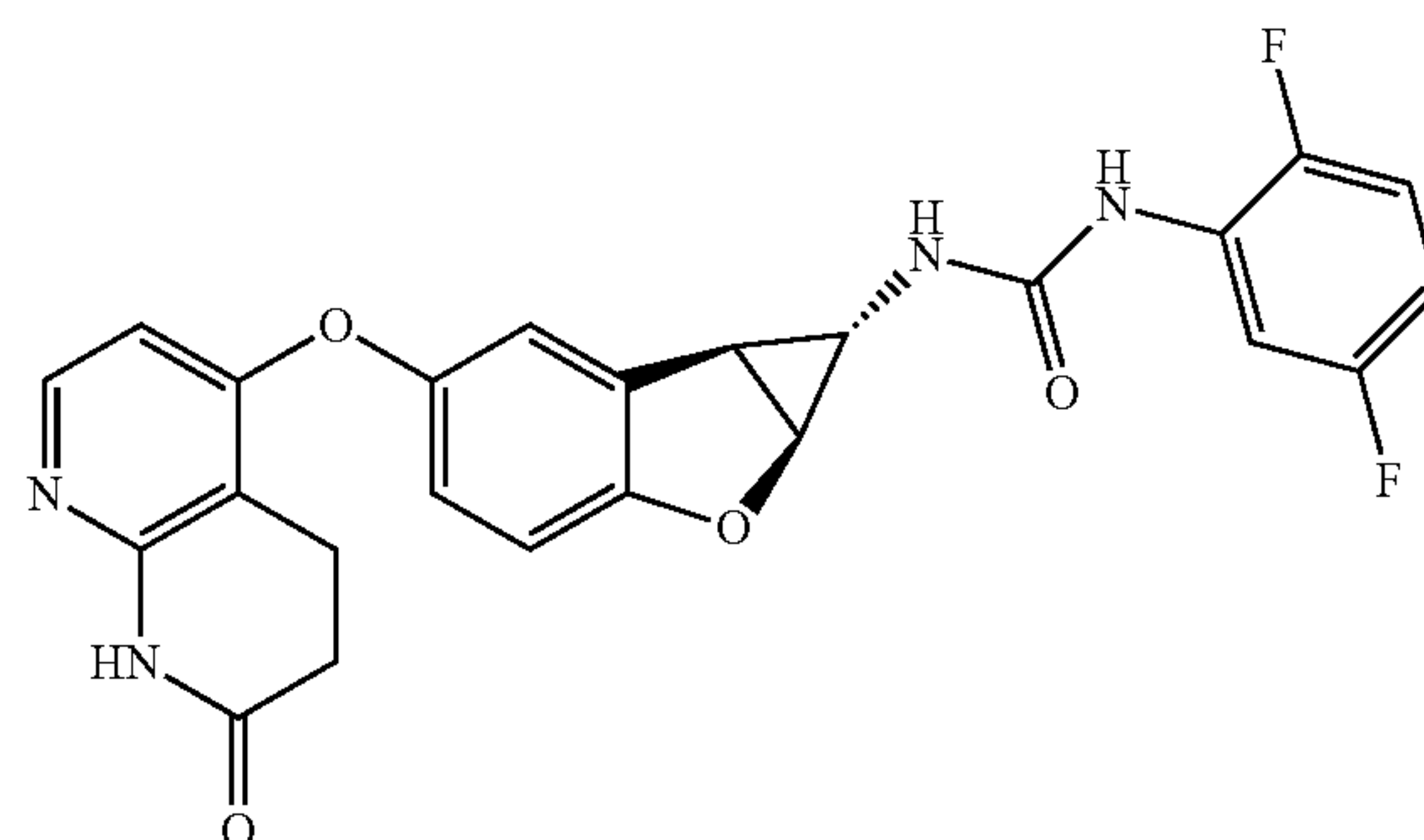
Compound 1.43
