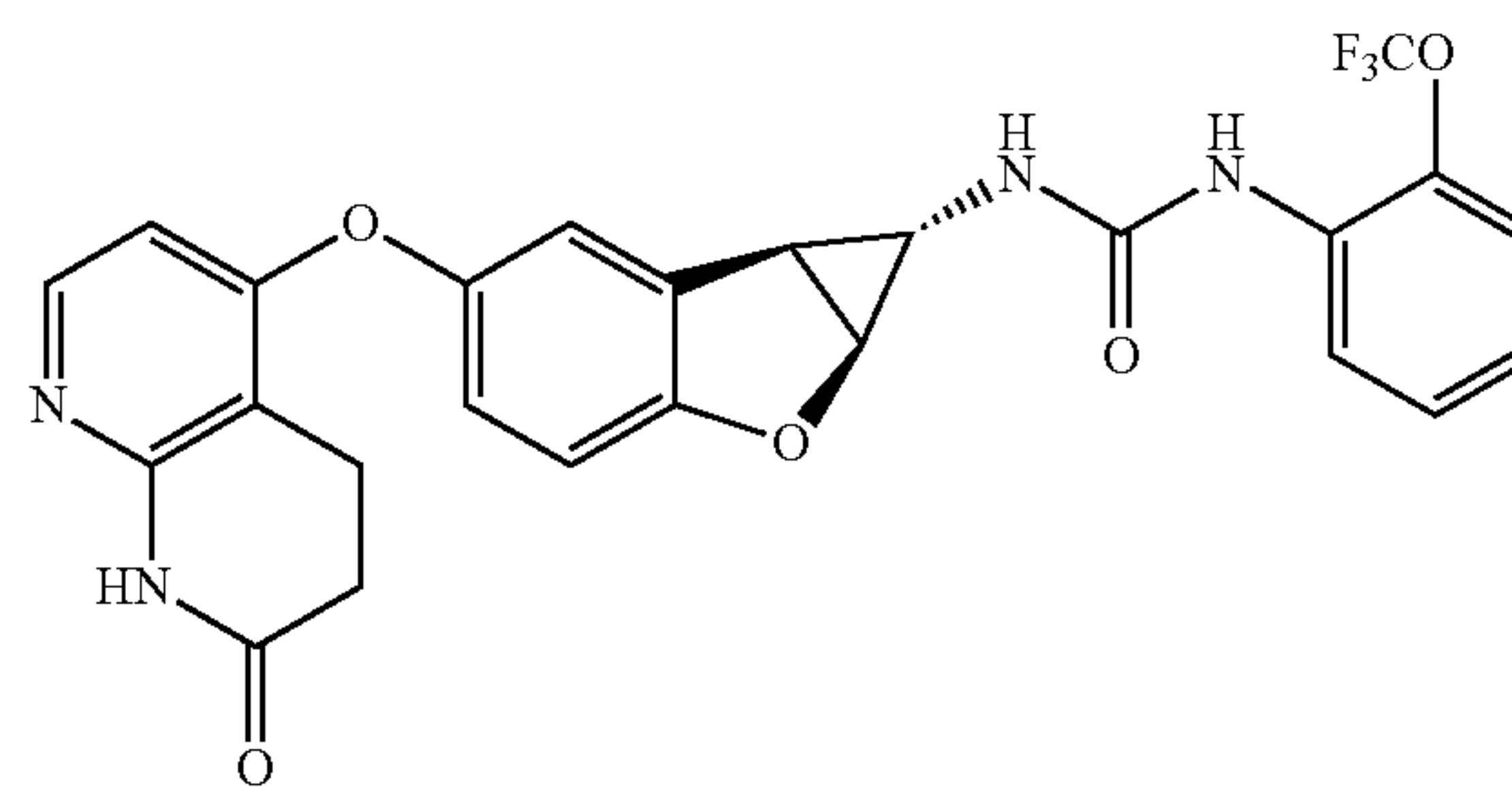
Compound 1.64
