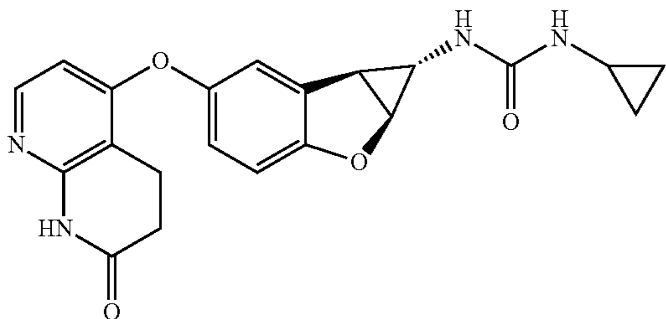
Compound 1.71
