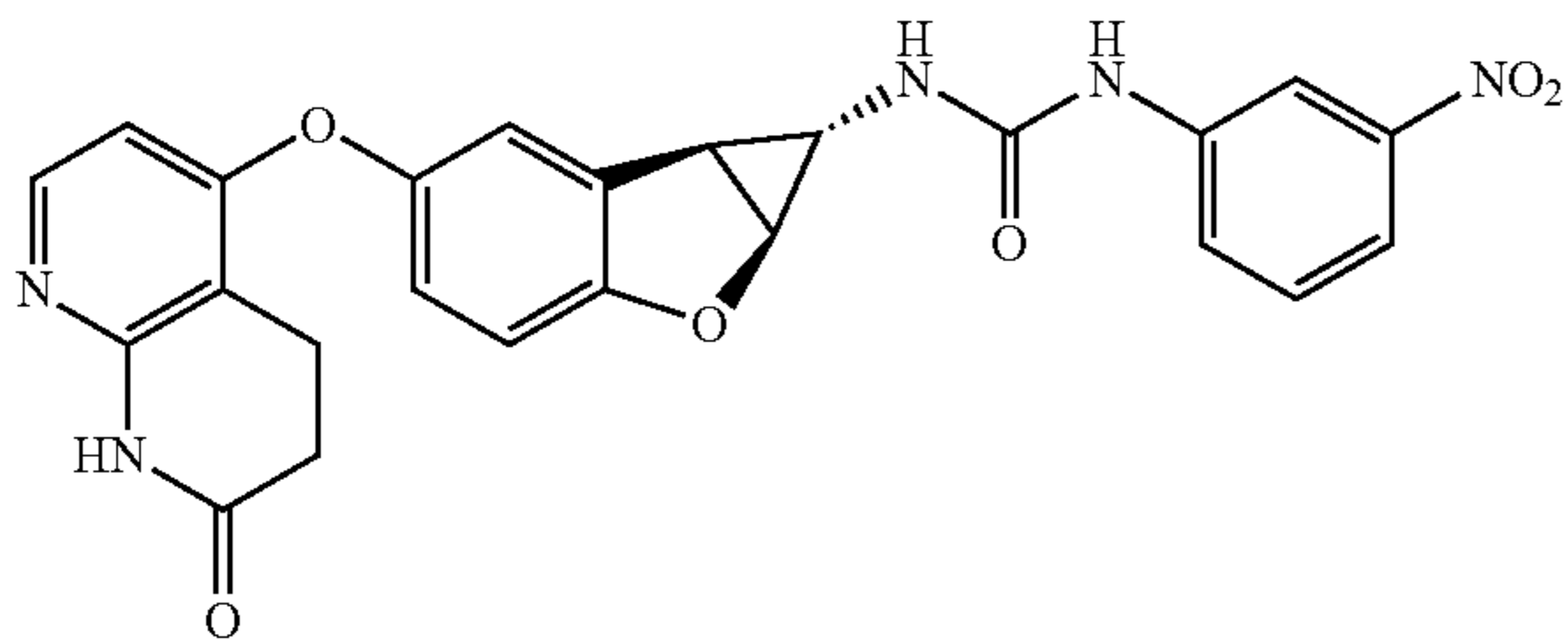
Compound 1.13
