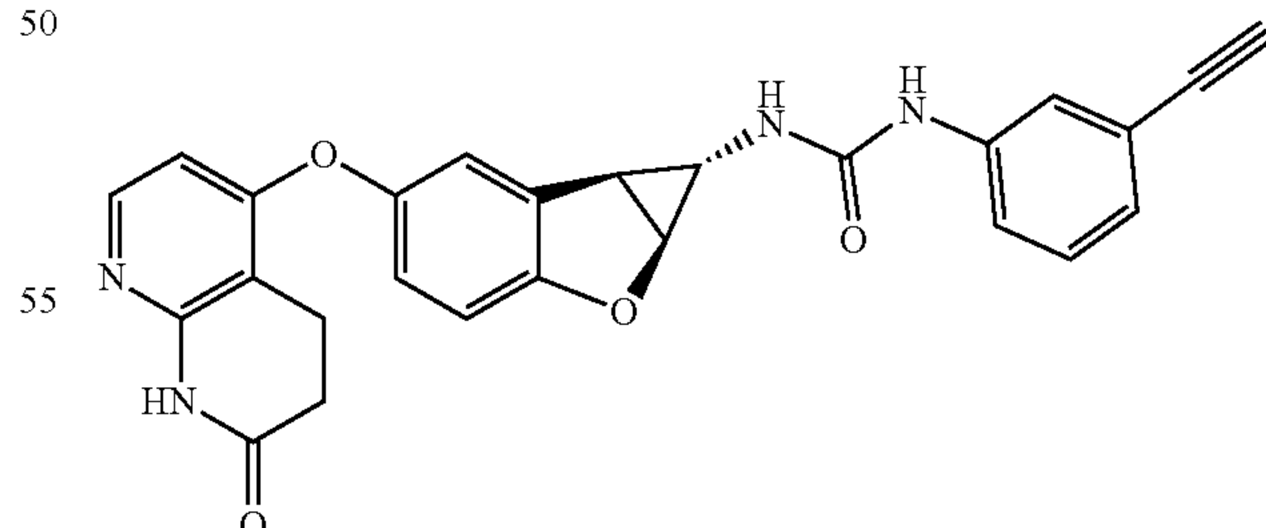
Compound 1.14
