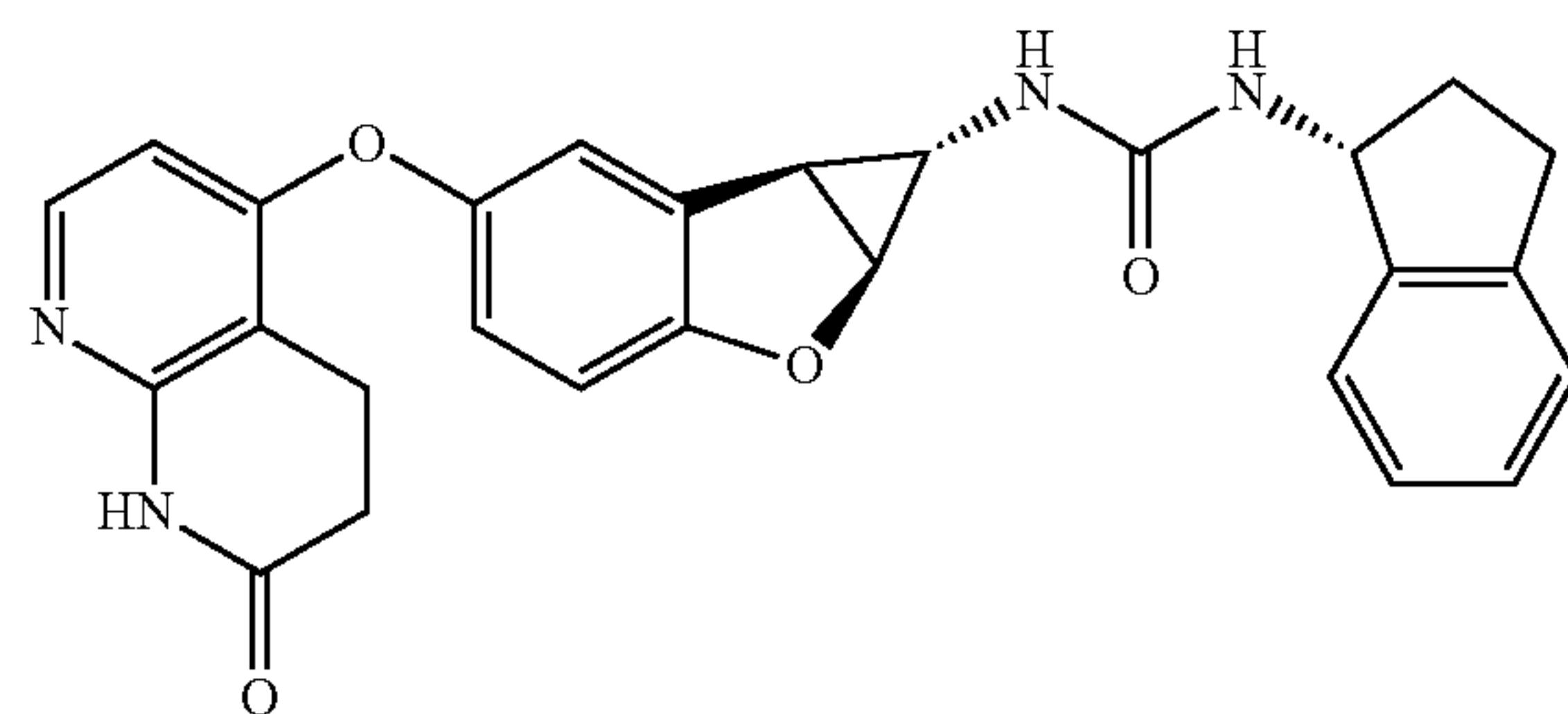
Compound 1.84
