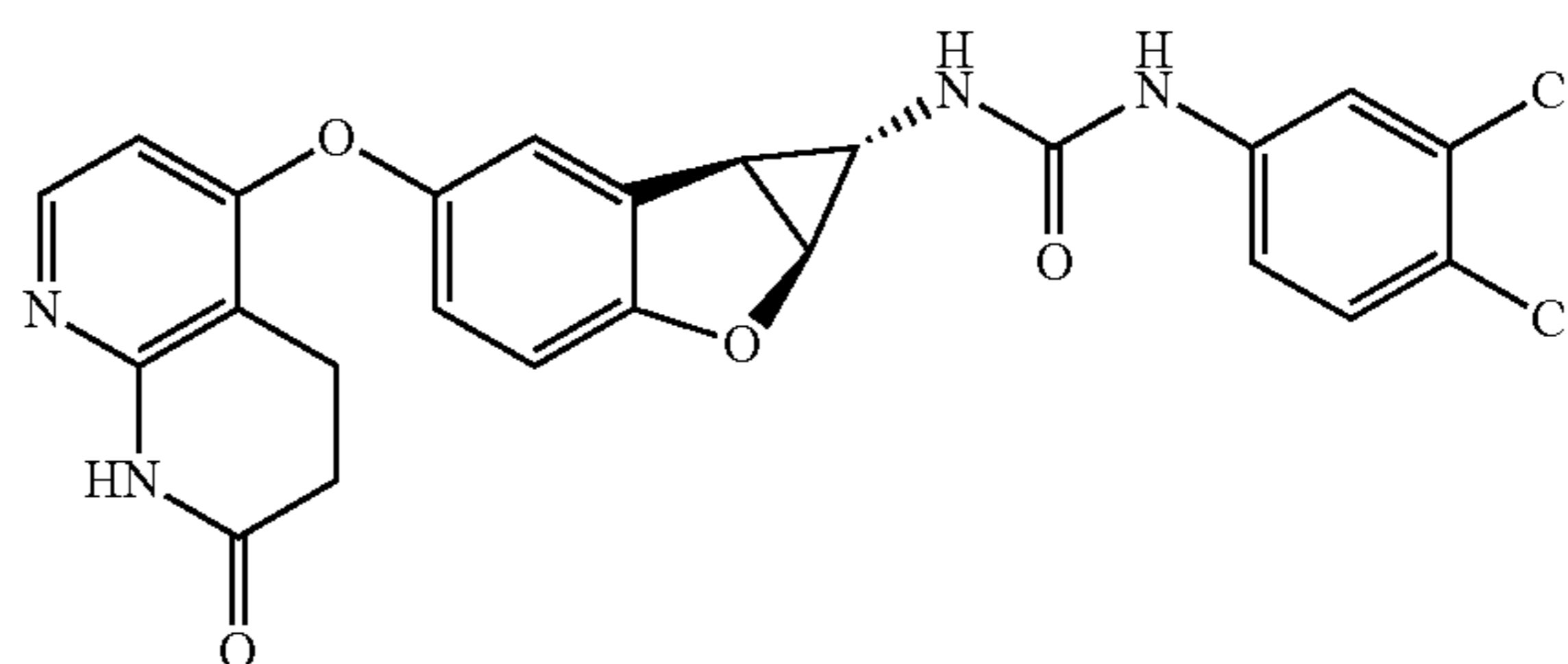
Compound 1.28
