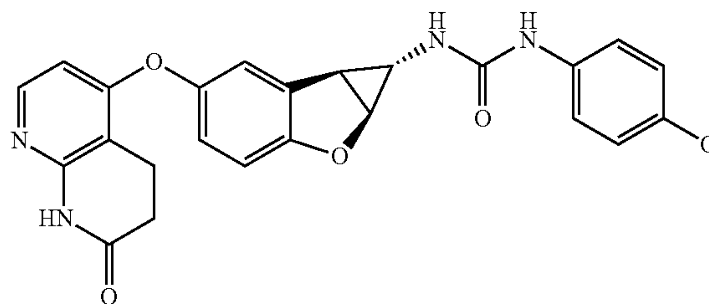
Compound 1.50
