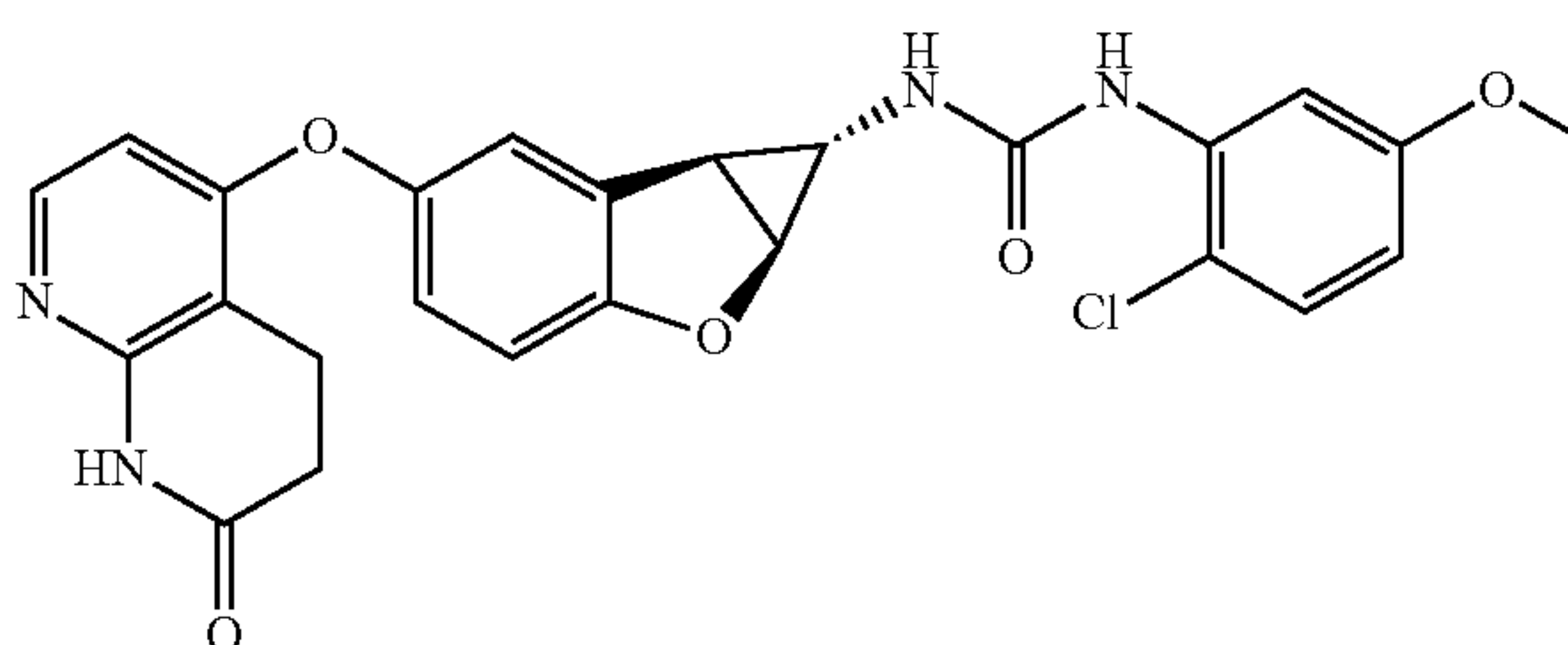
Compound 1.5
