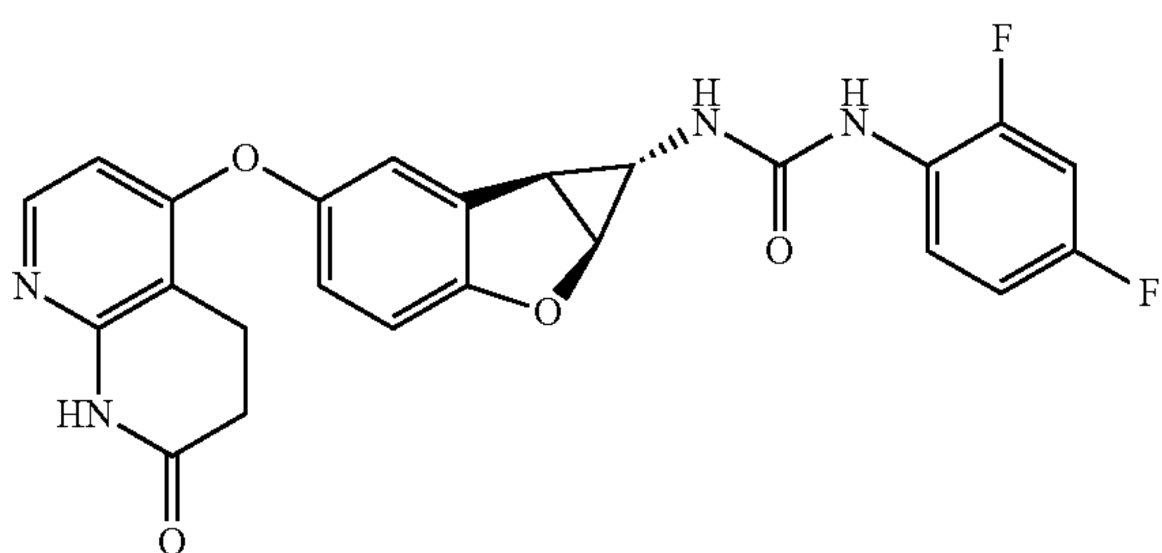
Compound 1.35
