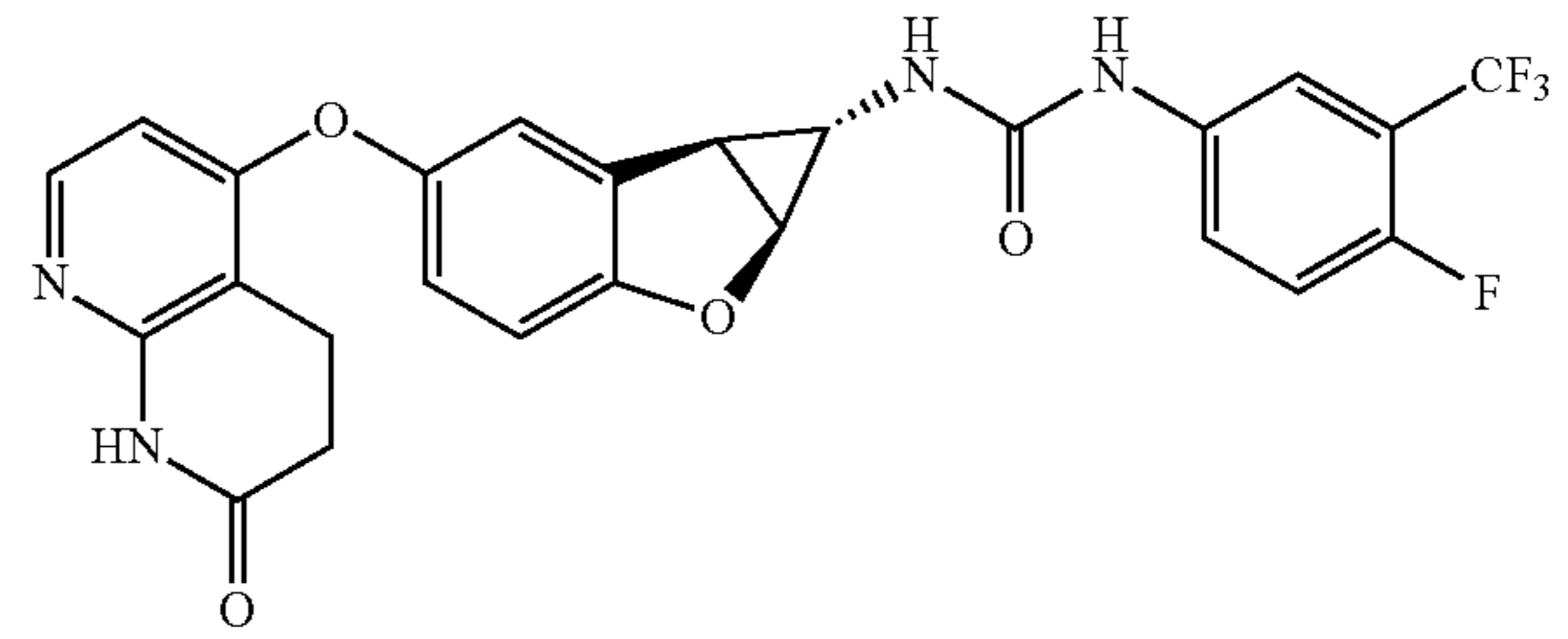
Compound 1.32
