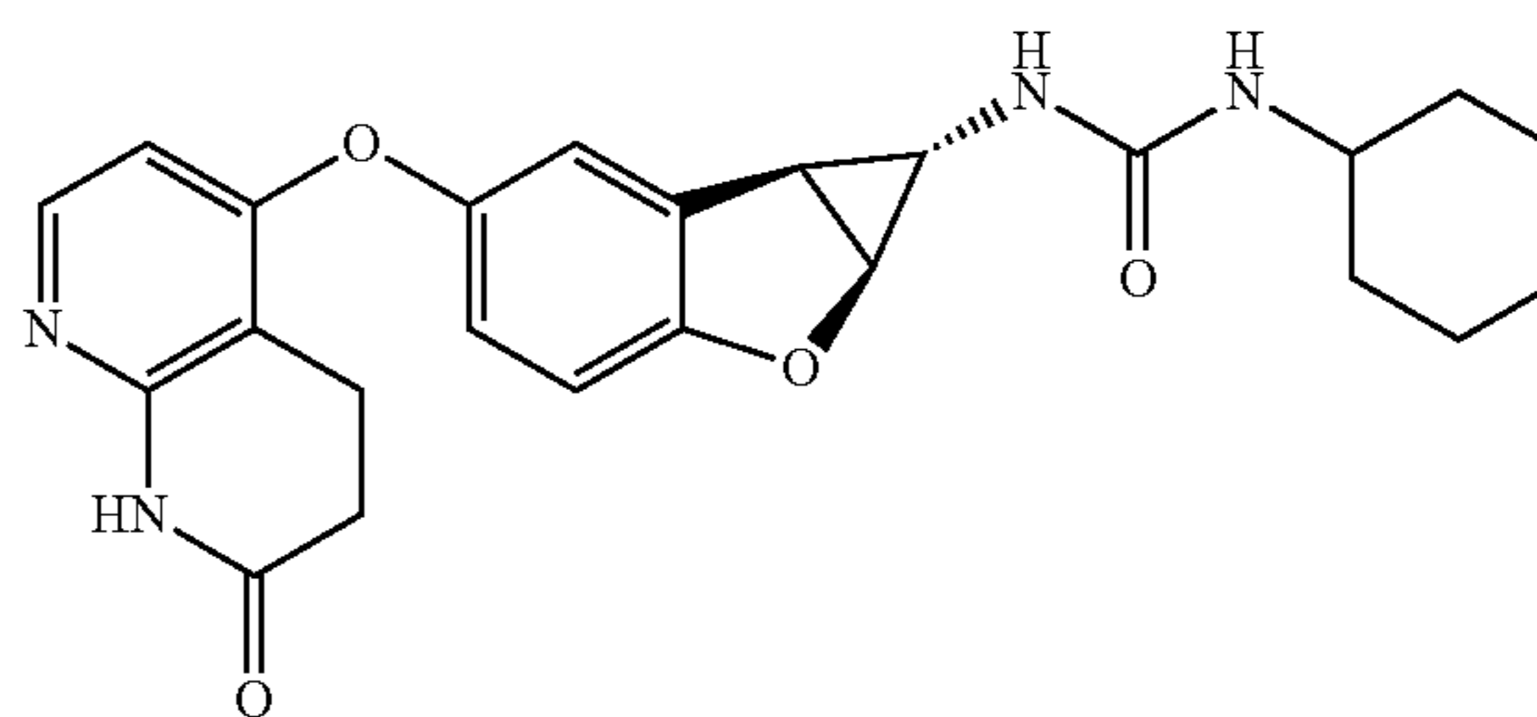
Compound 1.68
