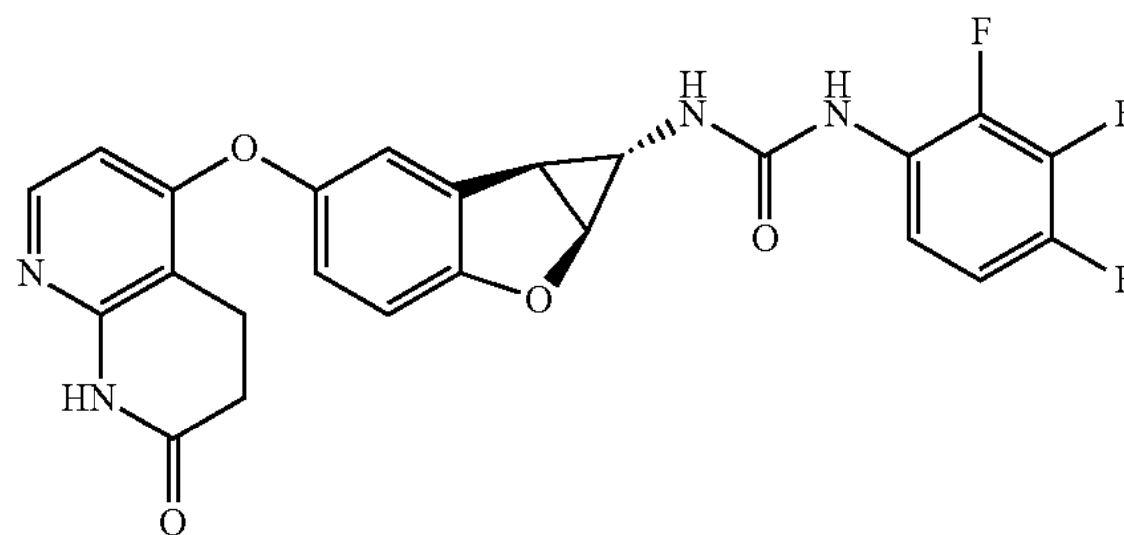
Compound 1.46
