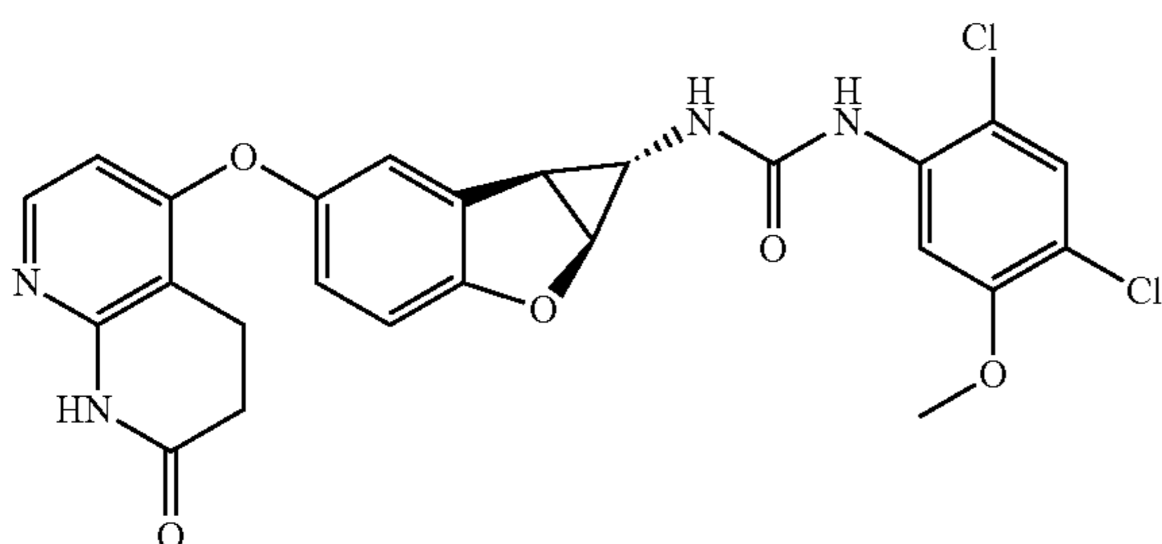
Compound 1.27
