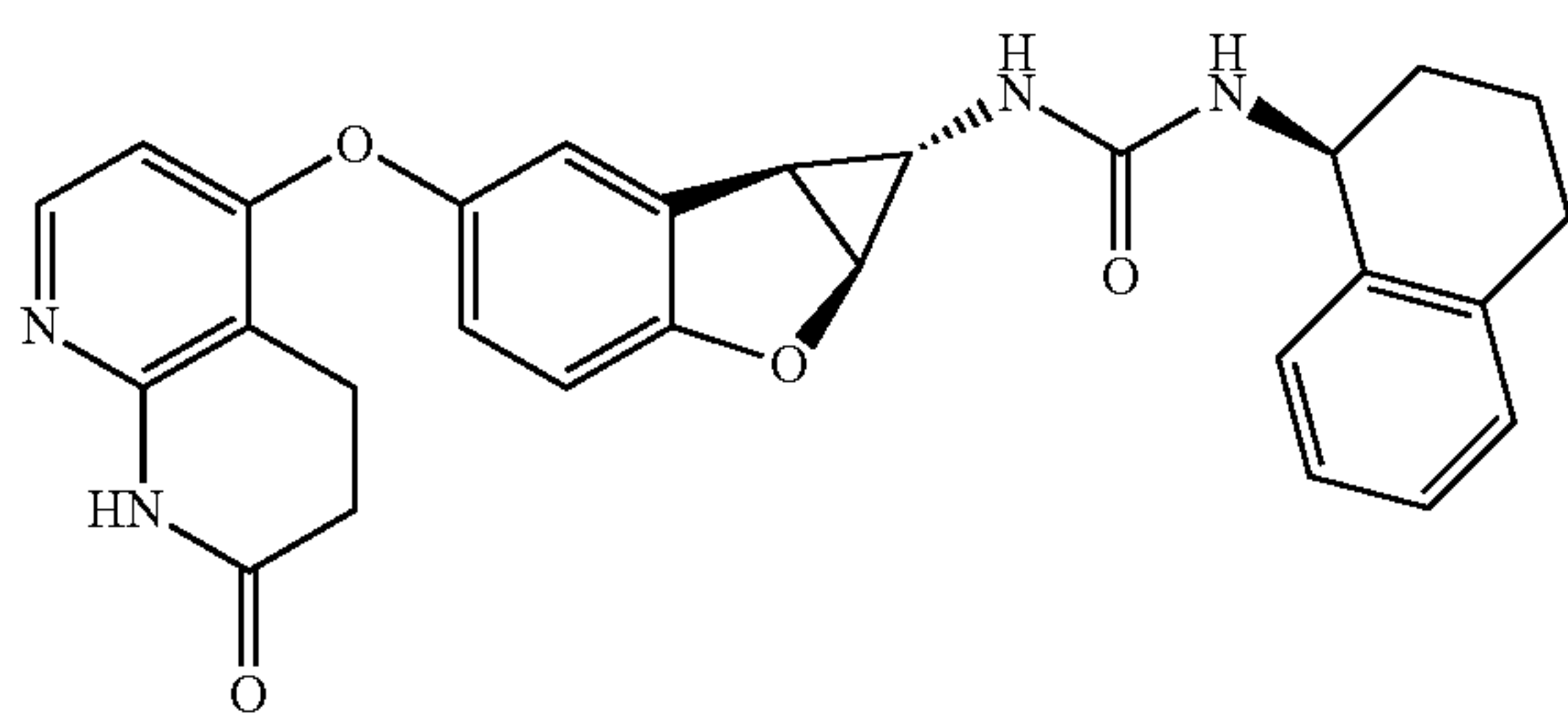
Compound 1.81
