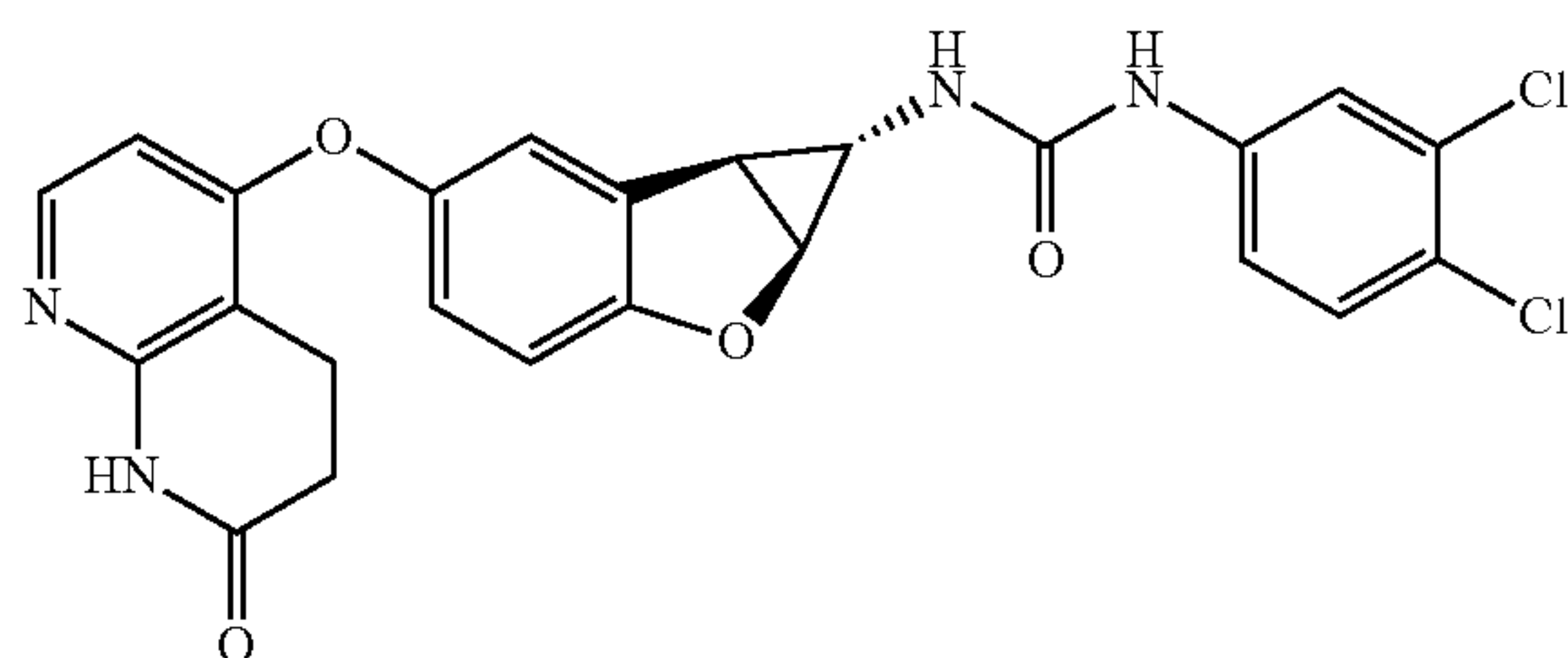
Compound 1.28
