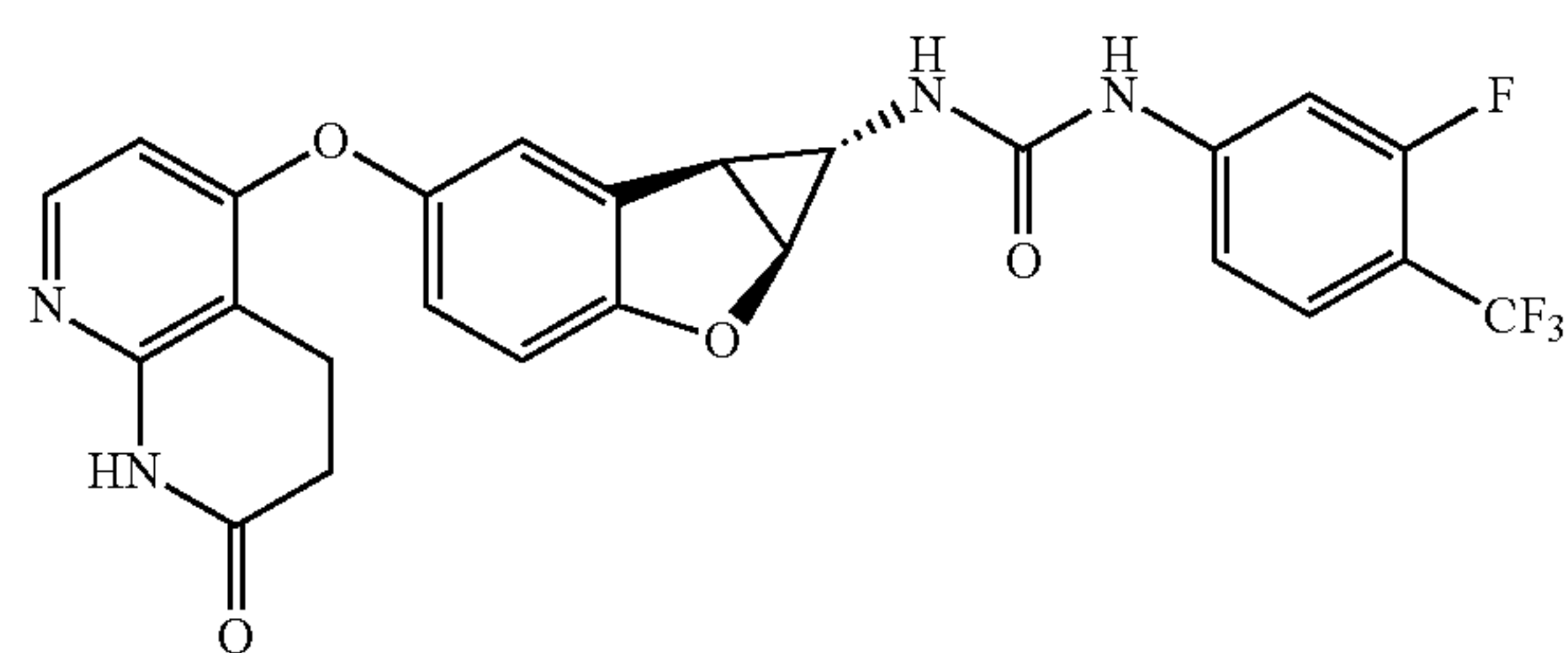
Compound 1.66
