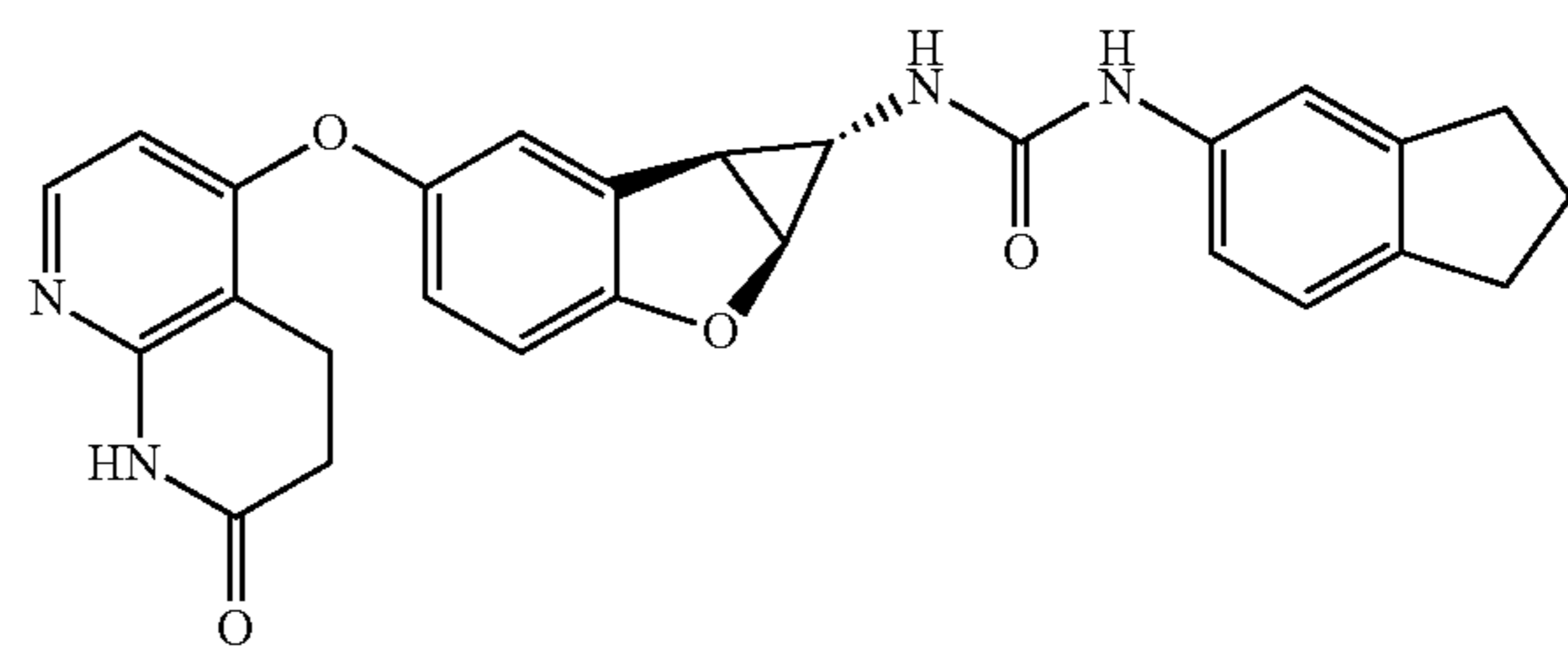
Compound 1.16
