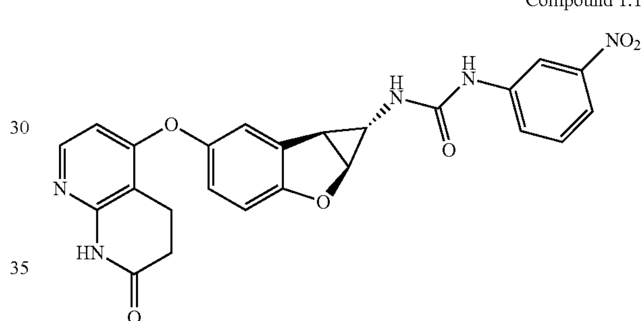
Compound 1.13
