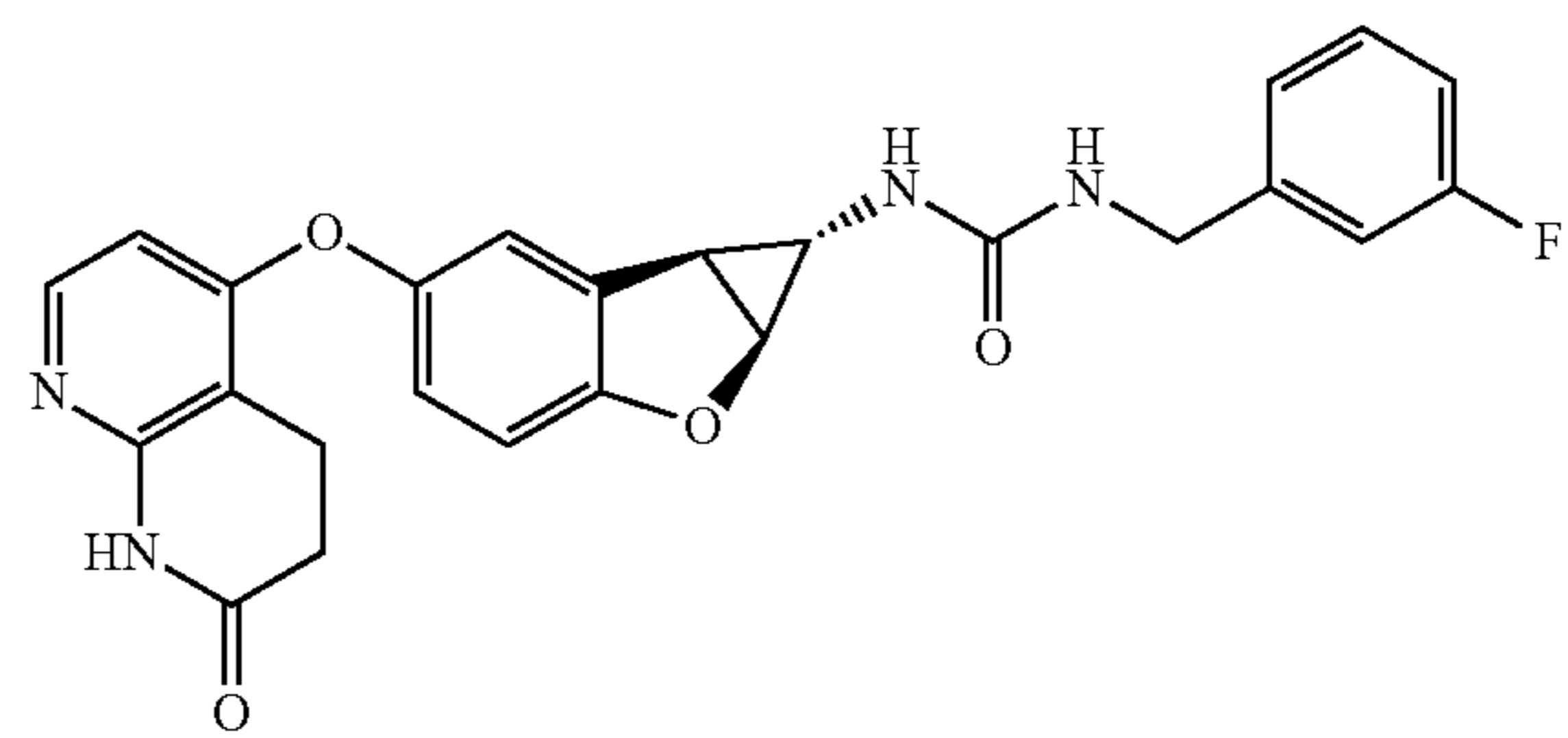
Compound 1.58
