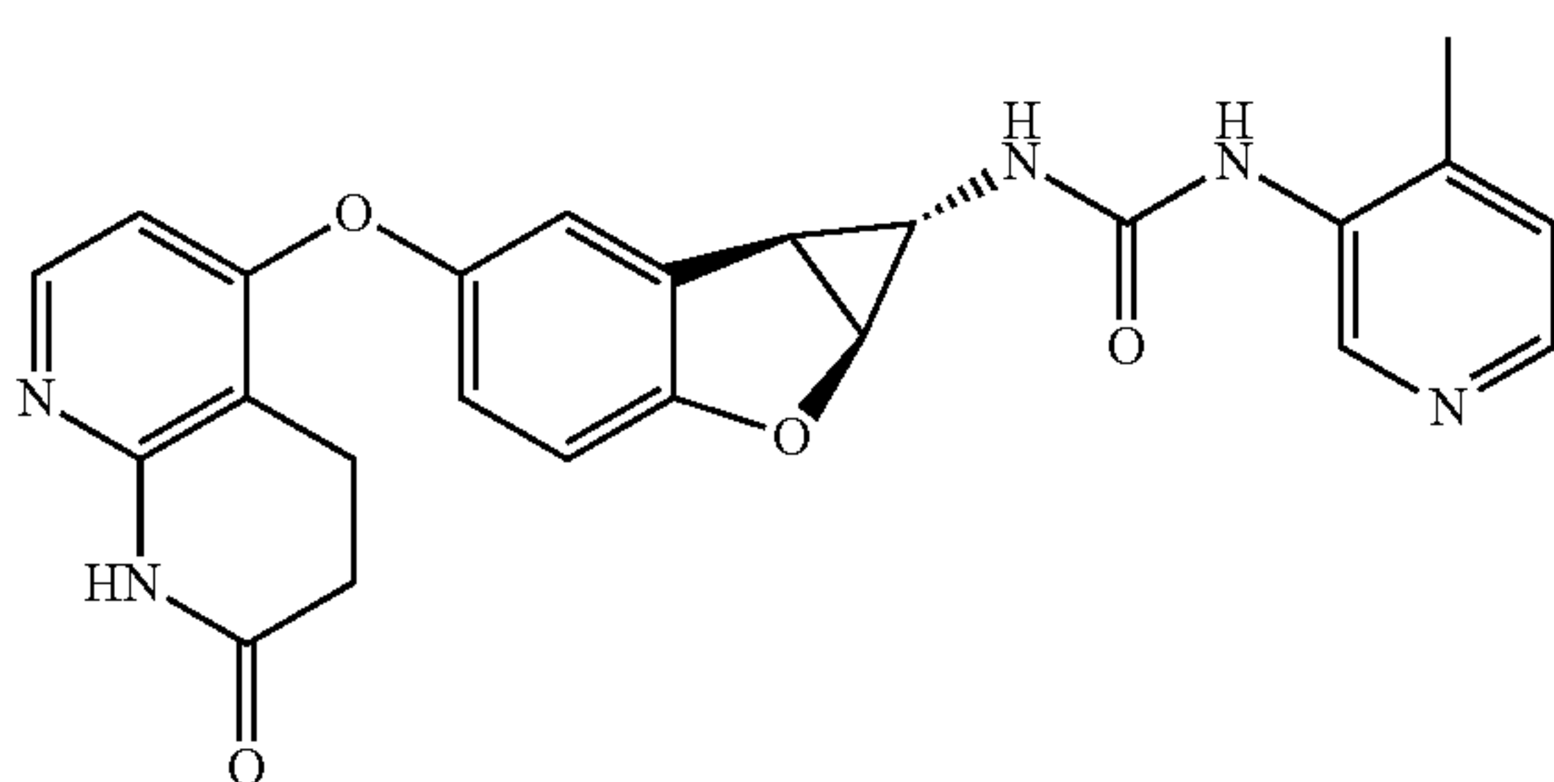
Compound 1.39
