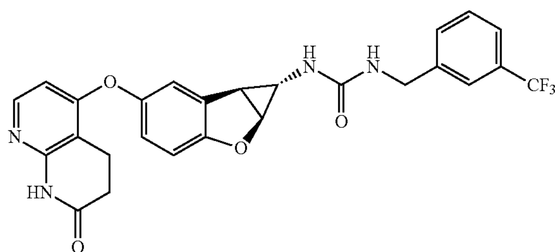
Compound 1.54
