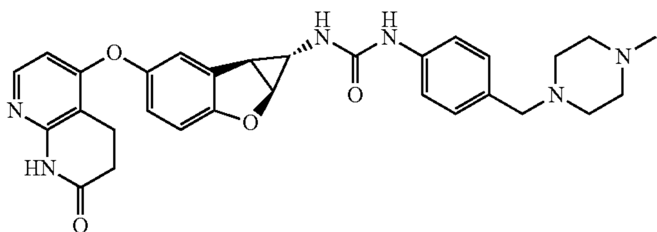
Compound 1.63
