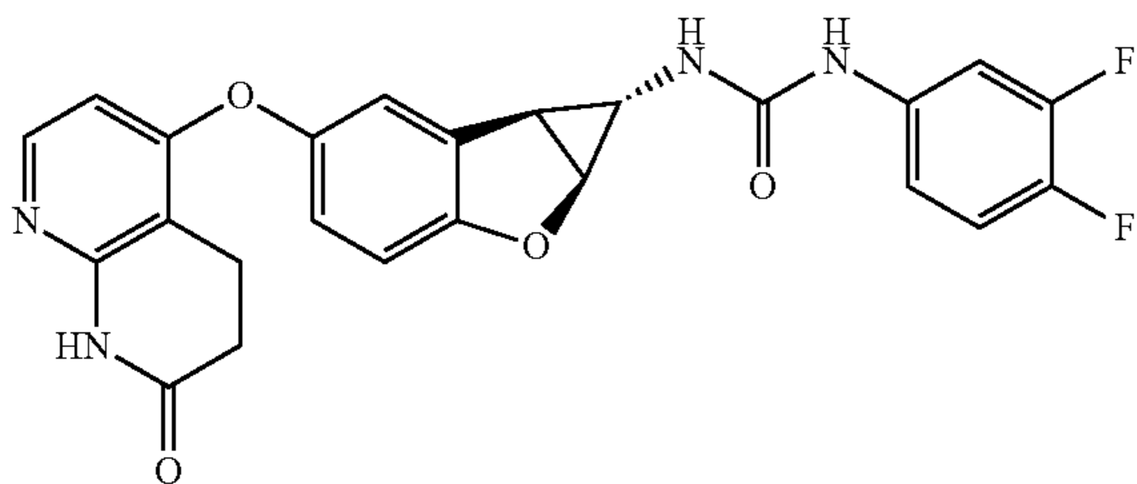
Compound 1.45
