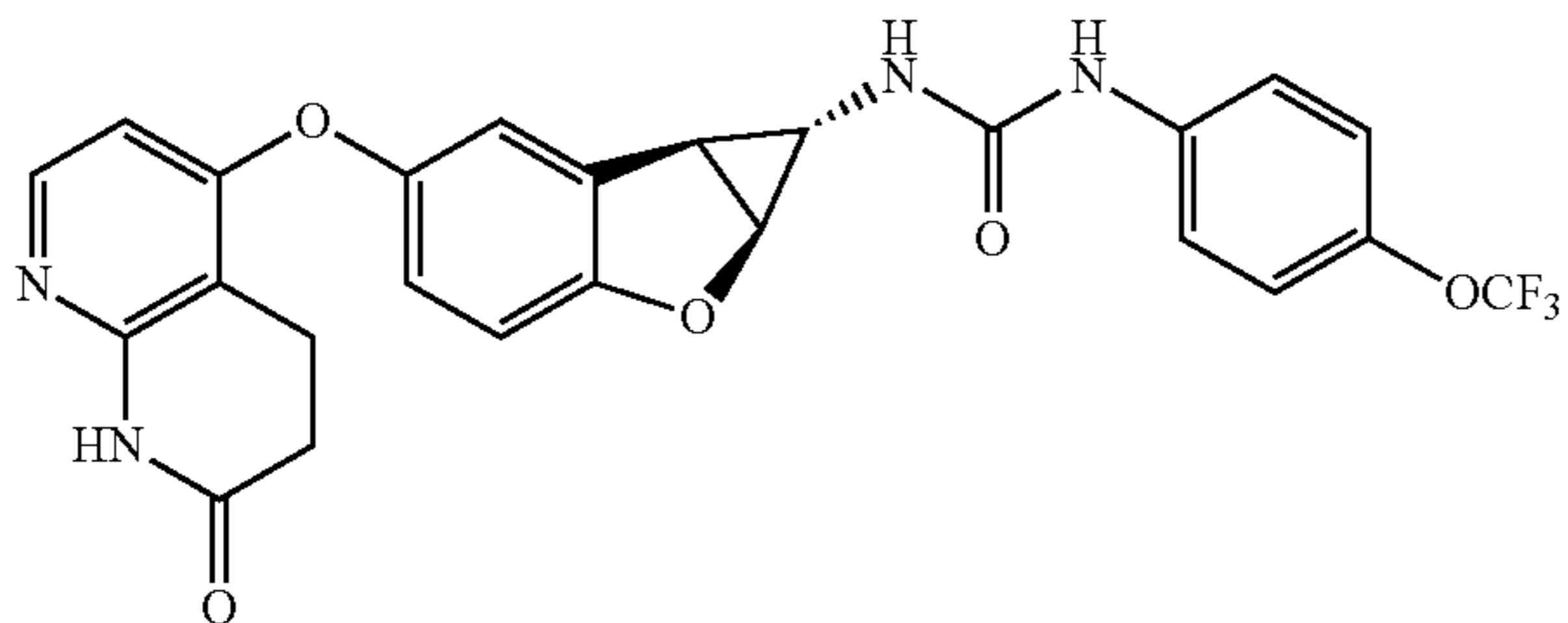
Compound 1.61
