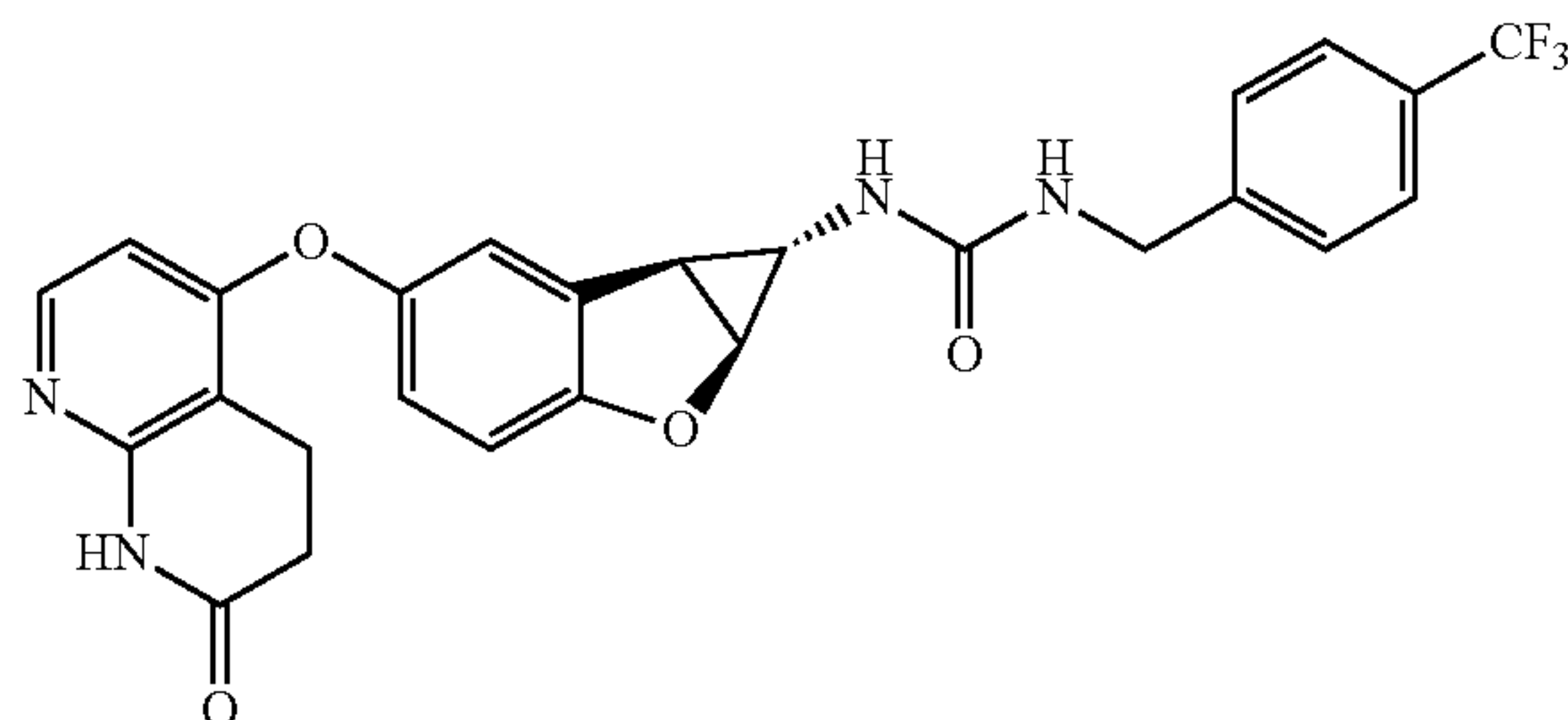
Compound 1.56
