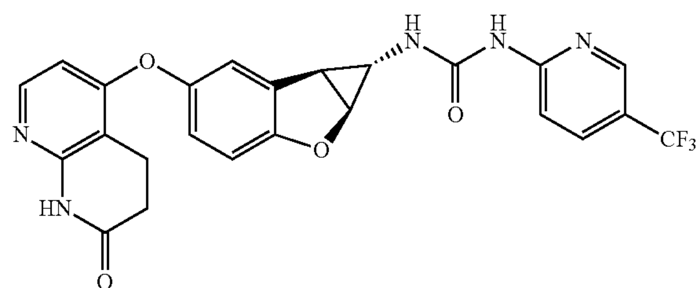
Compound 1.38
