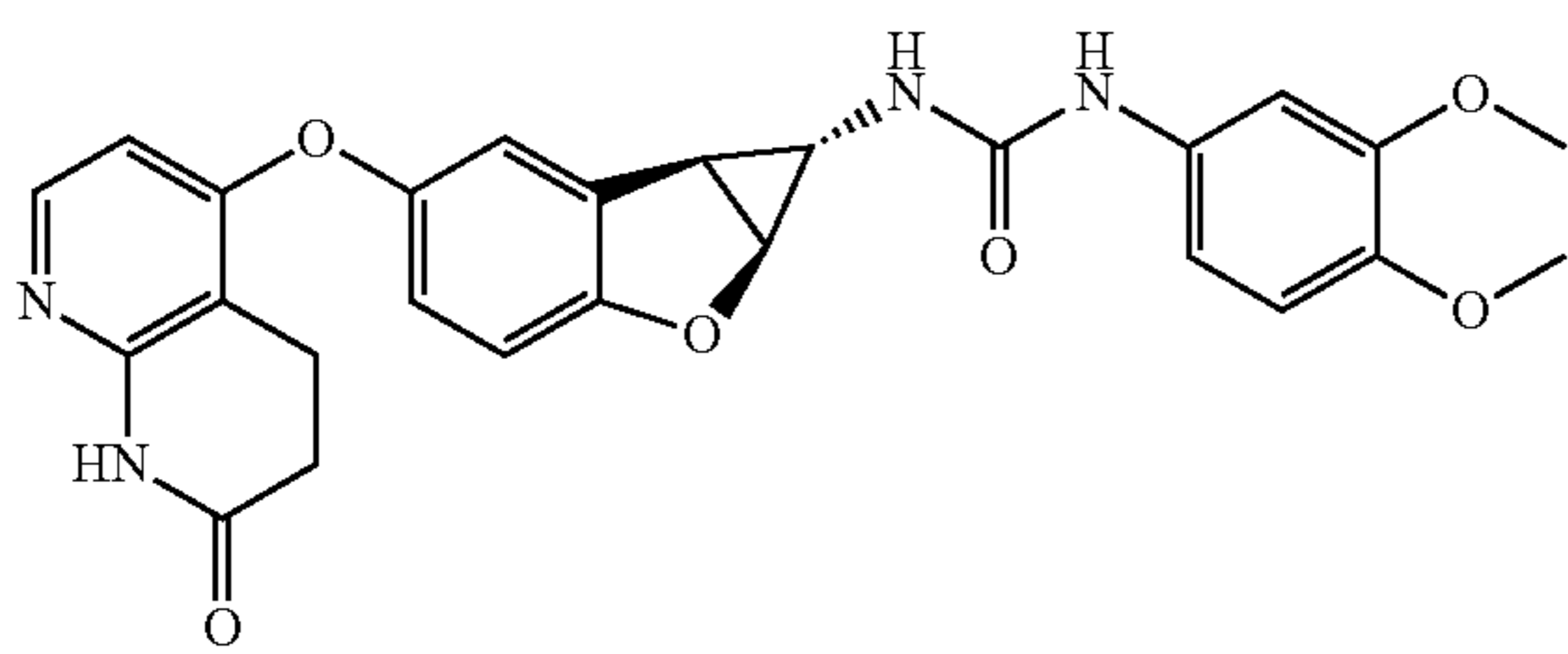
Compound 1.15
