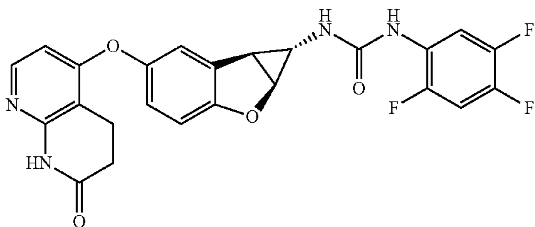
Compound 1.49
