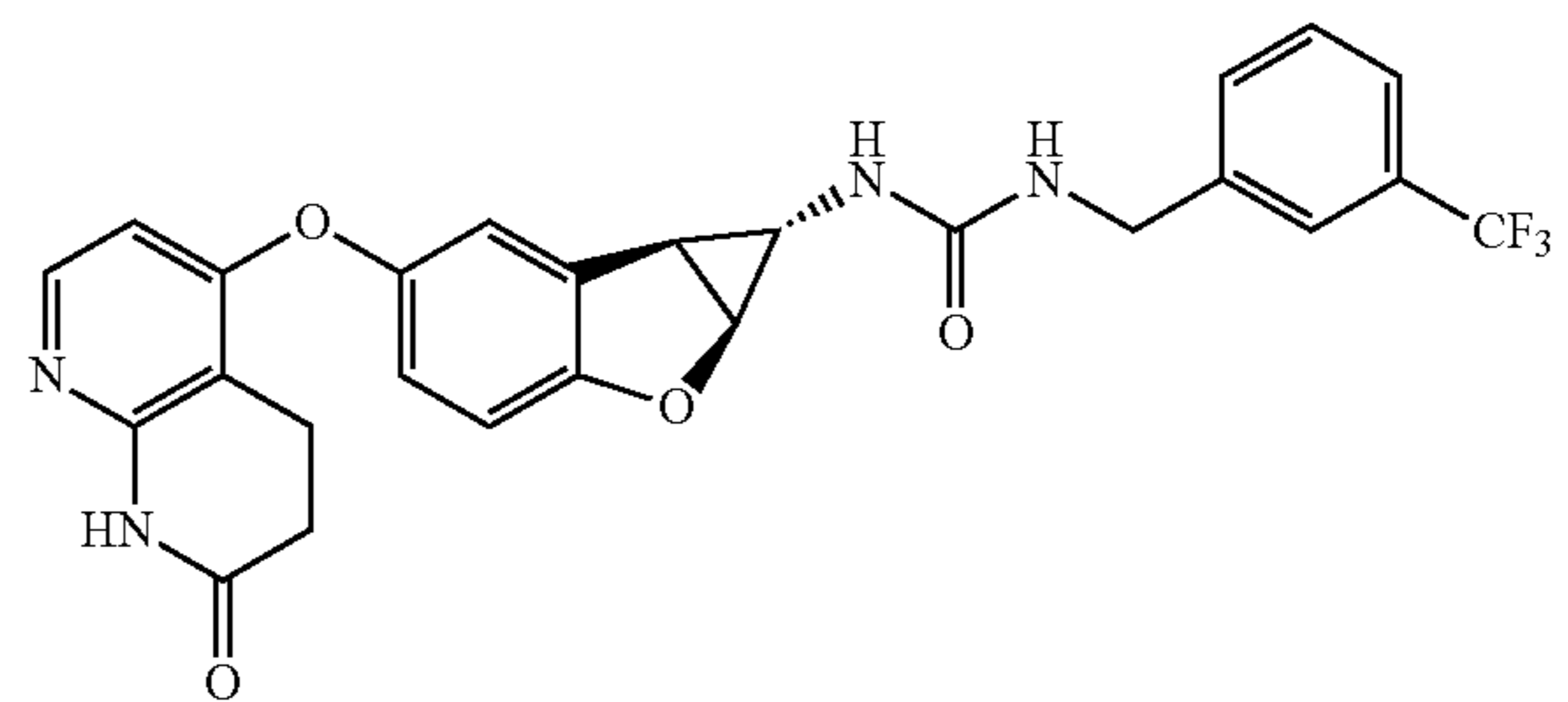
Compound 1.54
