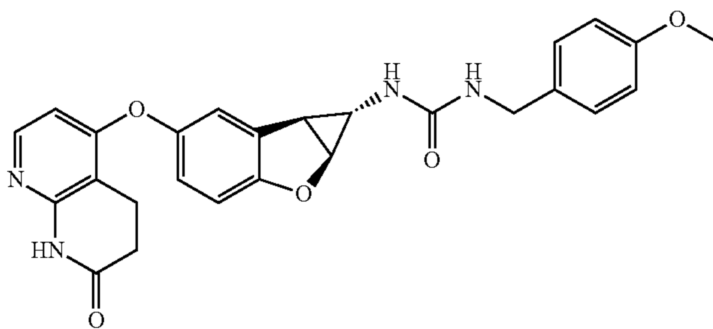
Compound 1.3
