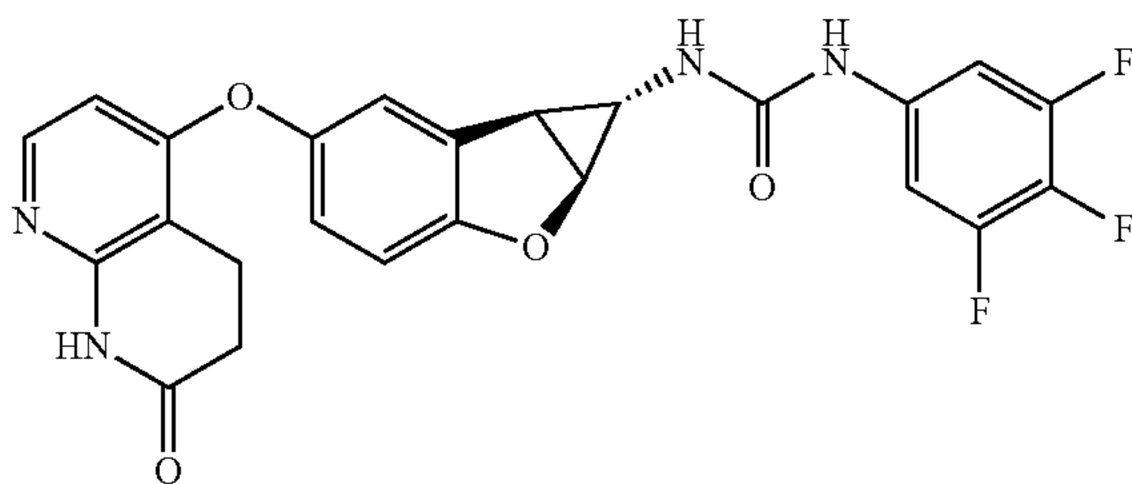
Compound 1.47
