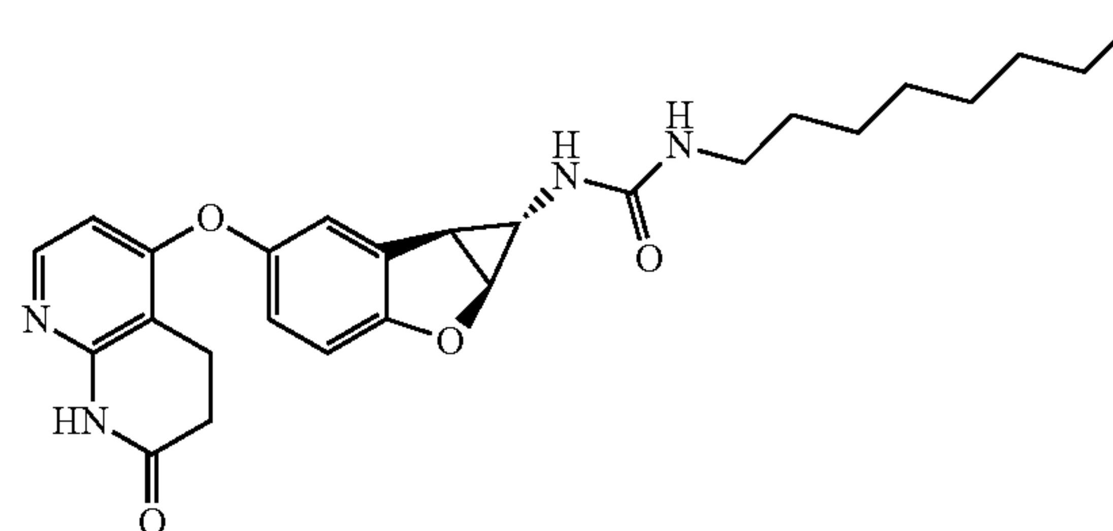
Compound 1.84
