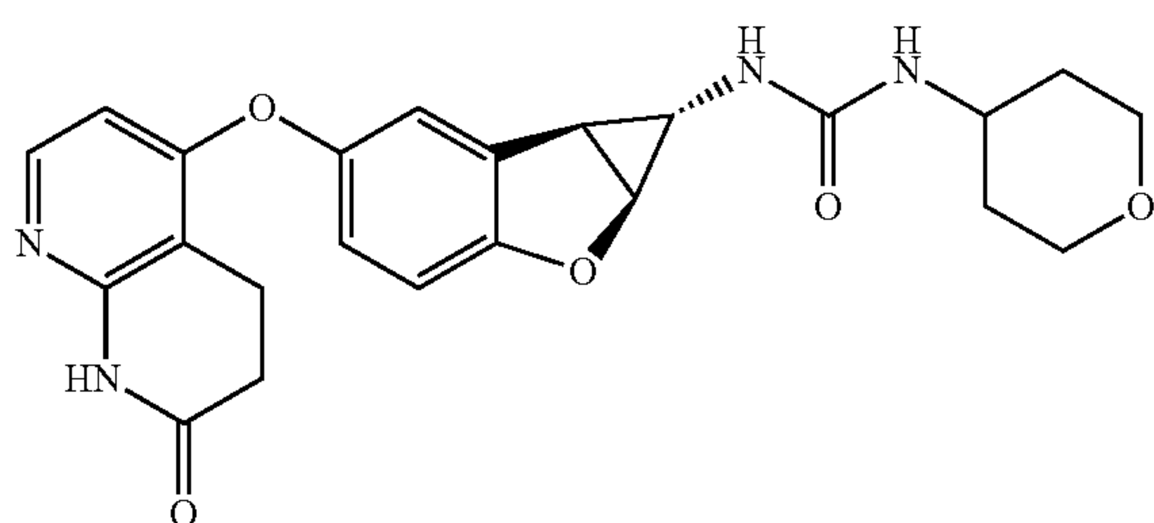
Compound 1.69
