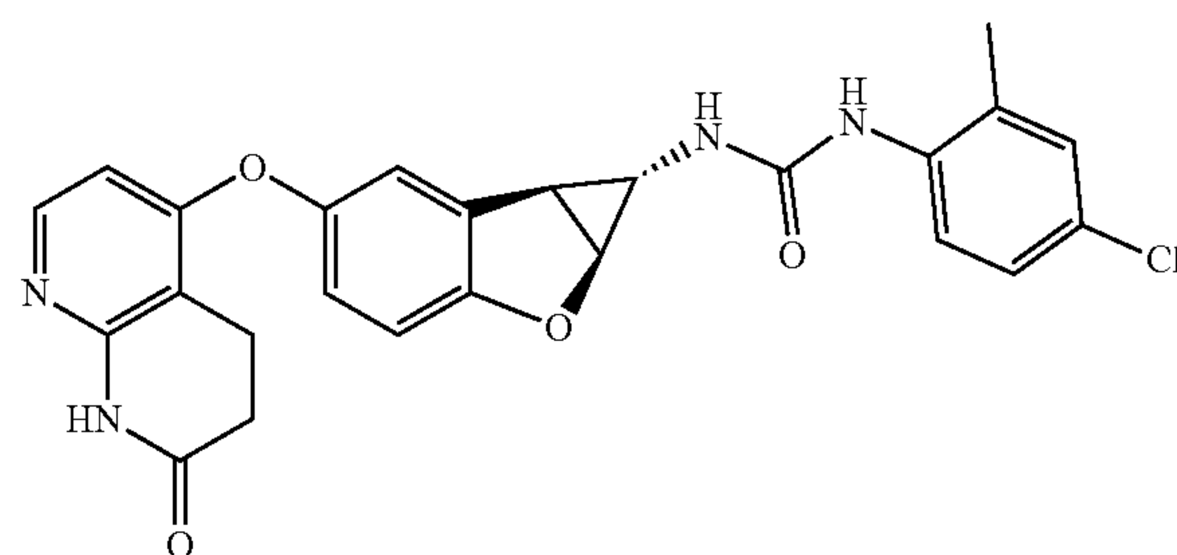
Compound 1.7
