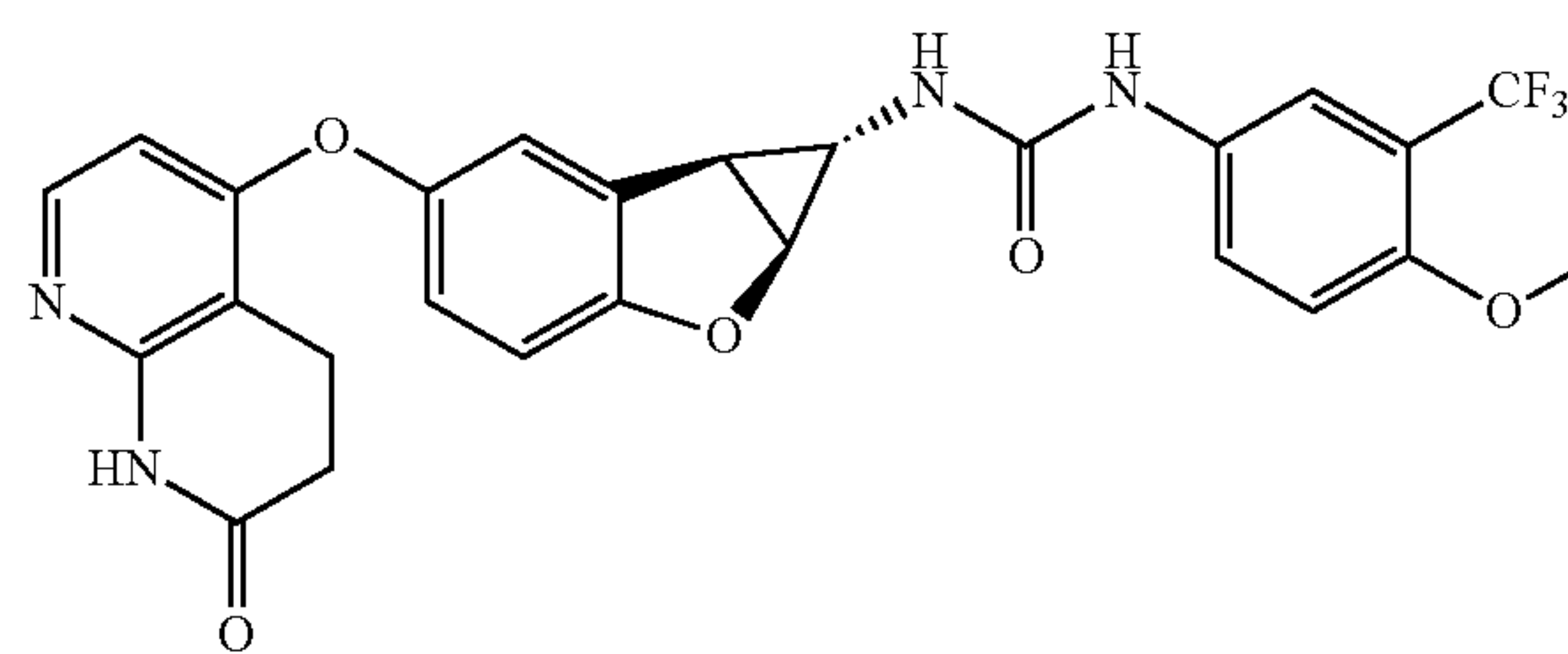
Compound 1.34
