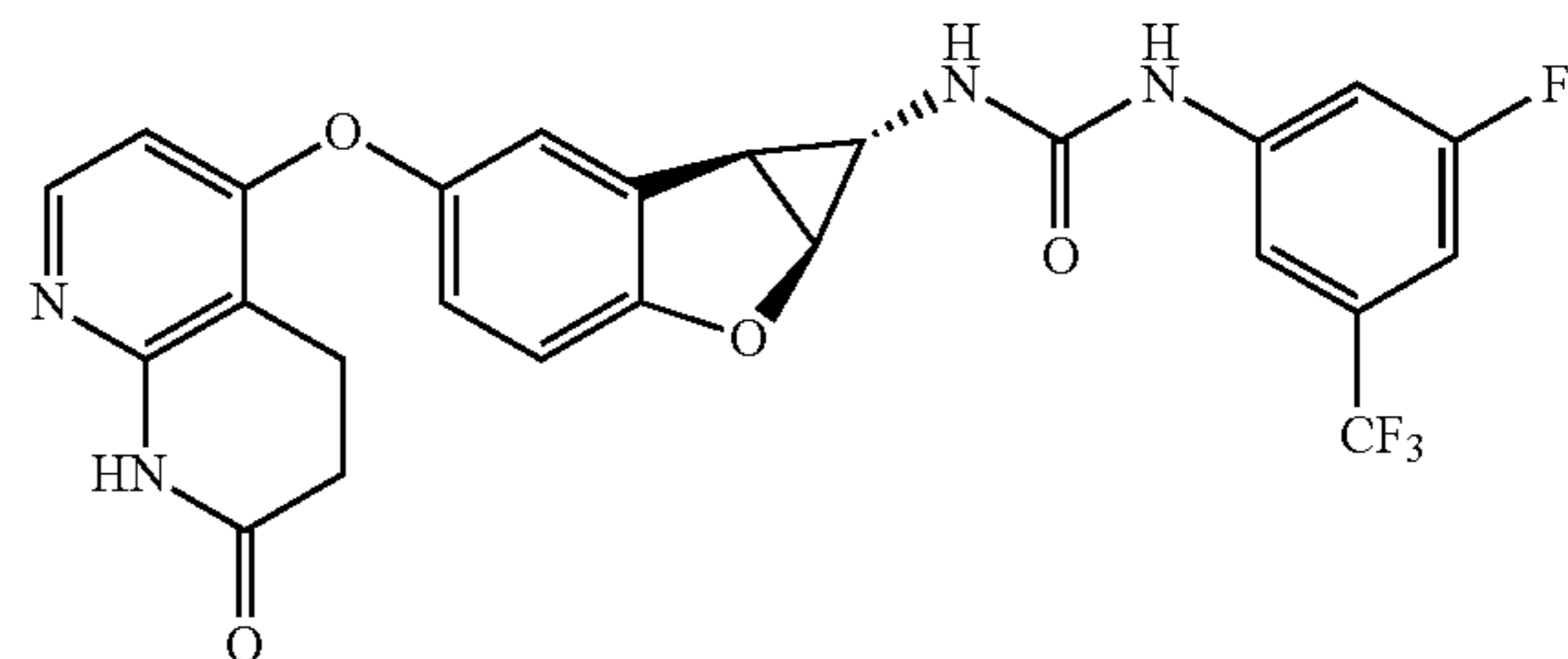
Compound 1.78
