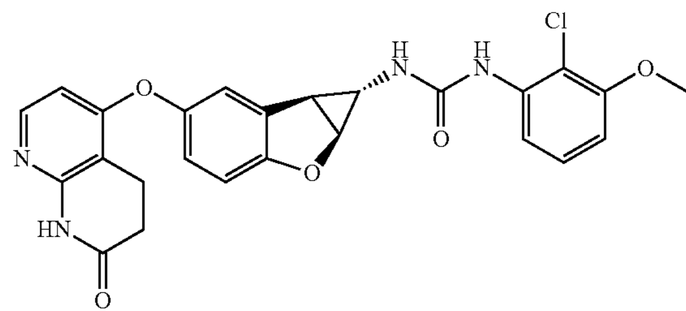
Compound 1.6
