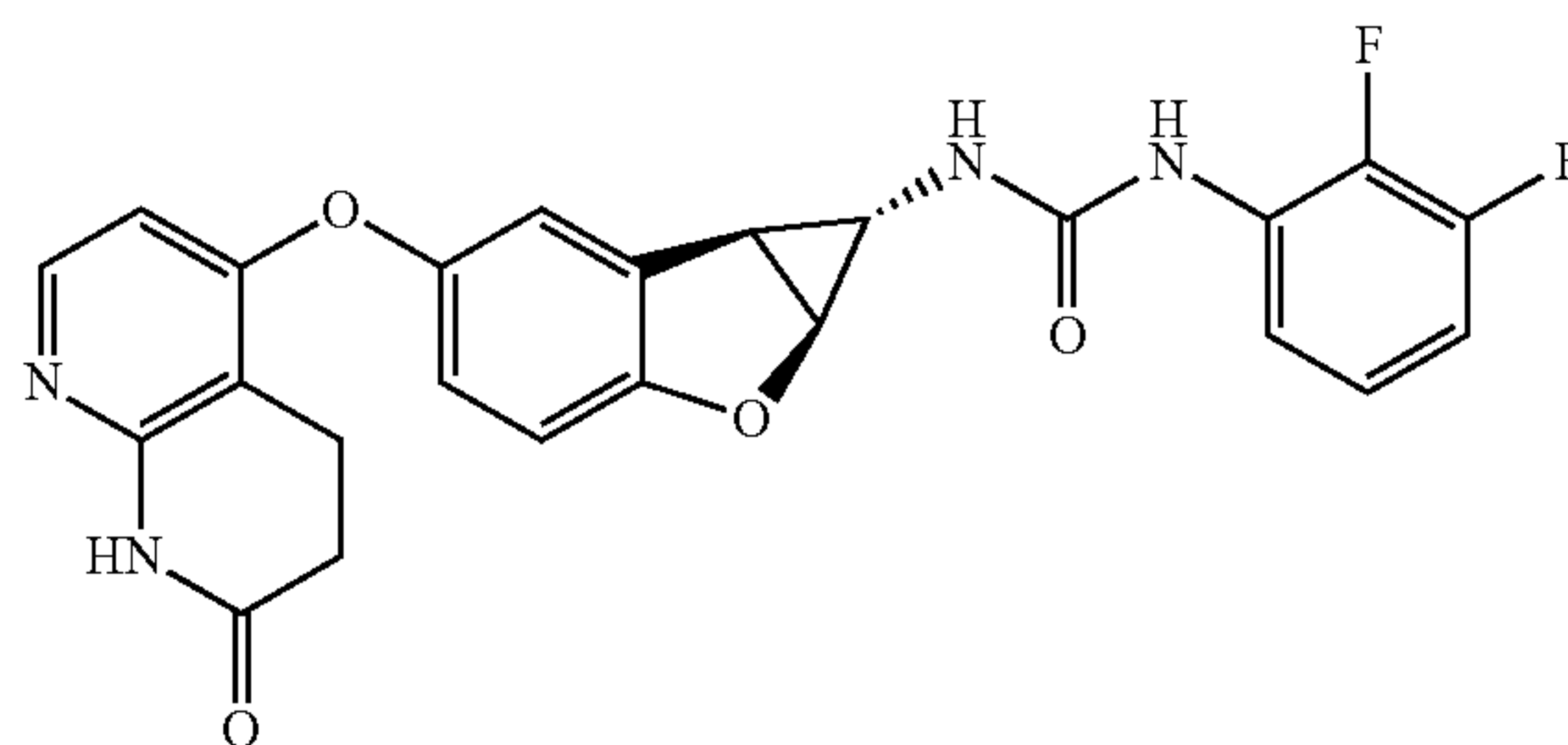
Compound 1.42
