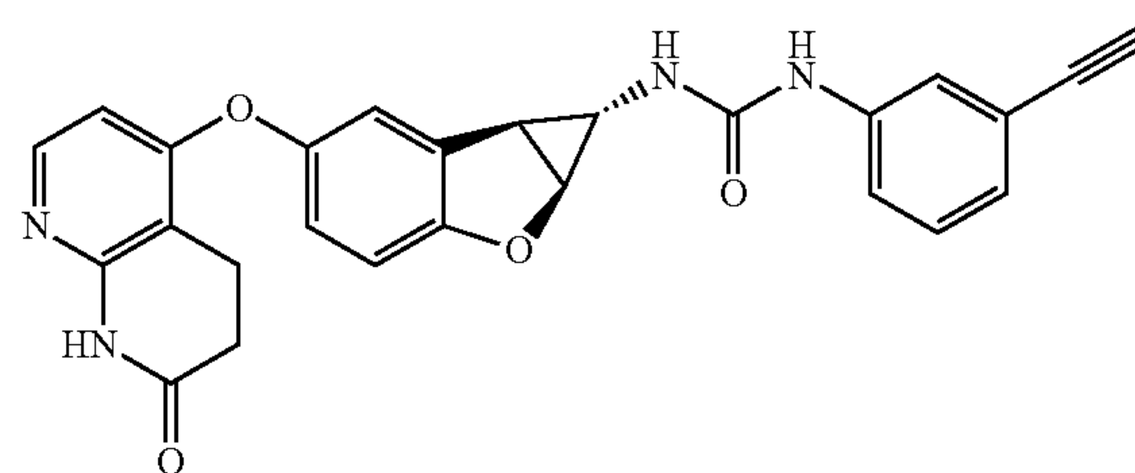
Compound 1.14
