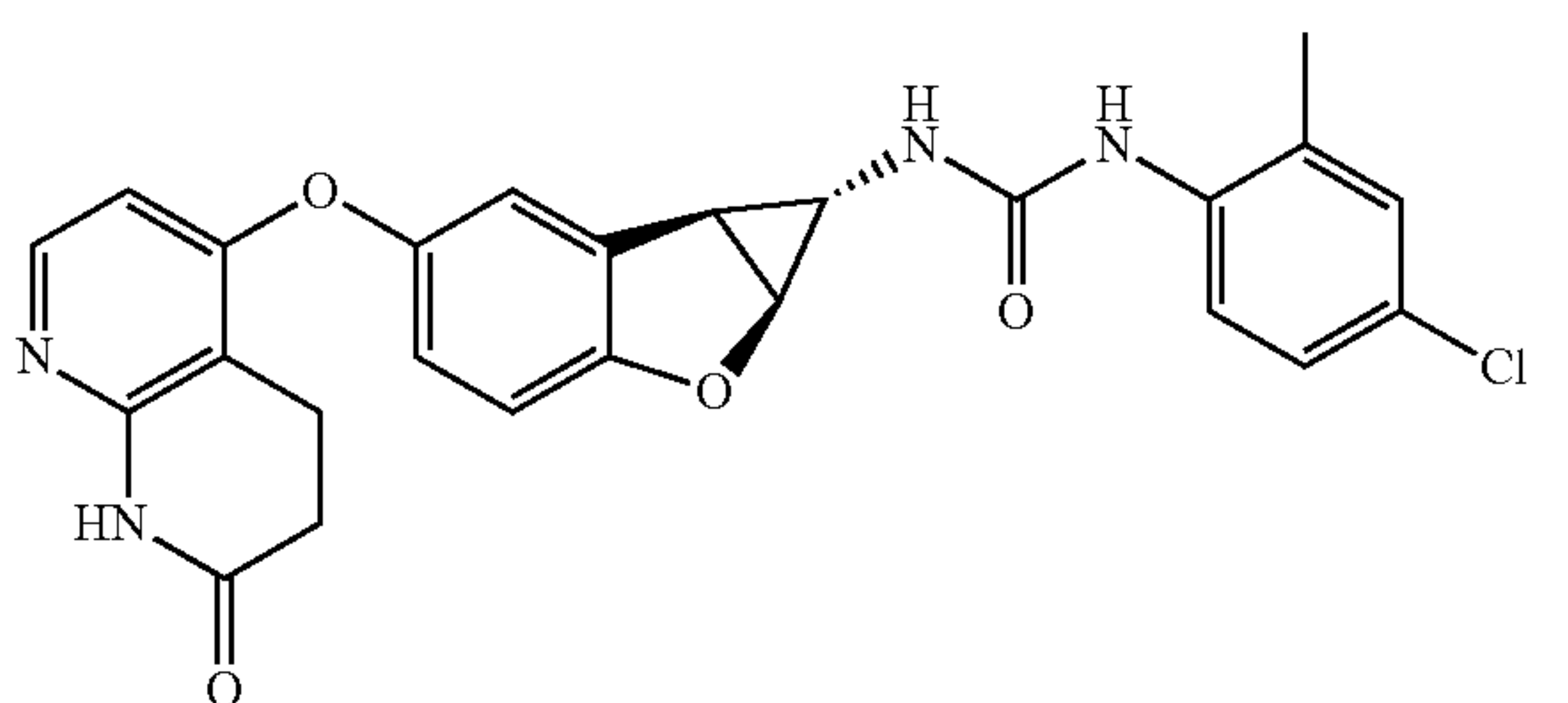
Compound 1.7
