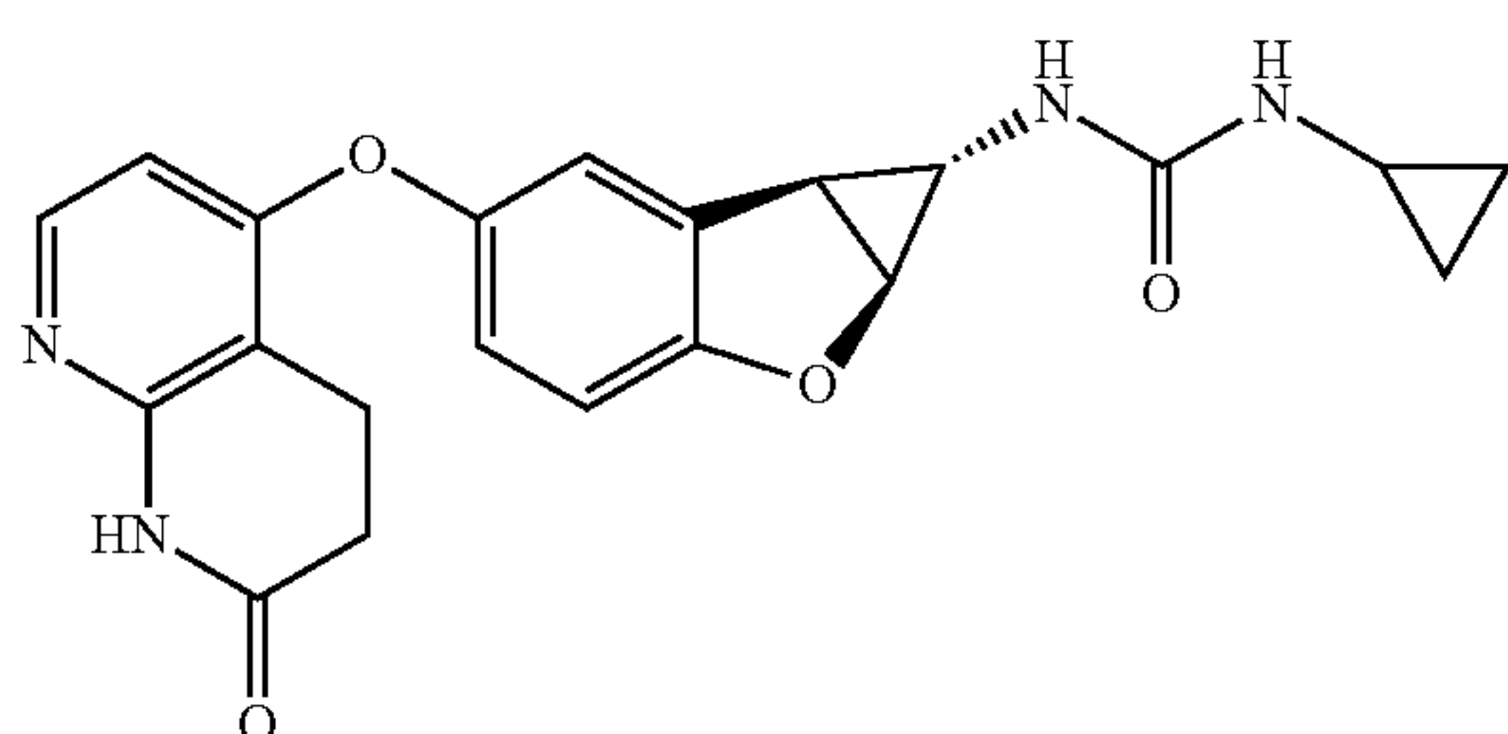
Compound 1.71
