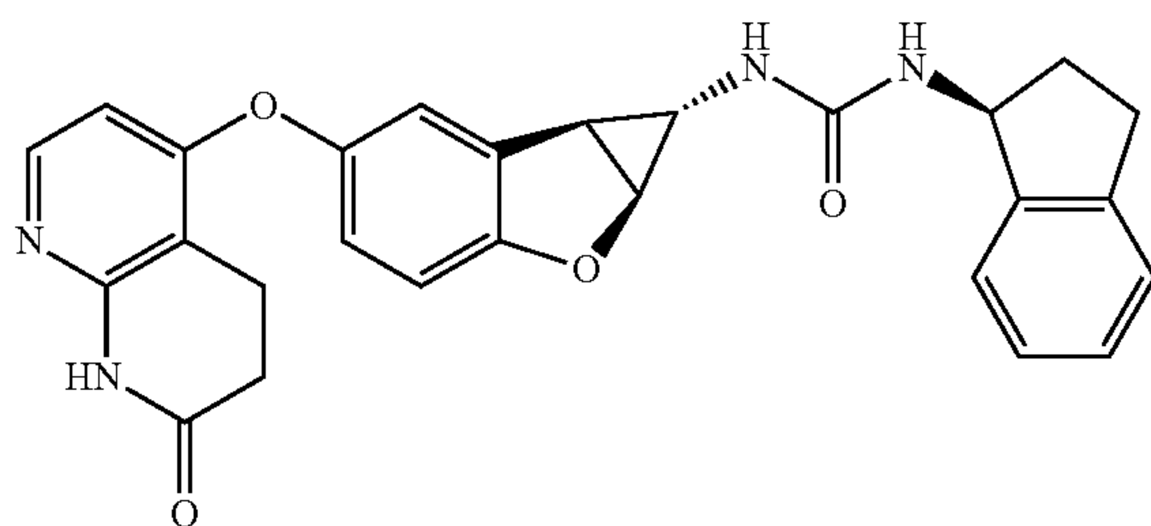
Compound 1.83
