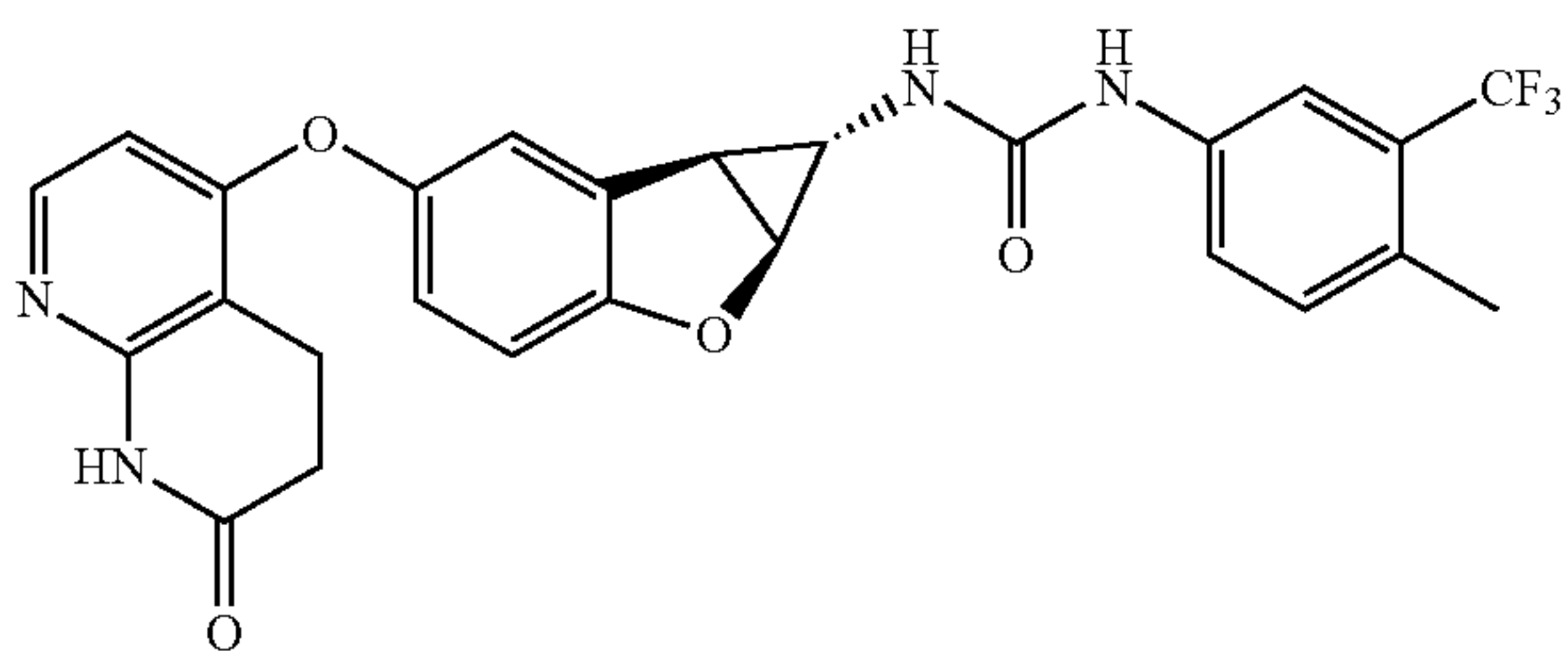
Compound 1.31
