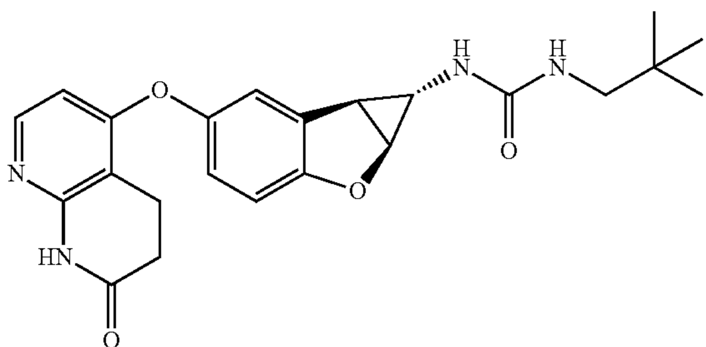
Compound 1.83
