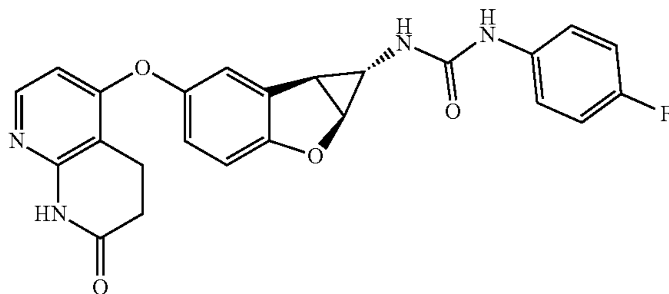
Compound 1.41
