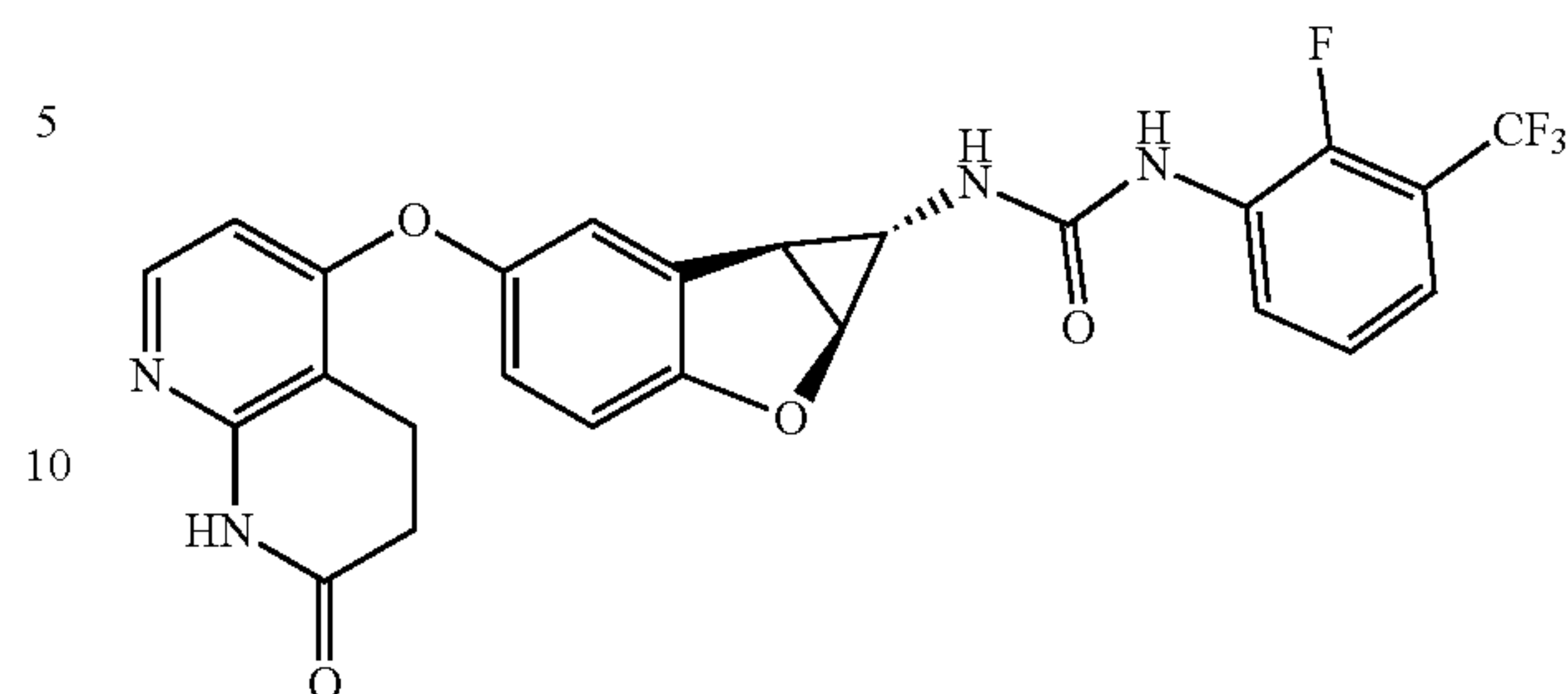
Compound 1.12
