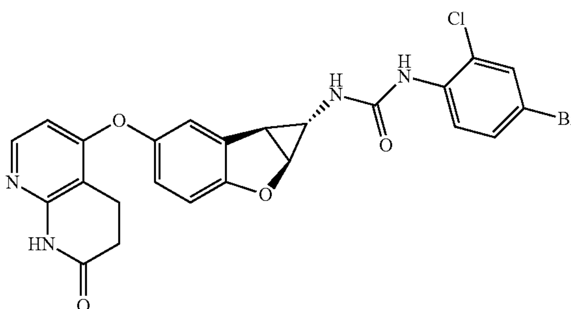
Compound 1.10
