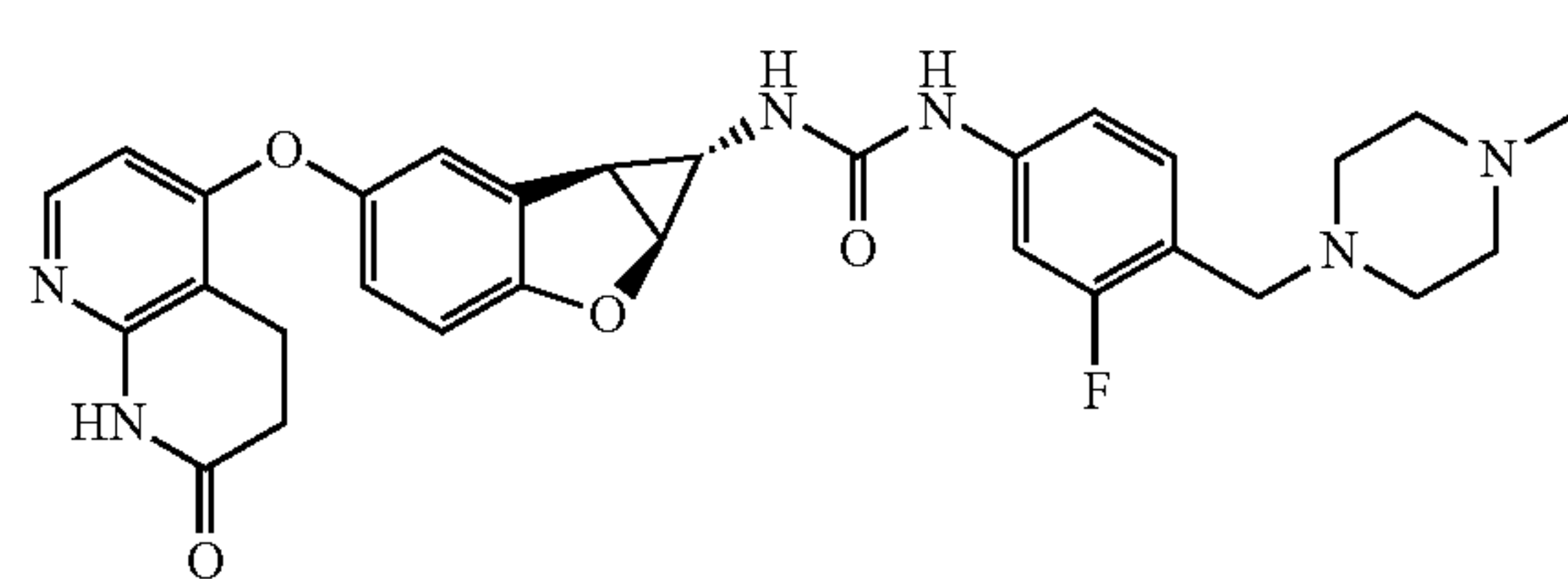
Compound 1.76
