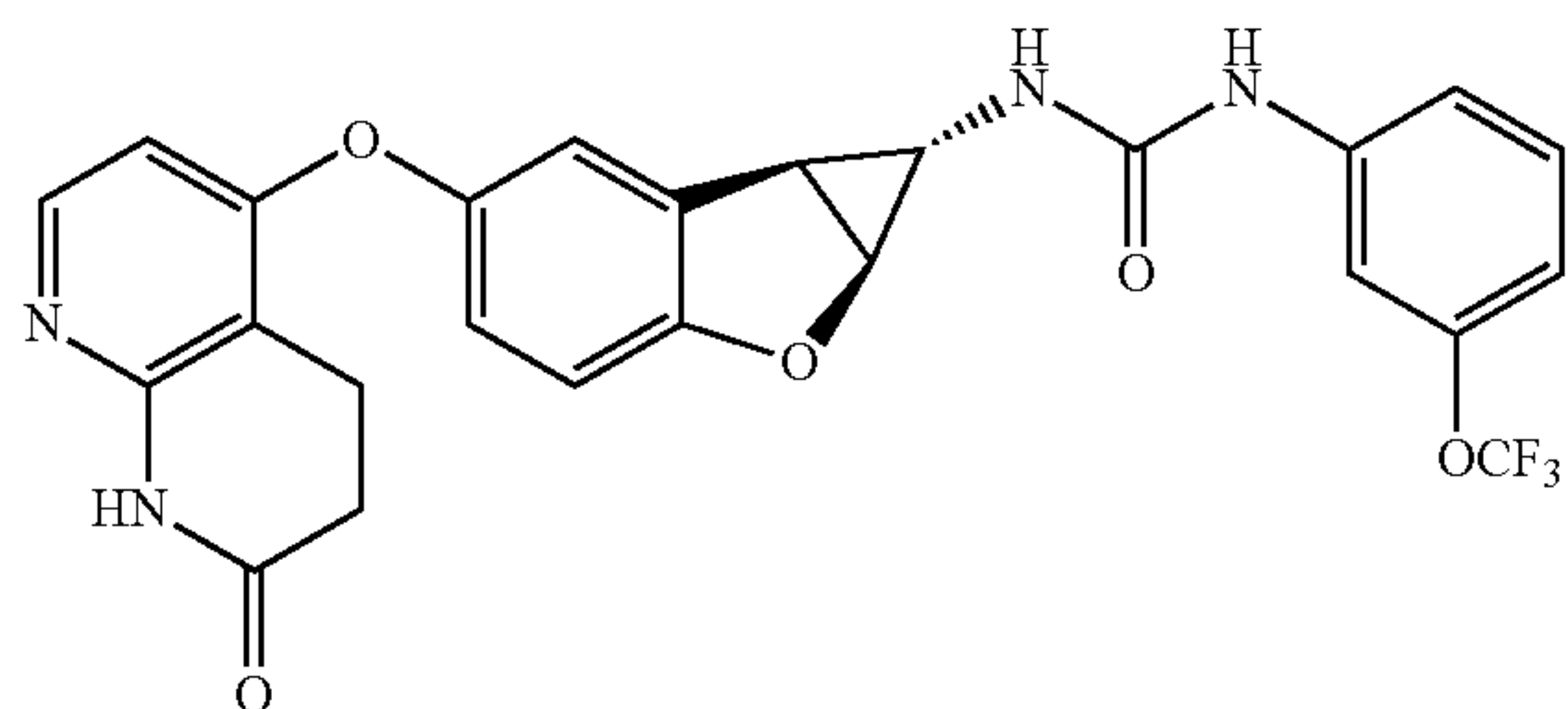
Compound 1.60
