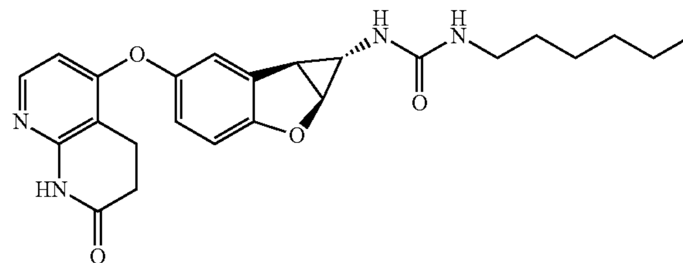
Compound 1.78
