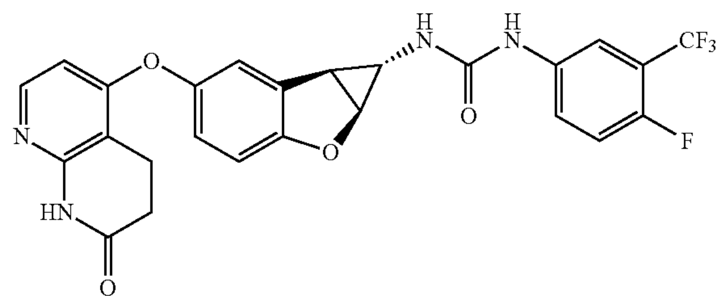
Compound 1.32
