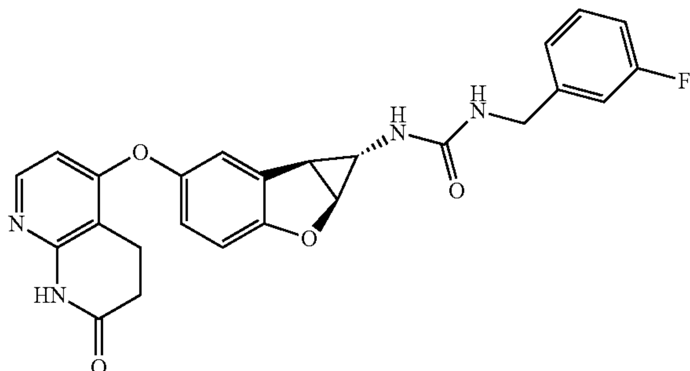
Compound 1.58
