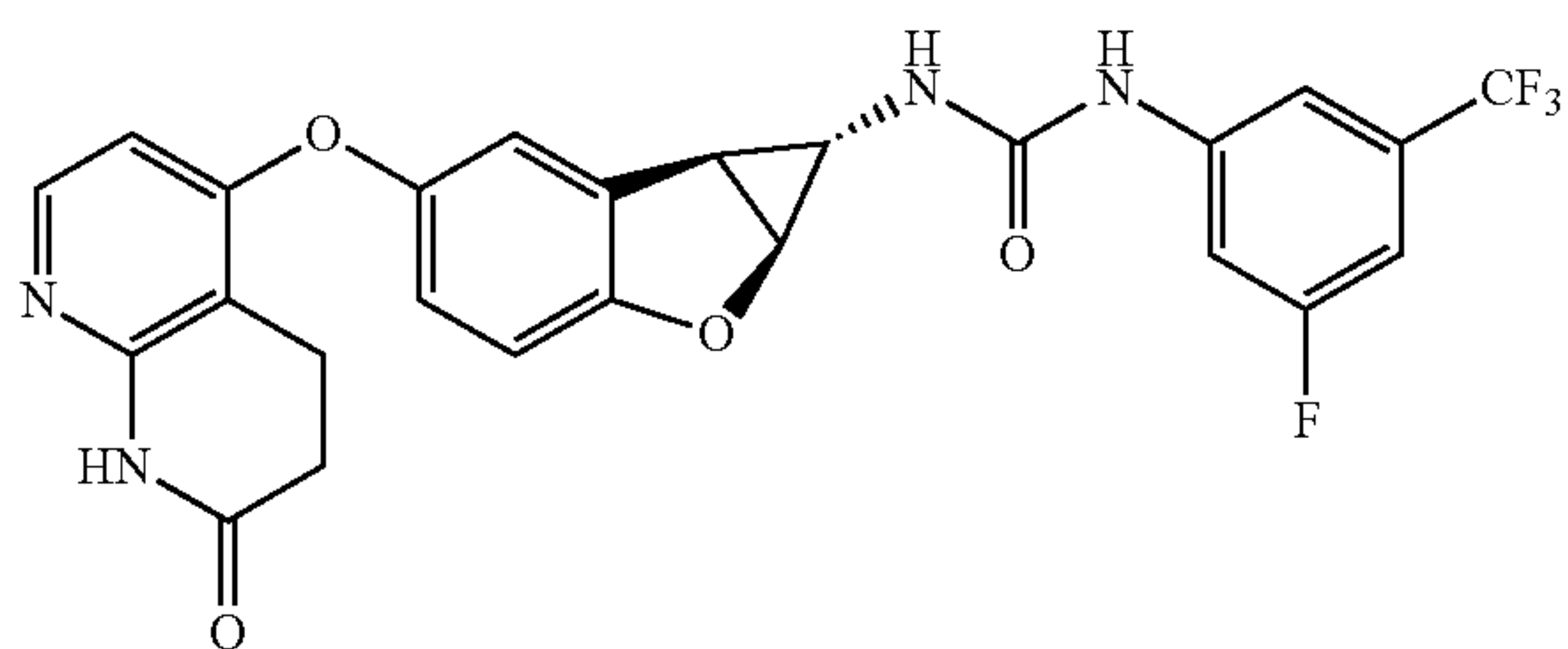
Compound 1.11
