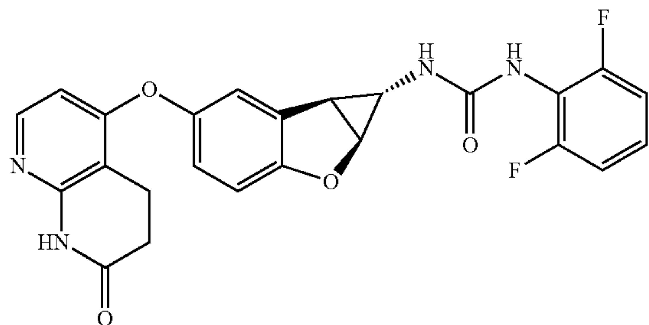
Compound 1.44
