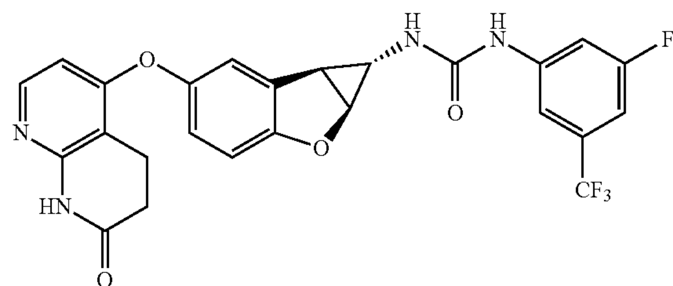
Compound 1.78
