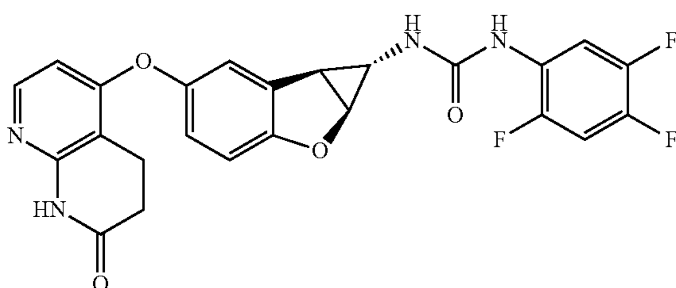
Compound 2.3
