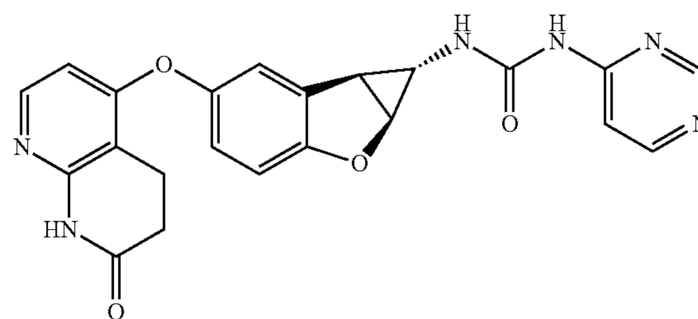
Compound 1.36
