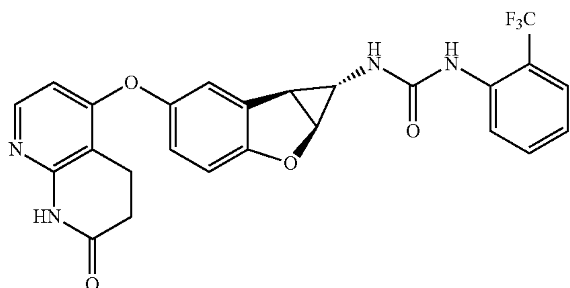
Compound 1.30
