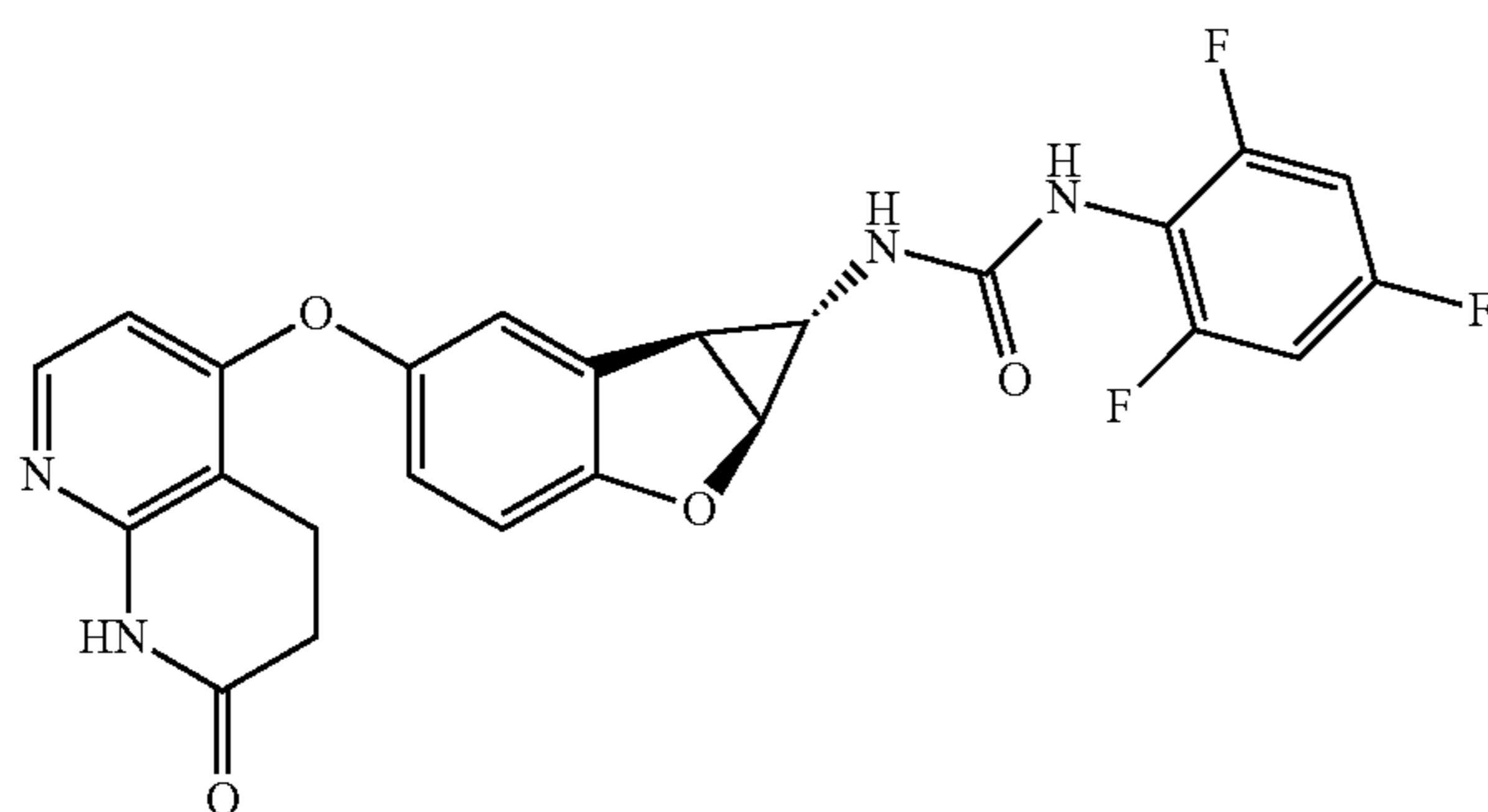
Compound 1.40
