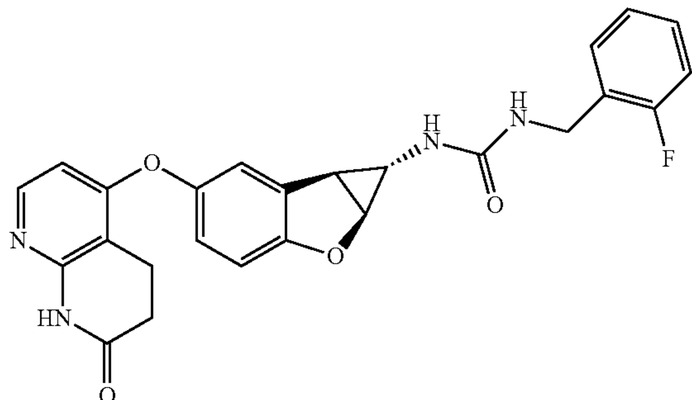
Compound 1.57
