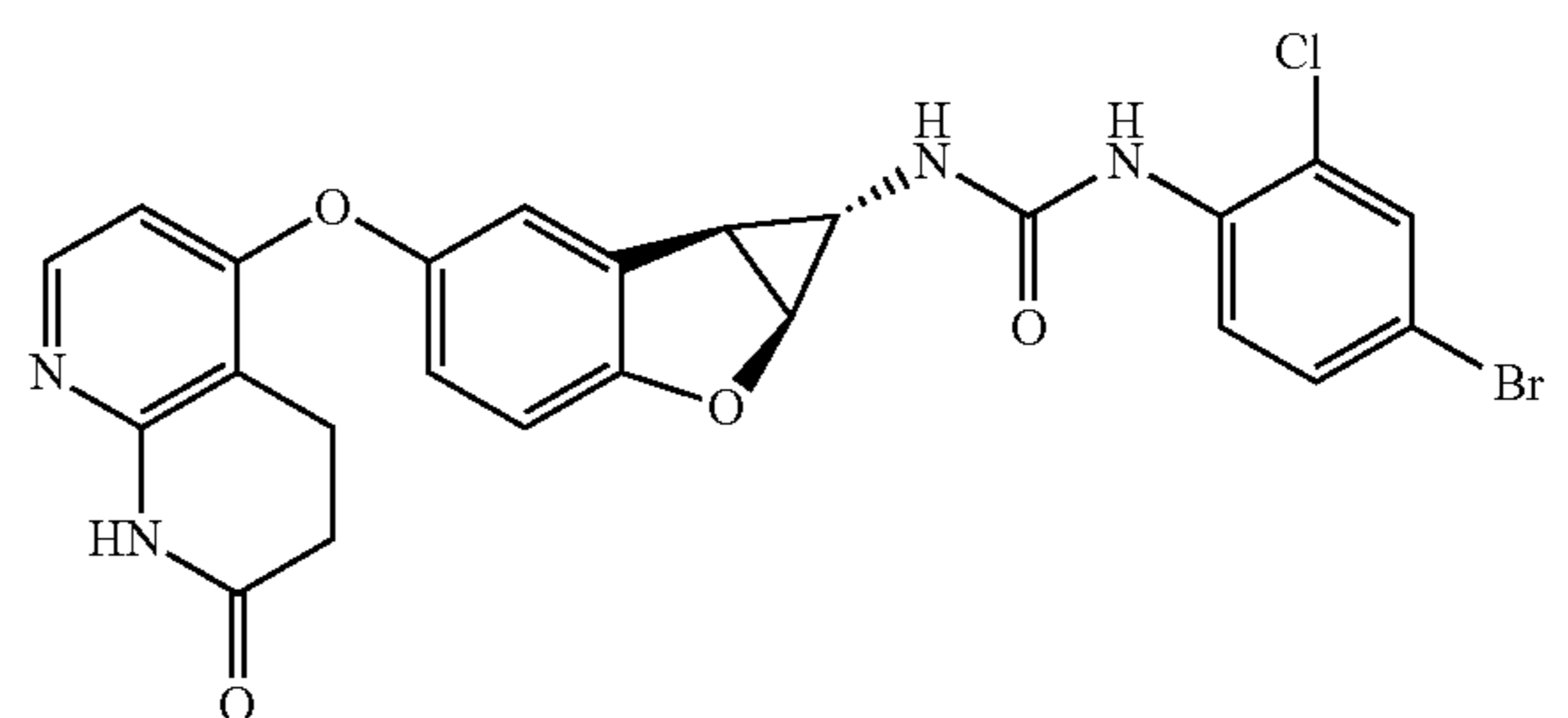
Compound 1.10
