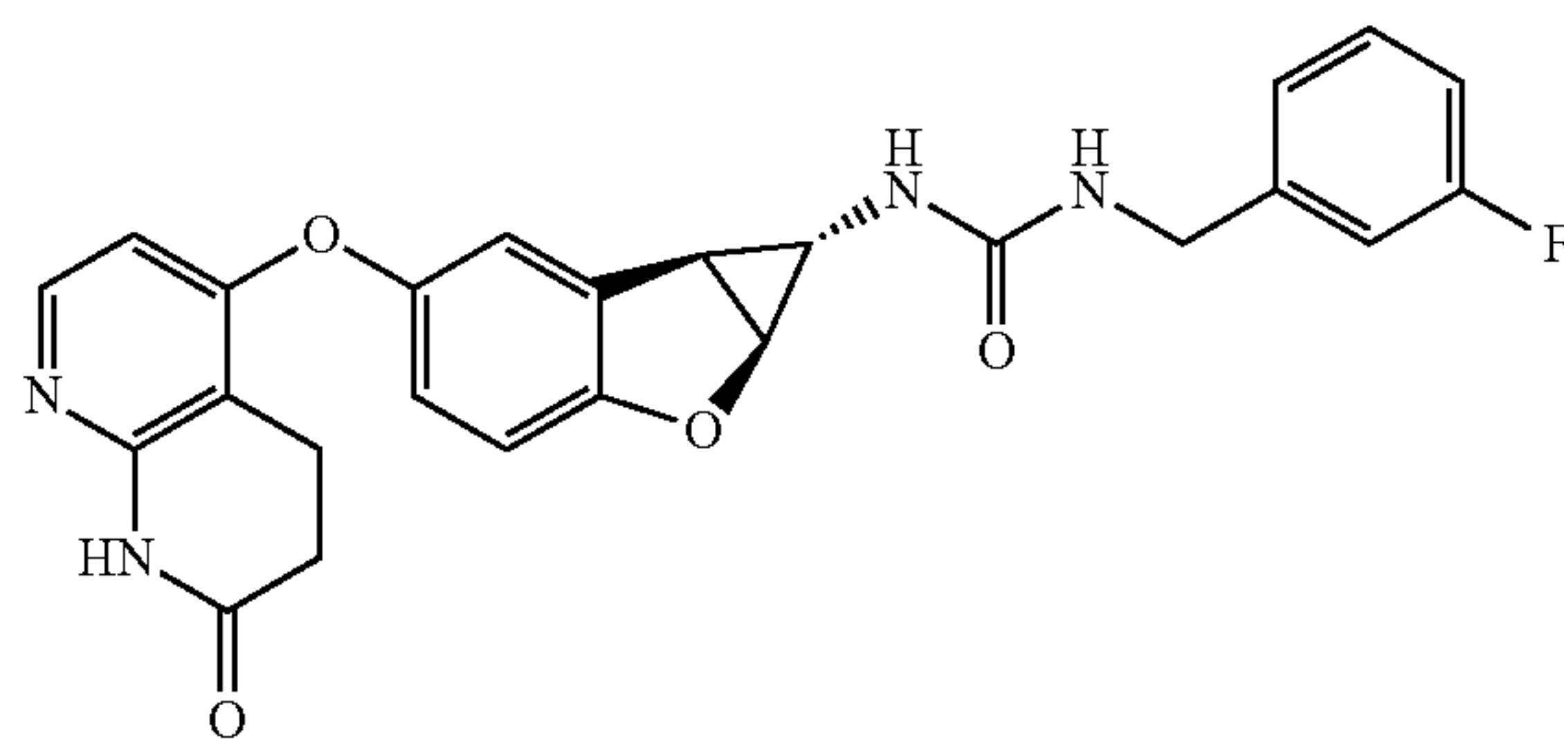
Compound 1.58
