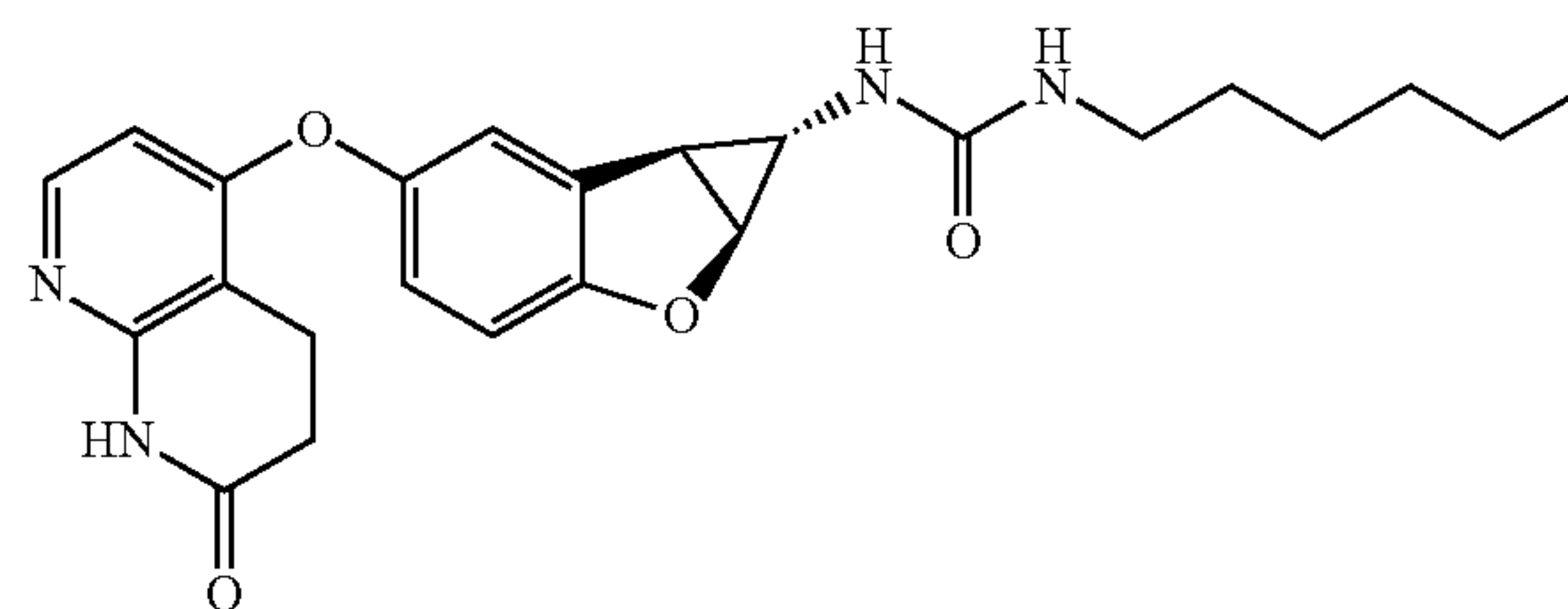
Compound 1.78
