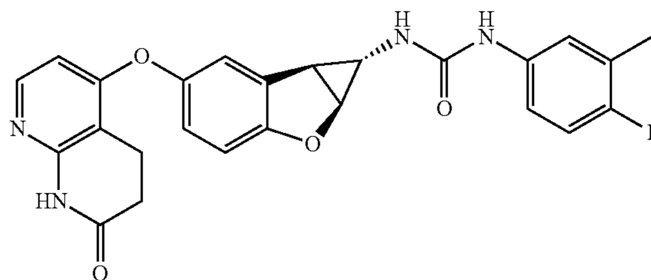
Compound 1.24
