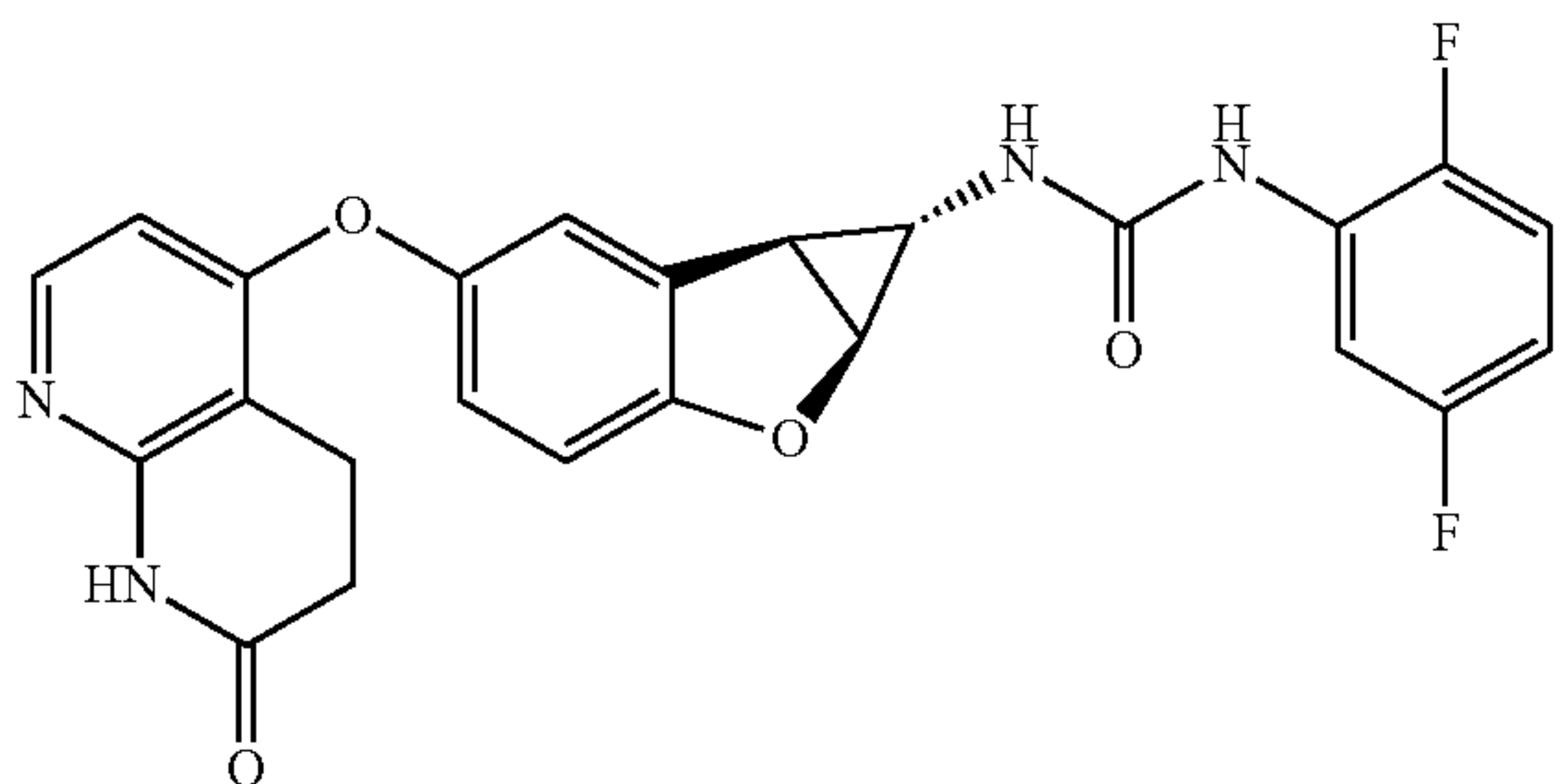
Compound 1.43
