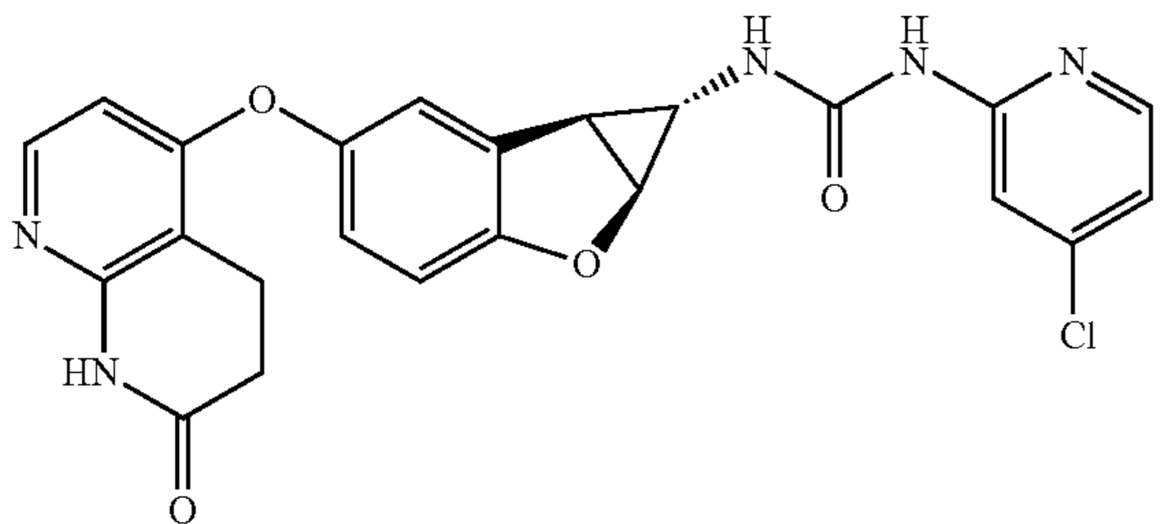
Compound 1.37
