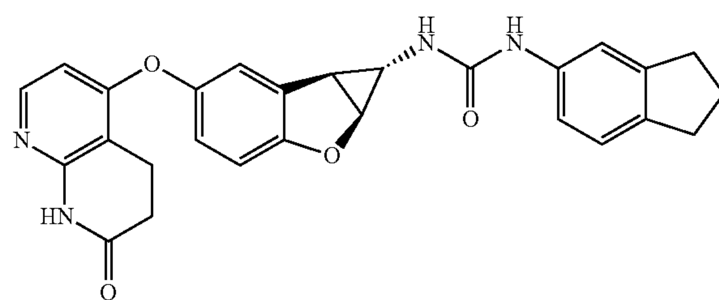
Compound 1.16
