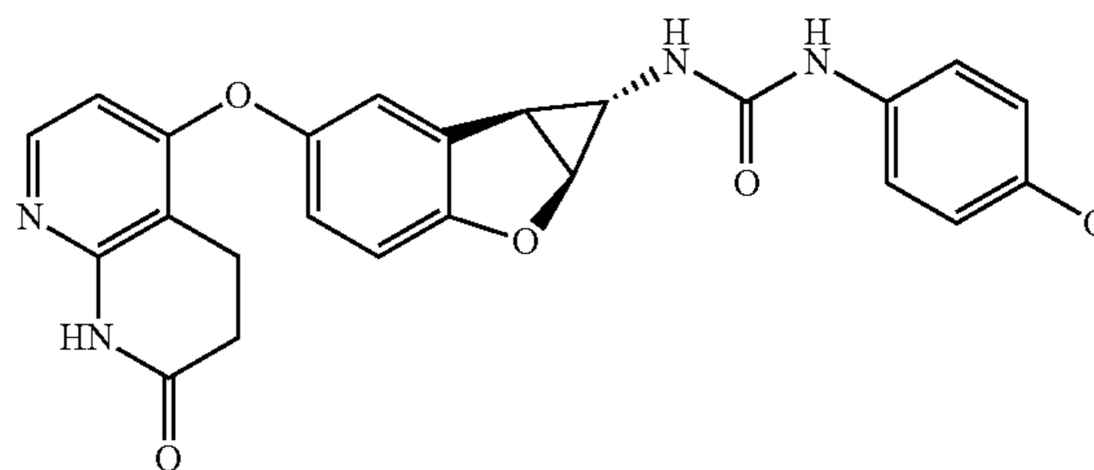
Compound 1.50
