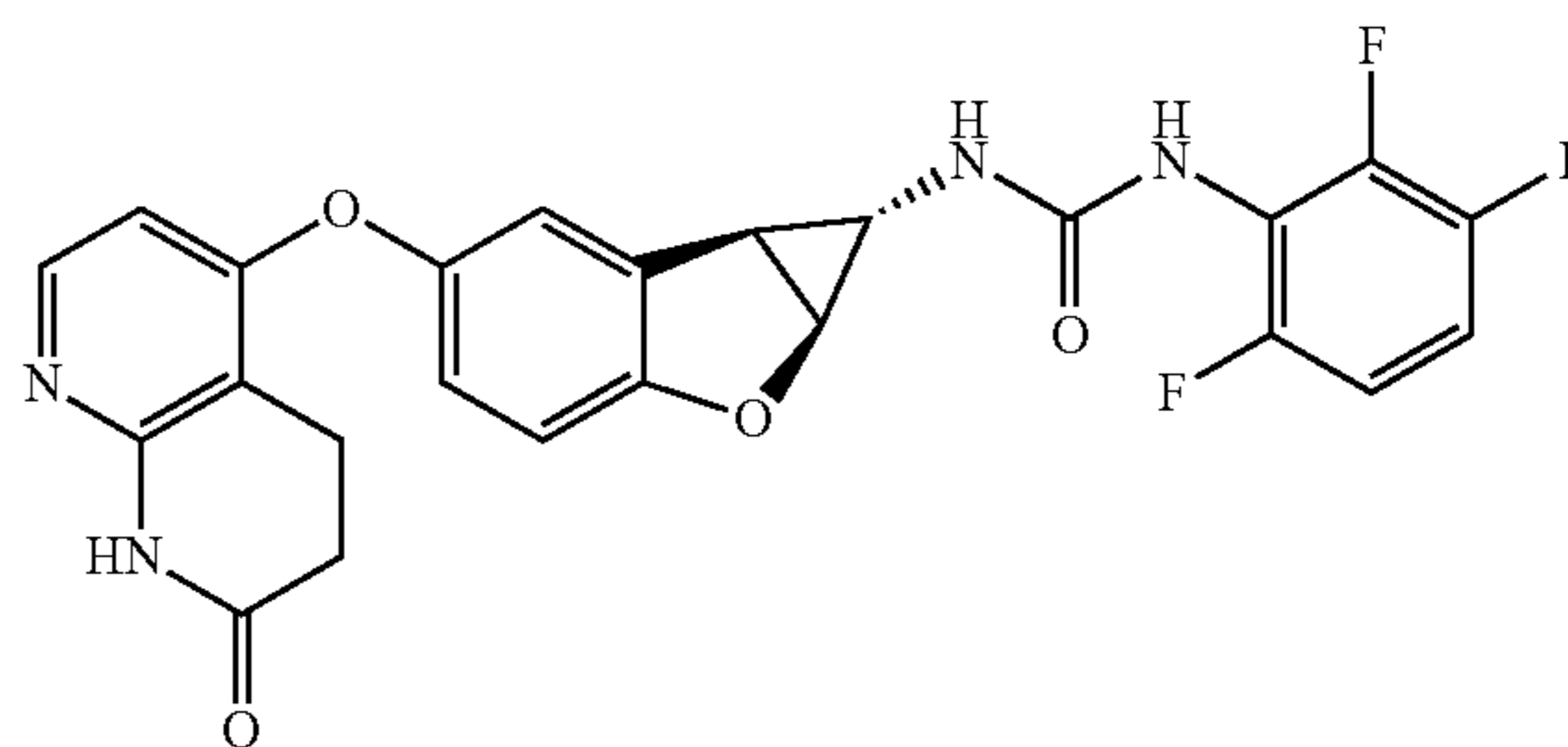
Compound 1.48
