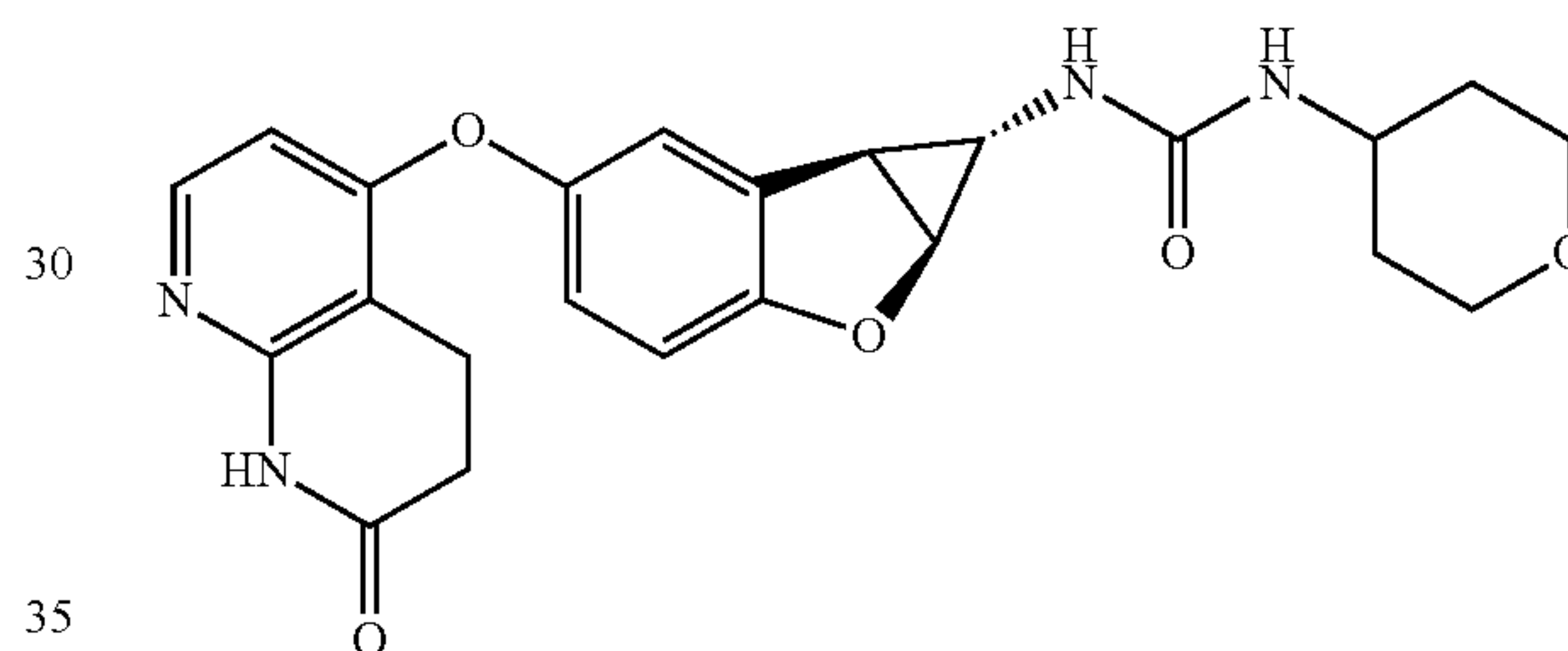
Compound 1.67
