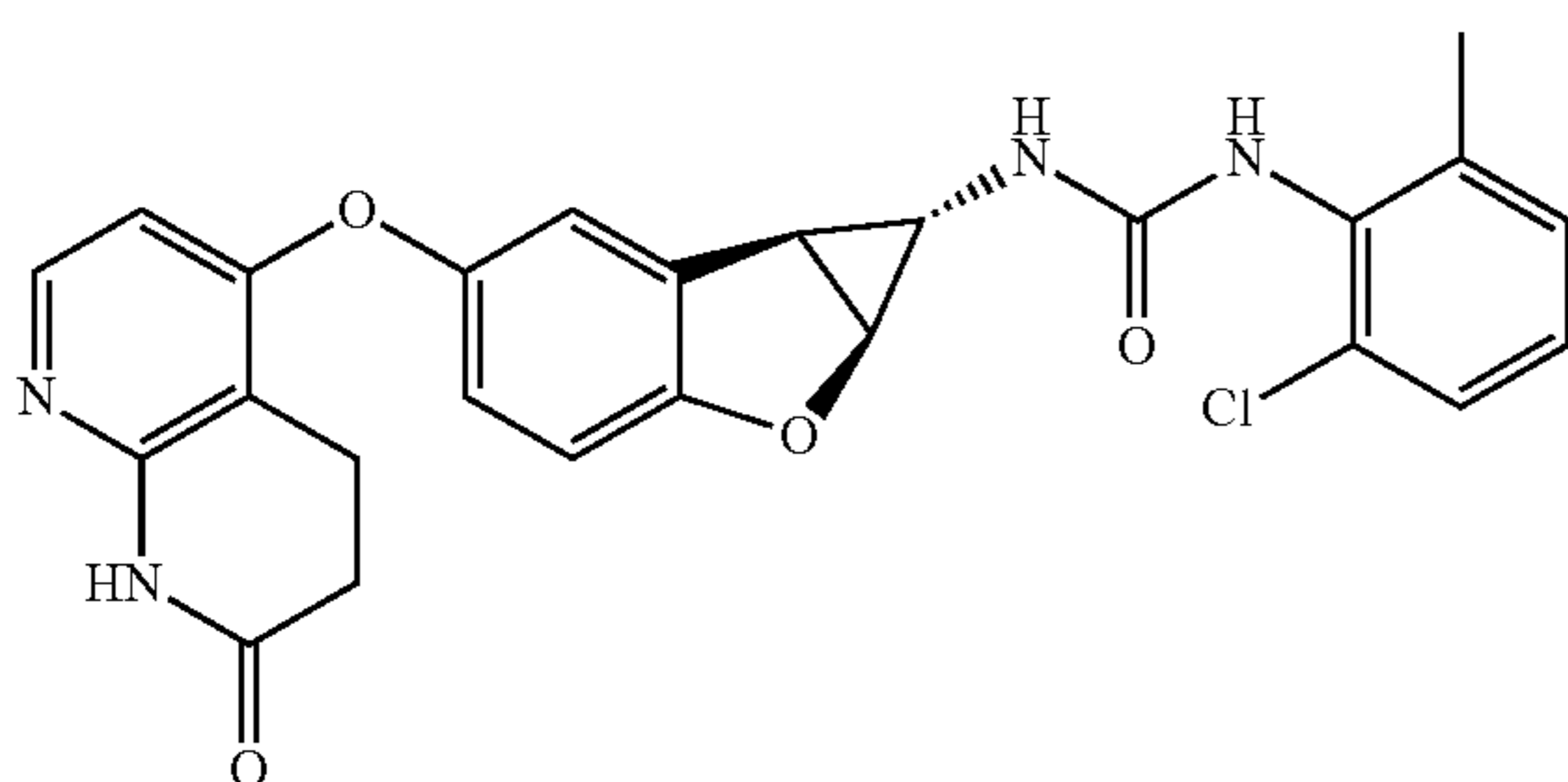
Compound 1.19
