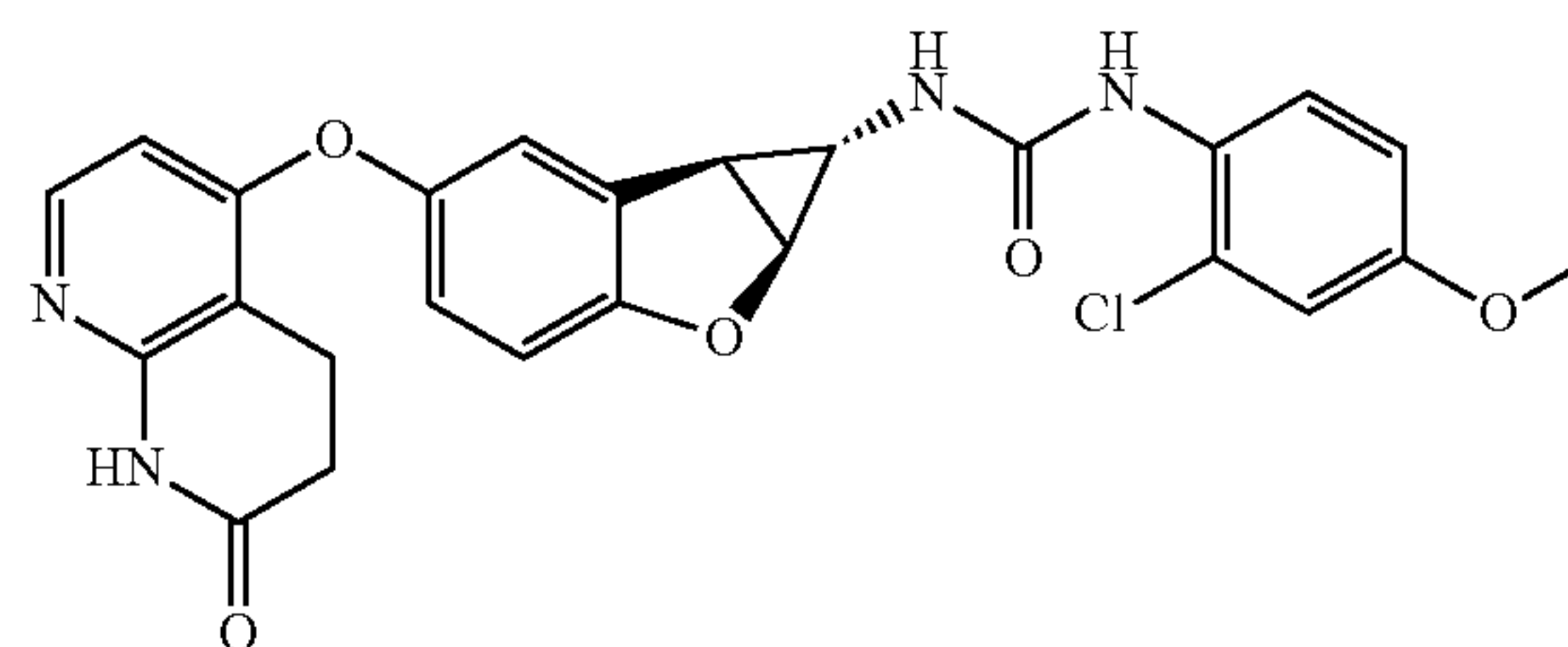
Compound 1.4
