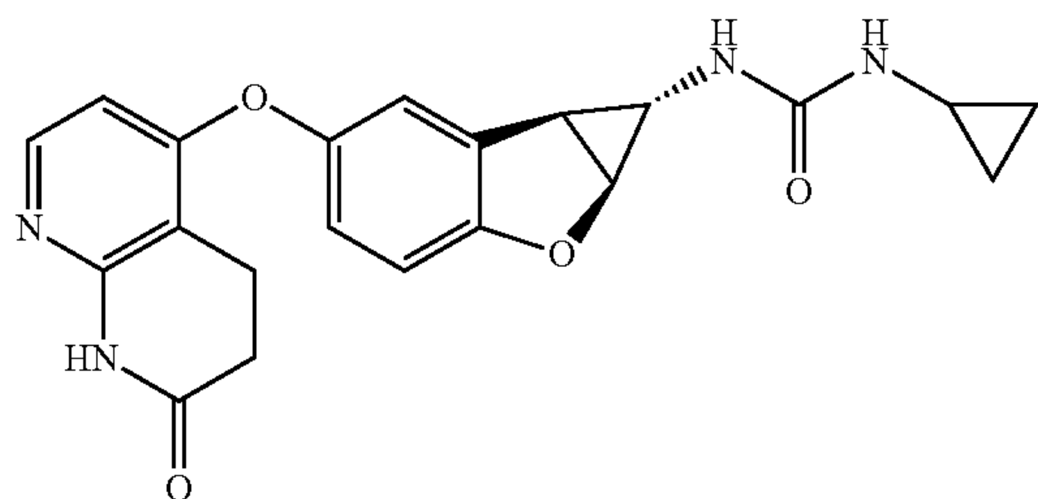
Compound 1.69
