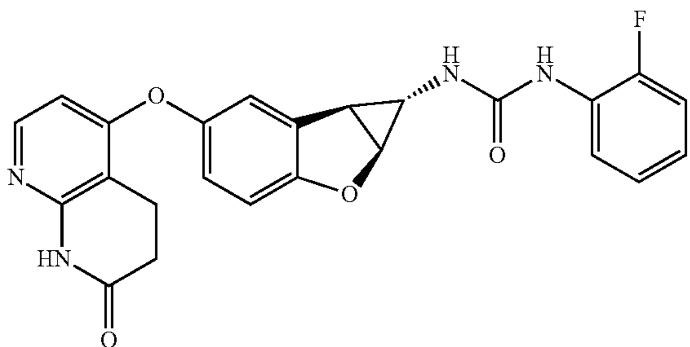
Compound 1.21
