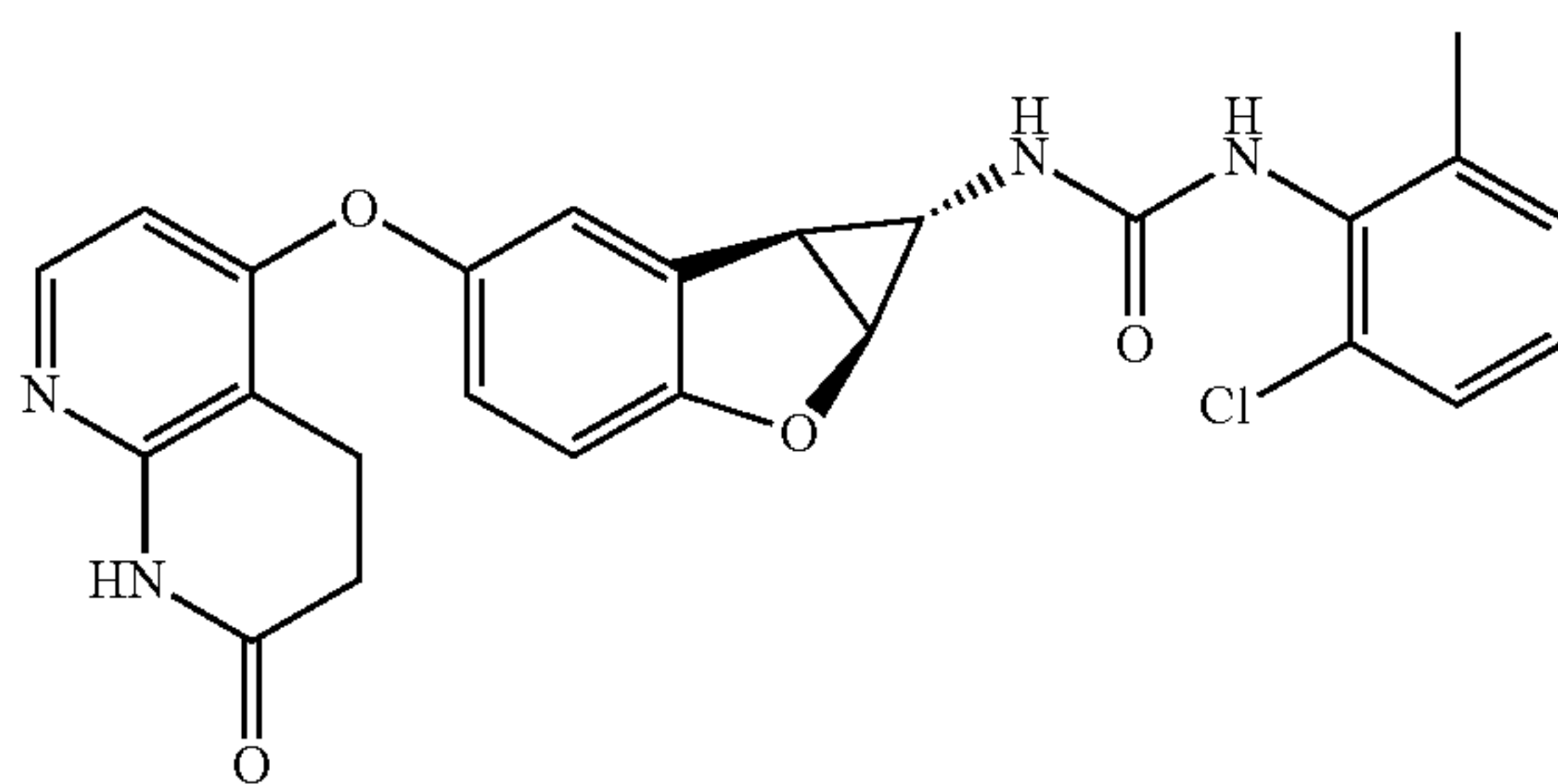
Compound 1.19
