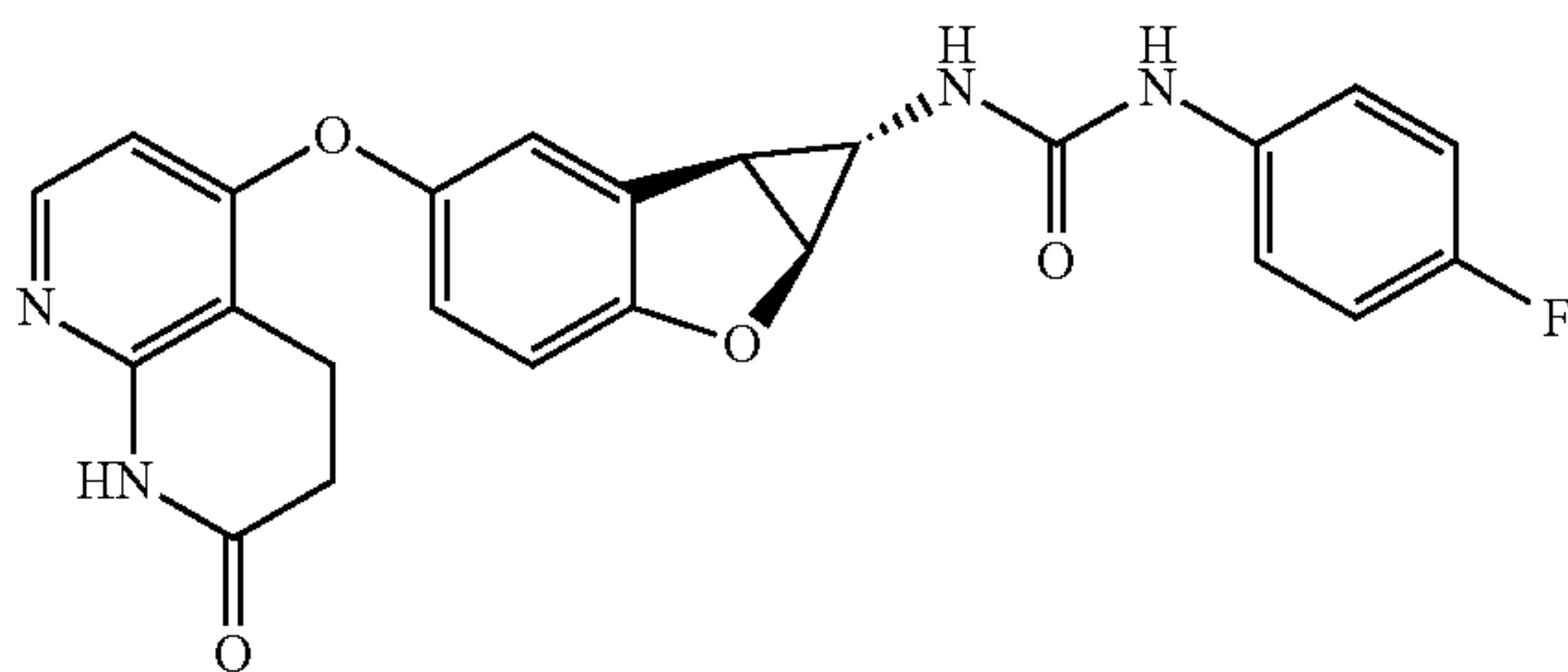
Compound 1.41
