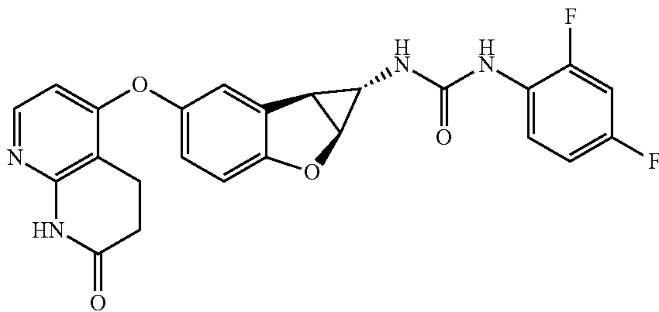
Compound 1.35
