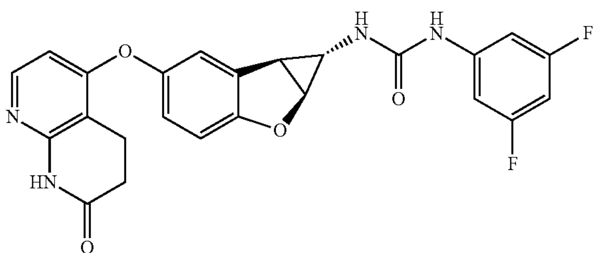
Compound 1.23
