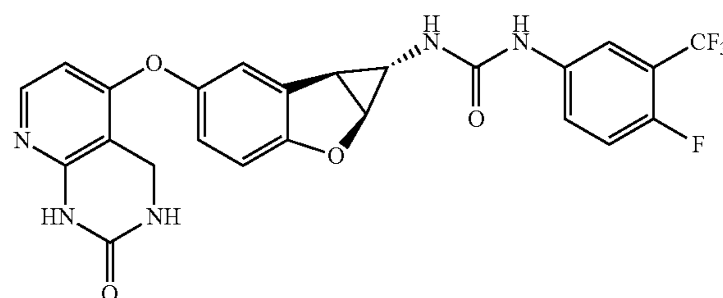
Compound 2.4
