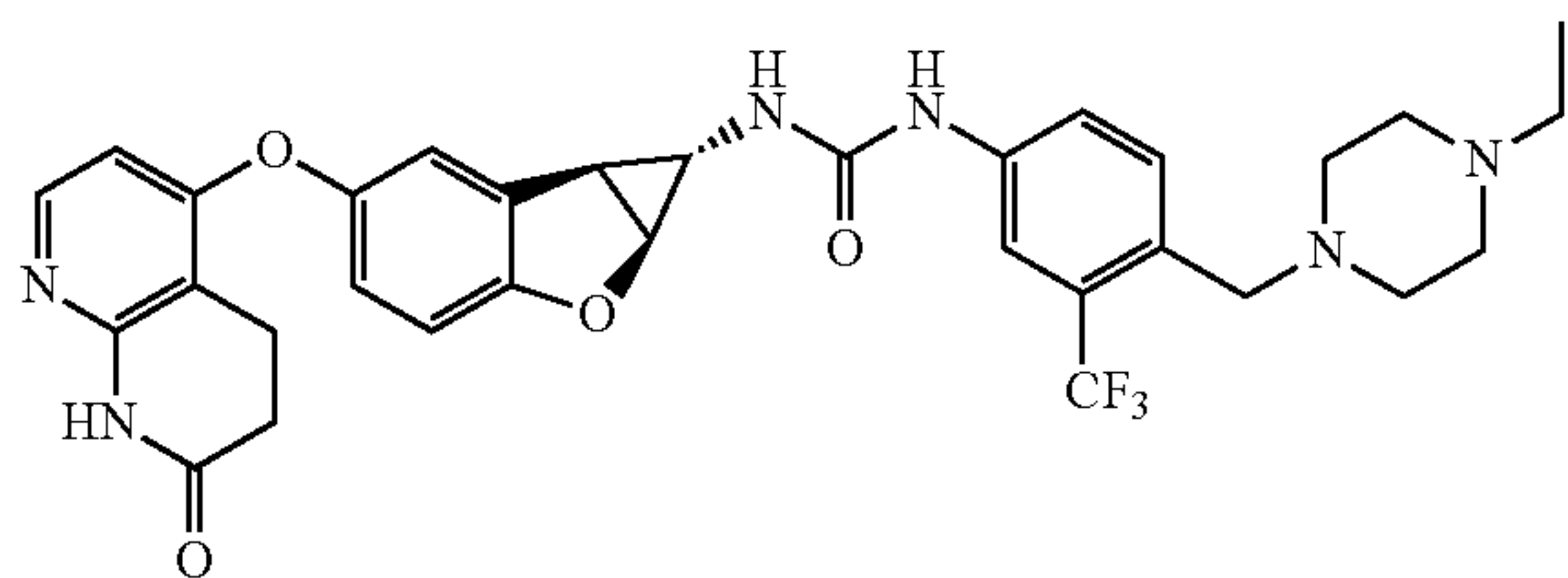
Compound 1.75
