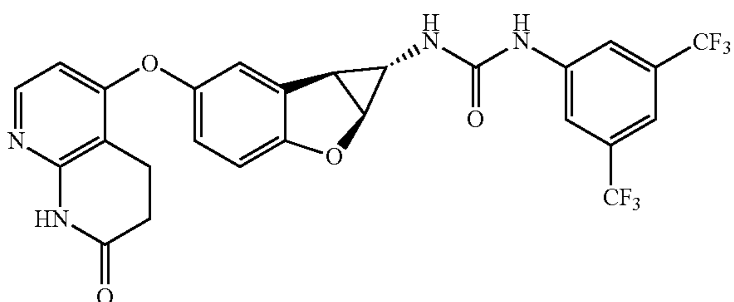
Compound 1.67
