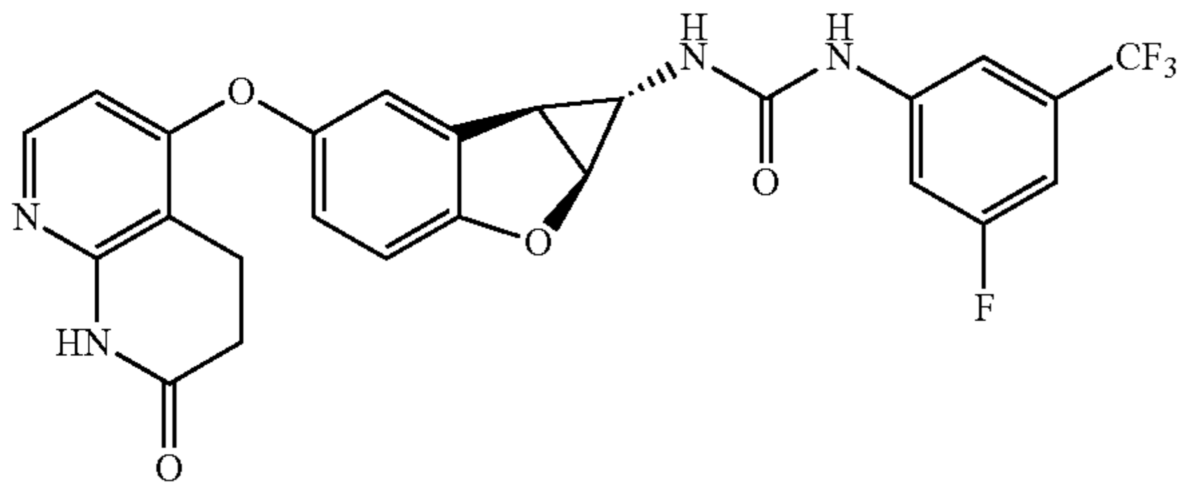
Compound 1.11
