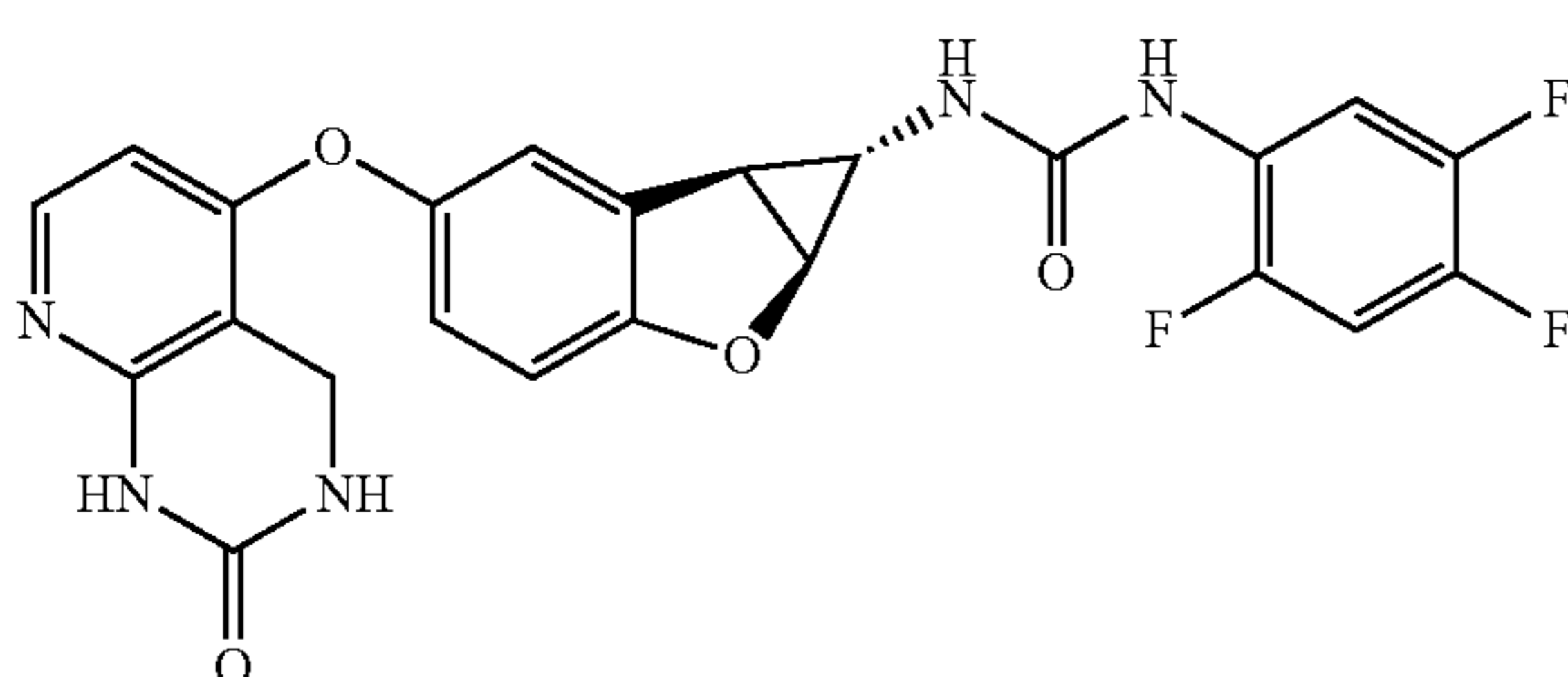
Compound 2.5
