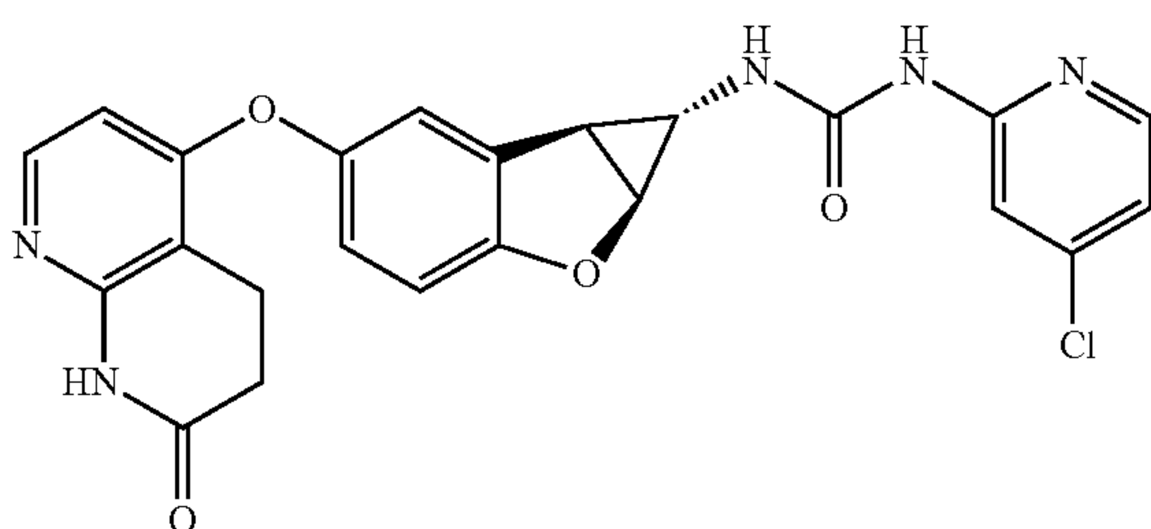
Compound 1.37
