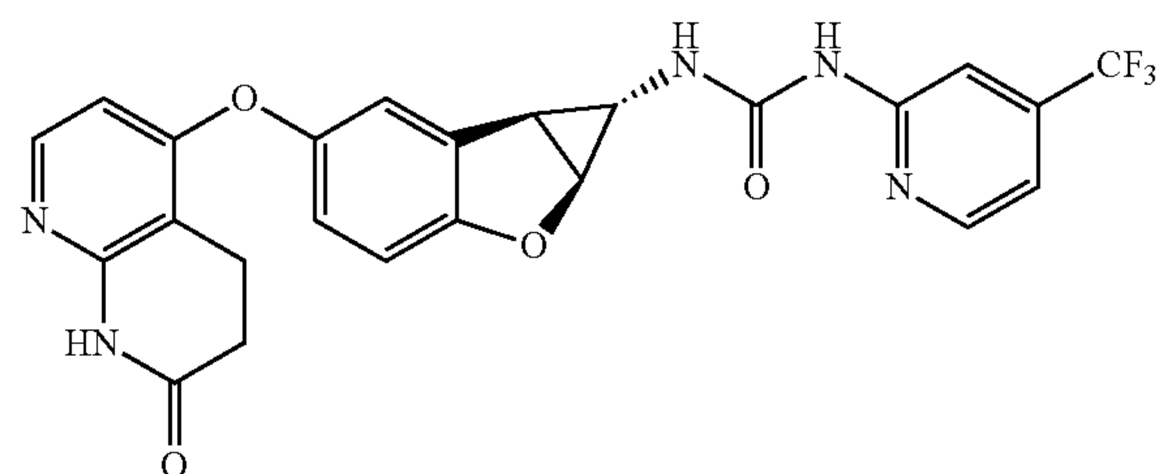
Compound 1.2
