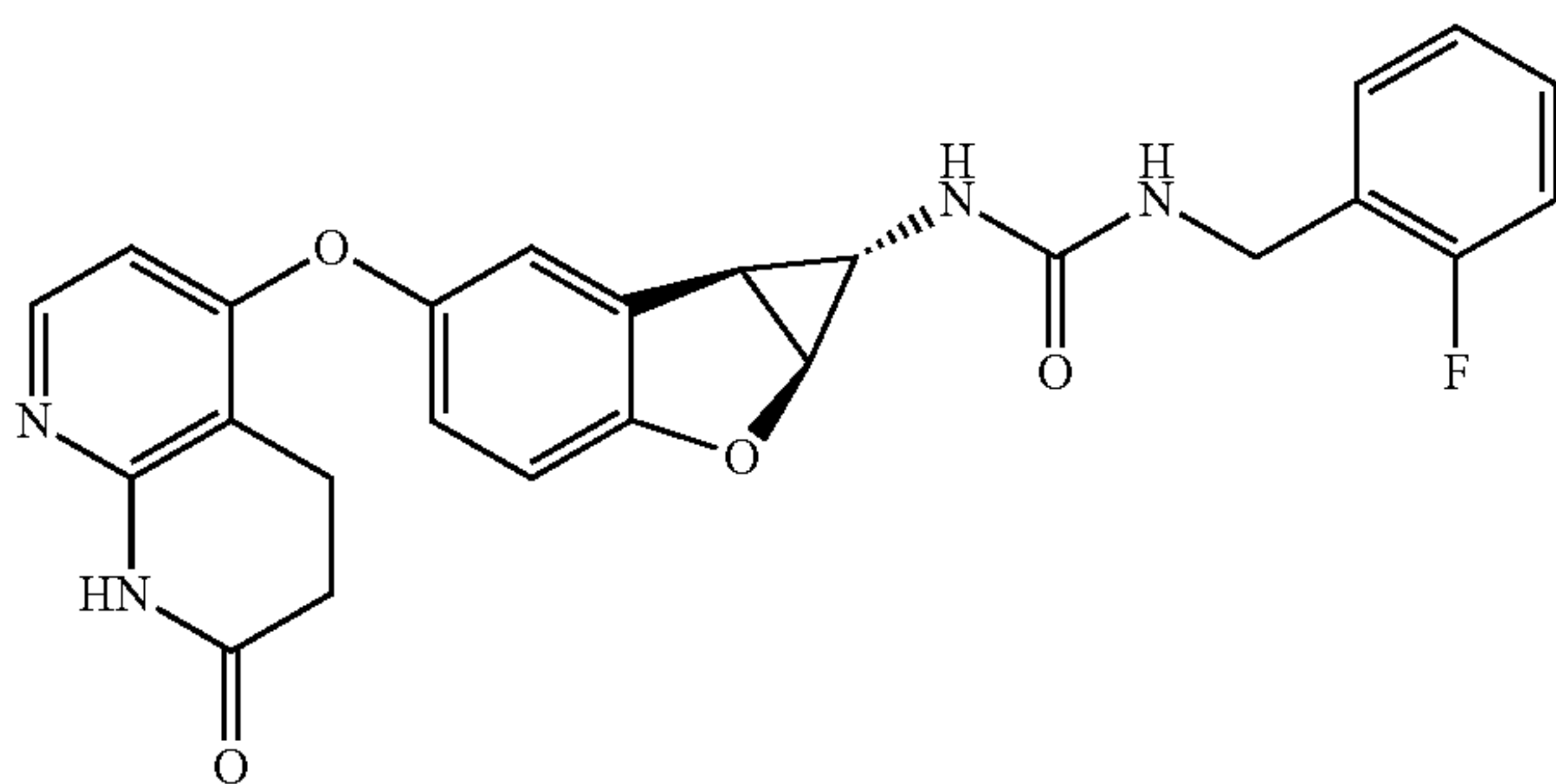
Compound 1.57
