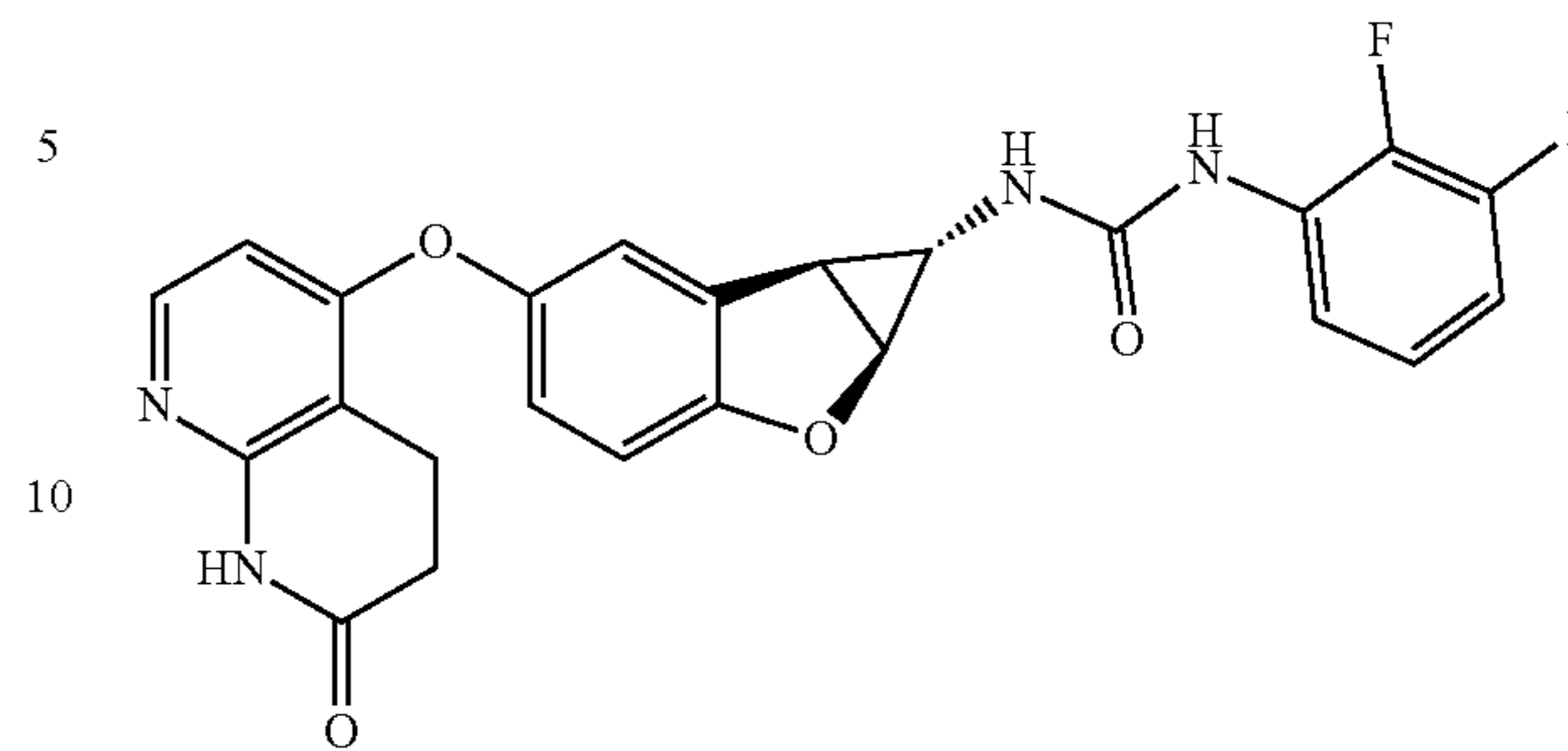
Compound 1.42
