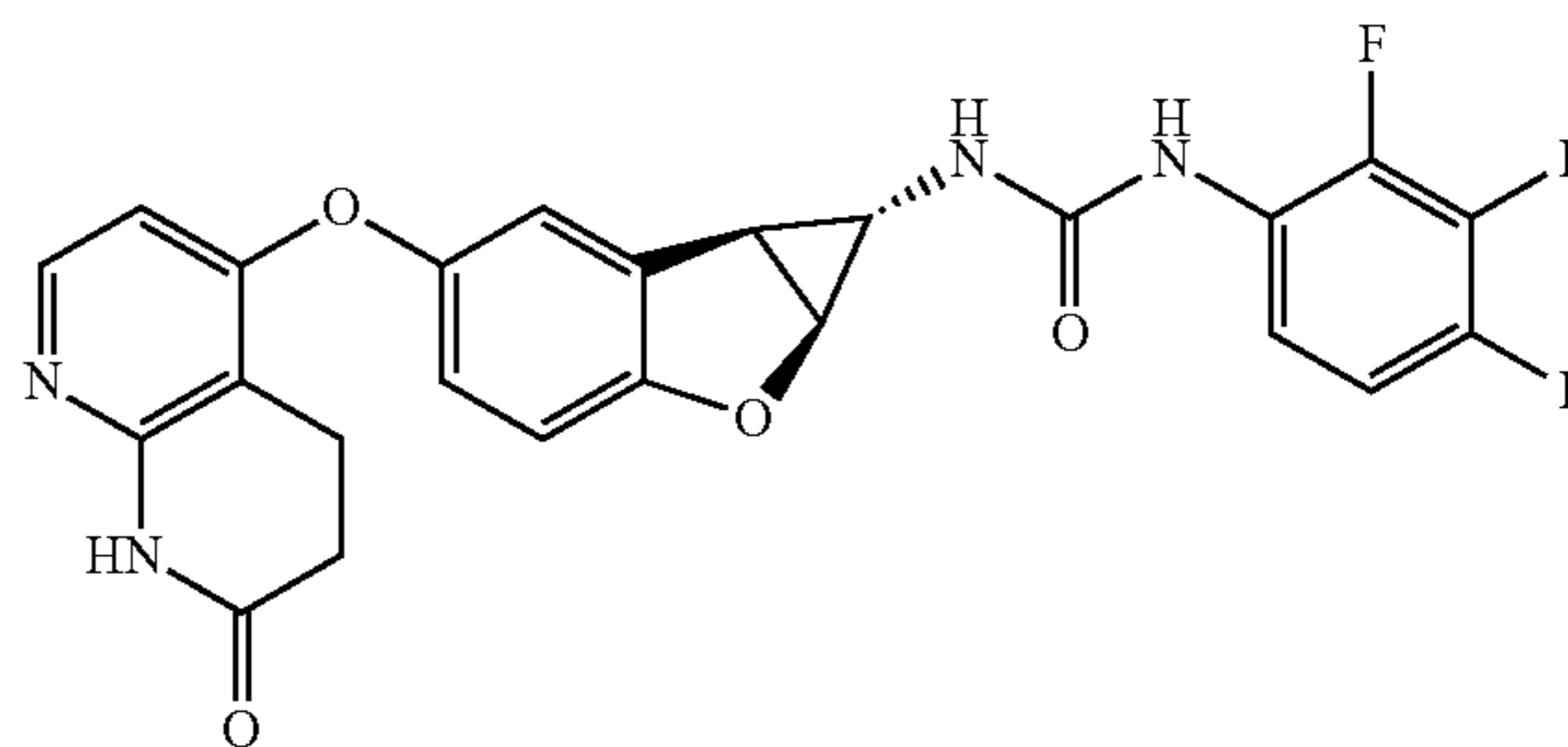
Compound 1.46
