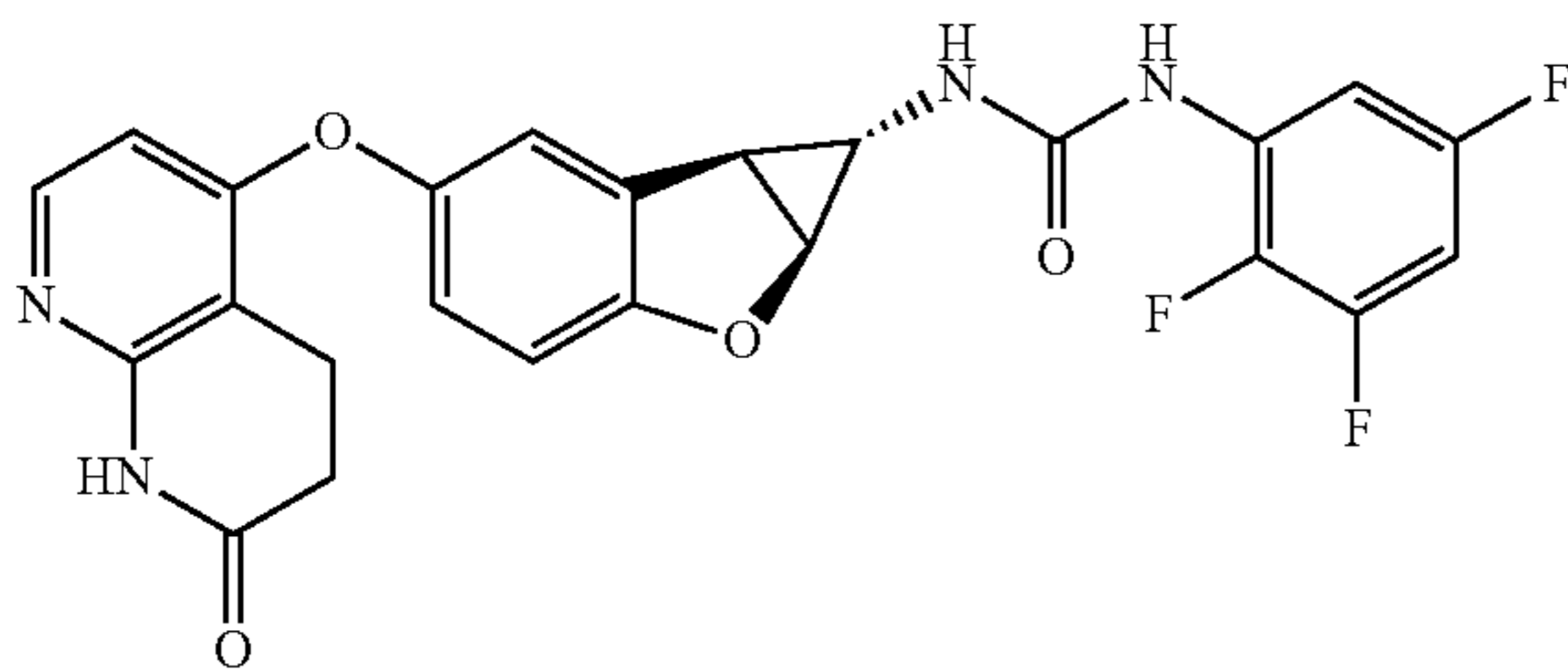
Compound 1.53
