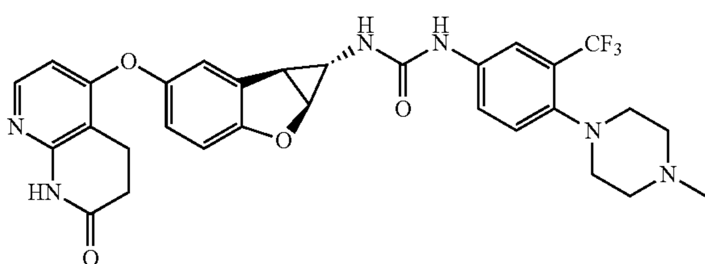
Compound 1.86
