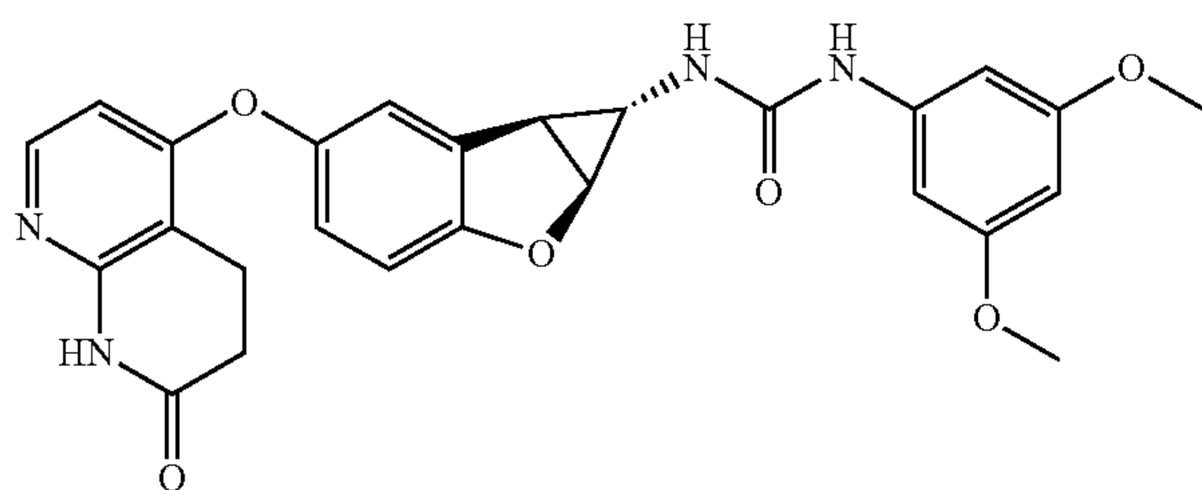
Compound 1.17
