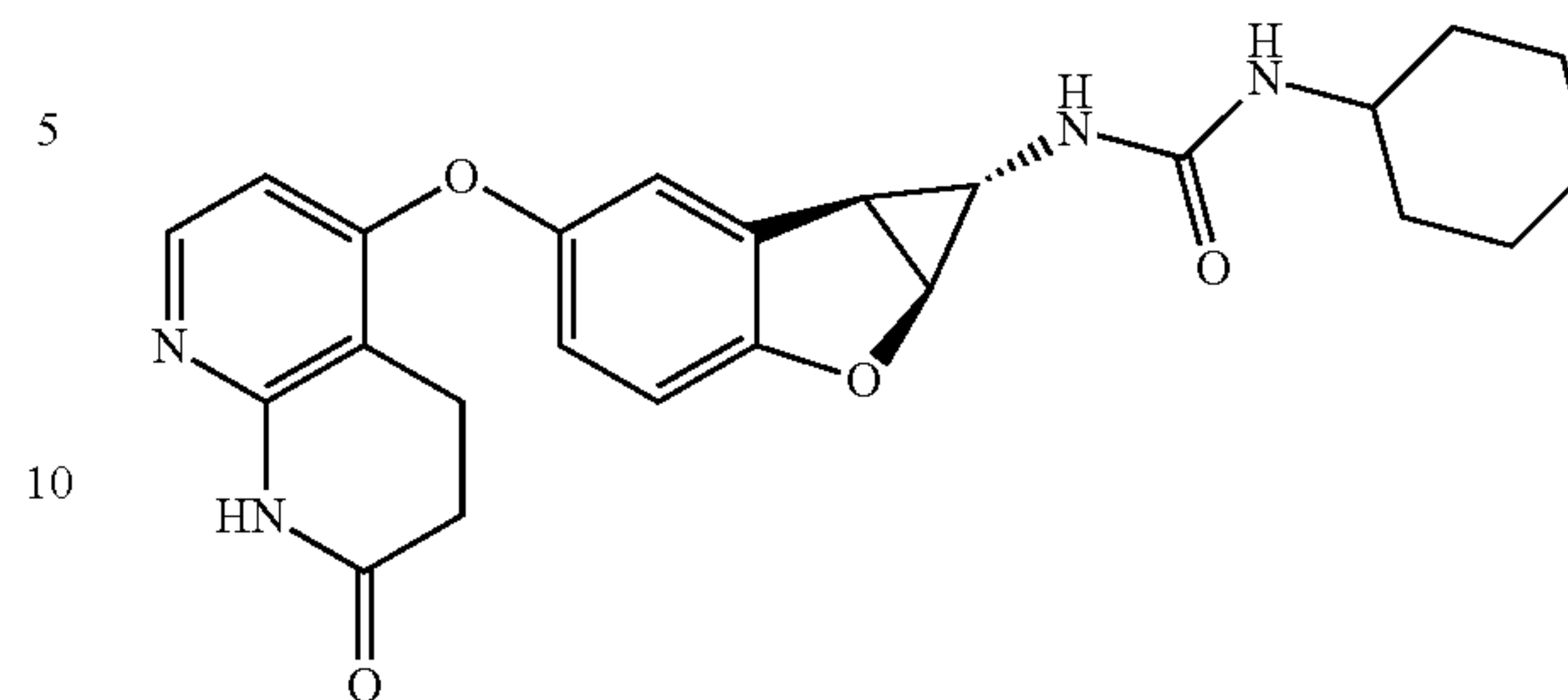
Compound 1.66
