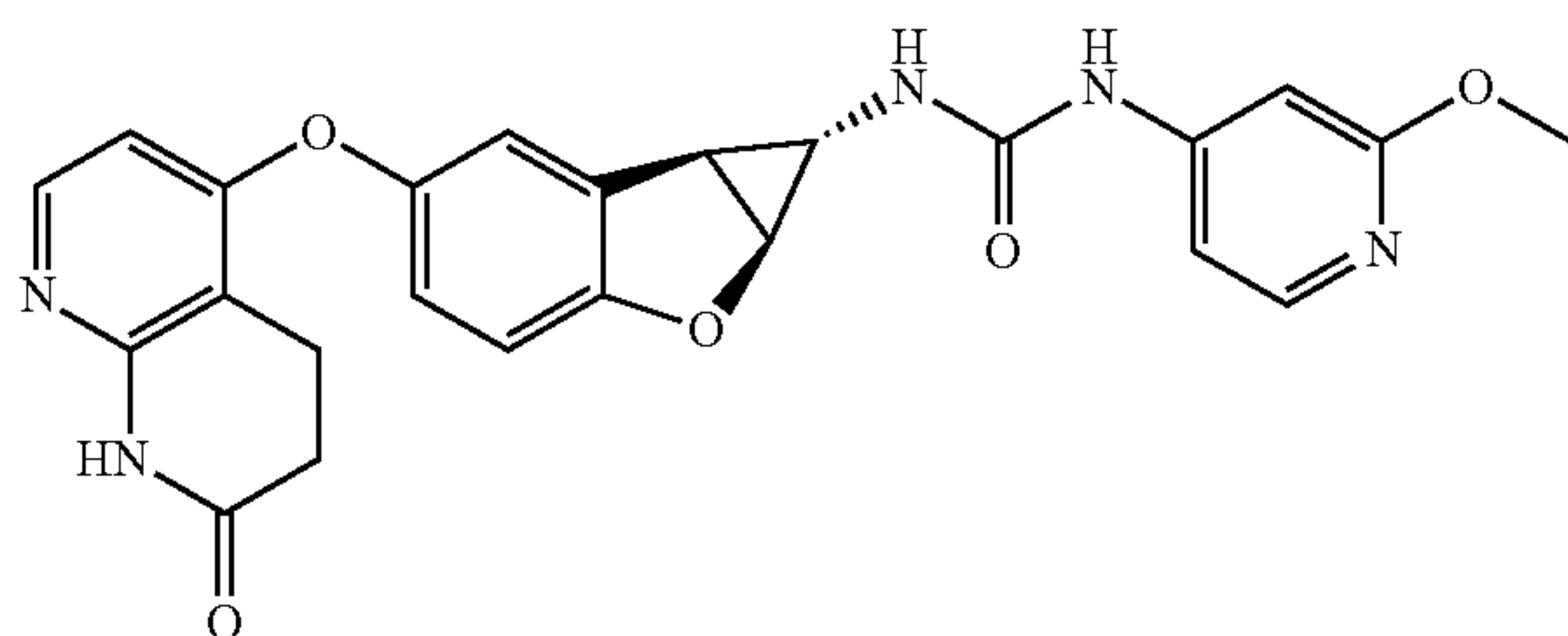
Compound 1.77
