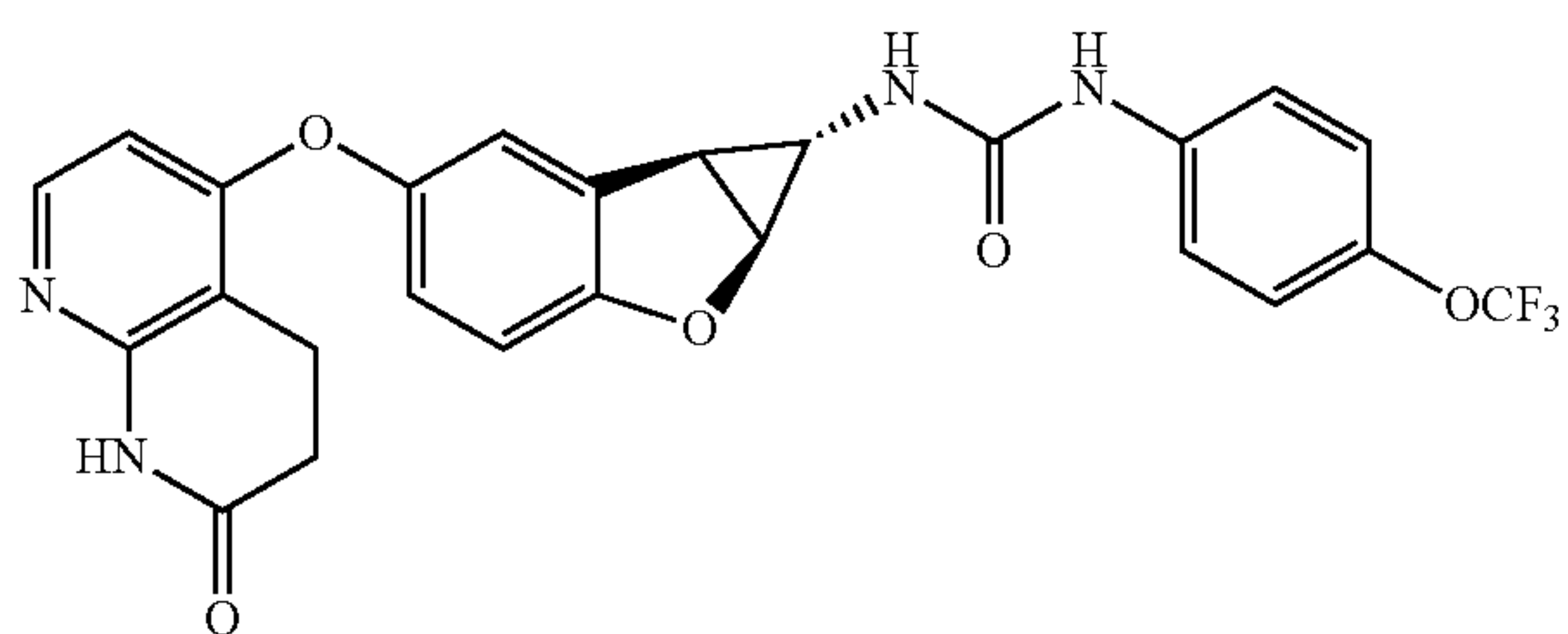
Compound 1.61
