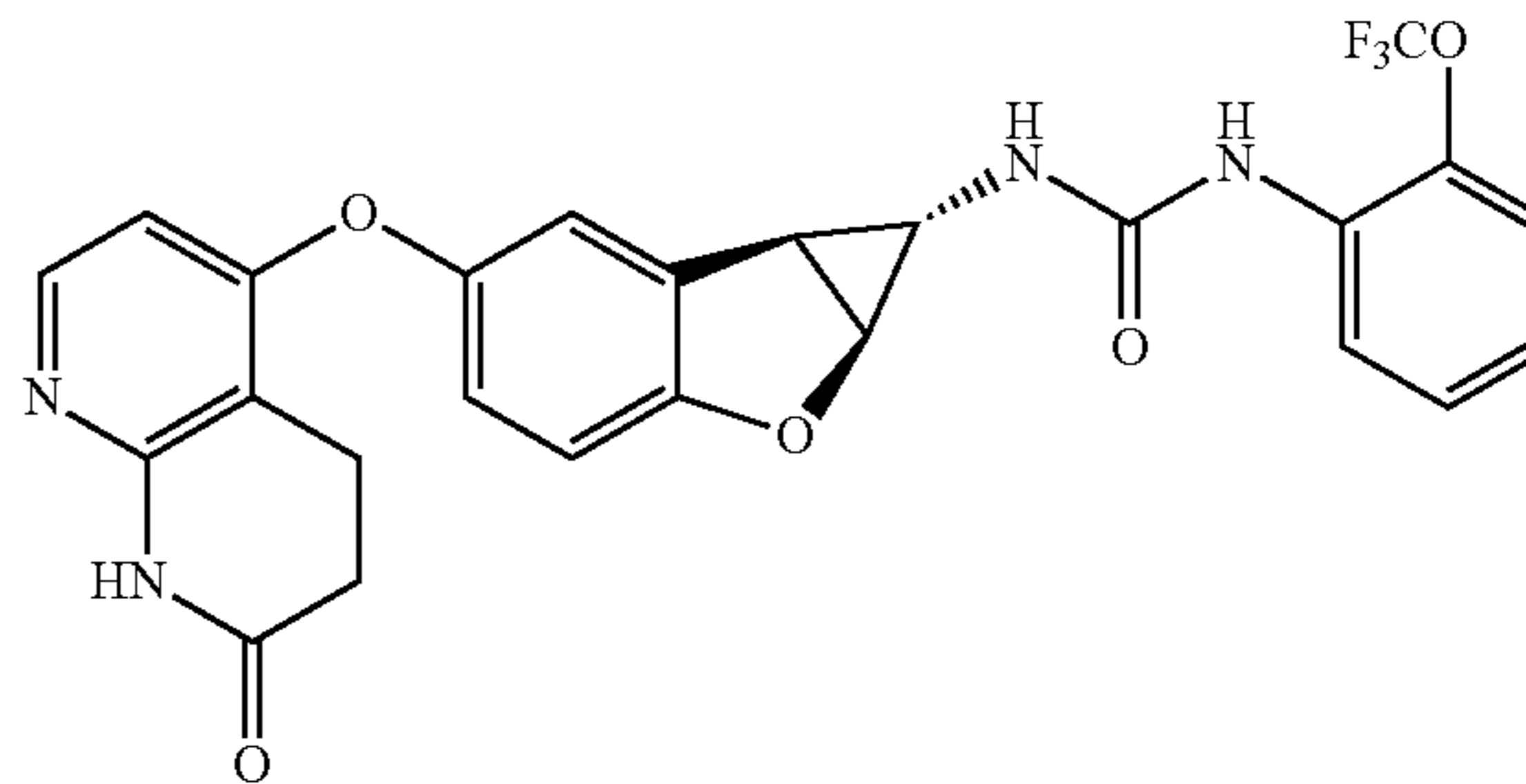
Compound 1.64
