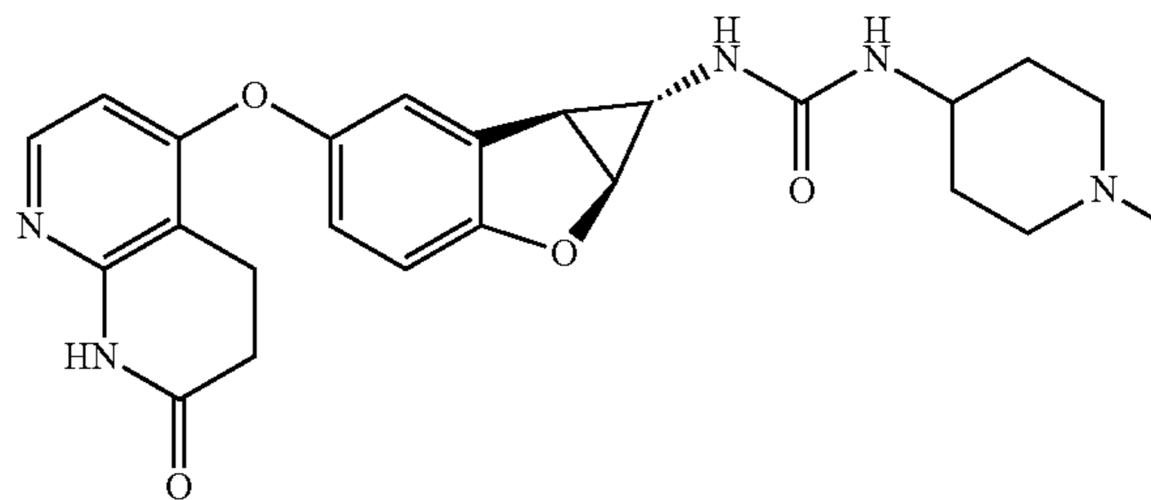
Compound 1.70
