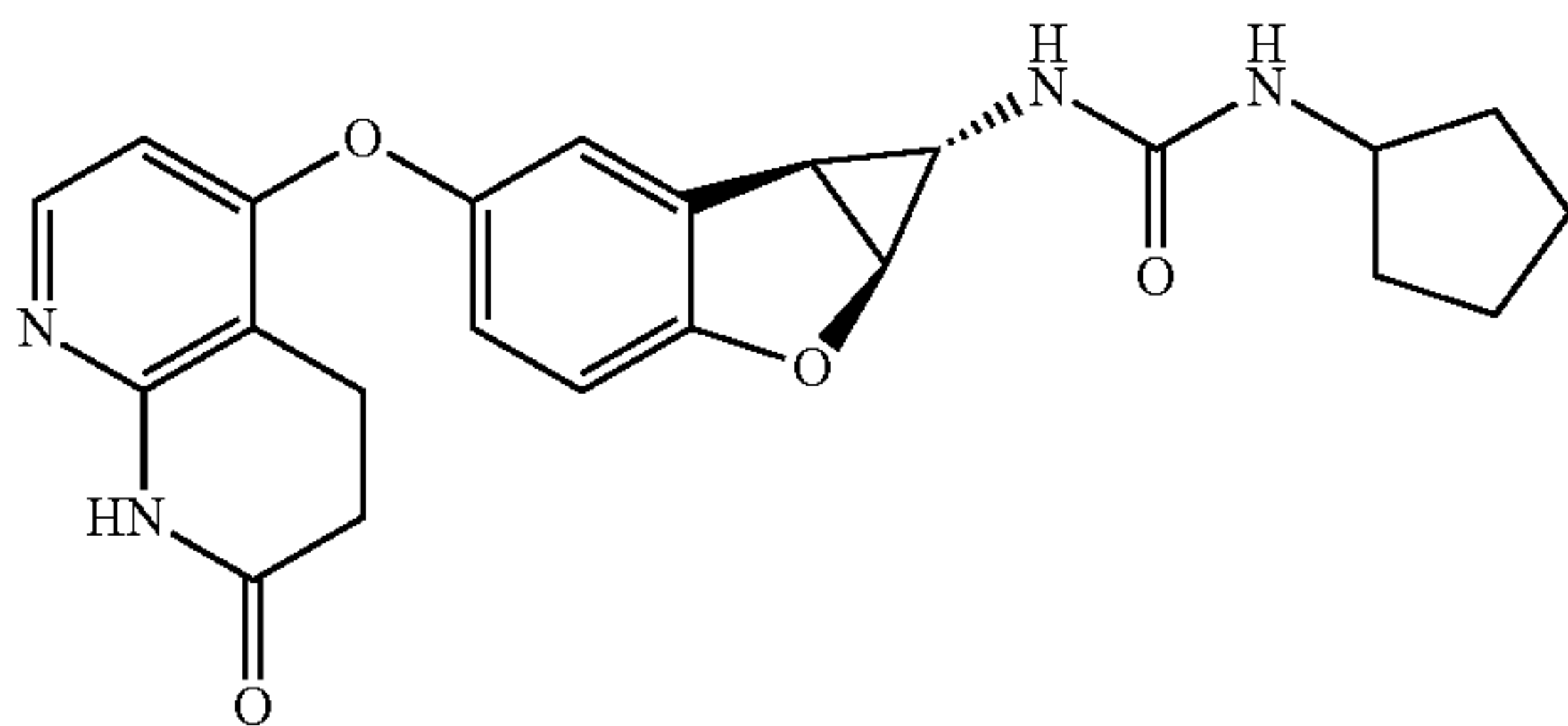
Compound 1.51
