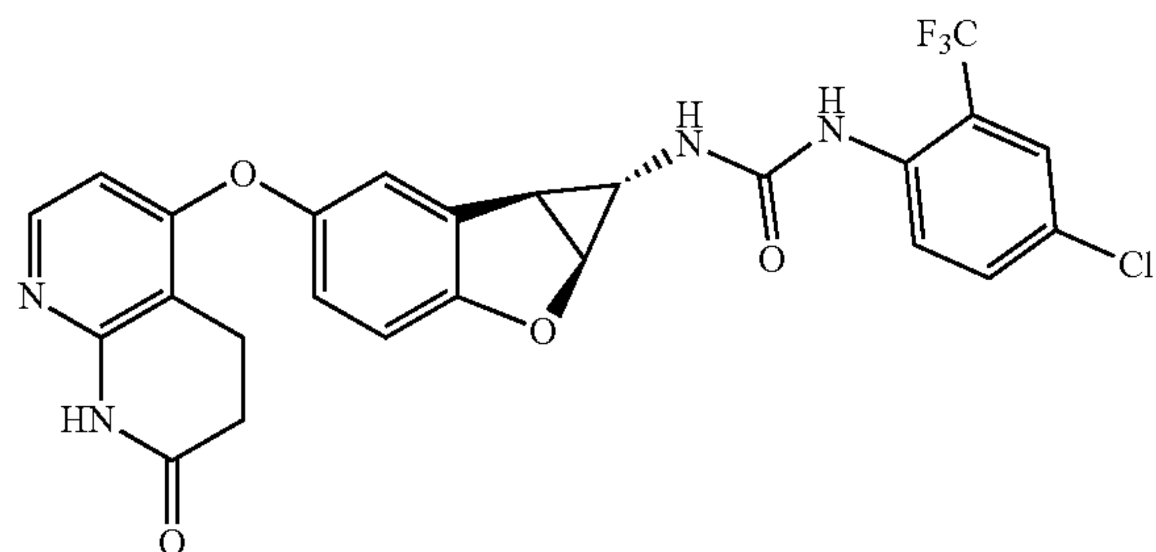
Compound 1.9
