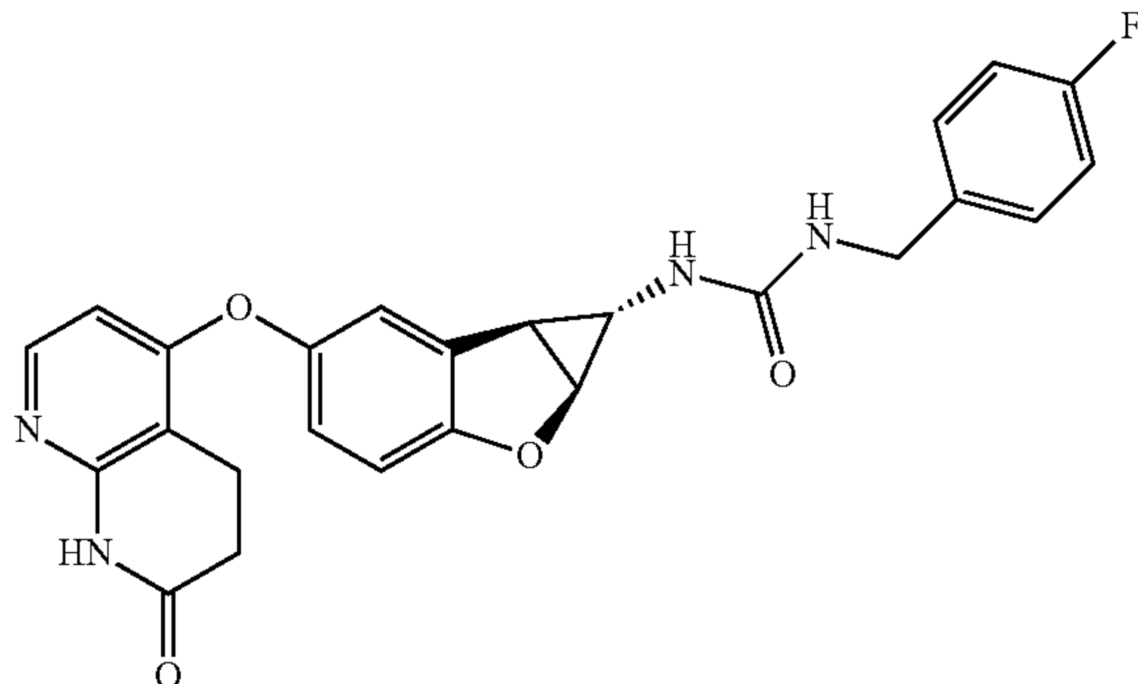
Compound 1.59
