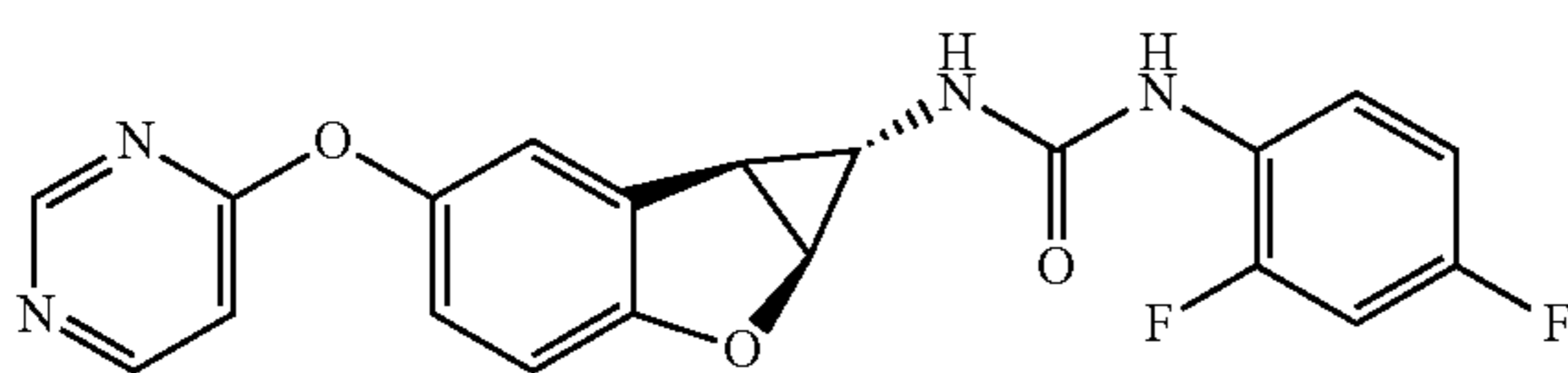
Compound 2.1
