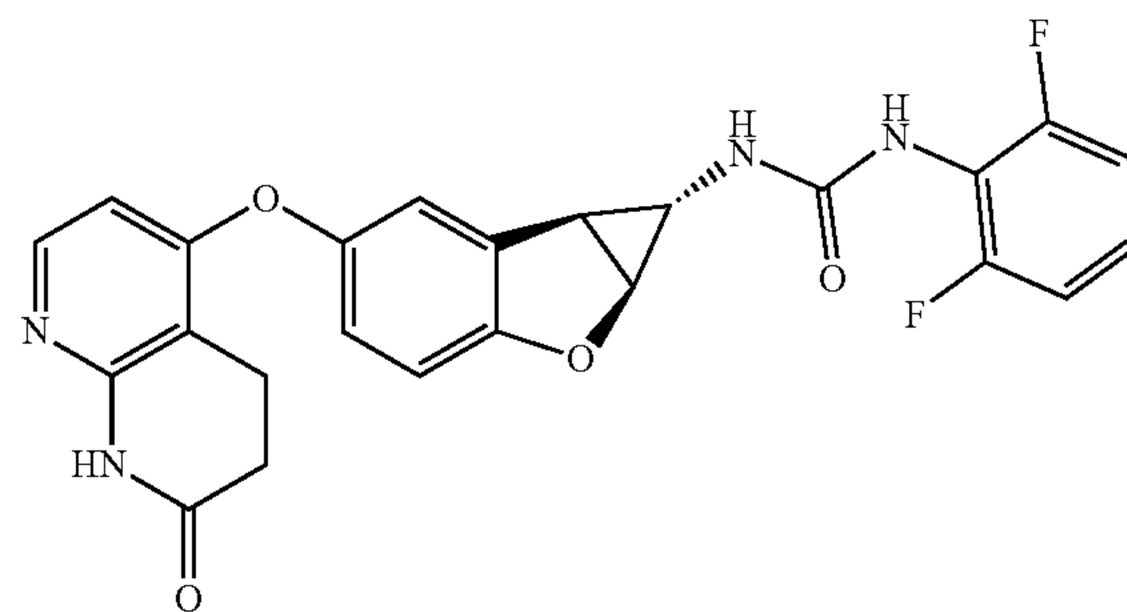
Compound 1.44
