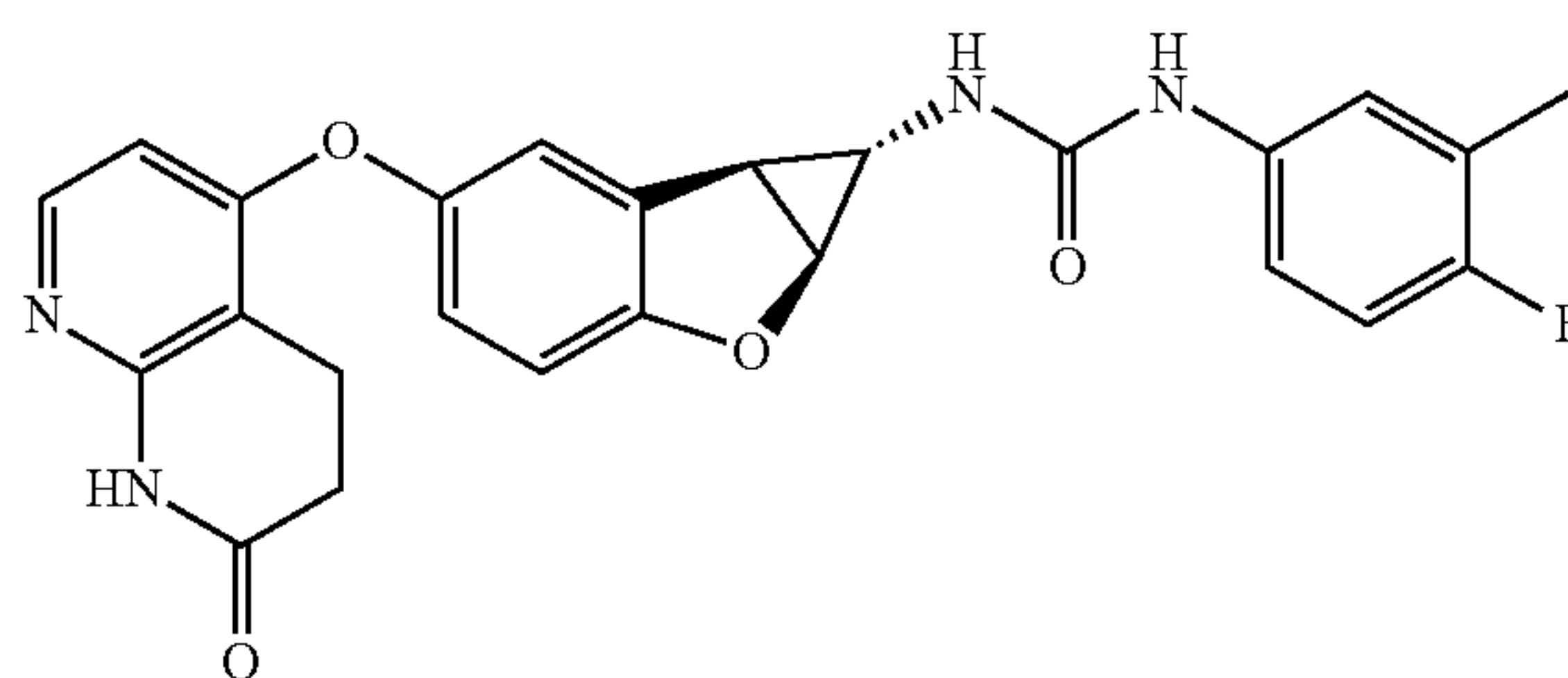
Compound 1.24
