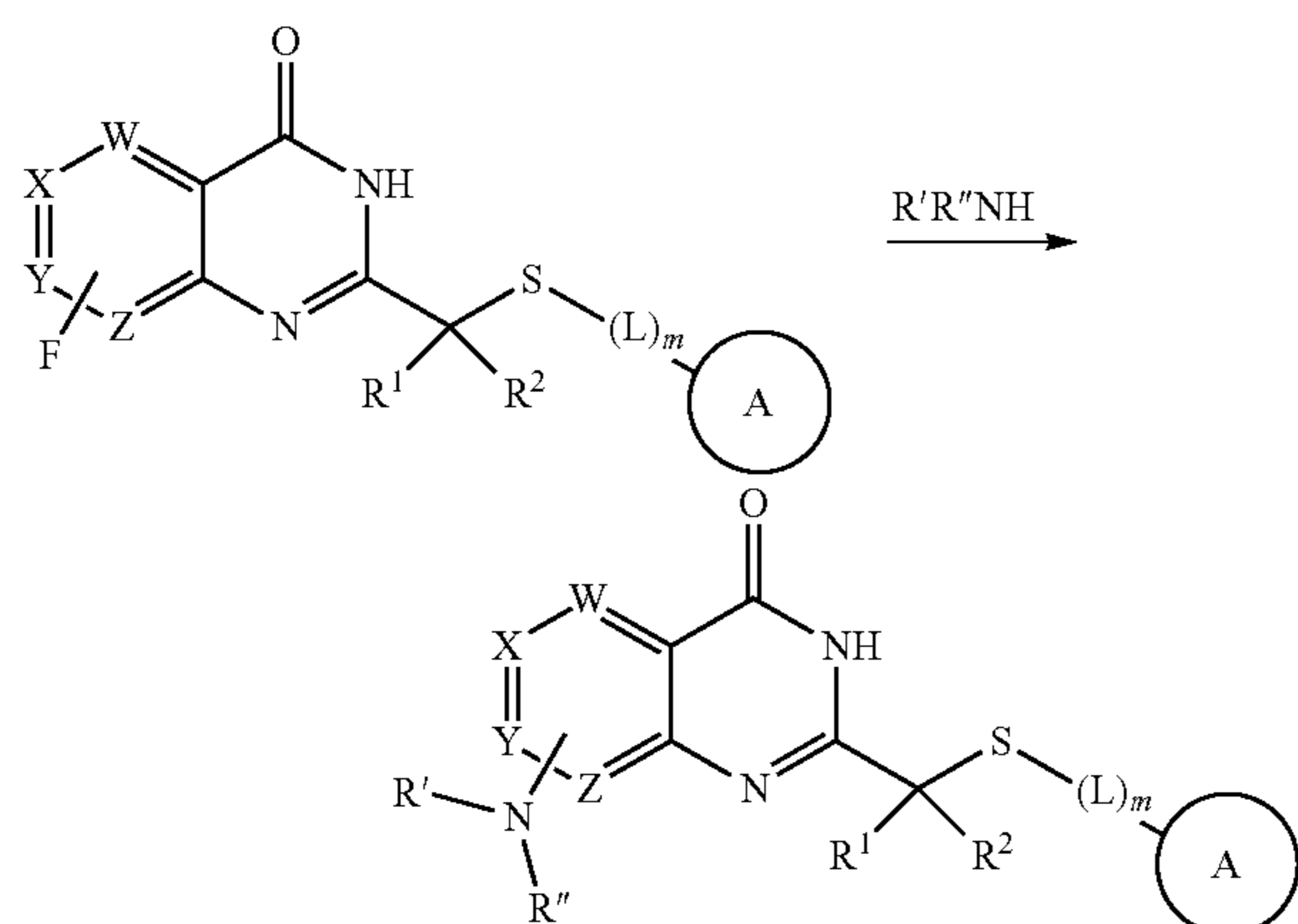
Scheme 4
