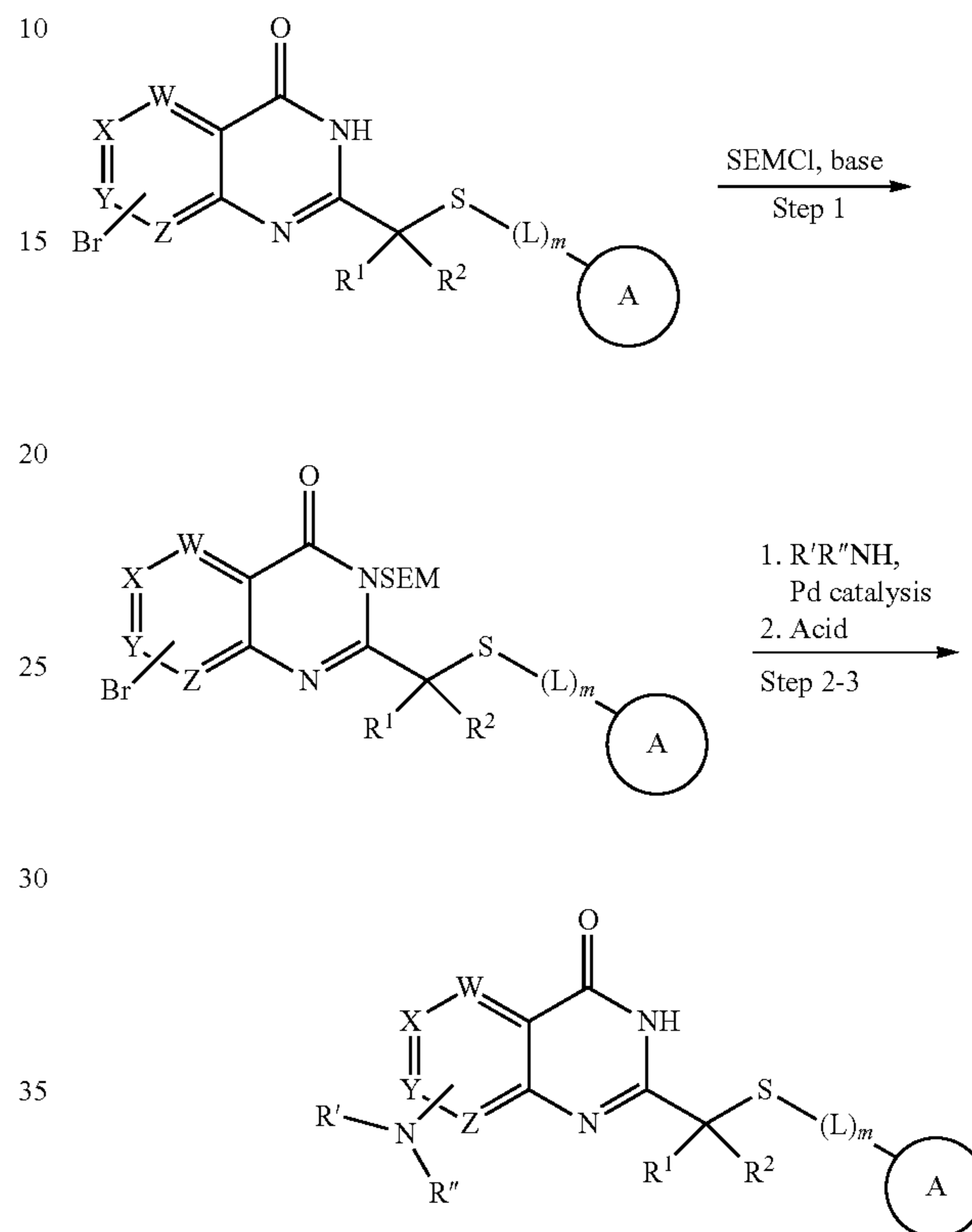
Scheme 6
