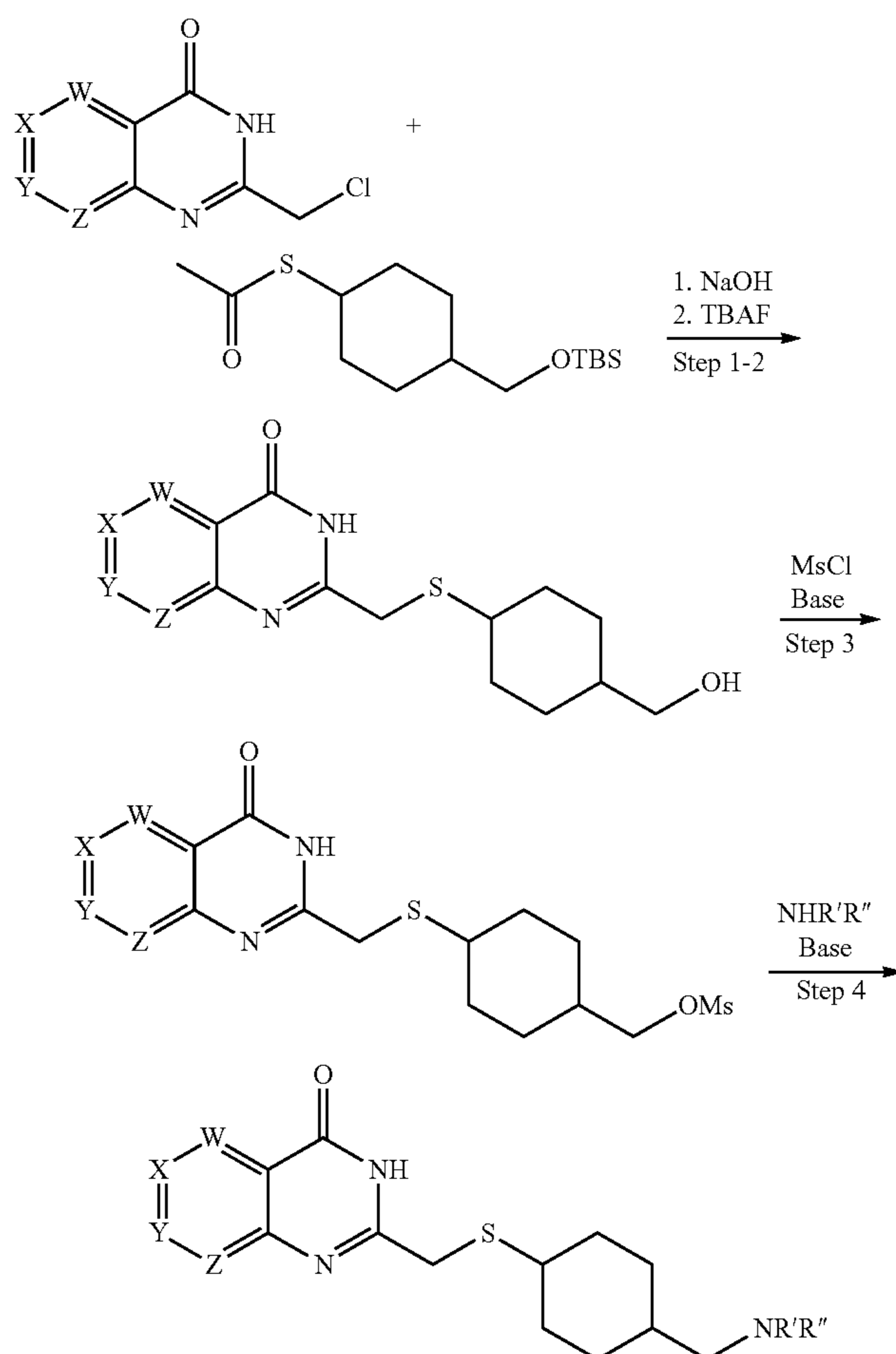
Scheme 14
