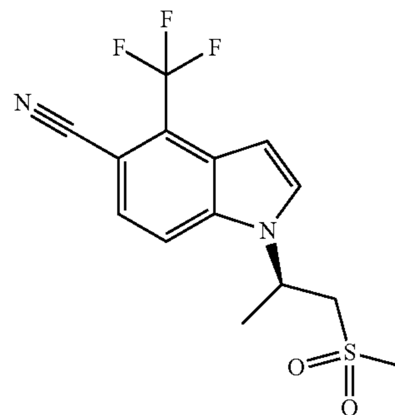
G. (R)-1-(1-(methylsulfonyl)propan-2-yl)-4-(trifluoromethyl)-1H-indole-5-carbonitrile
