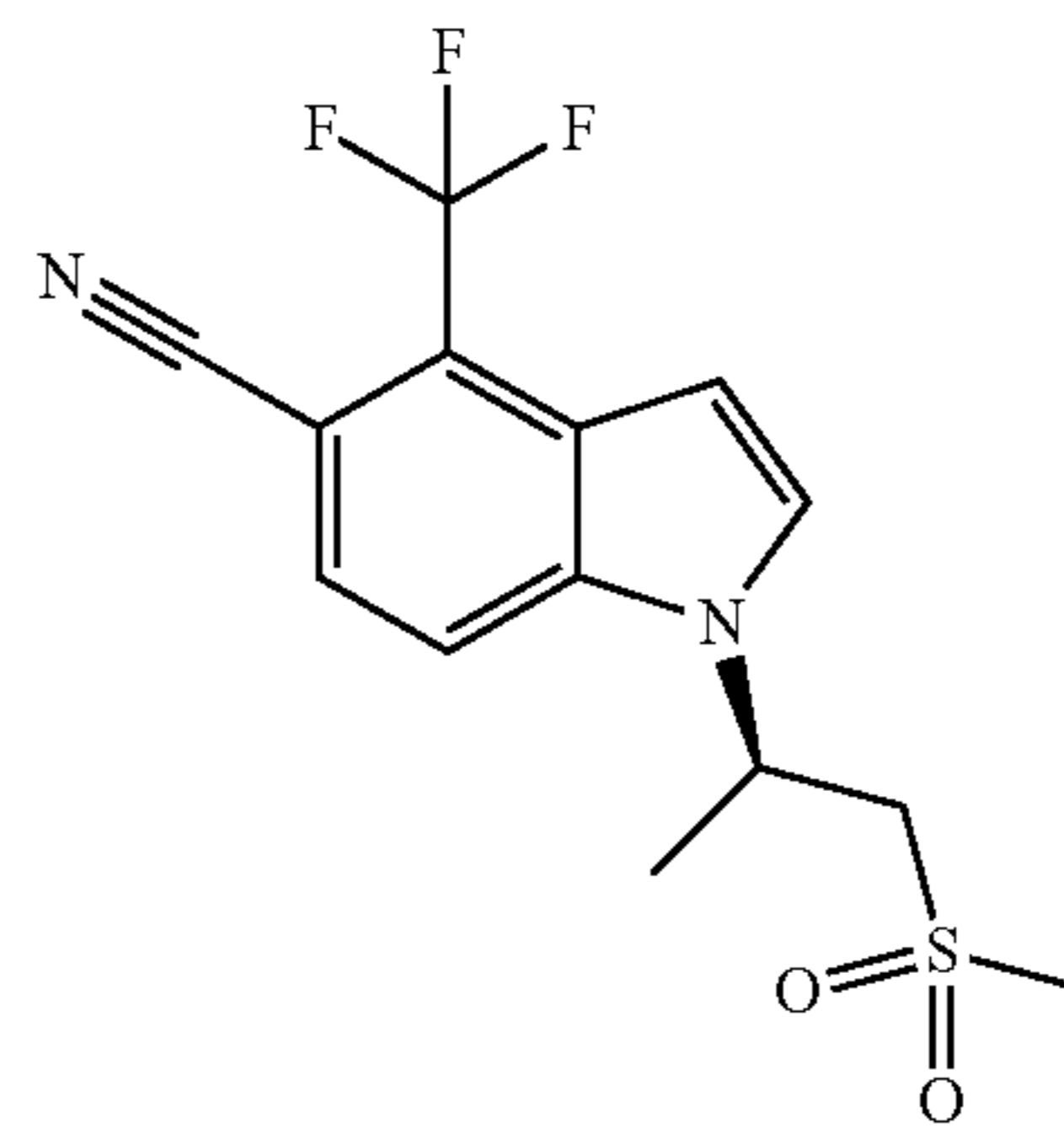
G. (R)-1-(1-(methylsulfonyl)propan-2-yl)-4-(trifluoromethyl)-1H-indole-5-carbonitrile
