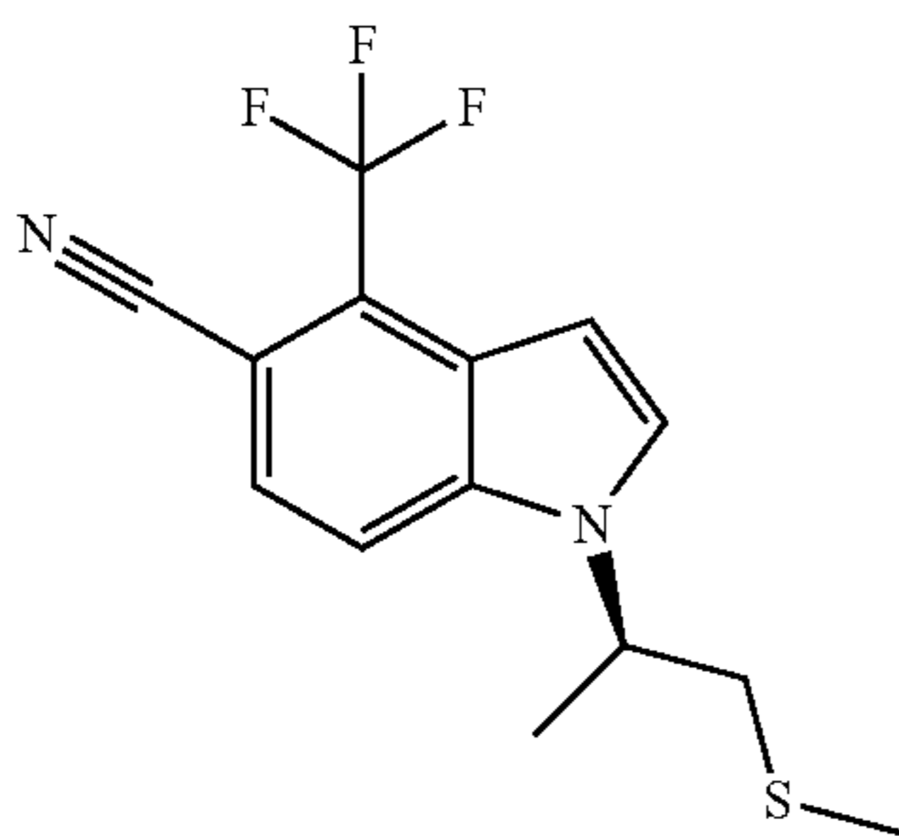
F. (R)-1-(1-(methylthio)propan-2-yl)-4-(trifluoromethyl)-1H-indole-5-carbonitrile
