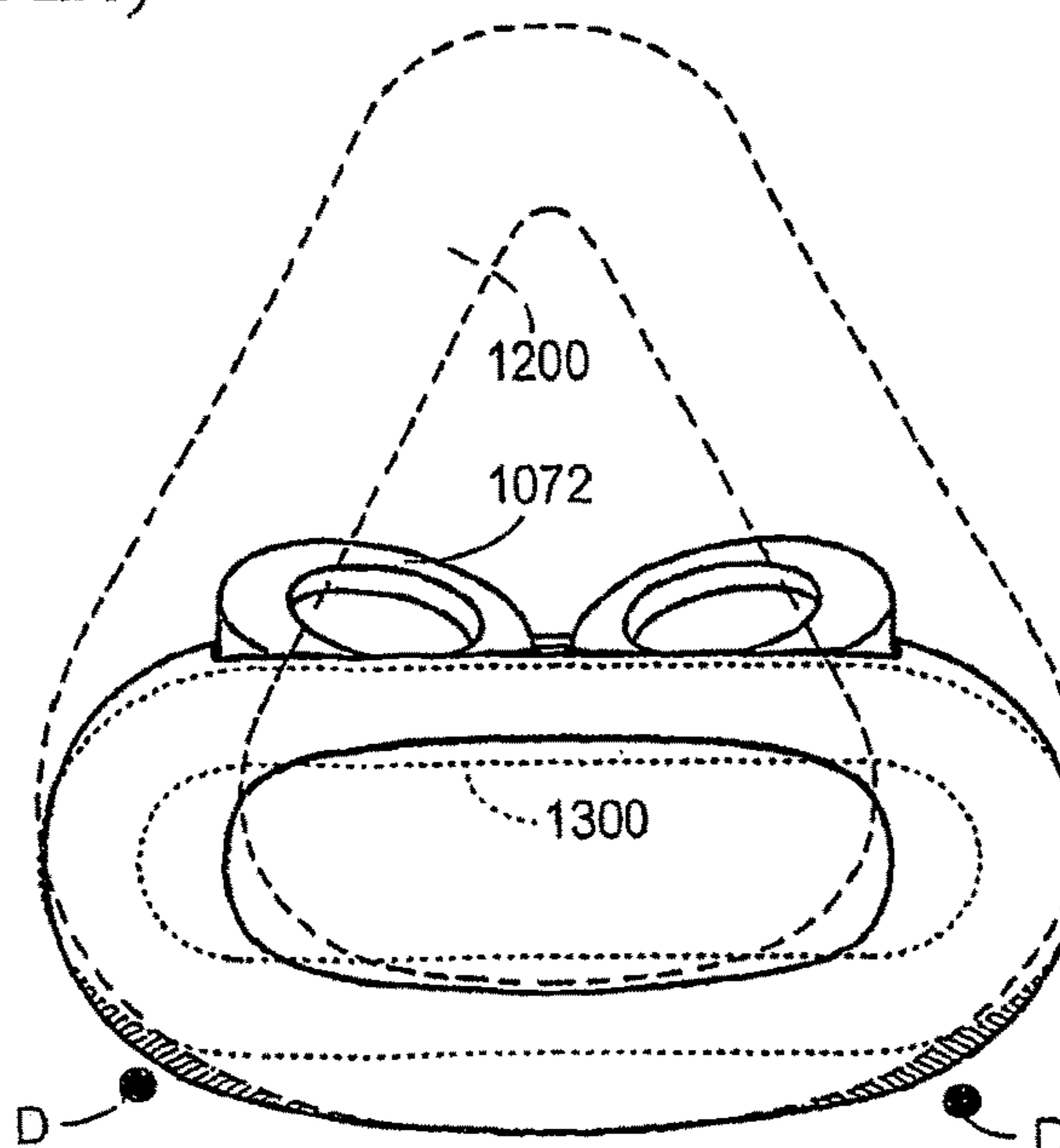
Fig. 92 (Prior Art)
