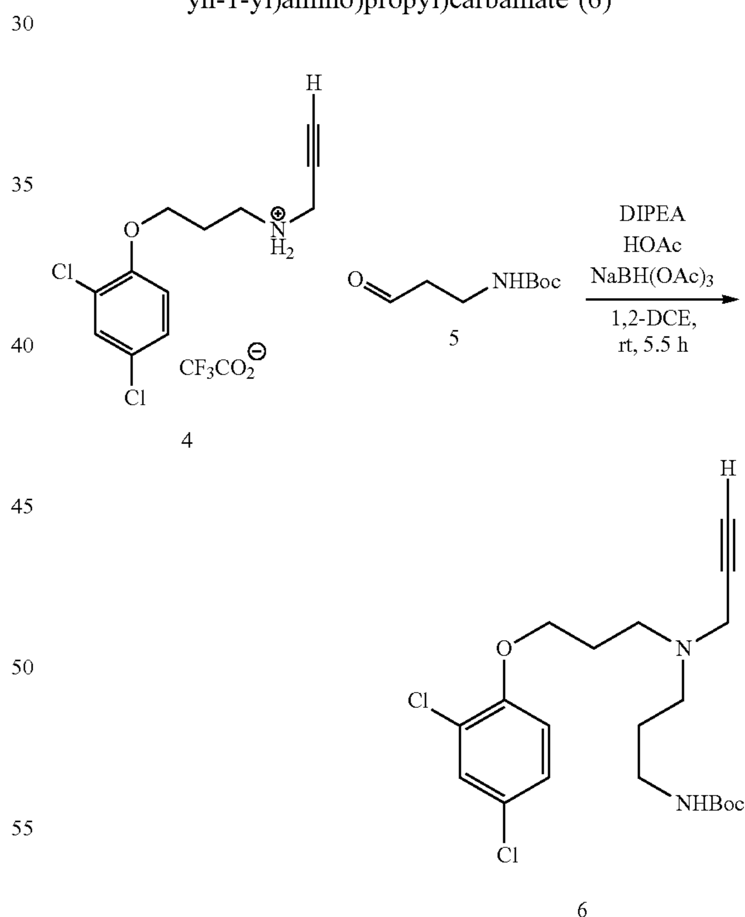
t-Butyl (3-((3-(2,4-dichlorophenoxy)propyl)(prop-2-yn-1-yl)amino)propyl)carbamate (6)
