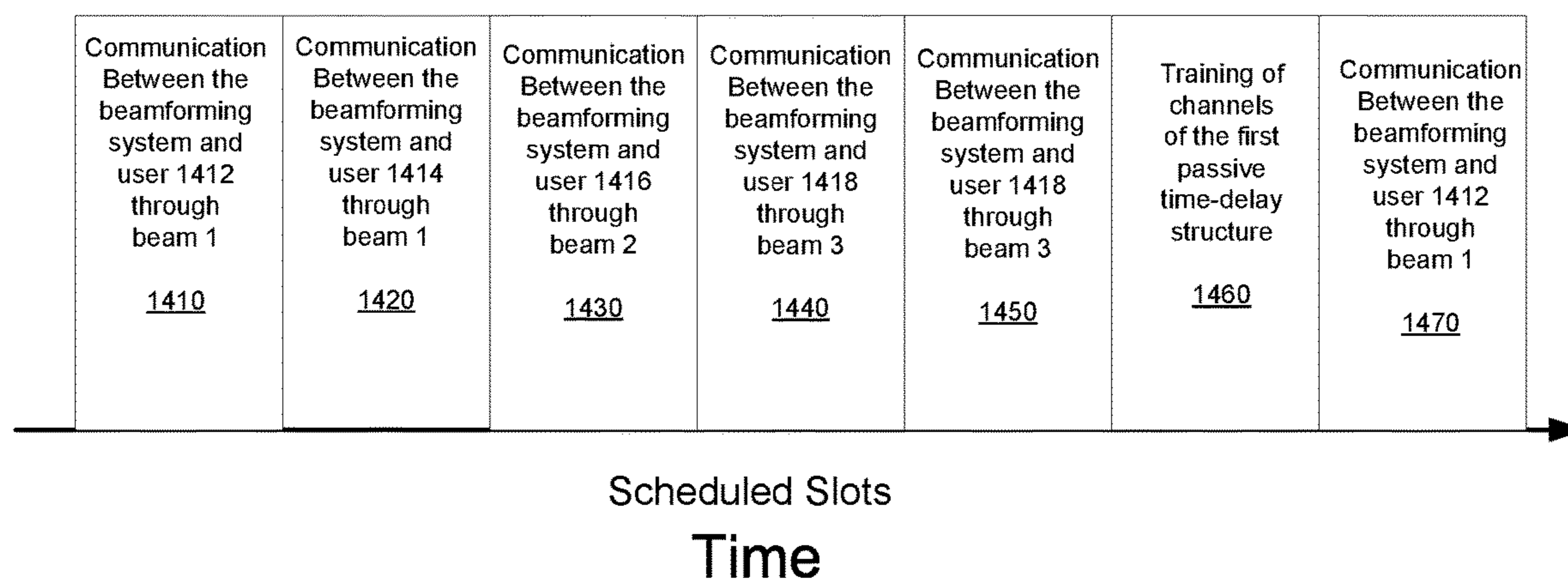
Example of Scheduled Communication of the Beamforming System
