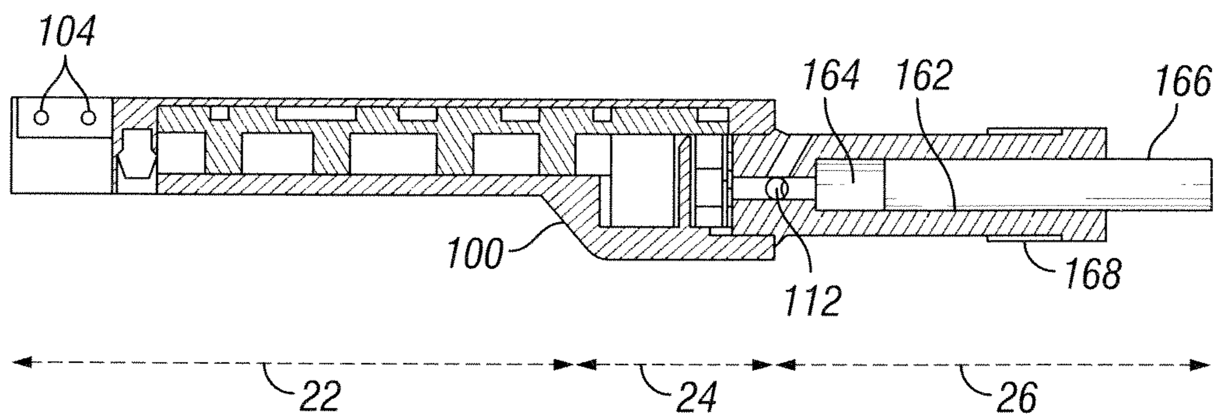
FIG. 2 (Prior Art)
