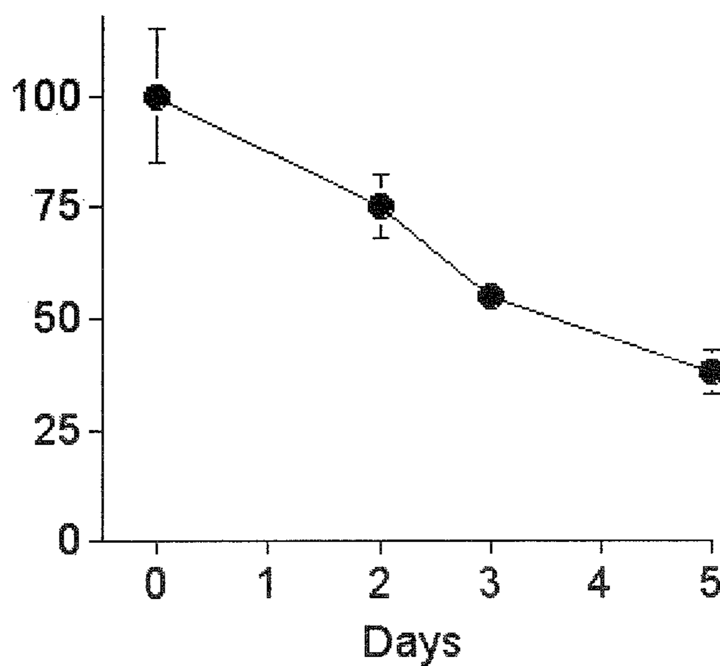
Zr-89 retention (%)
