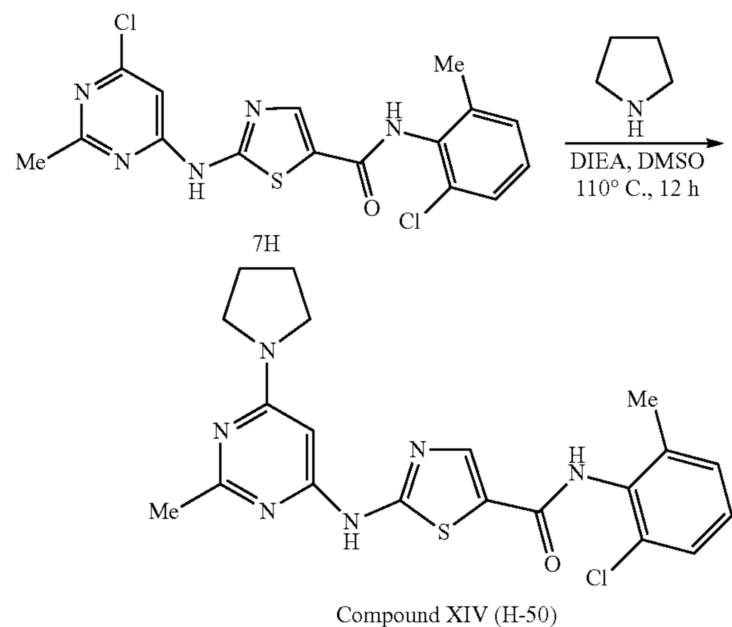
Scheme 14 Synthetic route for Compound XIV
