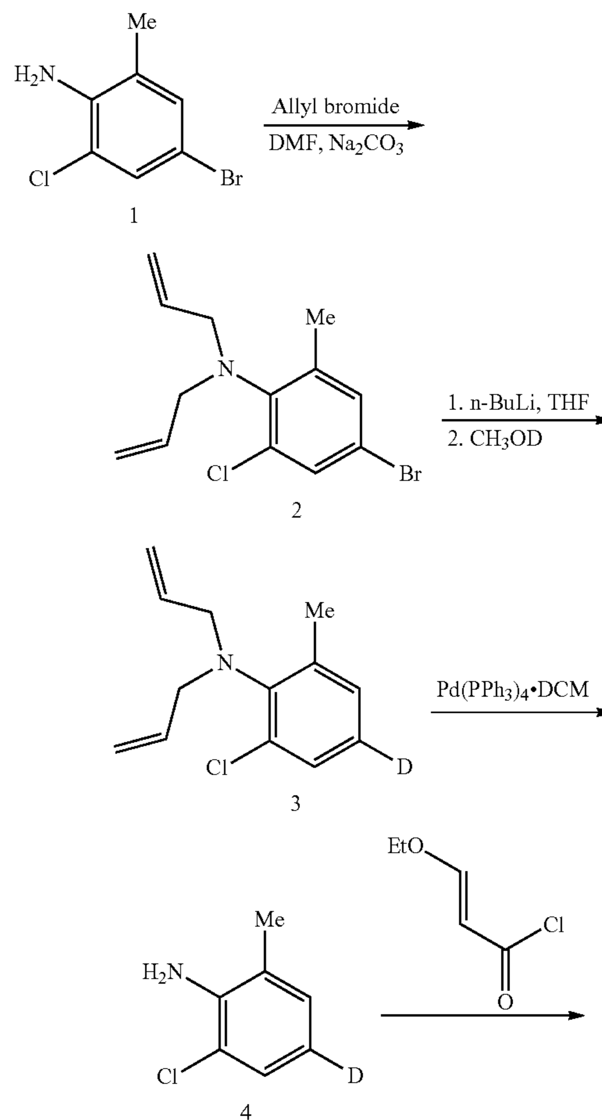
Scheme 1 Synthesis of Compound I
