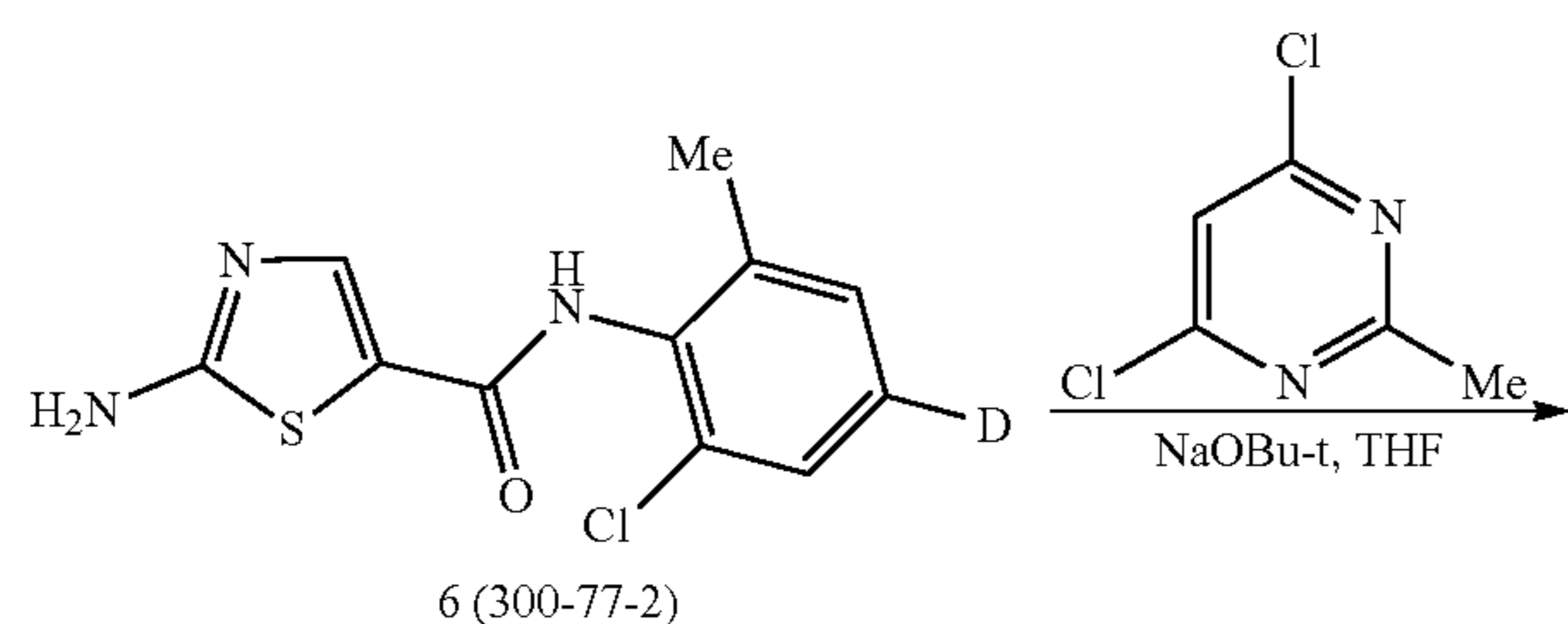
Scheme 7 Synthetic route for Compound VII
