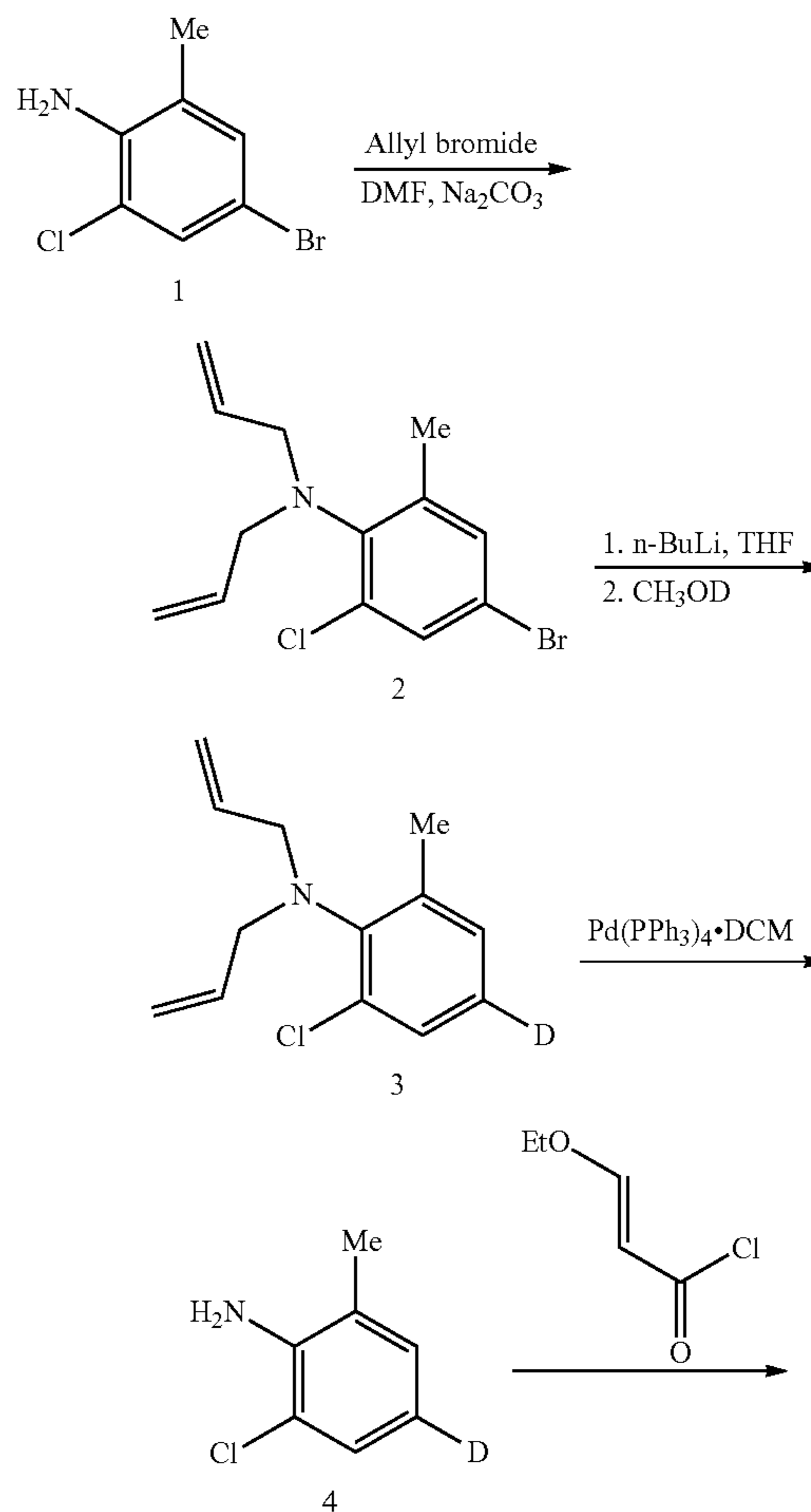
Scheme 1 Synthesis of Compound I
