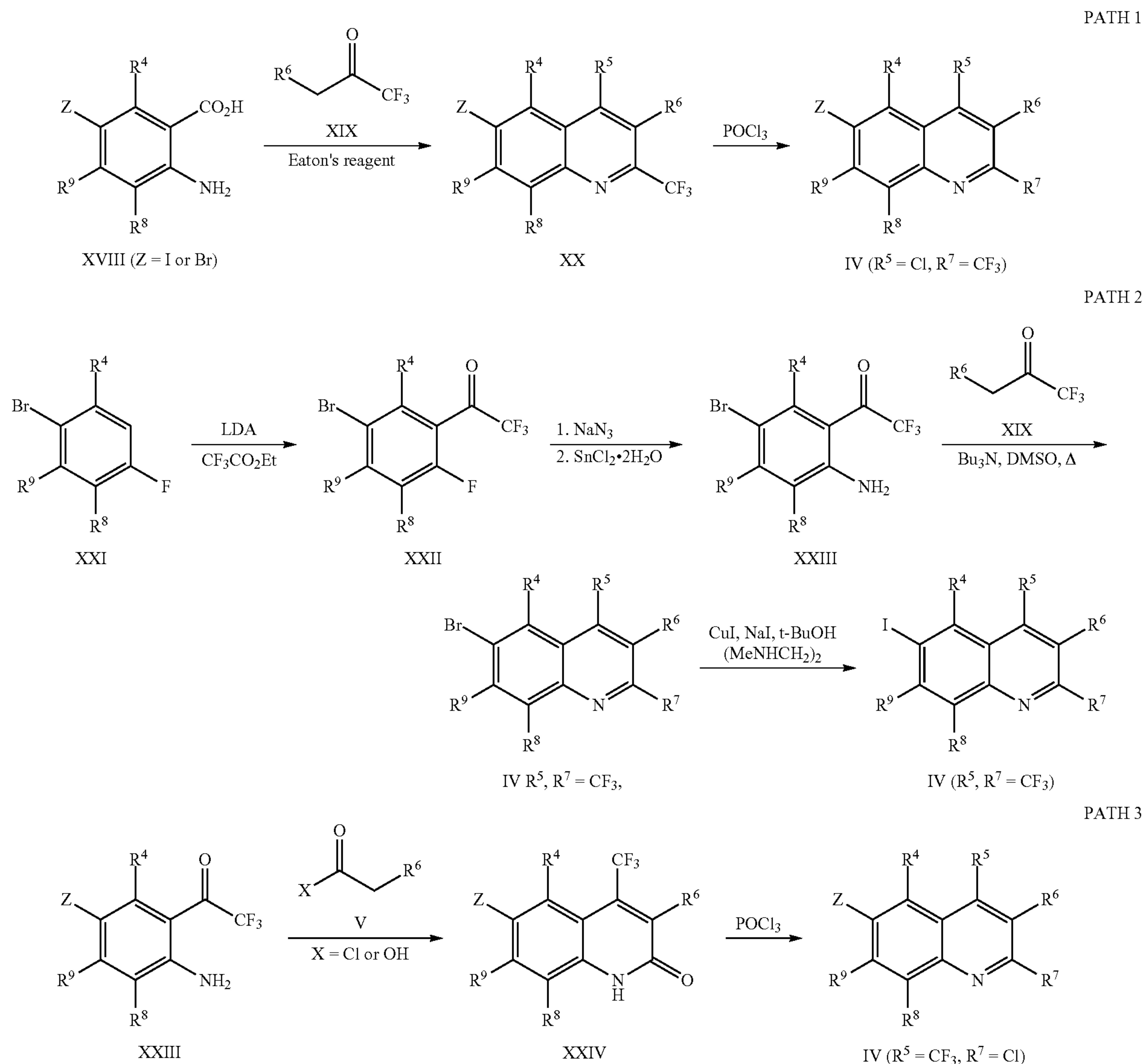
Scheme 3
