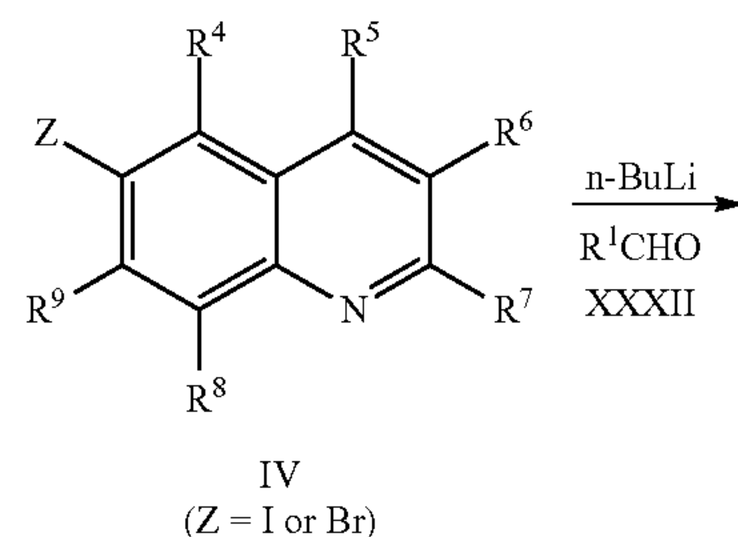
Scheme 7
