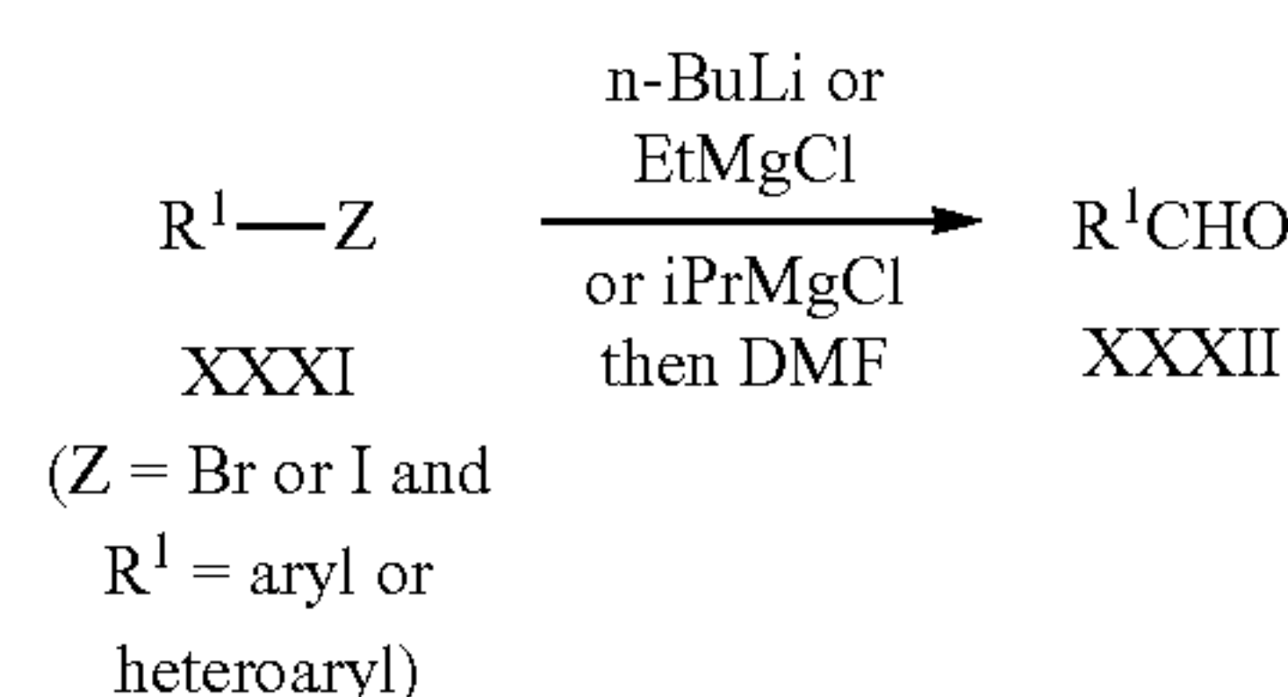
Scheme 6
