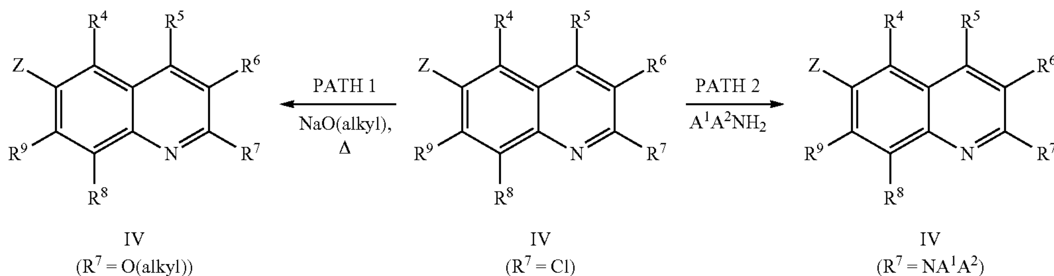
SCHEME 5
