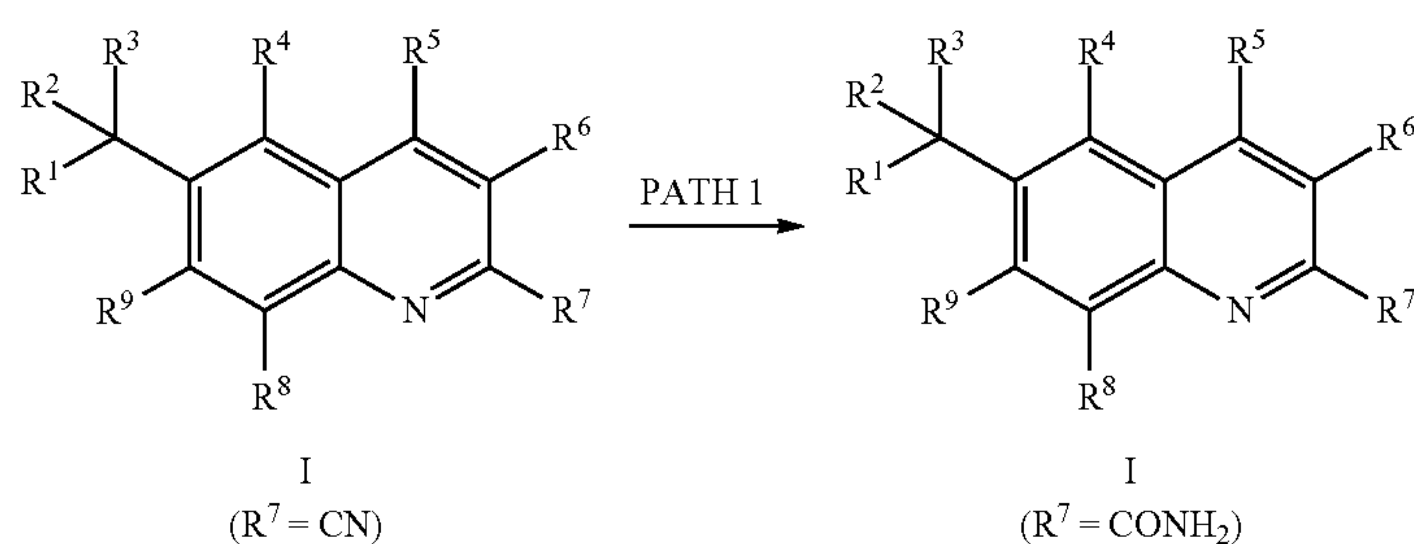
Scheme 17
