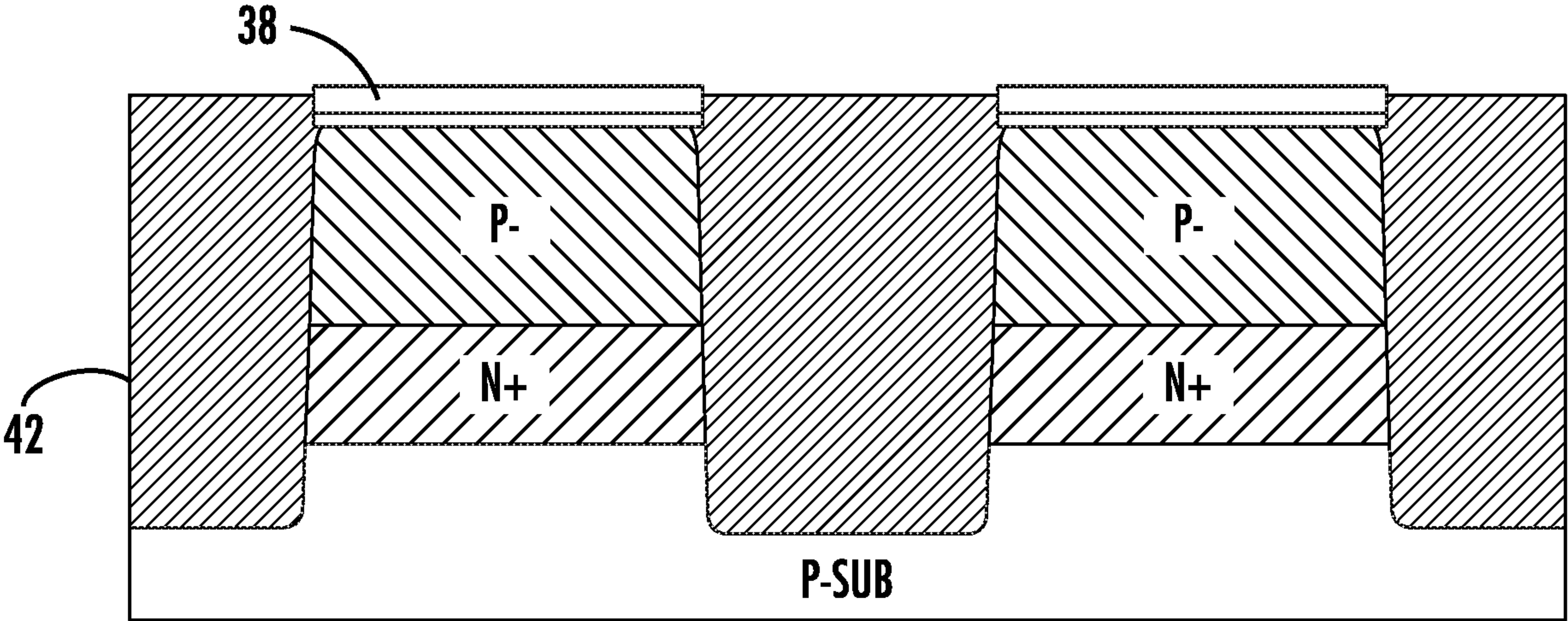
FIG. 6A (A~A')
