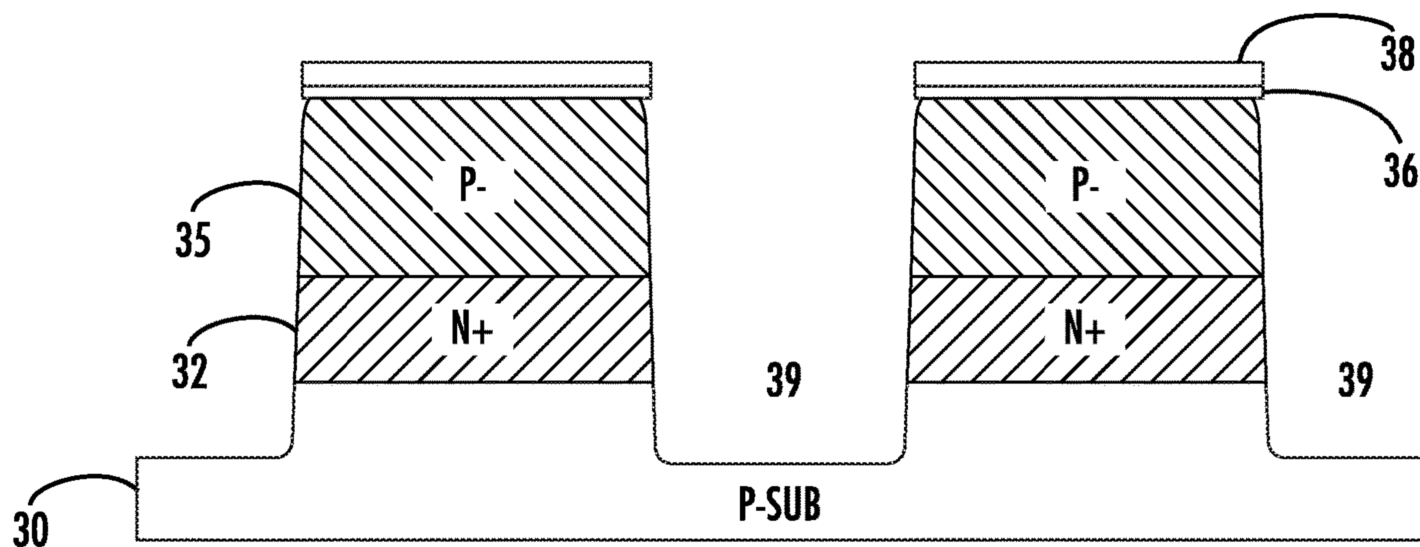
FIG. 5A (A~A')
