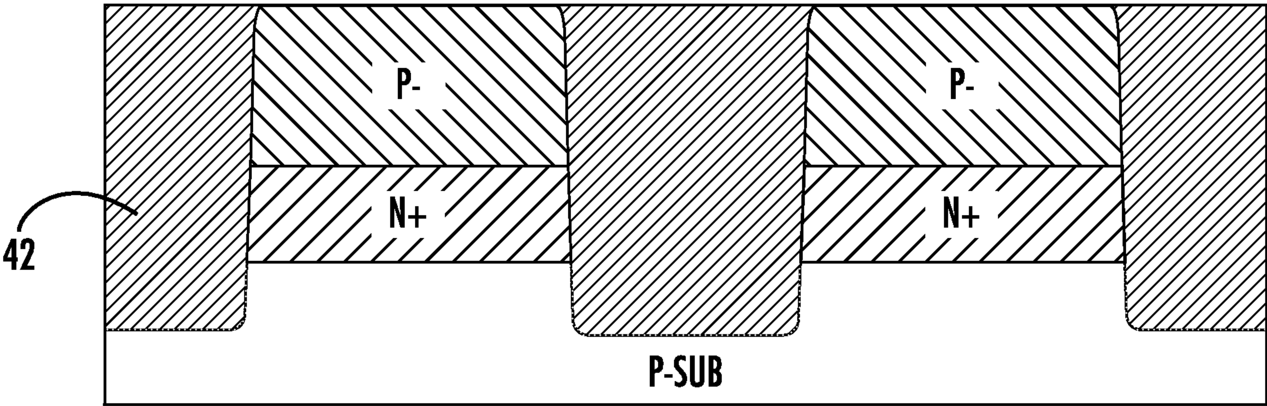
FIG. 7A (A~A')
