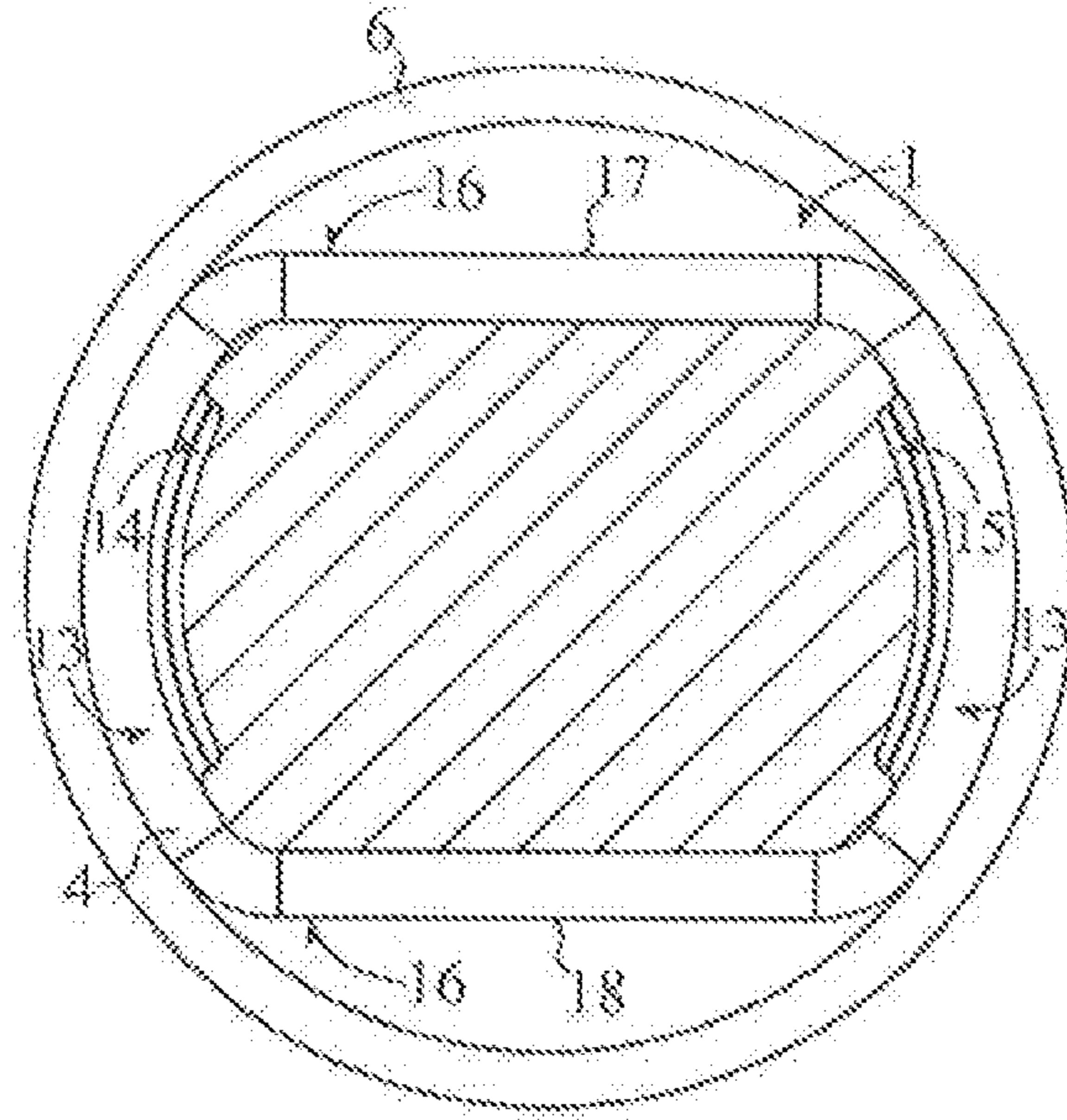
SECTION C-C
