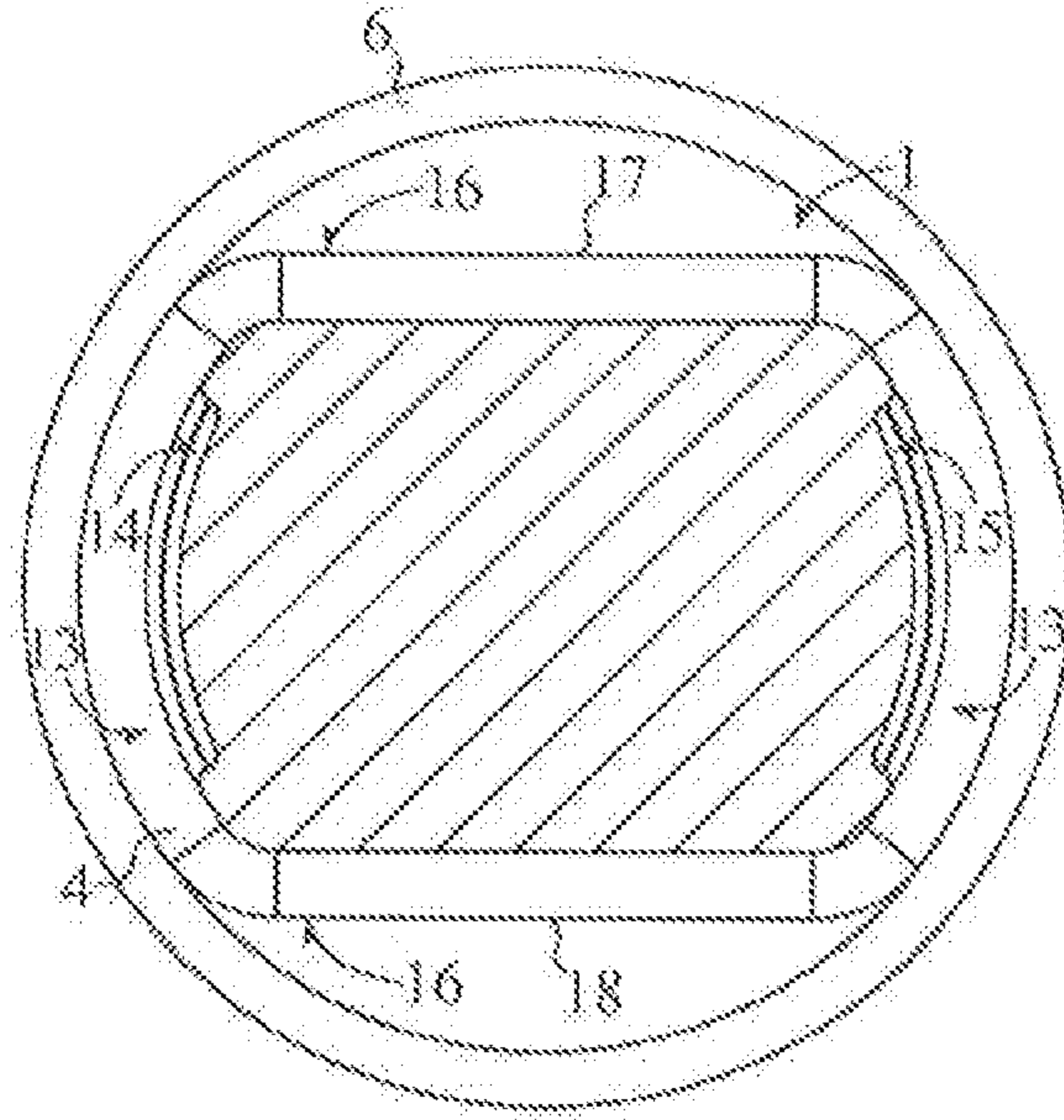
SECTION C-C
