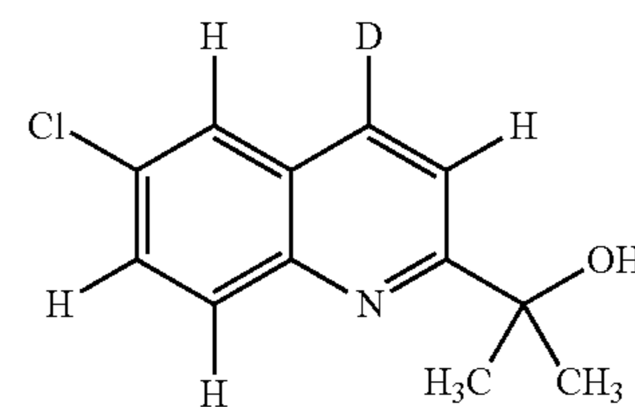
2-(6-chloroquinolin-2-yl-4-d)propan-2-ol
