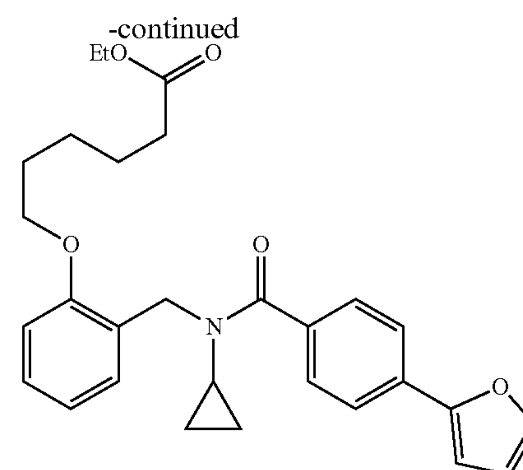
Reaction Step 4—Suzuki Coupling
