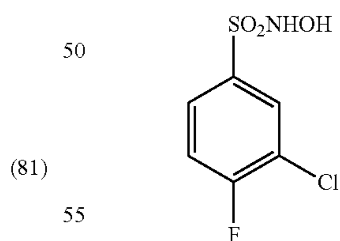
3-Chloro-4-fluoro-N-hydroxybenzene-1-sulfonamide
