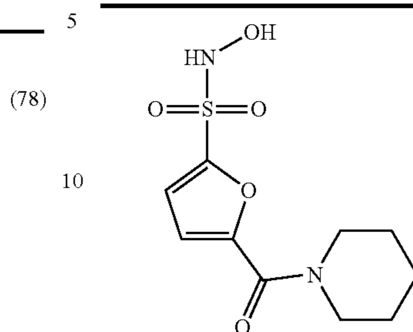
N-Hydroxy-5-(piperidine-1-carbonyl)furan-2-sulfonamide
