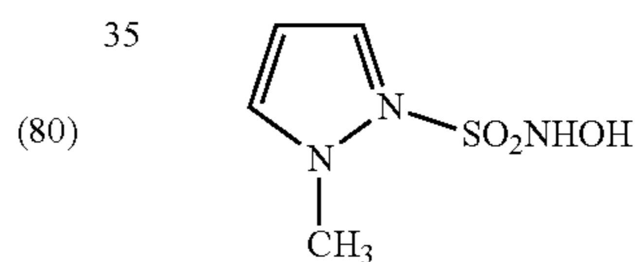
N-Hydroxy-1-methyl-1H-pyrazole-3-sulfonamide
