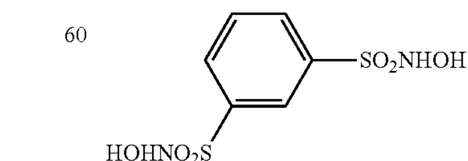
1-N,3-N-Dihydroxybenzene-1,3-disulfonamide
