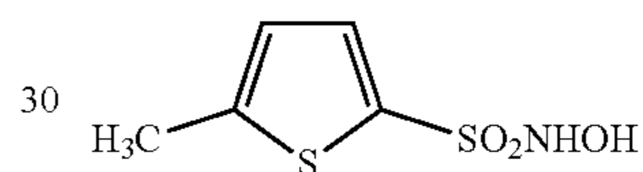
N-Hydroxy-5-methylthiophene-2-sulfonamide
