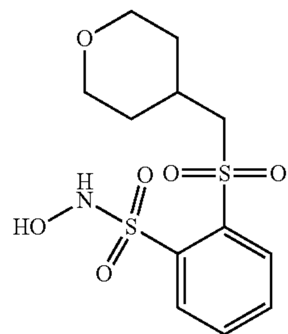
N-Hydroxy-2-(oxan-4-ylmethanesulfonyl)benzene-1-sulfonamide
