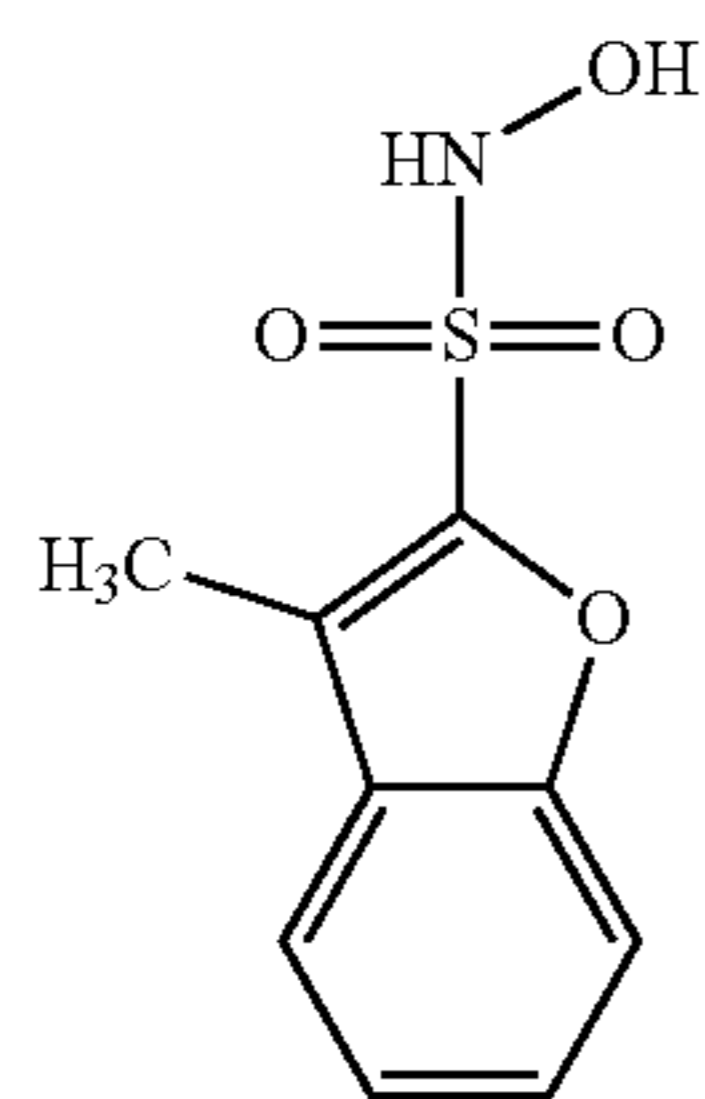
N-Hydroxy-3-methyl-1-benzofuran-2-sulfonamide
