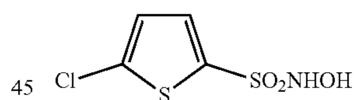
5-Chloro-N-hydroxythiophene-2-sulfonamide
