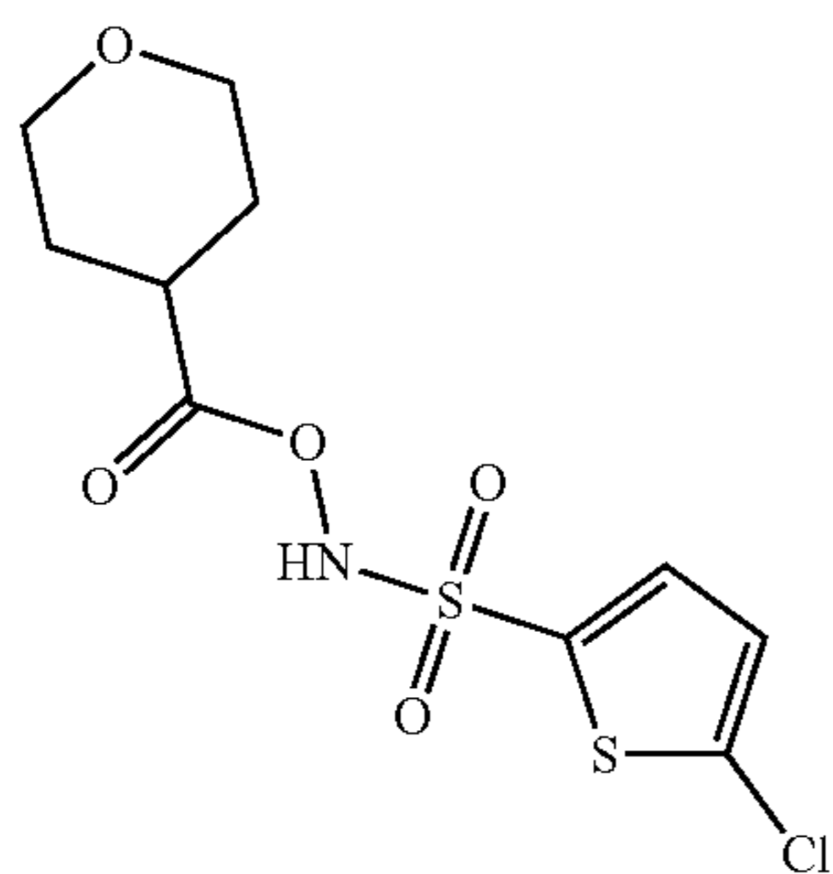
5-Chlorothiophene-2-sulfonamidooxane-4-carboxylate
