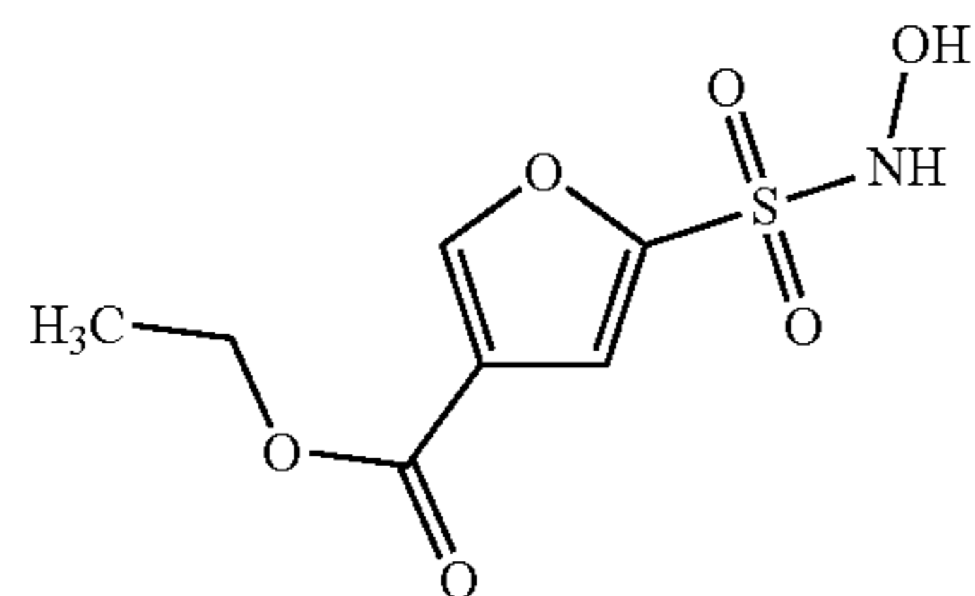
Ethyl 5-(hydroxysulfamoyl)furan-3-carboxylate
