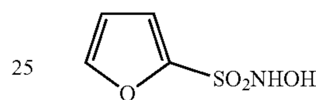
N-Hydroxyfuran-2-sulfonamide
