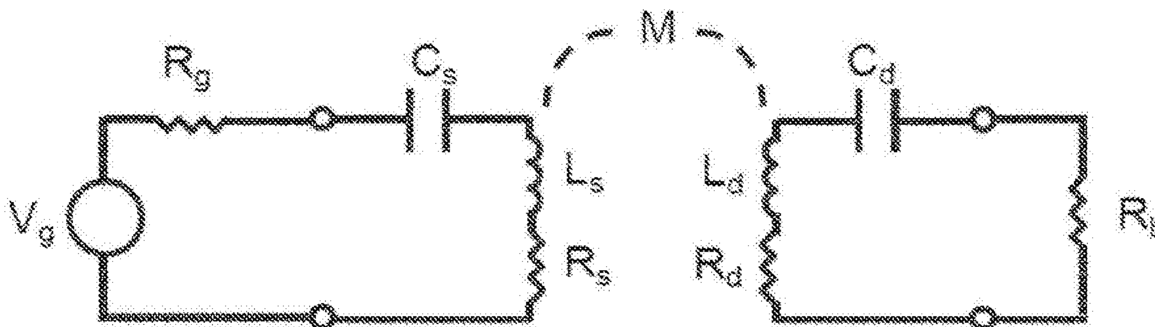
Figure 11: Equivalent circuit for the coupled resonator system.
