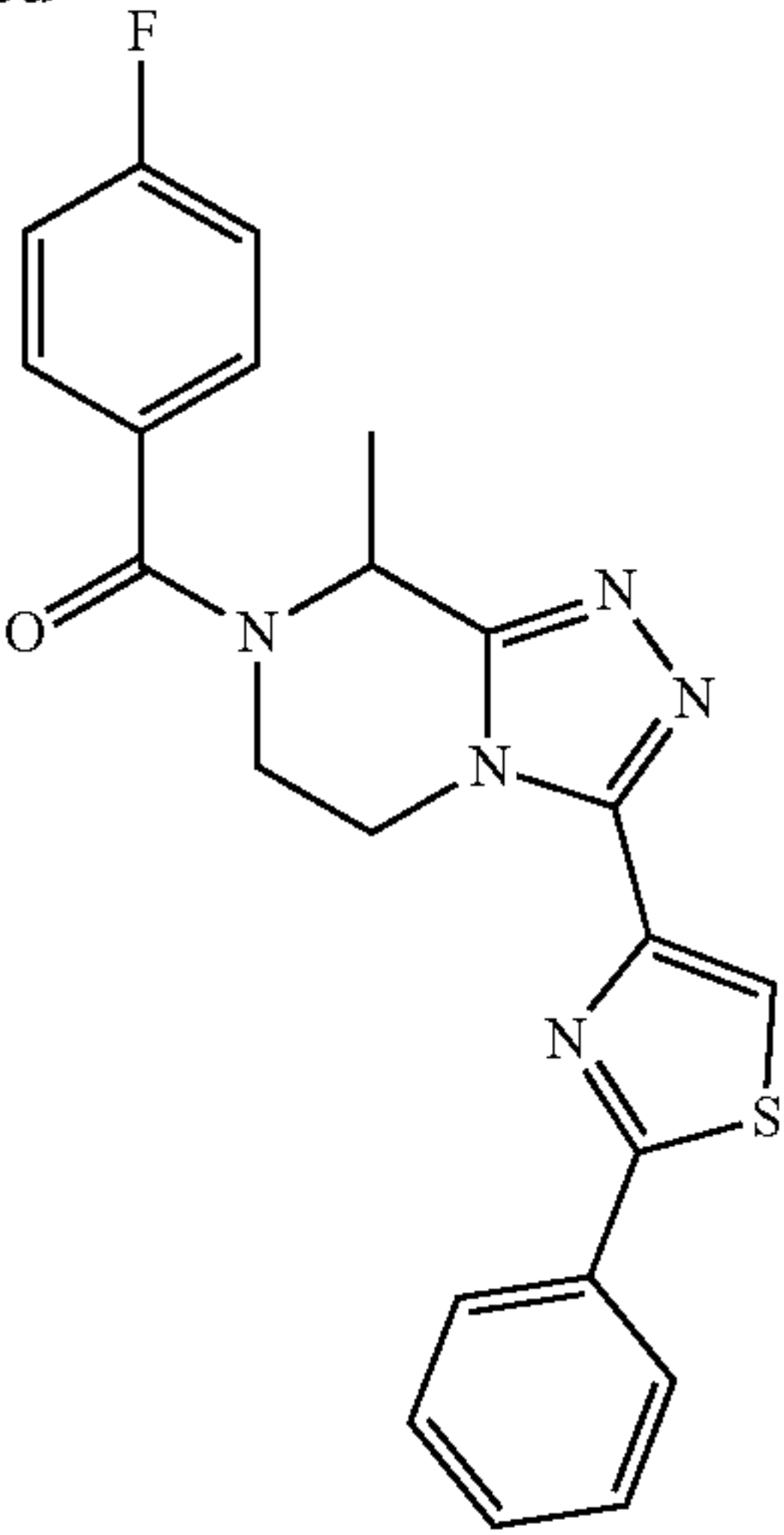
compound n° 166
