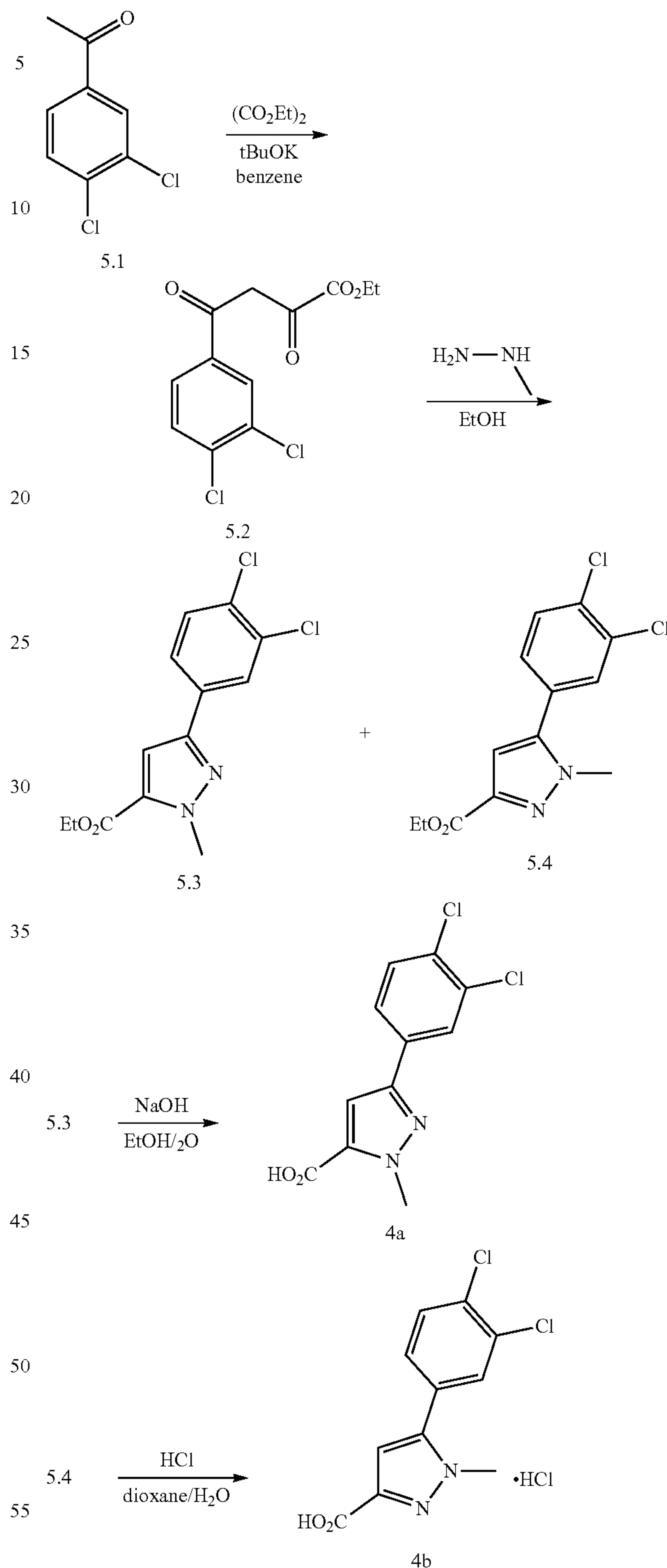
Scheme 5: Synthesis of intermediates 4a and 4b
