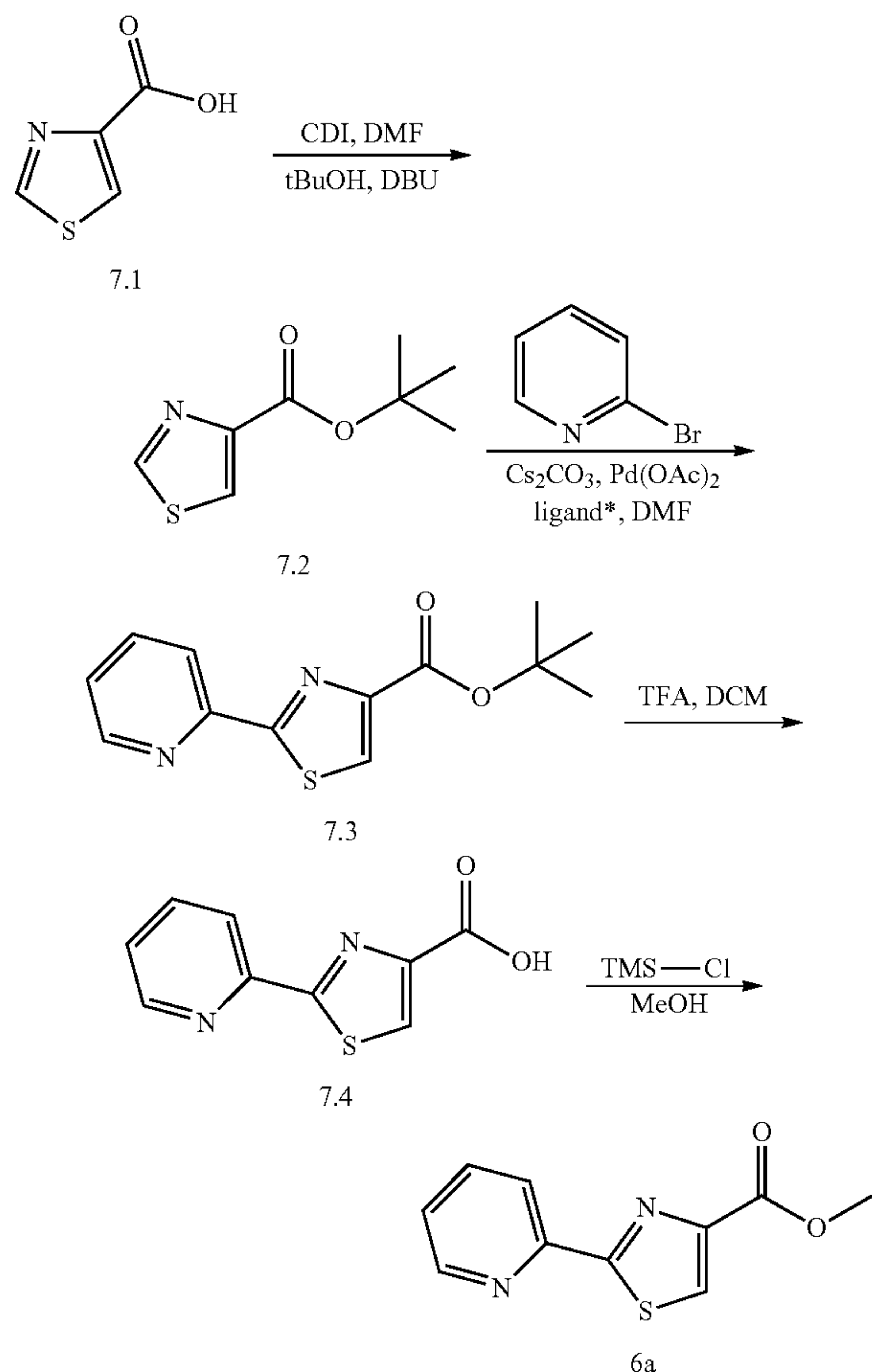
Scheme 7: Synthesis of intermediate 6a
