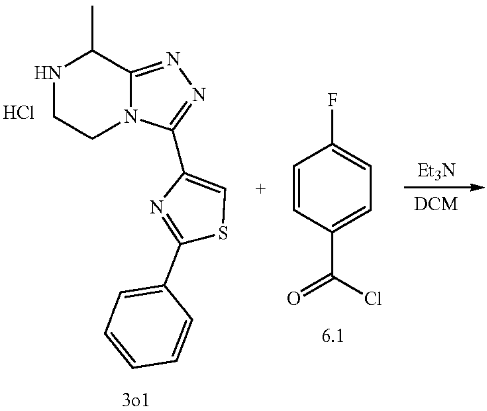
Scheme 13: synthesis of (4-fluorophenyl)(8-methyl-3-(2-phenylthiazol-4-yl)-5,6-dihydro [1,2,4]triazolo[4.3-a]pyrazin-7(8H)-yl)methanone (compound n° 166).
