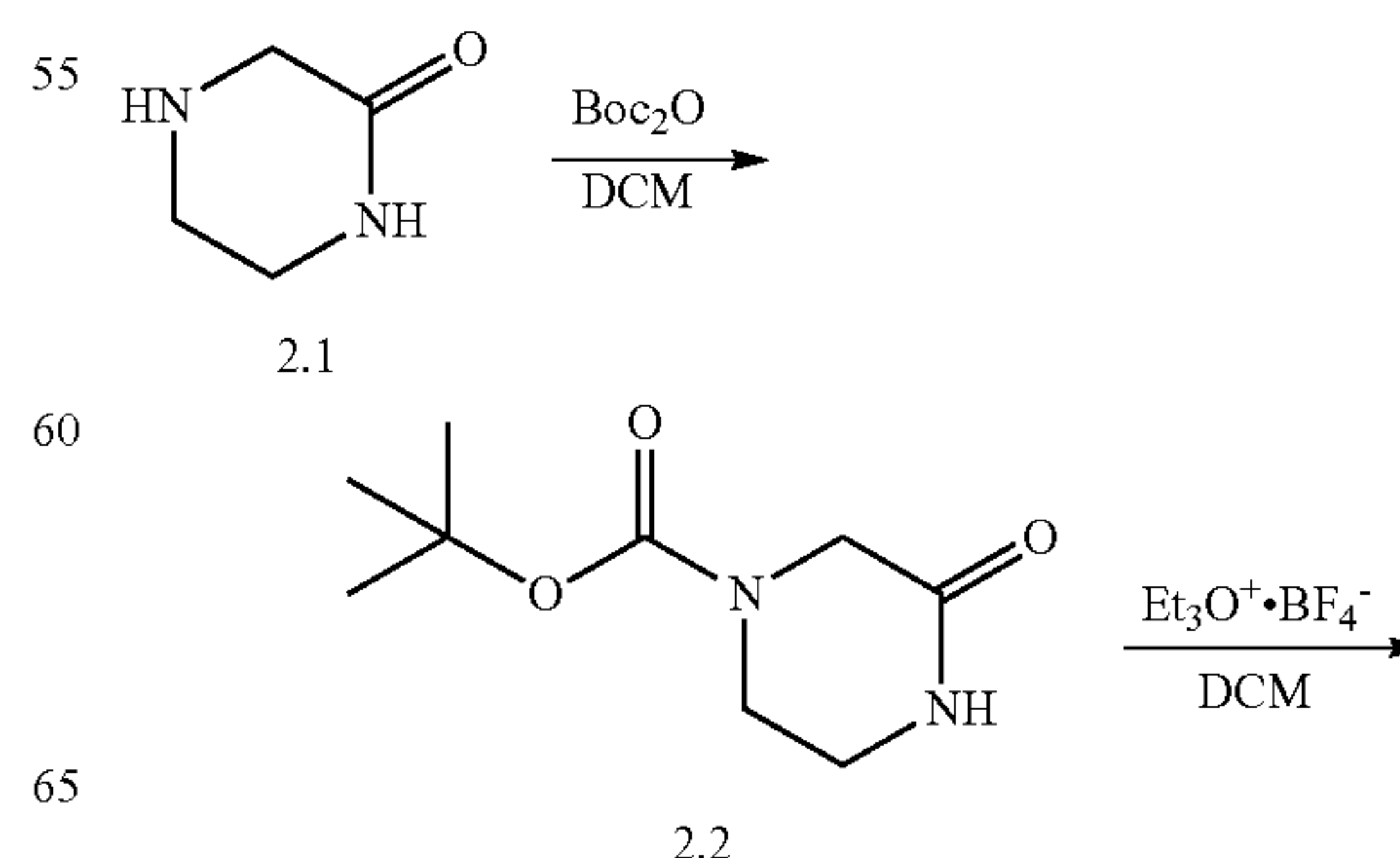
Scheme 2: Synthesis of tert-butyl 3-ethoxy-5,6-dihydropyrazine-1(2H)-carboxylate
