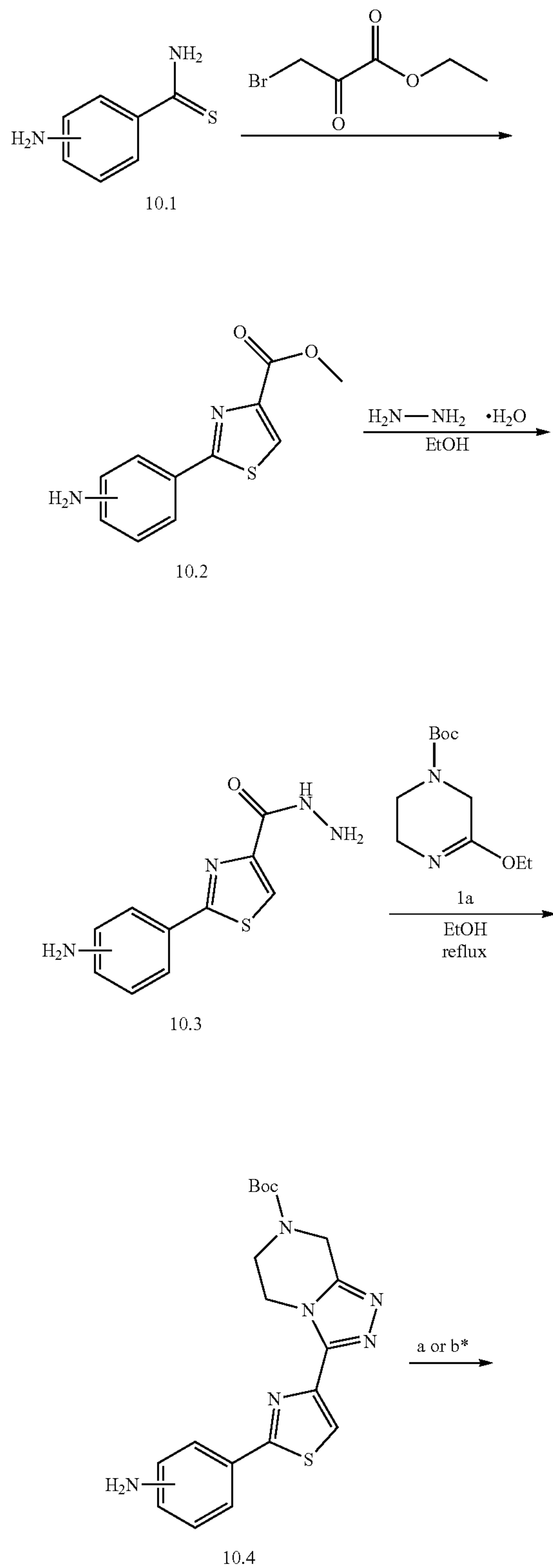
Scheme 10: Synthesis of compounds n° 283, 289, 290, 291, 292
