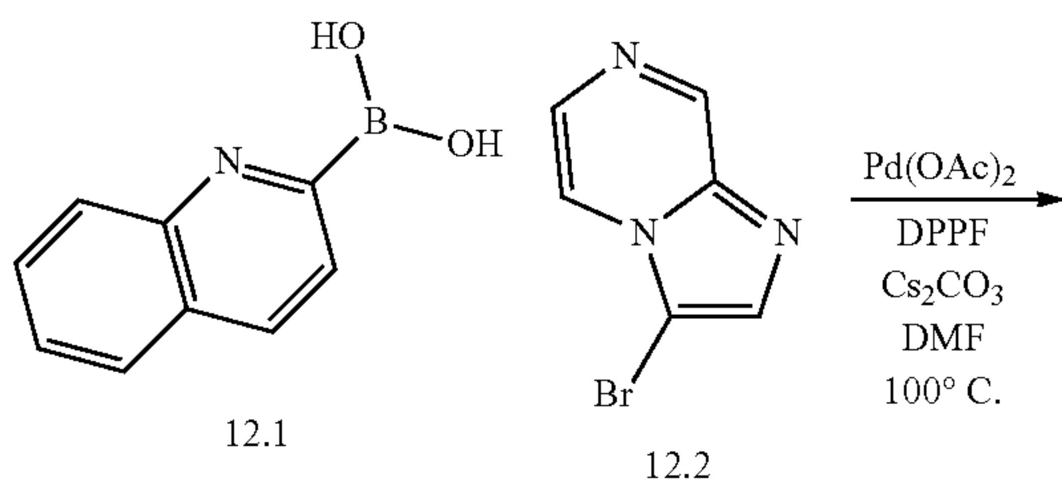
Scheme 11: Synthesis of compound n° 293
