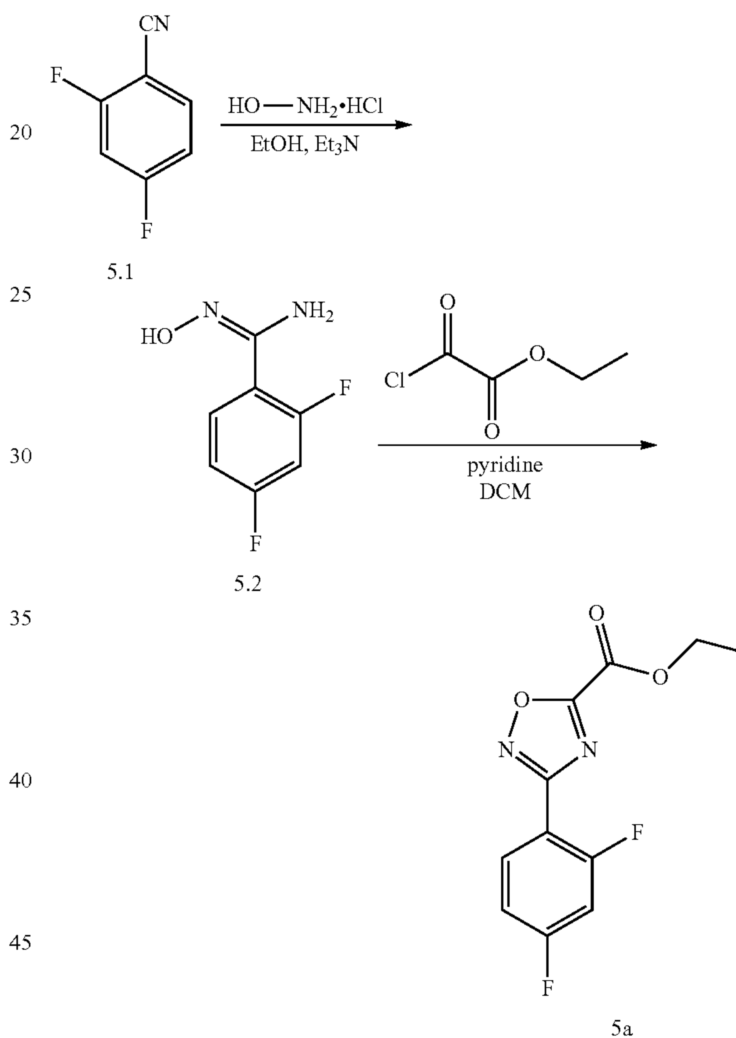
Scheme 6: synthesis of intermediate 5a
