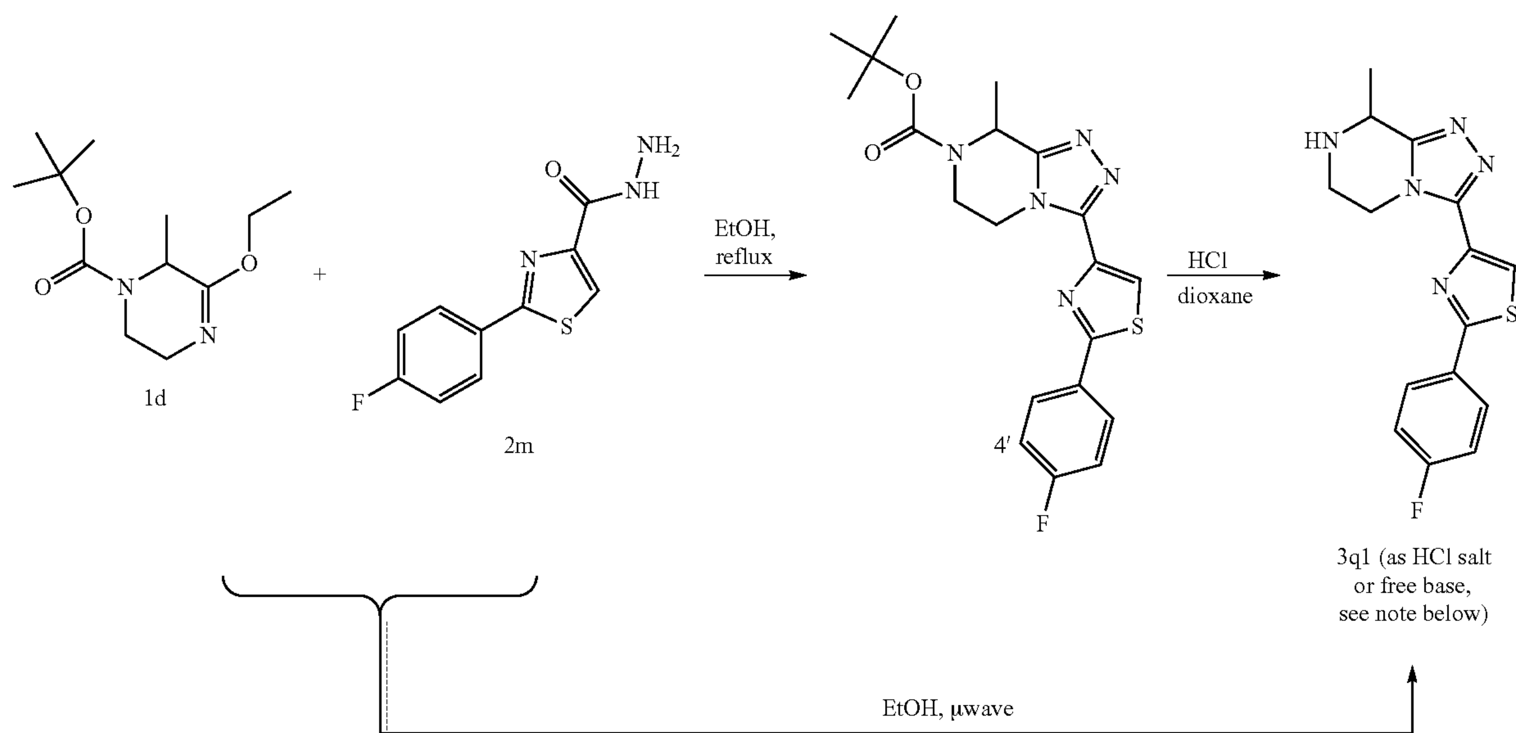
Scheme 4': Synthesis of 2-(4-fluorophenyl)-4-(8-methyl-5,6,7,8-tetrahydro-[1,2,4]triazolo[4,3-a]pyrazin-3-yl)thiazole
