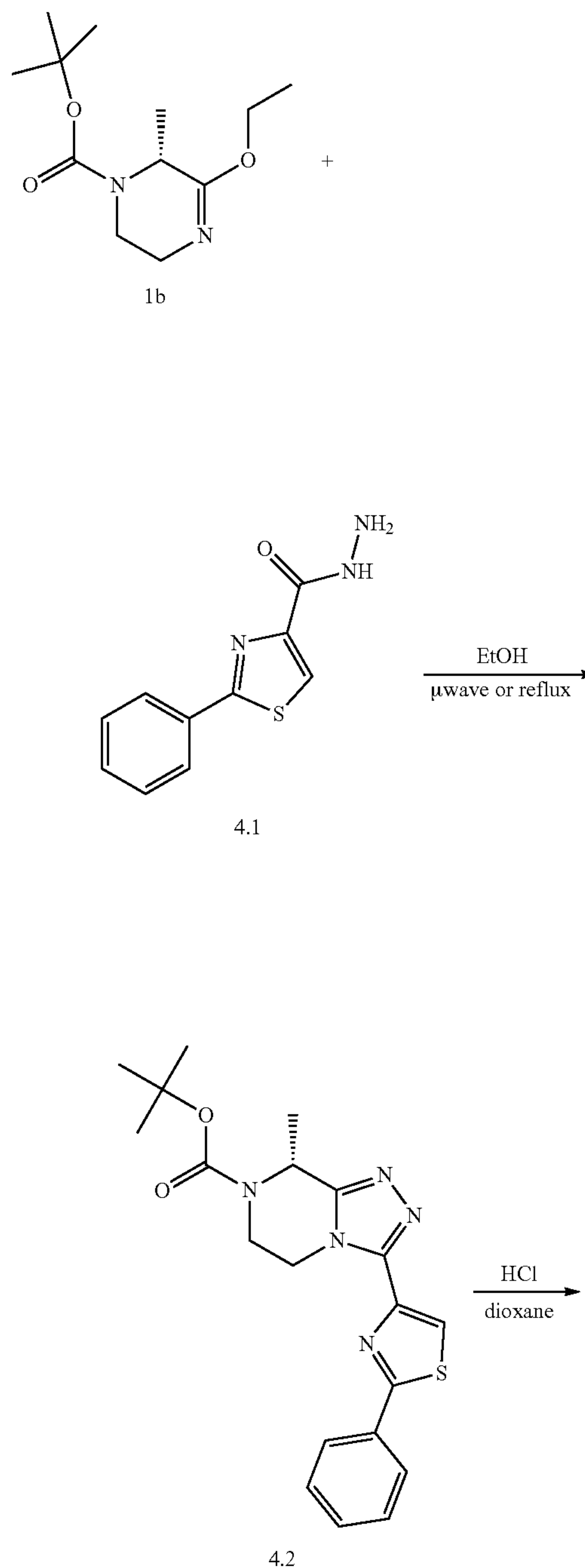
Scheme 4: Synthesis of (R)-4-(8-methyl-5,6,7,8-tetrahydro-[1,2,4]triazolo[4,3-a]pyrazin-3-yl)-2-phenylthiazole hydrochloride salt
