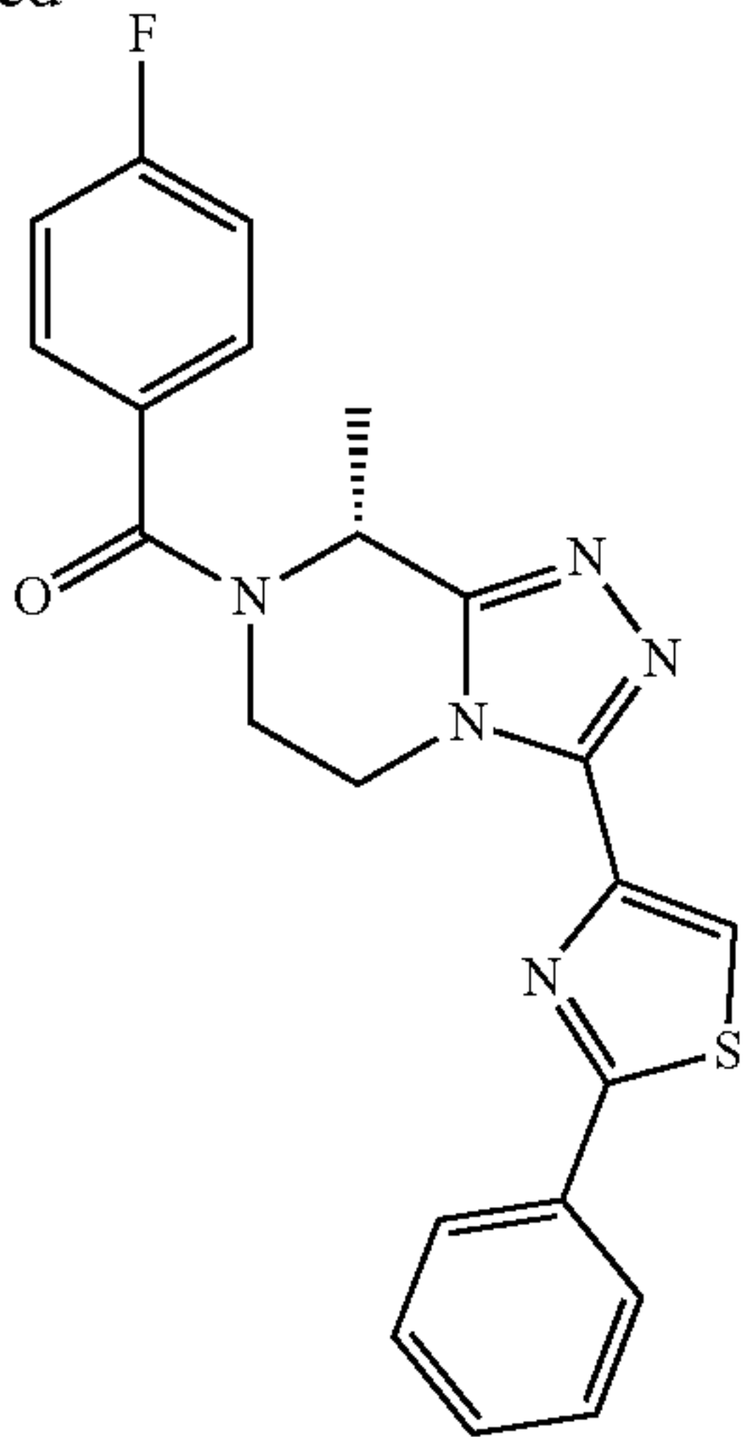
compound n° 45
