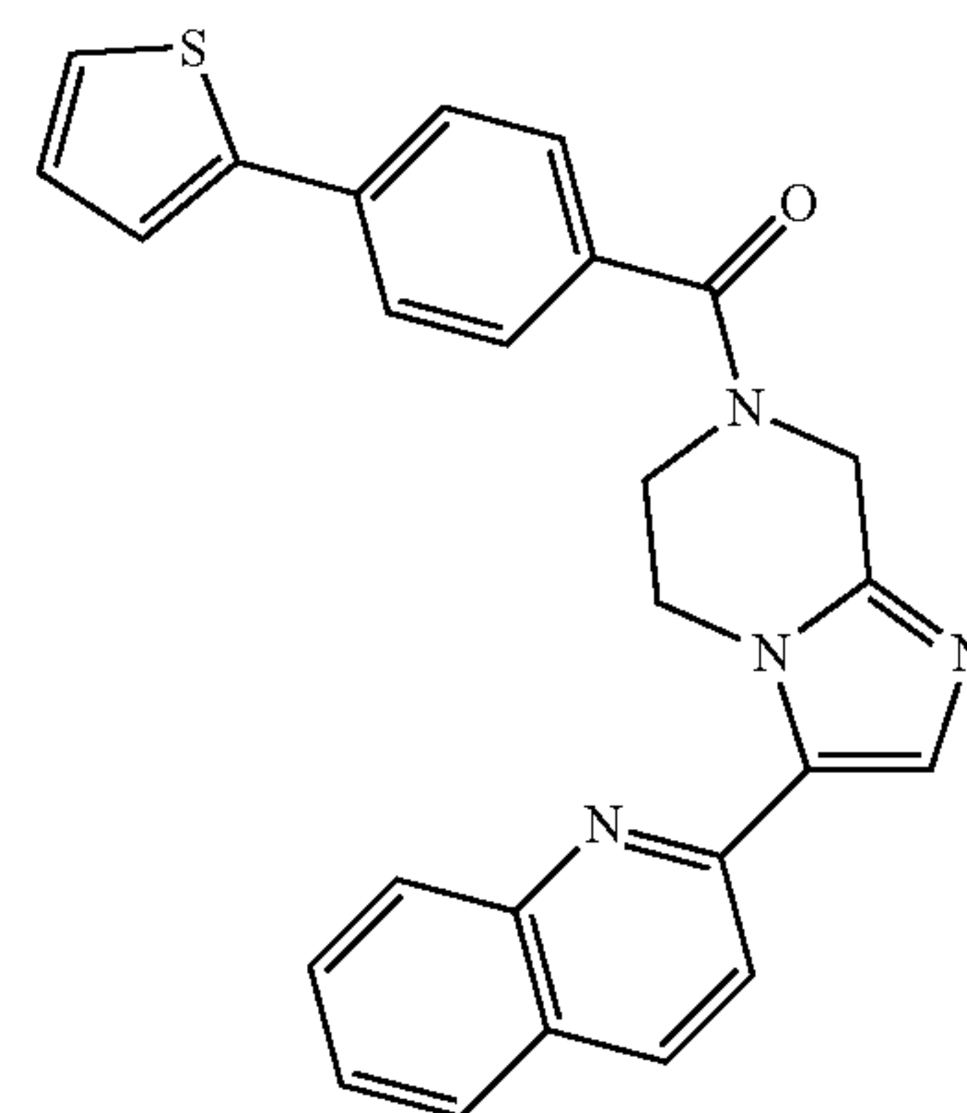
compound n° 293
