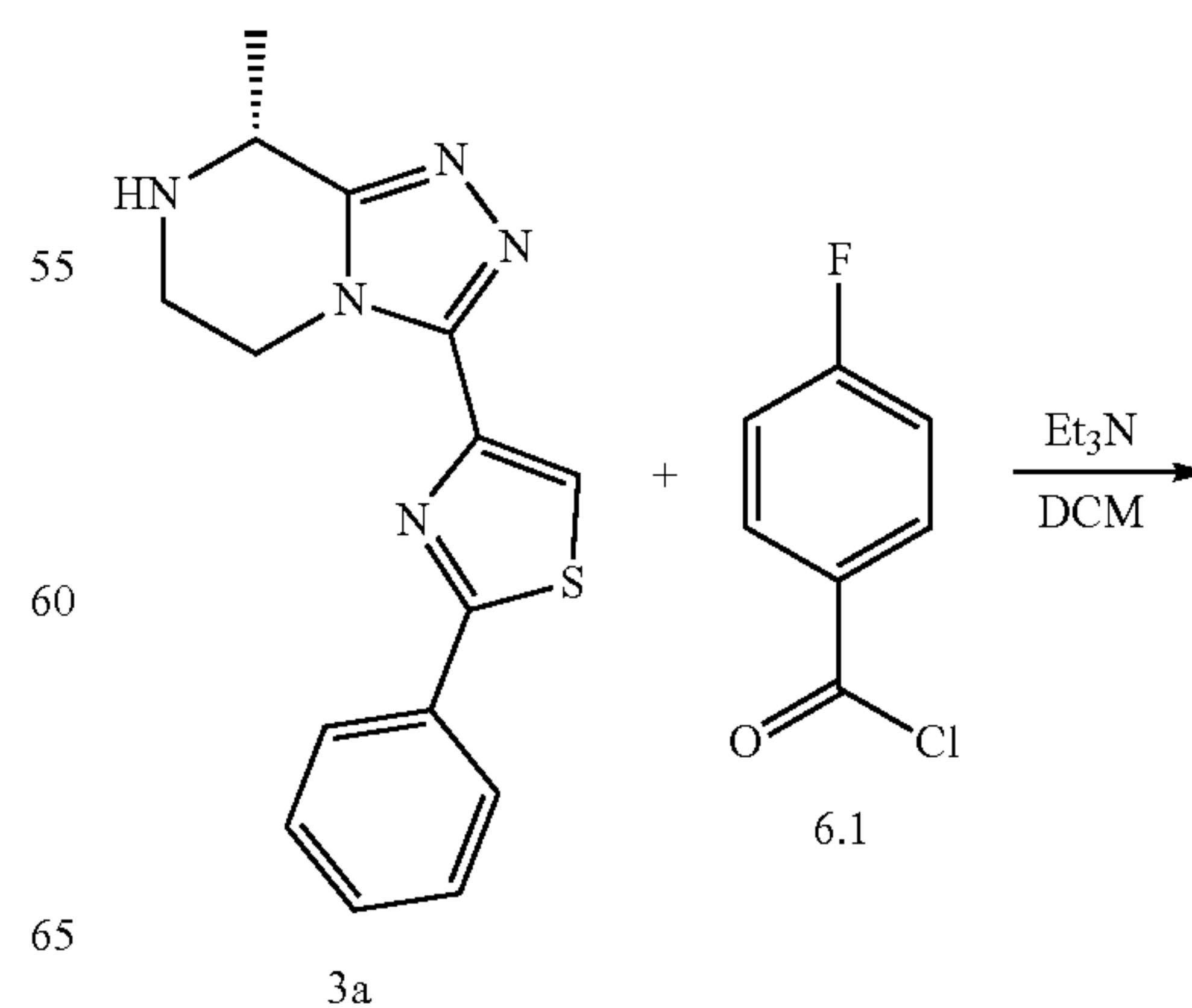
Scheme 12: synthesis of (R)-(4-fluorophenyl)(8-methyl-3-(2-phenylthiazol-4-yl)-5,6-dihydro [1,2,4]triazolo[4,3-a]pyrazin-7(8H)-yl)methanone (compound n° 45).
