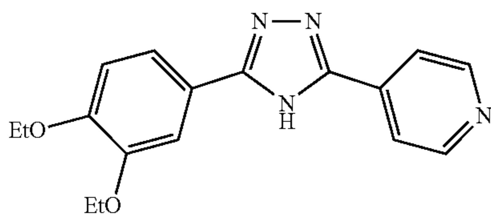
4-(5-(3,4-diethoxyphenyl)-4H-1,2,4-triazol-3-yl)pyridine
