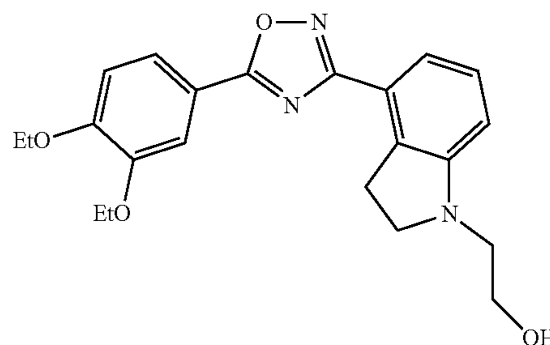
2-(4-(5-(3,4-diethoxyphenyl)-1,2,4-oxadiazol-3-yl)indolin-1-yl)ethanol
