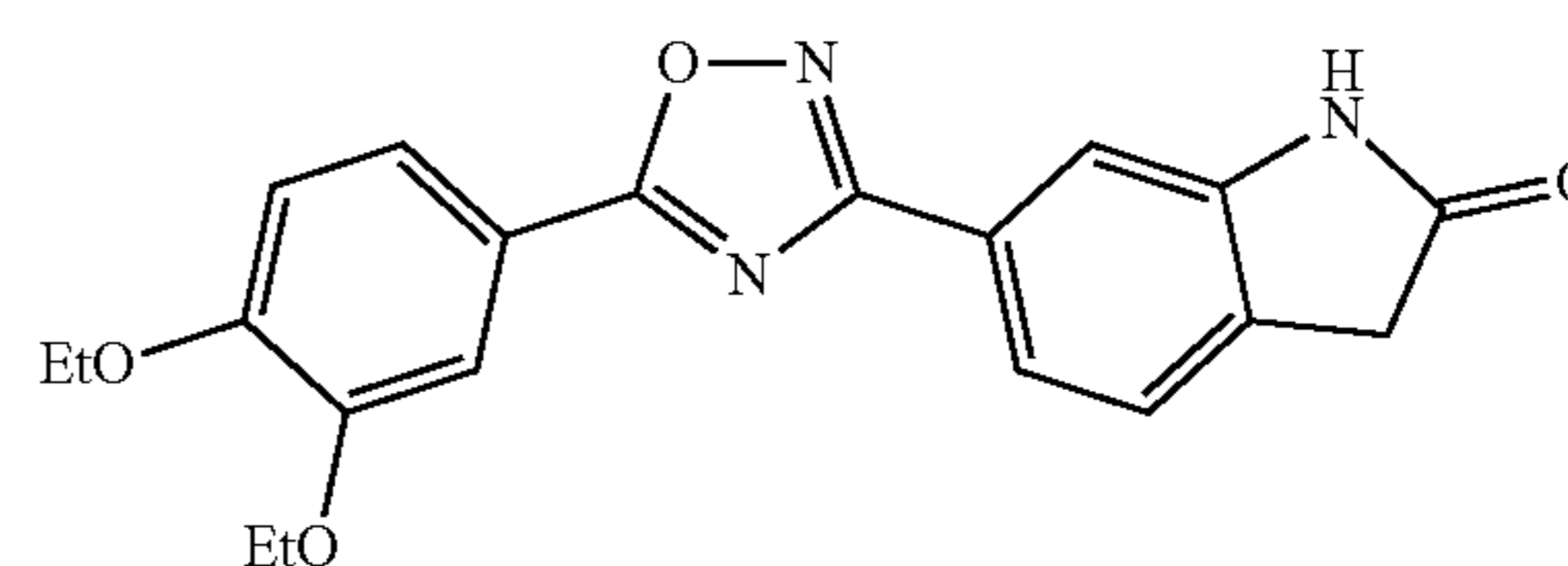
6-(5-(3,4-diethoxyphenyl)-1,2,4-oxadiazol-3-yl)indolin-2-one
