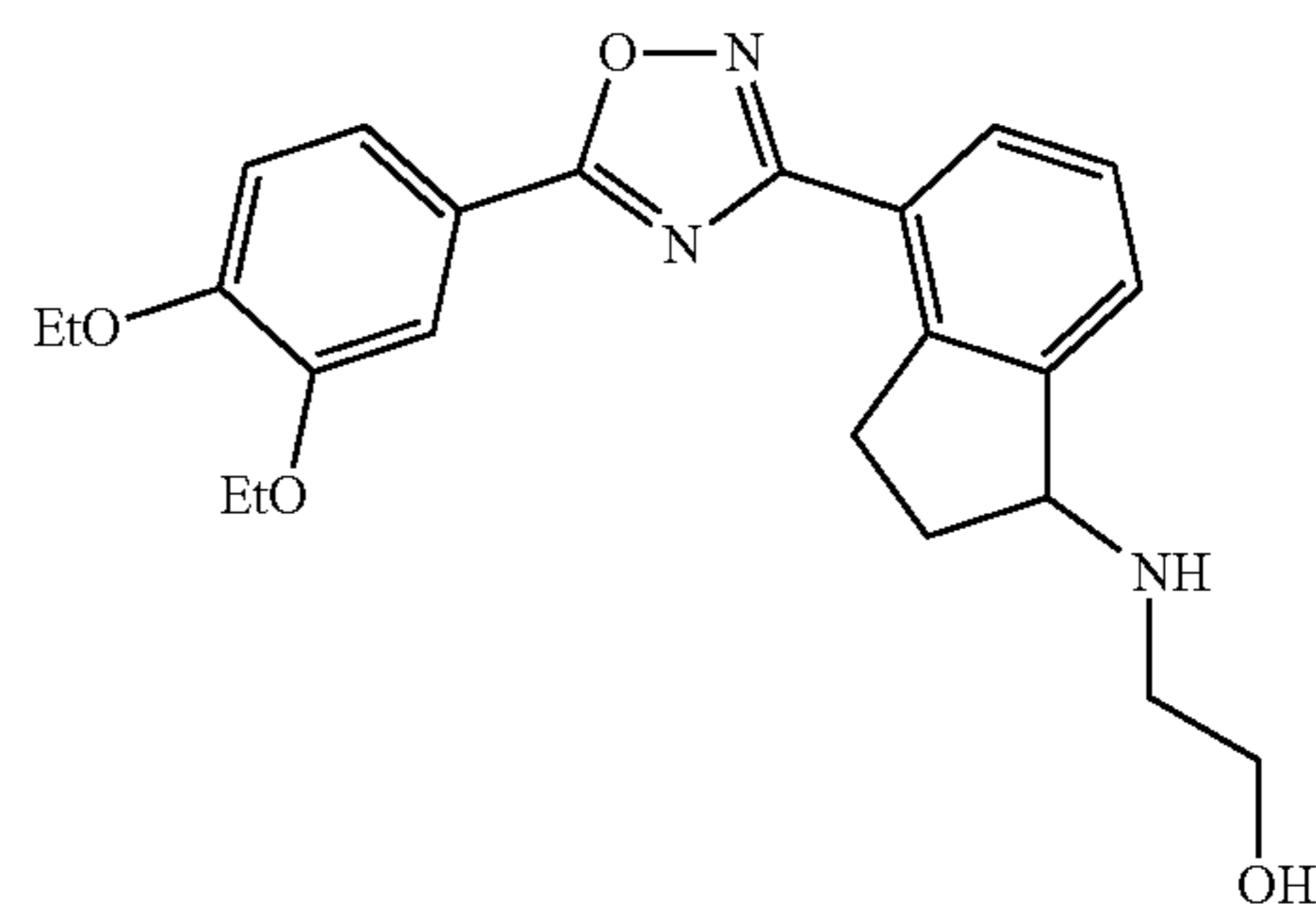
2-(4-(5-(3,4-diethoxyphenyl)-1,2,4-oxadiazol-3-yl)-2,3-dihydro-1H-inden-1-ylamino)ethanol
