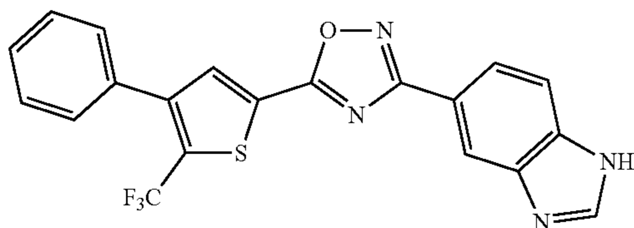
3-(1H-benzo[d]imidazol-5-yl)-5-(4-phenyl-5-(trifluoromethyl)thiophen-2-yl)-1,2,4-oxadiazole
