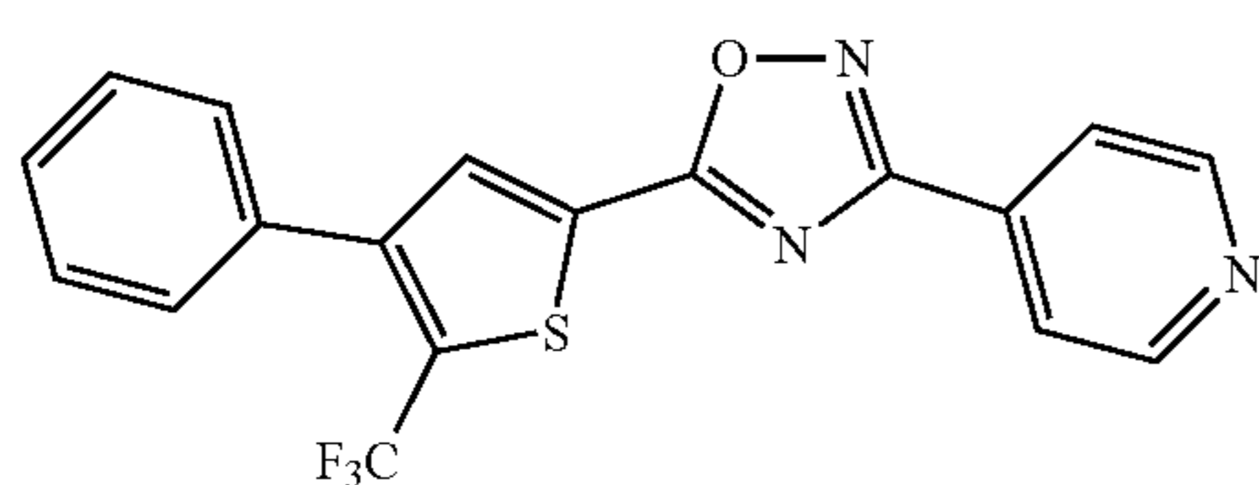
4-[5-(4-Phenyl-5-trifluoromethyl-thiophen-2-yl)-[1,2,4]oxadiazol-3-yl]pyridine
