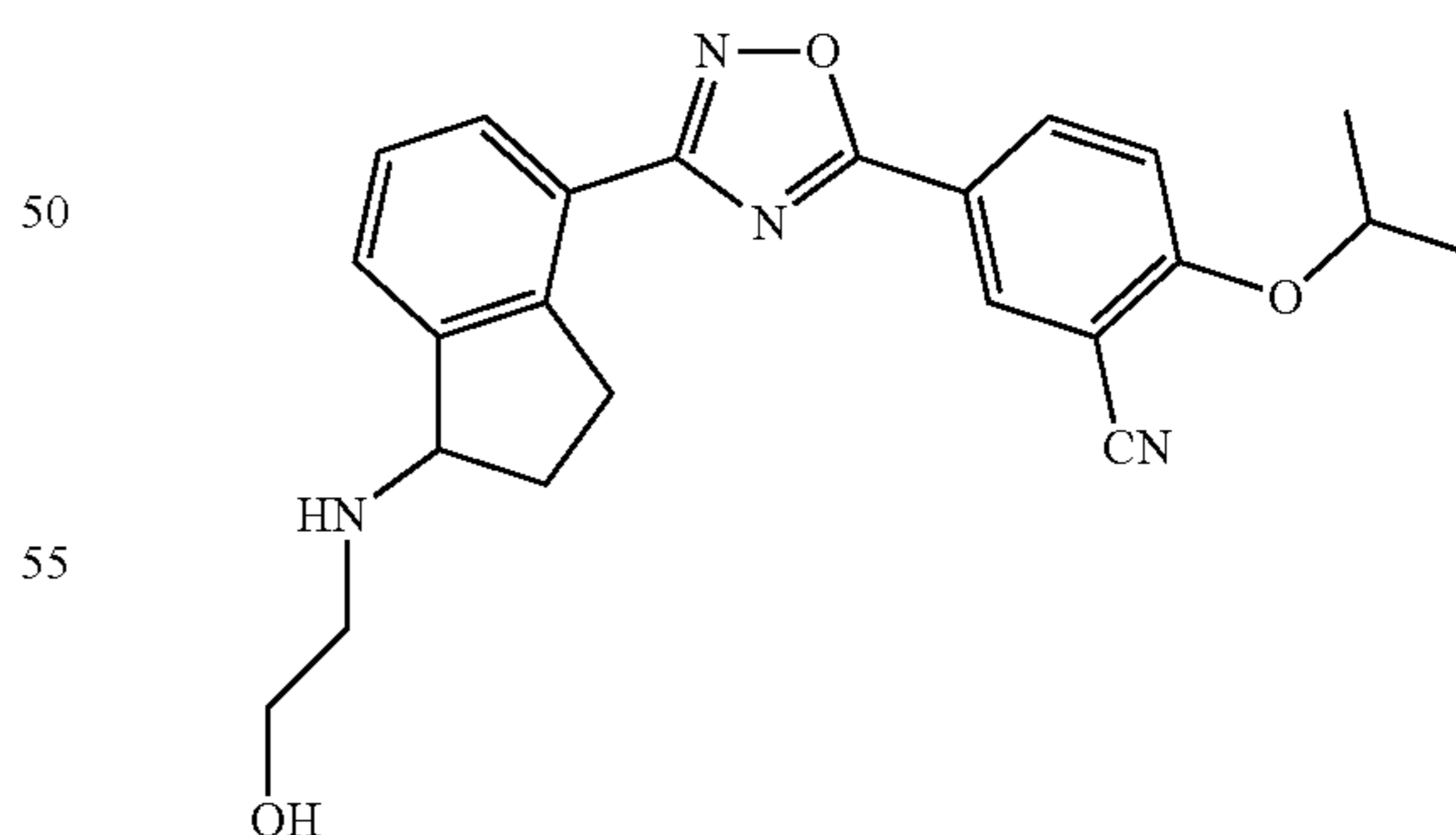
5-(3-(1-(2-hydroxyethylamino)-2,3-dihydro-1H-inden-4-yl)-1,2,4-oxadiazol-5-yl)-2-isopropoxybenzonitrile
