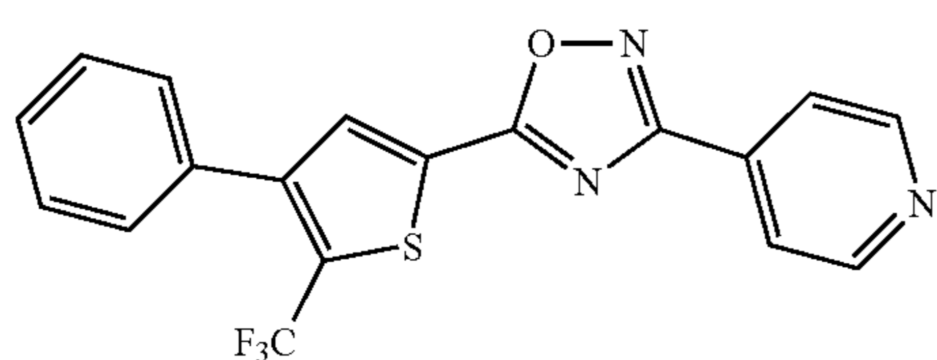
4-[5-(4-Phenyl-5-trifluoromethyl-thiophen-2-yl)-[1,2,4]oxadiazol-3-yl]pyridine
