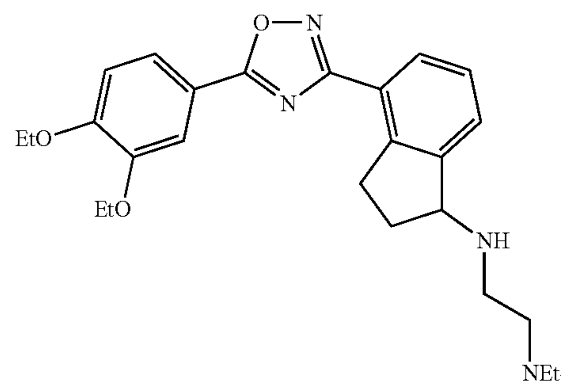
N1-(4-(5-(3,4-diethoxyphenyl)-1,2,4-oxadiazol-3-yl)-2,3-dihydro-1H-inden-1-yl)-N2,N2-diethylethane-1,2-diamine
