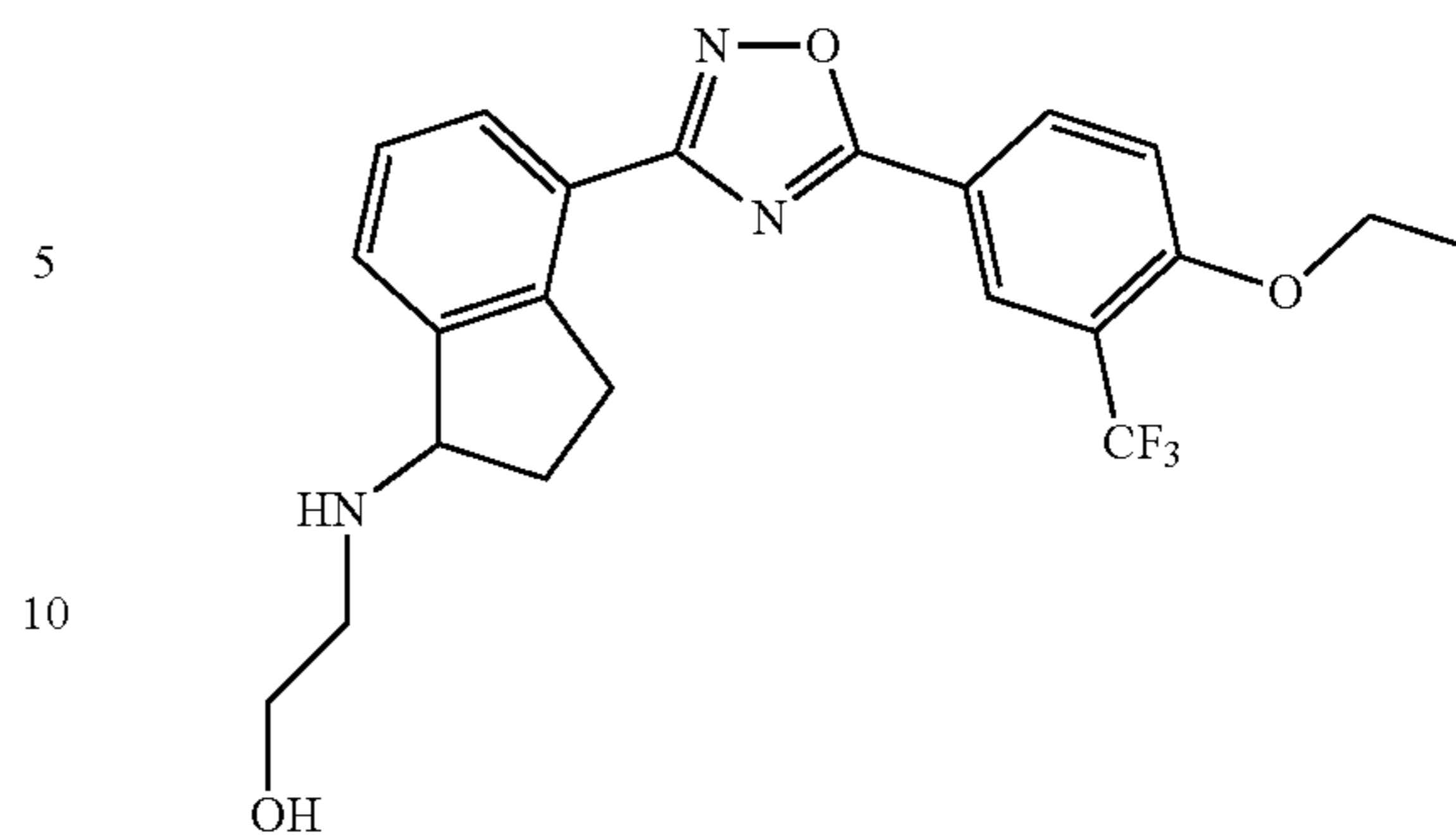
2-(4-(5-(4-ethoxy-3-(trifluoromethyl)phenyl)-1,2,4-oxadiazol-3-yl)-2,3-dihydro-1H-inden-1-ylamino)ethanol
