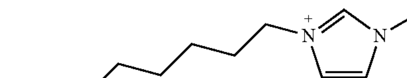
C6mim 1-Hexyl-3-methylimidazolium
