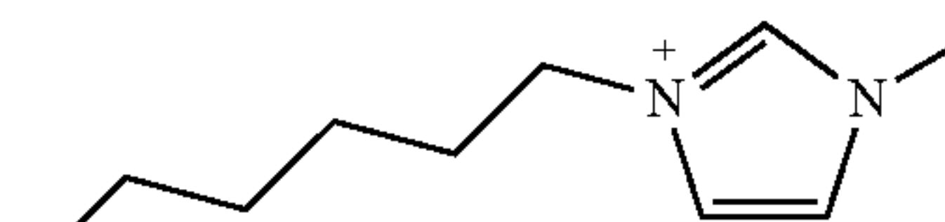
C6mim 1-Hexyl-3-methylimidazolium
