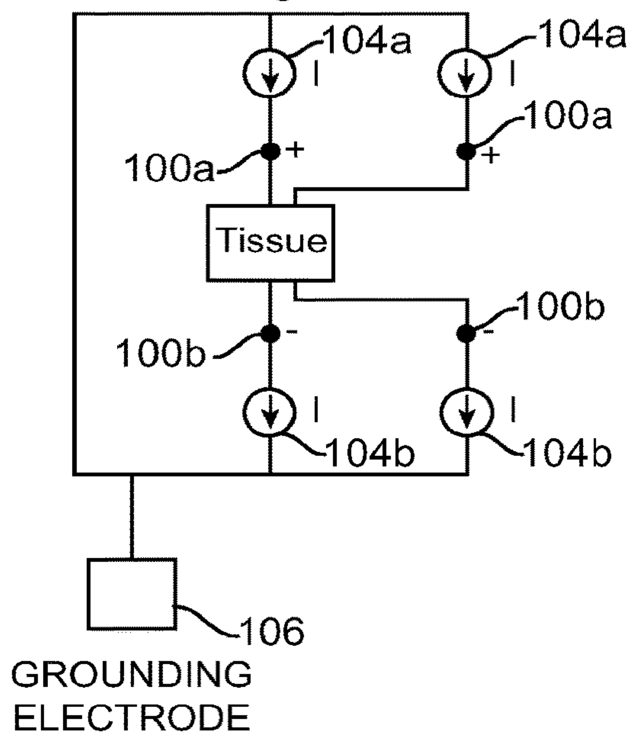
Symmetric Fully Isolated Current Regulated
