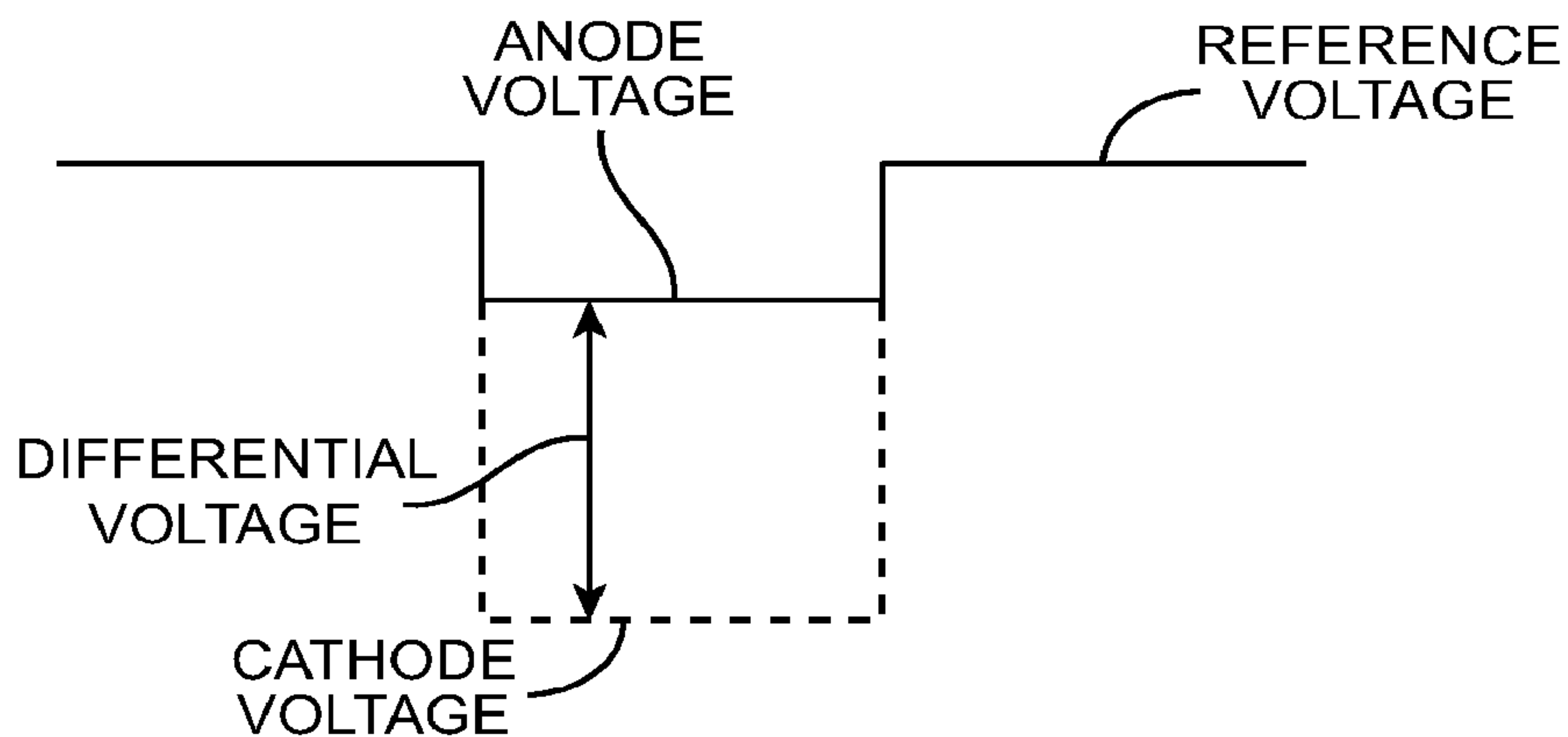
FIG. 2c (PRIOR ART)
