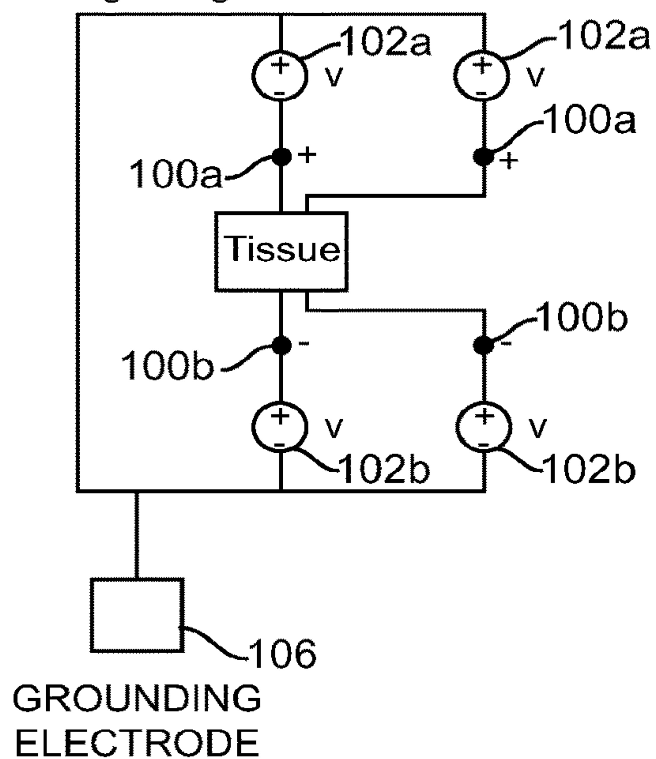
Symmetric Voltage Regulated
