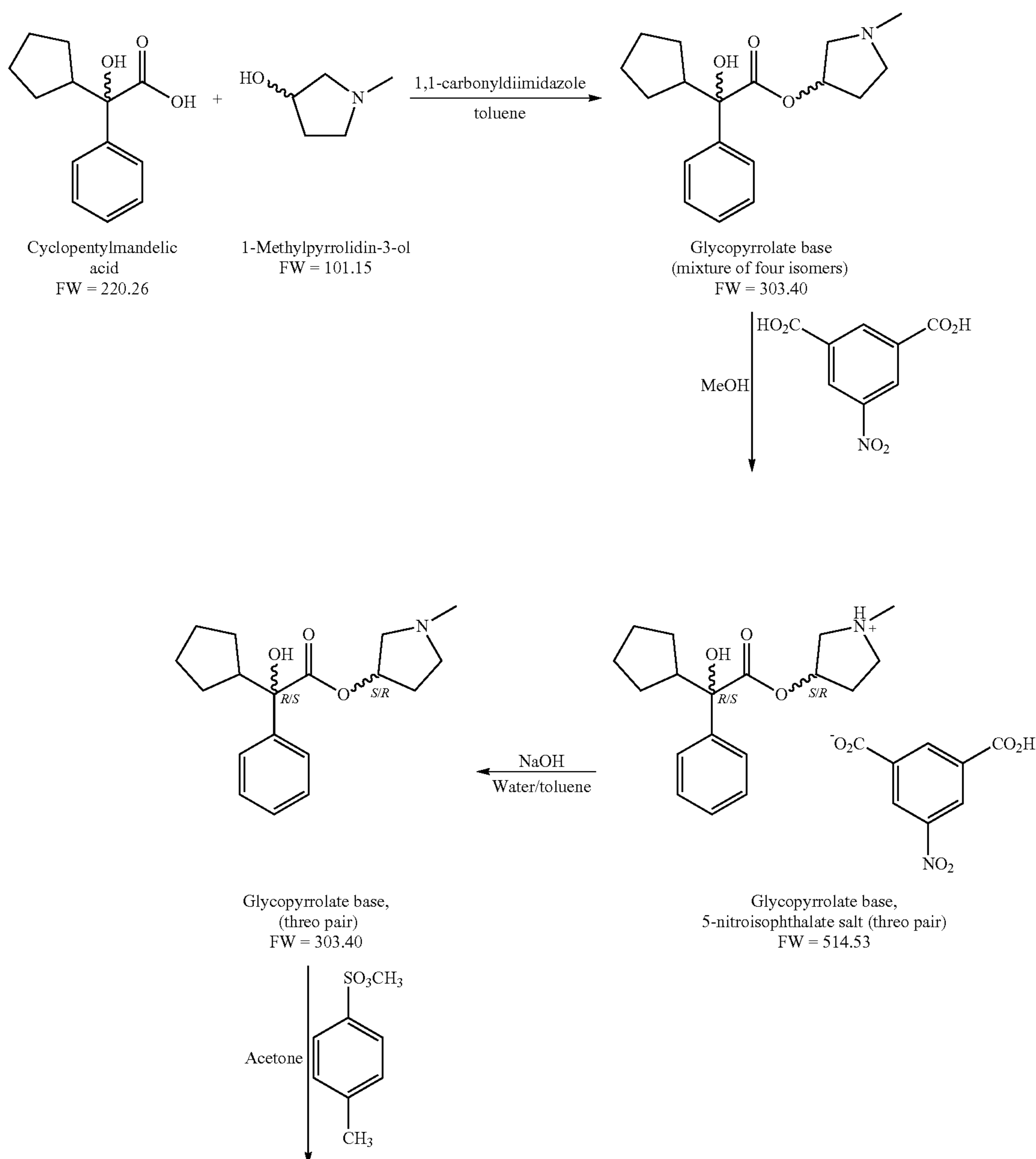
Scheme 1-Flow Diagram synthesis for Threo glycopyrrolate tosylate
