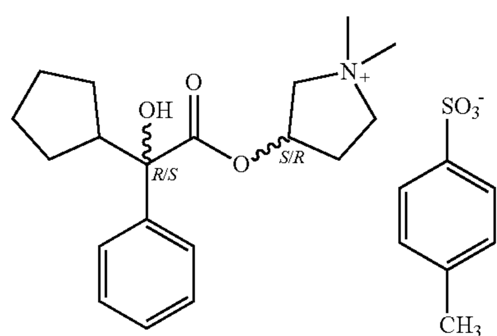
Glycopyrronium tosylate (threo pair) FW = 489.62
