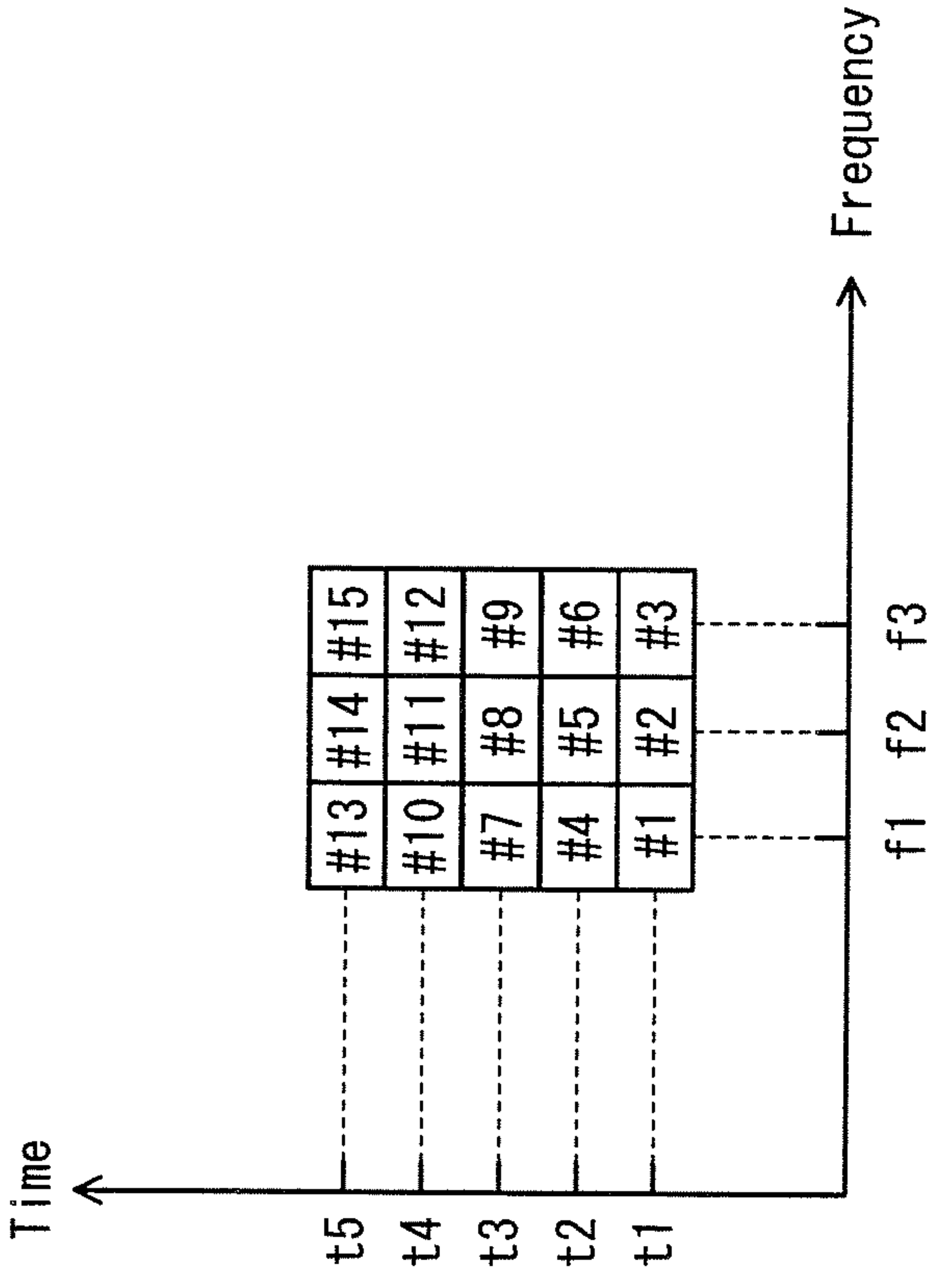
FIG. 75B Modulated signal z2
