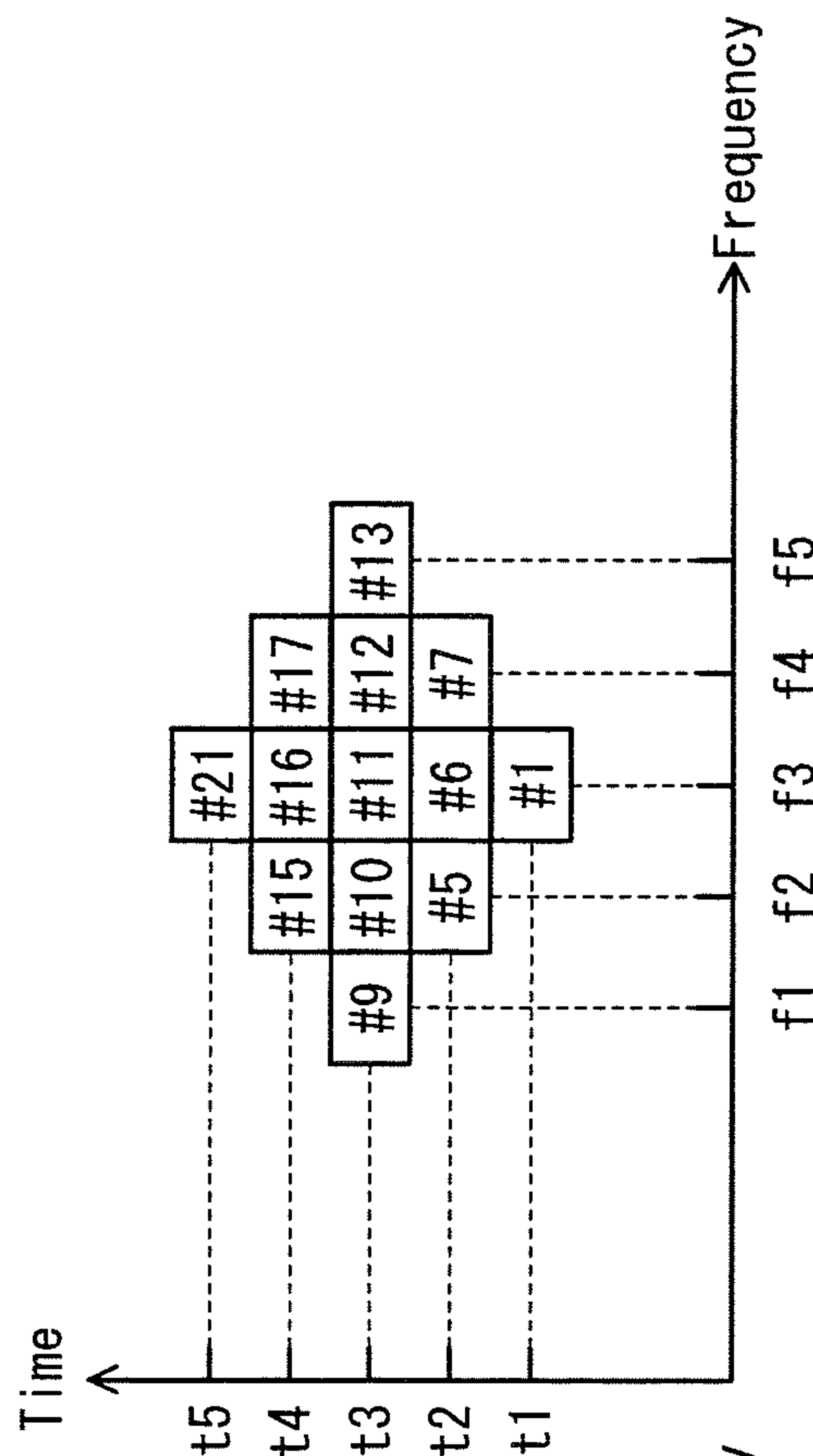
FIG. 77B Modulated signal z2
