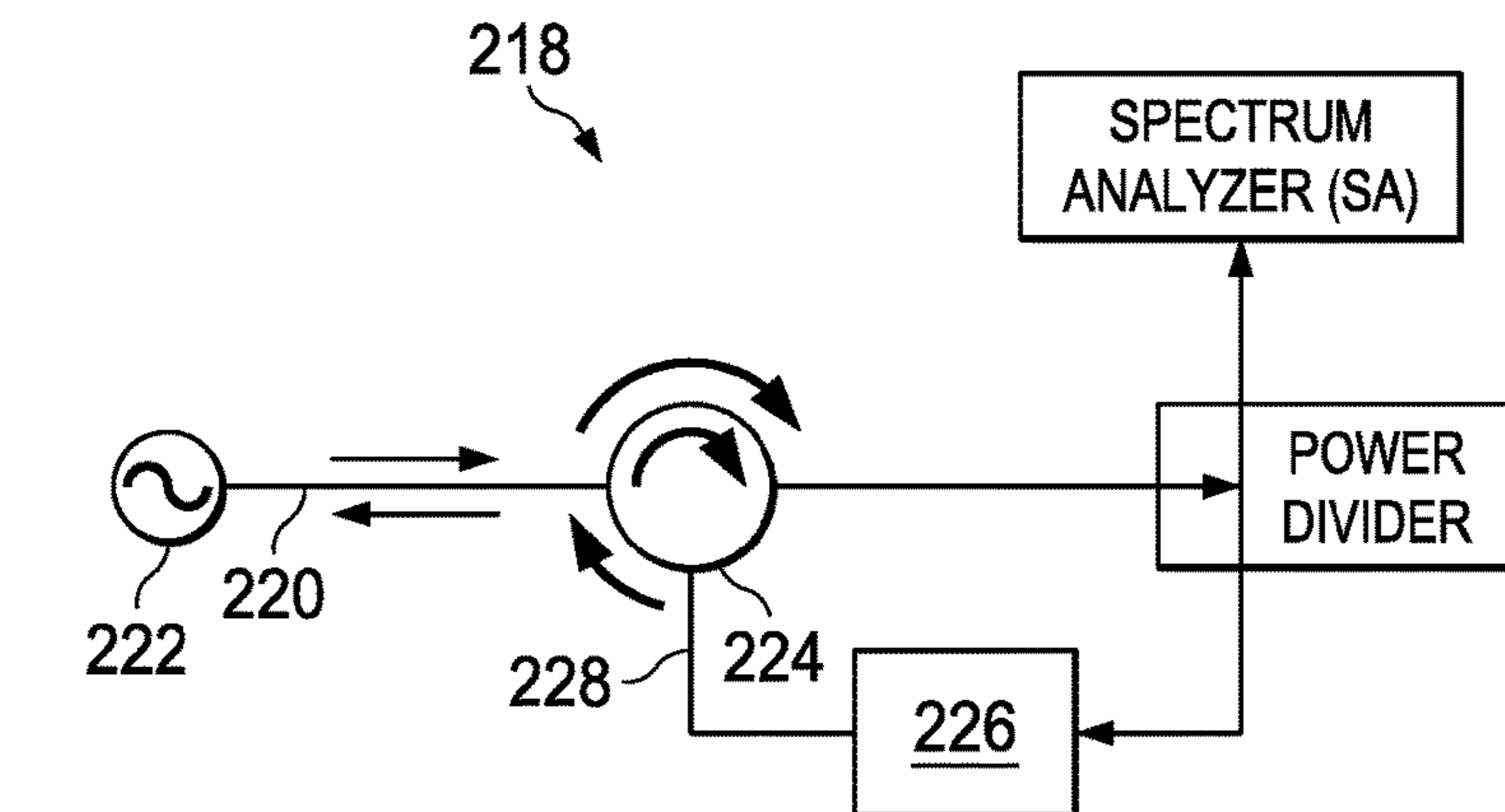
FIG. 2C (PRIOR ART)
