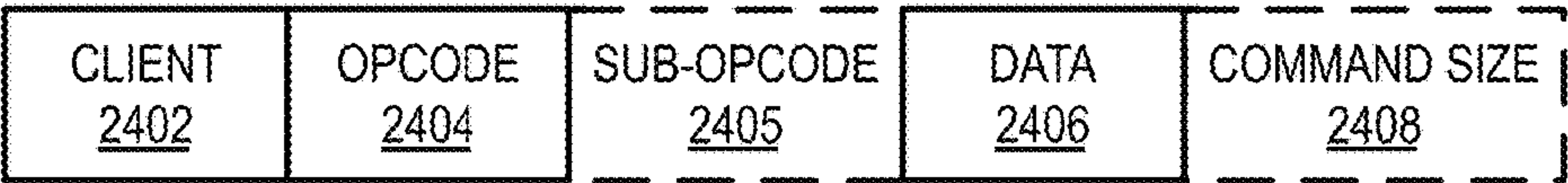
FIG. 24A GRAPHICS PROCESSOR COMMAND FORMAT 2400
