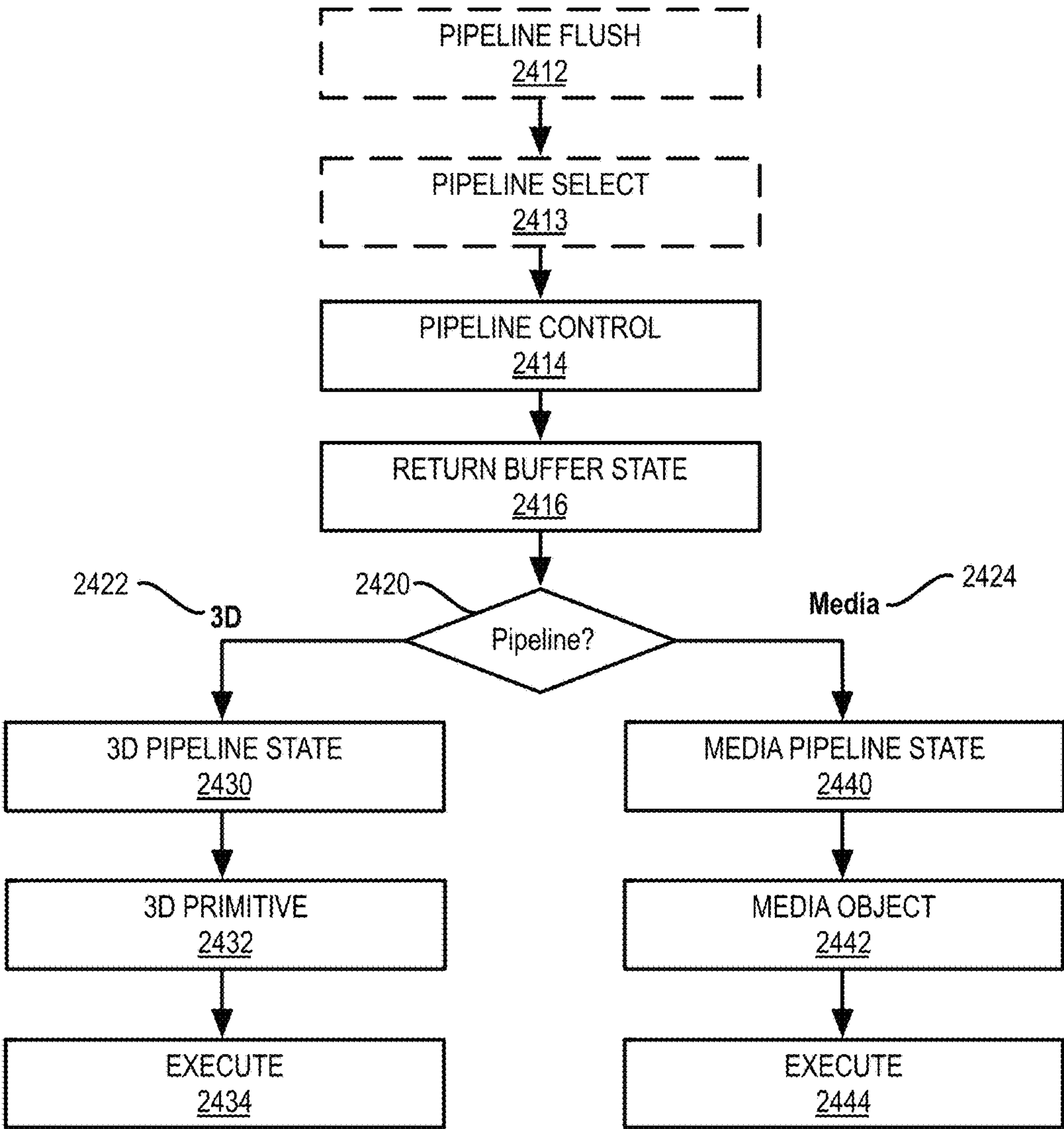
FIG. 24B GRAPHICS PROCESSOR COMMAND SEQUENCE 2410
