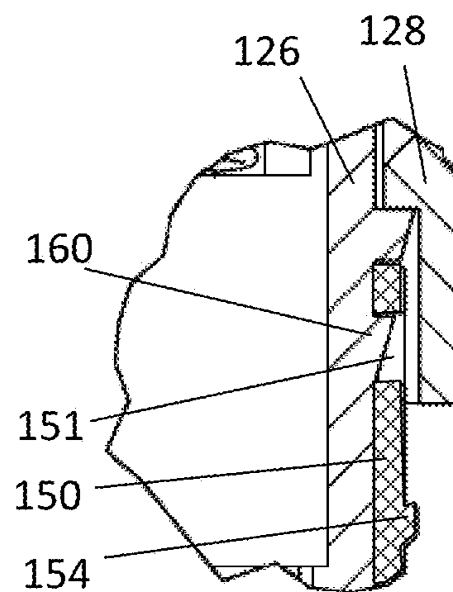
Detail E
