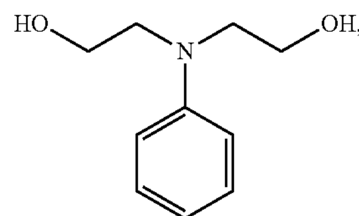
2,2'-(phenylazanediyl) bis(ethan-1-ol)
