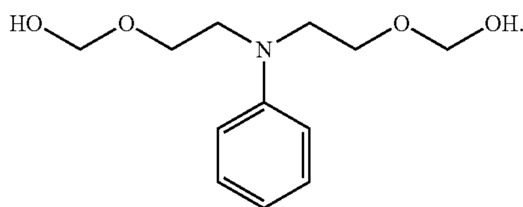
(((phenylazanediy)bis(ethane-2,1-diyl))bis(oxy))dimethanol
