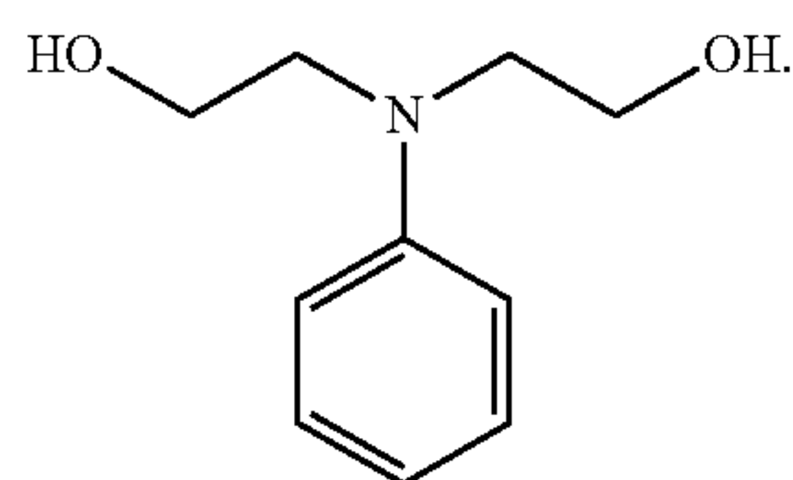
2,2'-(phenylazanediy)bis(ethan-1-ol)
