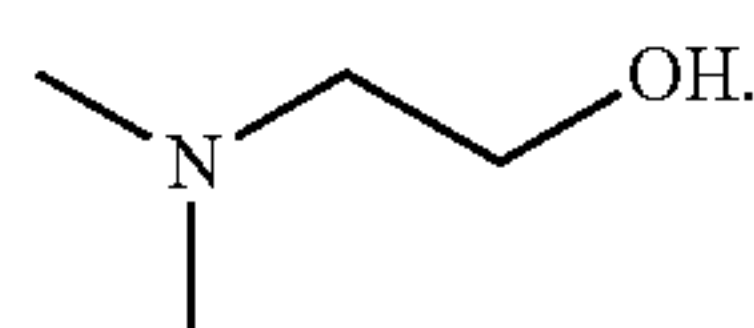
2-(dimethylamino)ethan-1-ol
