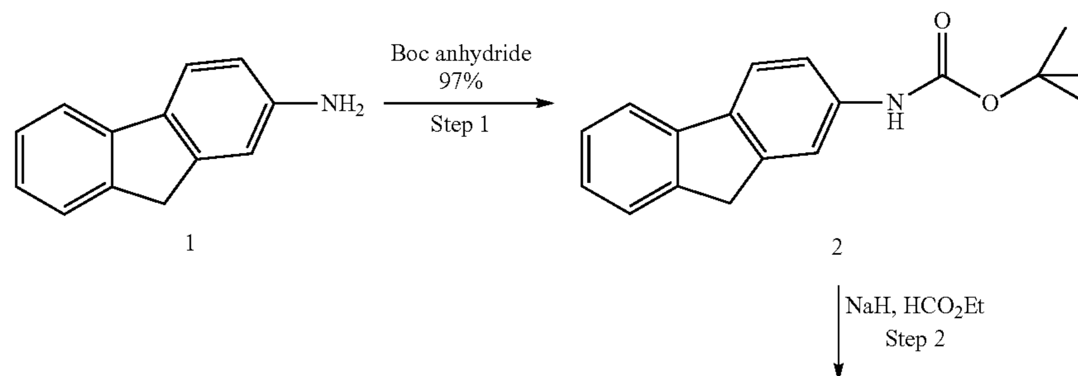
Scheme 1—Synthesis of MAL-FMS-NHS Linker
