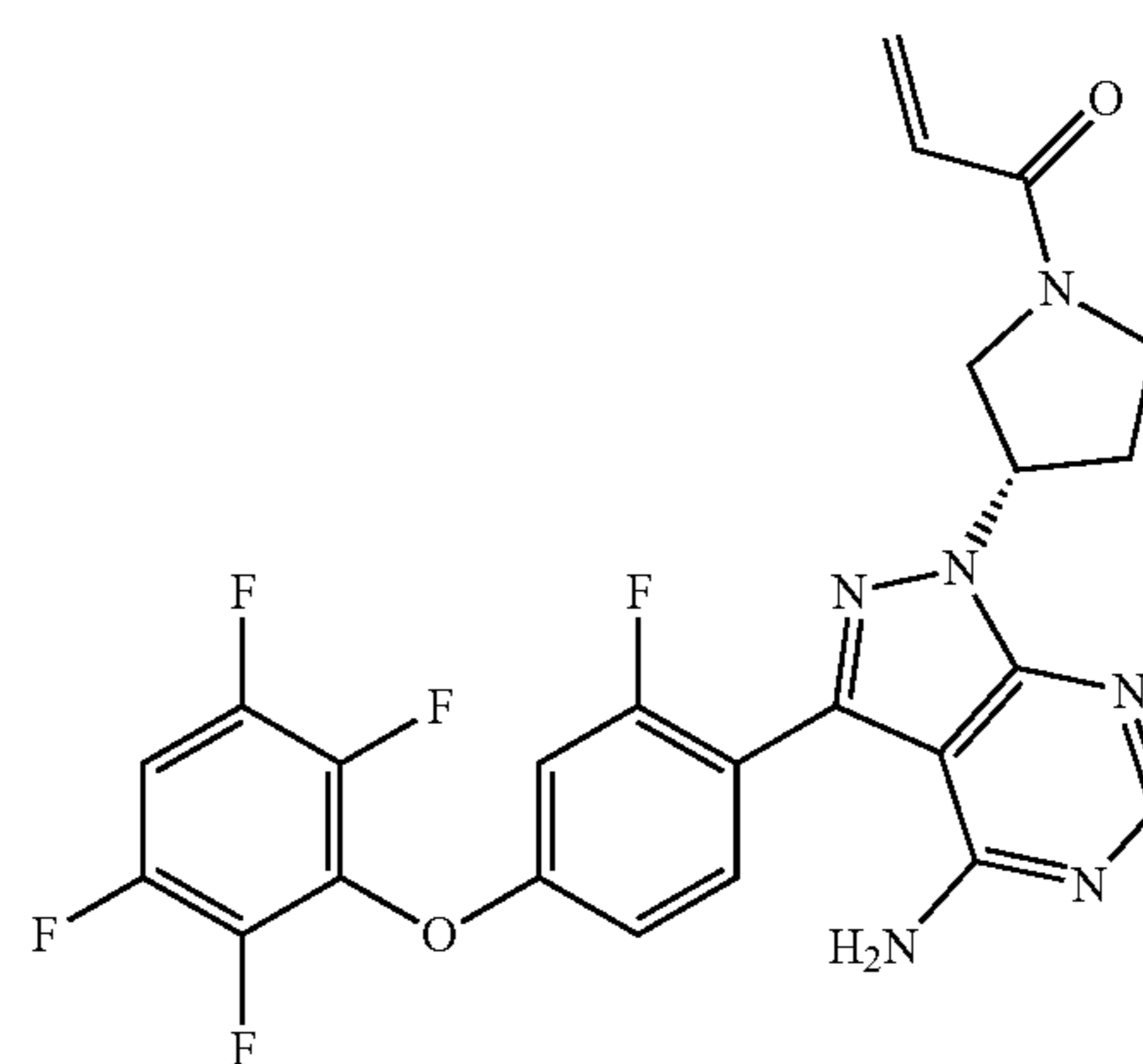
1-((S)-3-(4-amino-3-(2-fluoro-4-(2,3,5,6-tetrafluorophenoxy)phenyl)-1H-pyrazolo[3,4-d]pyrimidin-1-yl)pyrrolidin-1-yl)prop-2-en-1-one
