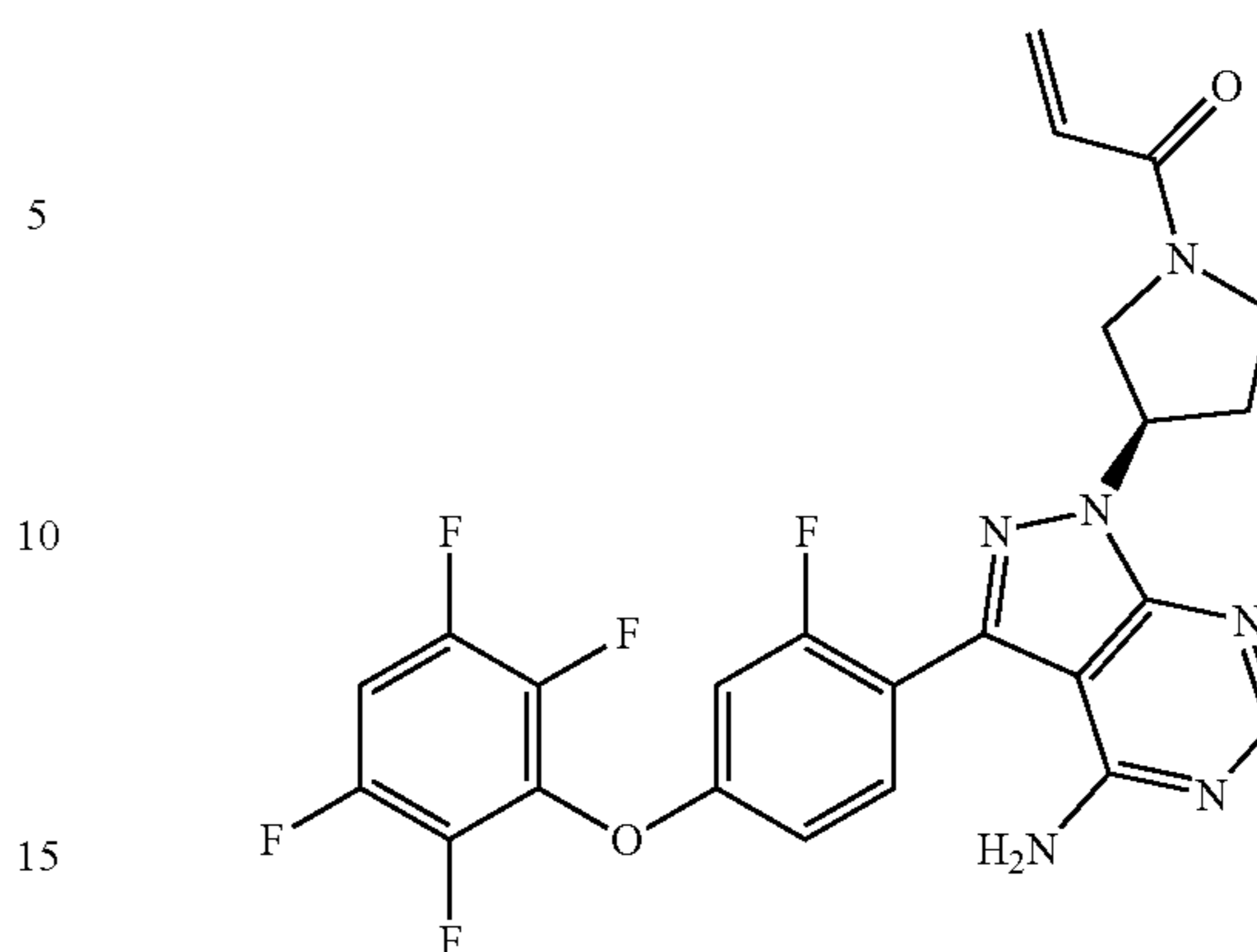
1-((R)-3-(4-amino-3-(2-fluoro-4-(2,3,5,6-tetrafluorophenoxy)phenyl)-1H-pyrazolo[3,4-d]pyrimidin-1-yl)pyrrolidin-1-yl)prop-2-en-1-one
