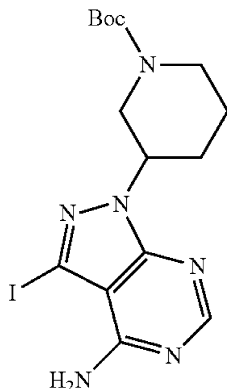
tert-butyl 3-(4-amino-3-iodo-1H-pyrazolo[3,4-d]pyrimidin-1-yl)piperidine-1-carboxylate
