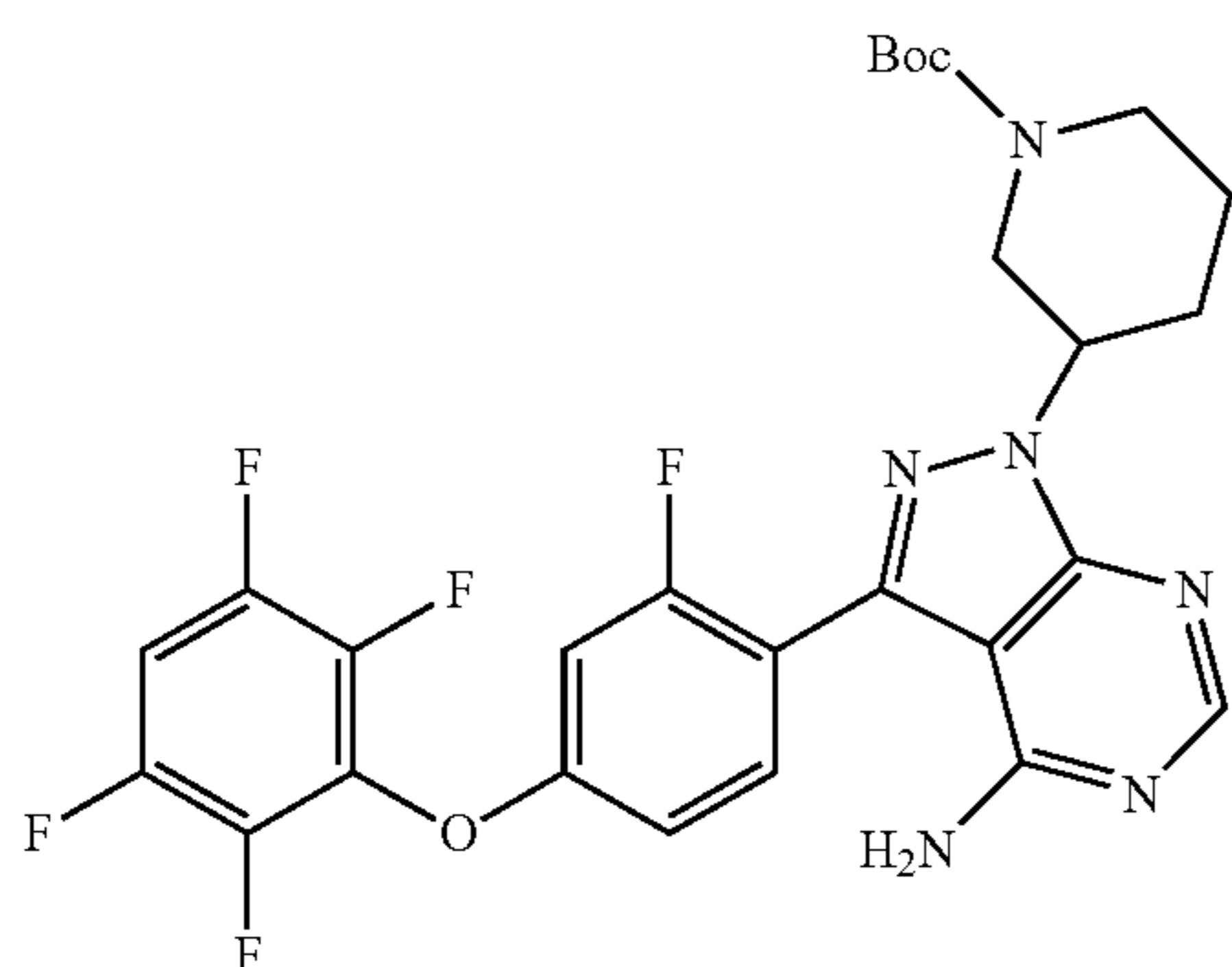
tert-butyl 3-(4-amino-3-(2-fluoro-4-(2,3,5,6-tetrafluorophenoxy)phenyl)-1H-pyrazolo[3,4-d]pyrimidin-1-yl)piperidine-1-carboxylate
