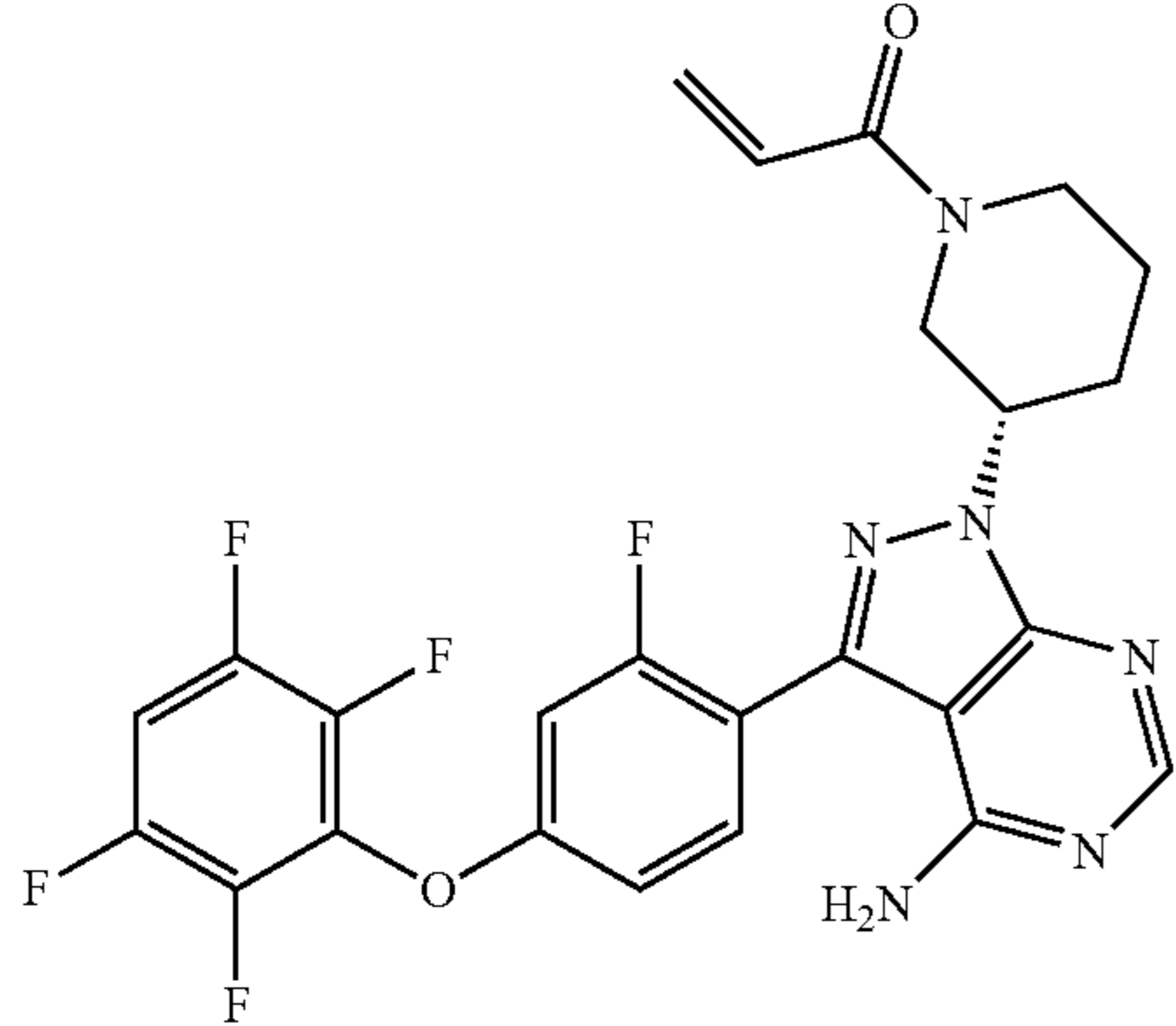
1-((S)-3-(4-amino-3-(2-fluoro-4-(2,3,5,6-tetrafluorophenoxy)phenyl)-1H-pyrazolo[3,4-d]pyrimidin-1-yl)piperidin-1-yl)prop-2-en-1-one
