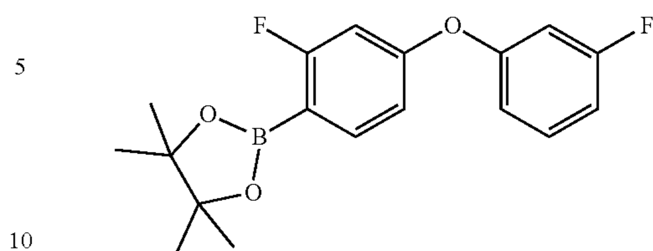
2-(2-fluoro-4-(3-fluorophenoxy)phenyl)-4,4,5,5-tetramethyl-1,3,2-dioxaborolane
