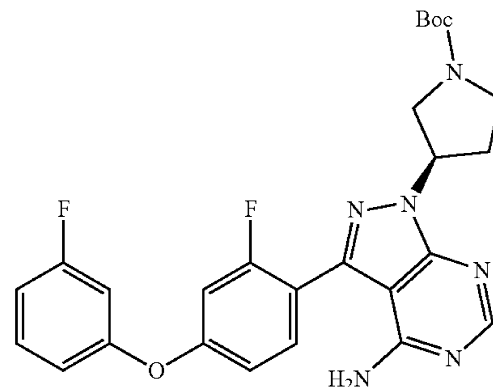
(3R)-tert-butyl 3-(4-amino-3-(2-fluoro-4-(3-fluorophenoxy)phenyl)-1H-pyrazolo[3,4-d]pyrimidin-1-yl)pyrrolidine-1-carboxylate
