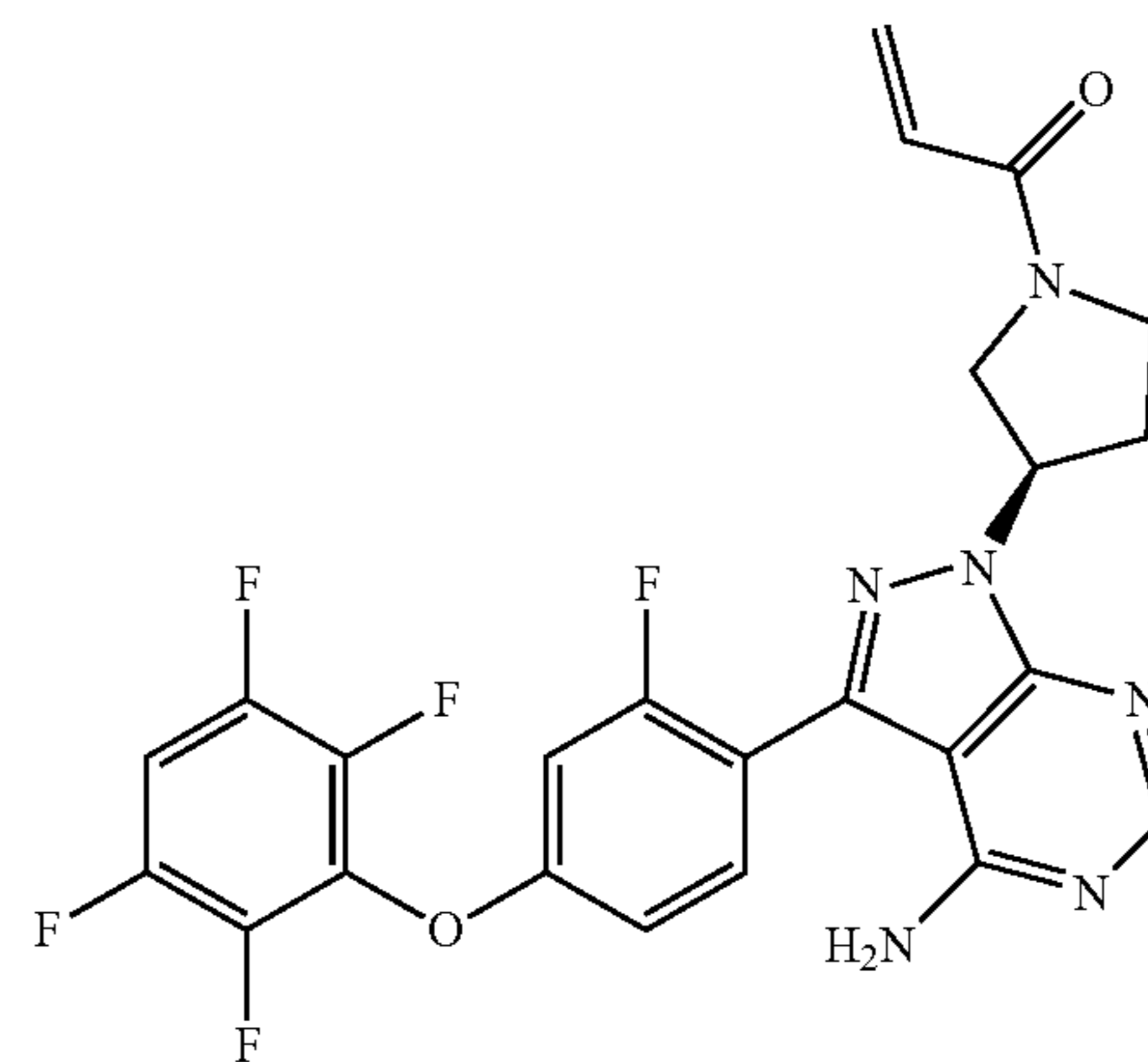
1-((R)-3-(4-amino-3-(2-fluoro-4-(2,3,5,6-tetrafluorophenoxy)phenyl)-1H-pyrazolo[3,4-d]pyrimidin-1-yl)pyrrolidin-1-yl)prop-2-en-1-one
