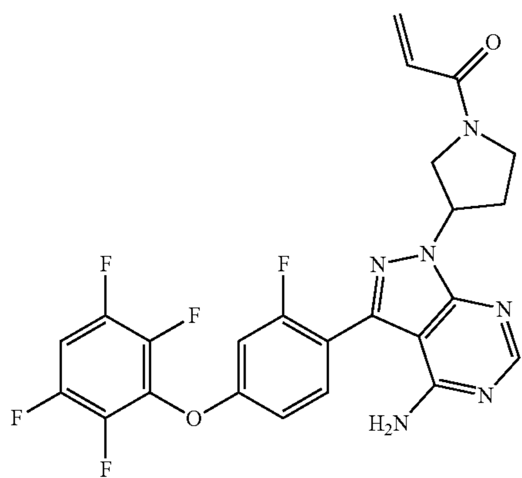
1-(3-(4-amino-3-(2-fluoro-4-(2,3,5,6-tetrafluorophenoxy)phenyl)-1H-pyrazolo[3,4-d]pyrimidin-1-yl)pyrrolidin-1-yl)prop-2-en-1-one
