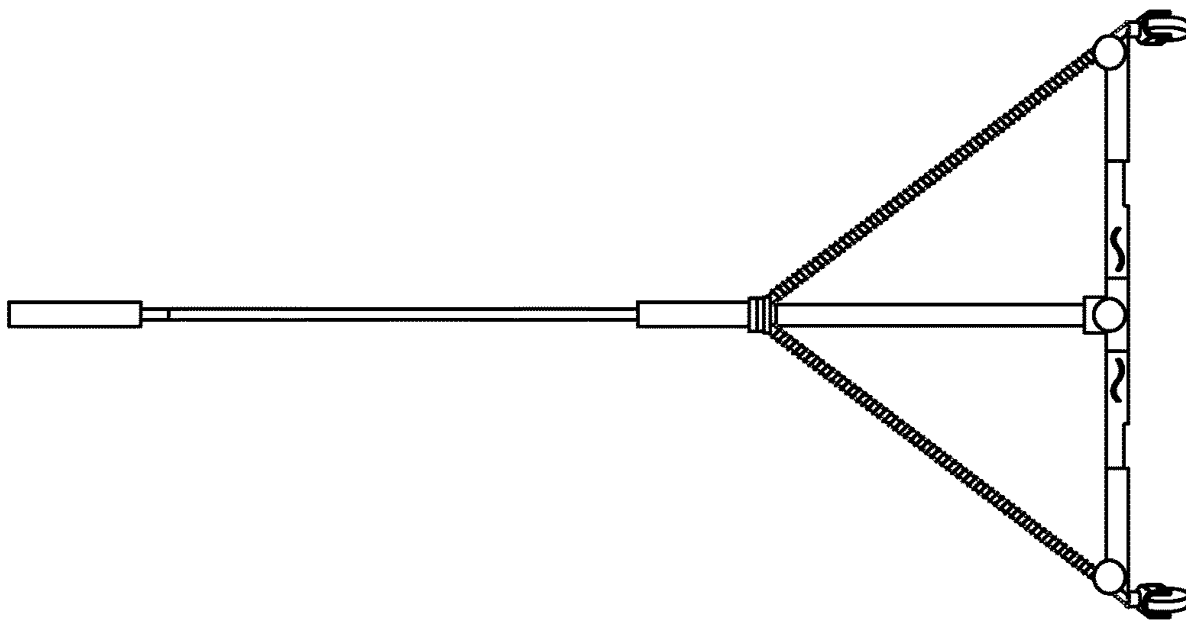
Deployed (Open)
