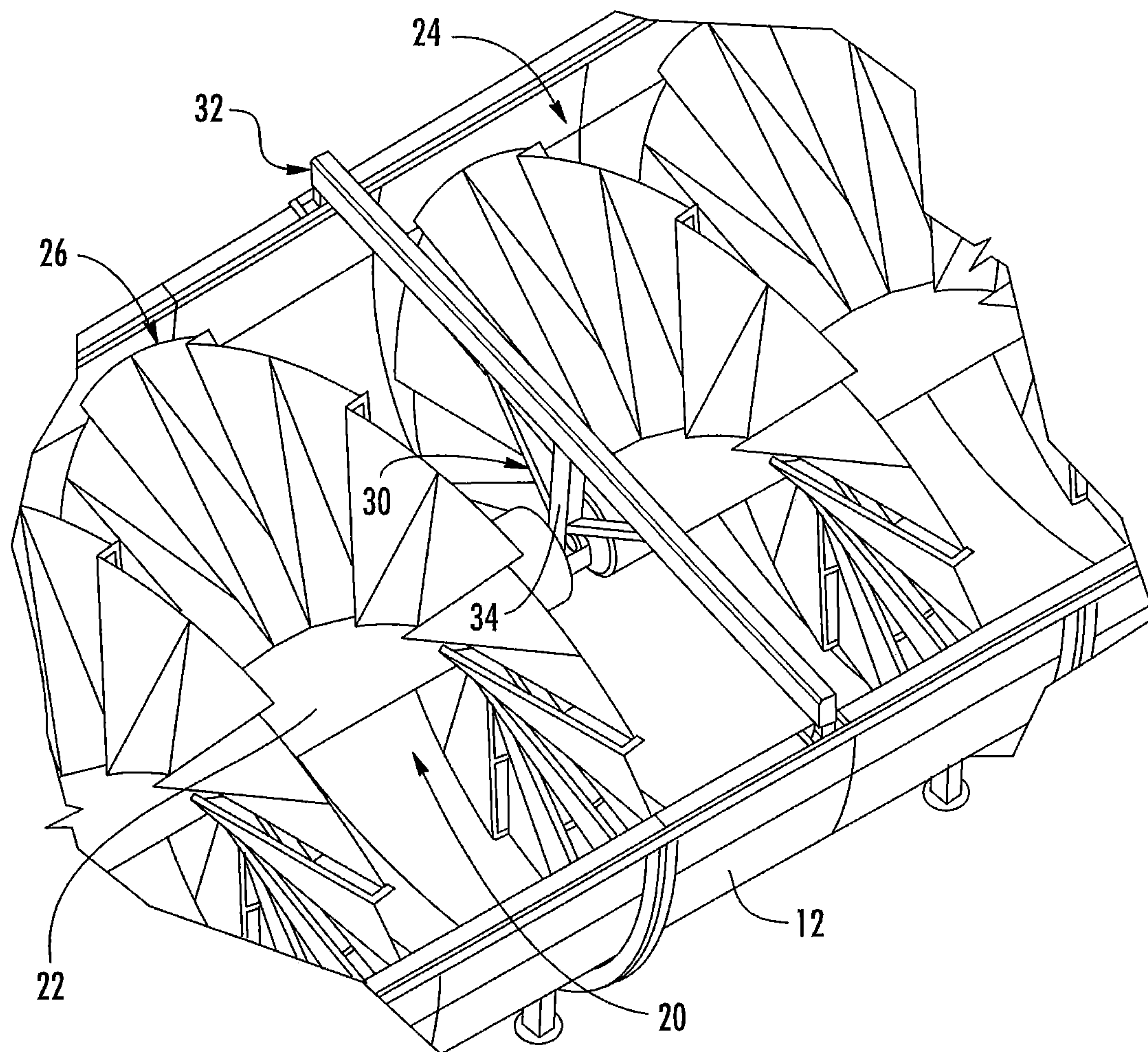
FIG. 3 (PRIOR ART)
