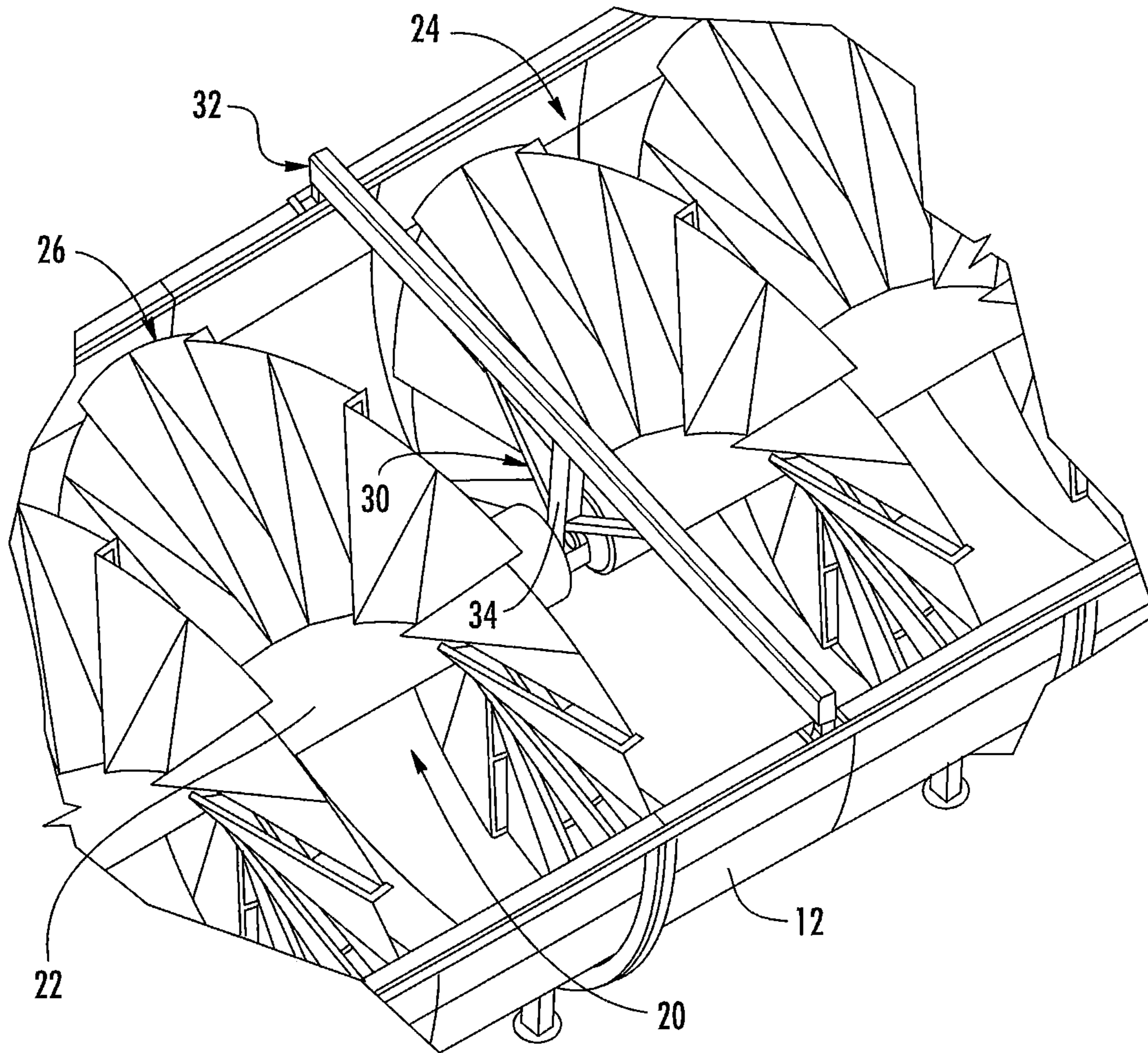
FIG. 3 (PRIOR ART)
