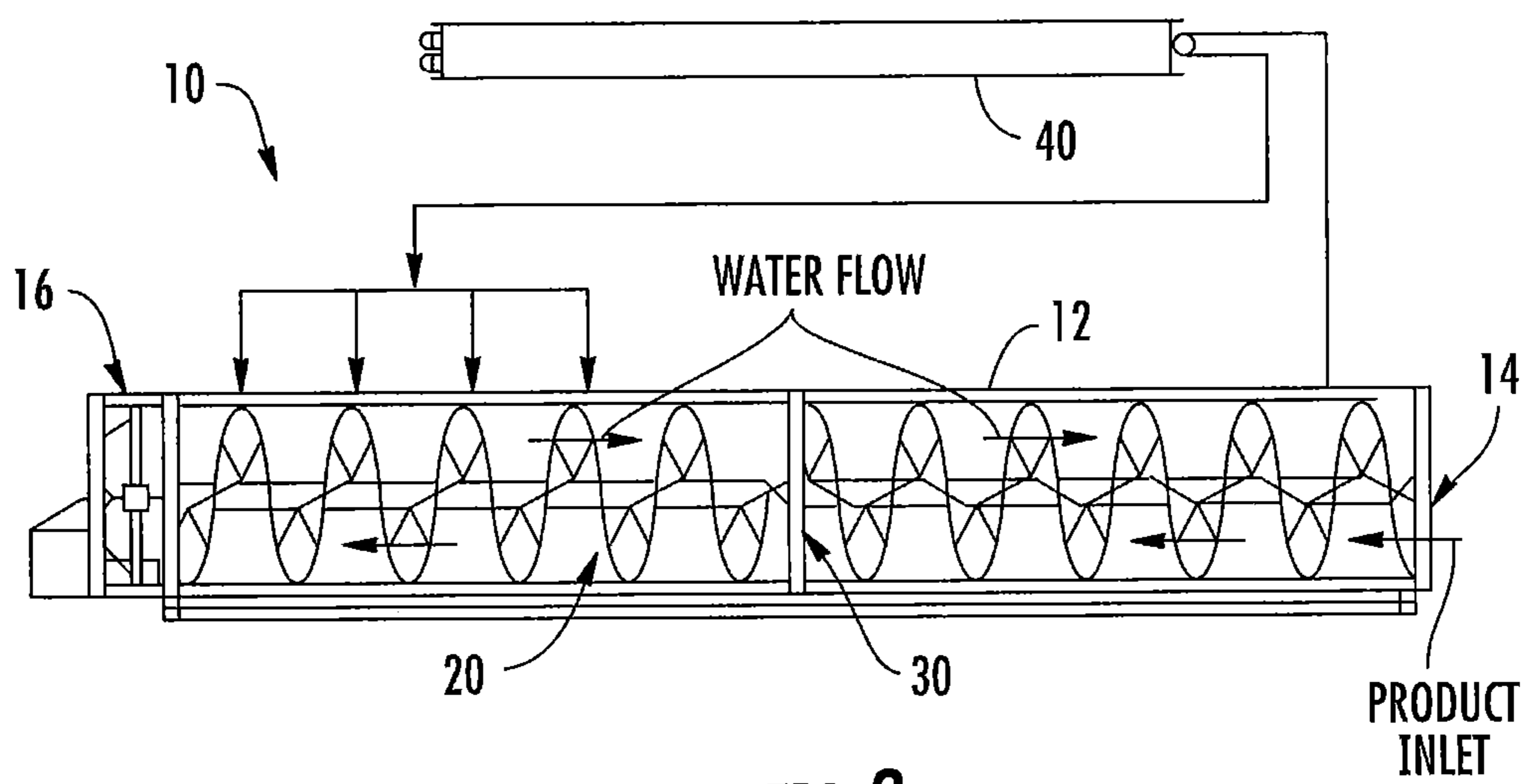
FIG. 2 (PRIOR ART)
