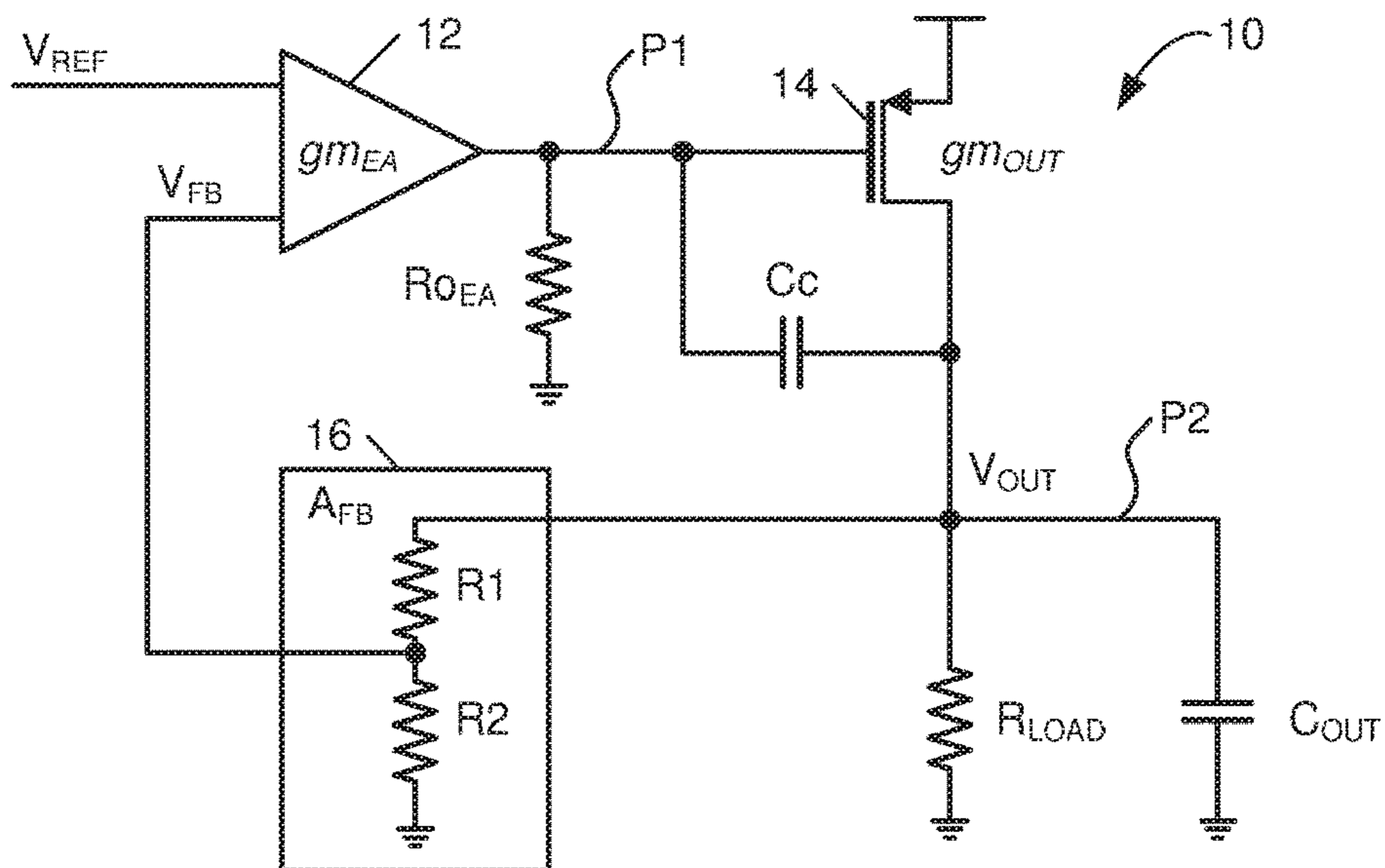
FIG. 1 (RELATED ART)
