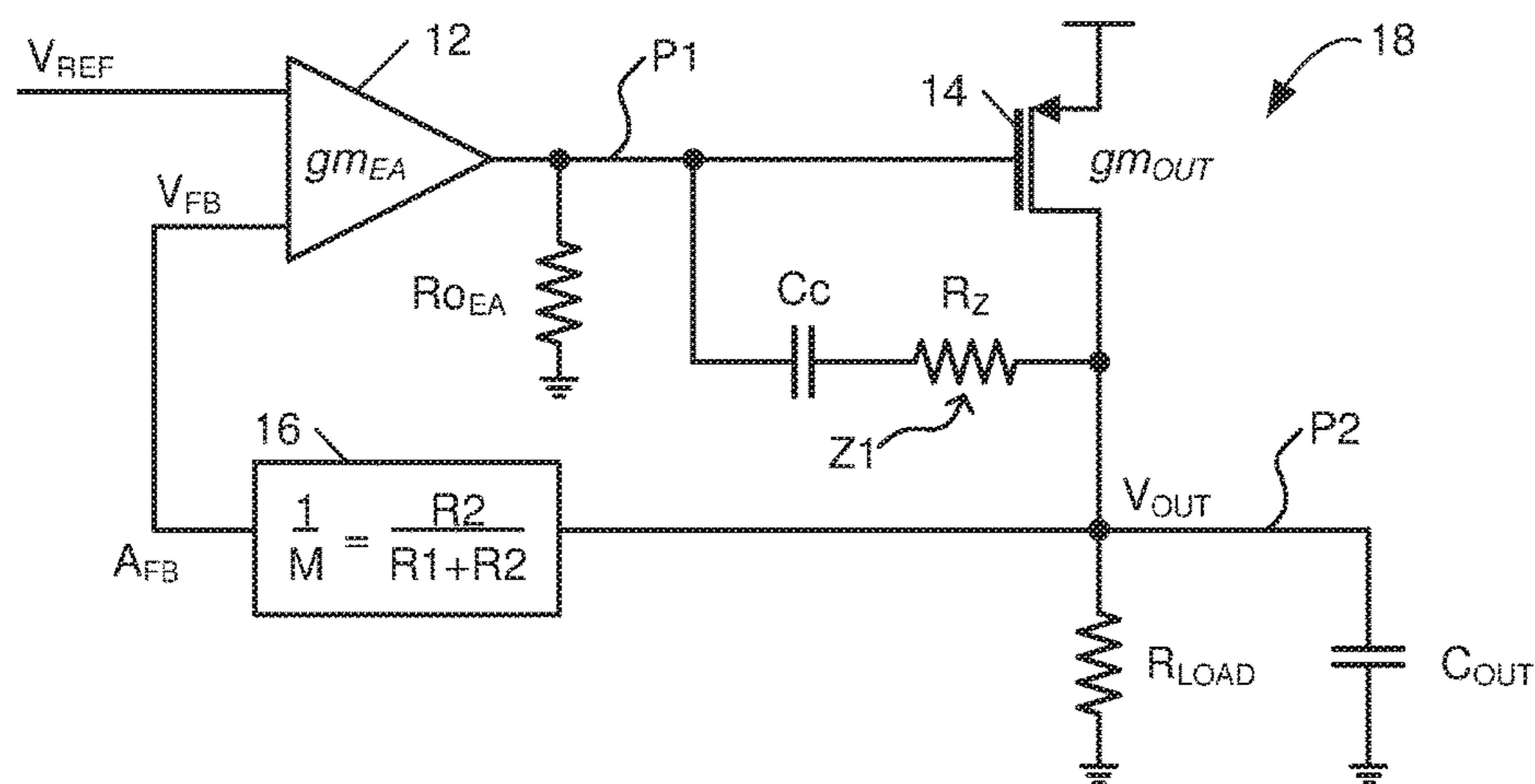
FIG. 3 (RELATED ART)
