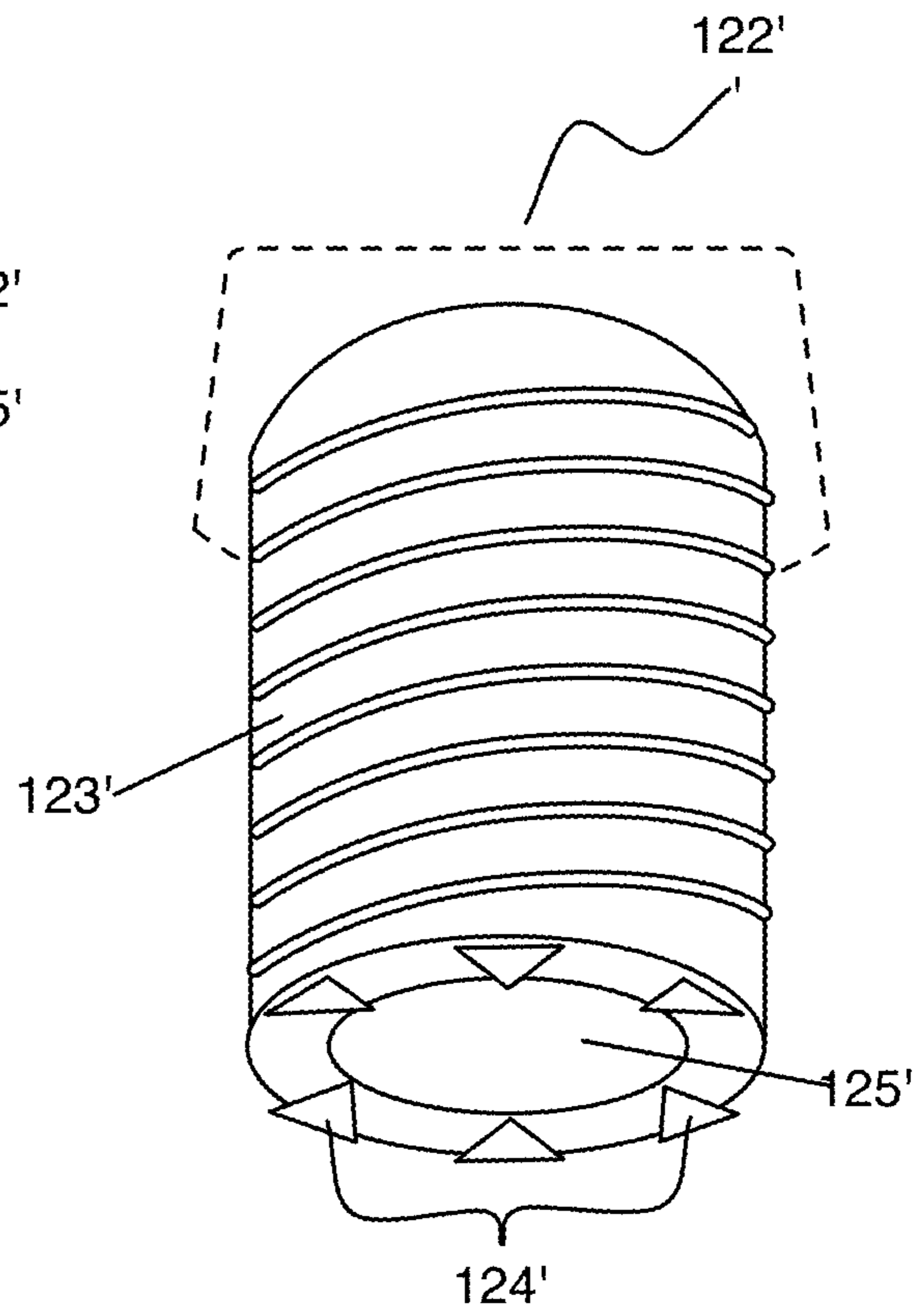
Isometric View
