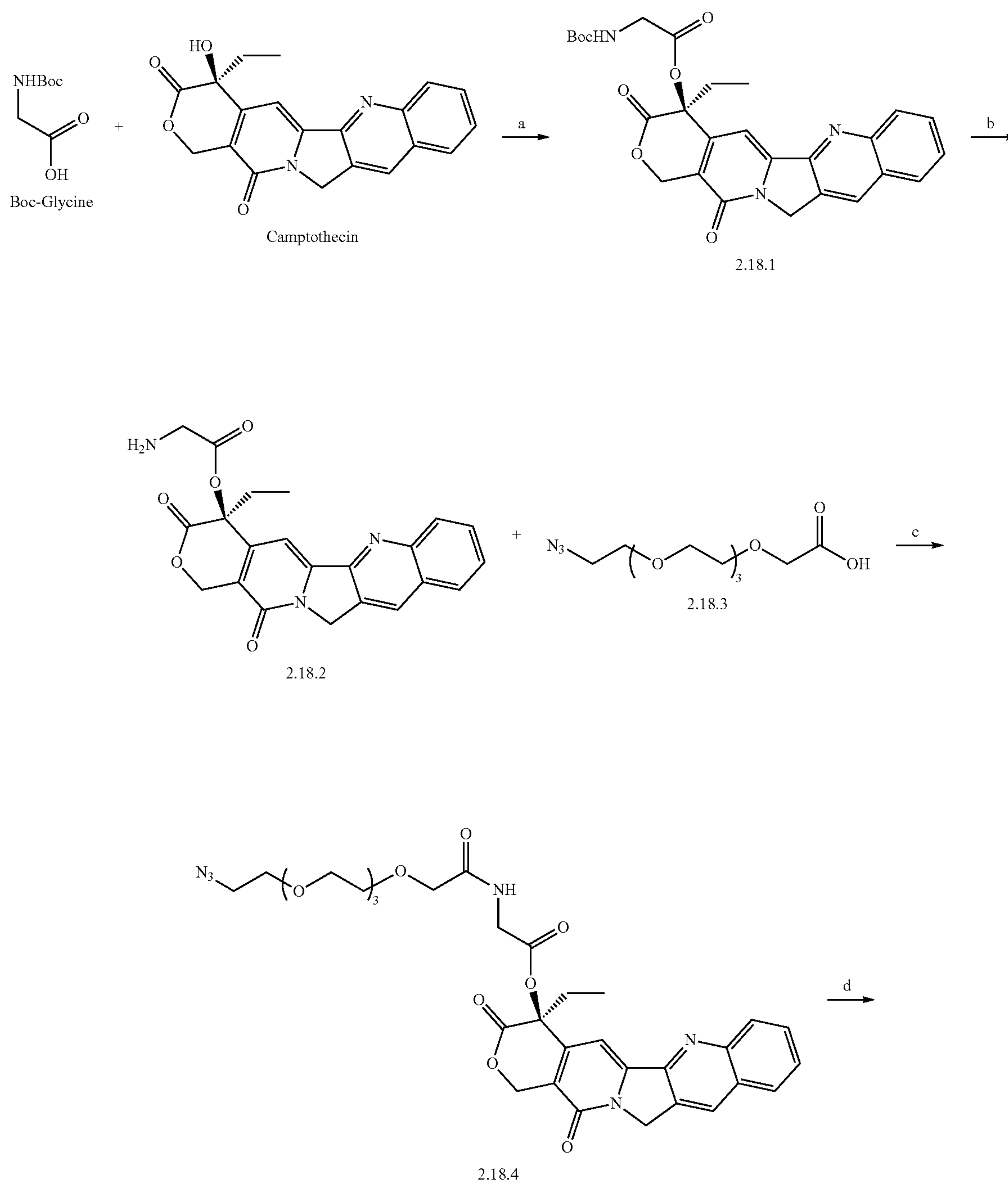
Scheme 6
