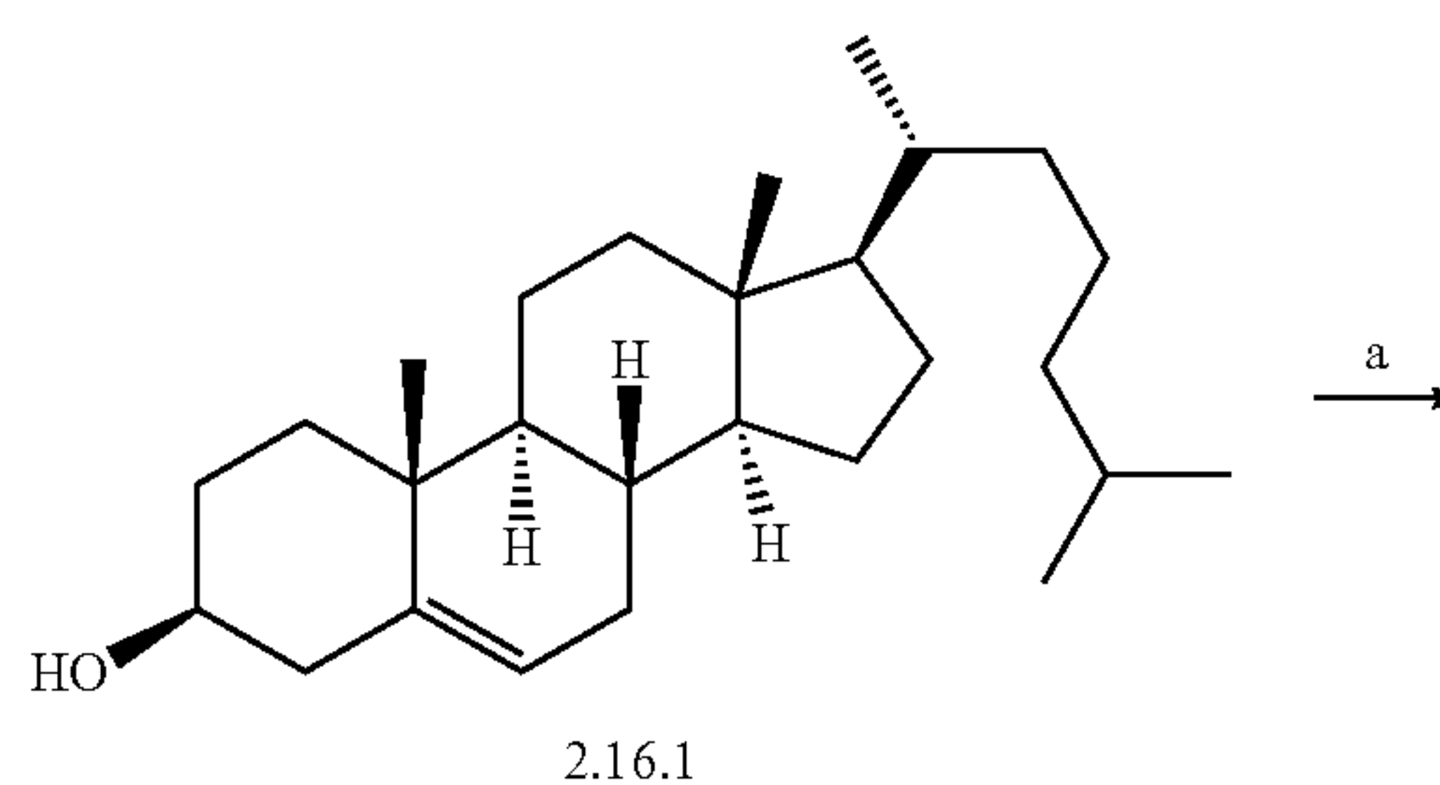
Scheme 4
