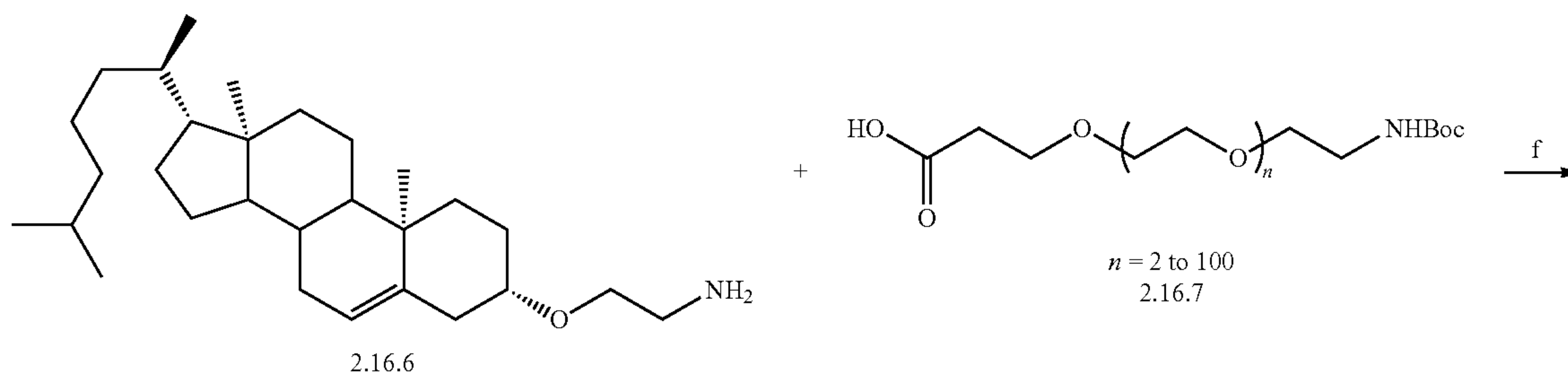
Scheme 5
