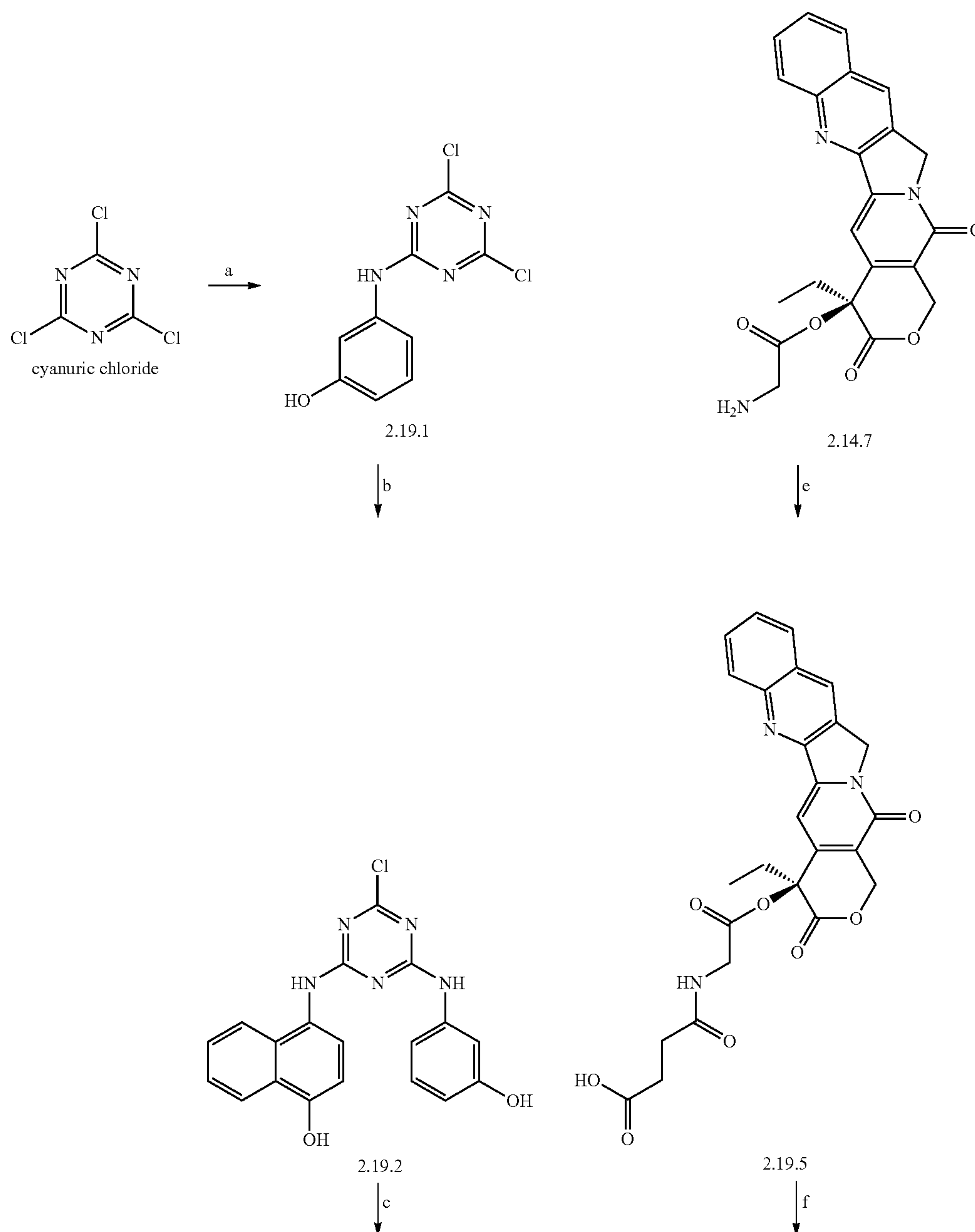
Scheme 7
