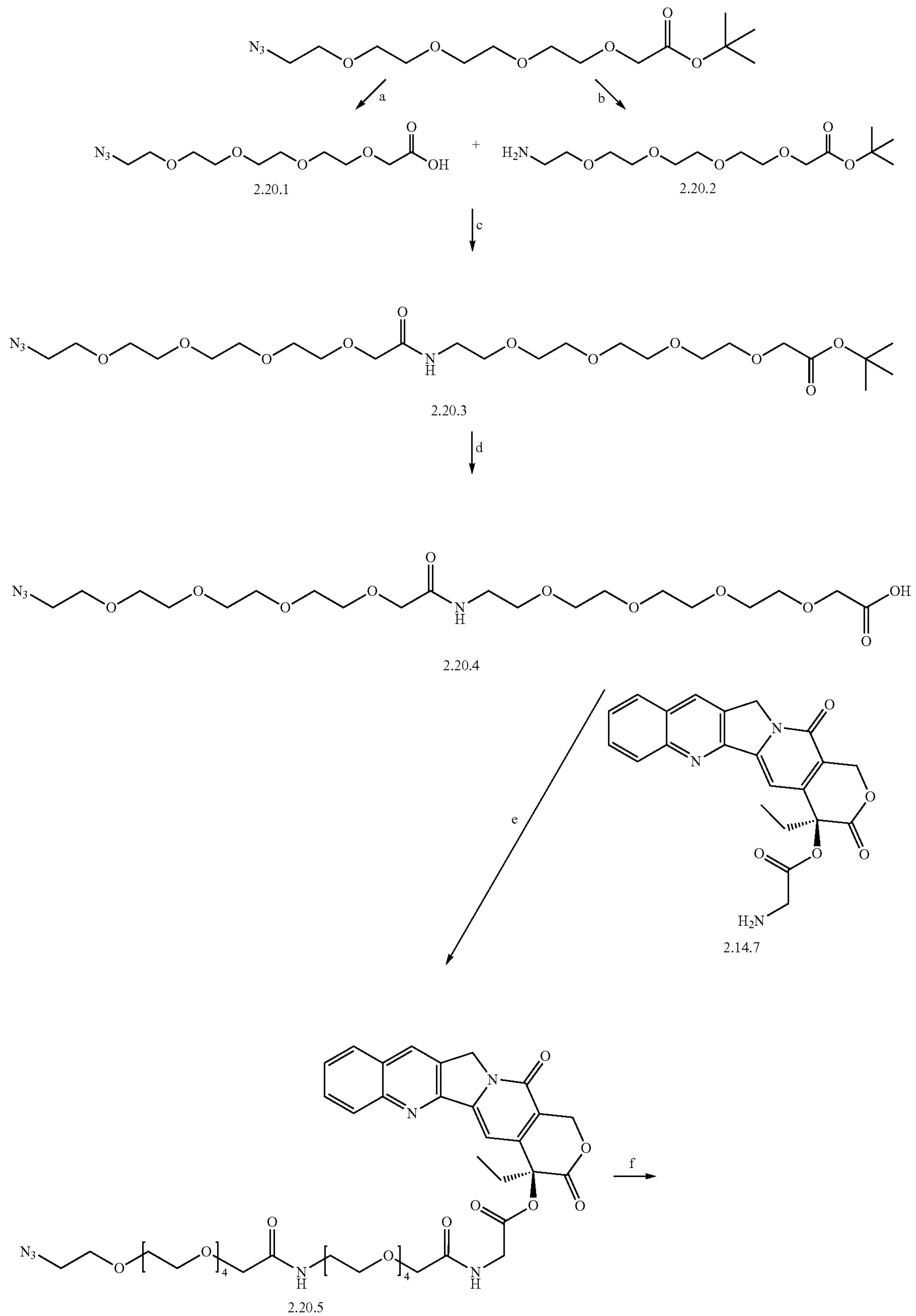
Scheme 8
