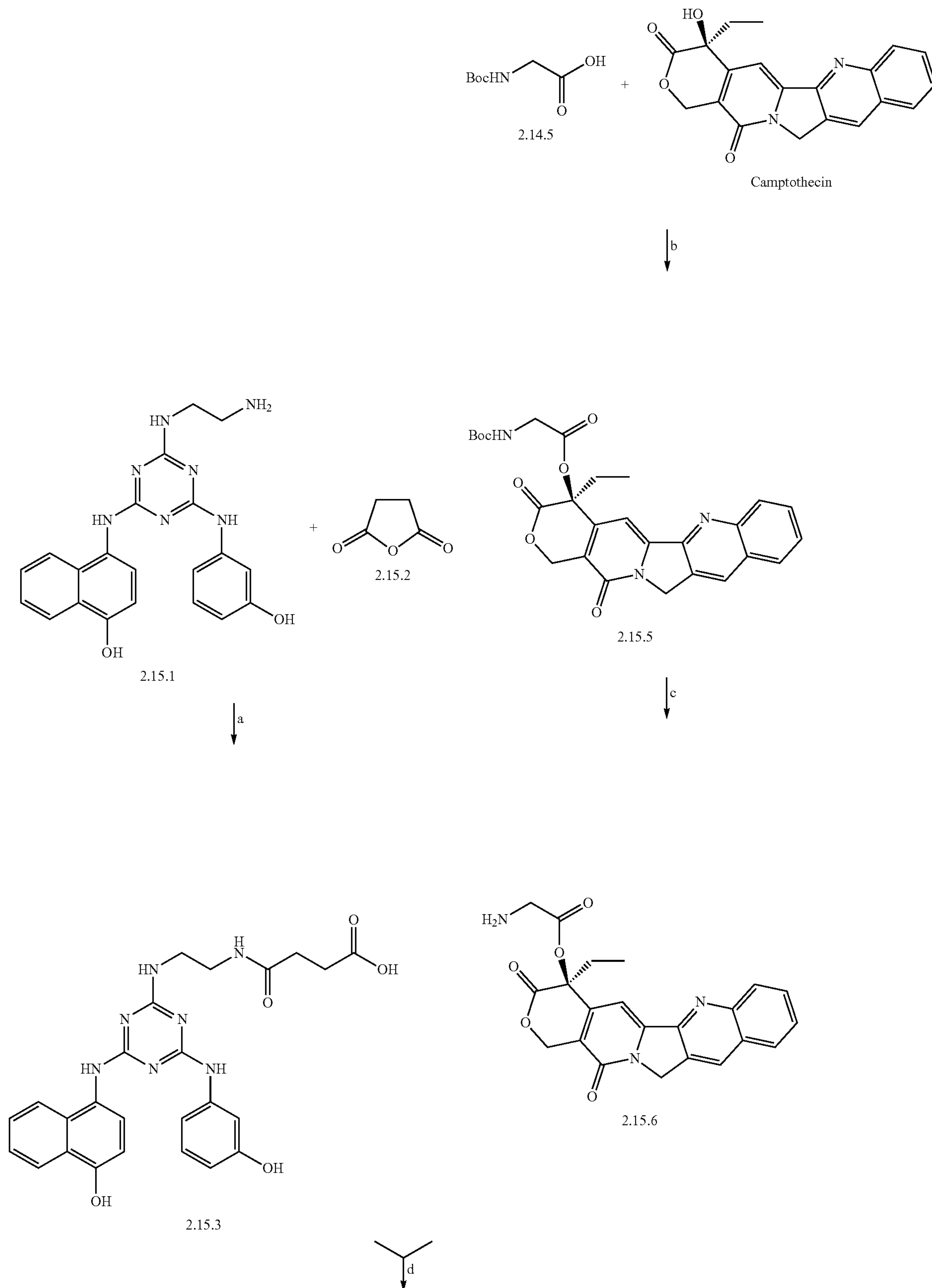
Scheme 3
