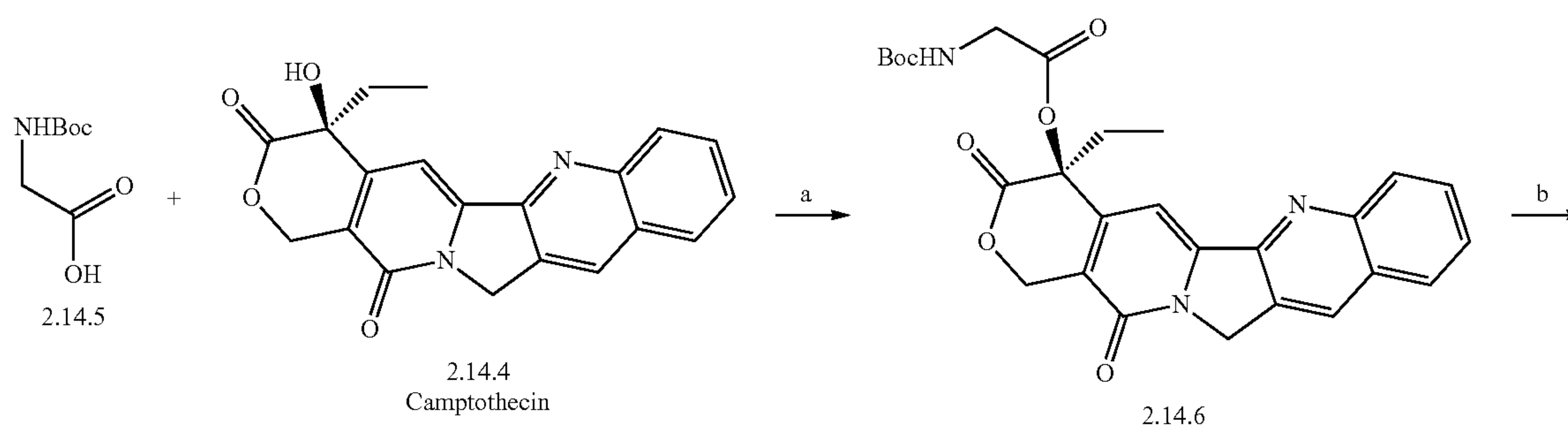
Scheme 2
