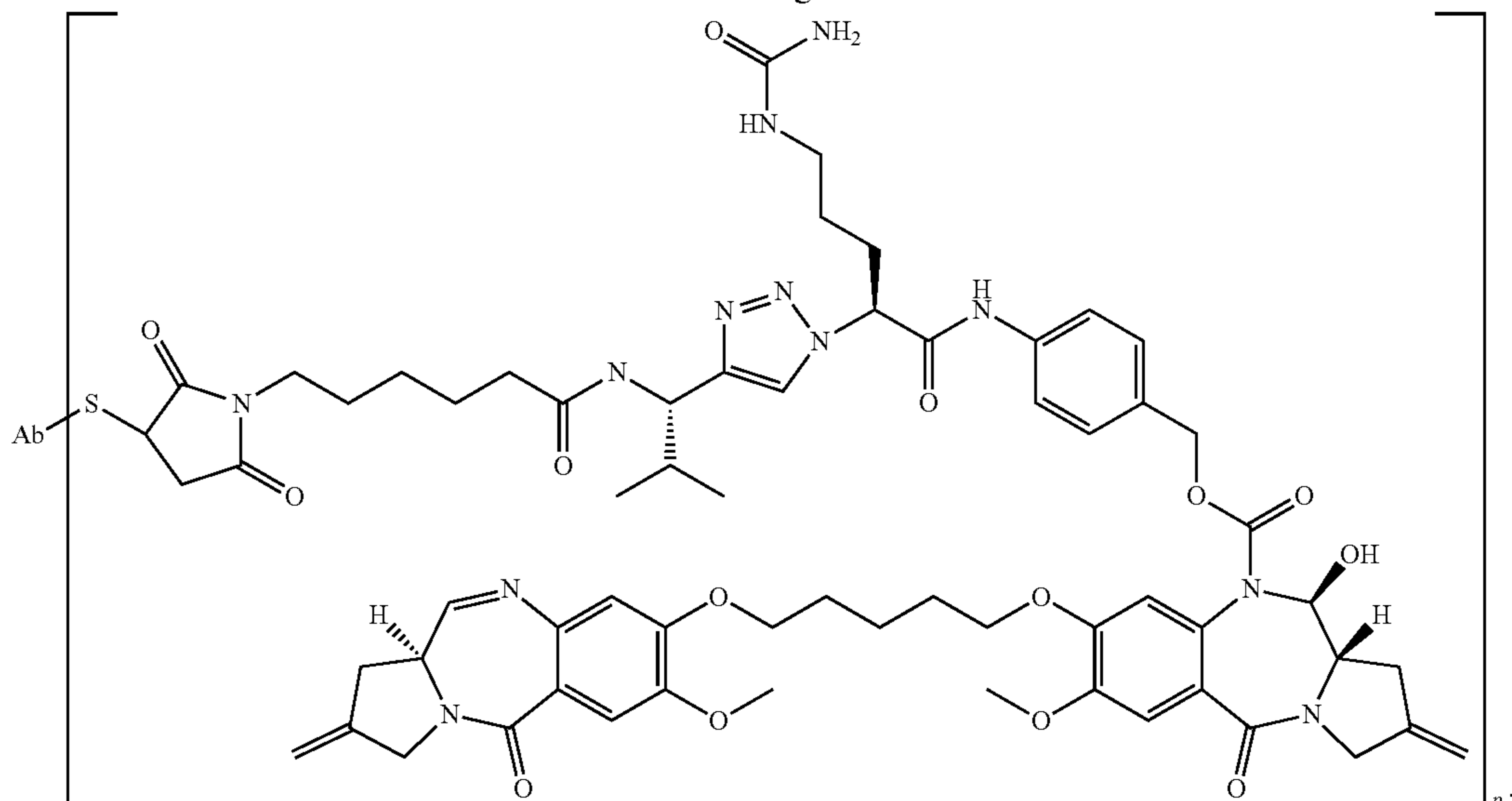
PBD dimer-PML-PAB-Ab
