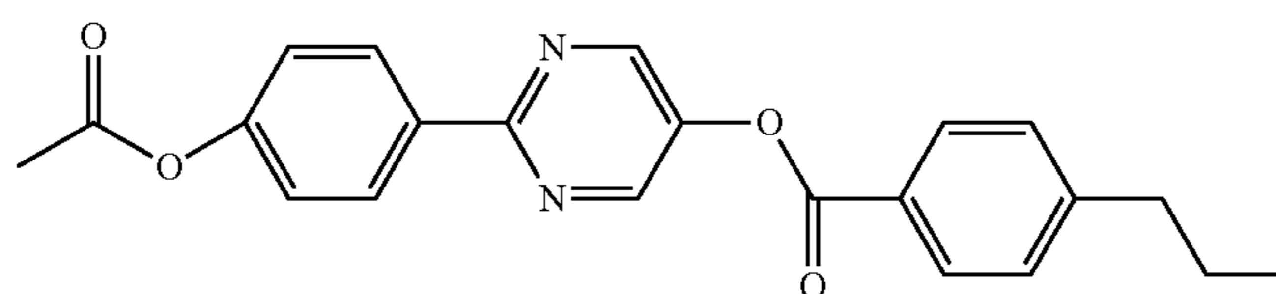
(8) {4-[2-(4'-methyl-biphenyl-4-carbonyloxy)-1,2-diphenyl-ethoxycarbonyl]-phenyl} ester
