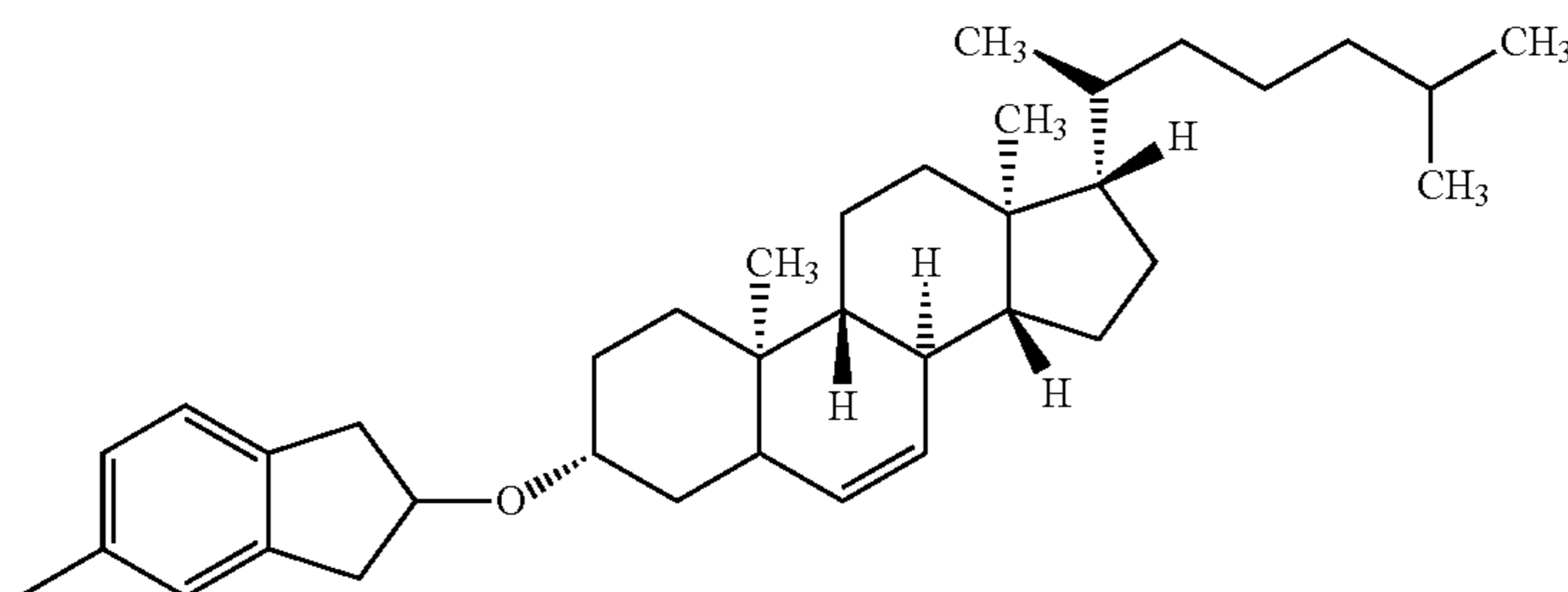
(15) 4-[17-(1,5-dimethyl-hexyl)-10,13-dimethyl-2,3,4,7,8,9,10,11,12,13,14,15,16,17-tetradecahydro-1H-cyclopenta[a]phenanthren-3-yloxy-carbonyloxy]-piperidin-1-yl
