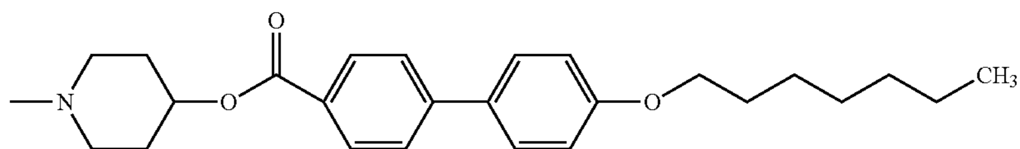
(31) 4-(4-butyl-phenylcarbonyloxy)-piperidin-1-yl
