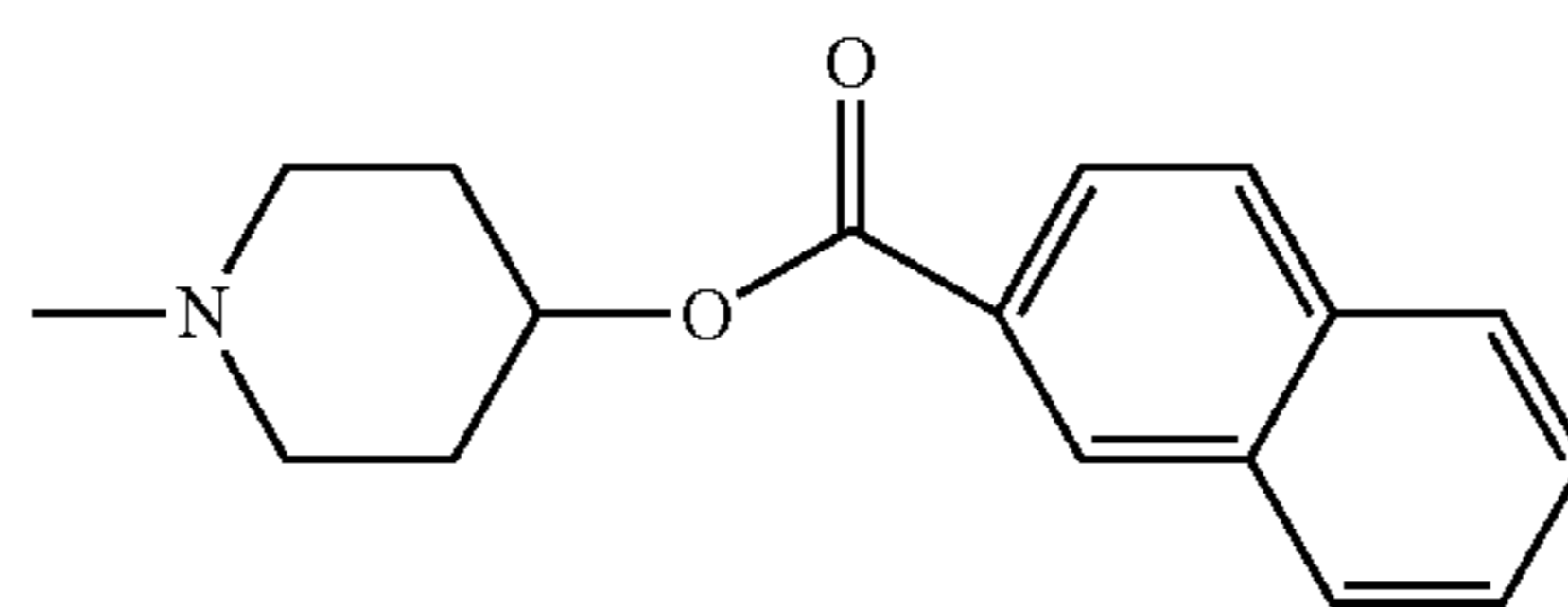
(18) 4-hydroxy-piperidin-1-yl
