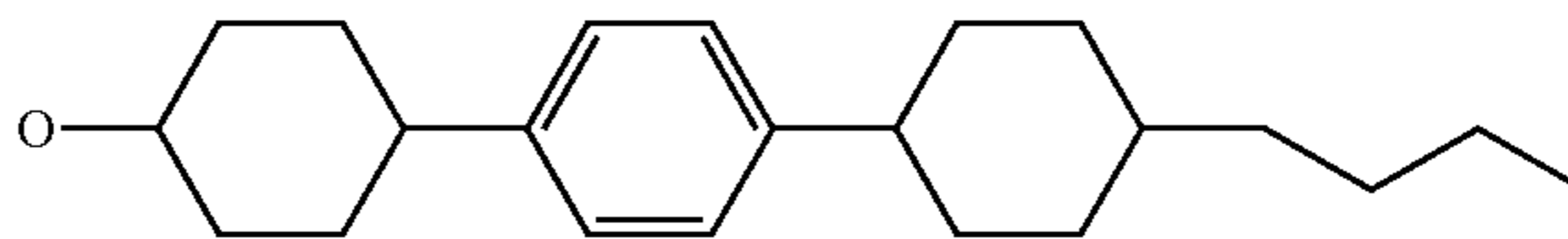
(2) 4''-butyl-[1,1';4',1'']tercyclohexan-4-yloxy
