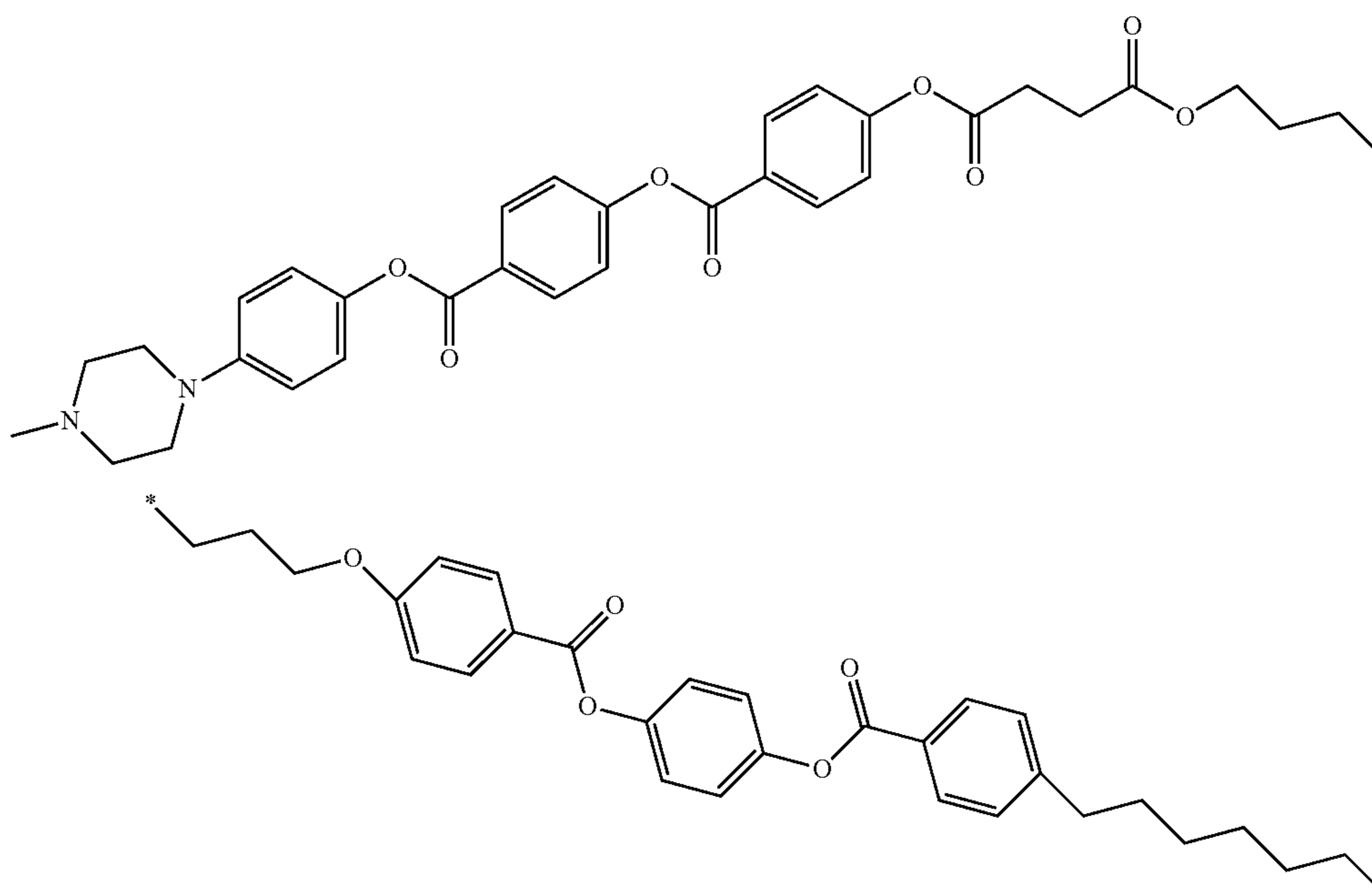
(11) {4-[4-(4-{4-[4-(4-nonyl-benzoyloxy)-benzoyloxy]-benzoyloxy}-benzoyloxy)-phenyl]-piperazin-1-yl}
