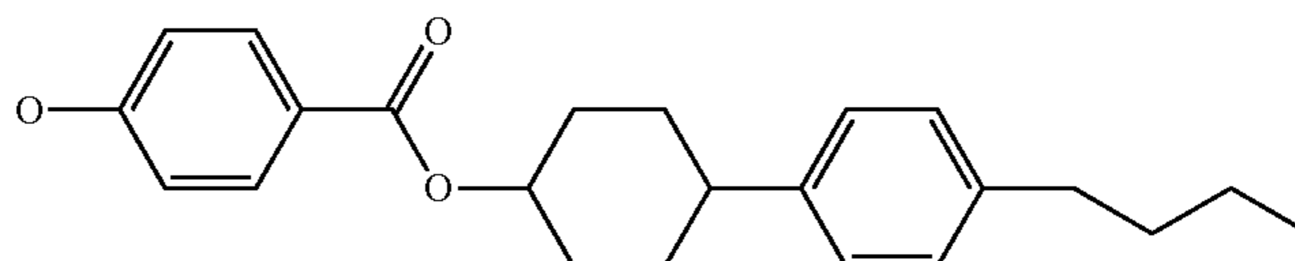
(4) 4'-(4-butyl-benzoyloxy)-biphenyl-4-carbonyloxy
