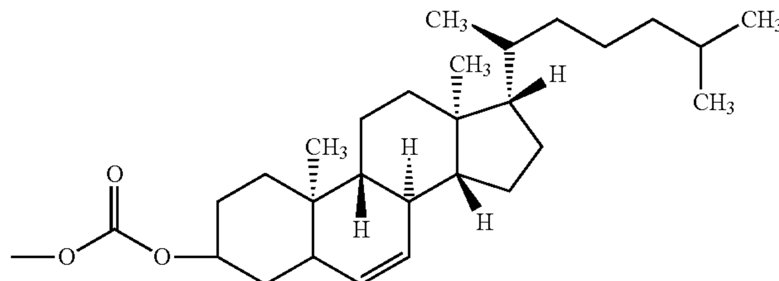
(37) 4-[17-(1,5-dimethyl-hexyl)-10,13-dimethyl-2,3,4,7,8,9,10,11,12,13,14,15,16,17-tetradecahydro-1H-cyclopenta[a]phenanthren-3-yl]oxy-carbonyloxy
