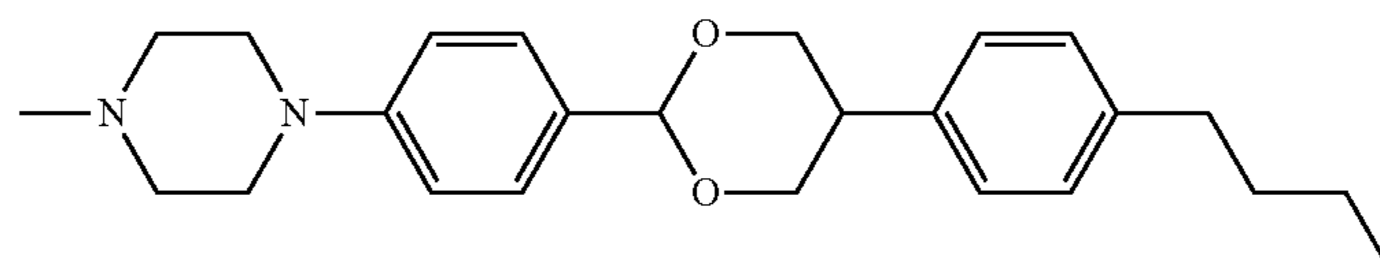
(36) 4-(7-(4-propylphenylcarbonyloxy)bicyclo[3.3.0]oct-2-yl)oxycarbonyl)phenyl
