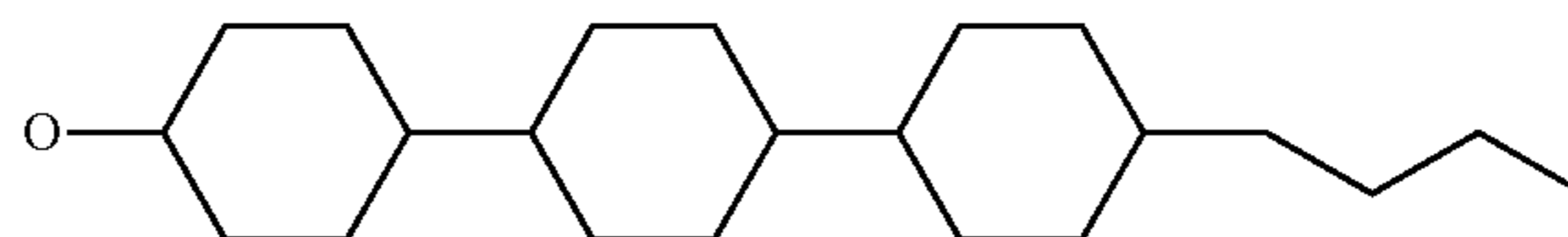
(3) 4-[4-(4-butyl-phenyl)-cyclohexyloxy]carbonyl]-phenoxy
