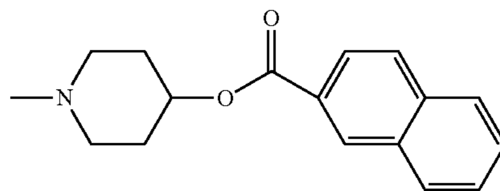
(18) 4-hydroxy-piperidin-1-yl
