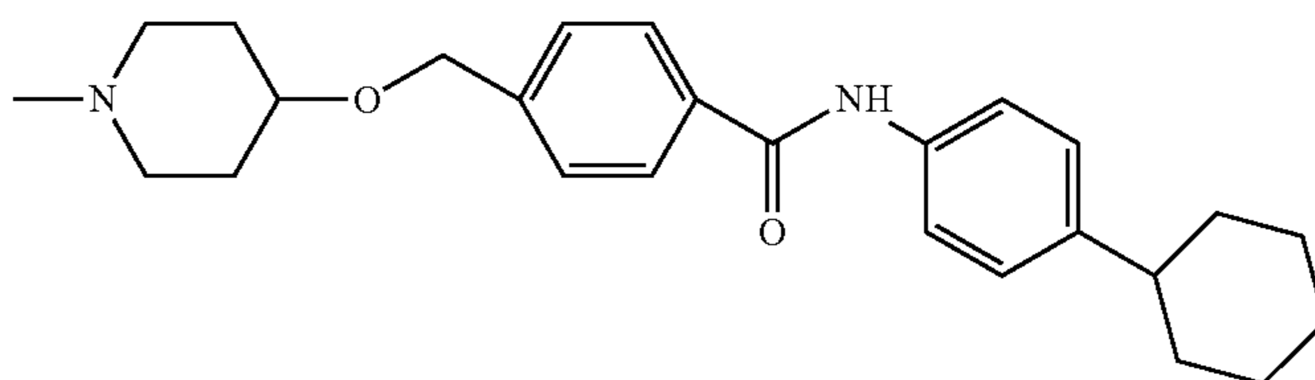
(26) 4-[4-(4-cyclohexyl-phenyl-carbamoyl)-benzoyloxy]-piperidin-1-yl
