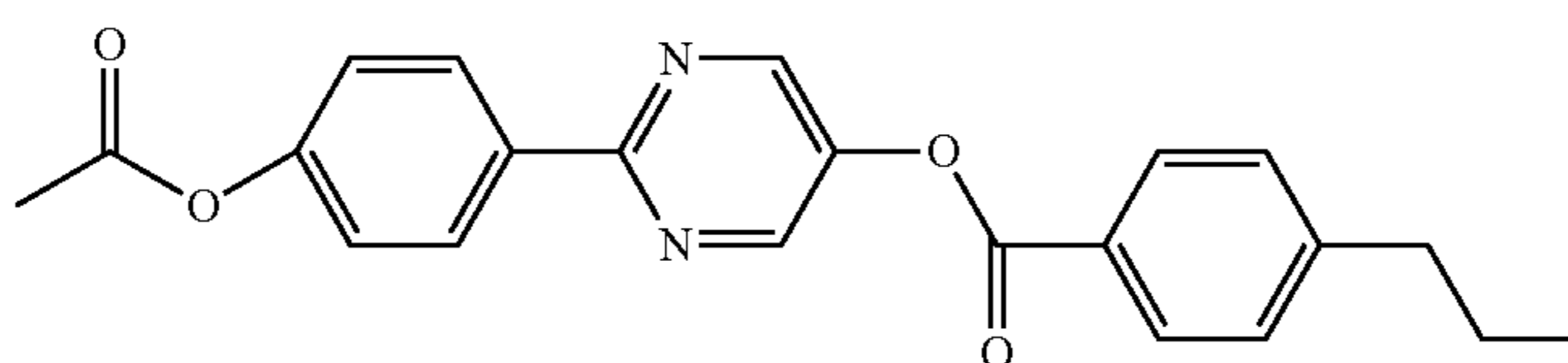
(8) {4-[2-(4'-methyl-biphenyl-4-carbonyloxy)-1,2-diphenyl-ethoxycarbonyl]-phenyl} ester
