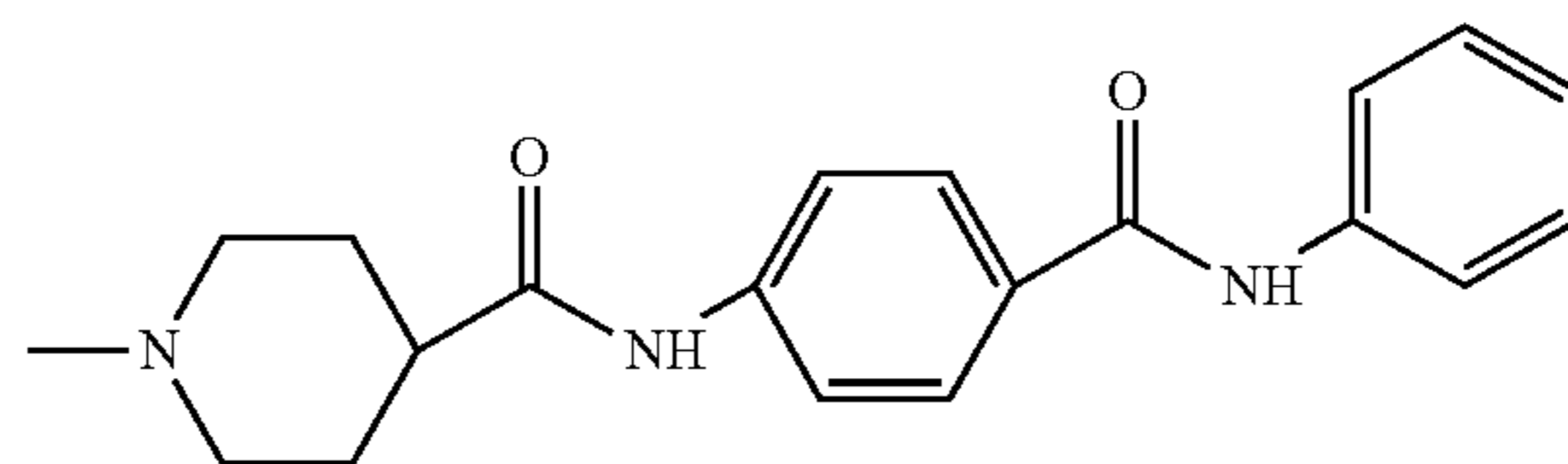
(20) 4-(4-(4-phenylpiperidin-1-yl)- benzoyloxy)-piperidin-1-yl
