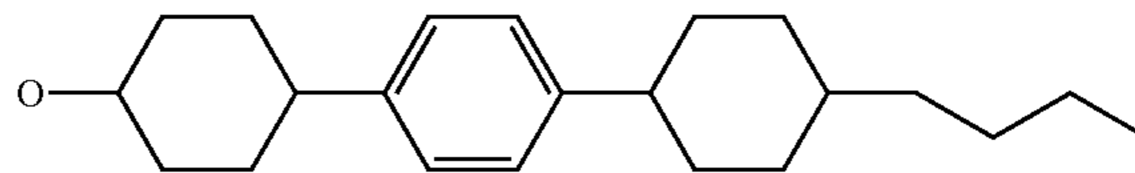
(2) 4''-butyl-[1,1';4',1'']tercyclohexan-4-yloxy
