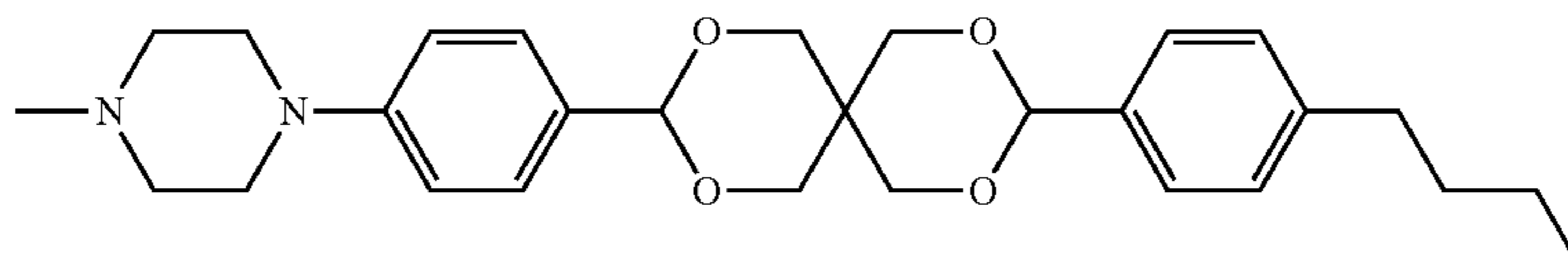
(34) 4-(6-(4-butylphenyl)carbonyloxy-(4,8-dioxabicyclo[3.3.0]oct-2-yl)oxycarbonyl)phenyl
