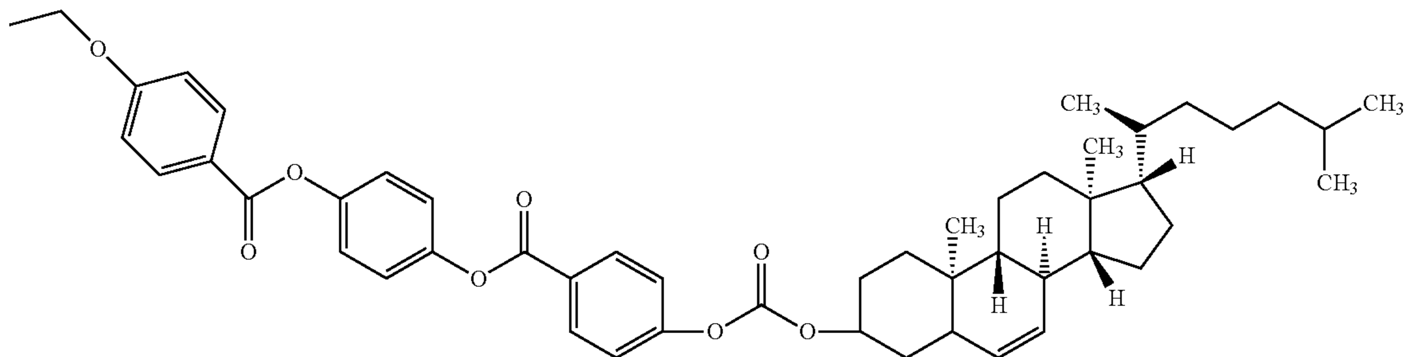
(25) 4-[4-(4-cyclohexyl-phenyl-carbamoyl)-benzyloxy]-piperidin-1-yl
