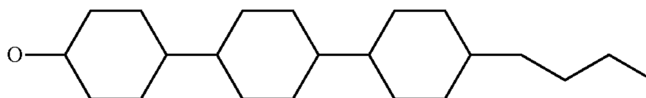
(3) 4-[4-(4-butyl-phenyl)-cyclohexyloxy-carbonyl]-phenoxy
