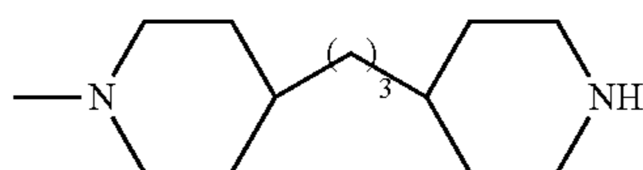
(29) 4-(4-hexyloxy-benzoyloxy)-piperidin-1-yl
