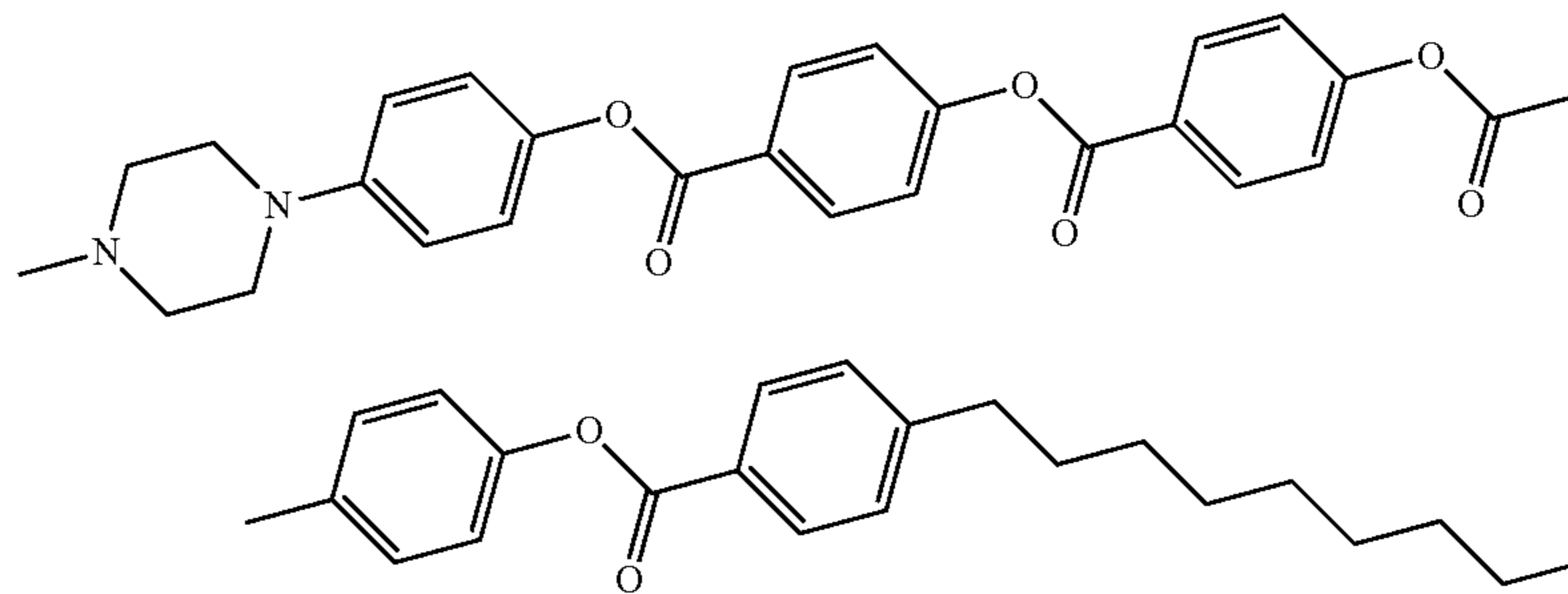
(12) 4-(4'-propyl-biphenyl-4-ylethynyl)-phenyl
