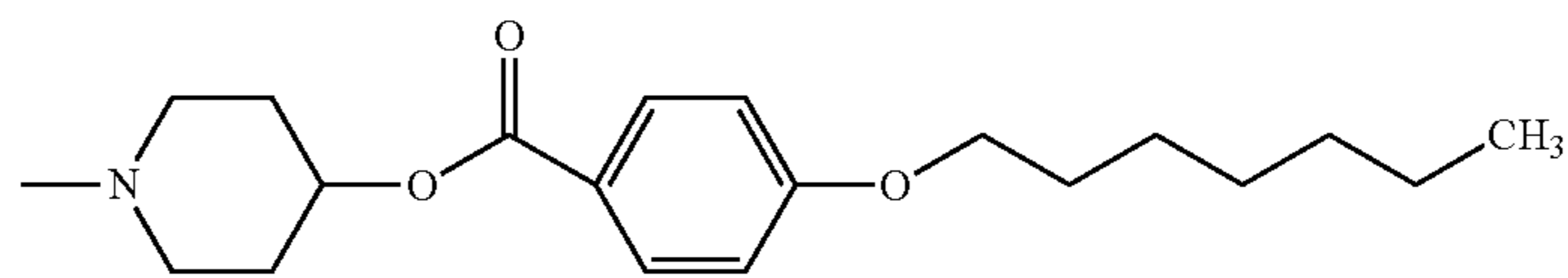
(30) 4-(4'-hexyloxy-biphenyl-4-carbonyloxy)-piperidin-1-yl
