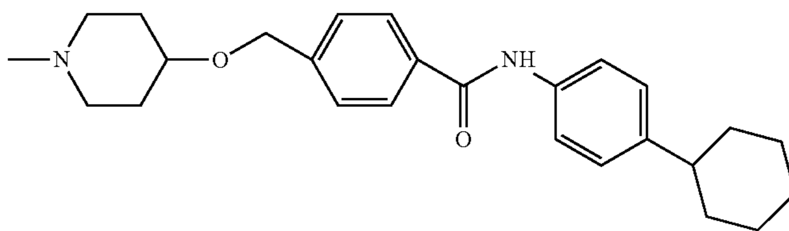
(26) 4-[4-(4-cyclohexyl-phenyl-carbamoyl)-benzoyloxy]-piperidin-1-yl
