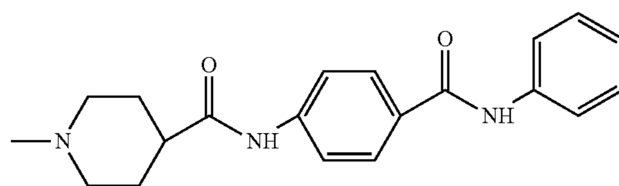
(20) 4-(4-(4-phenylpiperidin-1-yl)- benzoyloxy)-piperidin-1-yl
