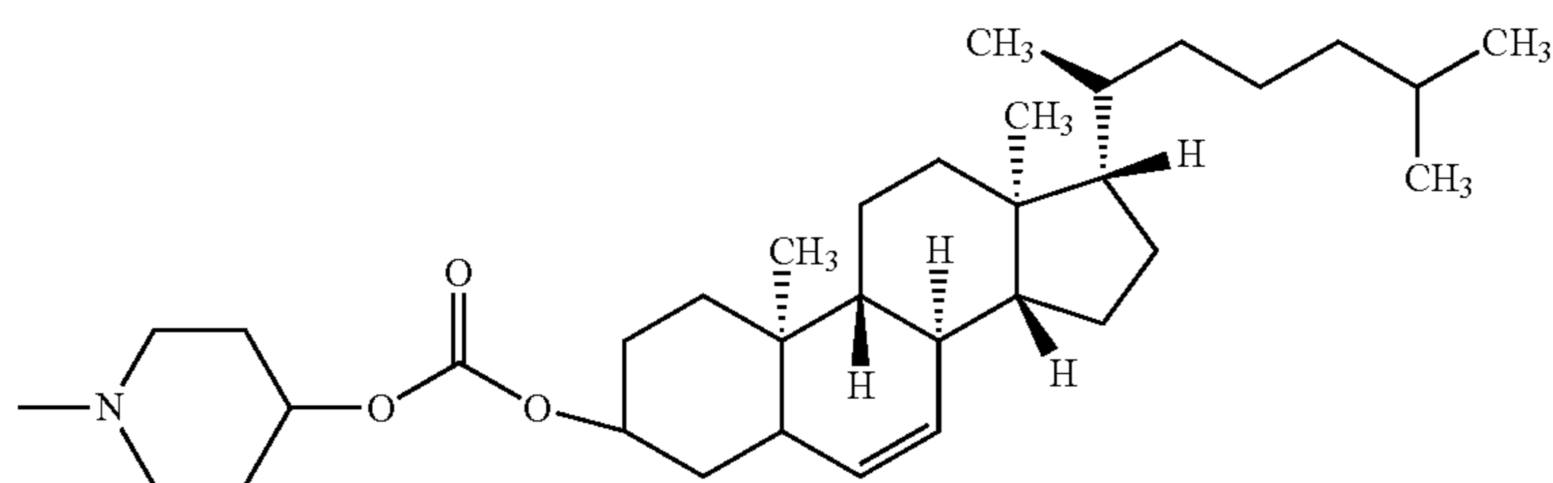
4-[17-(1,5-dimethyl-hexyl)-10,13-dimethyl-2,3,4,7,8,9,10,11,12,13,14,15,16,17-tetradecahydro-1H-cyclopenta[a]phenanthren-3-yloxy-carbonyloxy]-piperidin-1-yl
