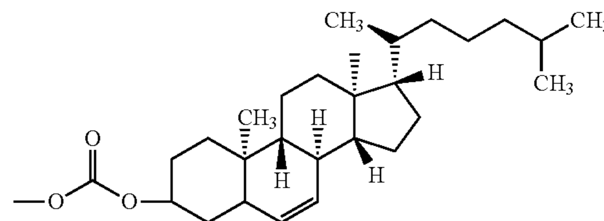
4-[17-(1,5-dimethyl-hexyl)-10,13-dimethyl- 2,3,4,7,8,9,10,11,12,14,14,15,16,17- tetradecahydro-1H-cyclopenta[a] phenanthren-3-yloxy]carbonyloxy
