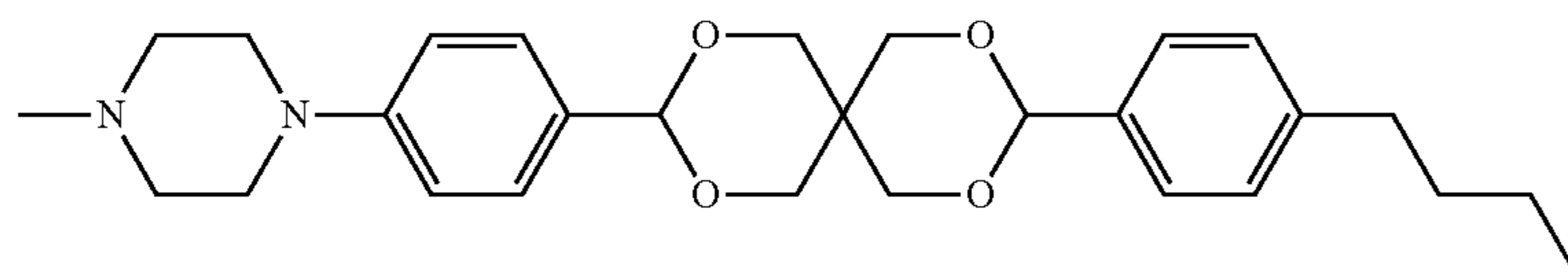
4-(4-(9-(4-butylphenyl)-2,4,8,10-tetraoxaspiro [5.5]undec-3-yl)phenyl)piperazin-1-yl
