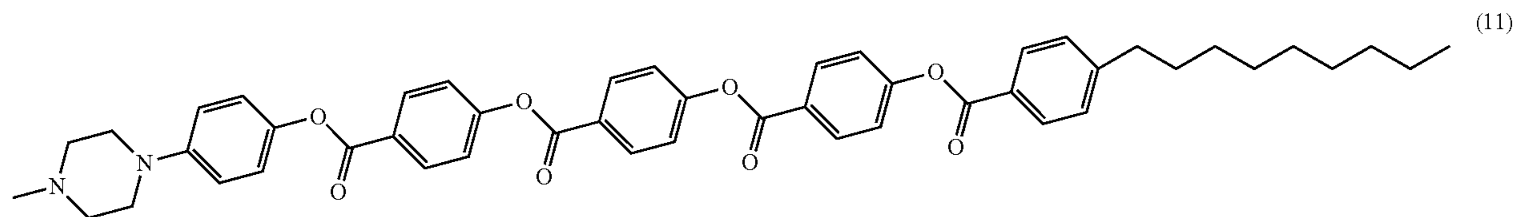
(4-[4-(4-{4-[4-(4-nonyl-benzoyloxy)-benzoyloxy]-benzoyloxy]-benzoyloxy}-phenyl]-piperazin-1-yl)
