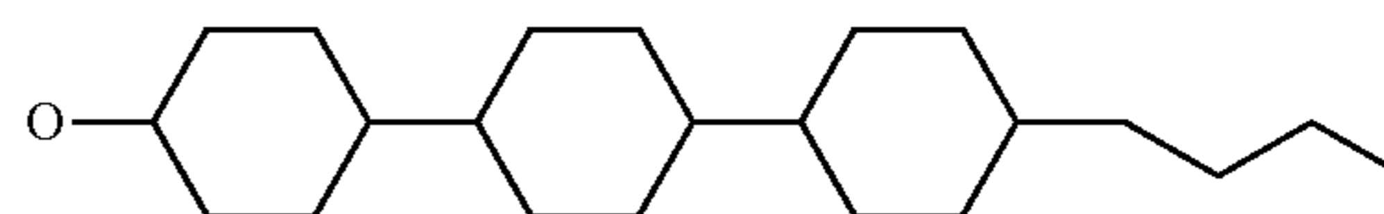
4''-butyl-[1,1';4',1'']tercyclohexan-4-yloxy
