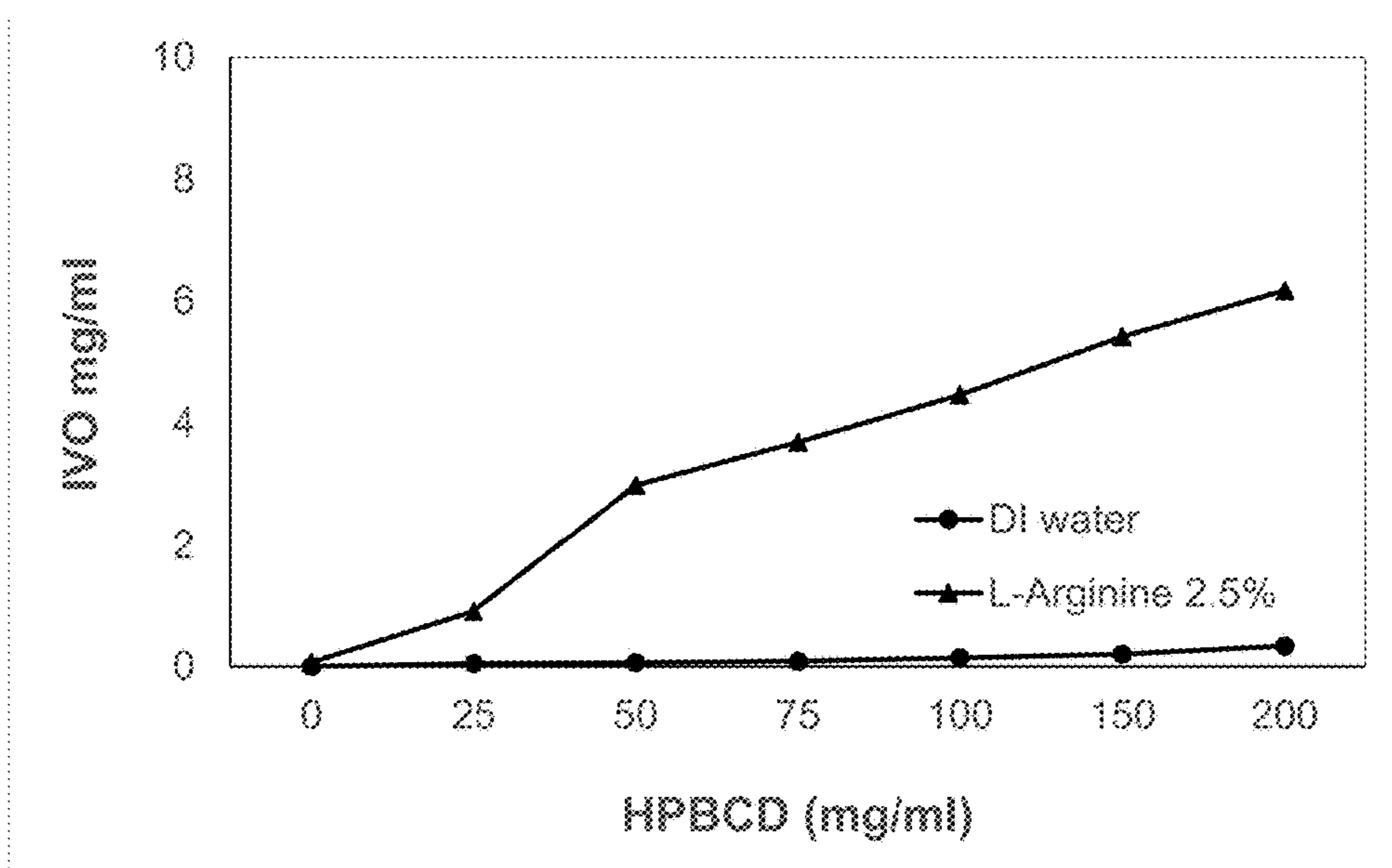
Figure 4. Effect of HPBCD on the solubility of IVO in 2.5% L-ARG solution
