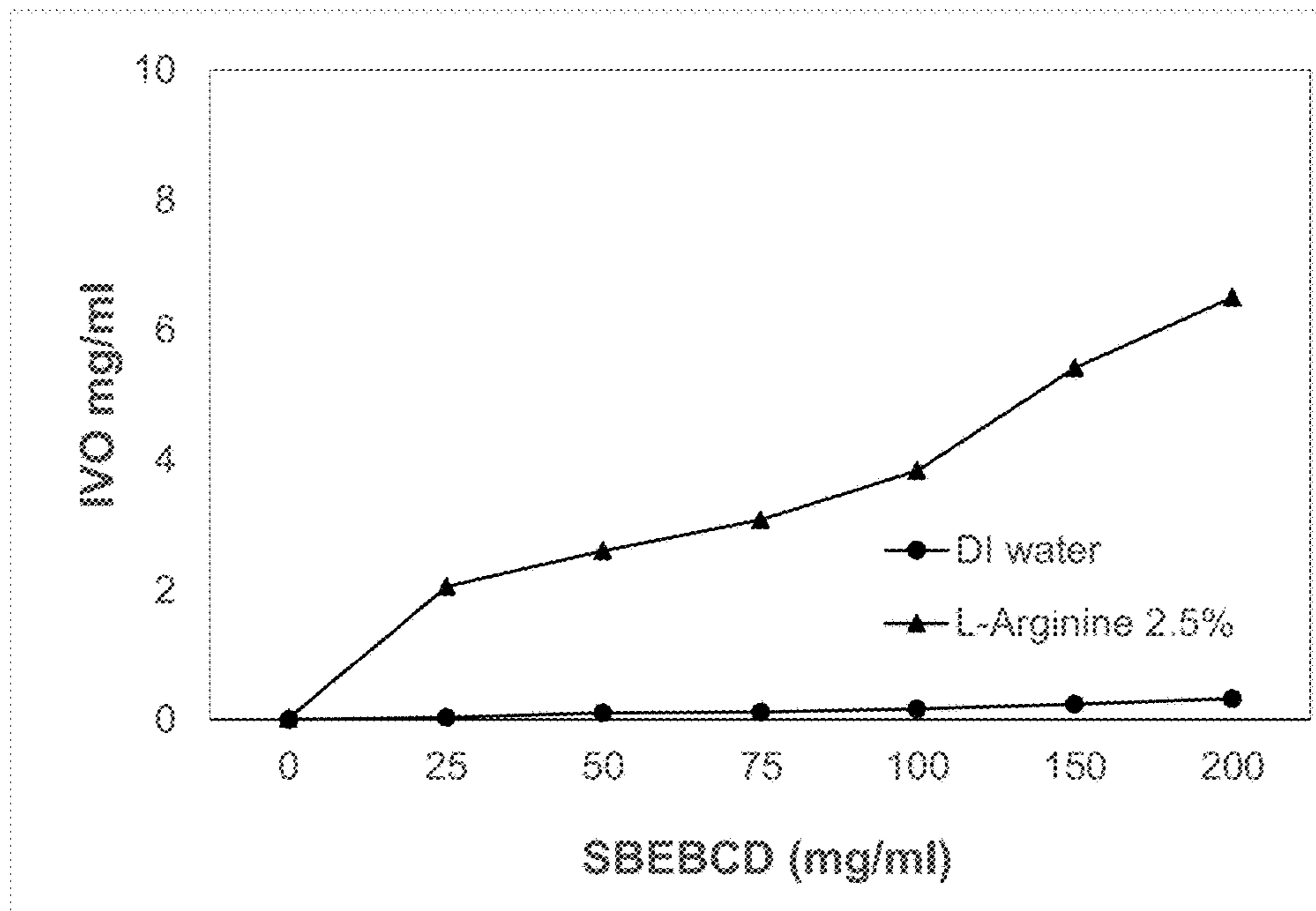
Figure 5. Effect of SBEB CD on the solubility of IVO in 2.5% L-ARG solution
