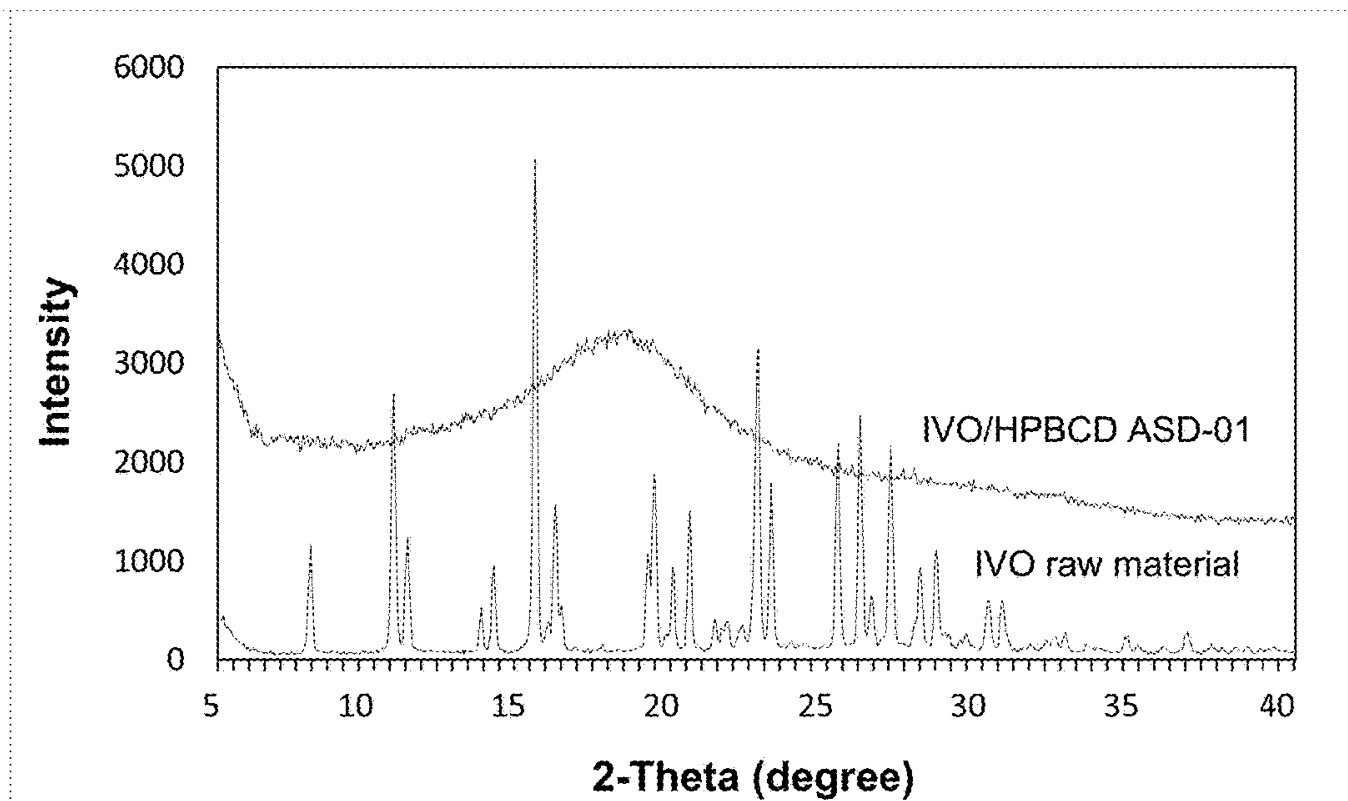
Figure 2. XRPD of raw material and IVO/HPBCD ASD-01
