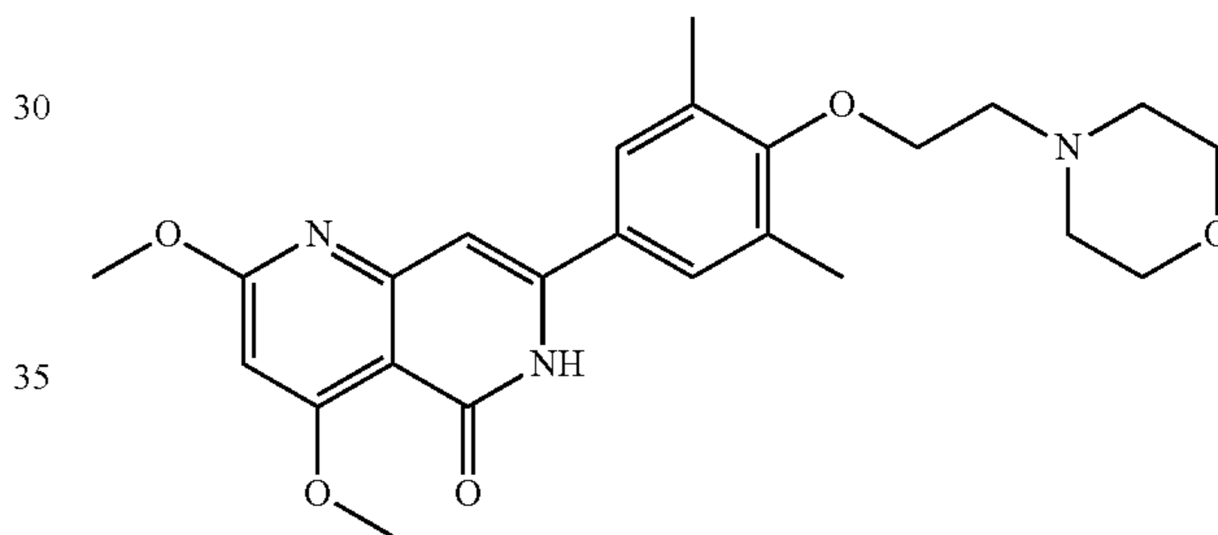
7-(3,5-dimethyl-4-(2-morpholinoethoxy)phenyl)-2,4-dimethoxy-1,6-naphthyridin-5(6H)-one
