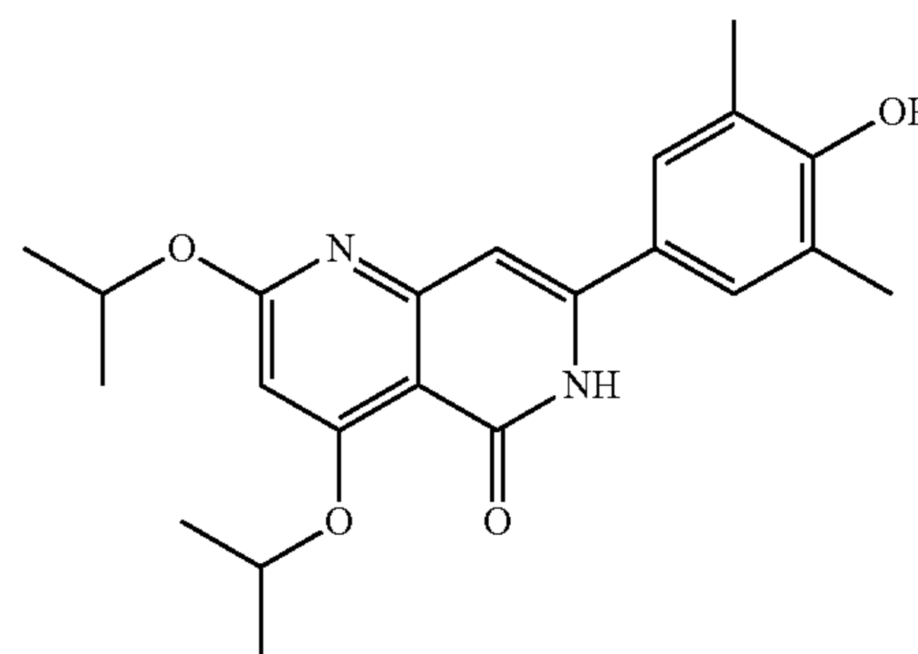
7-(4-hydroxy-3,5-dimethylphenyl)-2,4-diisopropoxy-1,6-naphthyridin-5(6H)-one
