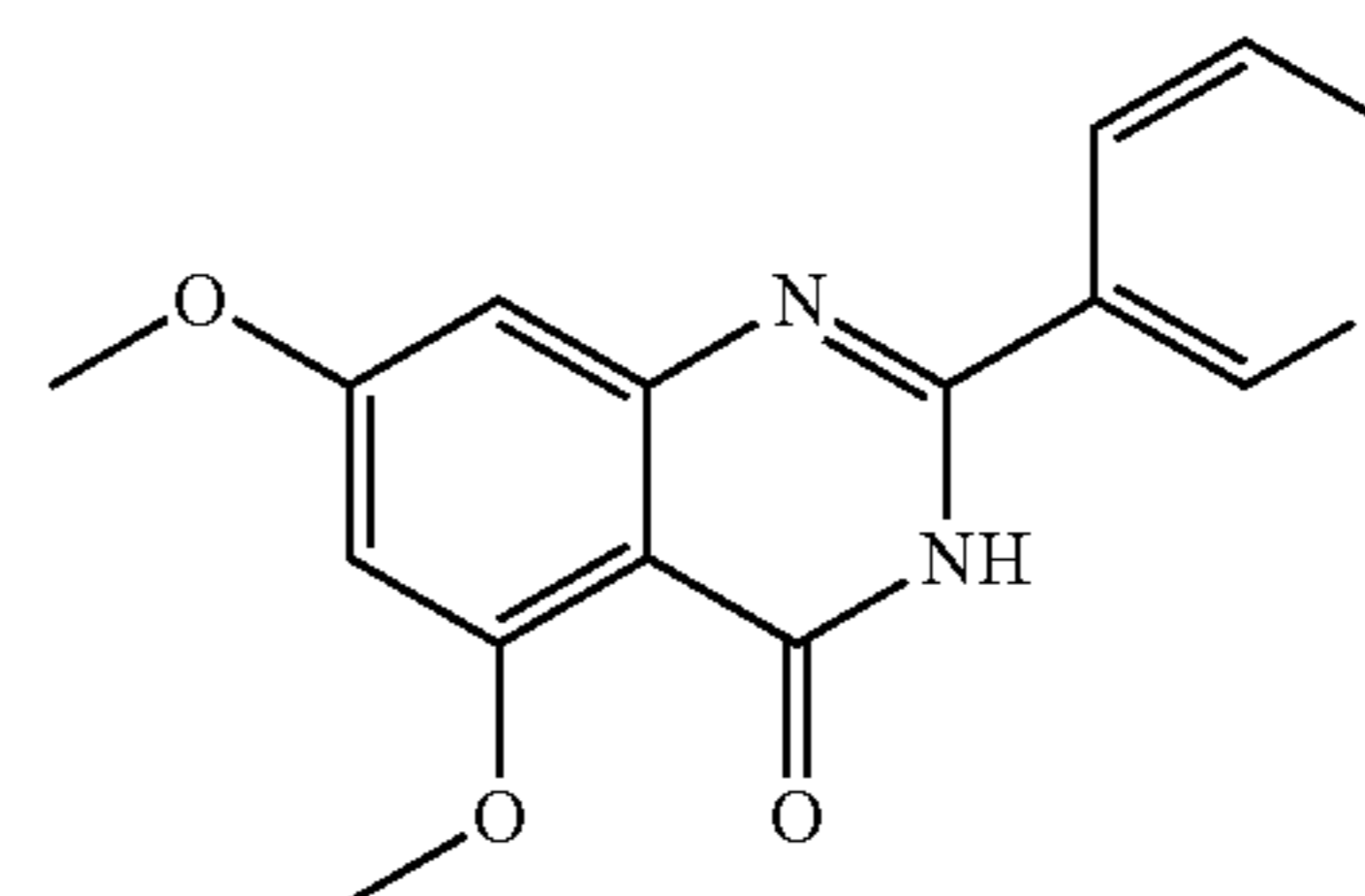
5,7-dimethoxy-2-(pyridin-3-yl)quinazolin-4(3H)-one
