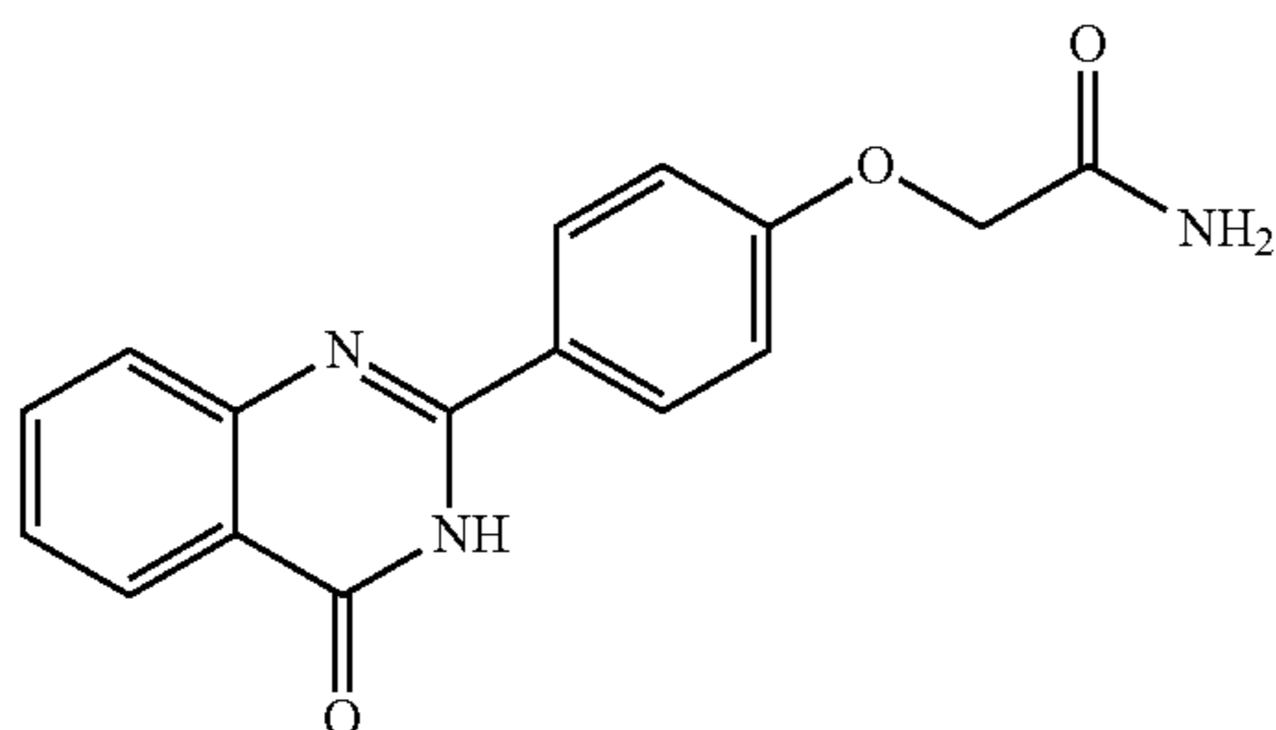
2-(4-(4-oxo-3,4-dihydroquinazolin-2-yl)phenoxy)acetamide
