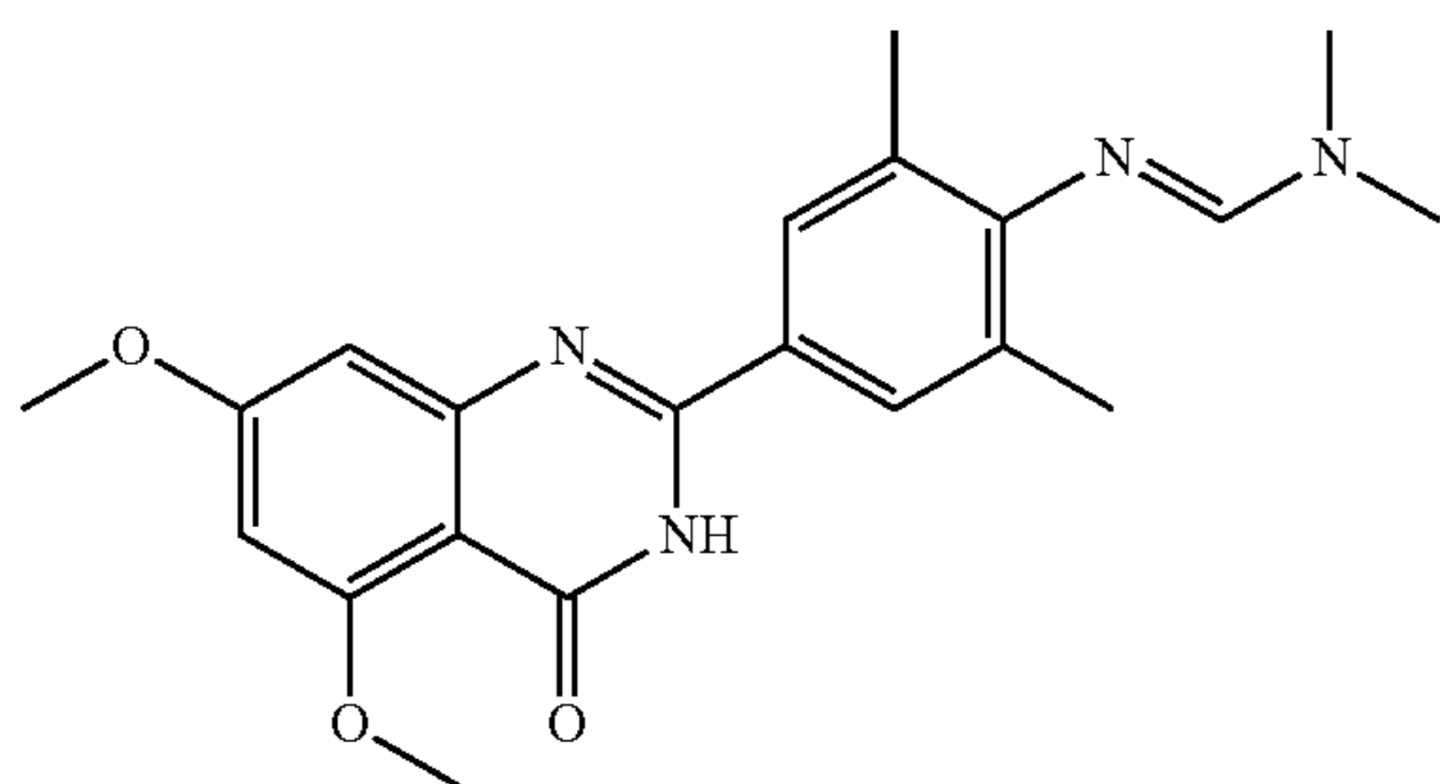
(E)-N'-(4-(5,7-dimethoxy-4-oxo-3,4-dihydroquinazolin-2-yl)-2,6-dimethylphenyl)-N,N-dimethylformimidamide
