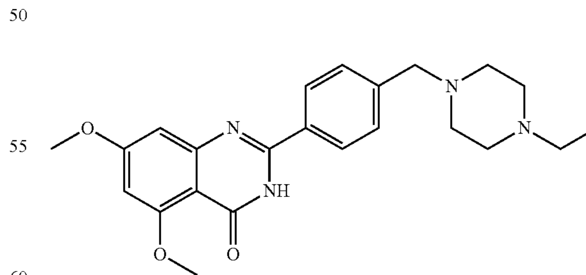
2-(4((4-ethylpiperazin-1-yl)methyl)phenyl)-5,7-dimethoxyquinazolin-4(3H)-one
