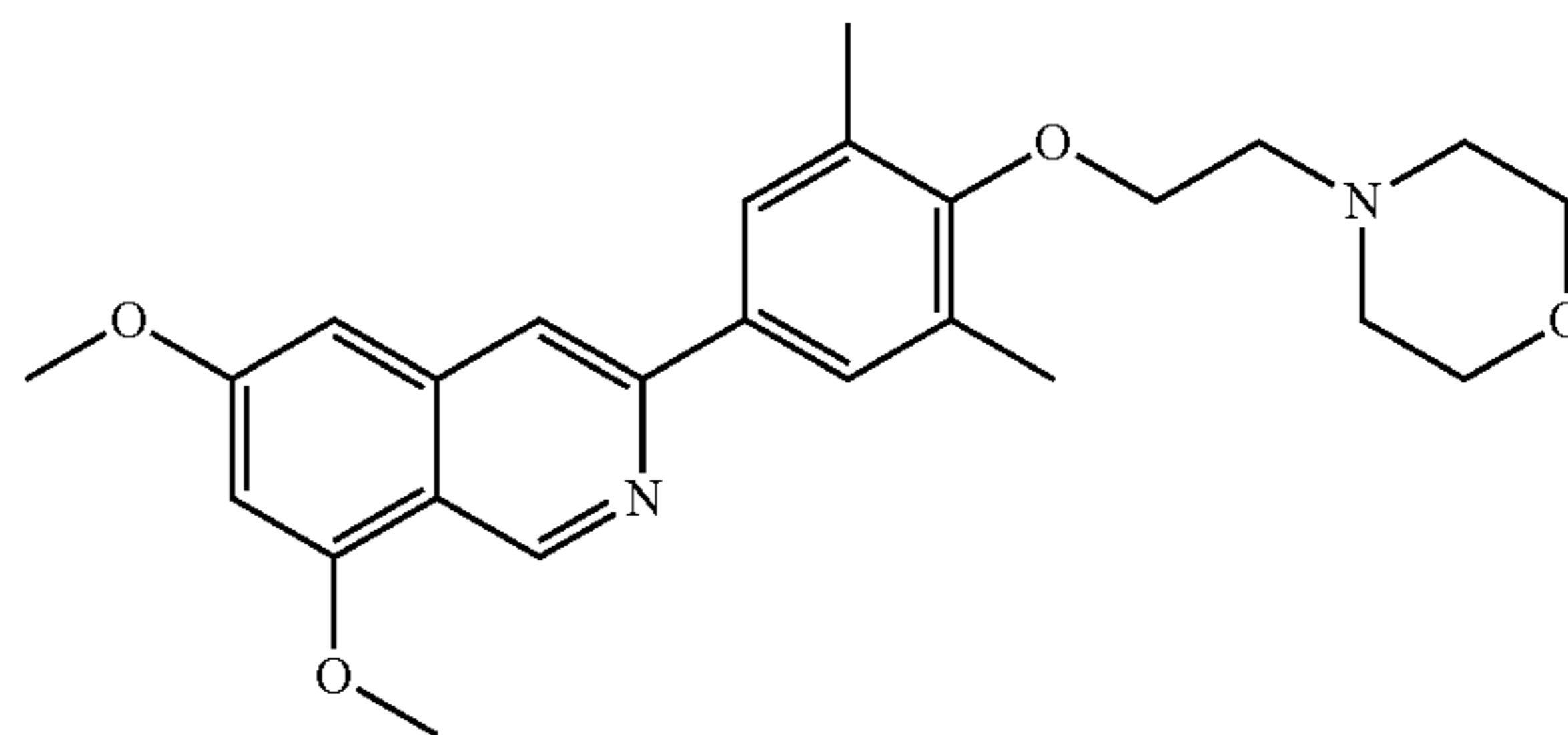
4-(2-(4-(6,8-dimethoxyisoquinolin-3-yl)-2,6-dimethylphenoxy)ethyl)morpholine
