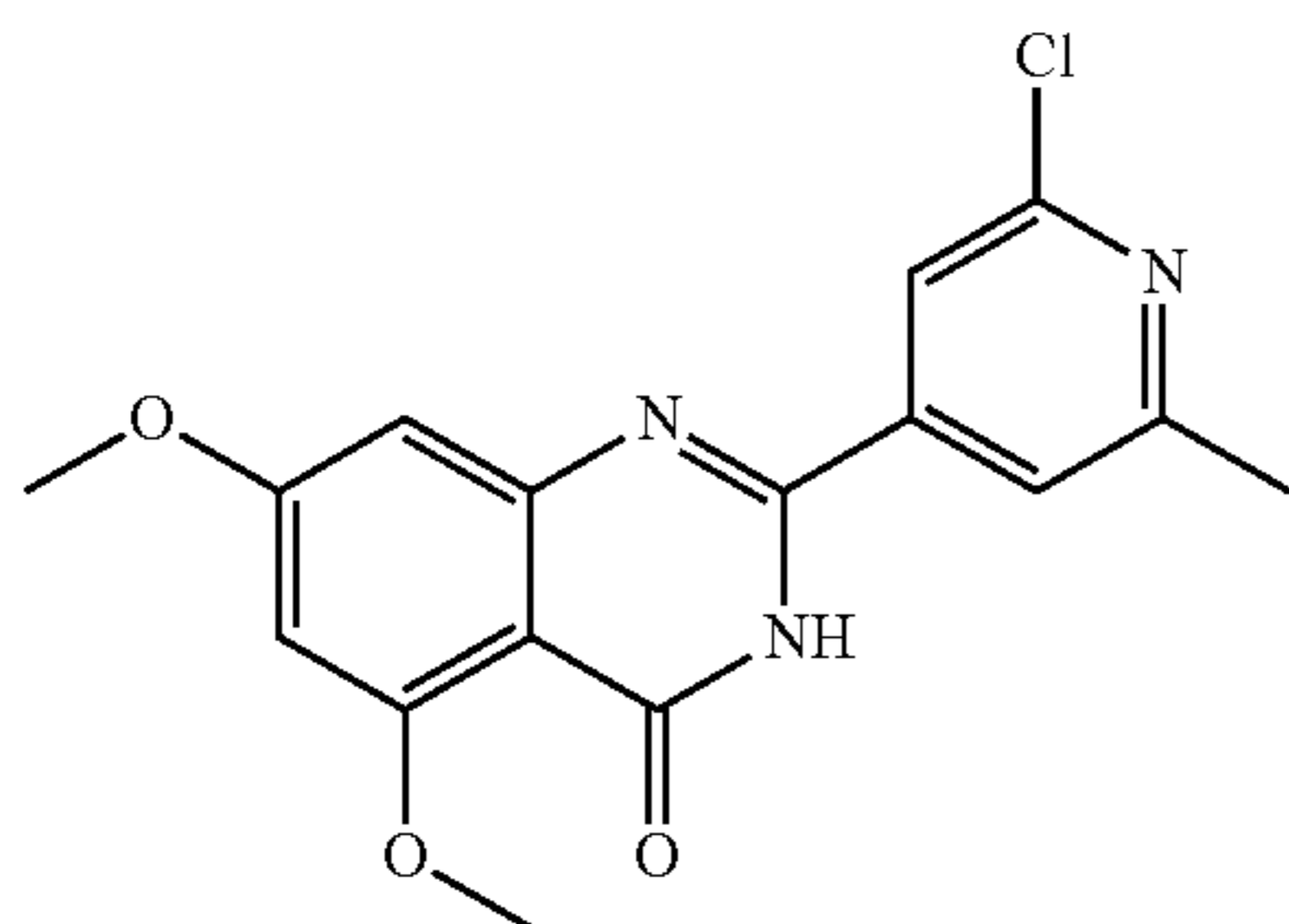
2-(2-chloro-6-methylpyridin-4-yl)-5,7-dimethoxyquinazolin-4(3H)-one
