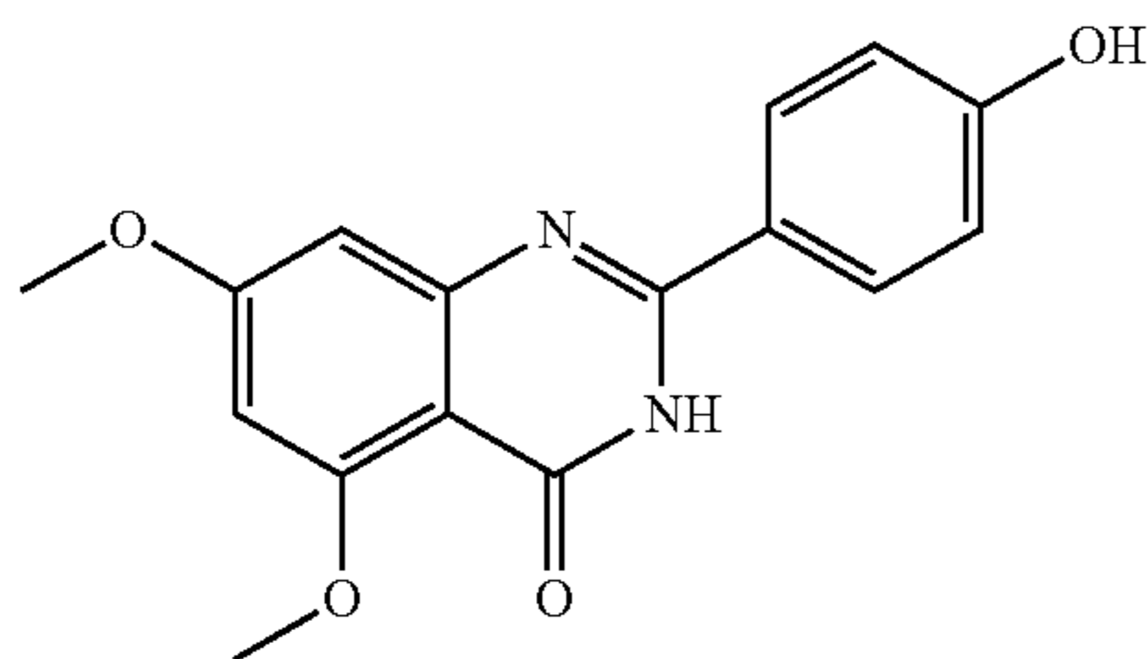
2-(4-hydroxyphenyl)-5,7-dimethoxyquinazolin-4(3H)-one
