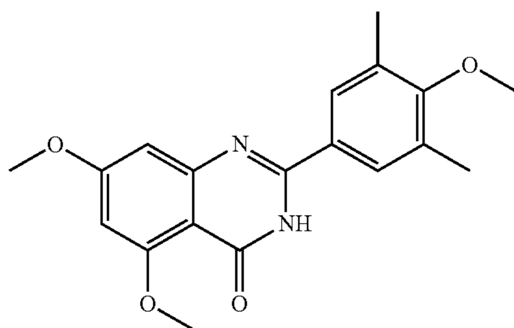
5,7-dimethoxy-2-(4-methoxy-3,5-dimethylphenyl)quinazolin-4(3H)-one
