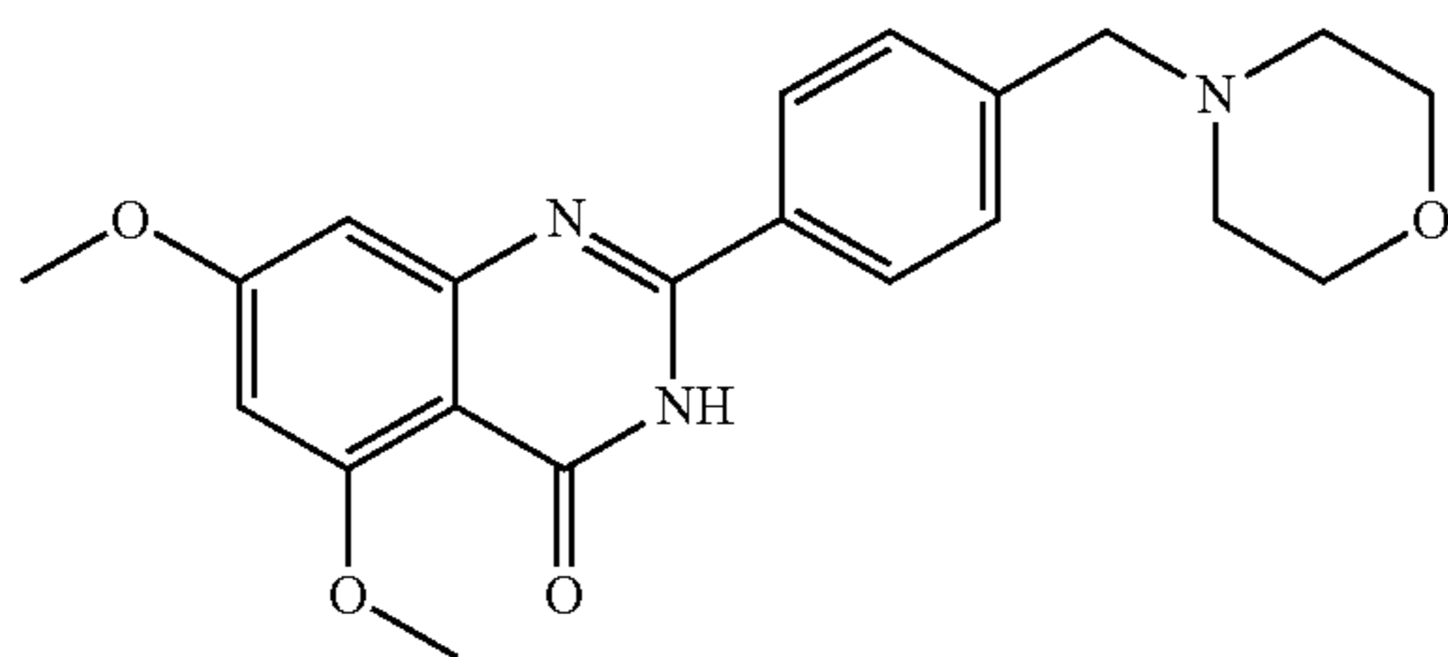
5,7-dimethoxy-2-(4-(morpholinomethyl)phenyl)quinazolin-4(3H)-one
