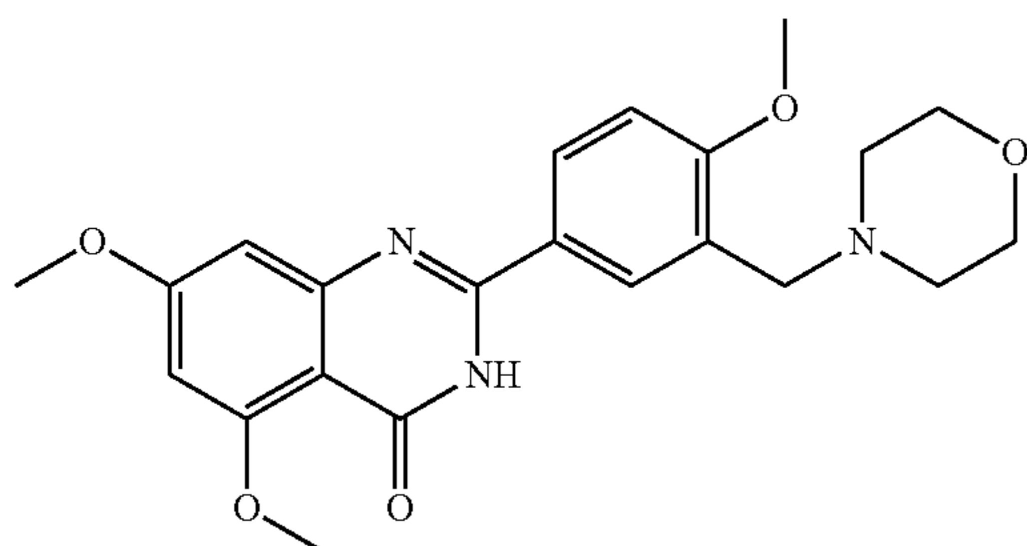
5,7-dimethoxy-2-(4-methoxy-3-(morpholinomethyl)phenyl)quinazolin-4(3H)-one
