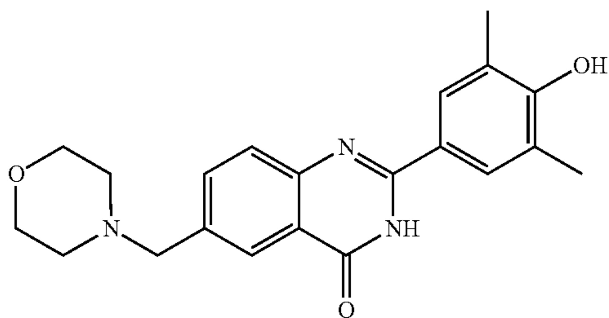
2-(4-hydroxy-3,5-dimethylphenyl)-6-(morpholinomethyl)quinazolin-4(3H)-one
