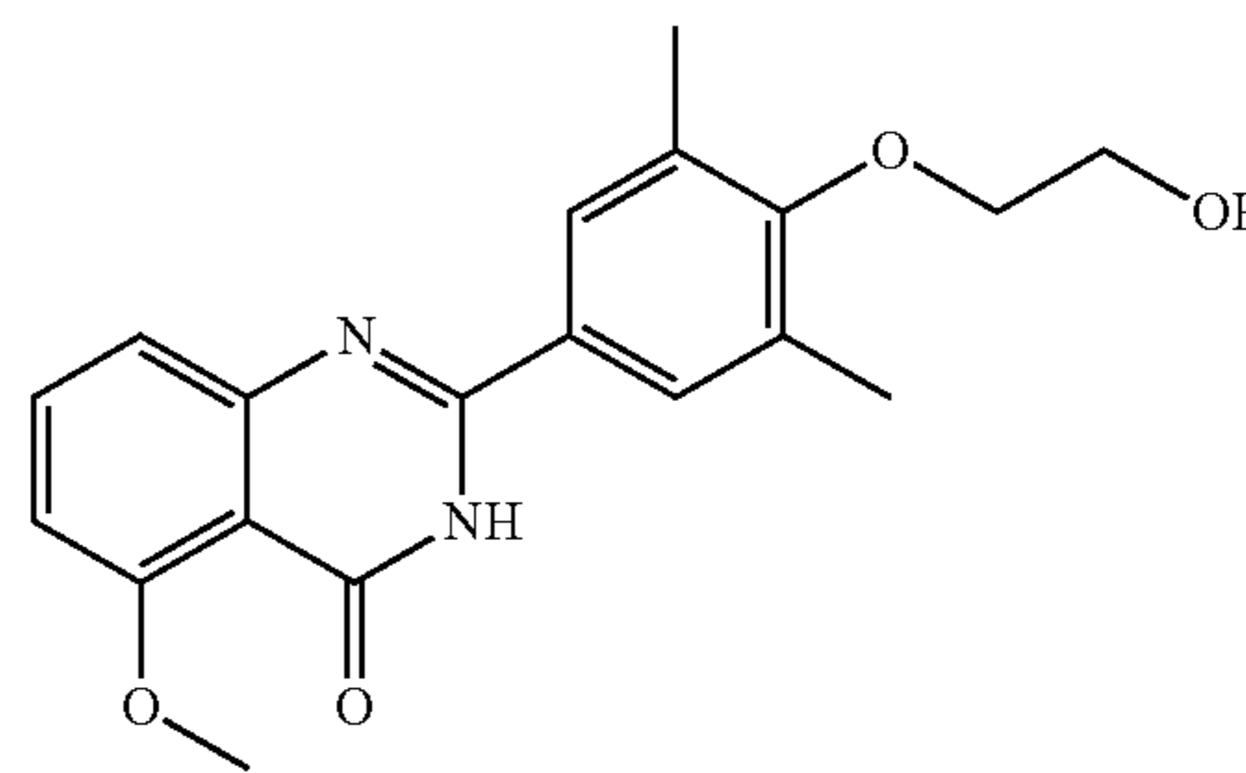
2-(4-(2-hydroxyethoxy)-3,5-dimethylphenyl)-5-methoxyquinazolin-4(3H)-one
