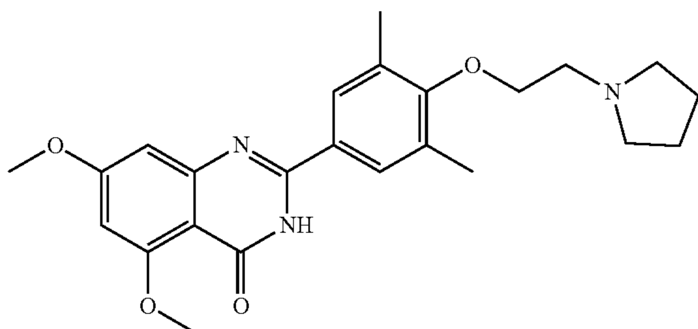
2-(3,5-dimethyl-4-(2-(pyrrolidin-1-yl)ethoxy)phenyl)-5,7-dimethoxyquinazolin-4(3H)-one
