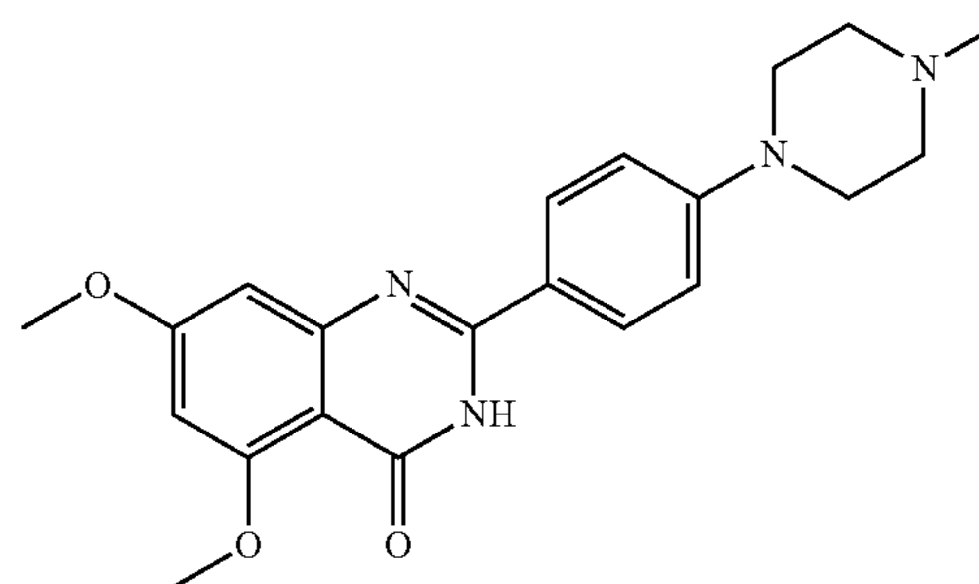
5,7-dimethoxy-2-(4-(4-methylpiperazin-1-yl)phenyl)quinazolin-4(3H)-one
