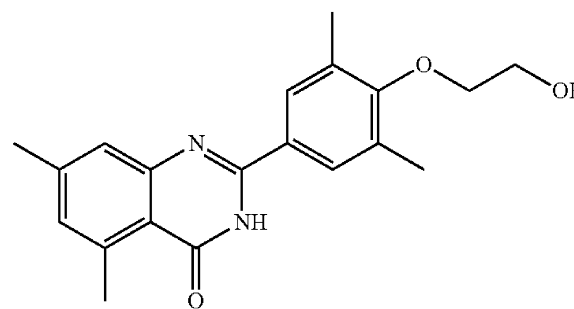
2-(4-(2-hydroxyethoxy)-3,5-dimethylphenyl)-5,7-dimethylquinazolin-4(3H)-one
