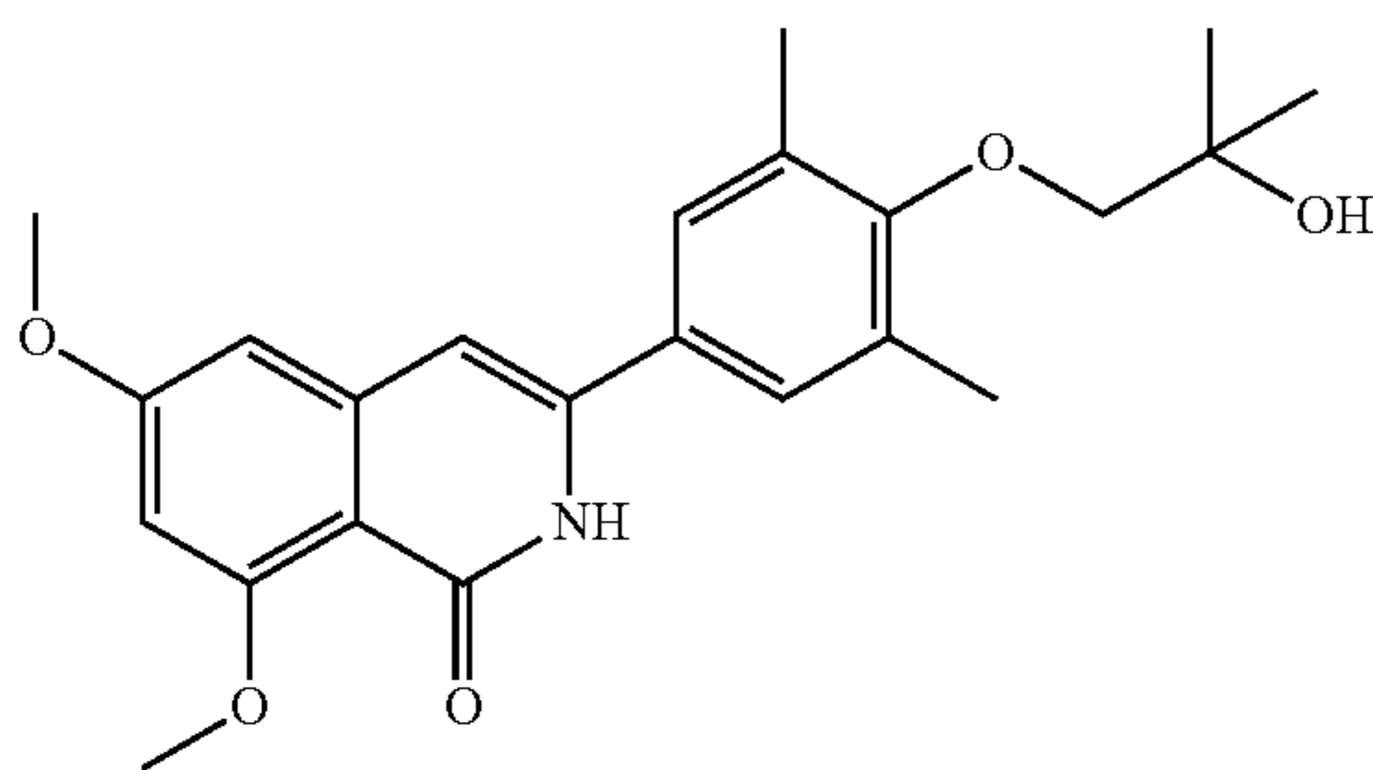
3-(4-(2-hydroxy-2-methylpropoxy)-3,5-dimethylphenyl)-6,8-dimethoxyisoquinolin-1(2H)-one
