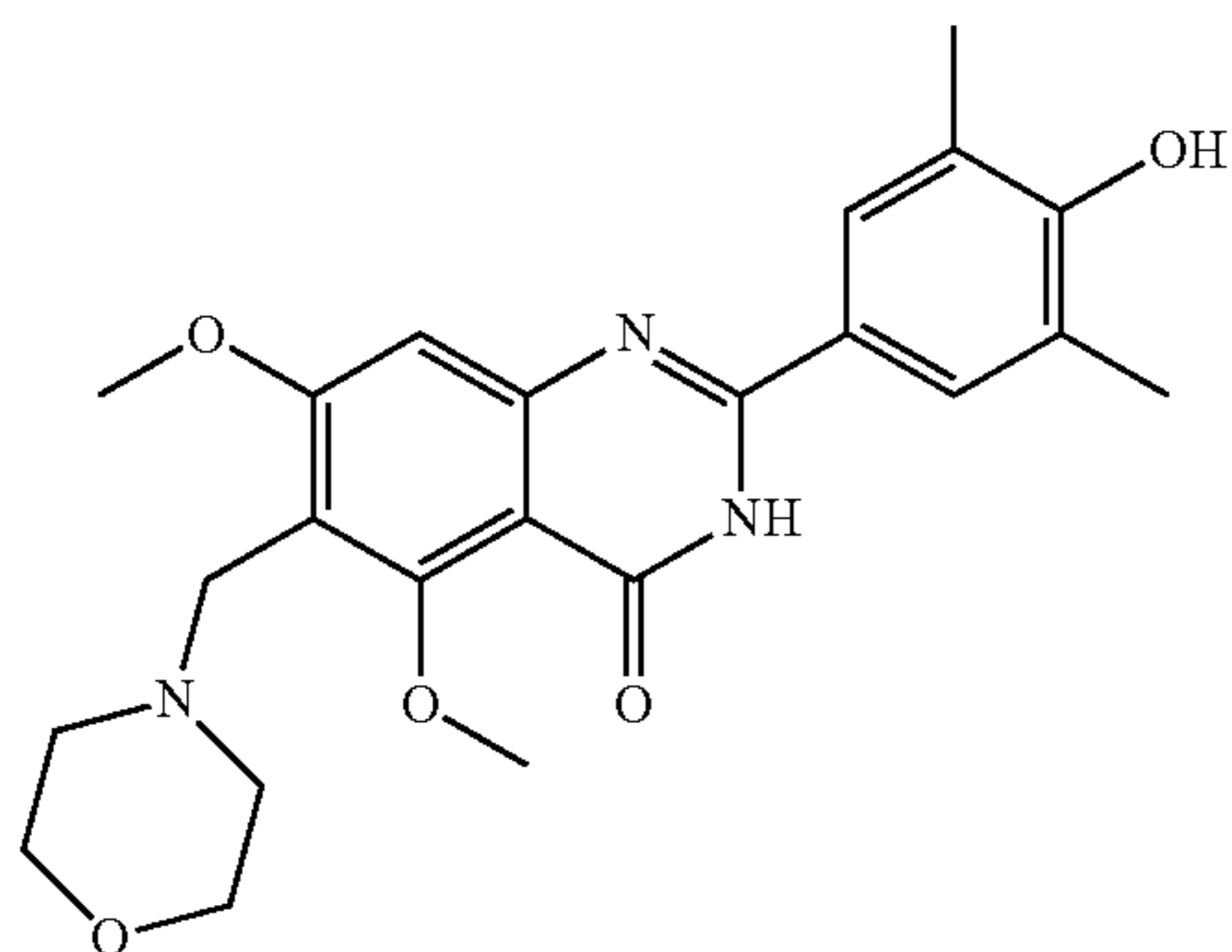
2-(4-hydroxy-3,5-dimethylphenyl)-5,7-dimethoxy-6-(morpholinomethyl)quinazolin-4(3H)-one
