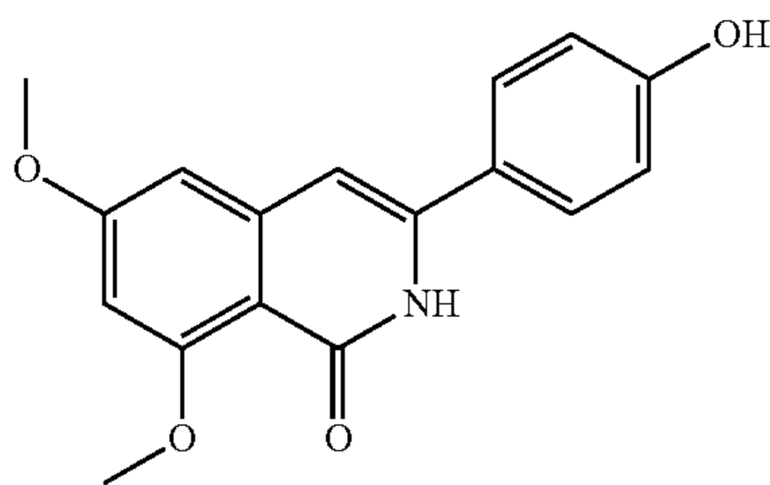
3-(4-hydroxyphenyl)-6,8-dimethoxyisoquinolin-1(2H)-one
