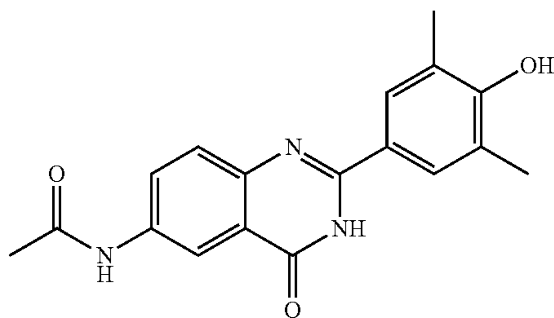
N-(2-(4-hydroxy-3,5-dimethylphenyl)-4-oxo-3,4-dihydroquinazolin-6-yl)acetamide
