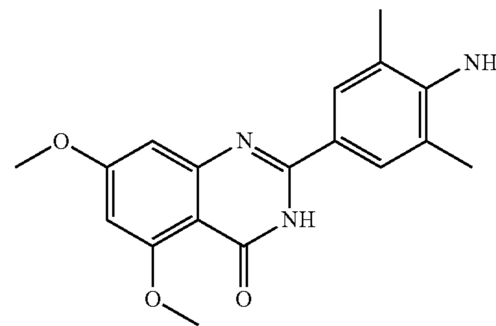
2-(4-amino-3,5-dimethylphenyl)-5,7-dimethoxyquinazolin-4(3H)-one
