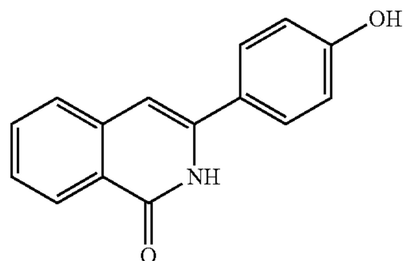
3-(4-Hydroxyphenyl)-2H-isoquinolin-1-one
