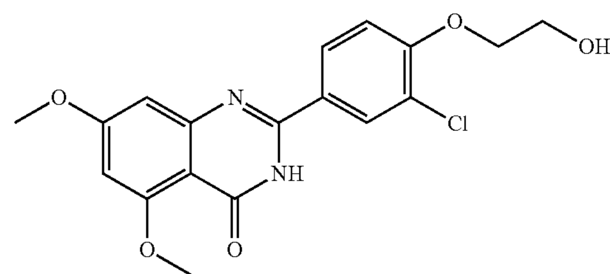
2-(3-chloro-4-(2-hydroxyethoxy)phenyl)-5,7-dimethoxyquinazolin-4(3H)-one
