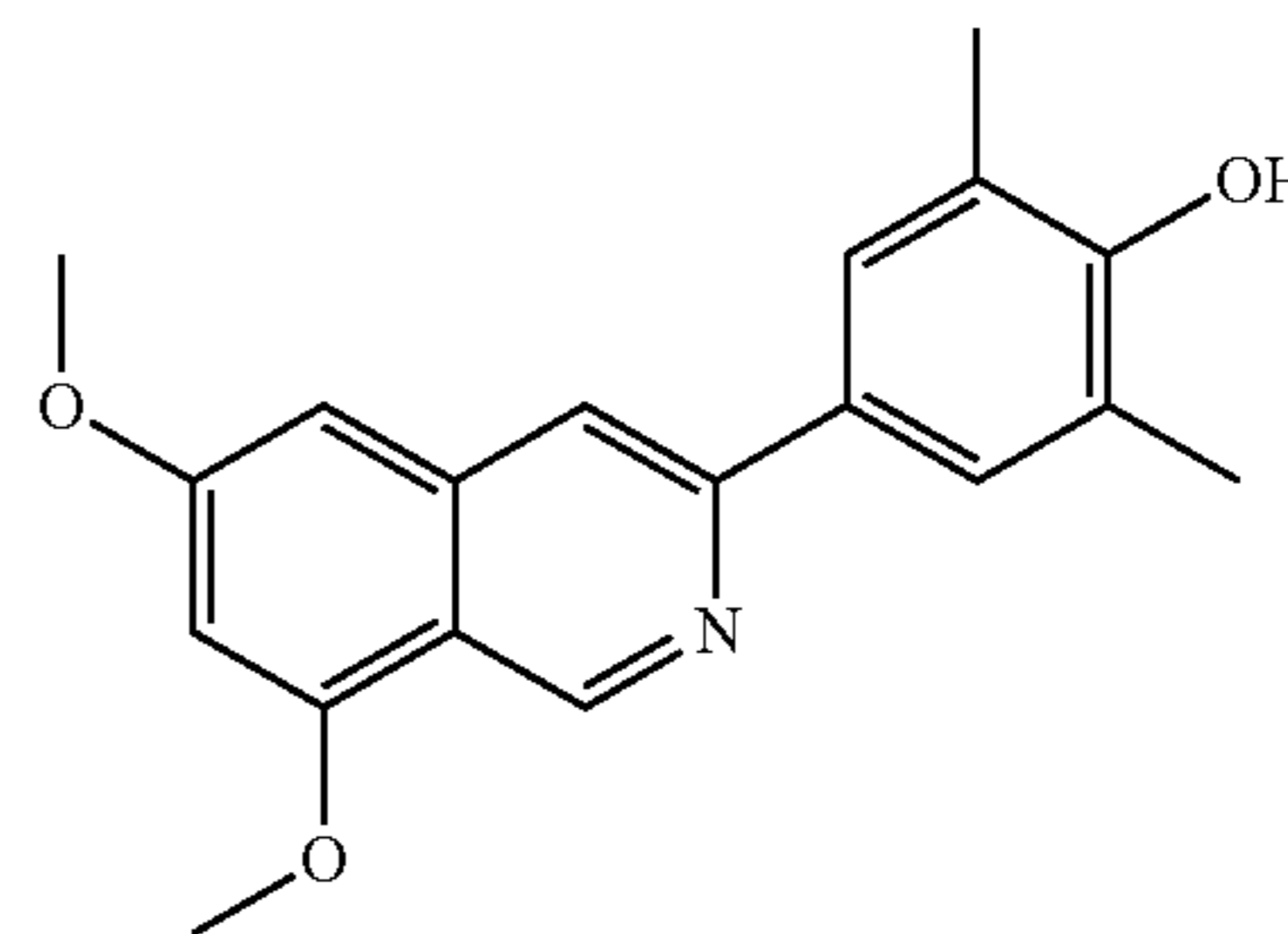
4-(6,8-dimethoxyisoquinolin-3-yl)-2,6-dimethylphenol
