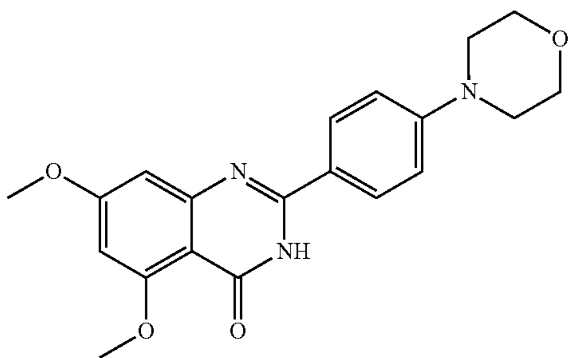
5,7-dimethoxy-2-(4-morpholinophenyl)quinazolin-4(3H)-one
