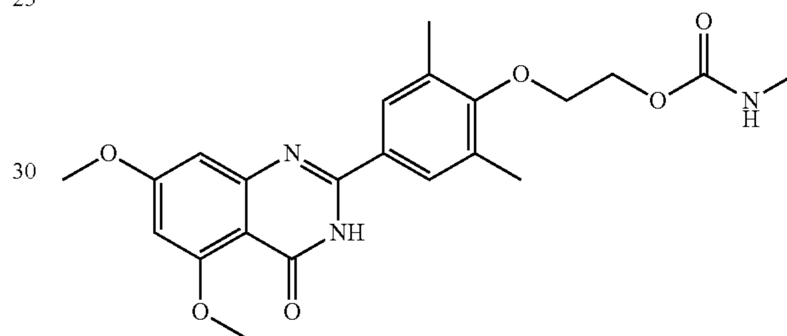
2-(4-(5,7-Dimethoxy-4-oxo-3,4-dihydroquinazolin-2-yl)-2,6-dimethyl-phenoxy)ethyl methylcarbamate
