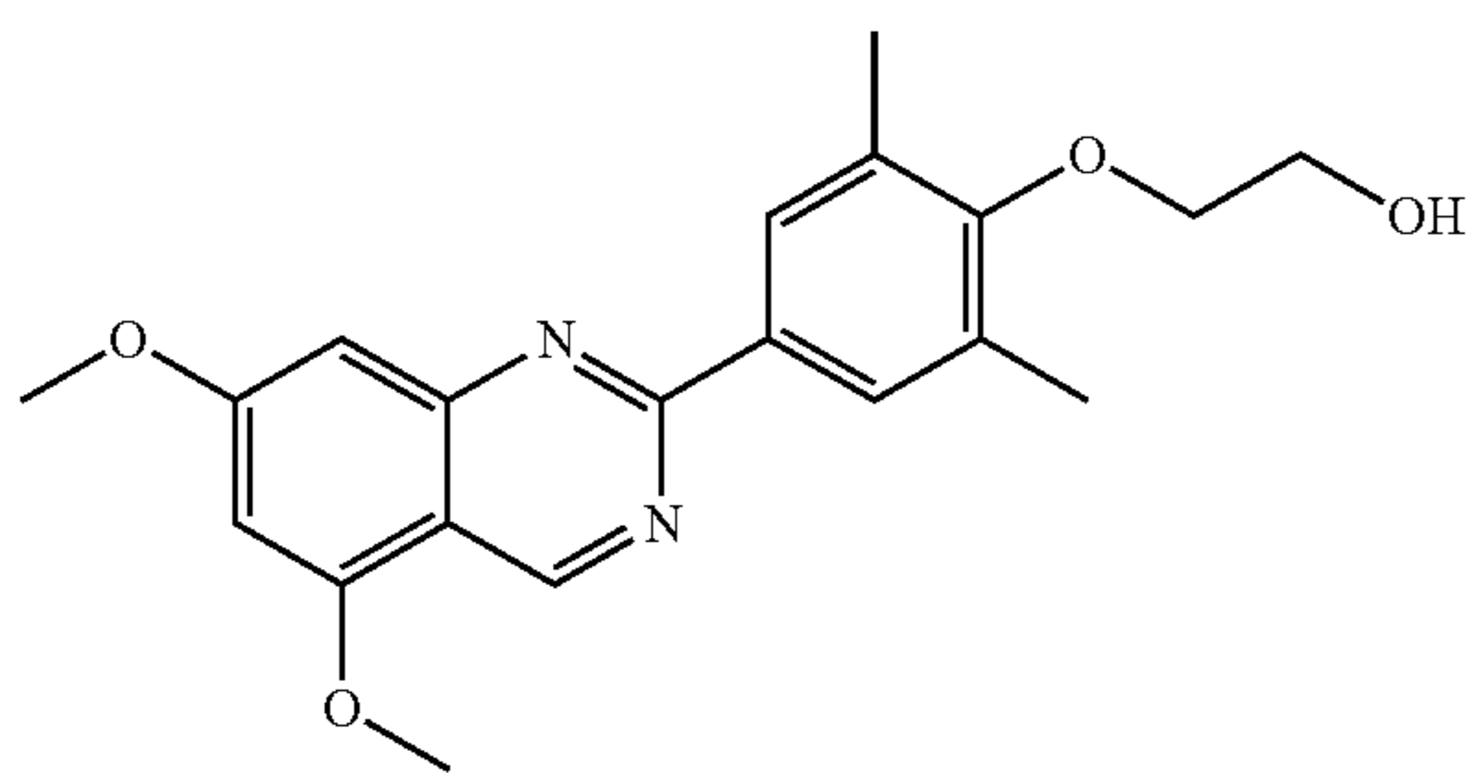
2-(4-(5,7-dimethoxyquinazolin-2-yl)-2,6-dimethylphenoxy)ethanol
