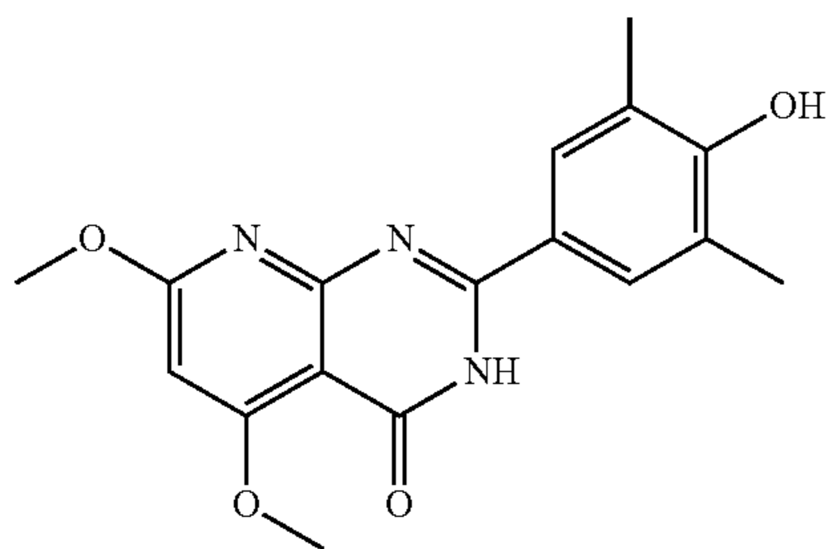
2-(4-hydroxy-3,5-dimethylphenyl)-5,7-dimethoxy-pyrido[2,3-d]pyrimidin-4(3H)-one
