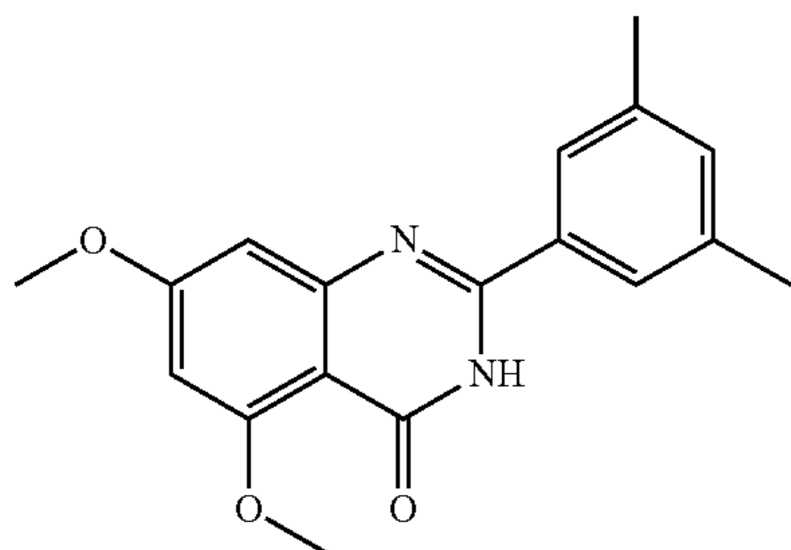
2-(3,5-dimethylphenyl)-5,7-dimethoxyquinazolin-4(3H)-one
