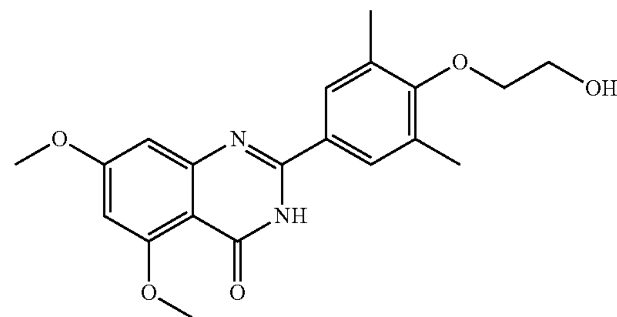
2-(4-(2-hydroxyethoxy)-3,5-dimethylphenyl)-5,7-dimethoxyquinazolin-4(3H)-one
