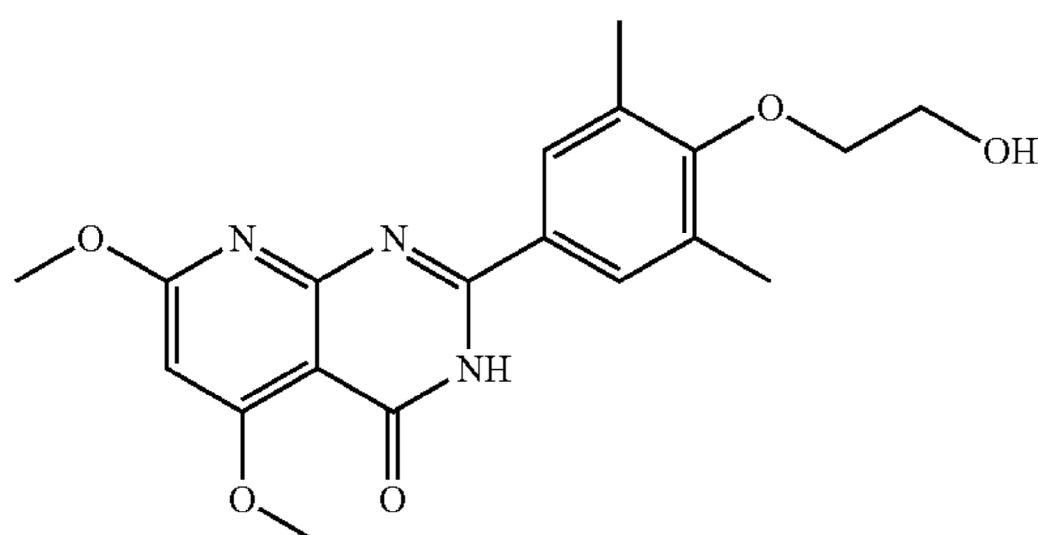
2-(4-(2-hydroxyethoxy)-3,5-dimethylphenyl)-5,7-dimethoxy-1-methylquinazolin-4(1H)-one
