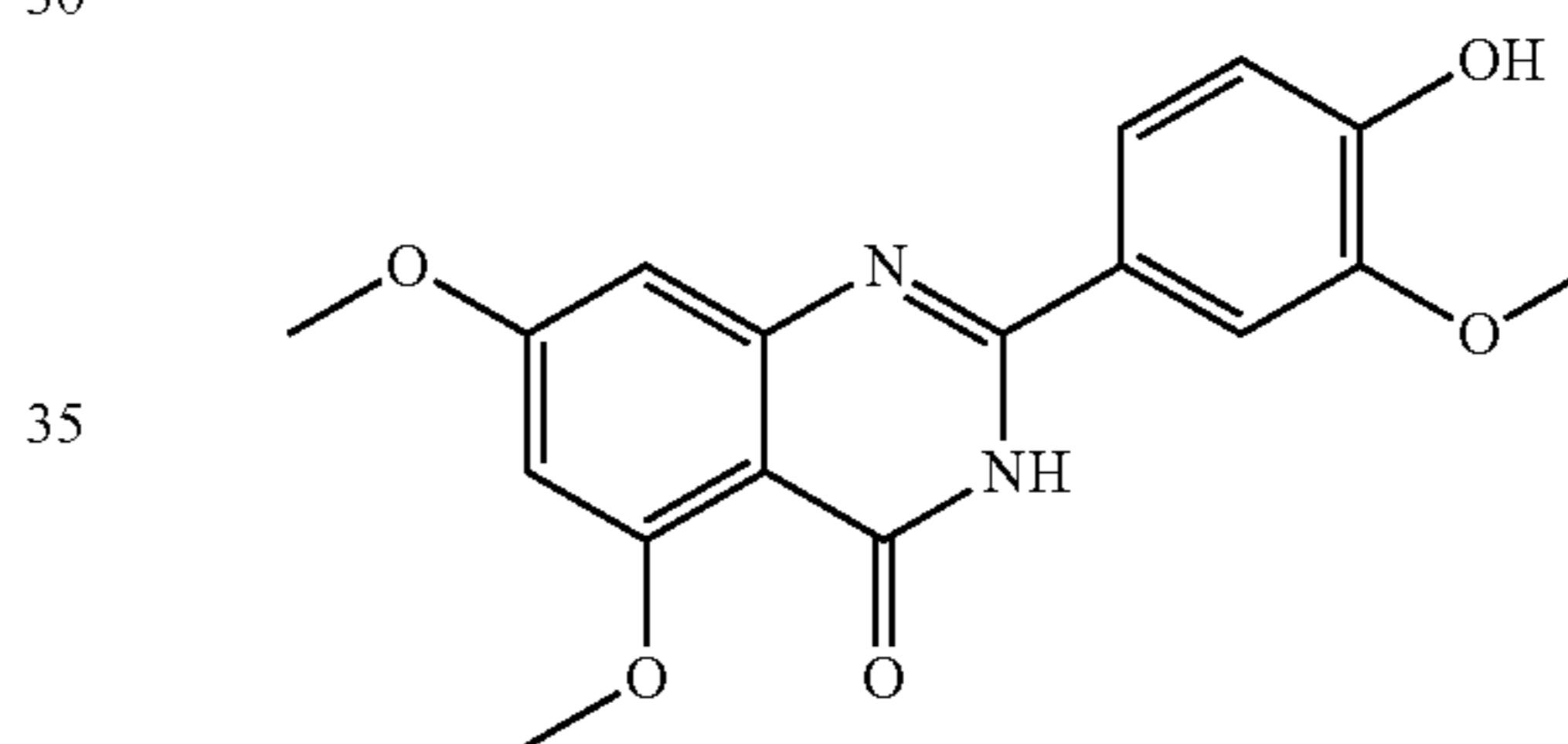
2-(4-hydroxy-3-methoxyphenyl)-5,7-dimethoxyquinazolin-4(3H)-one
