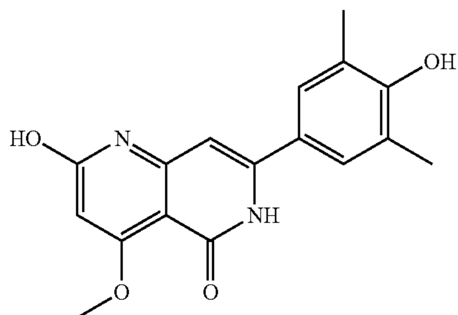
2-hydroxy-7-(4-hydroxy-3,5-dimethylphenyl)-4-methoxy-1,6-naphthyridin-5(6H)-one
