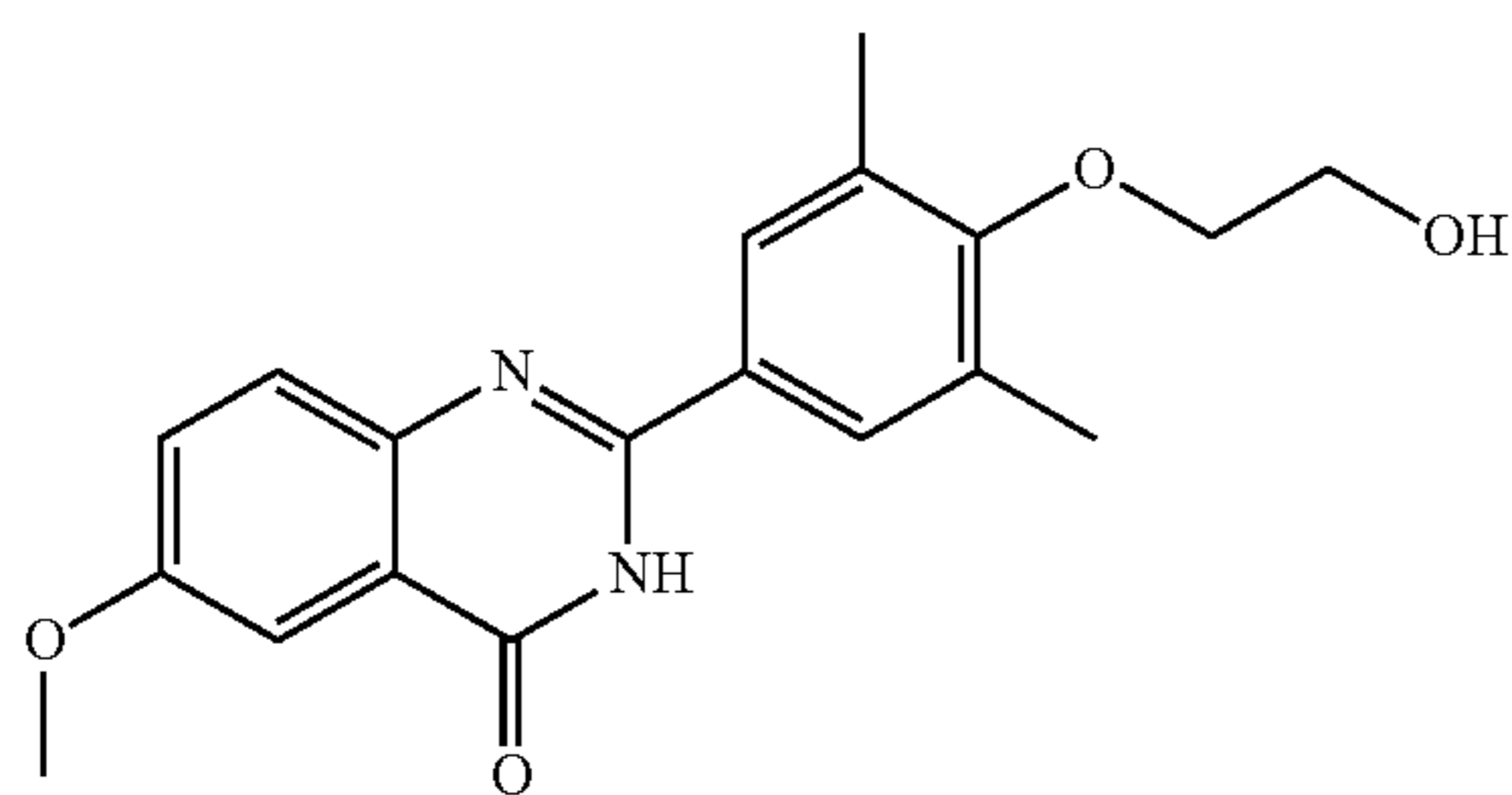
2-(4-(2-hydroxyethoxy)-3,5-dimethylphenyl)-6-methoxyquinazolin-4(3H)-one
