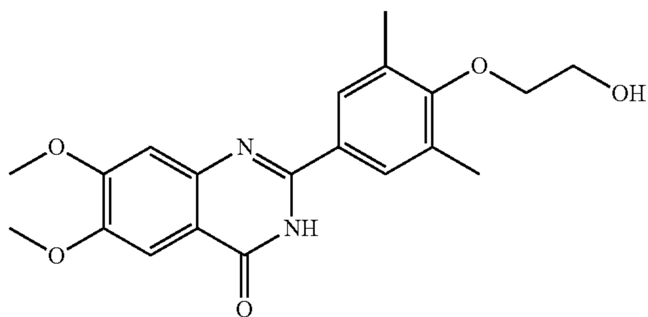
2-(4-(2-hydroxyethoxy)-3,5-dimethylphenyl)-6,7-dimethoxyquinazolin-4(3H)-one
