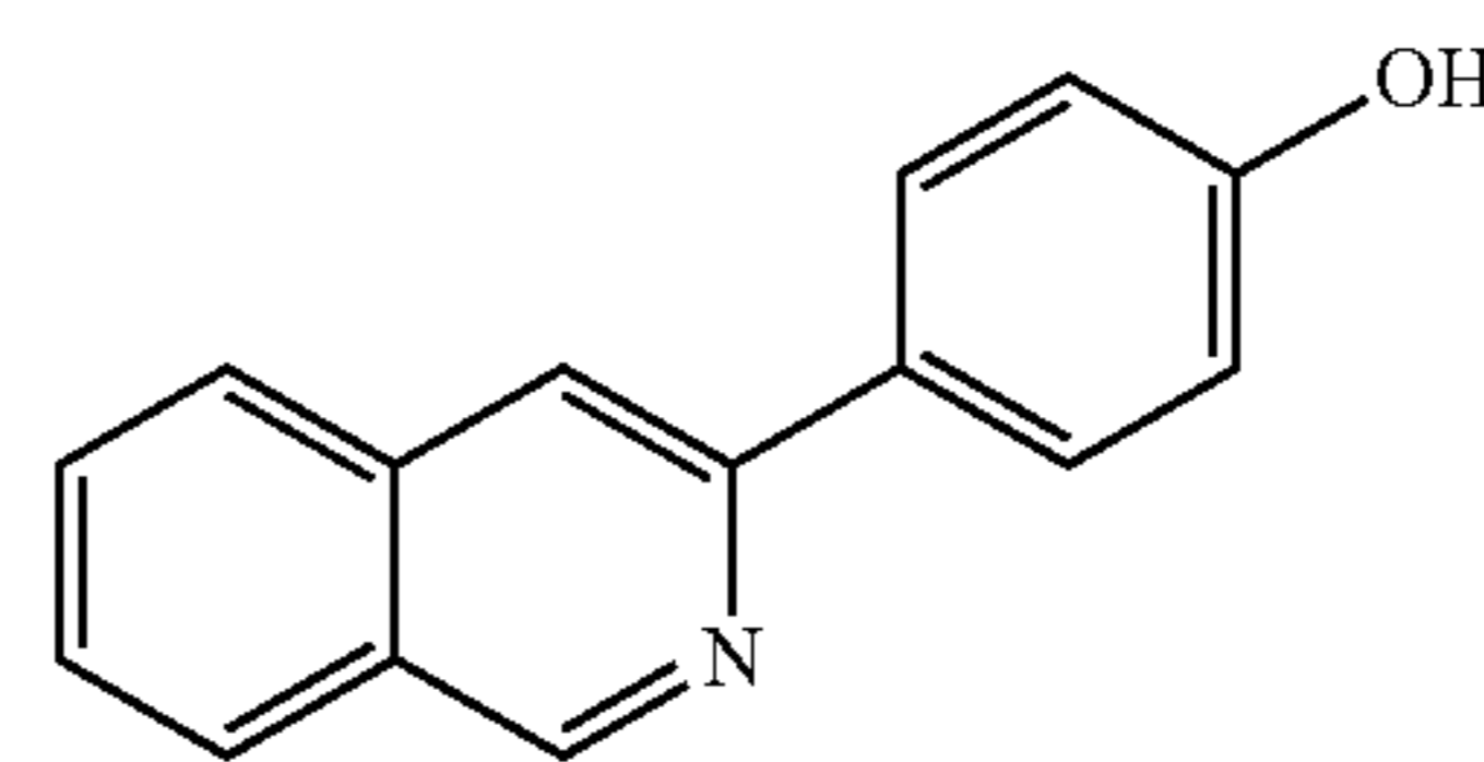
4-Isoquinolin-3-yl-phenol
