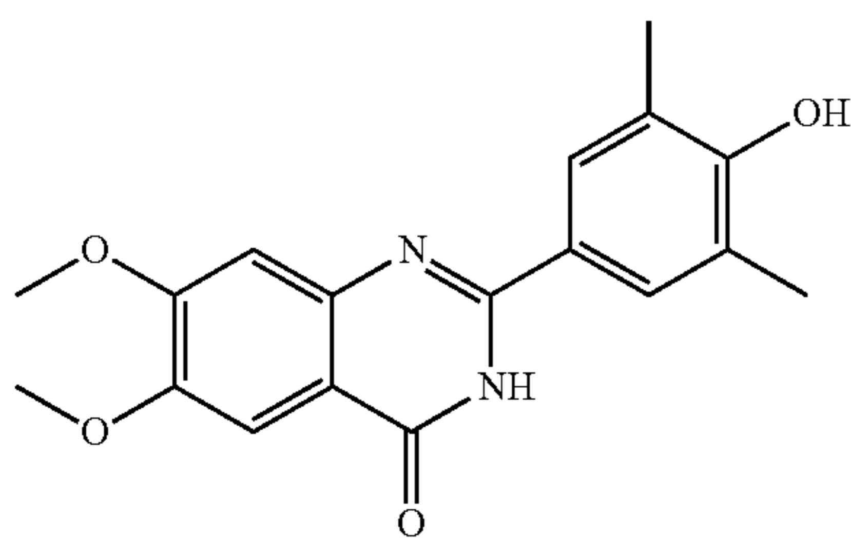
2-(4-hydroxy-3,5-dimethylphenyl)-6,7-dimethoxyquinazolin-4(3H)-one
