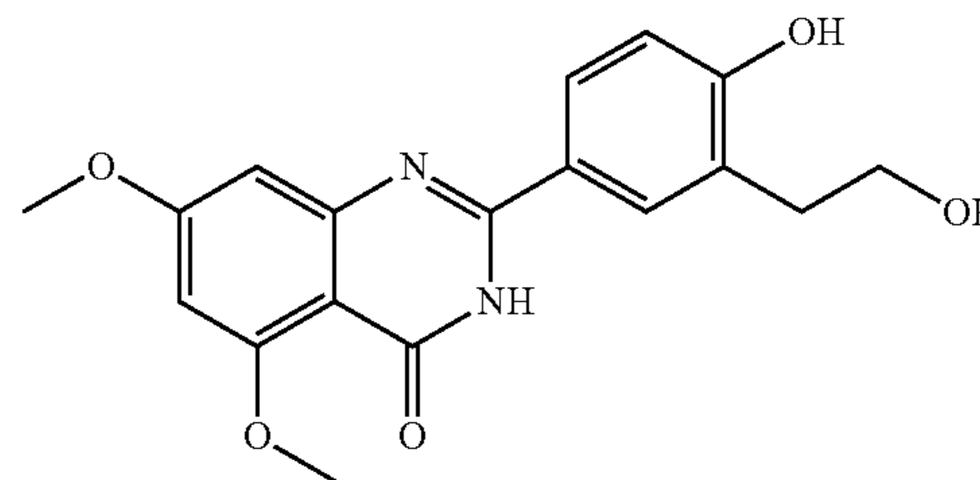
2-(4-hydroxy-3-(2-hydroxyethyl)phenyl)-5,7-dimethoxyquinazolin-4(3H)-one
