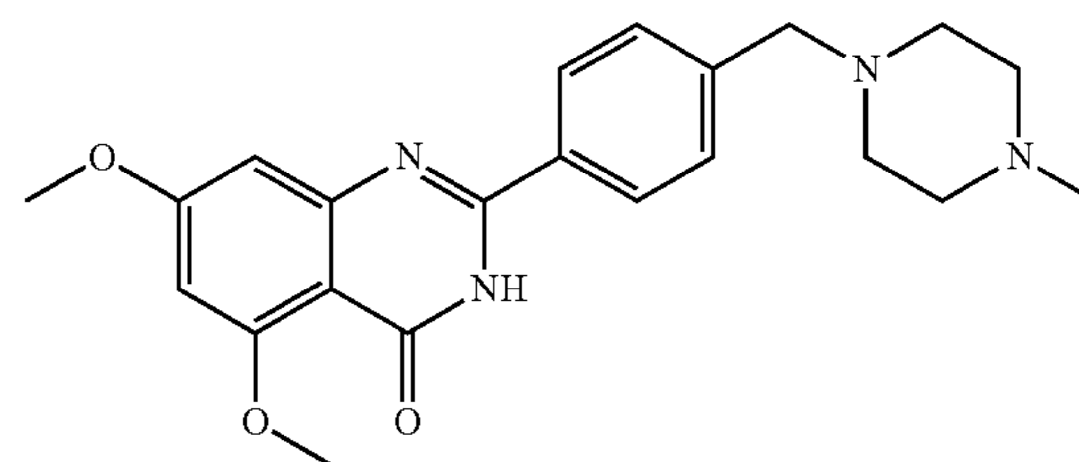
5,7-dimethoxy-2-((4-methylpiperazin-1-yl)methyl)phenylquinazolin-4(3H)-one
