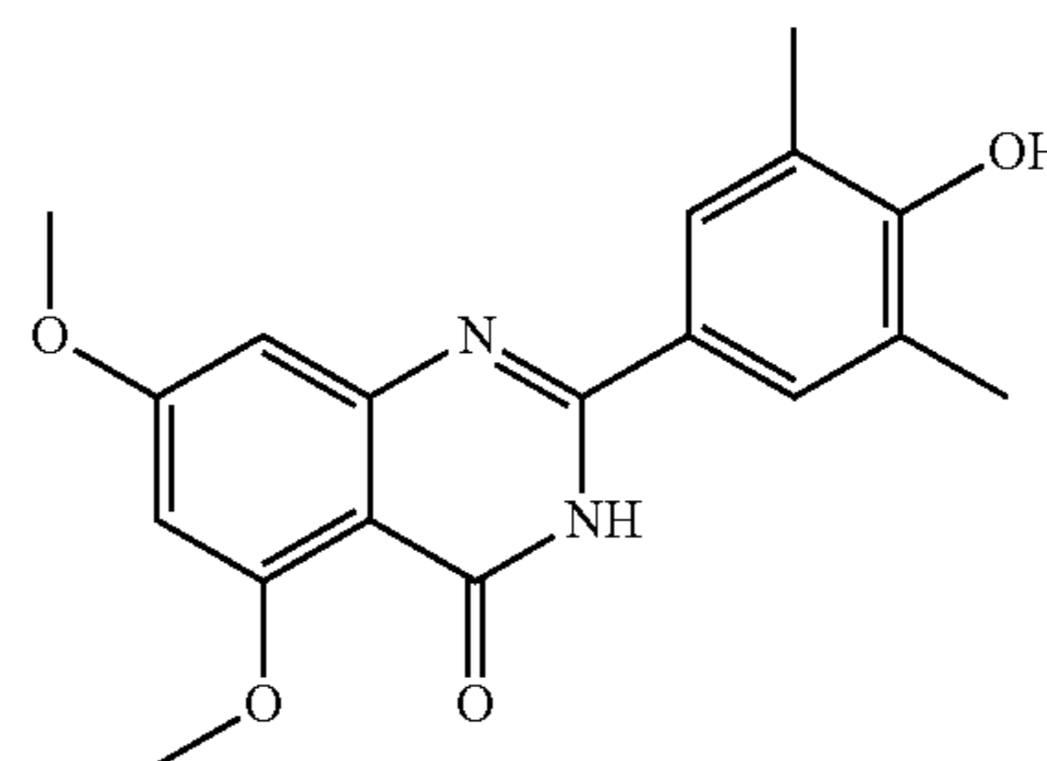
2-(4-hydroxy-3,5-dimethylphenyl)-5,7-dimethoxyquinazolin-4(3H)-one
