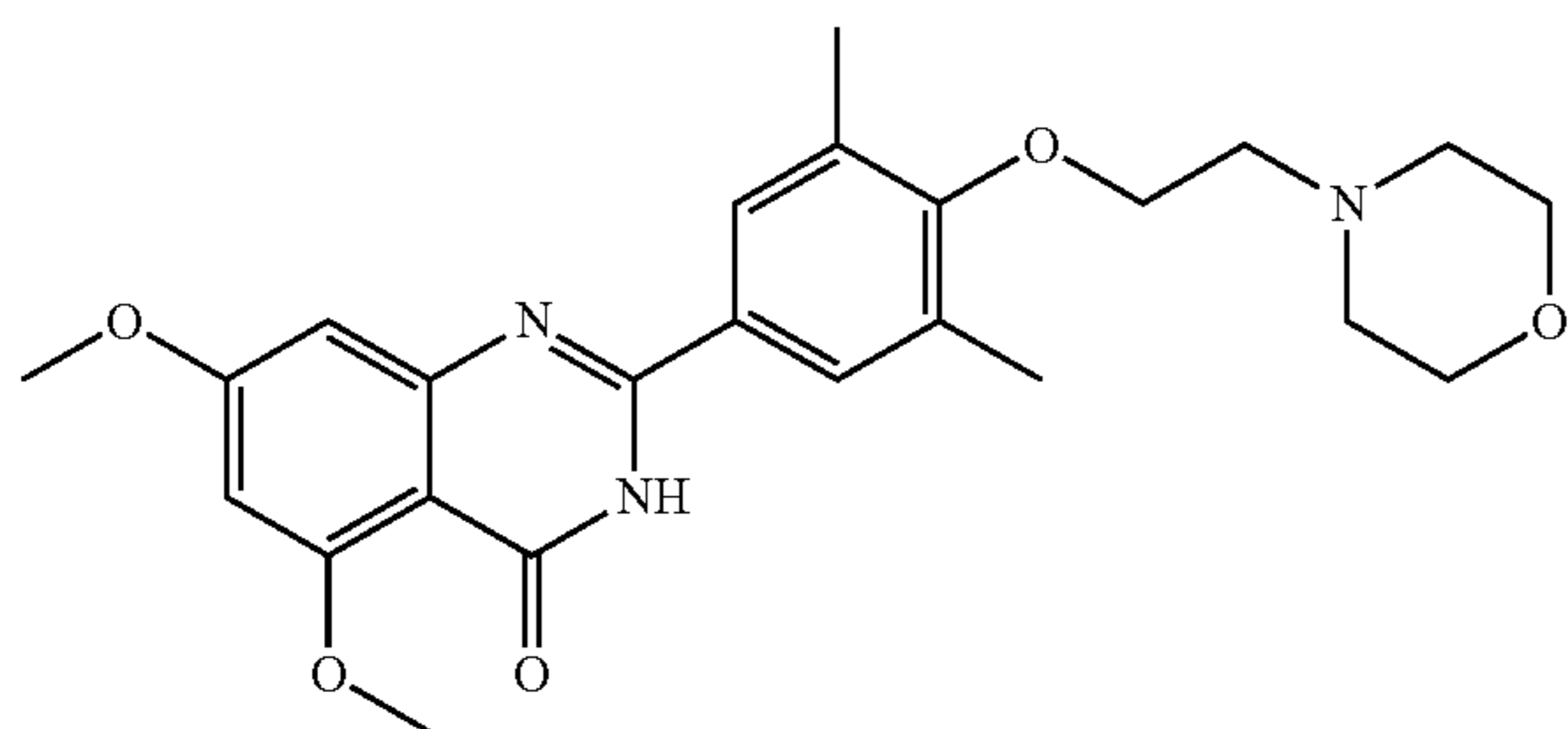
2-(3,5-dimethyl-4-(2-morpholinoethoxy)phenyl)-5,7-dimethoxyquinazolin-4(3H)-one
