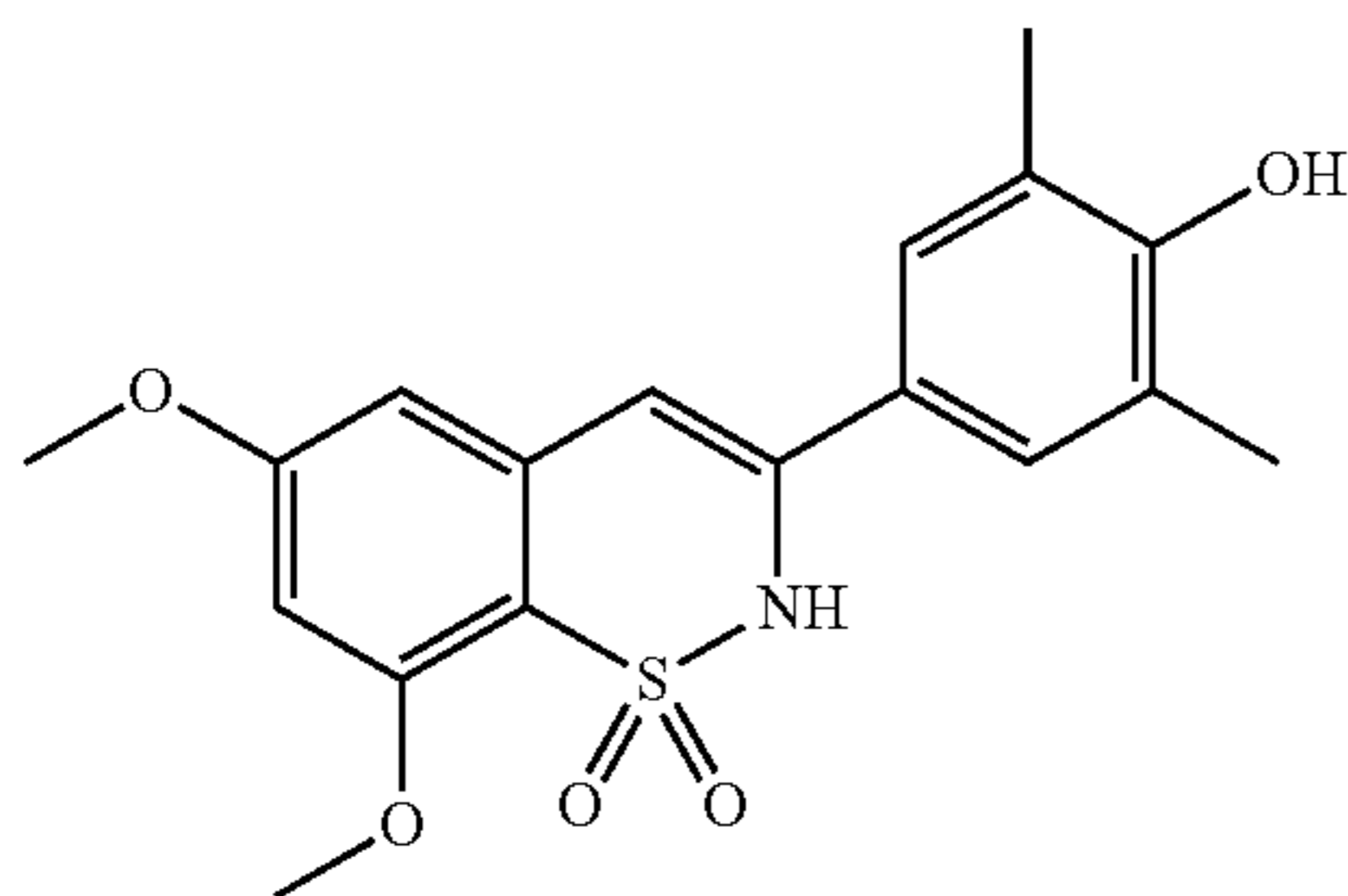
6,8-dimethoxy-3-(4-hydroxy-3,5-dimethylphenyl)- 2H-1,2-benzothiazine-1,1-dioxide
