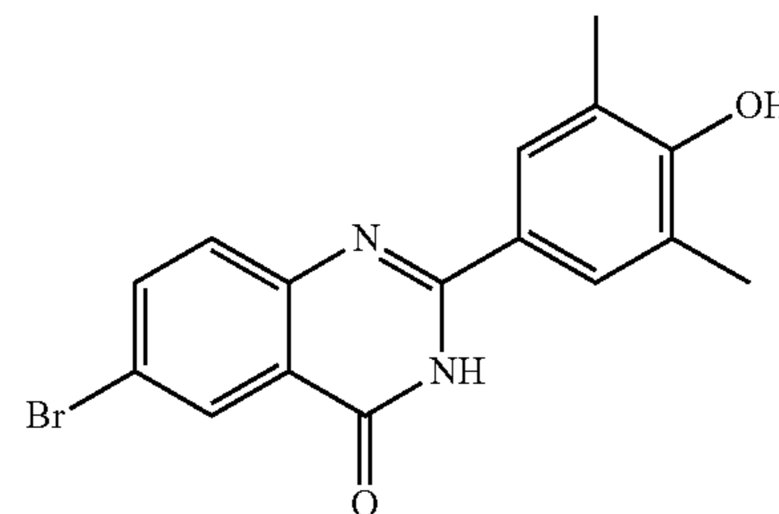
6-bromo-2-(4-hydroxy-3,5-dimethylphenyl)quinazolin-4(3H)-one
