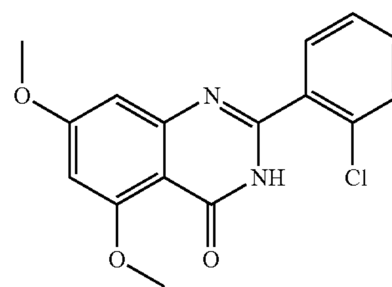
2-(2-chlorophenyl)-5,7-dimethoxyquinazolin-4(3H)-one
