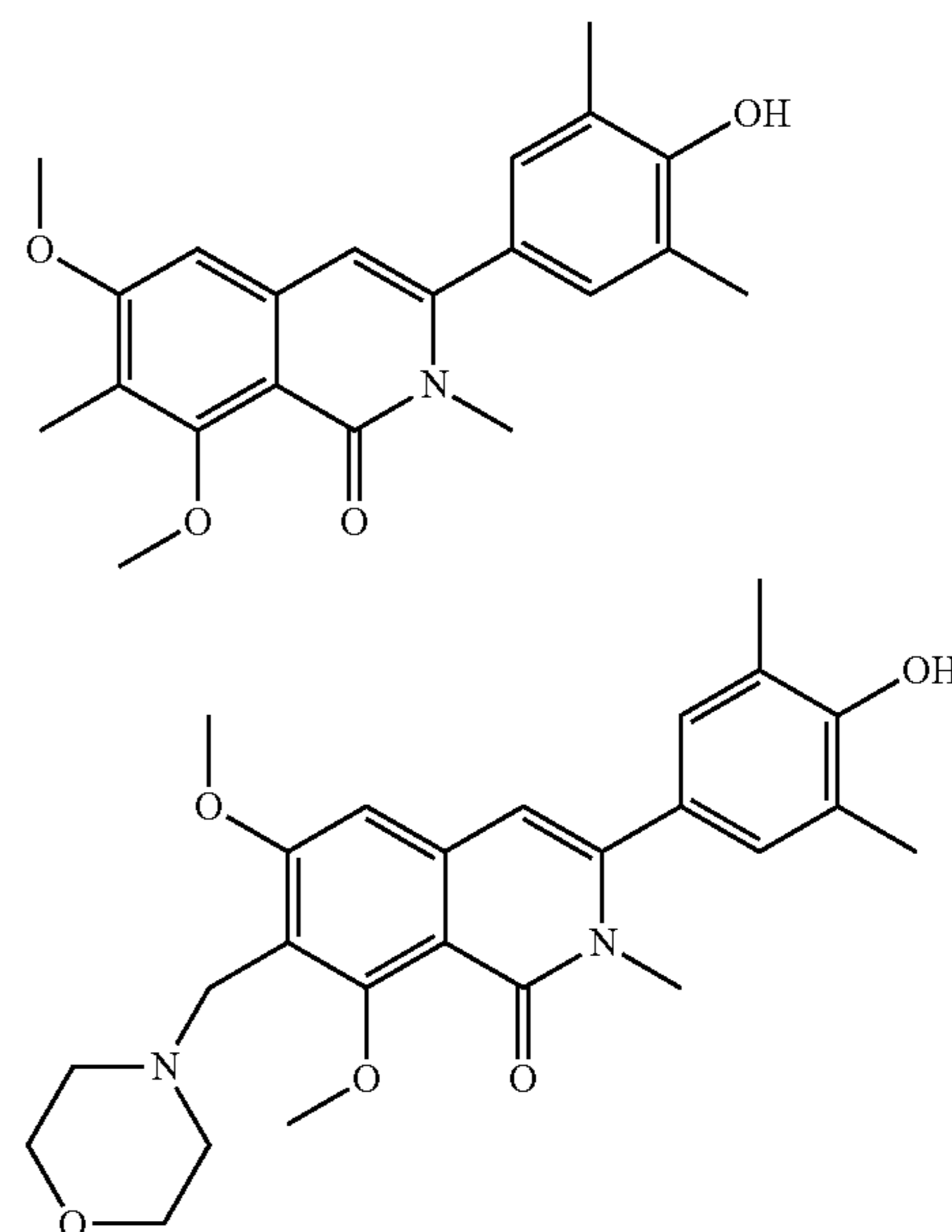
3-(4-hydroxy-3,5-dimethylphenyl)-6,8-dimethoxy-2,7-dimethylisoquinolin-1(2H)-one (left) and
