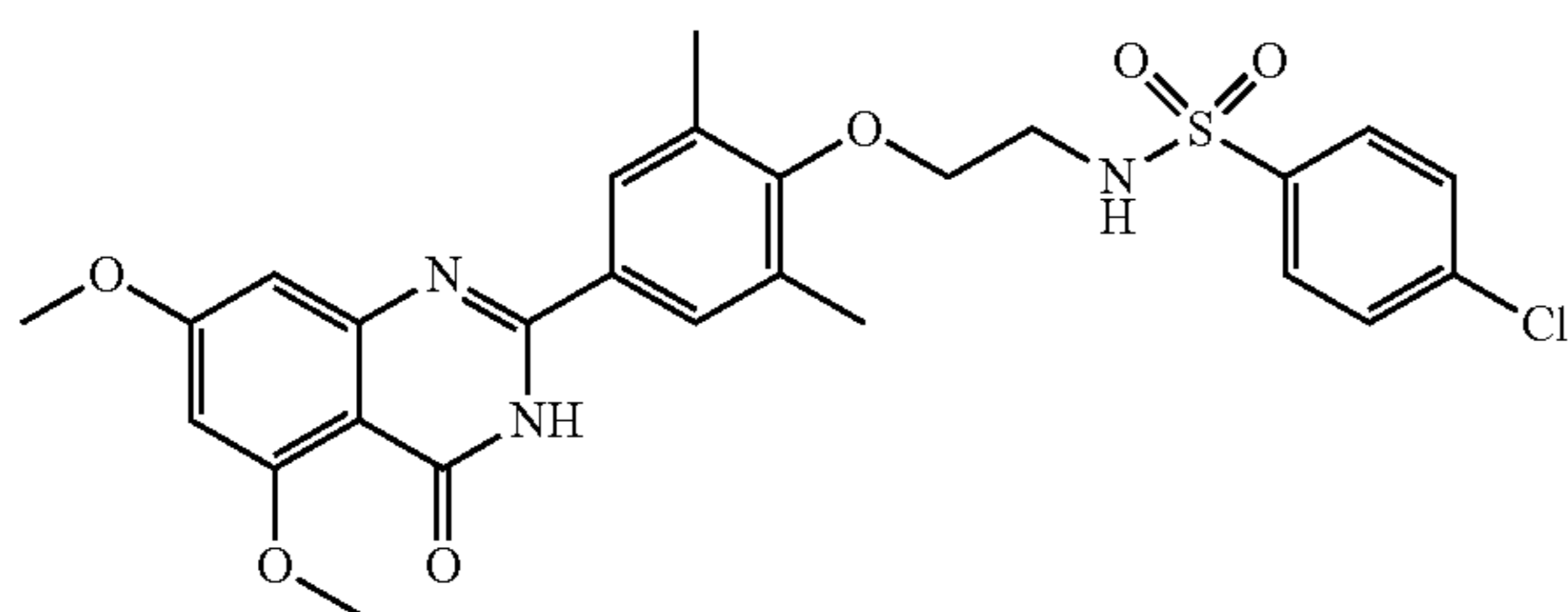
4-chloro-N-(2-(4-(5,7-dimethoxy-4-oxo-3,4-dihydroquinazolin-2-yl))-2,6-dimethylphenoxy)ethyl)benzenesulfonamide
