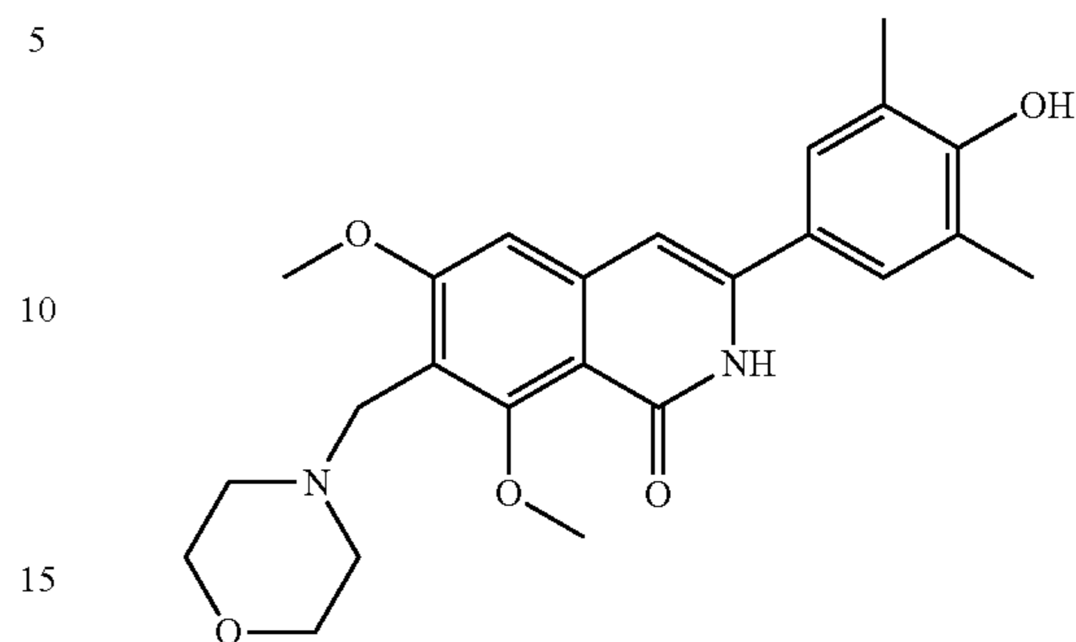
3-(4-hydroxy-3,5-dimethylphenyl)-6,8-dimethoxy-7-(morpholinomethyl)isoquinolin-1(2H)-one
