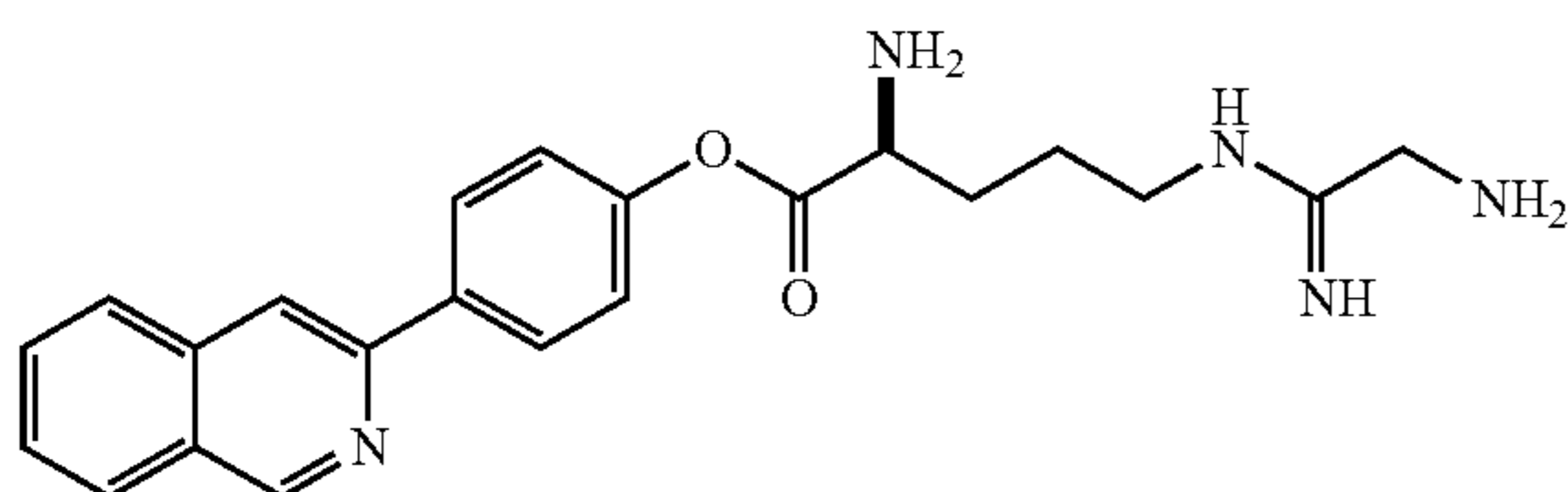
4-(isoquinolin-3-yl)phenyl 2-amino-5-guanidinopentanoate tetrahydrochloride
