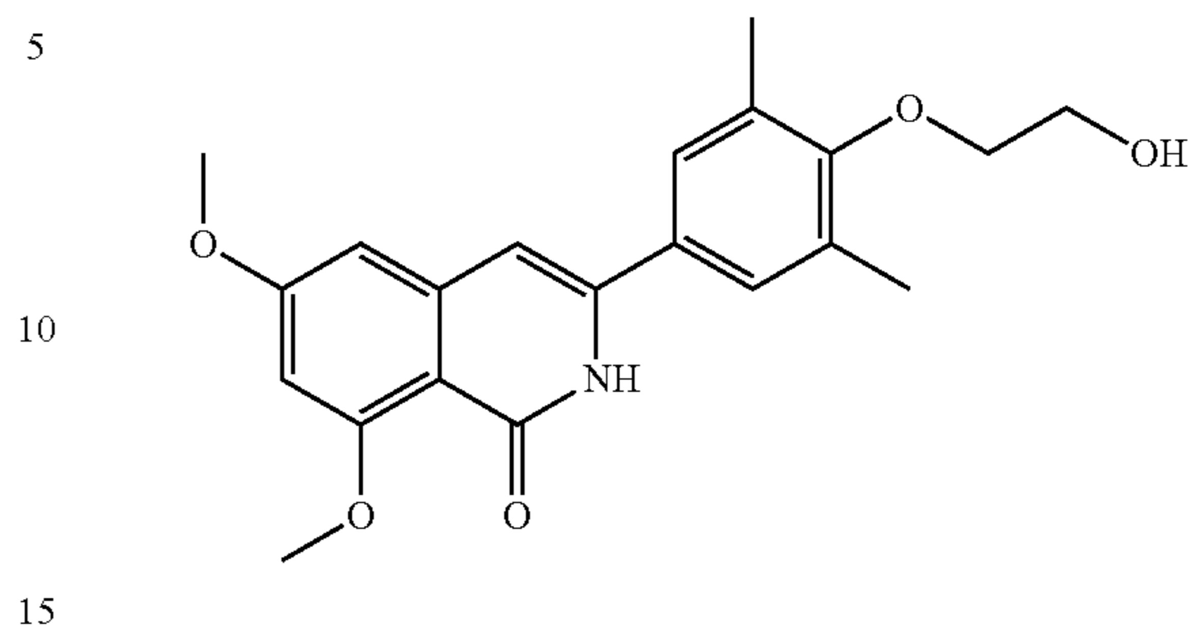
3-(4-(2-hydroxyethoxy)-3,5-dimethylphenyl)-6,8-dimethoxyisoquinolin-1(2H)-one
