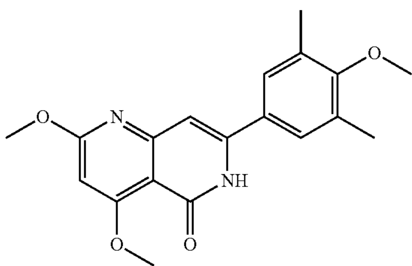
2,4-dimethoxy-7-(4-methoxy-3,5-dimethylphenyl)-1,6-naphthyridin-5(6H)-one
