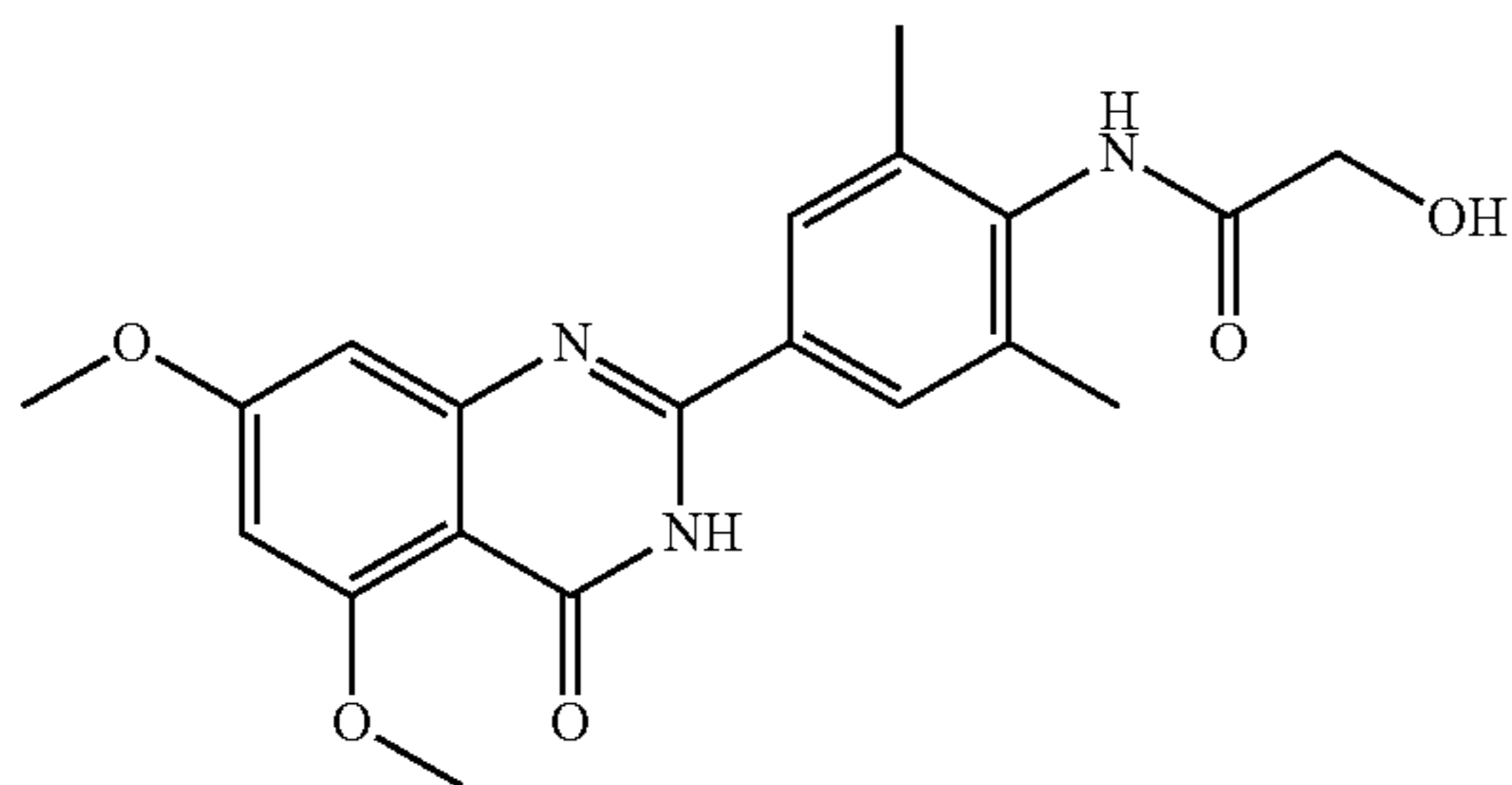
N-(4-(5,7-dimethoxy-4-oxo-3,4-dihydroquinazolin-2-yl)-2,6-dimethylphenyl)-2-hydroxyacetamide
