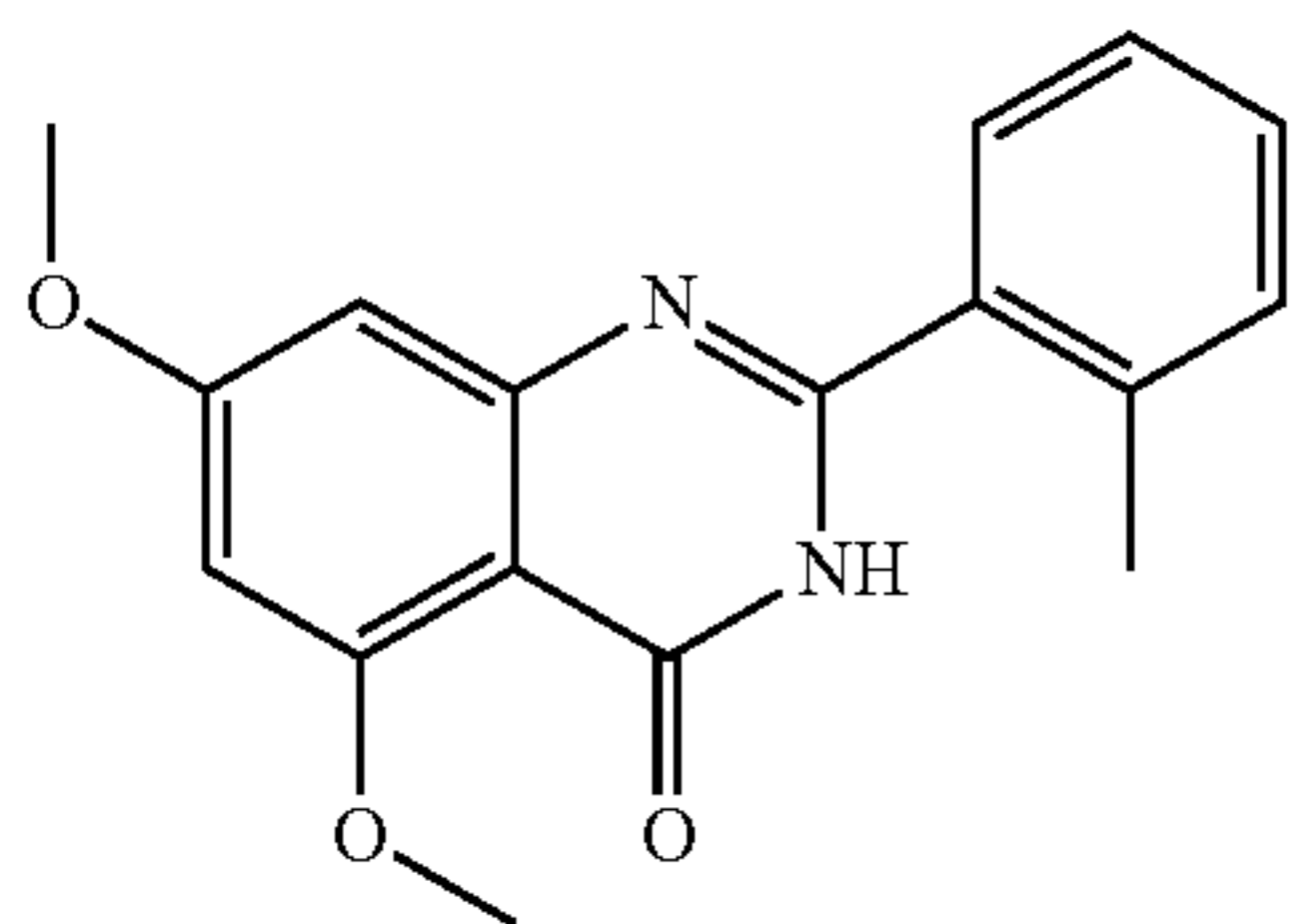
5,7-dimethoxy-2-o-tolylquinazolin-4(3H)-one
