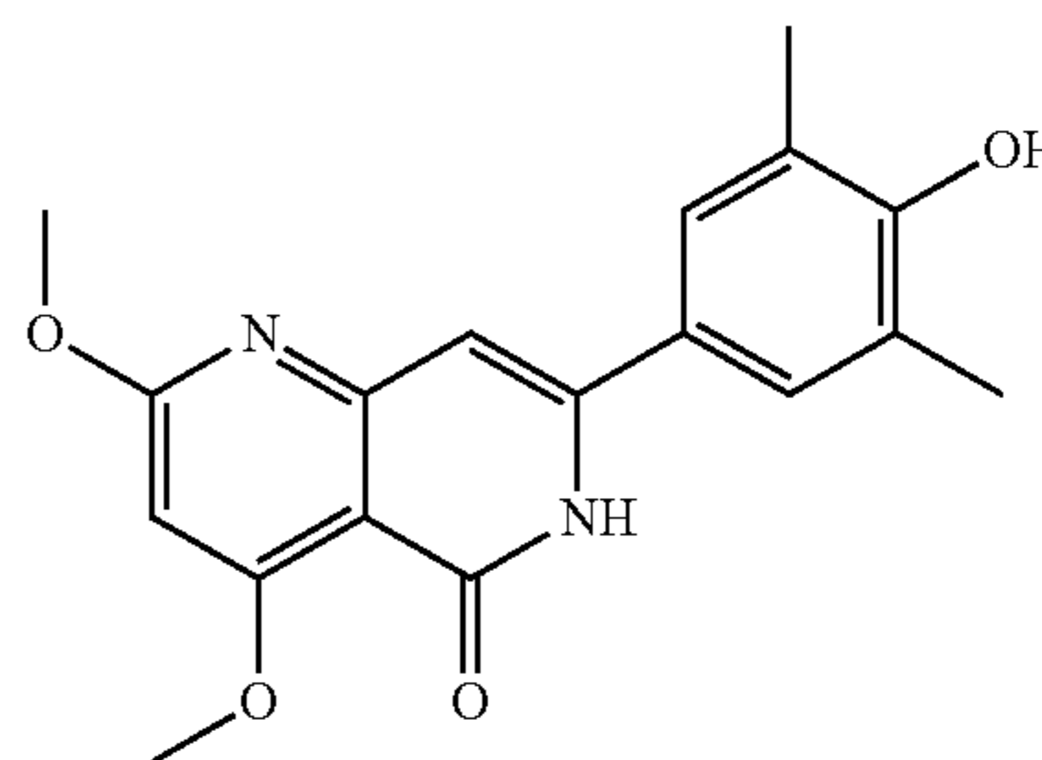
7-(4-hydroxy-3,5-dimethylphenyl)-2,4-dimethoxy-1, 6-naphthyridin-5(6H)-one
