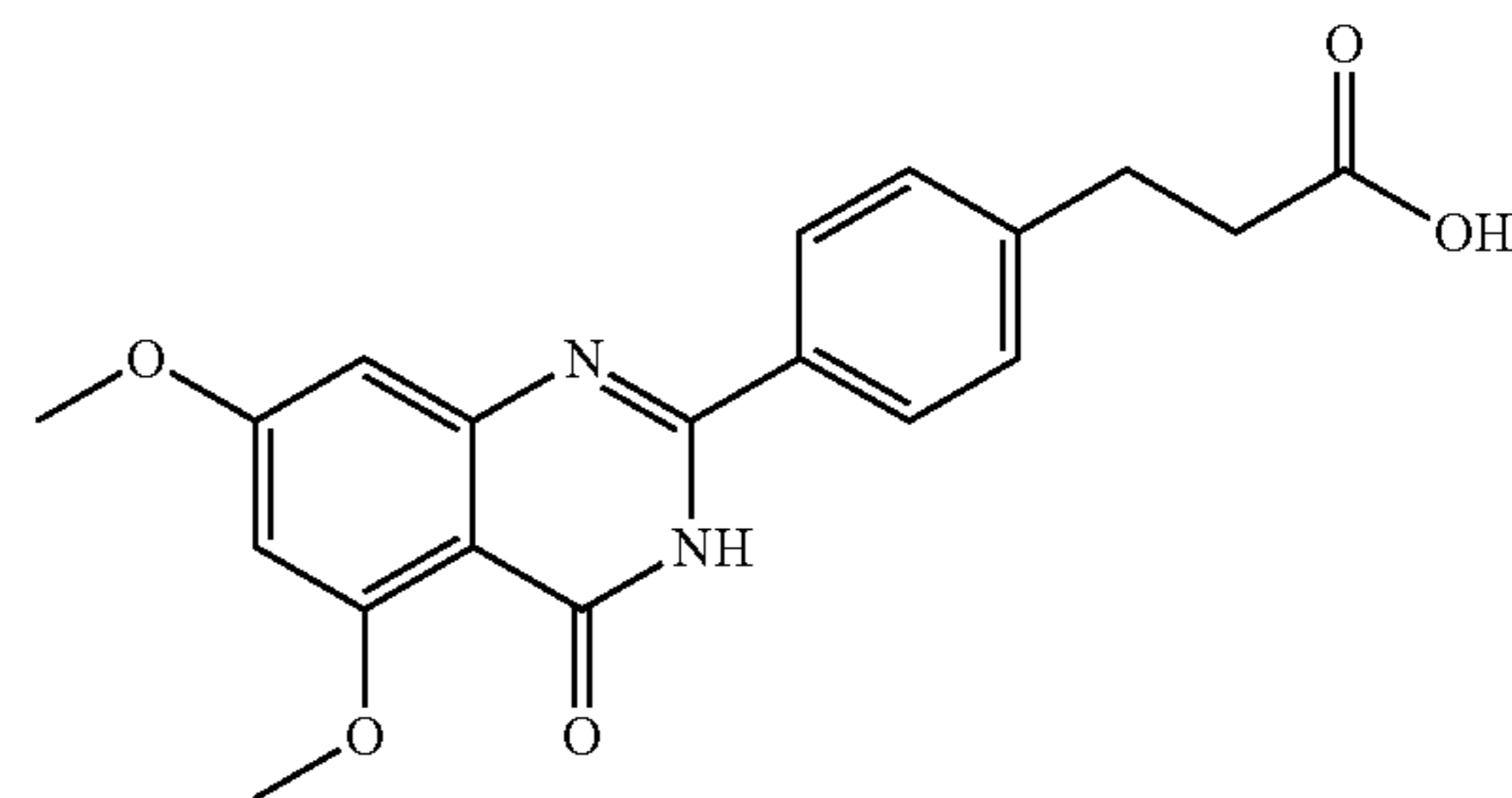
3-(4-(5,7-dimethoxy-4-oxo-3,4-dihydroquinazolin-2-yl)phenyl)propanoic acid
