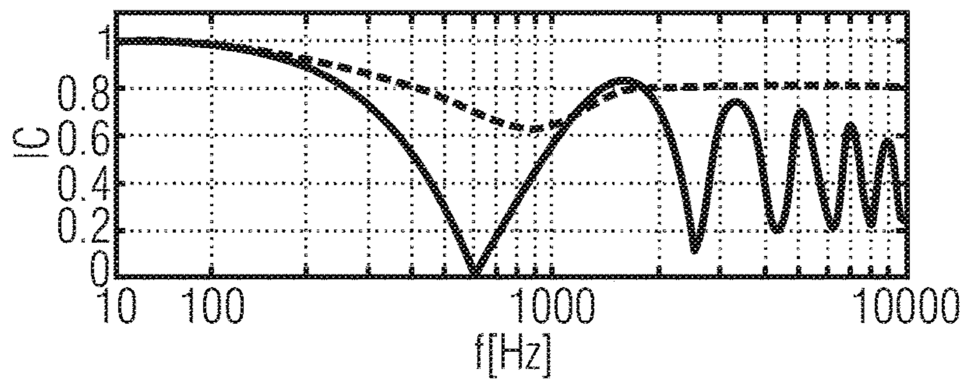
IC(f_0) for two sound sources at azimuth \pm 30^\circ , with head orientation 0^\circ
